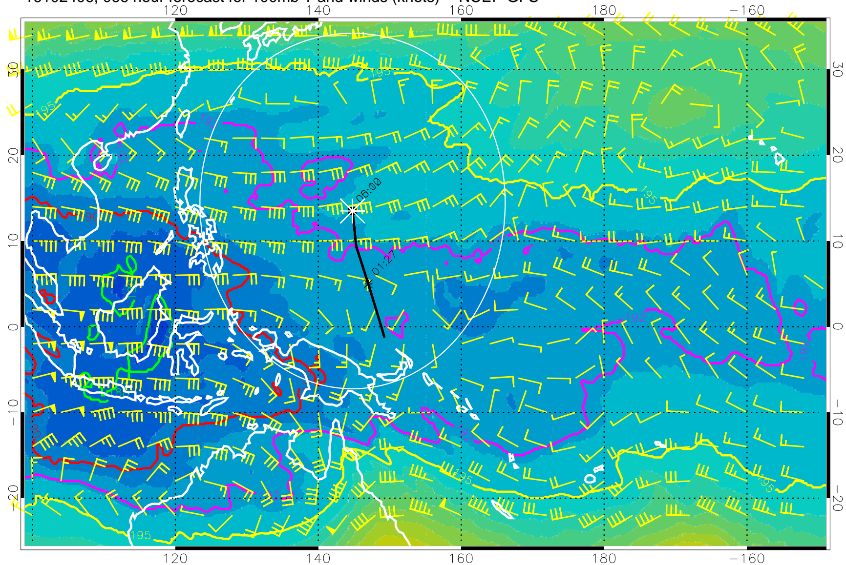
16102406, 066 hour forecast for 100mb T and winds (knots) -- NCEP GFS
