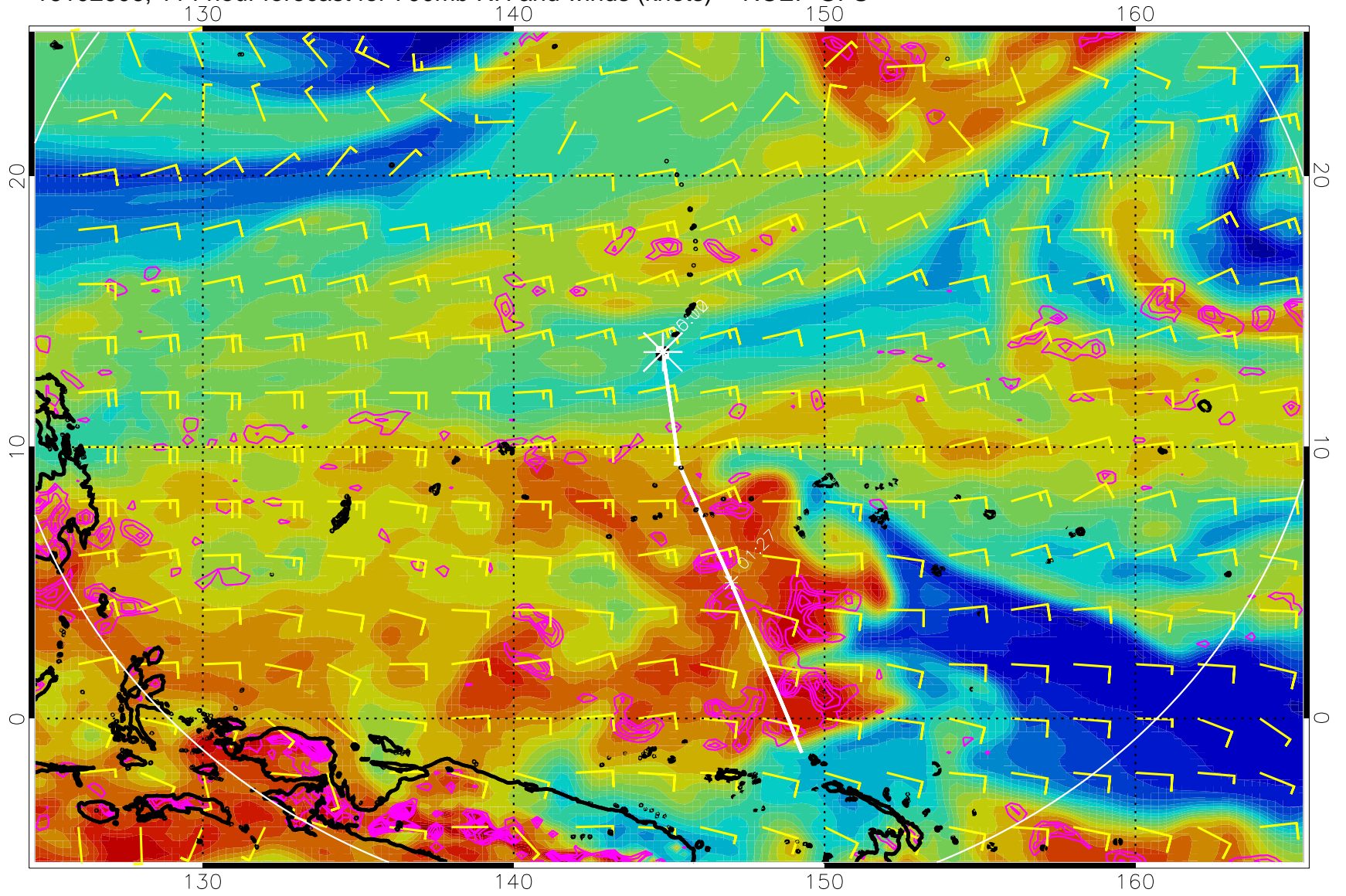
16102606, 114 hour forecast for 700mb RH and winds (knots) -- NCEP GFS
