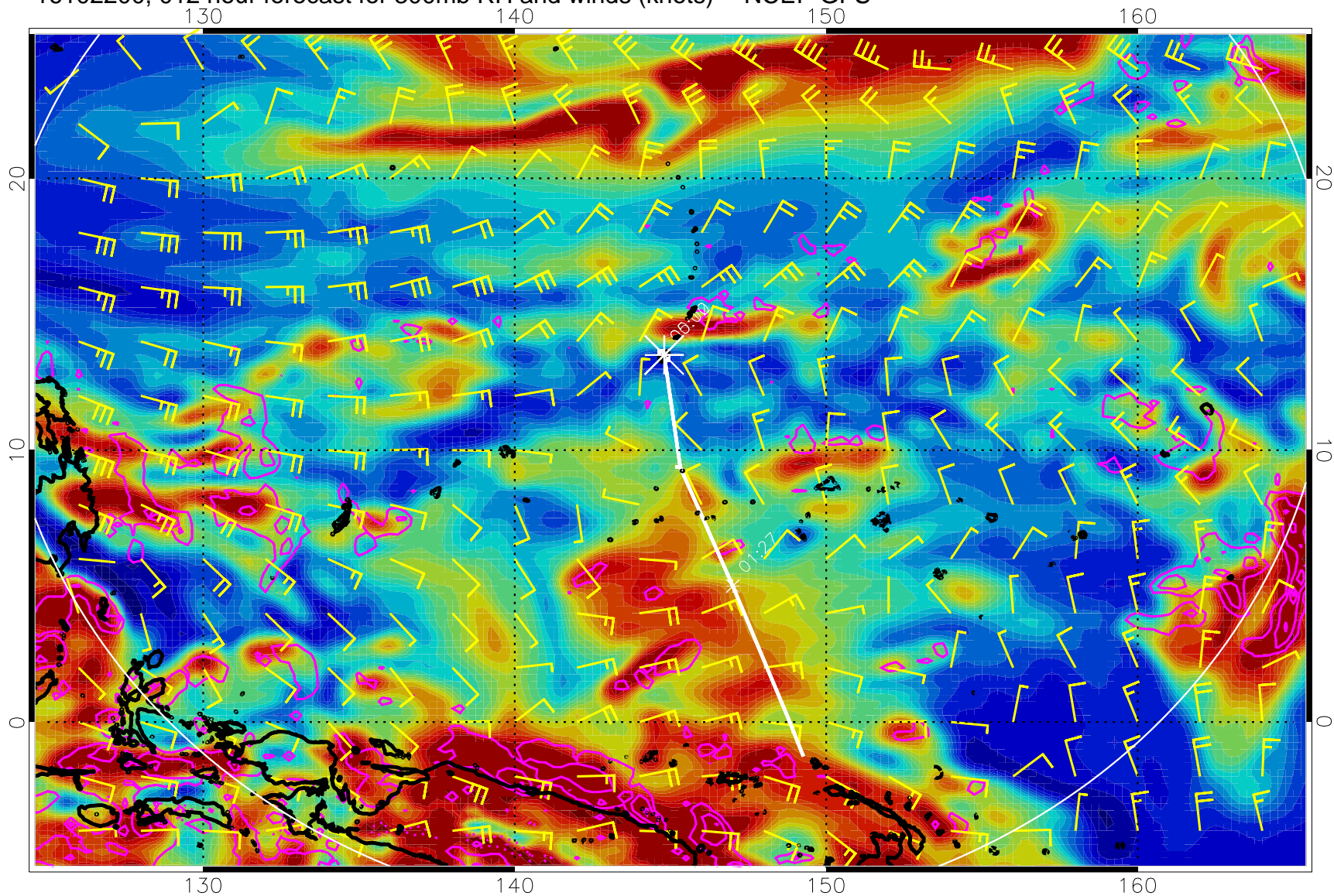
16102200, 012 hour forecast for 300mb RH and winds (knots) -- NCEP GFS
