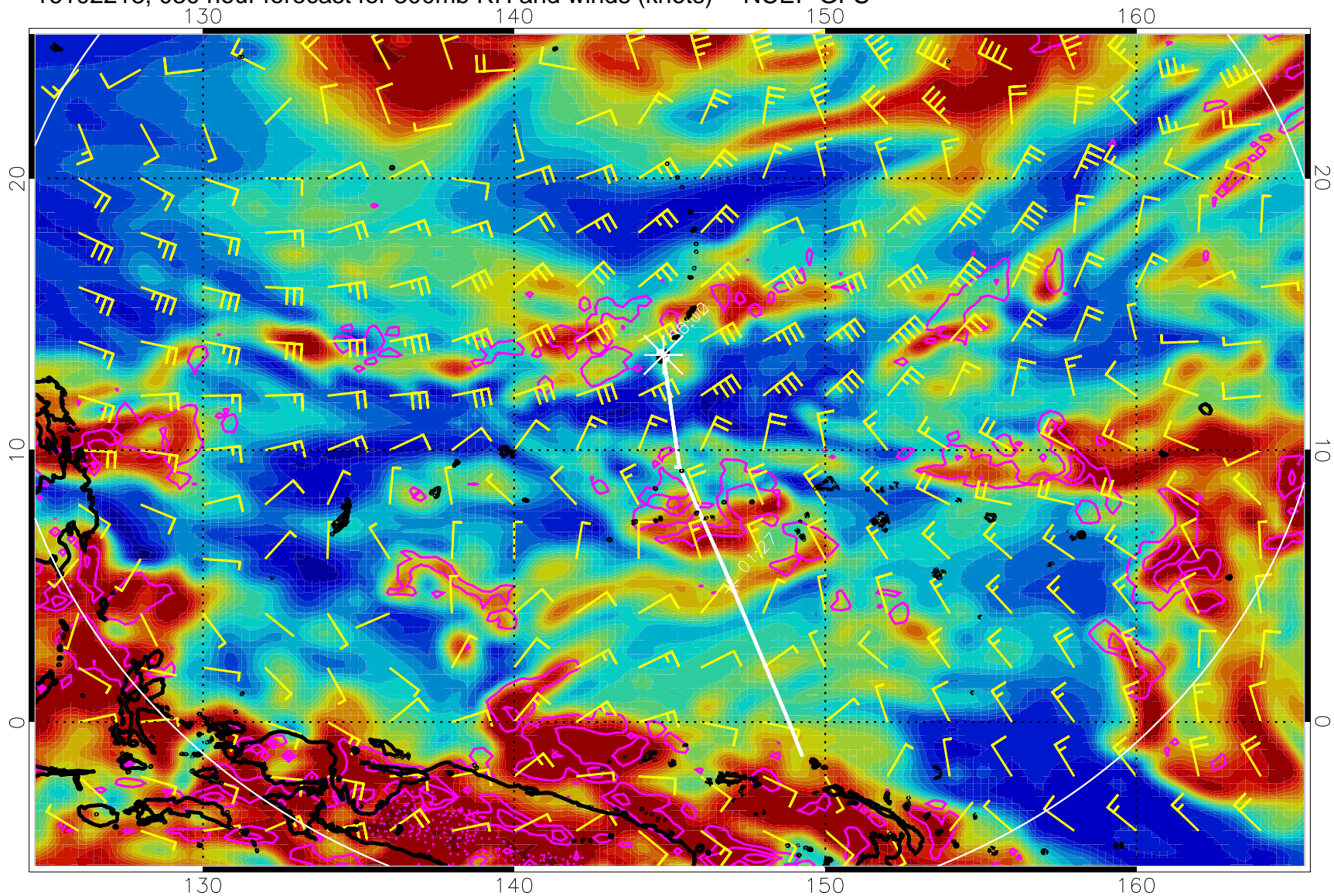
16102218, 030 hour forecast for 300mb RH and winds (knots) -- NCEP GFS
