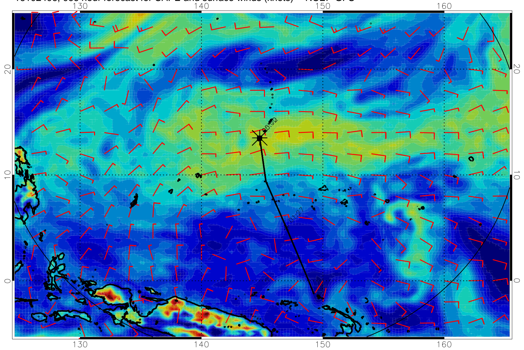
16102406, 066 hour forecast for CAPE and surface winds (knots) -- NCEP GFS
