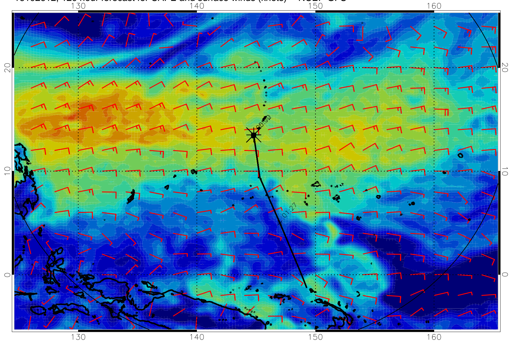
16102612, 120 hour forecast for CAPE and surface winds (knots) -- NCEP GFS
