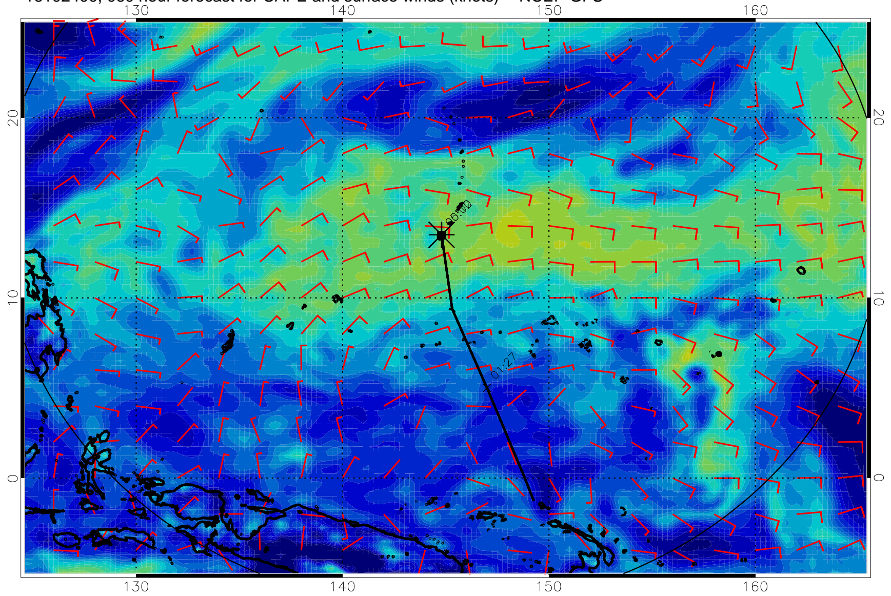
16102400, 060 hour forecast for CAPE and surface winds (knots) -- NCEP GFS
