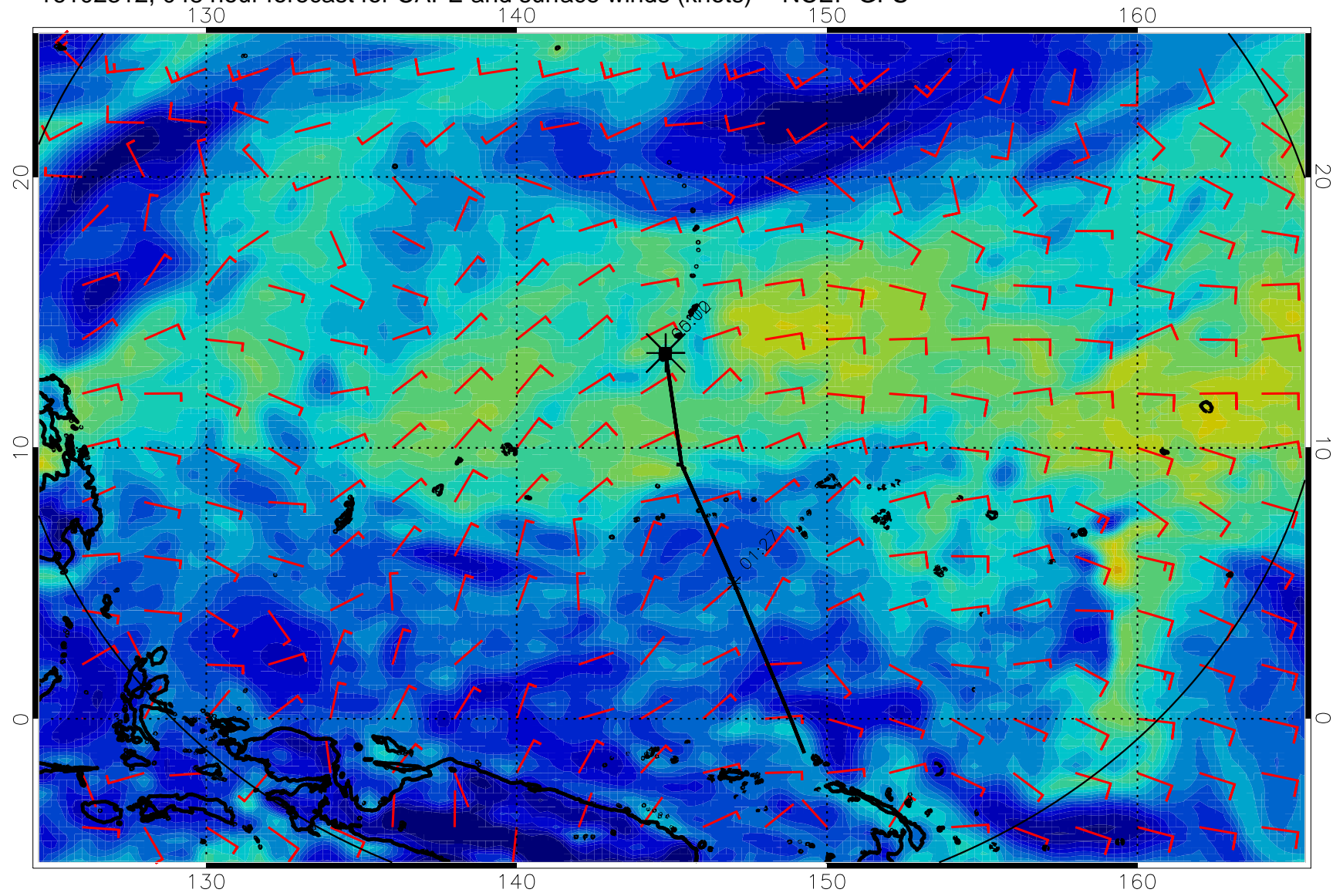
16102312, 048 hour forecast for CAPE and surface winds (knots) -- NCEP GFS
