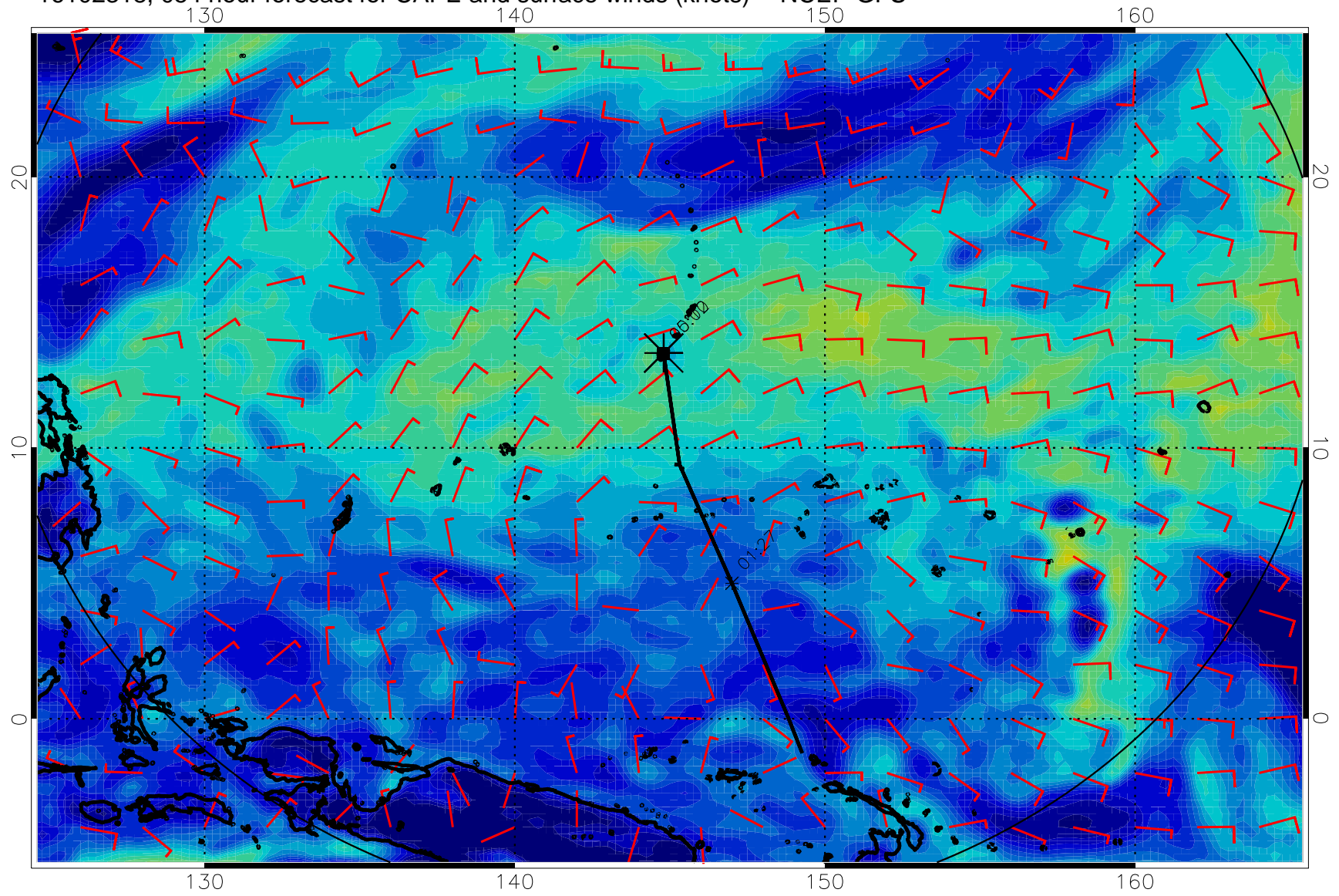
16102318, 054 hour forecast for CAPE and surface winds (knots) -- NCEP GFS
