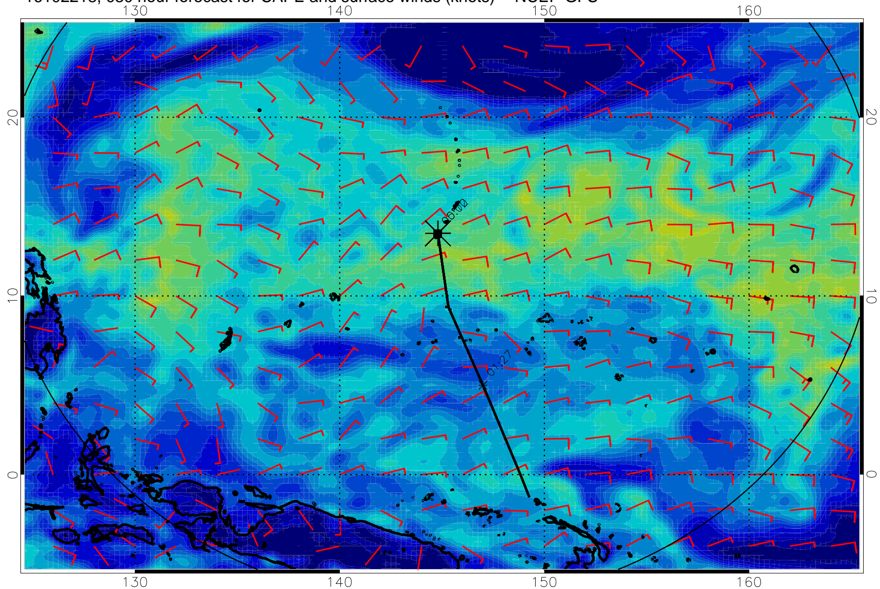
16102218, 030 hour forecast for CAPE and surface winds (knots) -- NCEP GFS
