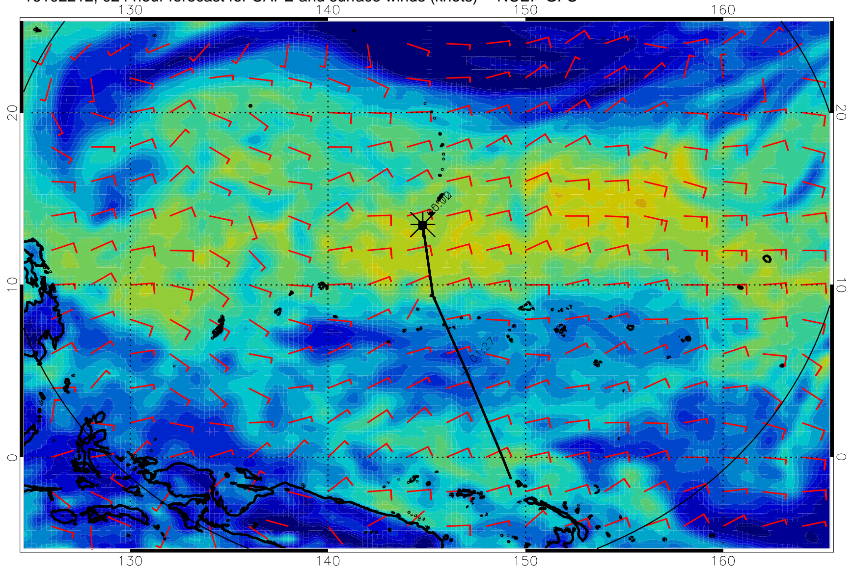
16102212, 024 hour forecast for CAPE and surface winds (knots) -- NCEP GFS
