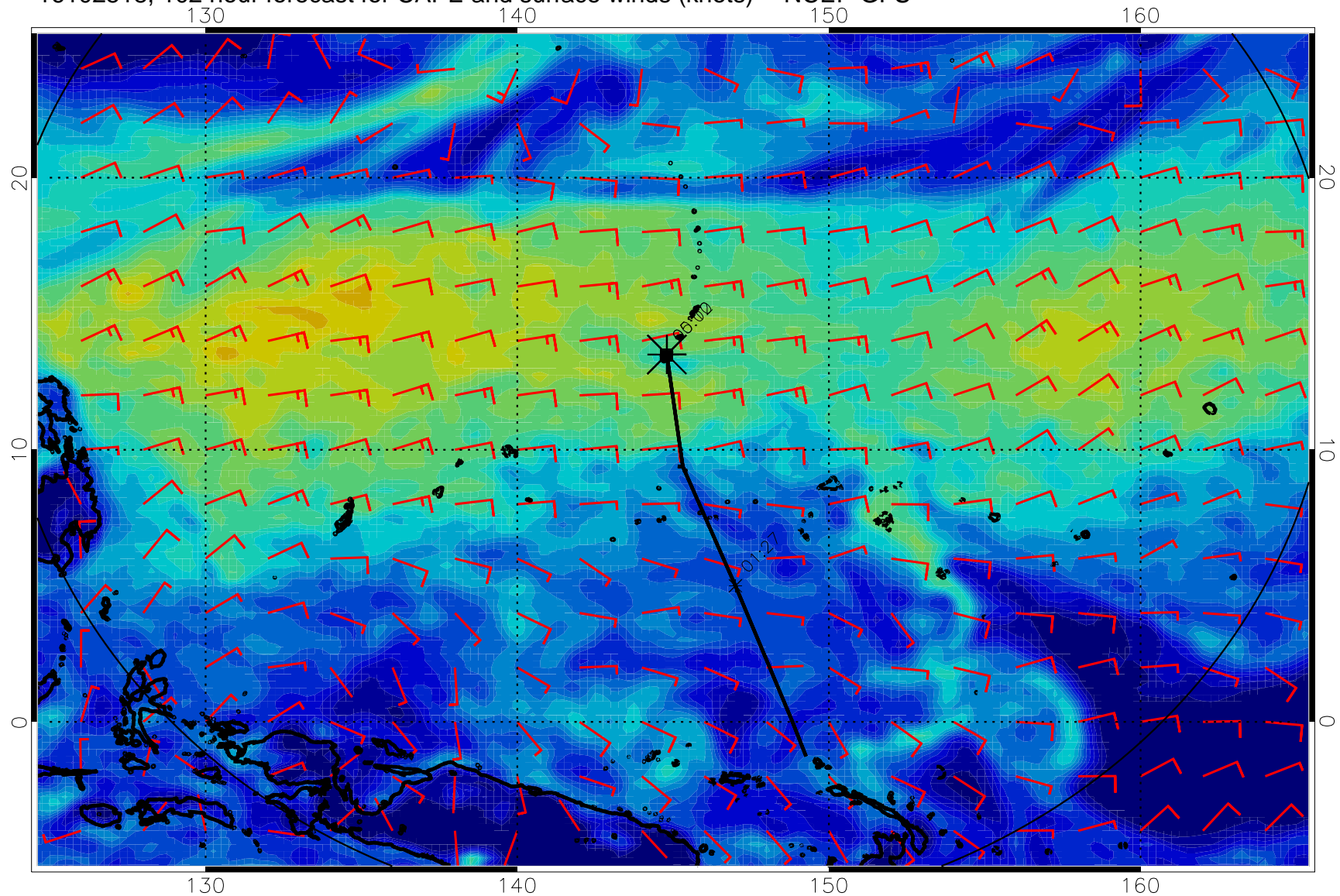
16102518, 102 hour forecast for CAPE and surface winds (knots) -- NCEP GFS
