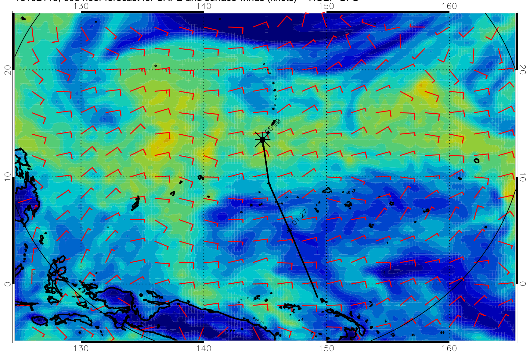
16102118, 006 hour forecast for CAPE and surface winds (knots) -- NCEP GFS
