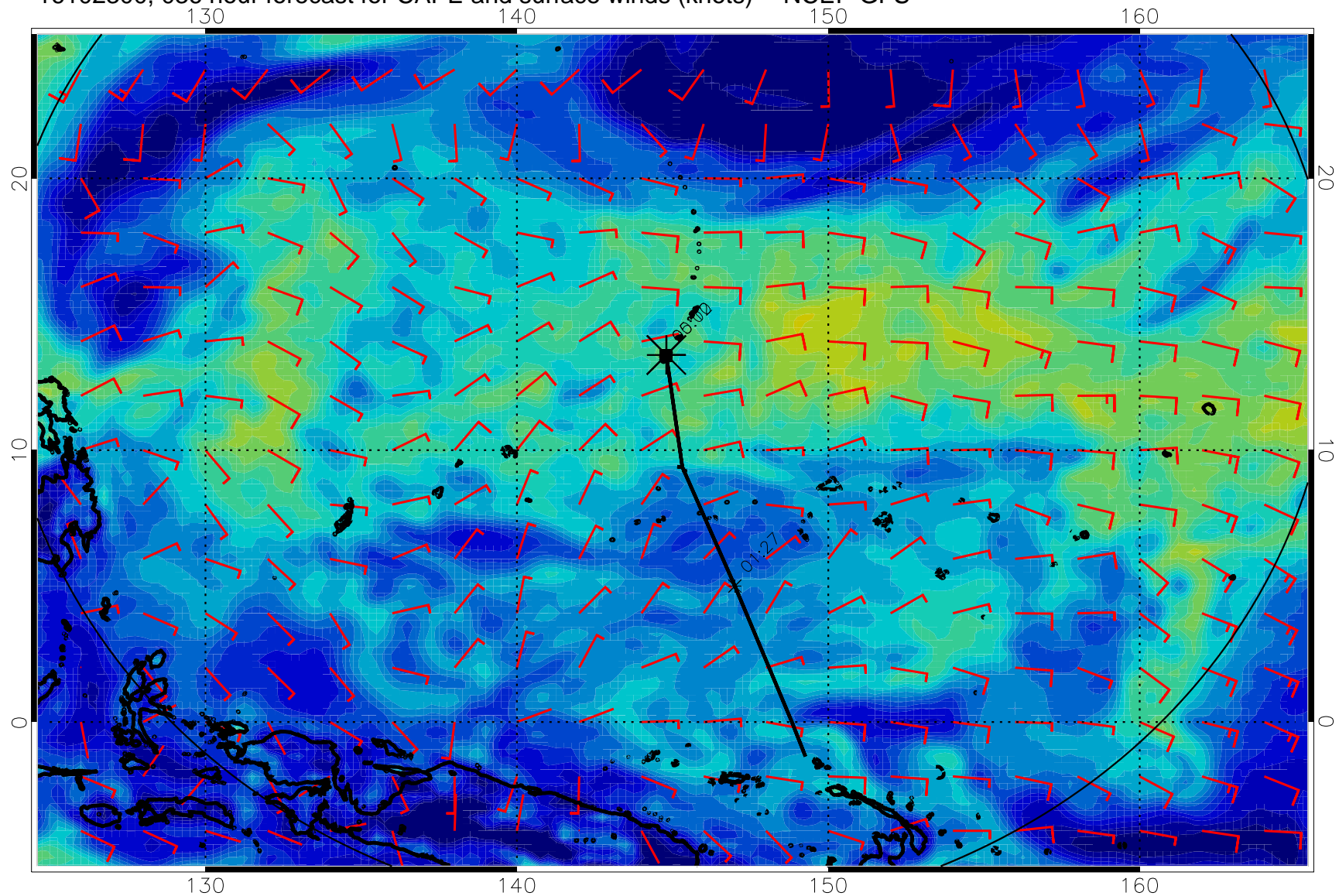
16102300, 036 hour forecast for CAPE and surface winds (knots) -- NCEP GFS
