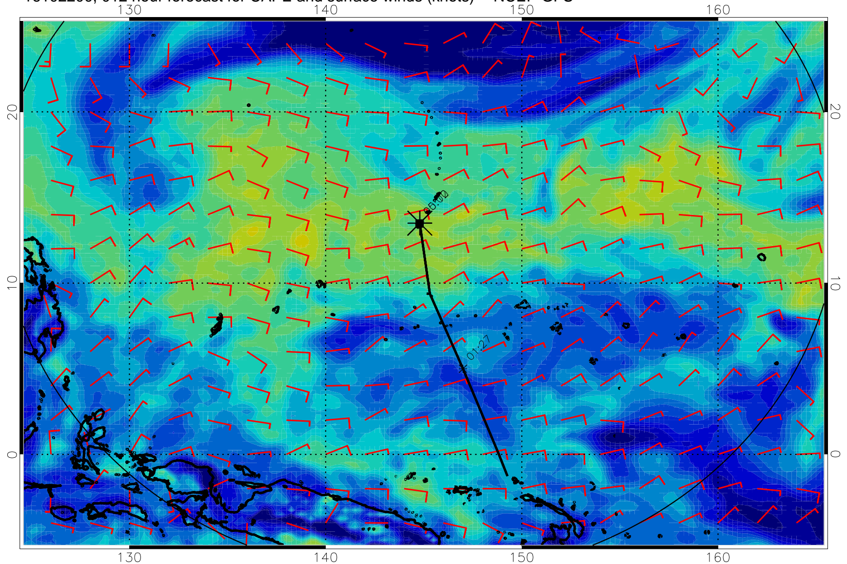
16102200, 012 hour forecast for CAPE and surface winds (knots) -- NCEP GFS
