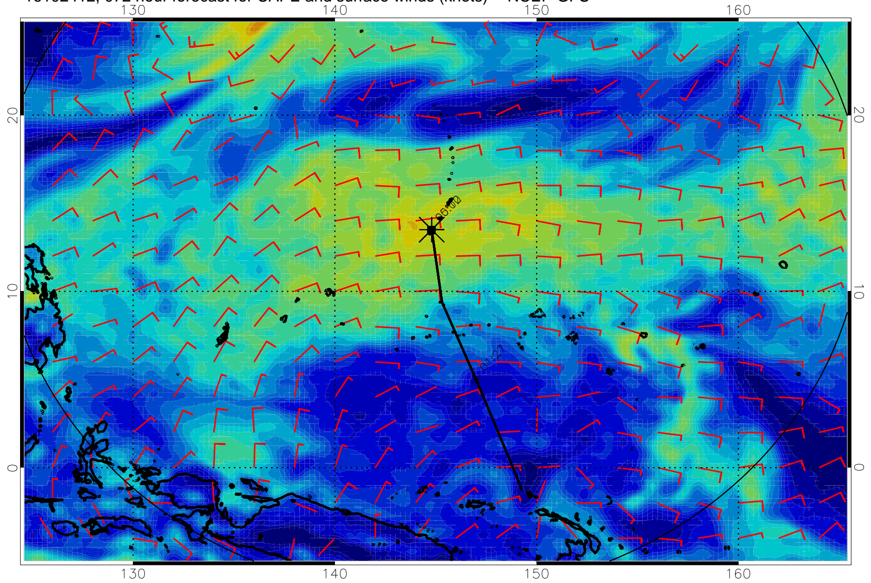
16102412, 072 hour forecast for CAPE and surface winds (knots) -- NCEP GFS
