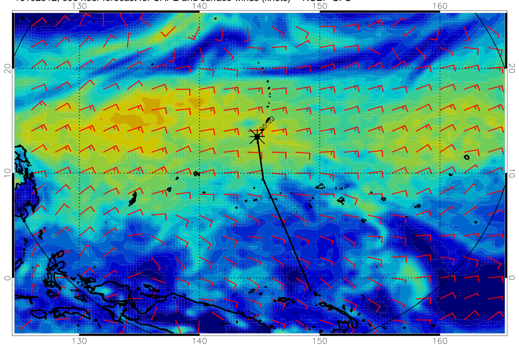
16102512, 096 hour forecast for CAPE and surface winds (knots) -- NCEP GFS
