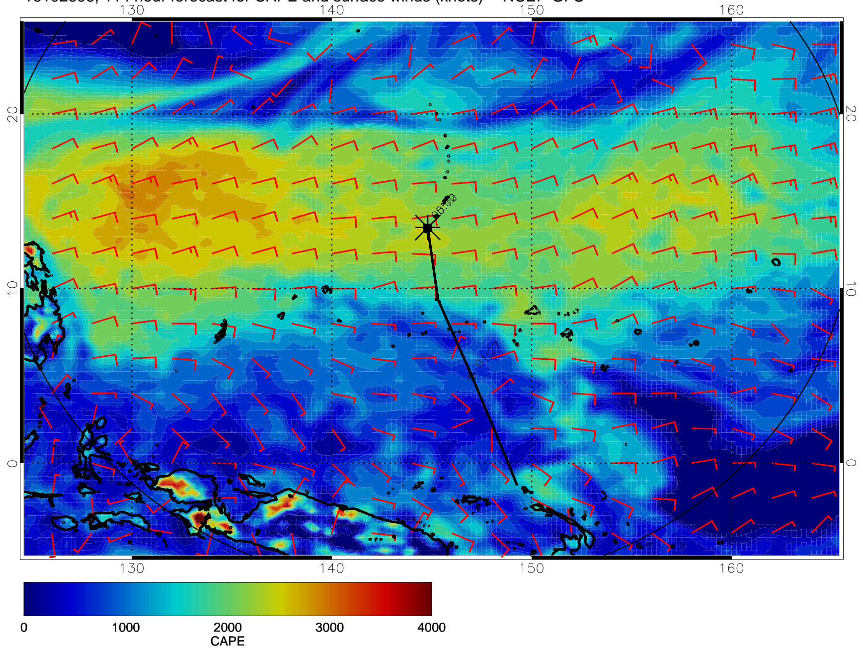
16102606, 114 hour forecast for CAPE and surface winds (knots) -- NCEP GFS
