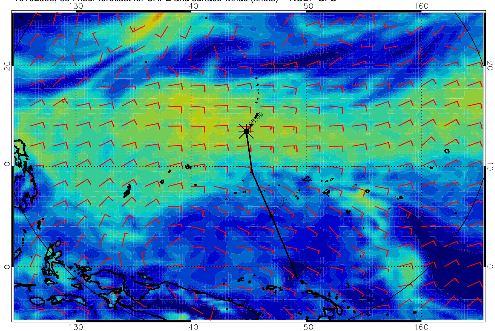
16102500, 084 hour forecast for CAPE and surface winds (knots) -- NCEP GFS
