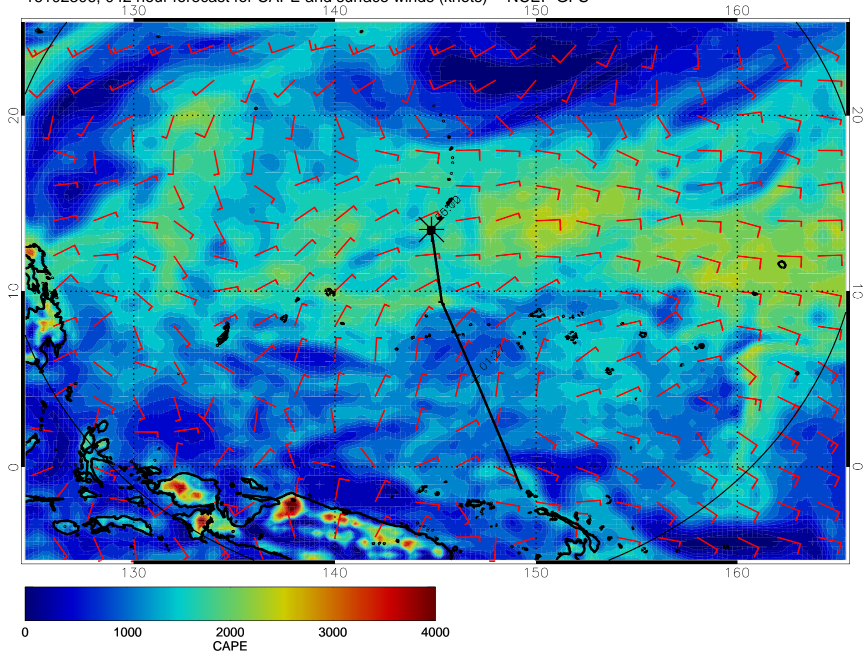
16102306, 042 hour forecast for CAPE and surface winds (knots) -- NCEP GFS
