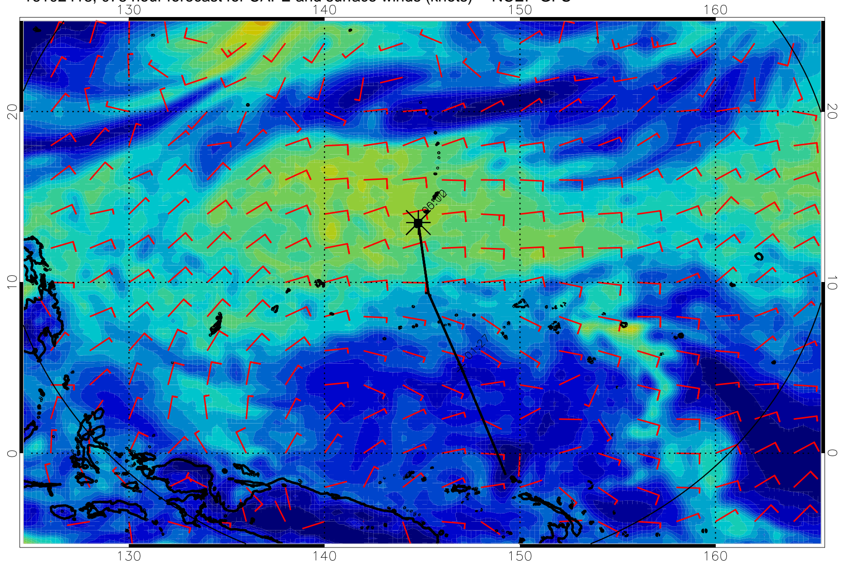
16102418, 078 hour forecast for CAPE and surface winds (knots) -- NCEP GFS
