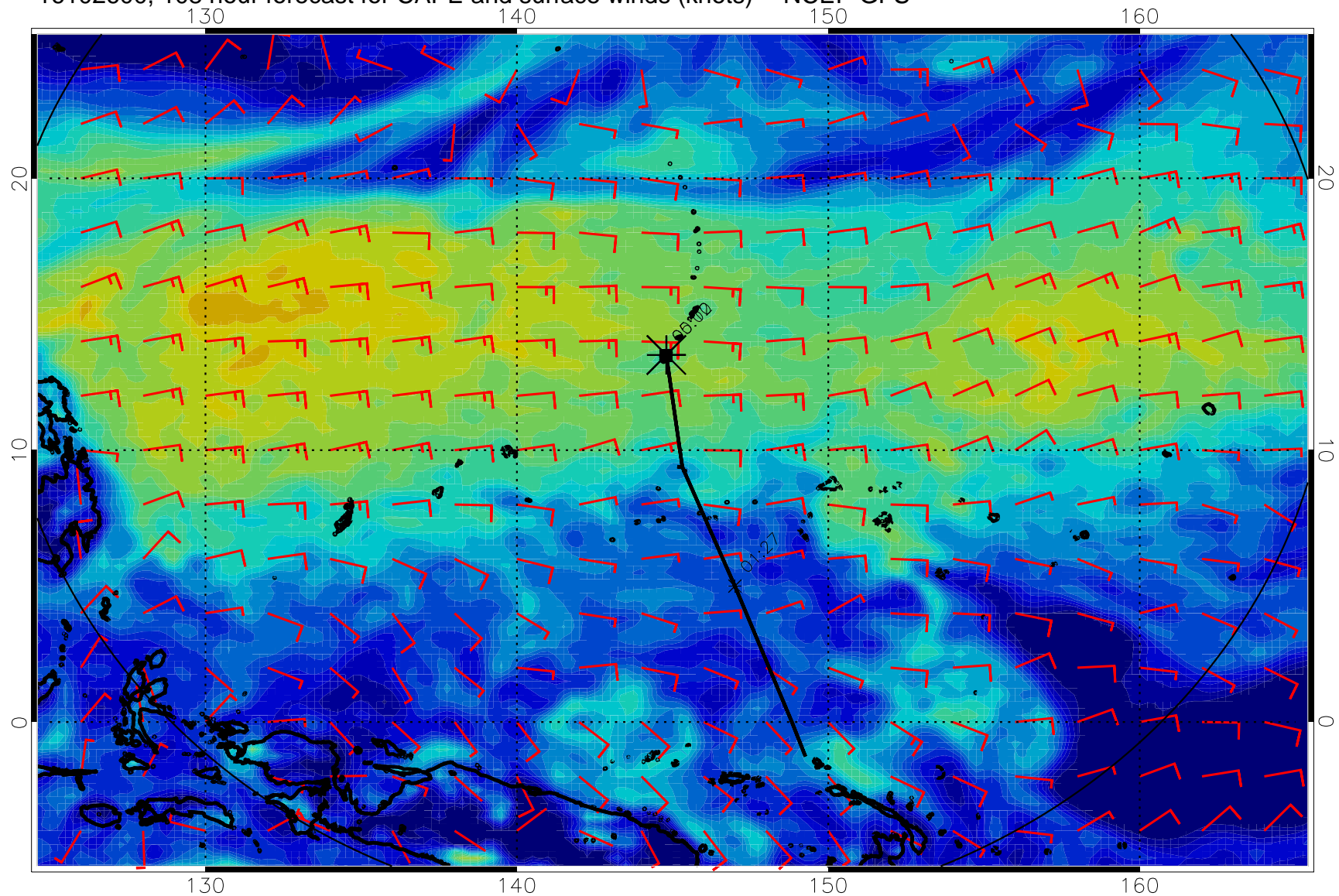
16102600, 108 hour forecast for CAPE and surface winds (knots) -- NCEP GFS
