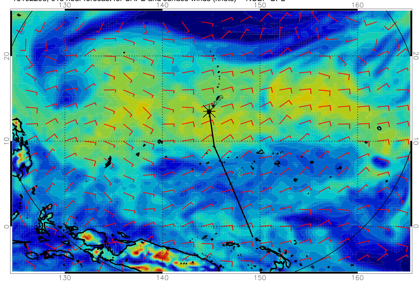
16102206, 018 hour forecast for CAPE and surface winds (knots) -- NCEP GFS
