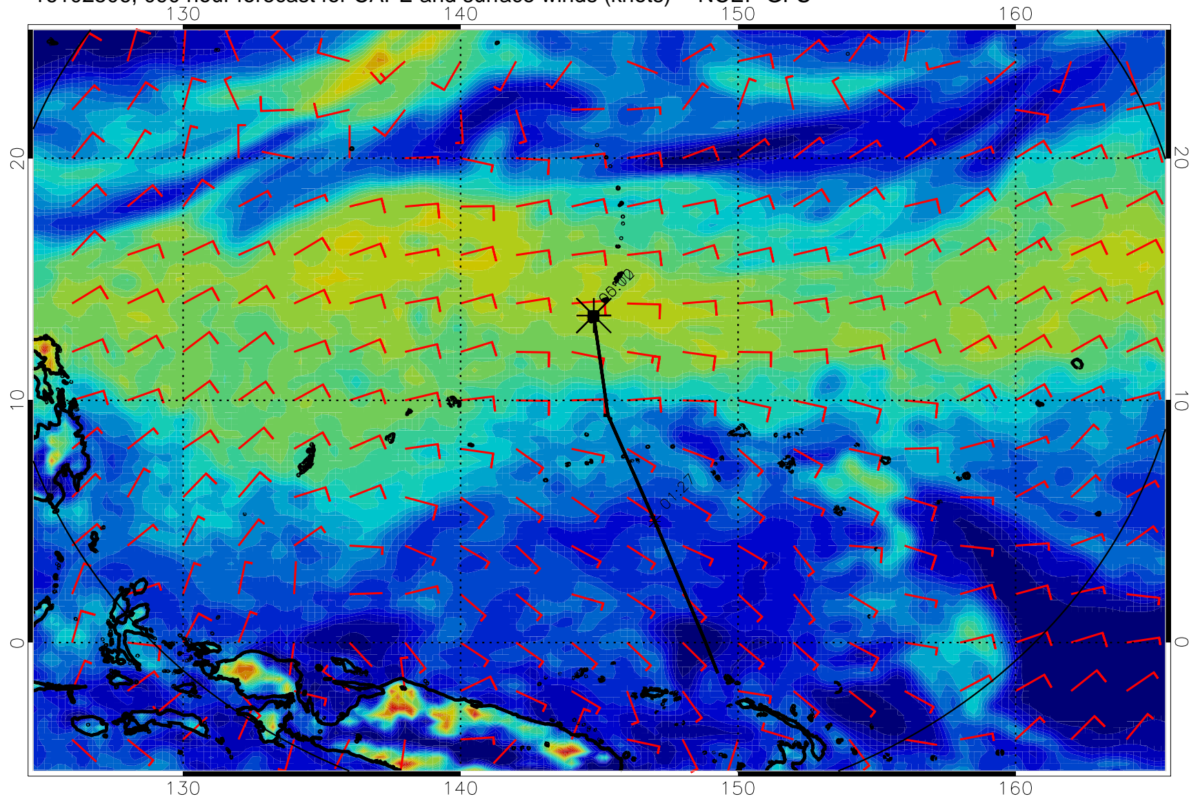
16102506, 090 hour forecast for CAPE and surface winds (knots) -- NCEP GFS
