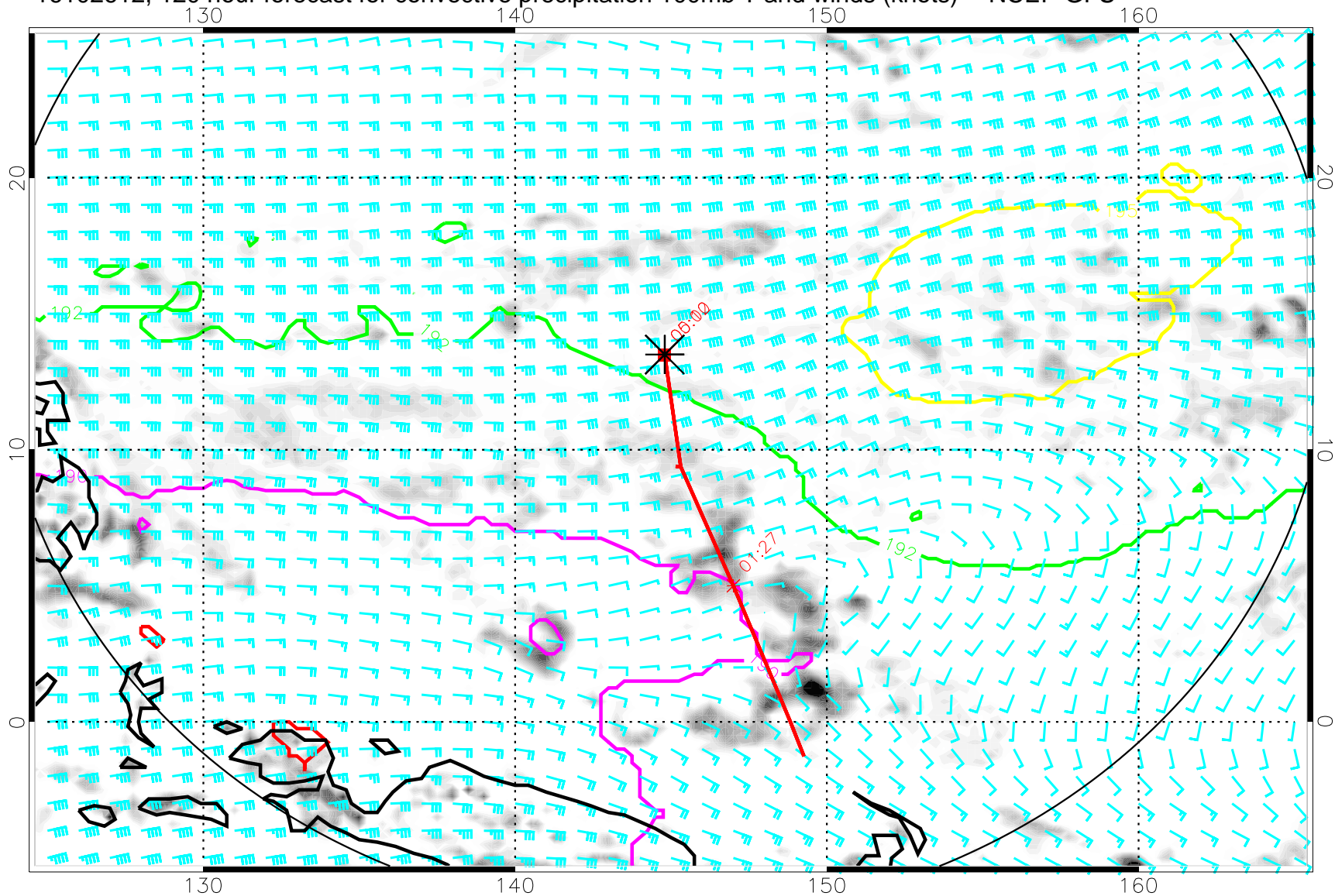
16102612, 120 hour forecast for convective precipitation 100mb T and winds (knots) -- NCEP GFS
