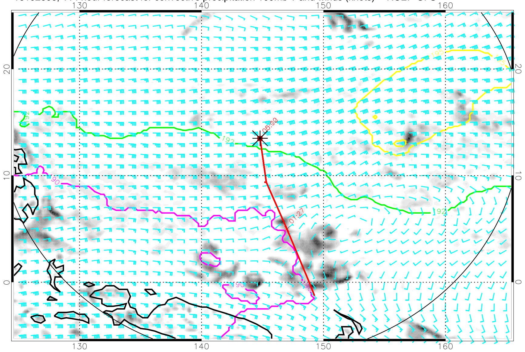
16102606, 114 hour forecast for convective precipitation 100mb T and winds (knots) -- NCEP GFS
