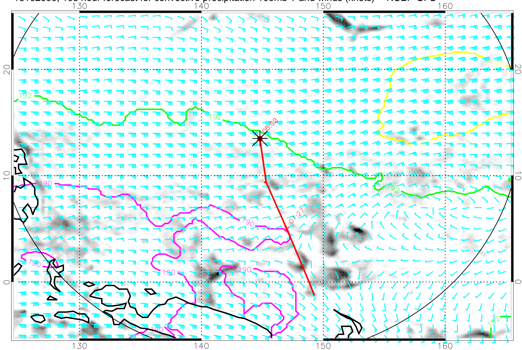
16102600, 108 hour forecast for convective precipitation 100mb T and winds (knots) -- NCEP GFS
