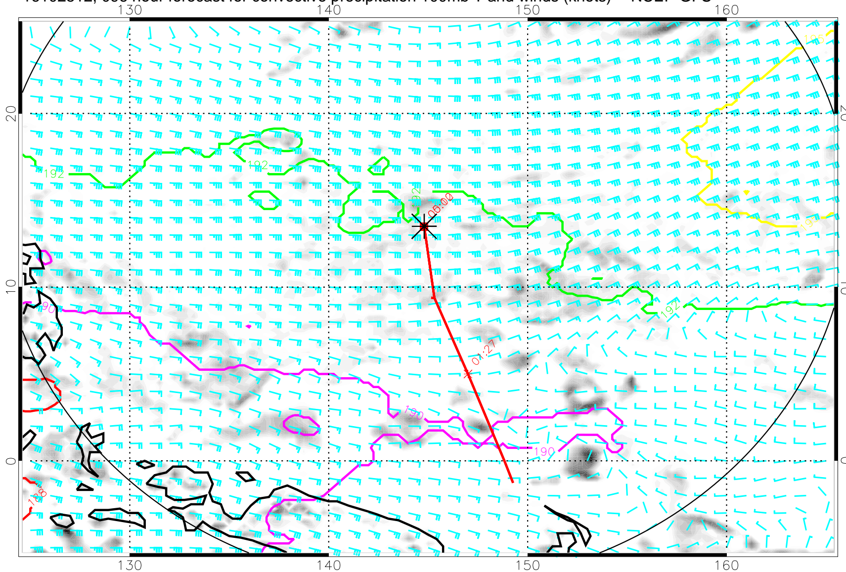
16102512, 096 hour forecast for convective precipitation 100mb T and winds (knots) -- NCEP GFS
