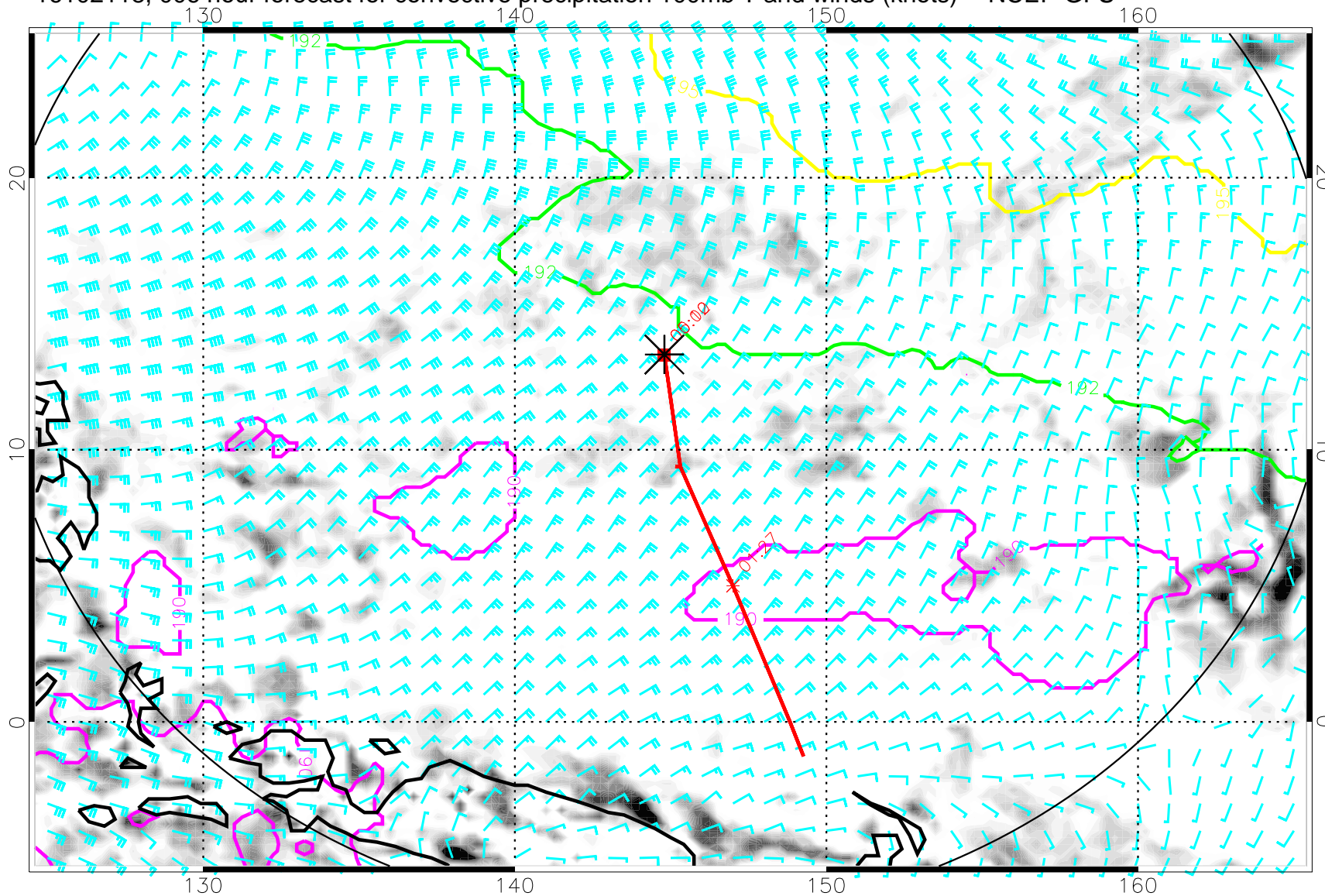
16102118, 006 hour forecast for convective precipitation 100mb T and winds (knots) -- NCEP GFS
