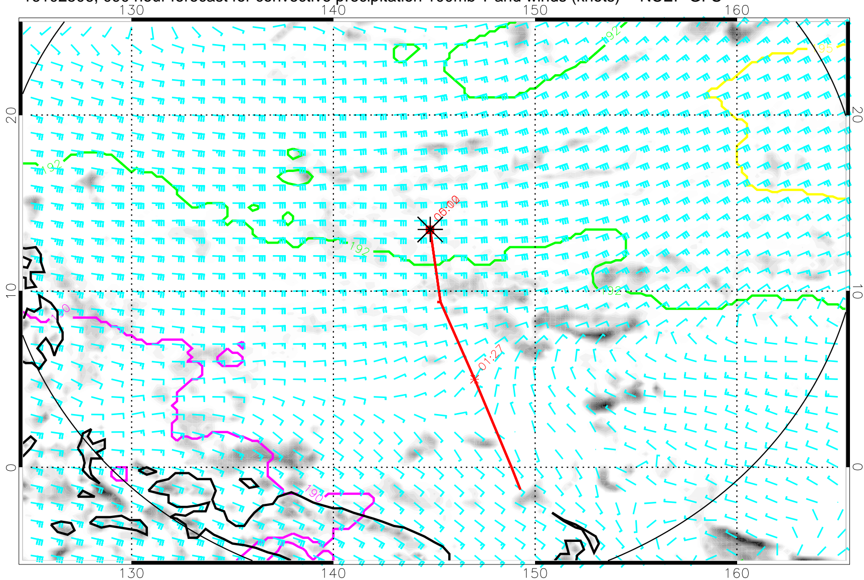
16102506, 090 hour forecast for convective precipitation 100mb T and winds (knots) -- NCEP GFS
