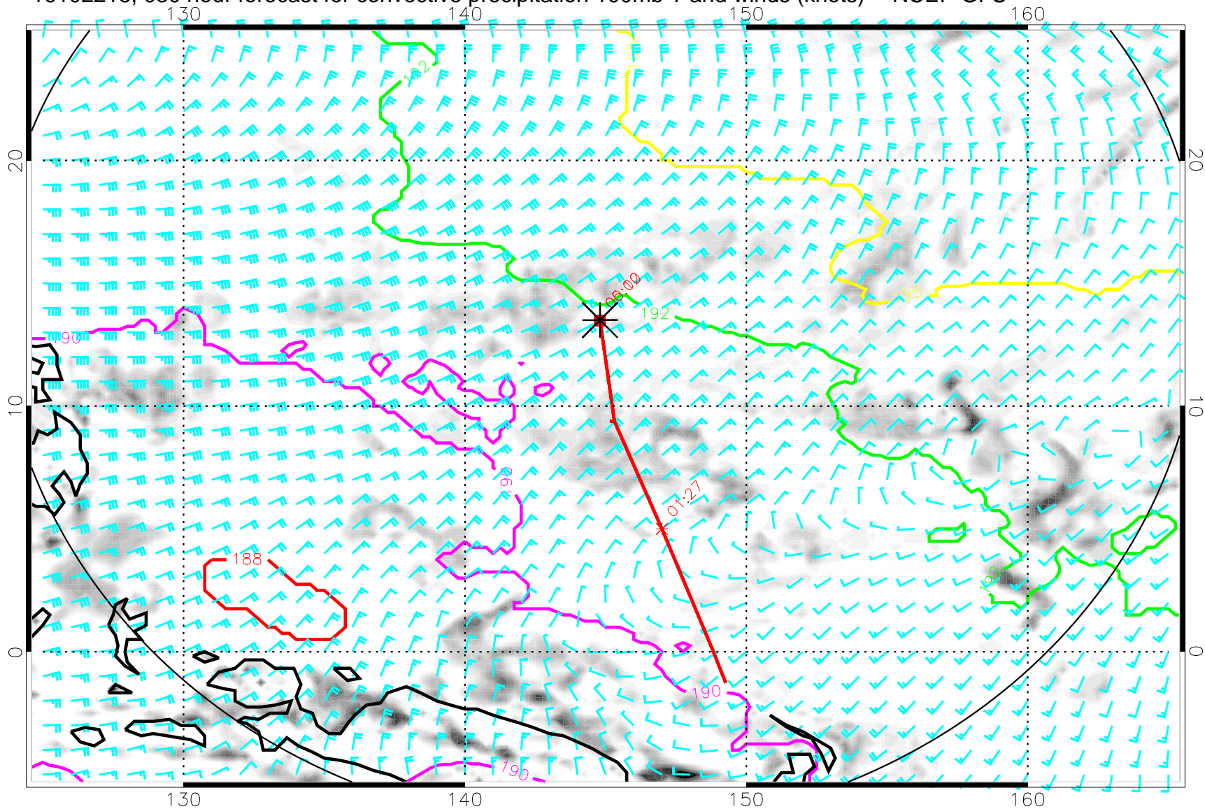
16102218, 030 hour forecast for convective precipitation 100mb T and winds (knots) -- NCEP GFS
