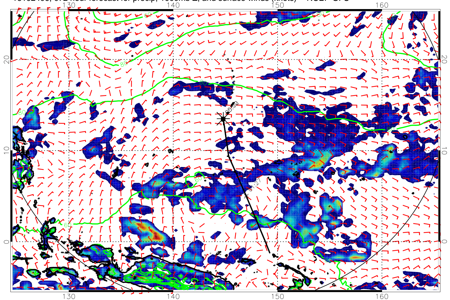
16102406, 072 hour forecast for precip, 1000mb Z, and surface winds (knots) -- NCEP GFS
