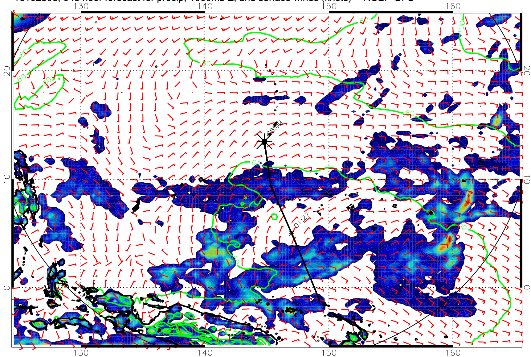
16102306, 048 hour forecast for precip, 1000mb Z, and surface winds (knots) -- NCEP GFS
