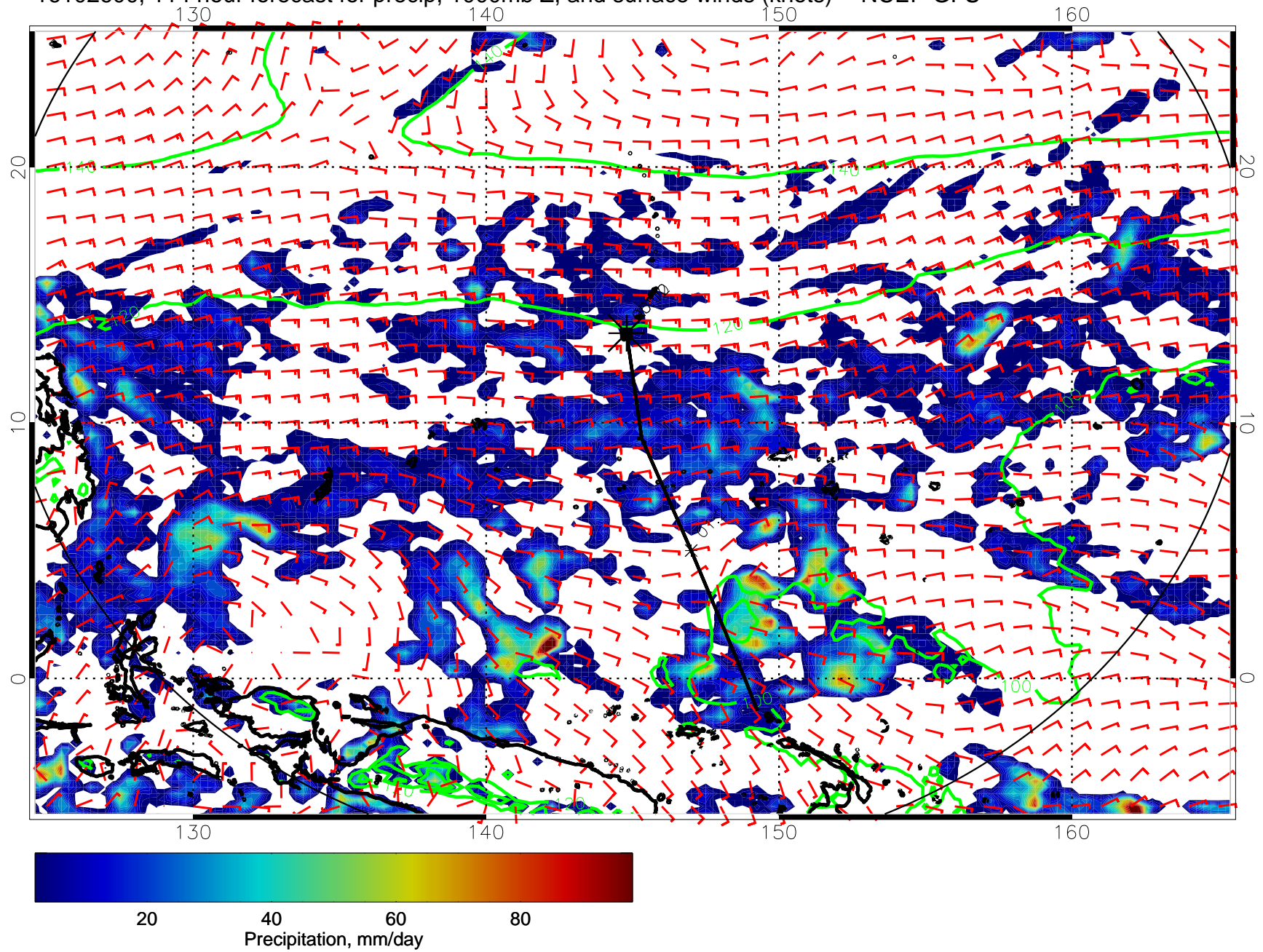
16102600, 114 hour forecast for precip, 1000mb Z, and surface winds (knots) -- NCEP GFS
