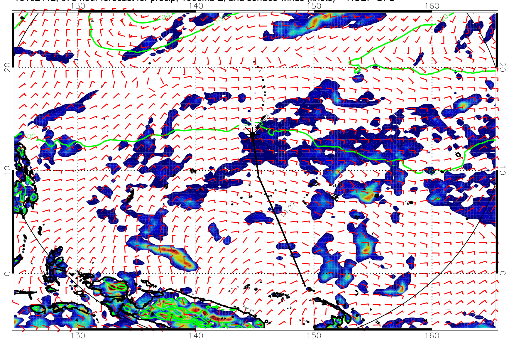
16102412, 078 hour forecast for precip, 1000mb Z, and surface winds (knots) -- NCEP GFS
