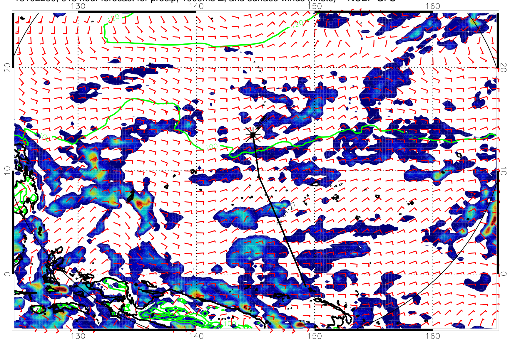
16102200, 018 hour forecast for precip, 1000mb Z, and surface winds (knots) -- NCEP GFS
