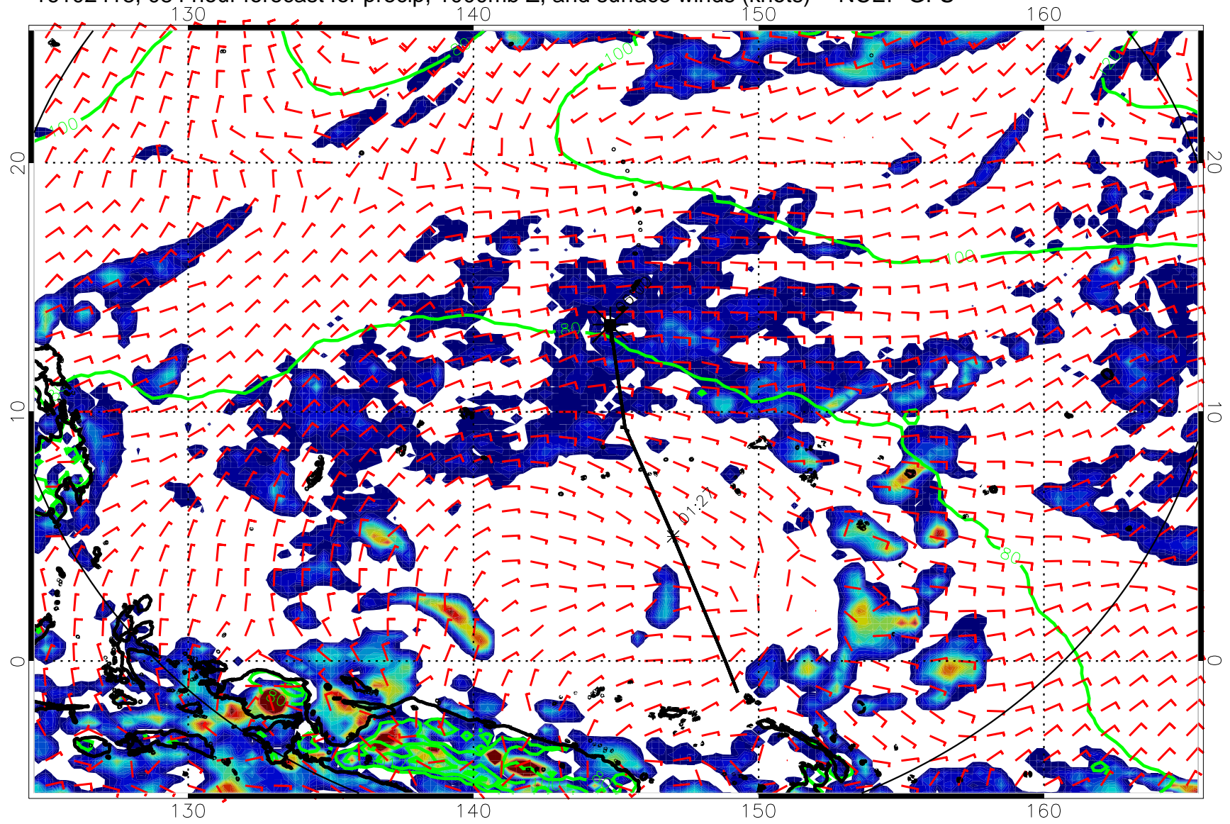
16102418, 084 hour forecast for precip, 1000mb Z, and surface winds (knots) -- NCEP GFS
