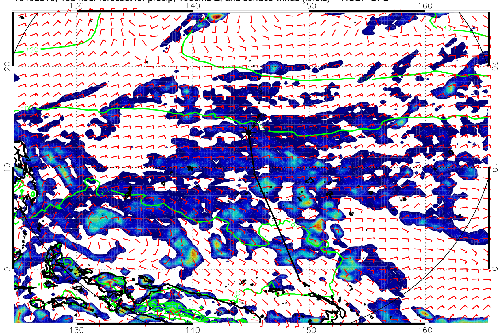
16102518, 108 hour forecast for precip, 1000mb Z, and surface winds (knots) -- NCEP GFS
