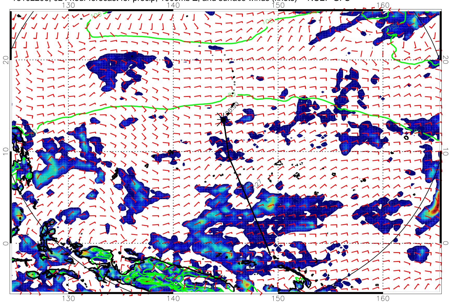
16102206, 024 hour forecast for precip, 1000mb Z, and surface winds (knots) -- NCEP GFS
