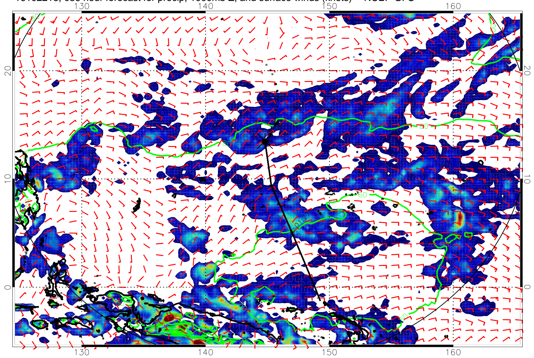
16102218, 036 hour forecast for precip, 1000mb Z, and surface winds (knots) -- NCEP GFS
