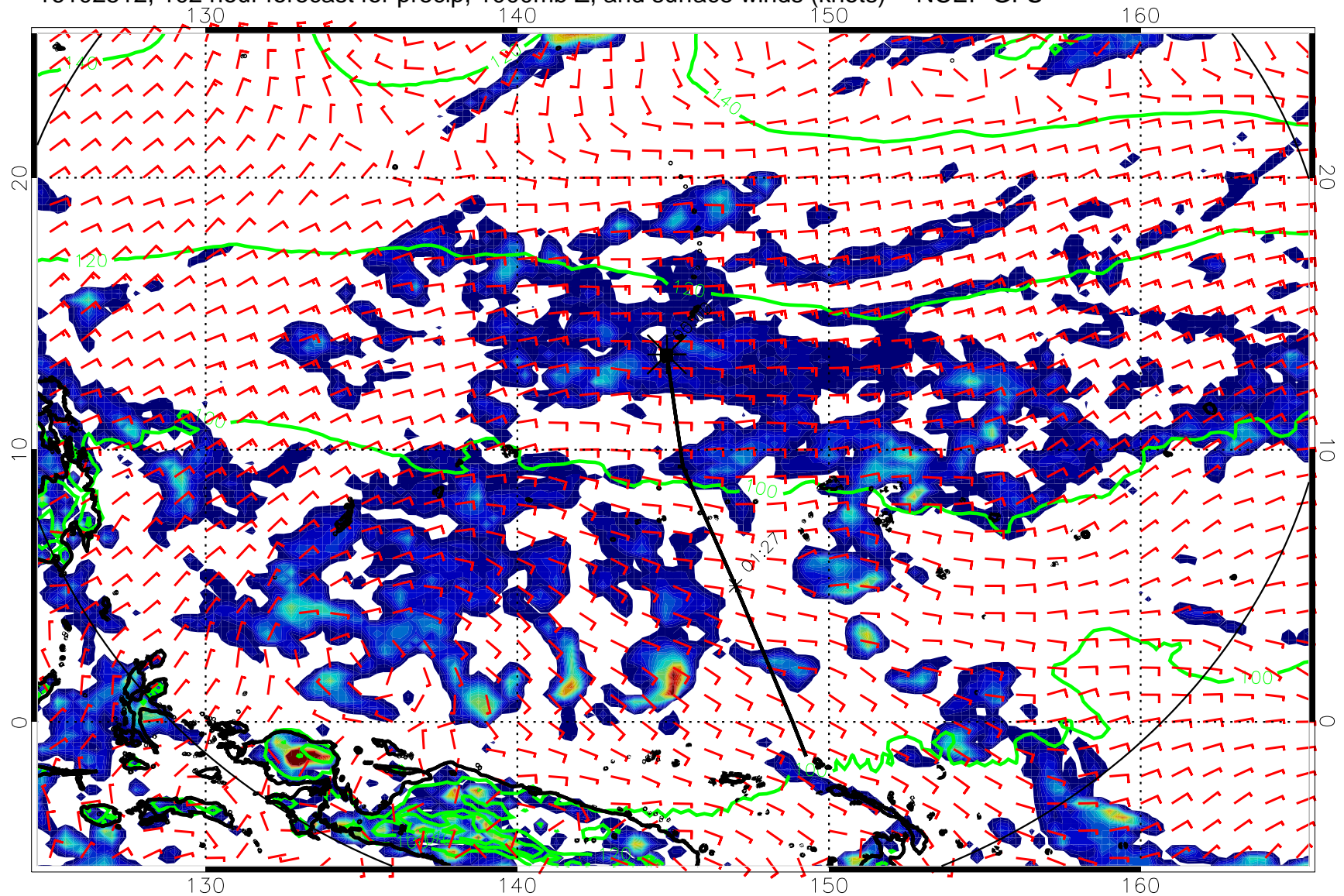
16102512, 102 hour forecast for precip, 1000mb Z, and surface winds (knots) -- NCEP GFS
