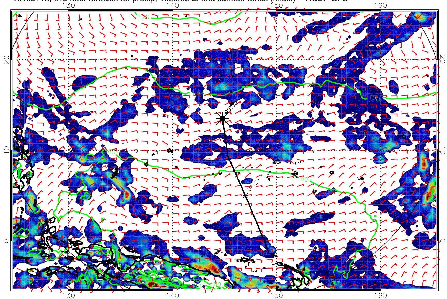
16102118, 012 hour forecast for precip, 1000mb Z, and surface winds (knots) -- NCEP GFS
