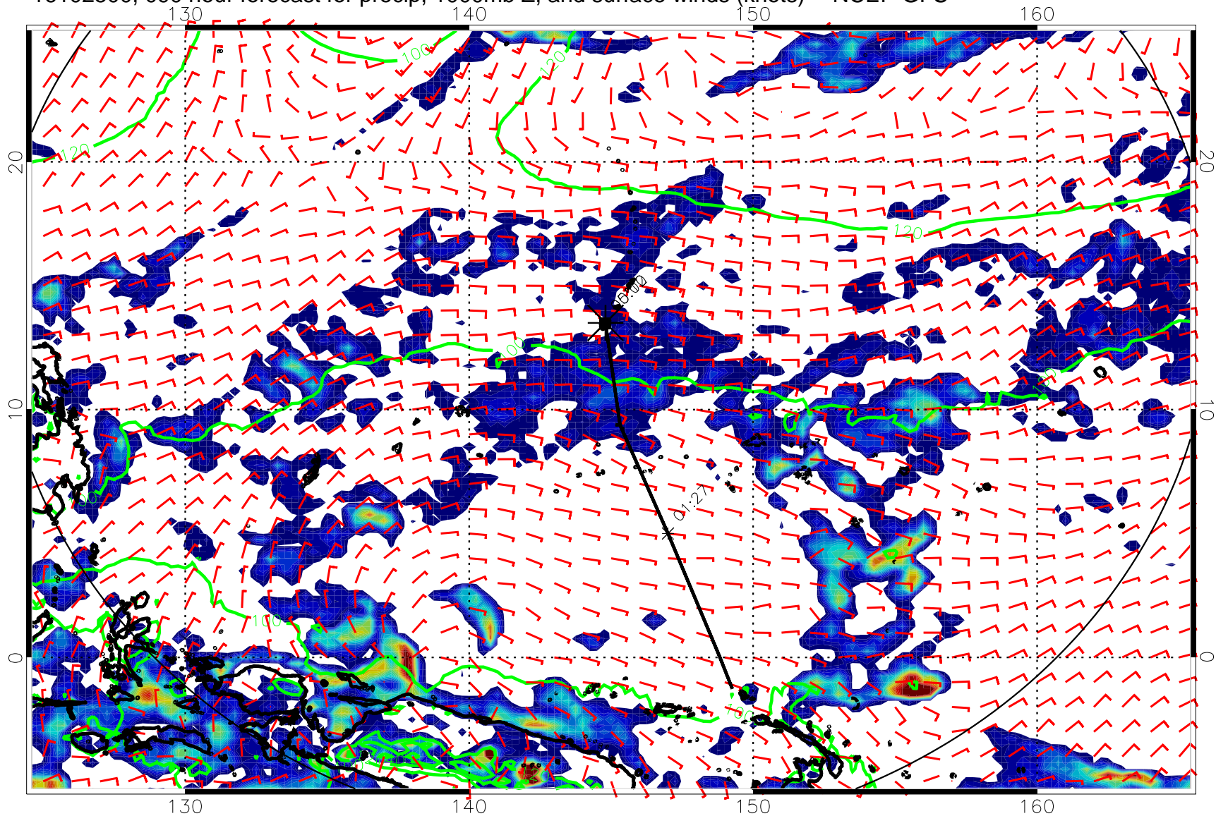
16102500, 090 hour forecast for precip, 1000mb Z, and surface winds (knots) -- NCEP GFS
