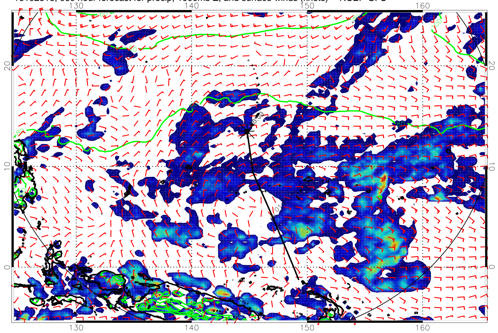
16102318, 060 hour forecast for precip, 1000mb Z, and surface winds (knots) -- NCEP GFS
