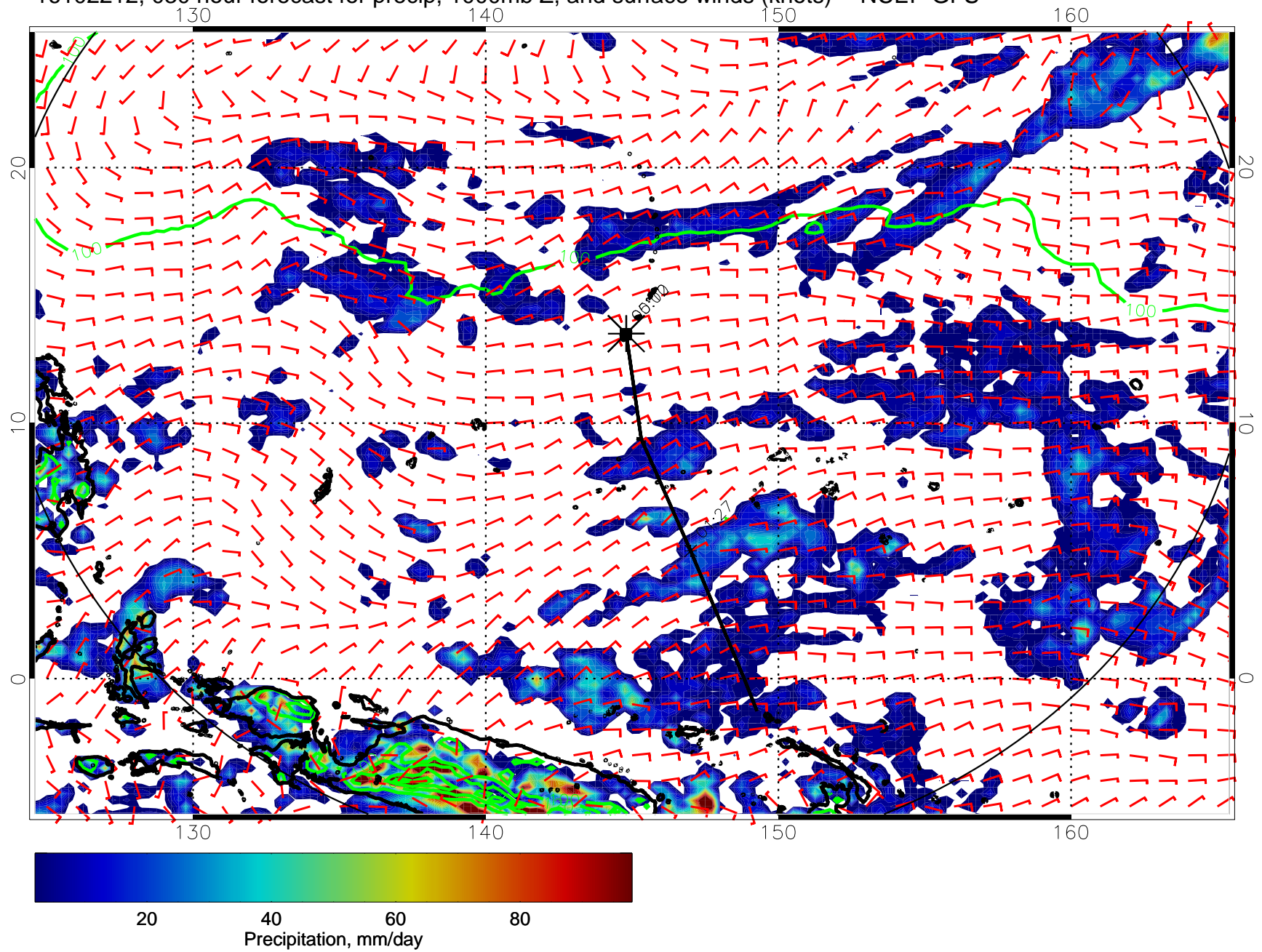
16102212, 030 hour forecast for precip, 1000mb Z, and surface winds (knots) -- NCEP GFS
