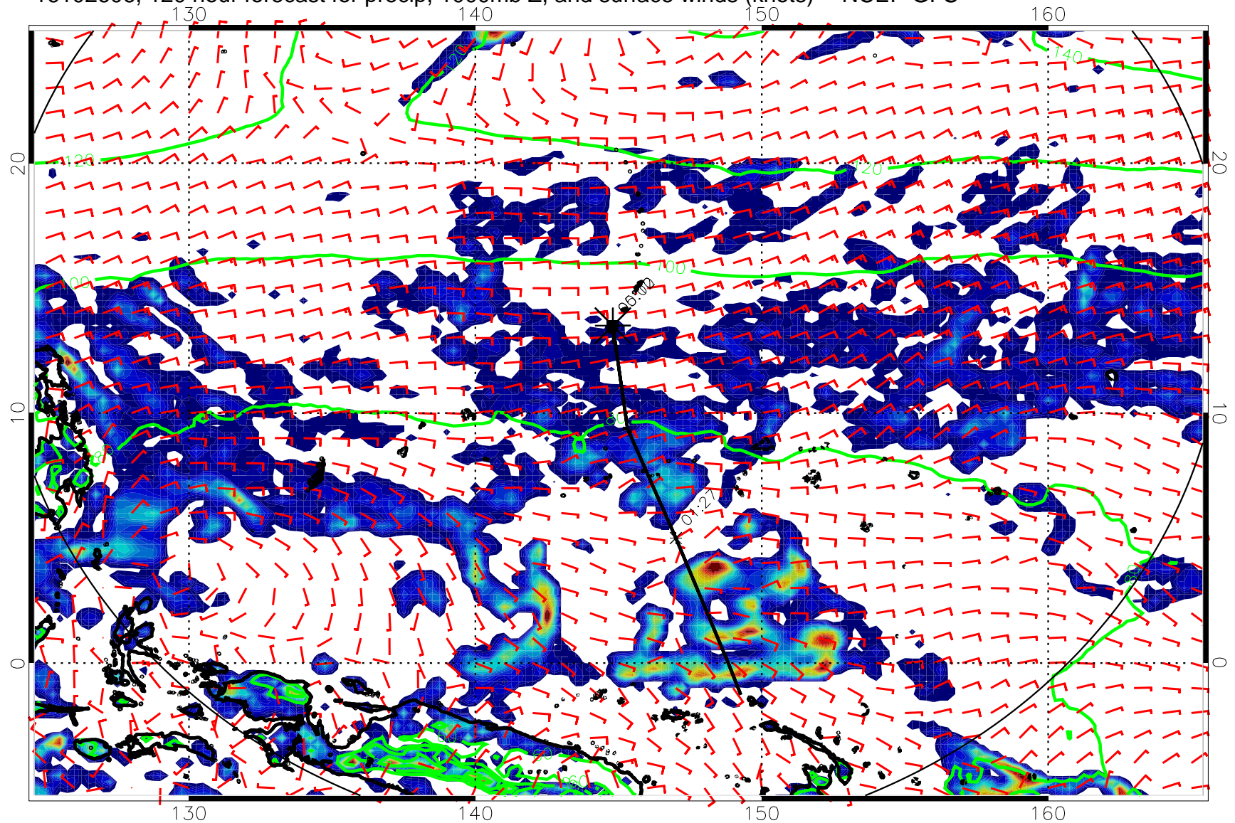
16102606, 120 hour forecast for precip, 1000mb Z, and surface winds (knots) -- NCEP GFS
