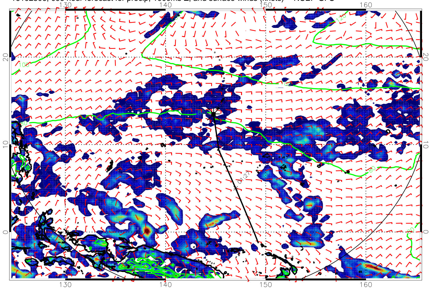
16102506, 096 hour forecast for precip, 1000mb Z, and surface winds (knots) -- NCEP GFS
