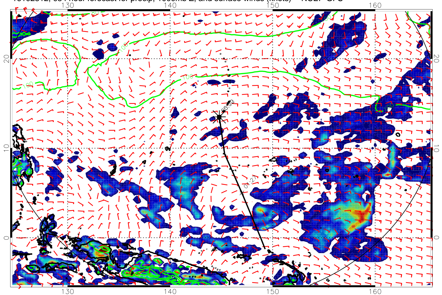
16102312, 054 hour forecast for precip, 1000mb Z, and surface winds (knots) -- NCEP GFS
