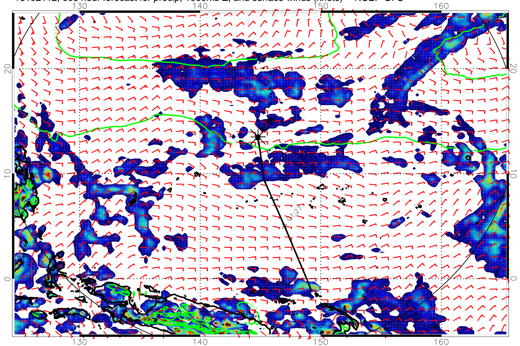
16102112, 006 hour forecast for precip, 1000mb Z, and surface winds (knots) -- NCEP GFS
