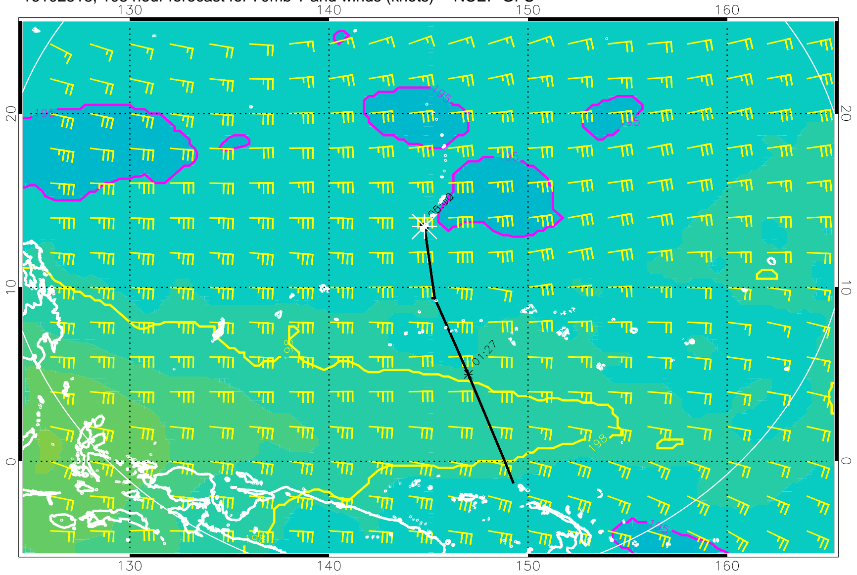
16102518, 108 hour forecast for 70mb T and winds (knots) -- NCEP GFS
