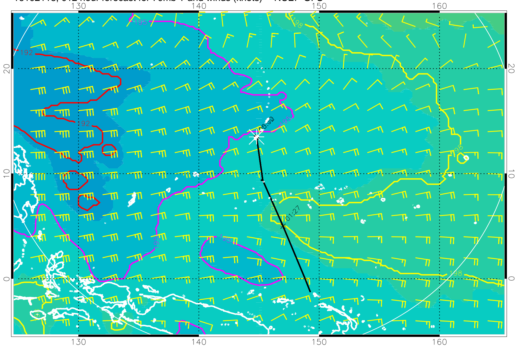
16102118, 012 hour forecast for 70mb T and winds (knots) -- NCEP GFS
