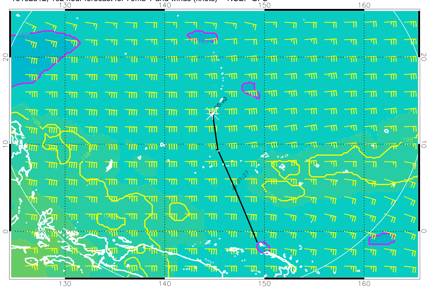
16102512, 102 hour forecast for 70mb T and winds (knots) -- NCEP GFS
