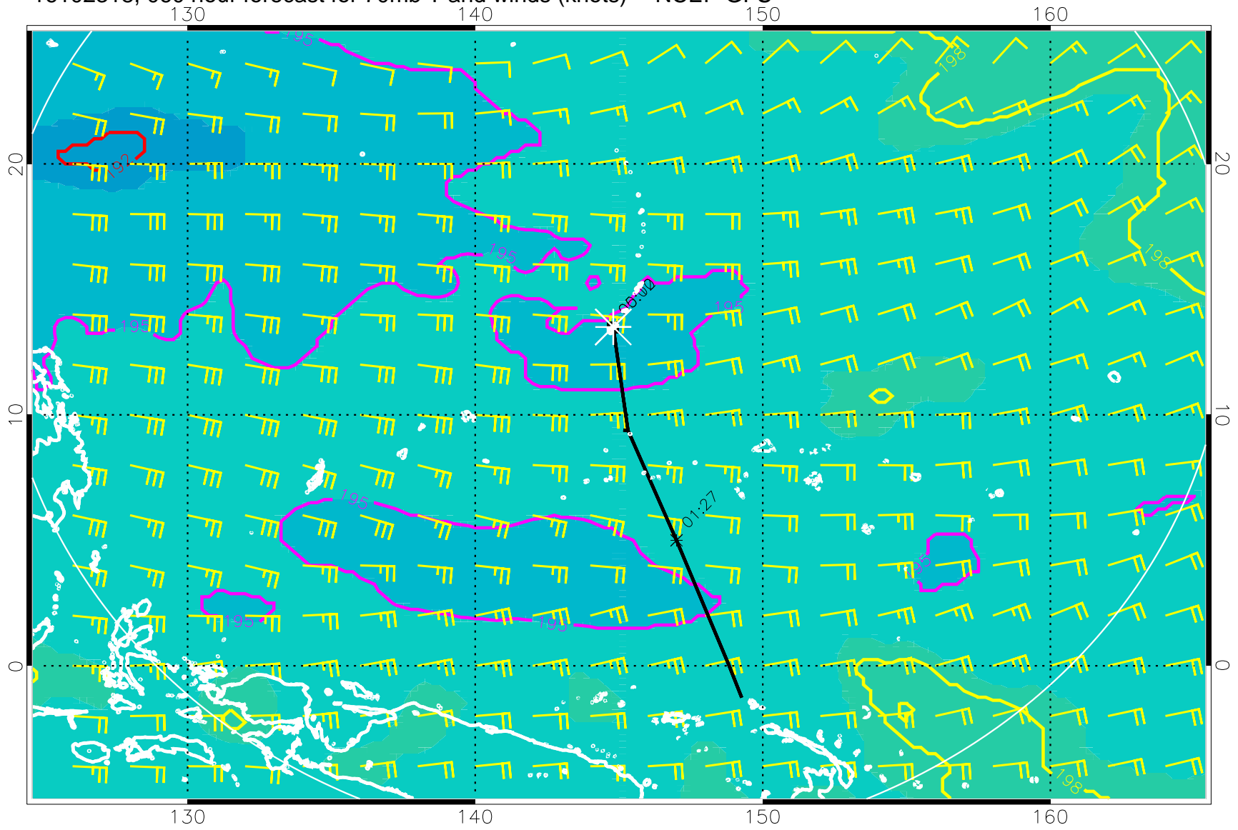
16102318, 060 hour forecast for 70mb T and winds (knots) -- NCEP GFS
