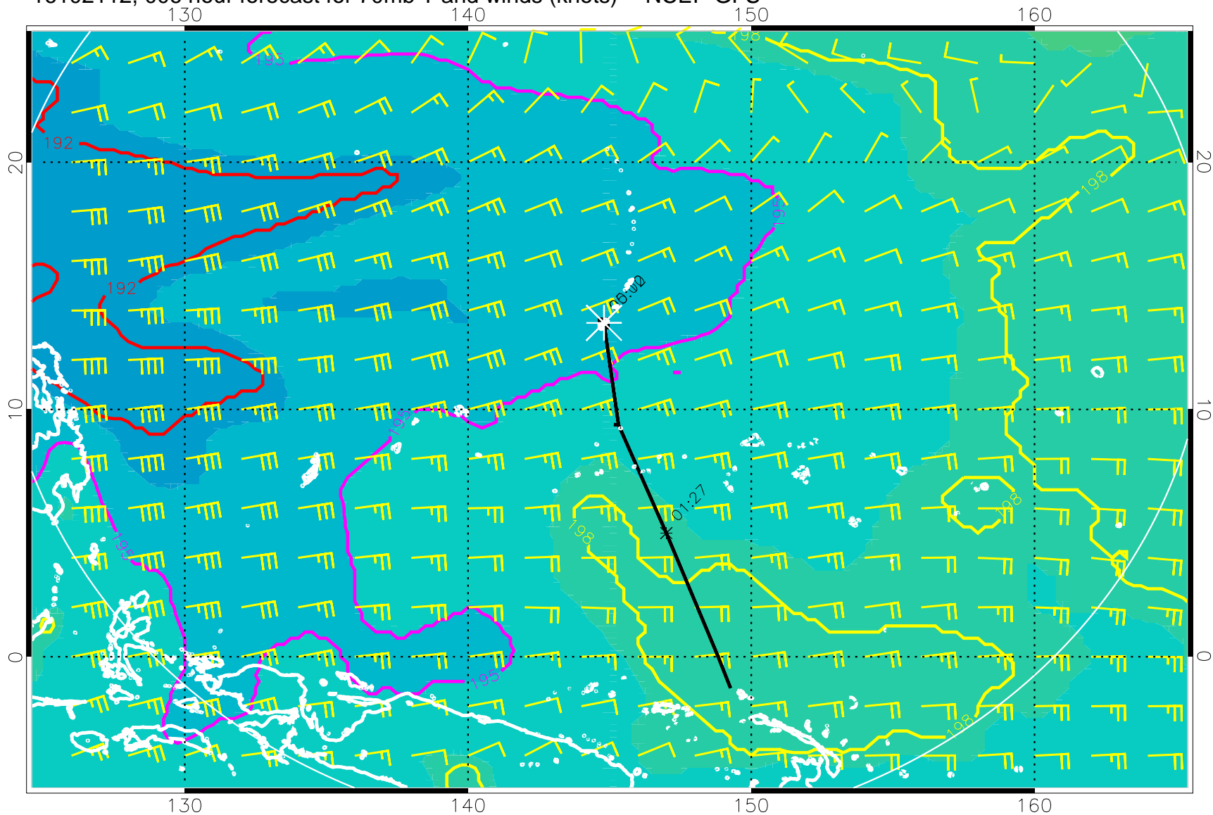
16102112, 006 hour forecast for 70mb T and winds (knots) -- NCEP GFS
