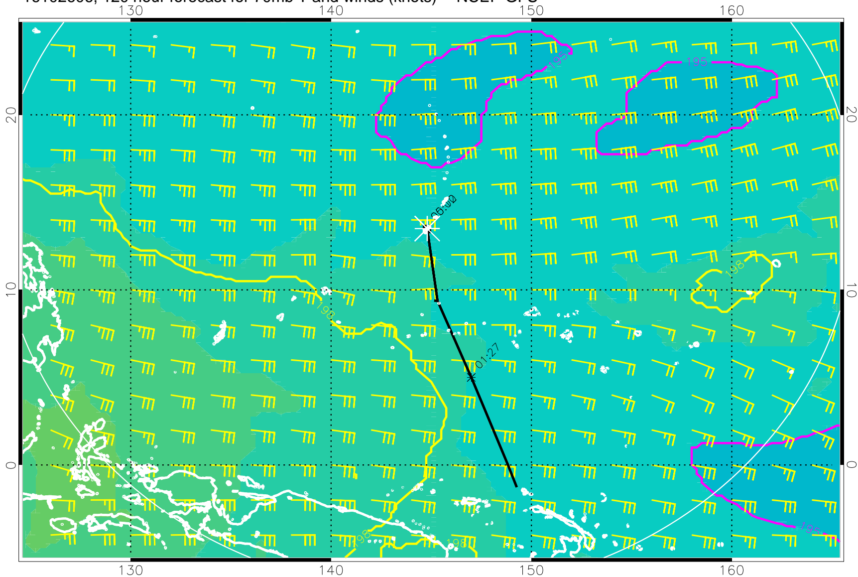
16102606, 120 hour forecast for 70mb T and winds (knots) -- NCEP GFS
