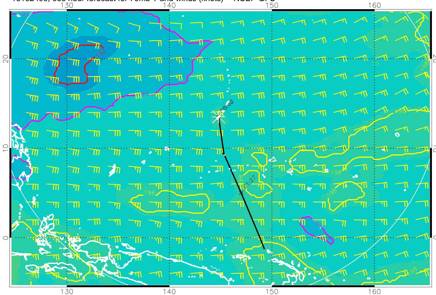
16102400, 066 hour forecast for 70mb T and winds (knots) -- NCEP GFS
