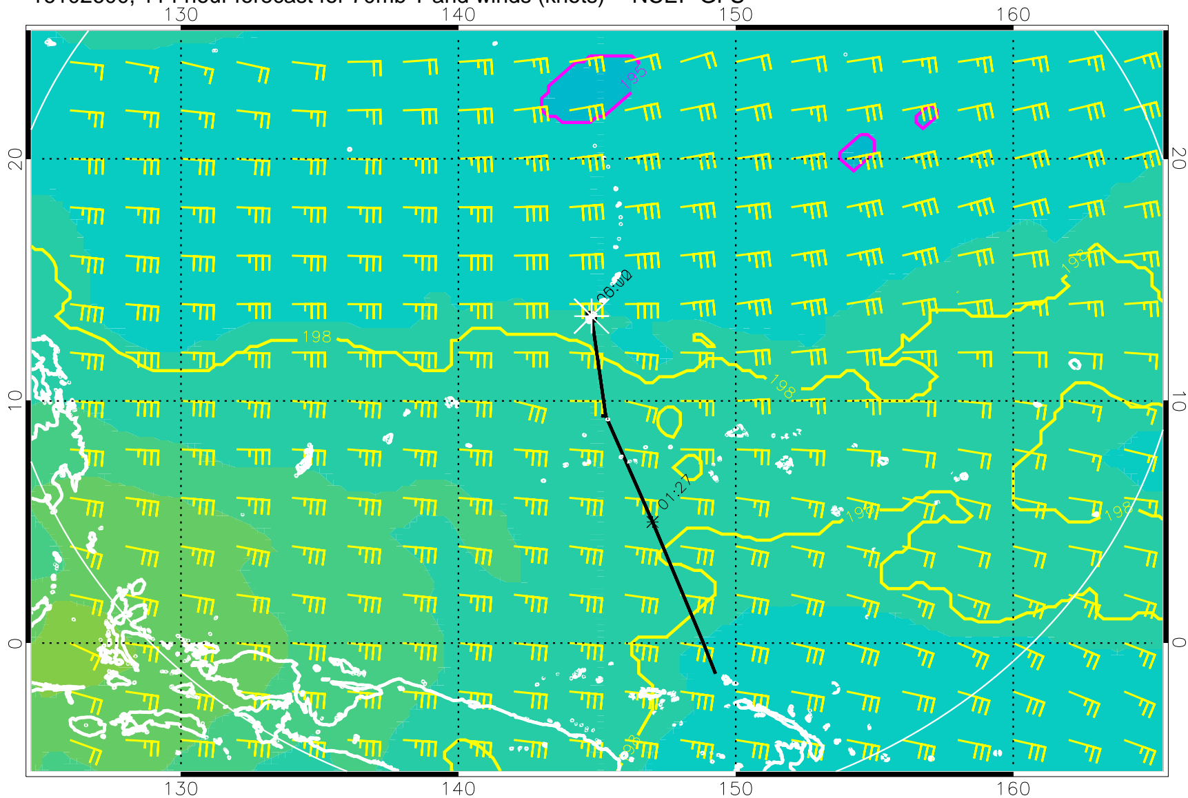
16102600, 114 hour forecast for 70mb T and winds (knots) -- NCEP GFS
