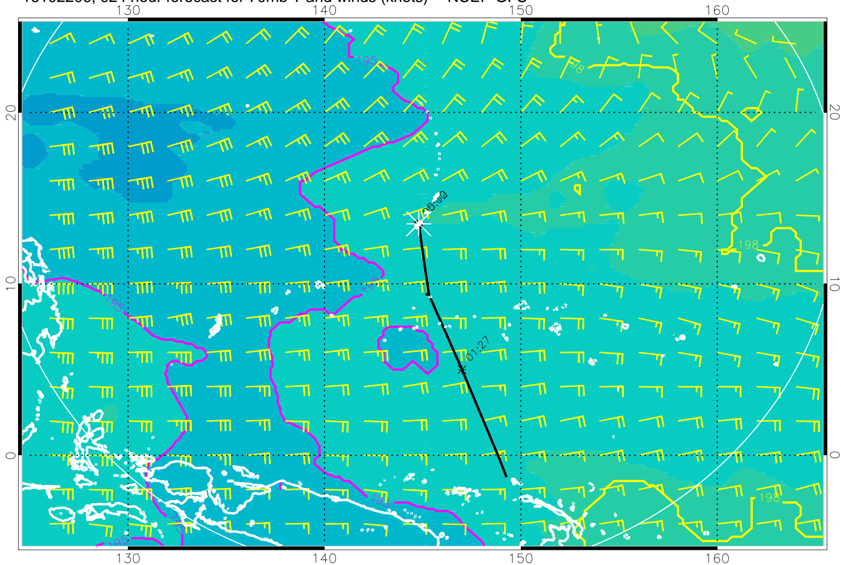
16102206, 024 hour forecast for 70mb T and winds (knots) -- NCEP GFS
