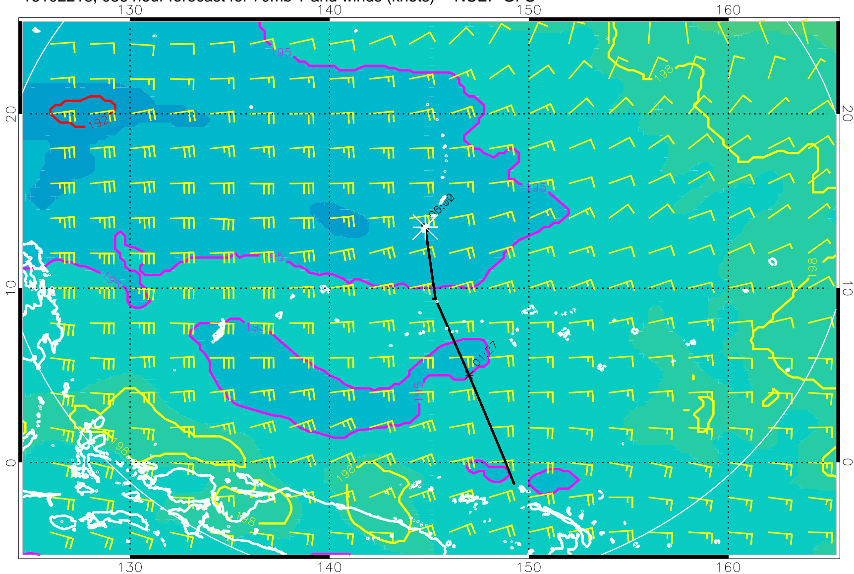
16102218, 036 hour forecast for 70mb T and winds (knots) -- NCEP GFS
