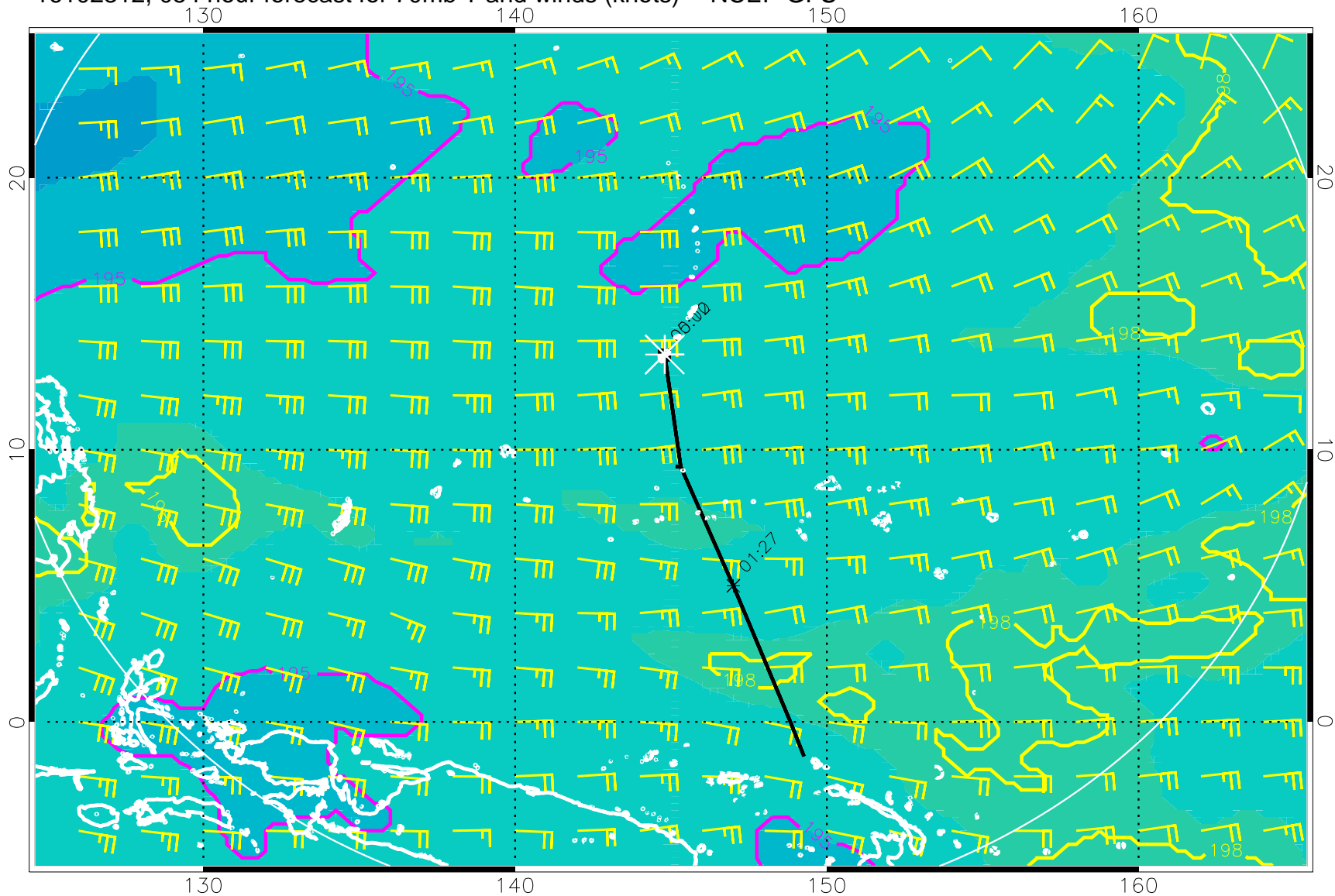
16102312, 054 hour forecast for 70mb T and winds (knots) -- NCEP GFS
