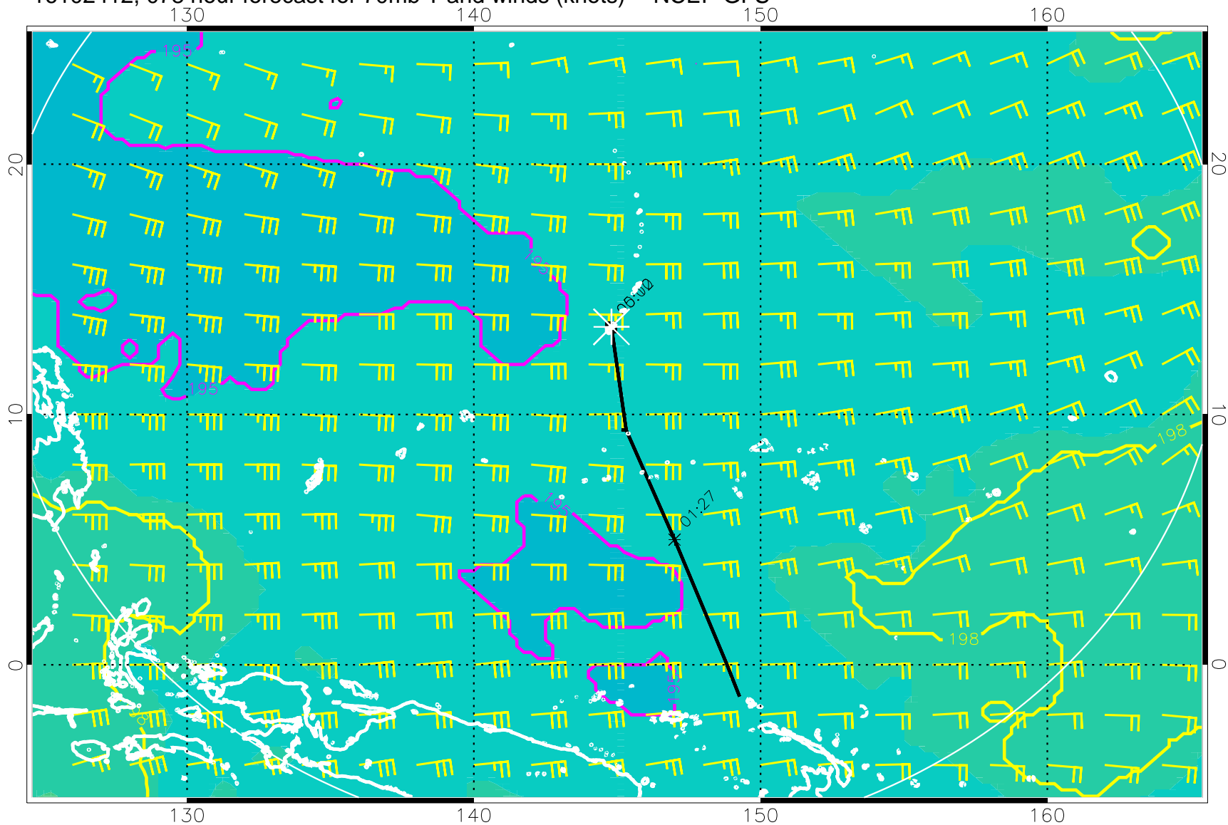
16102412, 078 hour forecast for 70mb T and winds (knots) -- NCEP GFS
