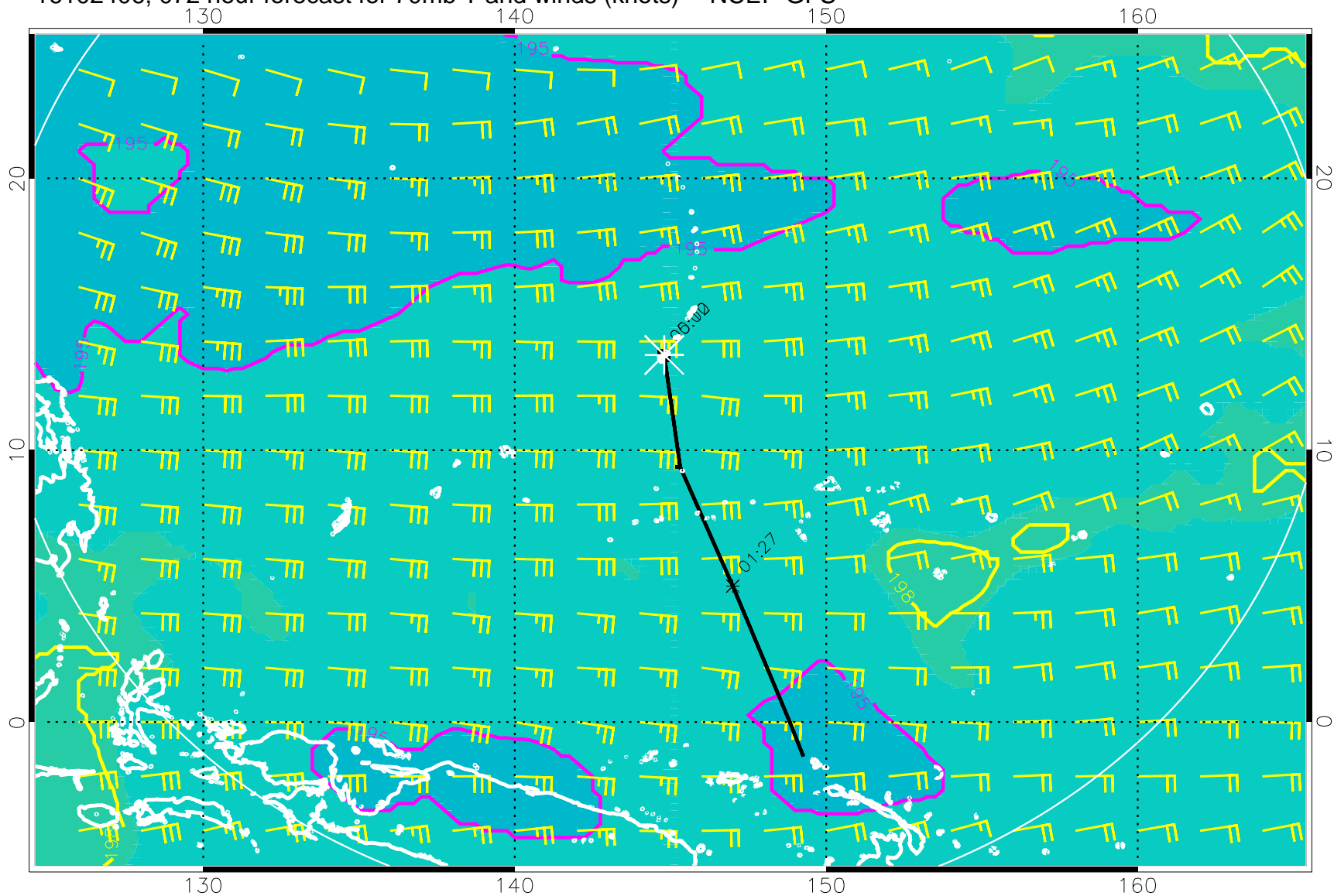
16102406, 072 hour forecast for 70mb T and winds (knots) -- NCEP GFS
