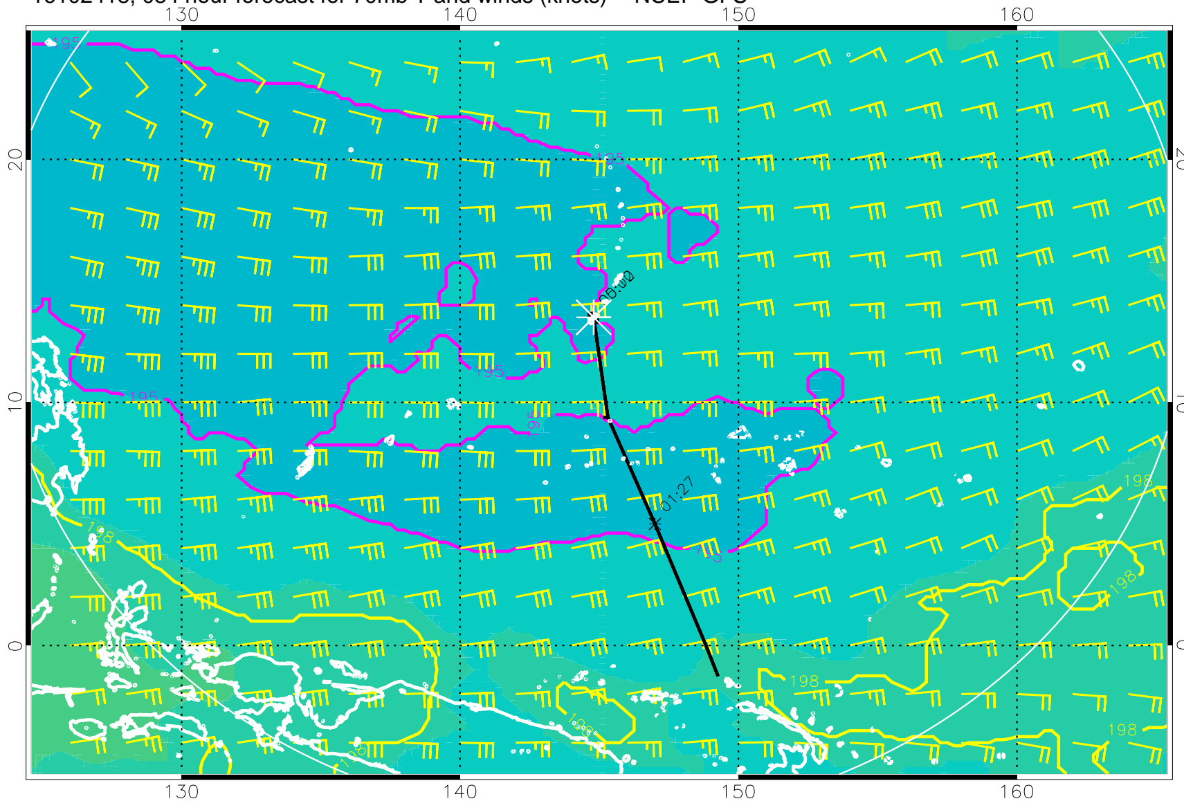
16102418, 084 hour forecast for 70mb T and winds (knots) -- NCEP GFS
