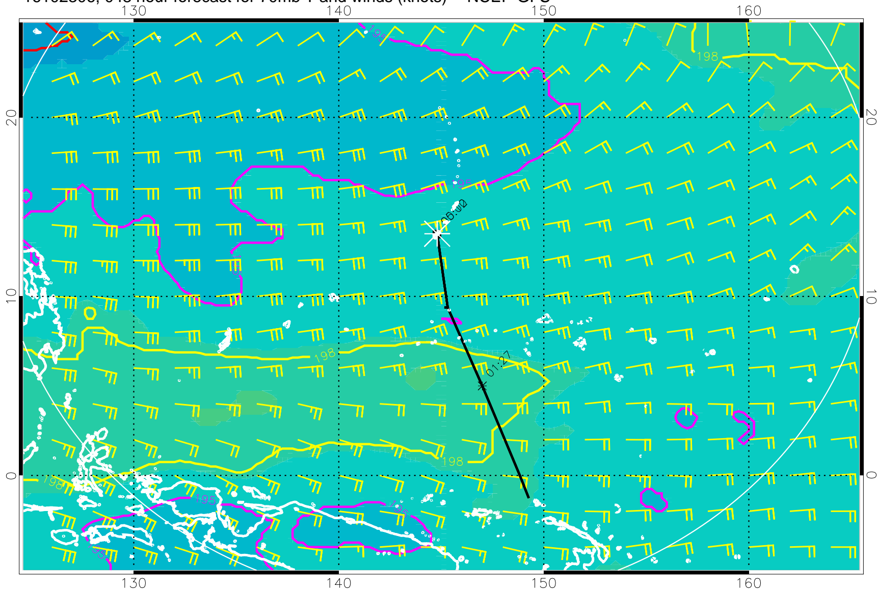
16102306, 048 hour forecast for 70mb T and winds (knots) -- NCEP GFS
