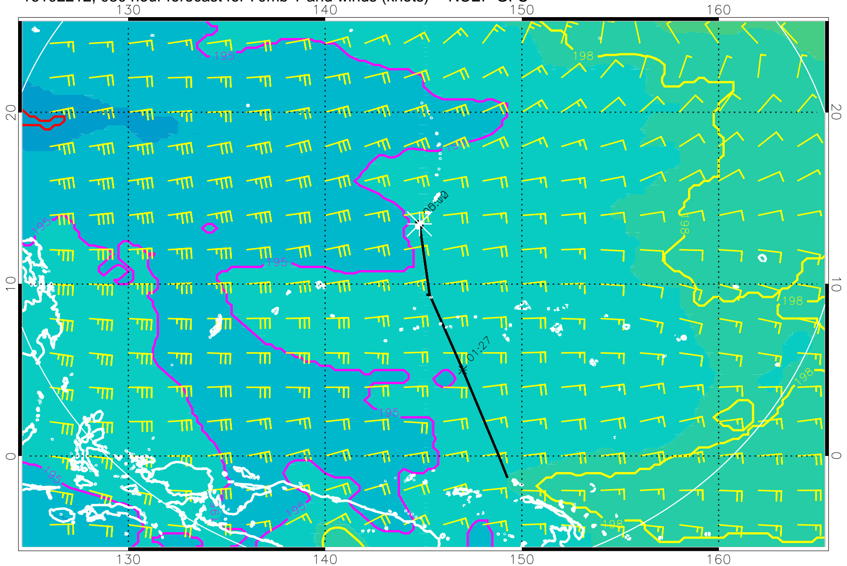
16102212, 030 hour forecast for 70mb T and winds (knots) -- NCEP GFS
