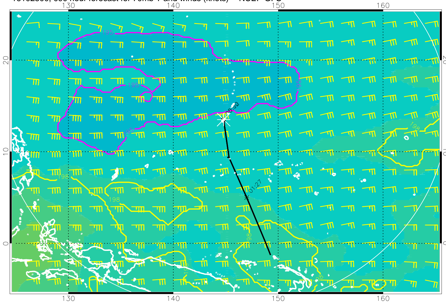
16102500, 090 hour forecast for 70mb T and winds (knots) -- NCEP GFS
