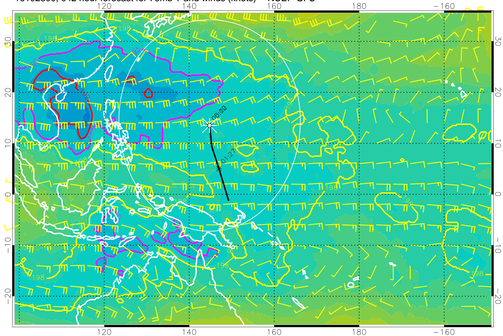
16102300, 042 hour forecast for 70mb T and winds (knots) -- NCEP GFS
