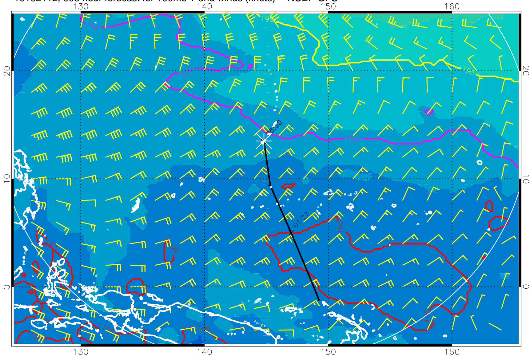
16102112, 006 hour forecast for 100mb T and winds (knots) -- NCEP GFS
