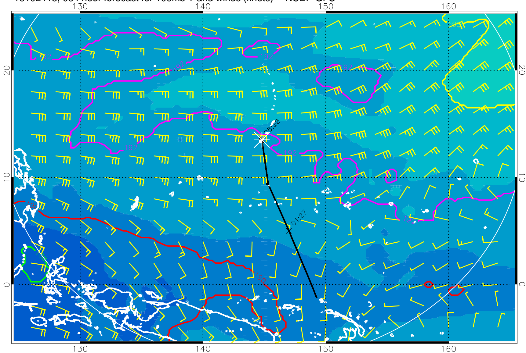
16102418, 084 hour forecast for 100mb T and winds (knots) -- NCEP GFS
