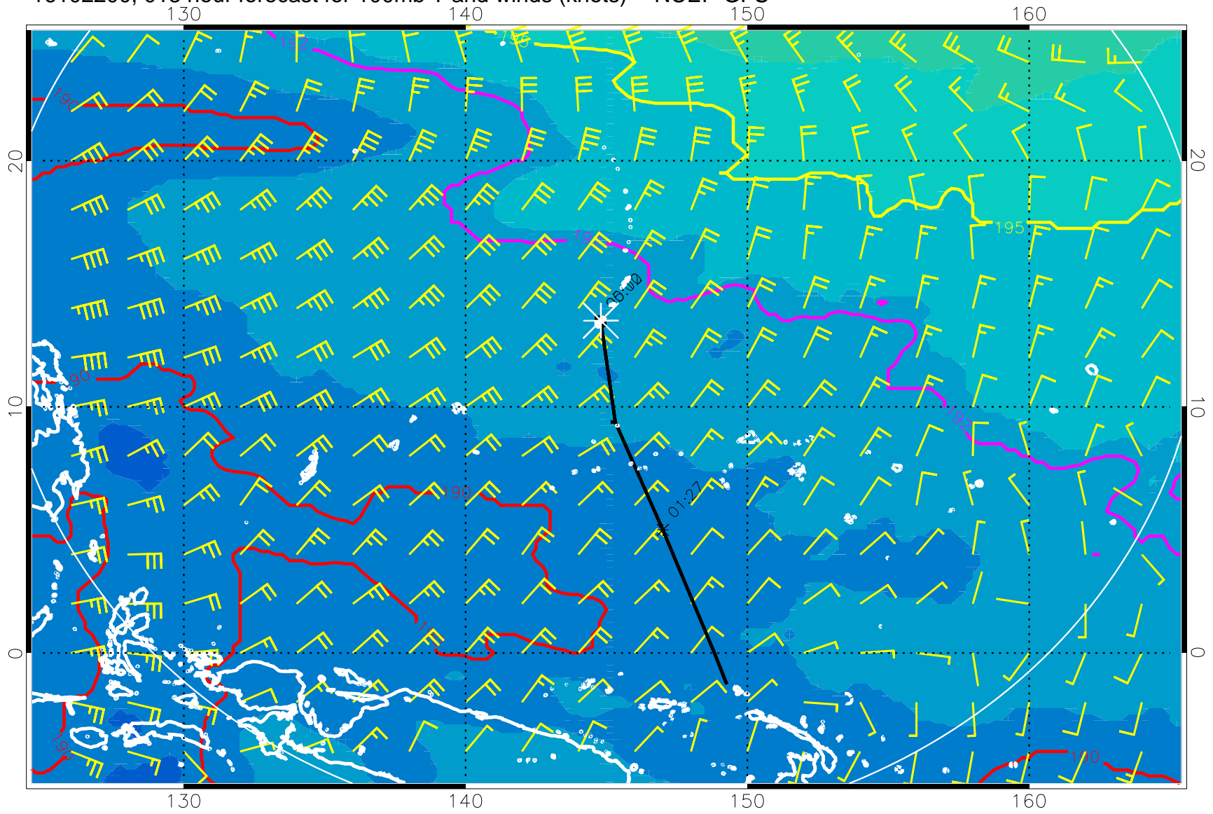
16102200, 018 hour forecast for 100mb T and winds (knots) -- NCEP GFS
