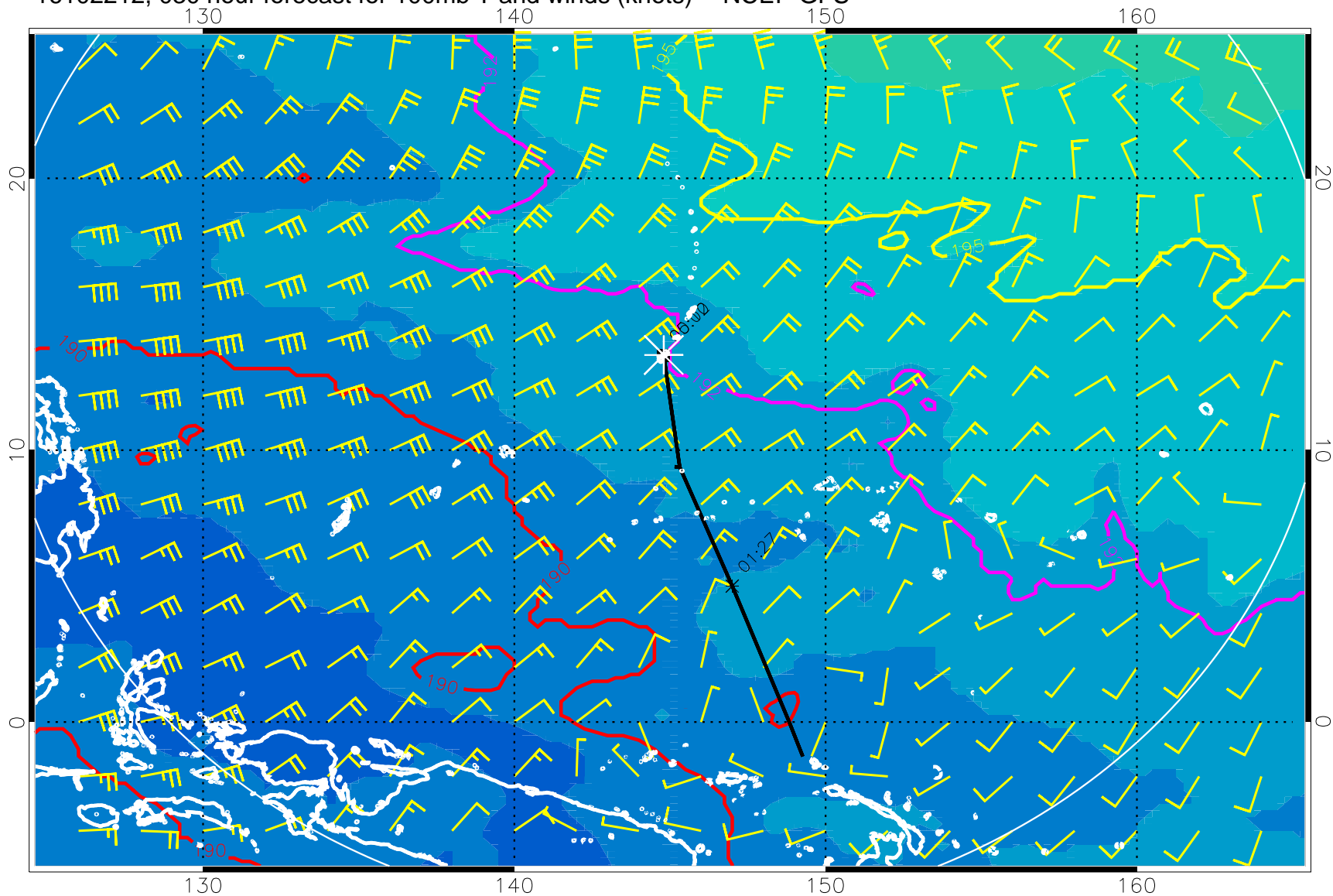
16102212, 030 hour forecast for 100mb T and winds (knots) -- NCEP GFS
