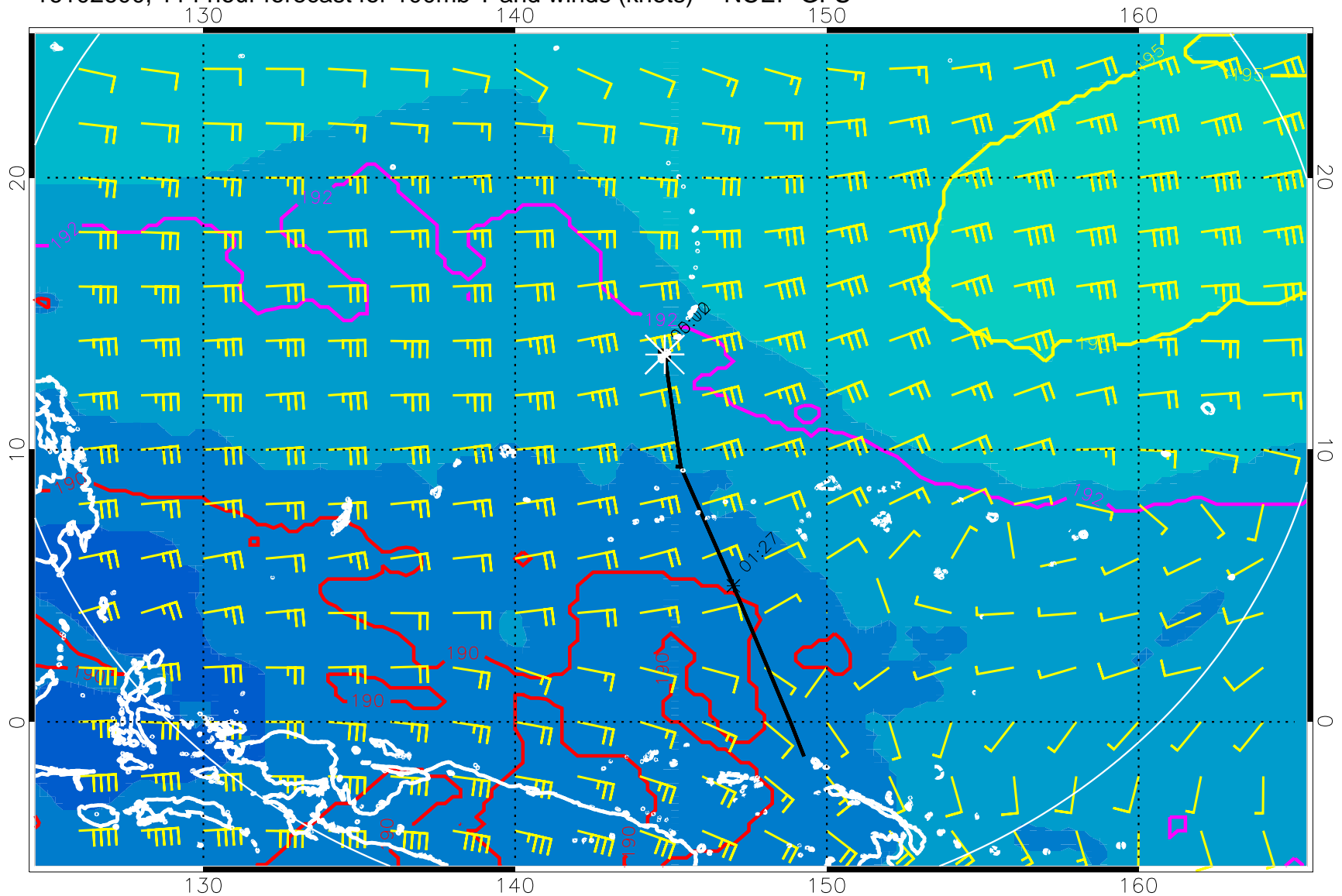
16102600, 114 hour forecast for 100mb T and winds (knots) -- NCEP GFS
