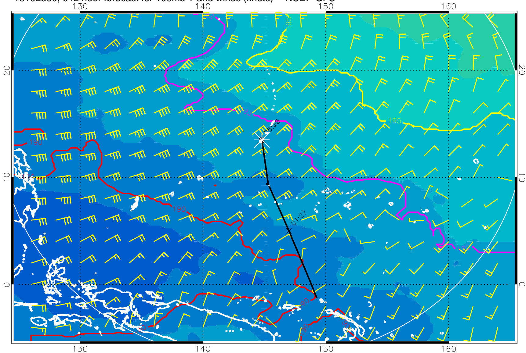
16102300, 042 hour forecast for 100mb T and winds (knots) -- NCEP GFS
