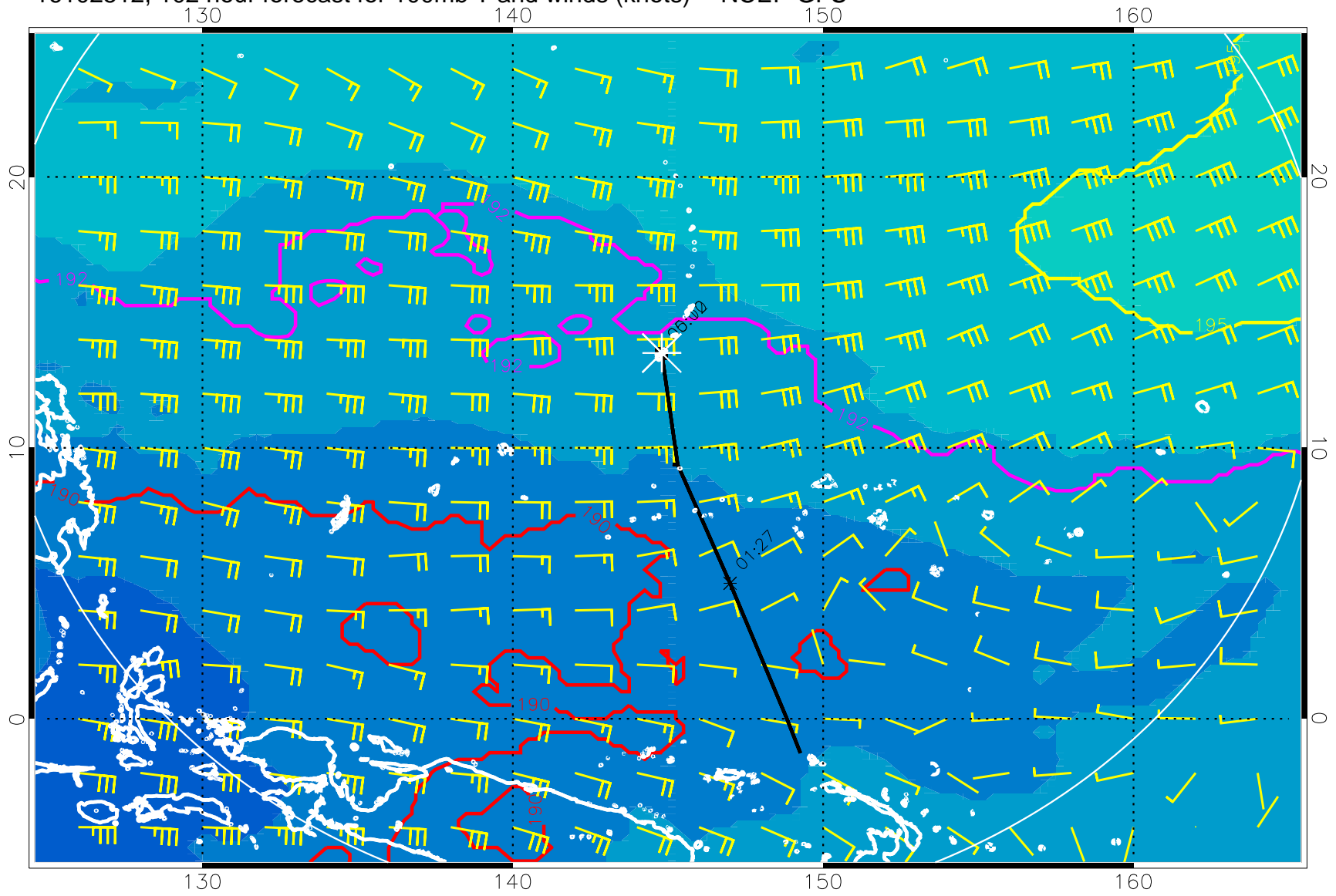
16102512, 102 hour forecast for 100mb T and winds (knots) -- NCEP GFS
