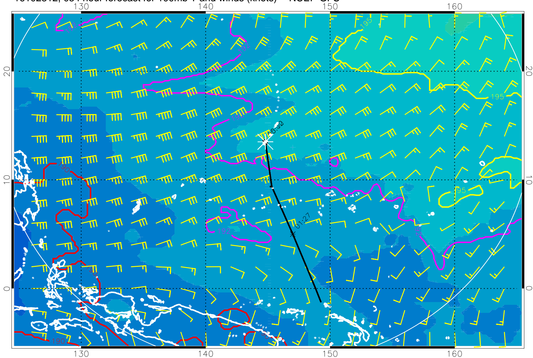
16102312, 054 hour forecast for 100mb T and winds (knots) -- NCEP GFS
