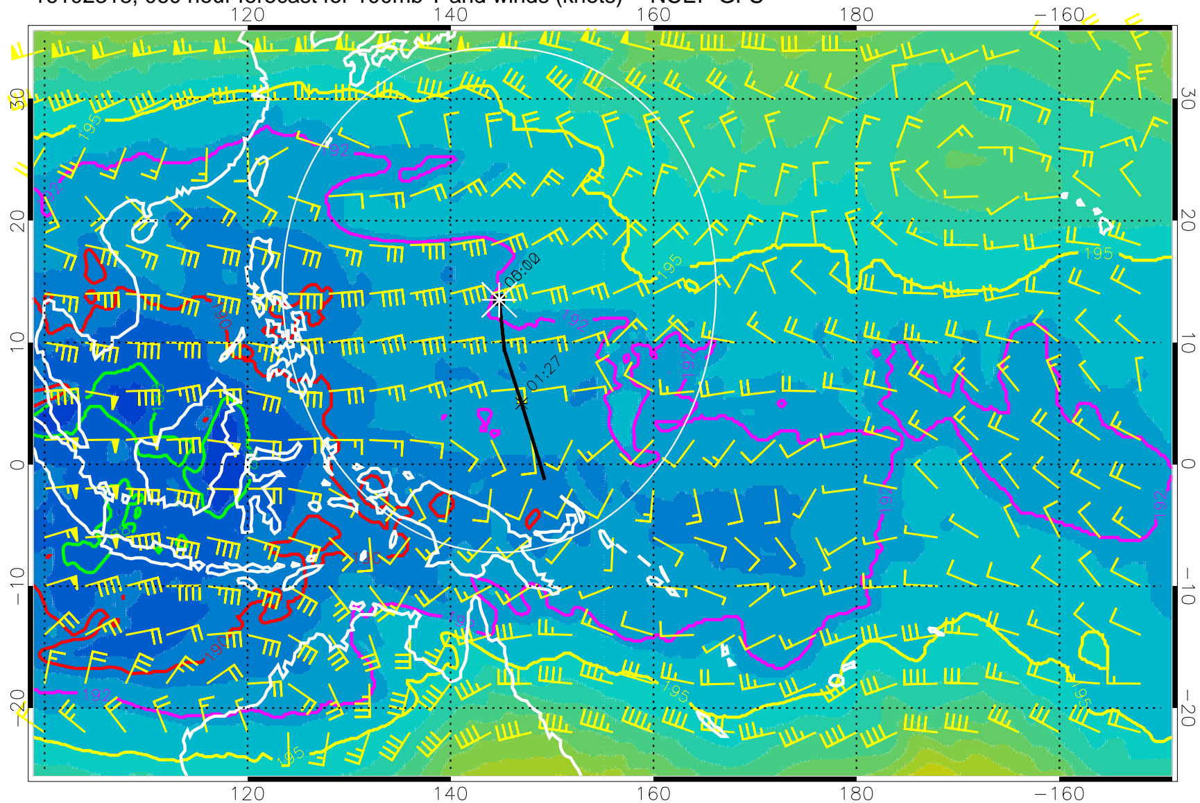
16102318, 060 hour forecast for 100mb T and winds (knots) -- NCEP GFS
