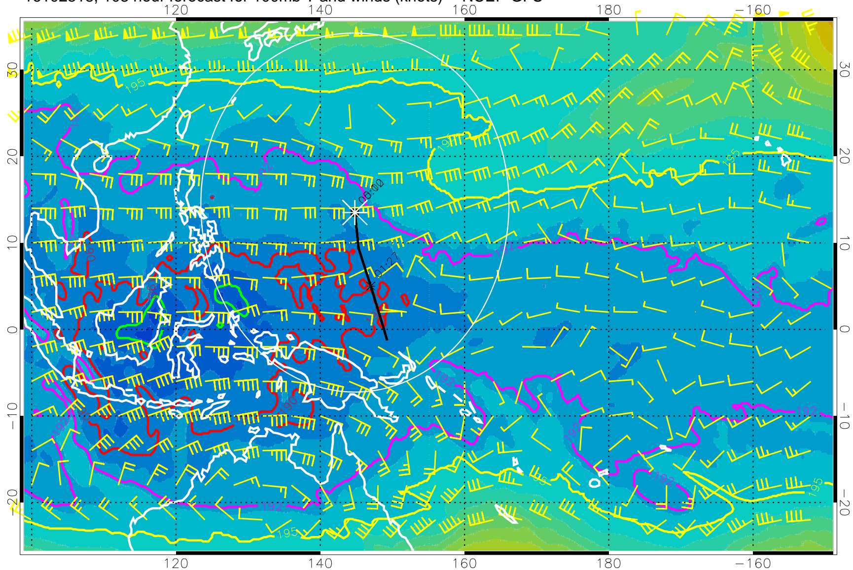
16102518, 108 hour forecast for 100mb T and winds (knots) -- NCEP GFS
