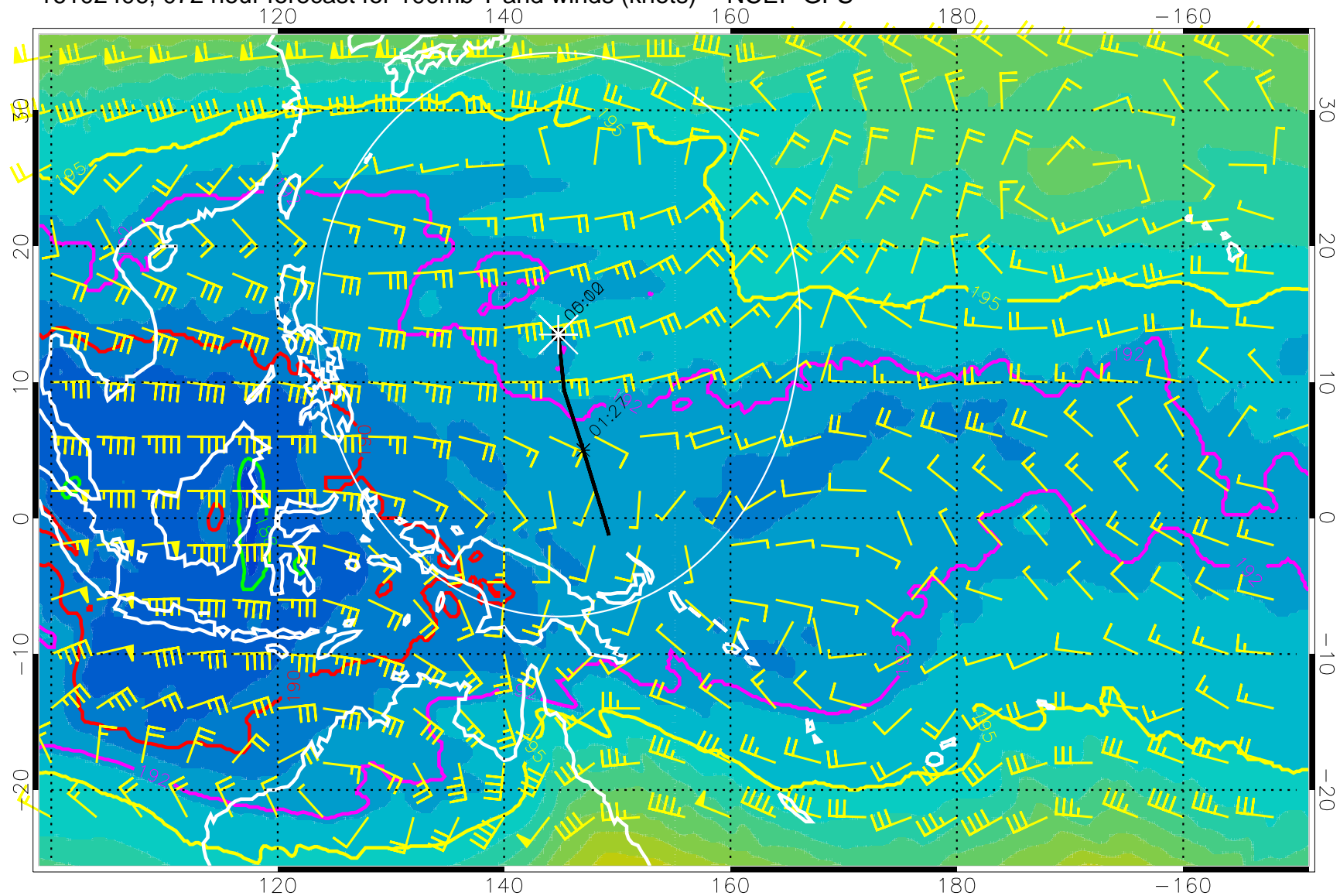
16102406, 072 hour forecast for 100mb T and winds (knots) -- NCEP GFS
