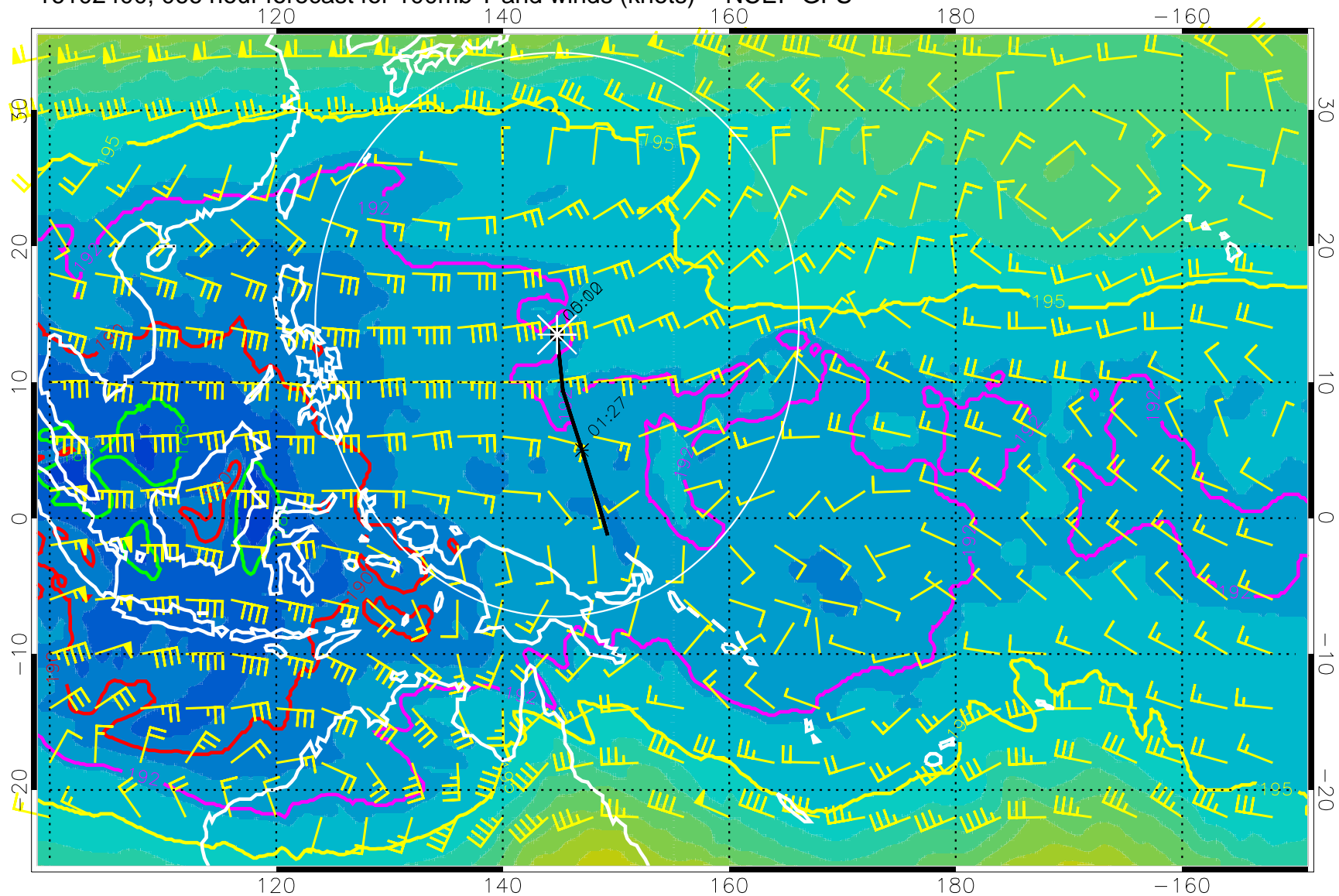
16102400, 066 hour forecast for 100mb T and winds (knots) -- NCEP GFS
