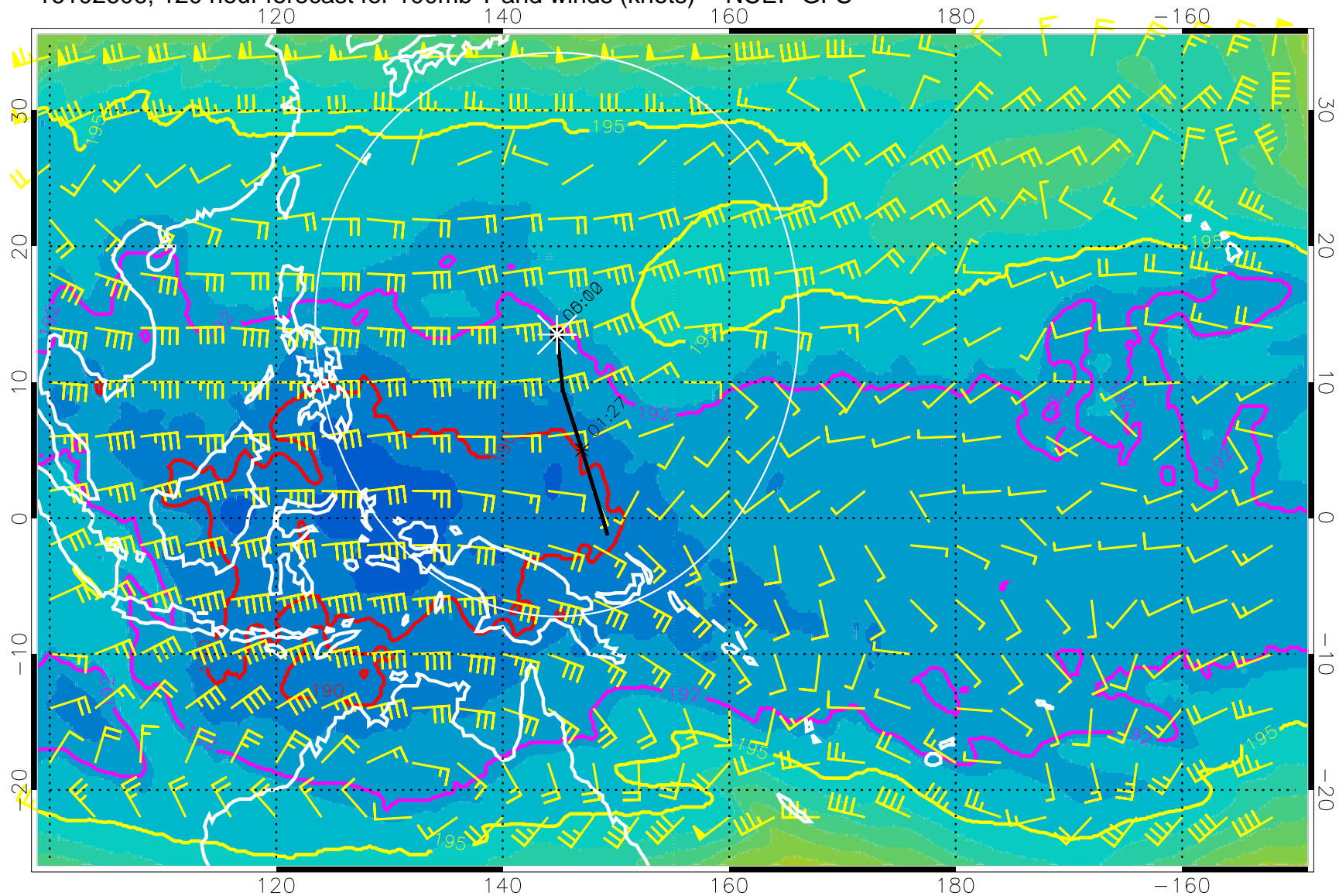
16102606, 120 hour forecast for 100mb T and winds (knots) -- NCEP GFS
