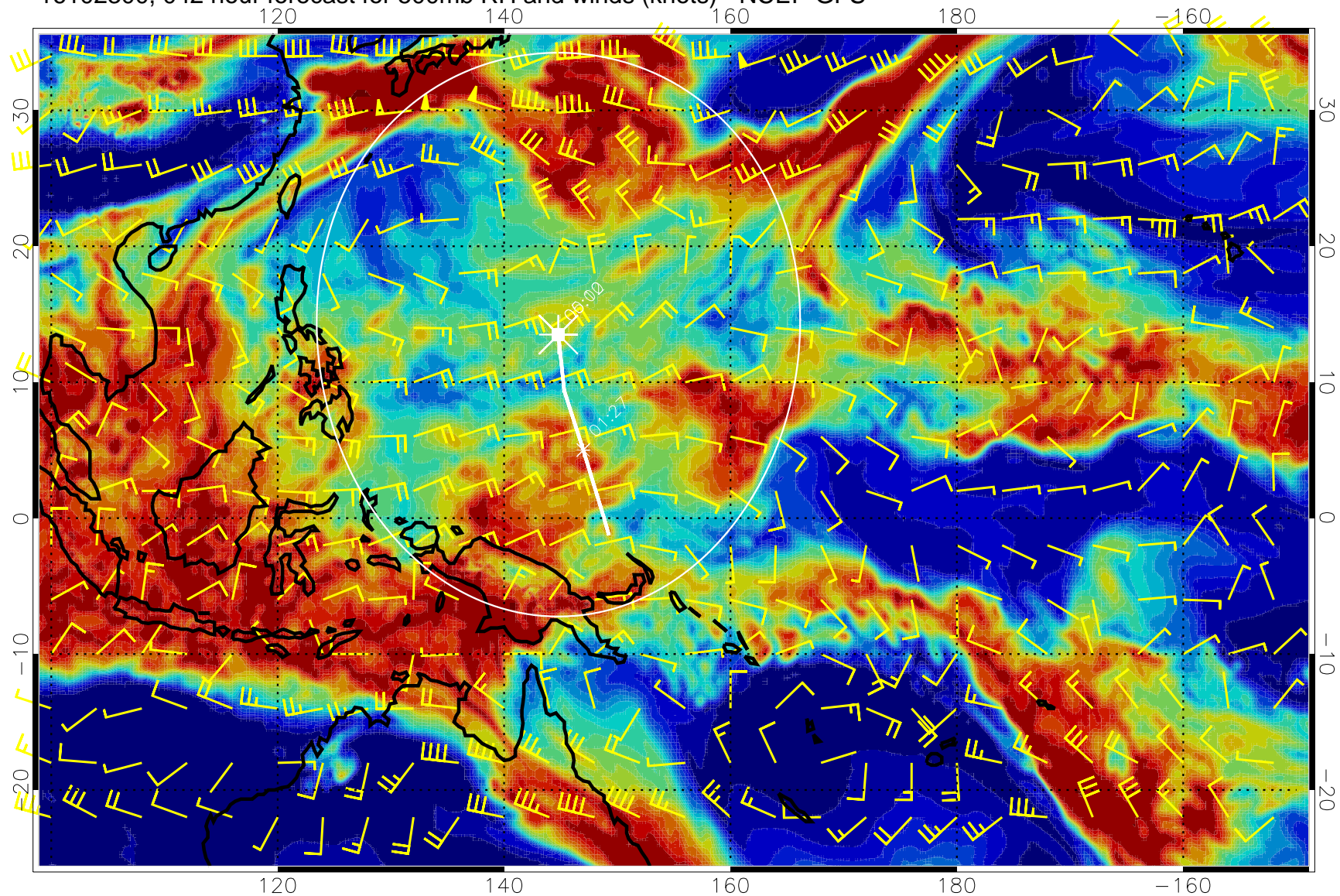
16102300, 042 hour forecast for 500mb RH and winds (knots) - NCEP GFS
