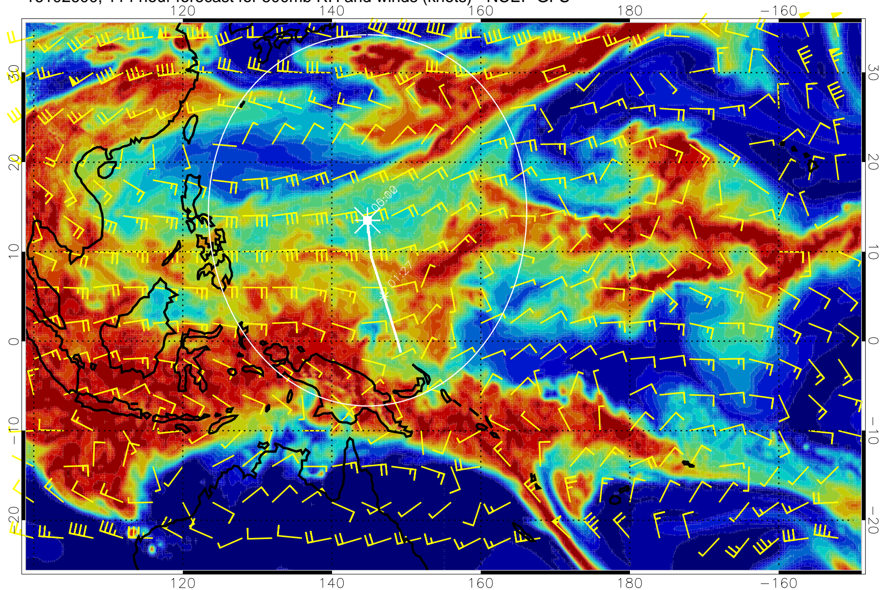
16102600, 114 hour forecast for 500mb RH and winds (knots) - NCEP GFS
