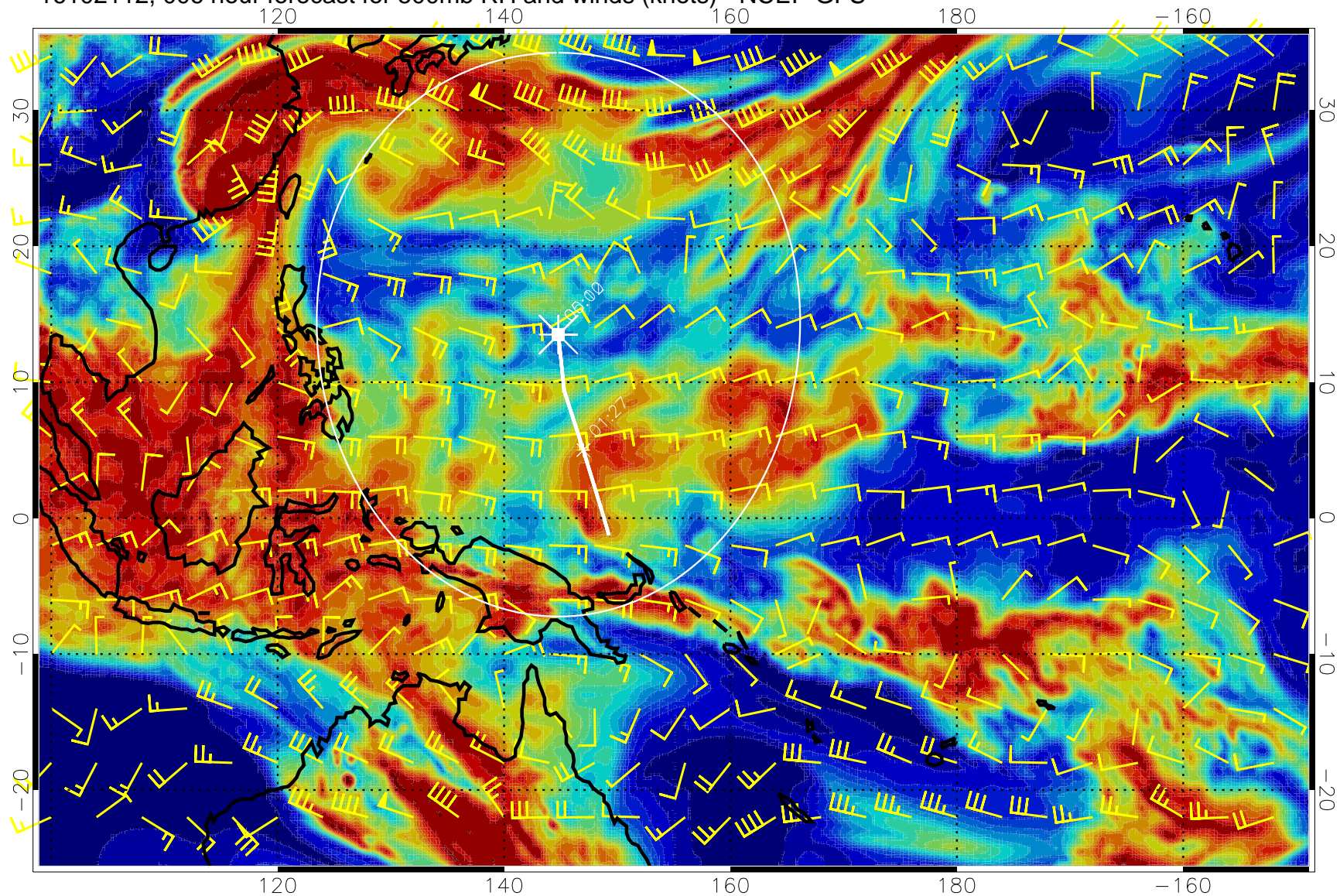
16102112, 006 hour forecast for 500mb RH and winds (knots) - NCEP GFS
