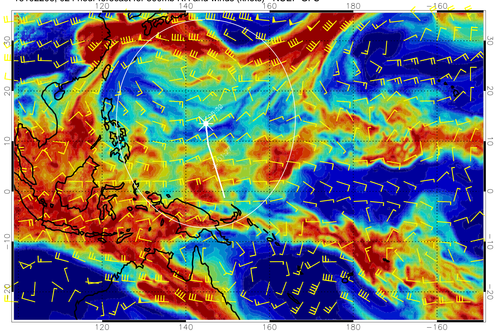
16102206, 024 hour forecast for 500mb RH and winds (knots) - NCEP GFS
