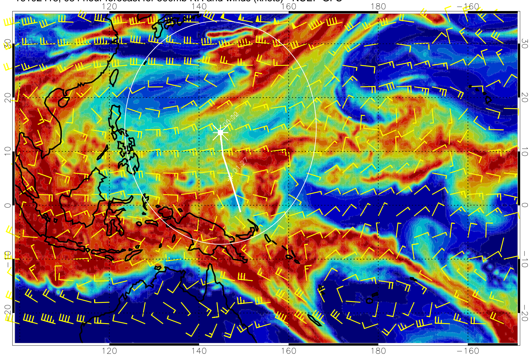
16102418, 084 hour forecast for 500mb RH and winds (knots) - NCEP GFS
