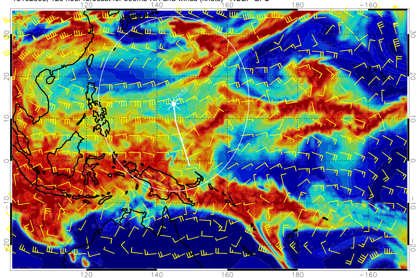
16102606, 120 hour forecast for 500mb RH and winds (knots) - NCEP GFS
