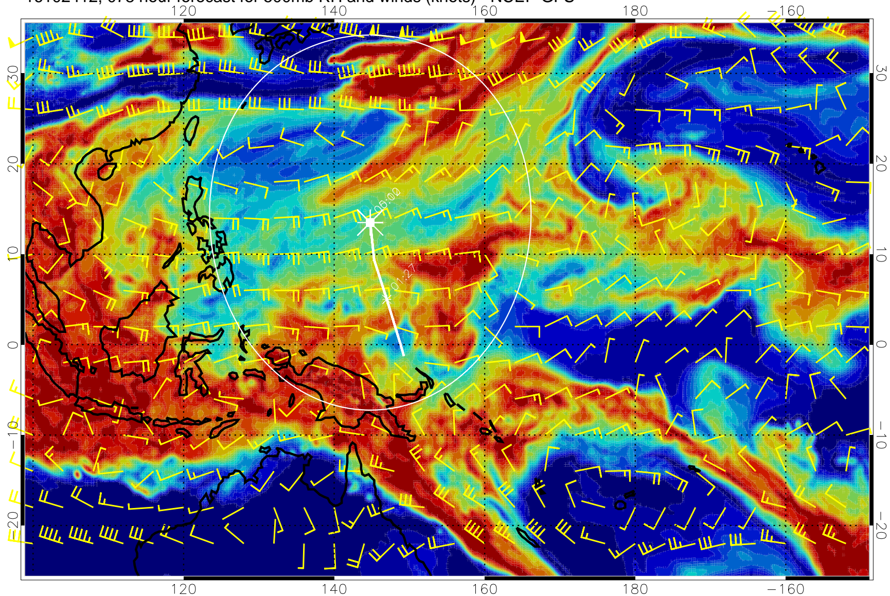
16102412, 078 hour forecast for 500mb RH and winds (knots) - NCEP GFS
