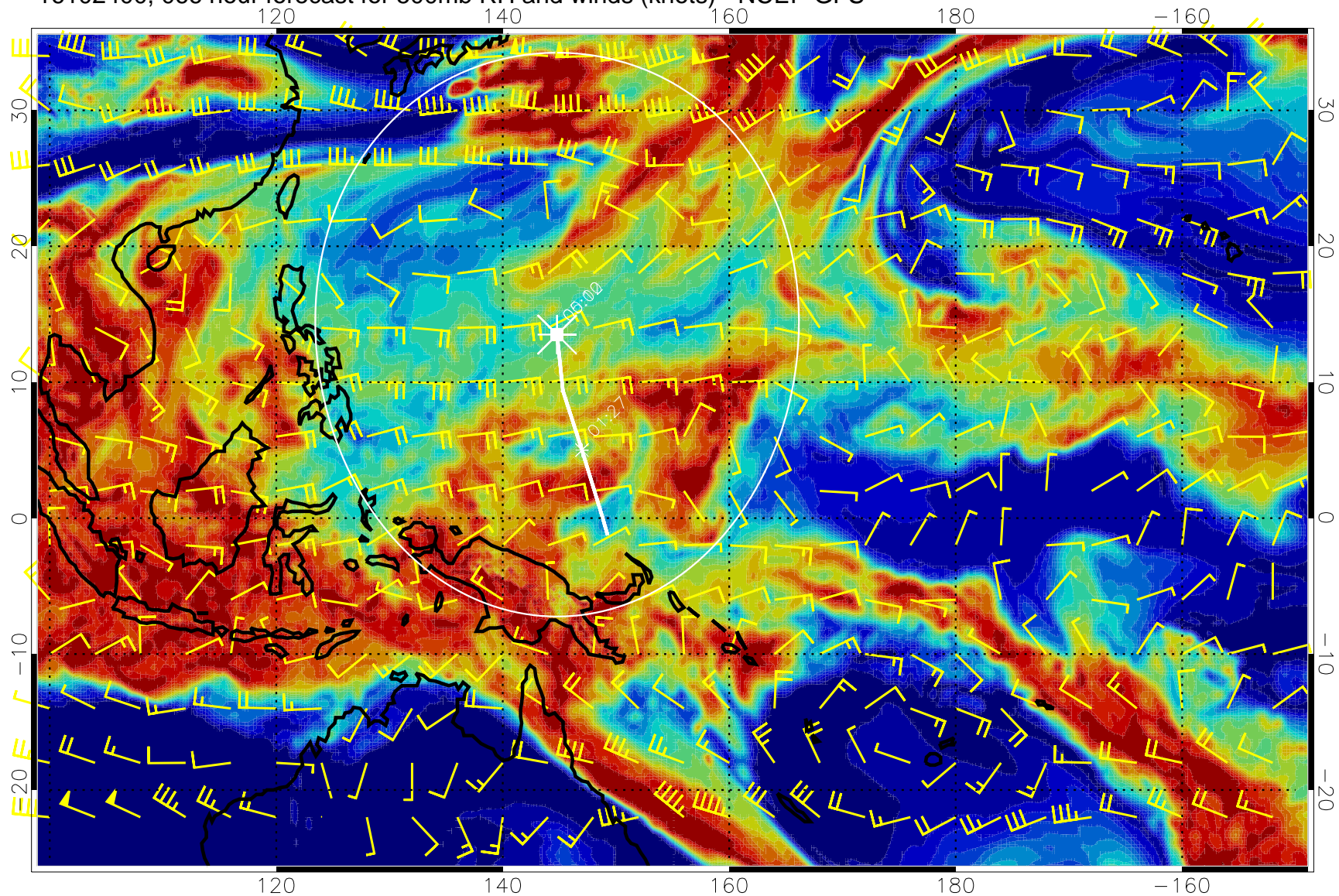
16102400, 066 hour forecast for 500mb RH and winds (knots) - NCEP GFS
