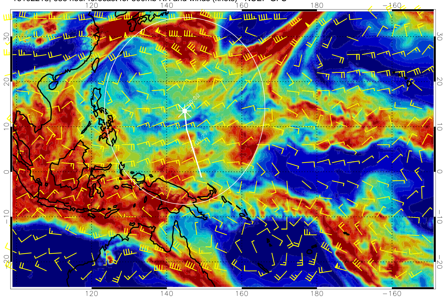
16102218, 036 hour forecast for 500mb RH and winds (knots) - NCEP GFS
