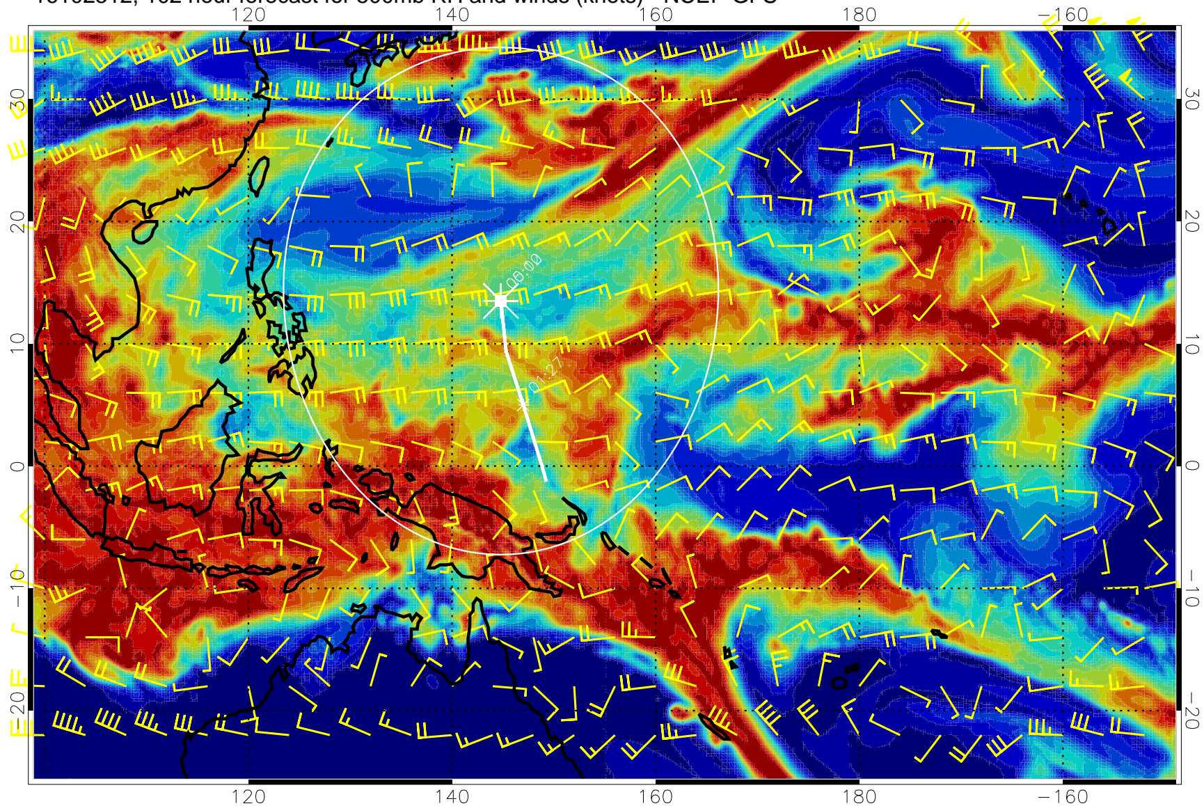
16102512, 102 hour forecast for 500mb RH and winds (knots) - NCEP GFS
