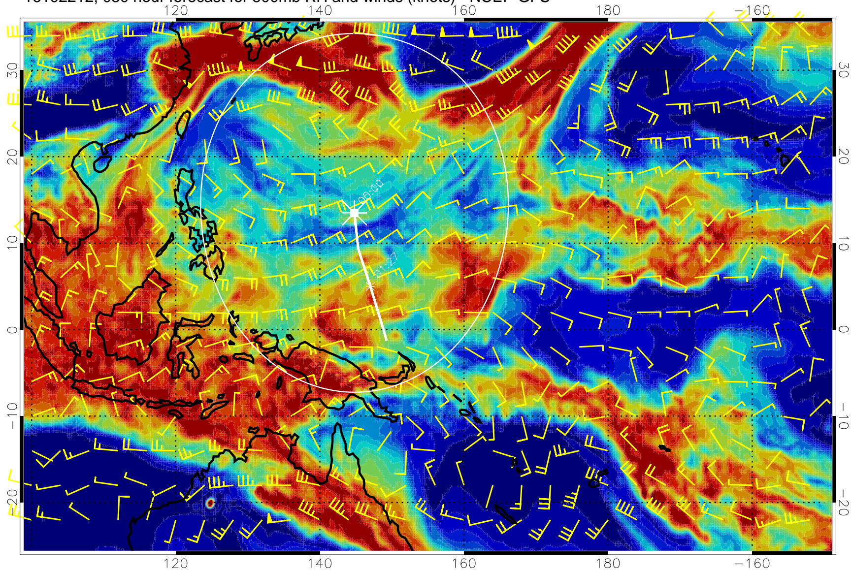
16102212, 030 hour forecast for 500mb RH and winds (knots) - NCEP GFS
