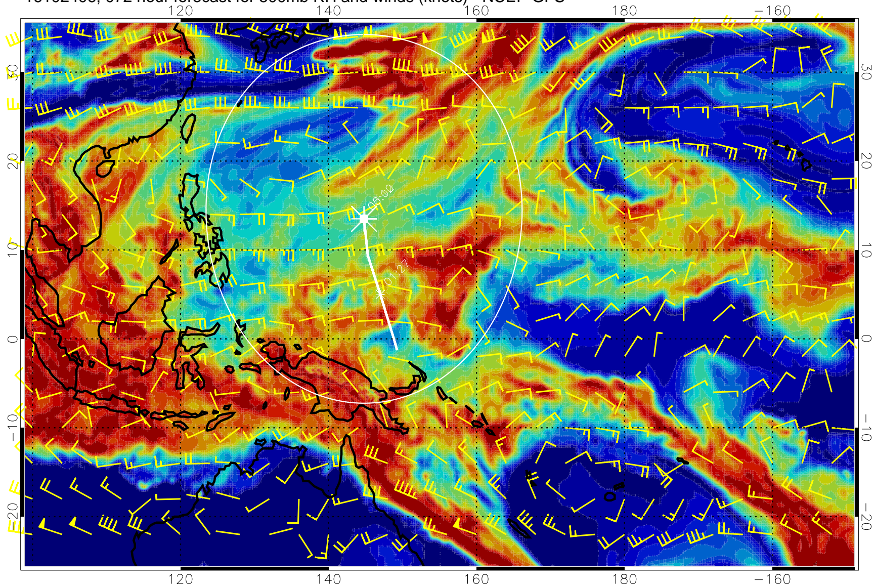
16102406, 072 hour forecast for 500mb RH and winds (knots) - NCEP GFS
