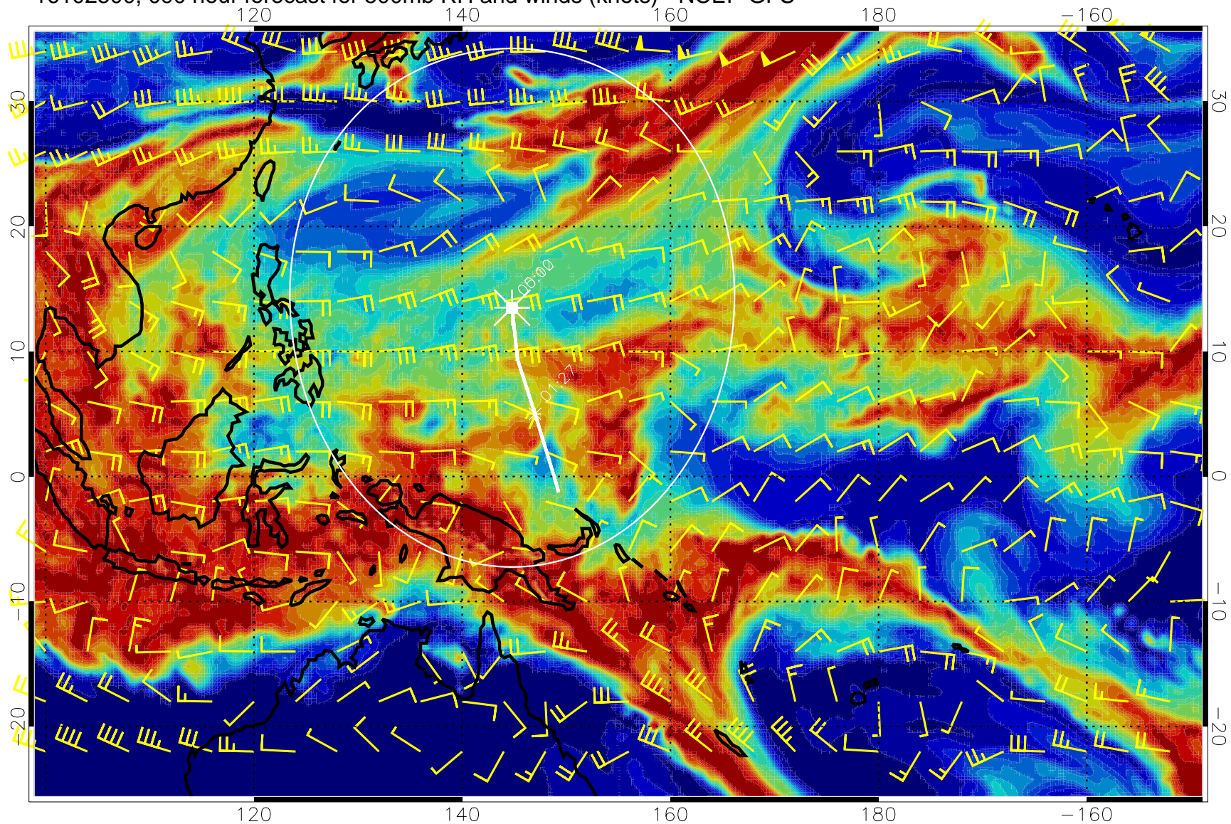
16102500, 090 hour forecast for 500mb RH and winds (knots) - NCEP GFS
