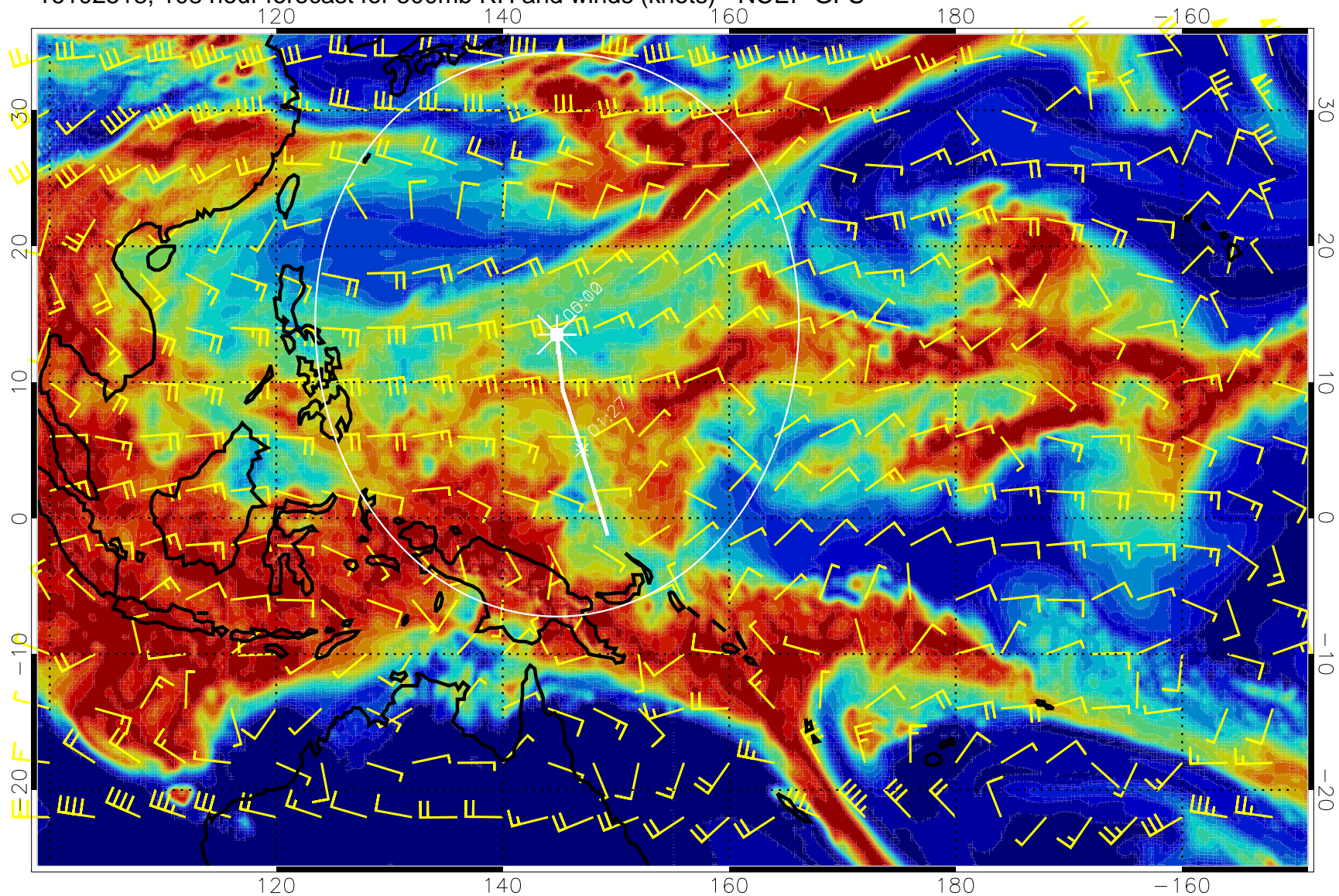
16102518, 108 hour forecast for 500mb RH and winds (knots) - NCEP GFS
