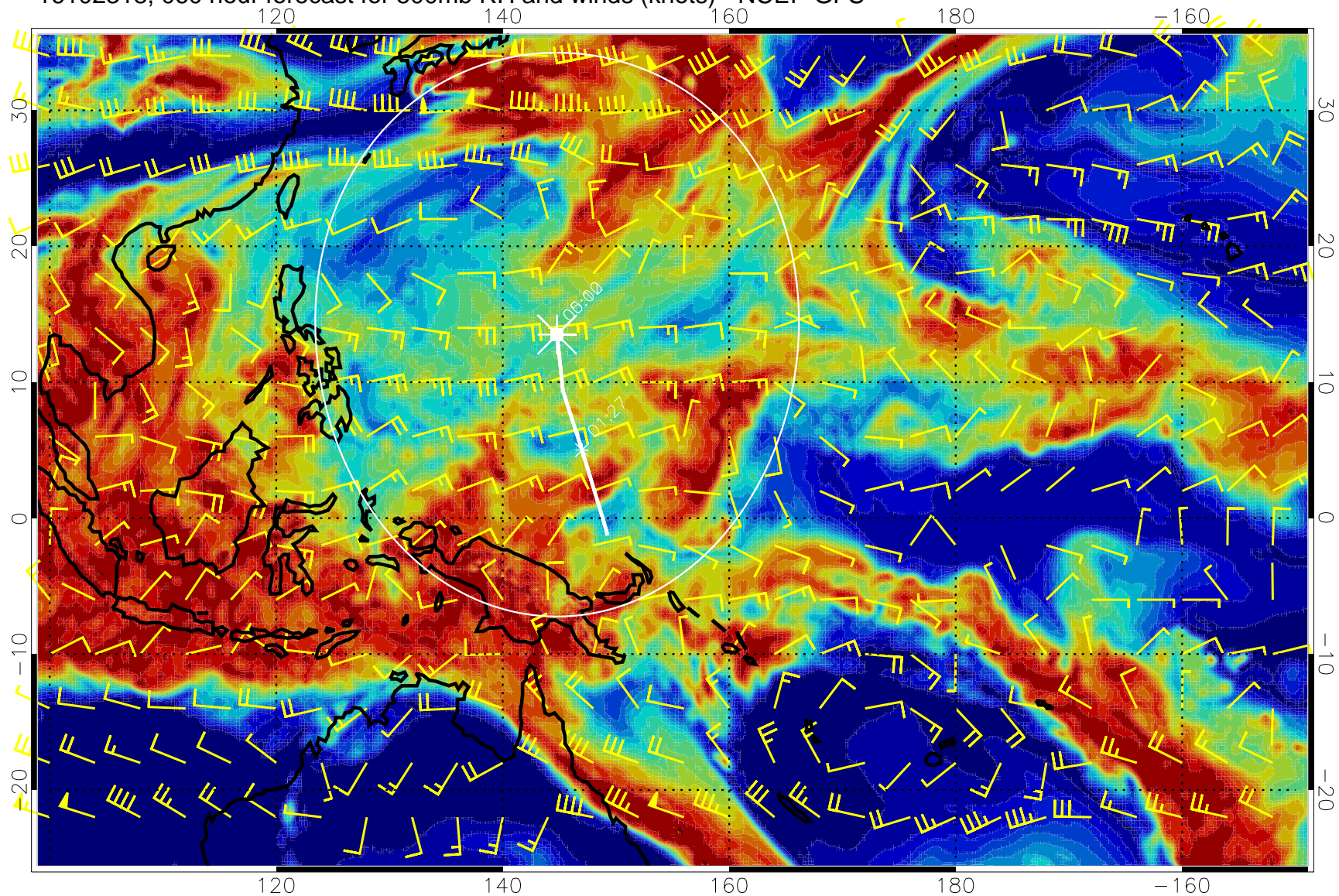
16102318, 060 hour forecast for 500mb RH and winds (knots) - NCEP GFS
