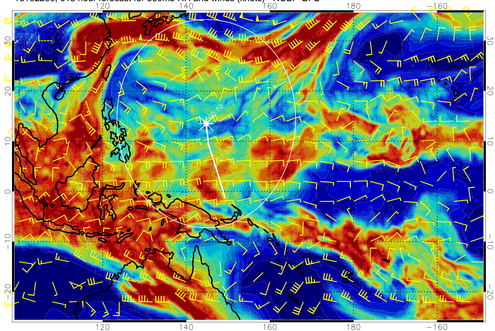
16102200, 018 hour forecast for 500mb RH and winds (knots) - NCEP GFS
