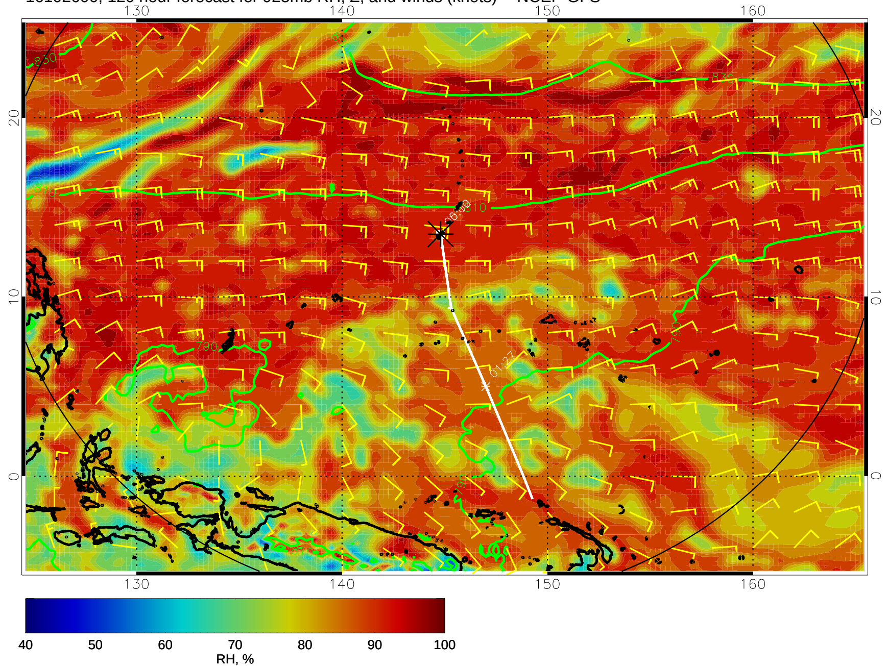
16102600, 120 hour forecast for 925mb RH, Z, and winds (knots) -- NCEP GFS
