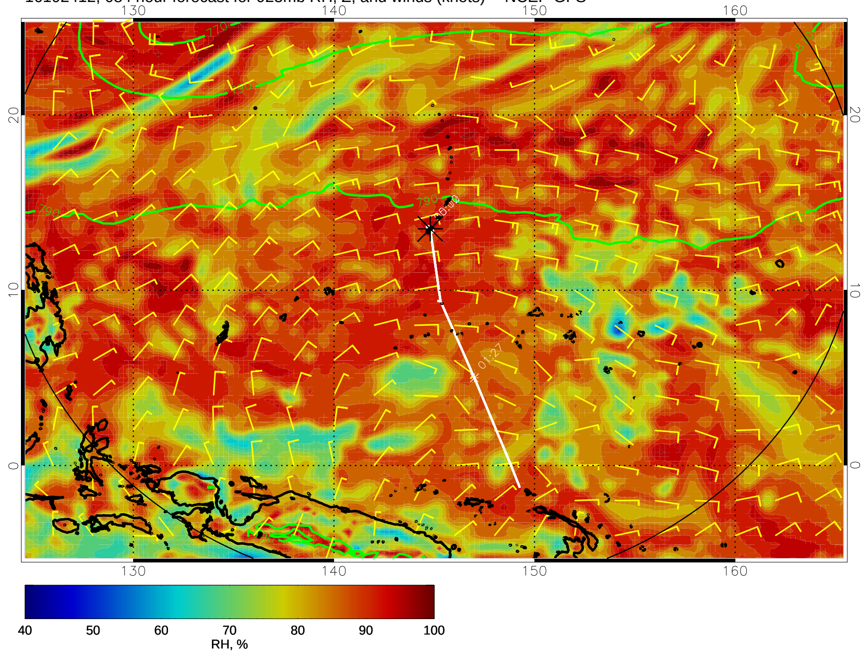
16102412, 084 hour forecast for 925mb RH, Z, and winds (knots) -- NCEP GFS
