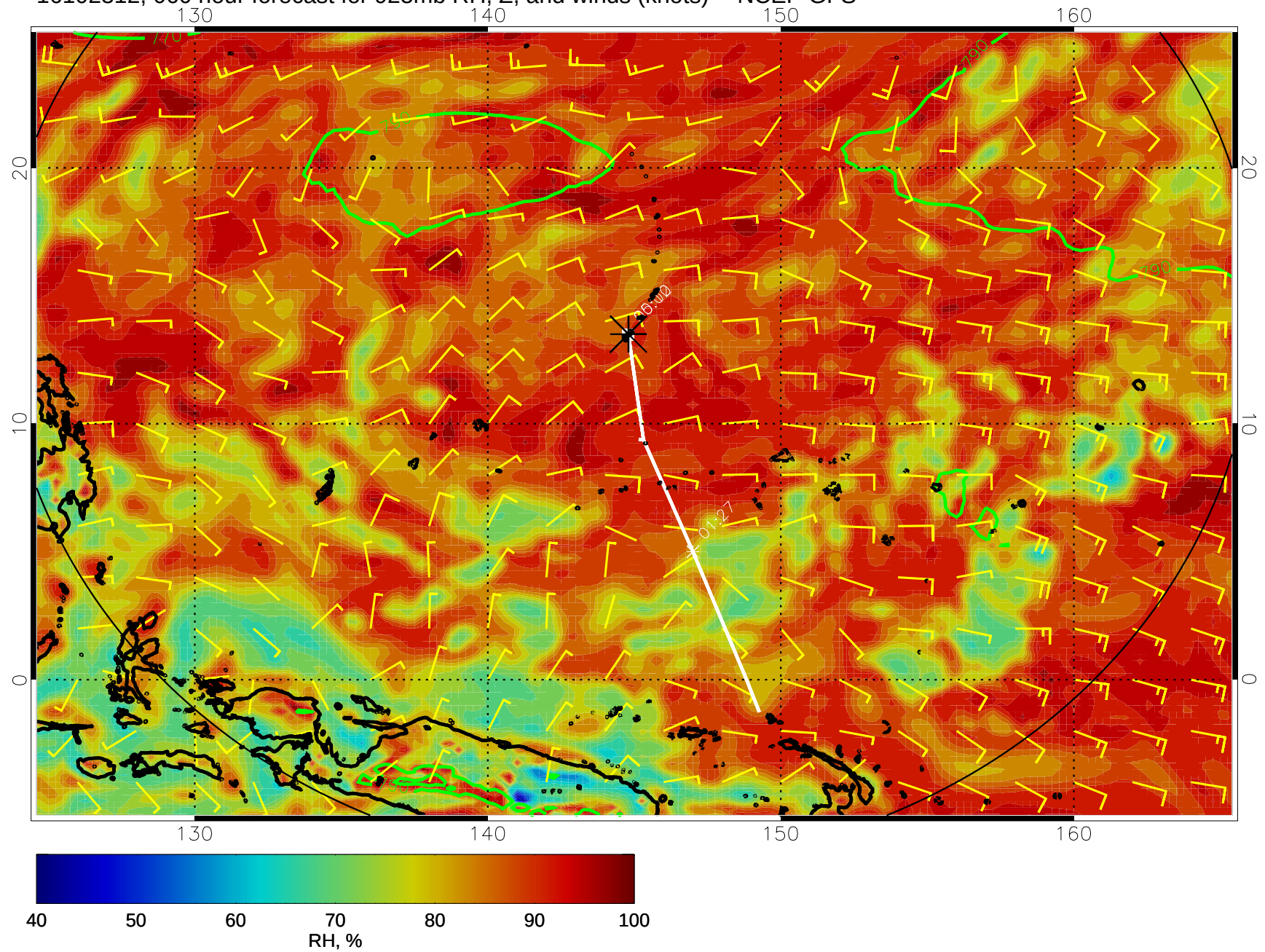
16102312, 060 hour forecast for 925mb RH, Z, and winds (knots) -- NCEP GFS
