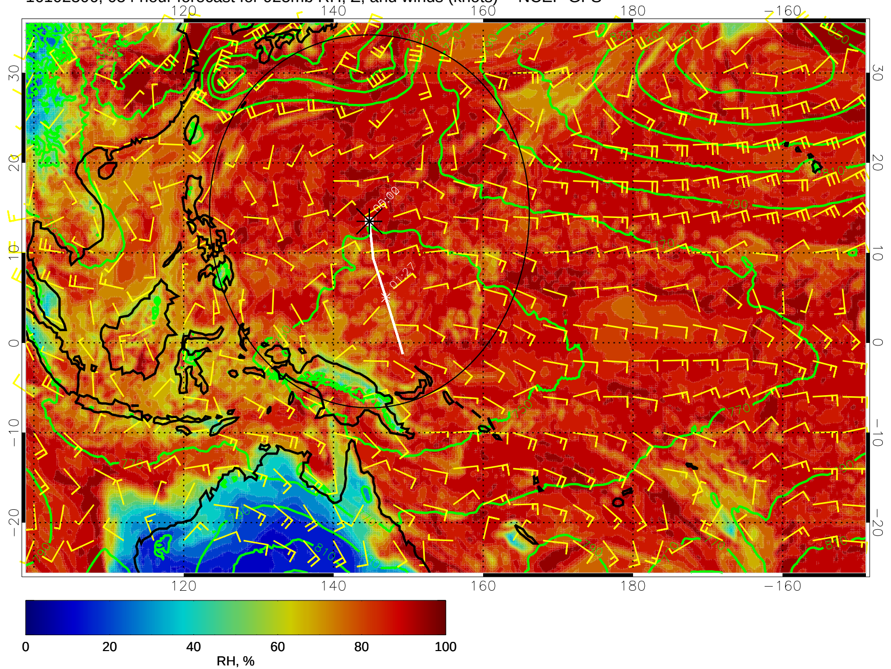
16102306, 054 hour forecast for 925mb RH, Z, and winds (knots) -- NCEP GFS
