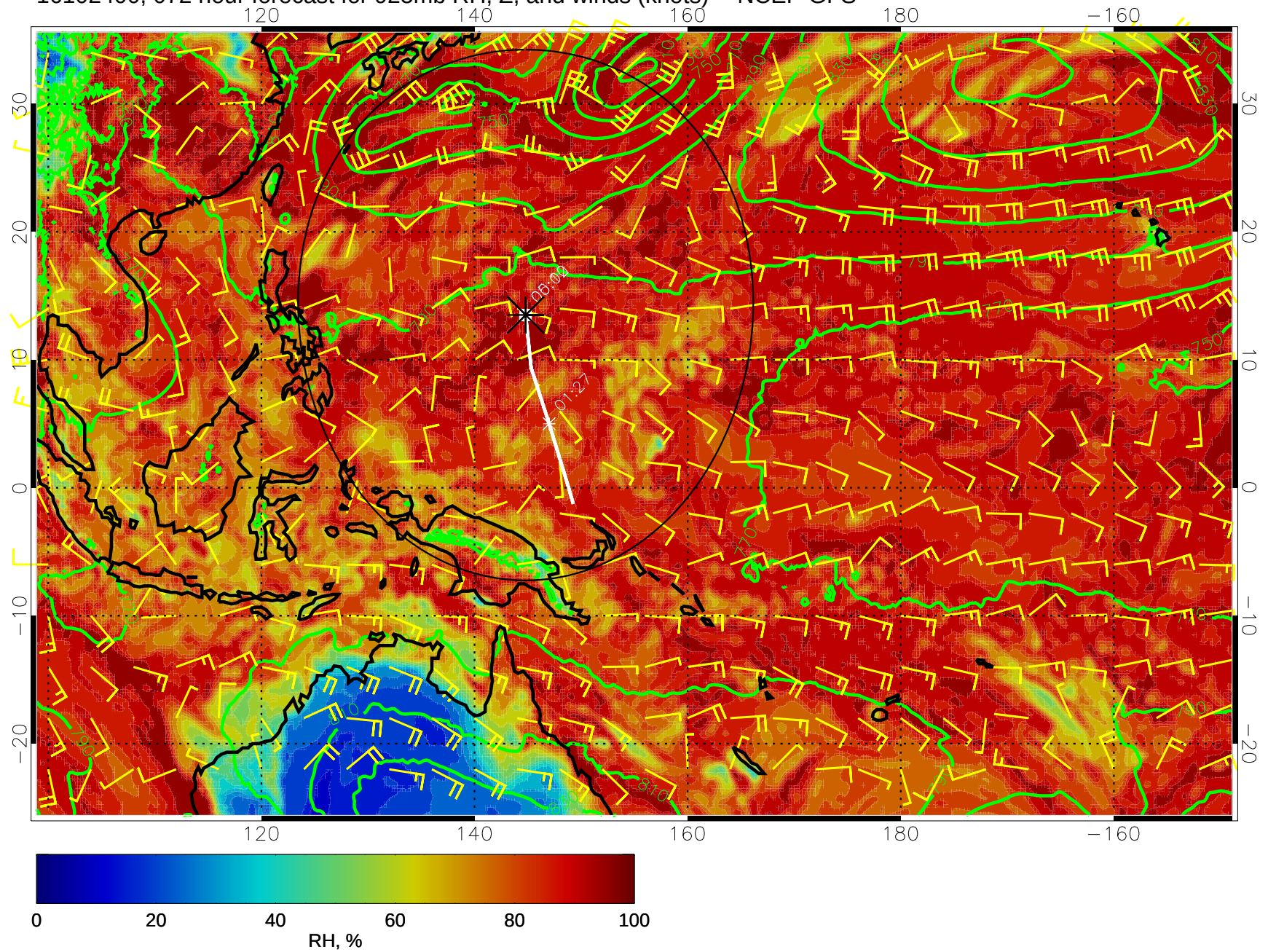
16102400, 072 hour forecast for 925mb RH, Z, and winds (knots) -- NCEP GFS
