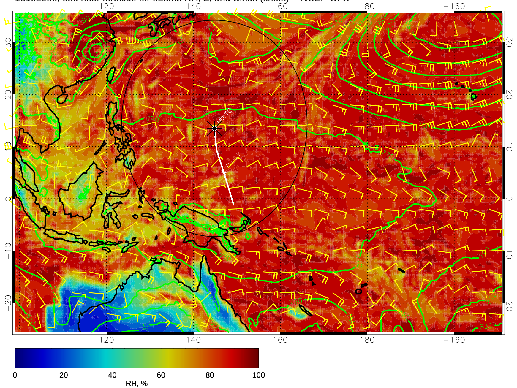
16102206, 030 hour forecast for 925mb RH, Z, and winds (knots) -- NCEP GFS
