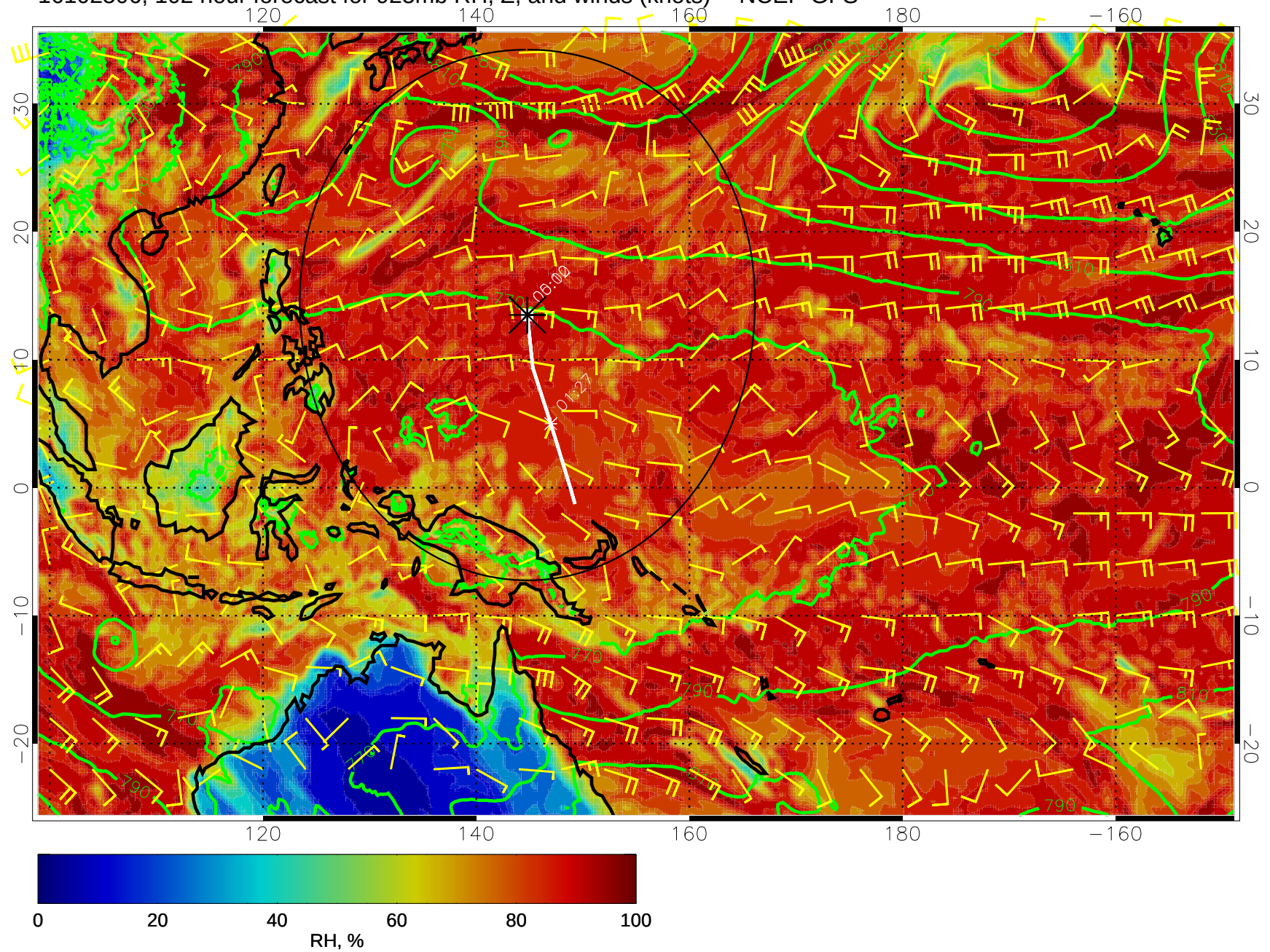
16102506, 102 hour forecast for 925mb RH, Z, and winds (knots) -- NCEP GFS
