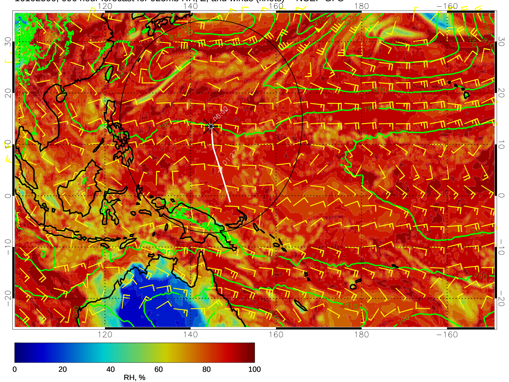
16102500, 096 hour forecast for 925mb RH, Z, and winds (knots) -- NCEP GFS
