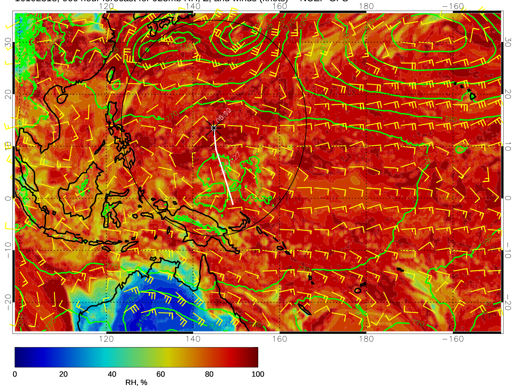
16102318, 066 hour forecast for 925mb RH, Z, and winds (knots) -- NCEP GFS
