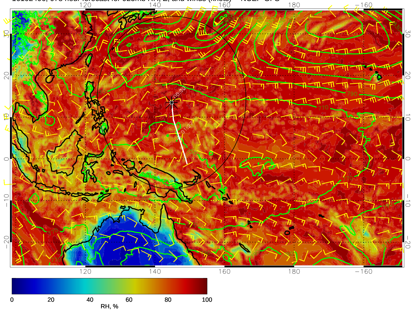
16102406, 078 hour forecast for 925mb RH, Z, and winds (knots) -- NCEP GFS
