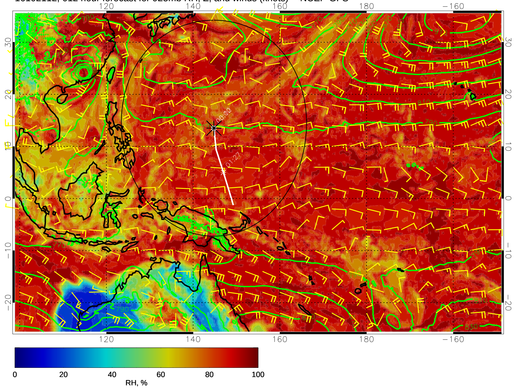
16102112, 012 hour forecast for 925mb RH, Z, and winds (knots) -- NCEP GFS
