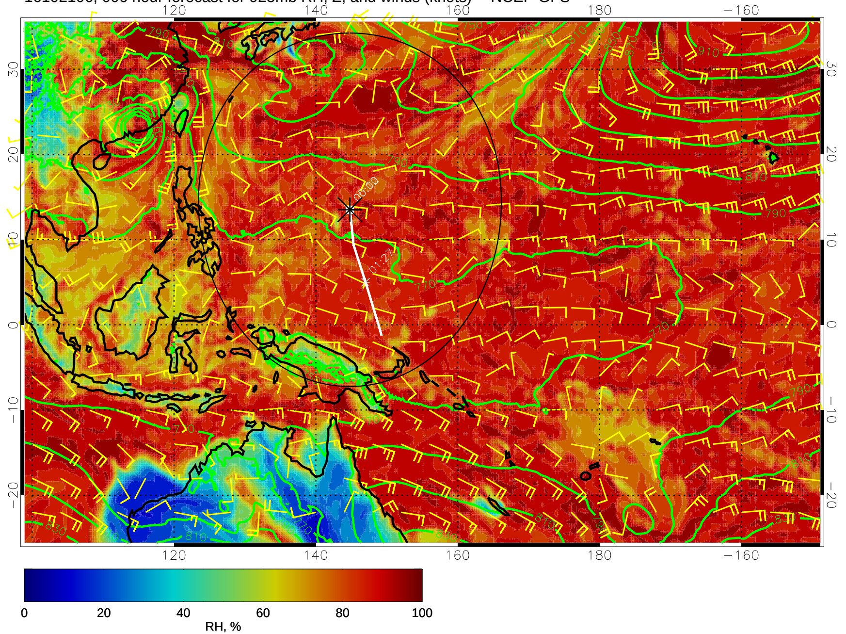
16102106, 006 hour forecast for 925mb RH, Z, and winds (knots) -- NCEP GFS
