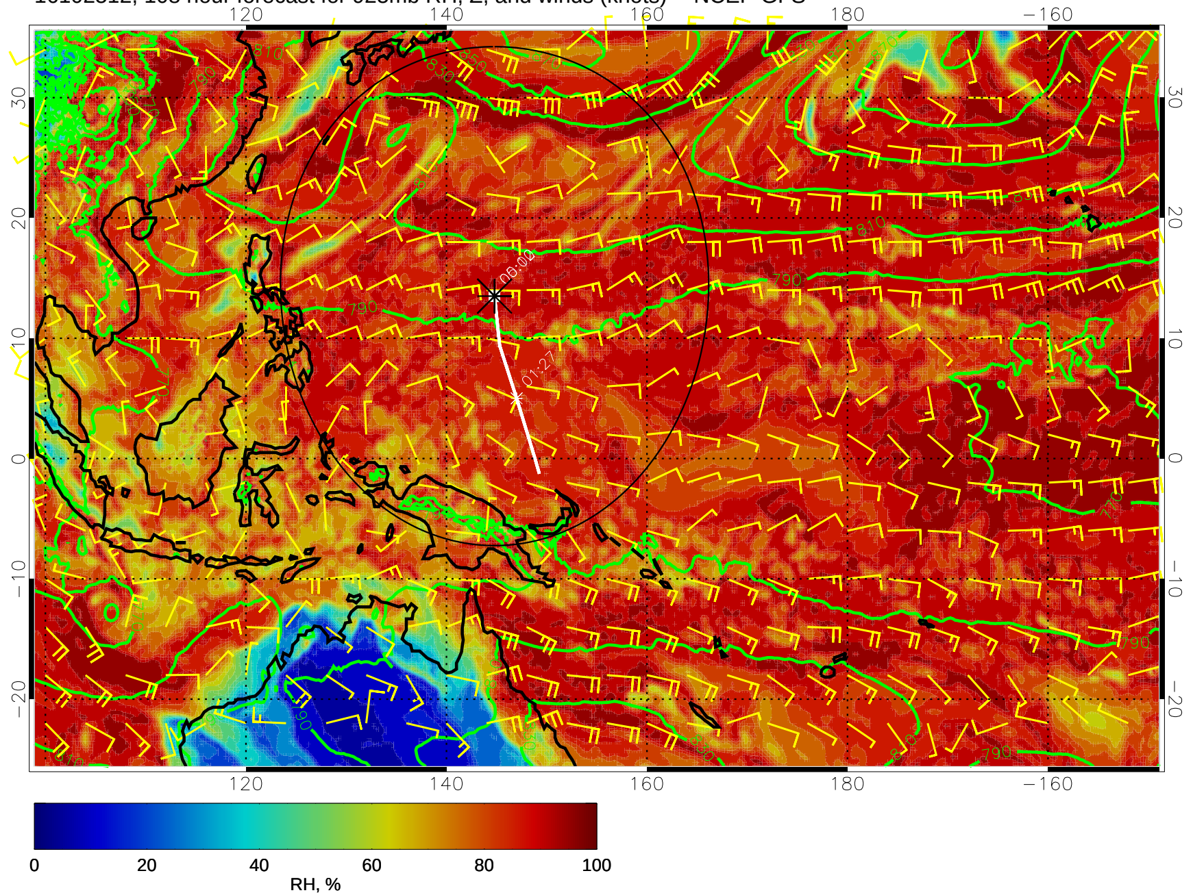
16102512, 108 hour forecast for 925mb RH, Z, and winds (knots) -- NCEP GFS
