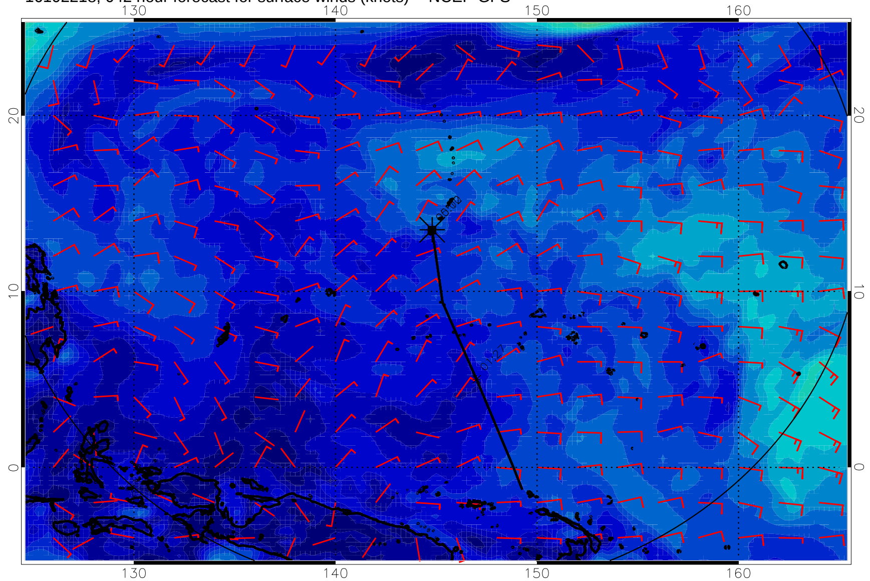
16102218, 042 hour forecast for surface winds (knots) -- NCEP GFS
