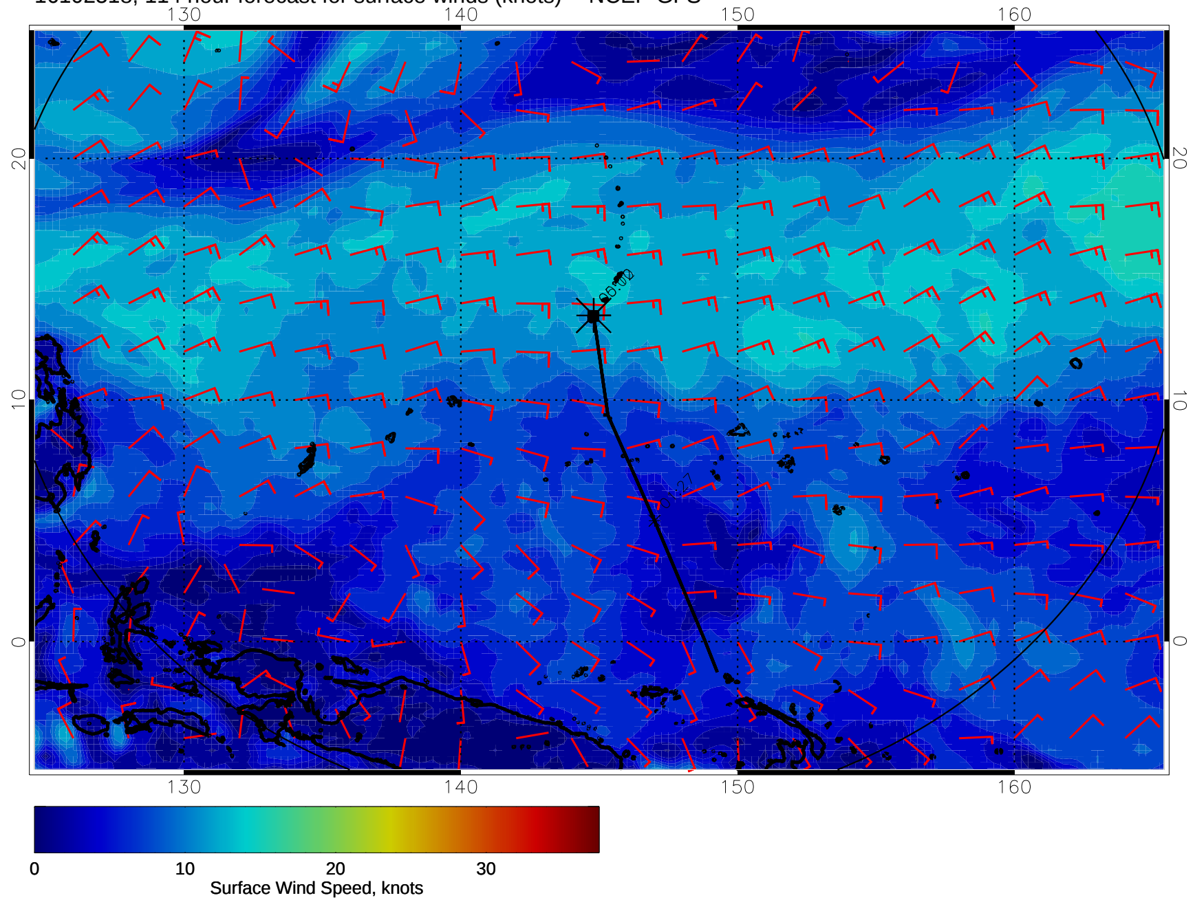
16102518, 114 hour forecast for surface winds (knots) -- NCEP GFS
