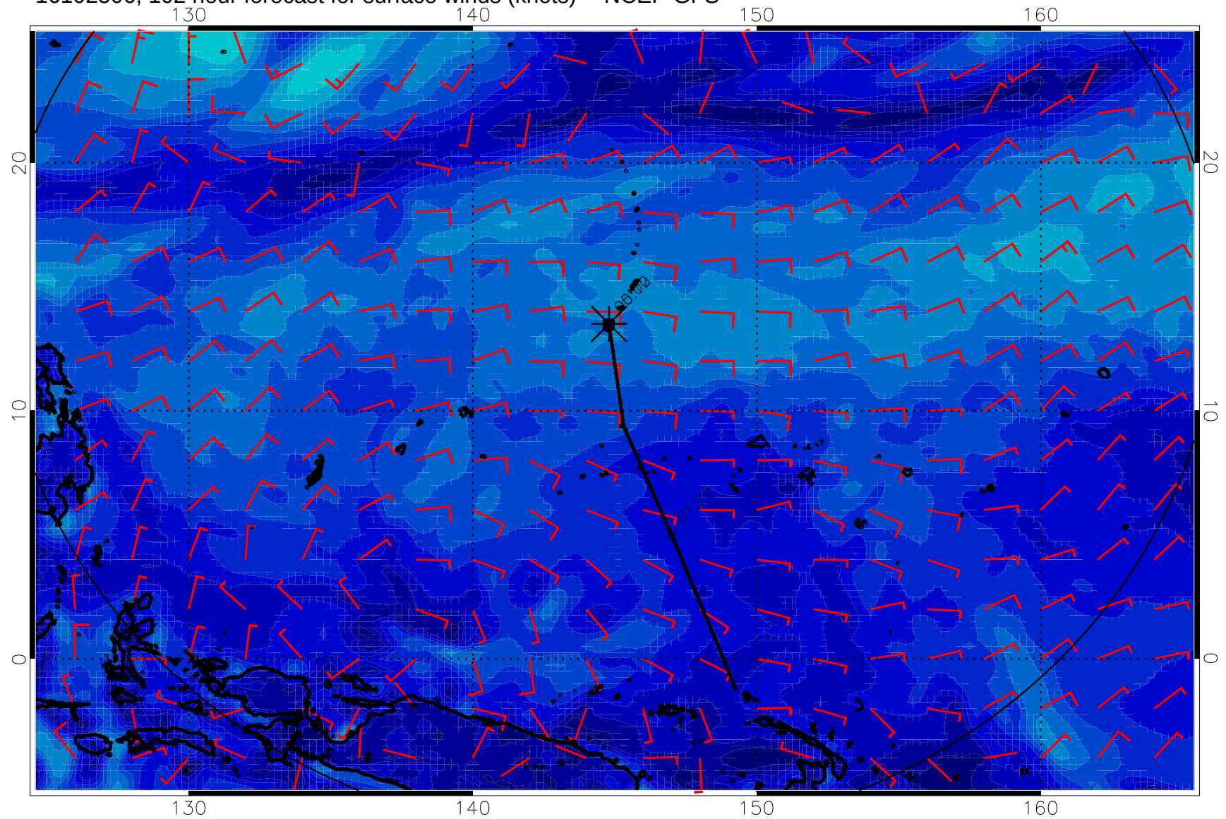
16102506, 102 hour forecast for surface winds (knots) -- NCEP GFS
