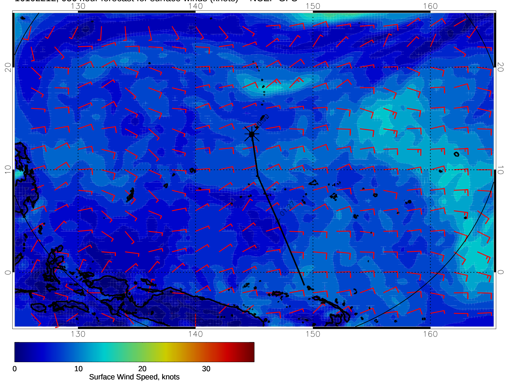
16102212, 036 hour forecast for surface winds (knots) -- NCEP GFS
