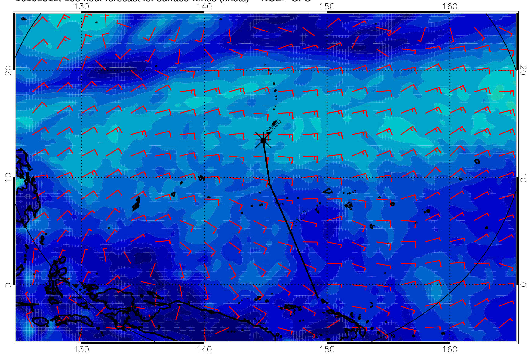
16102512, 108 hour forecast for surface winds (knots) -- NCEP GFS
