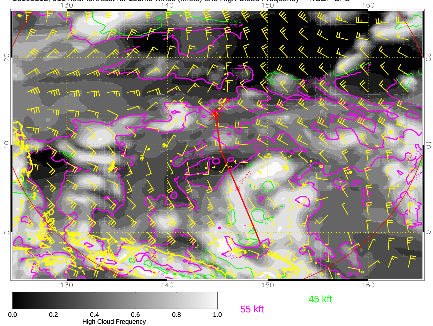
16102112, 012 hour forecast for 150mb winds (knots) and High Cloud Frequency -- NCEP GFS
