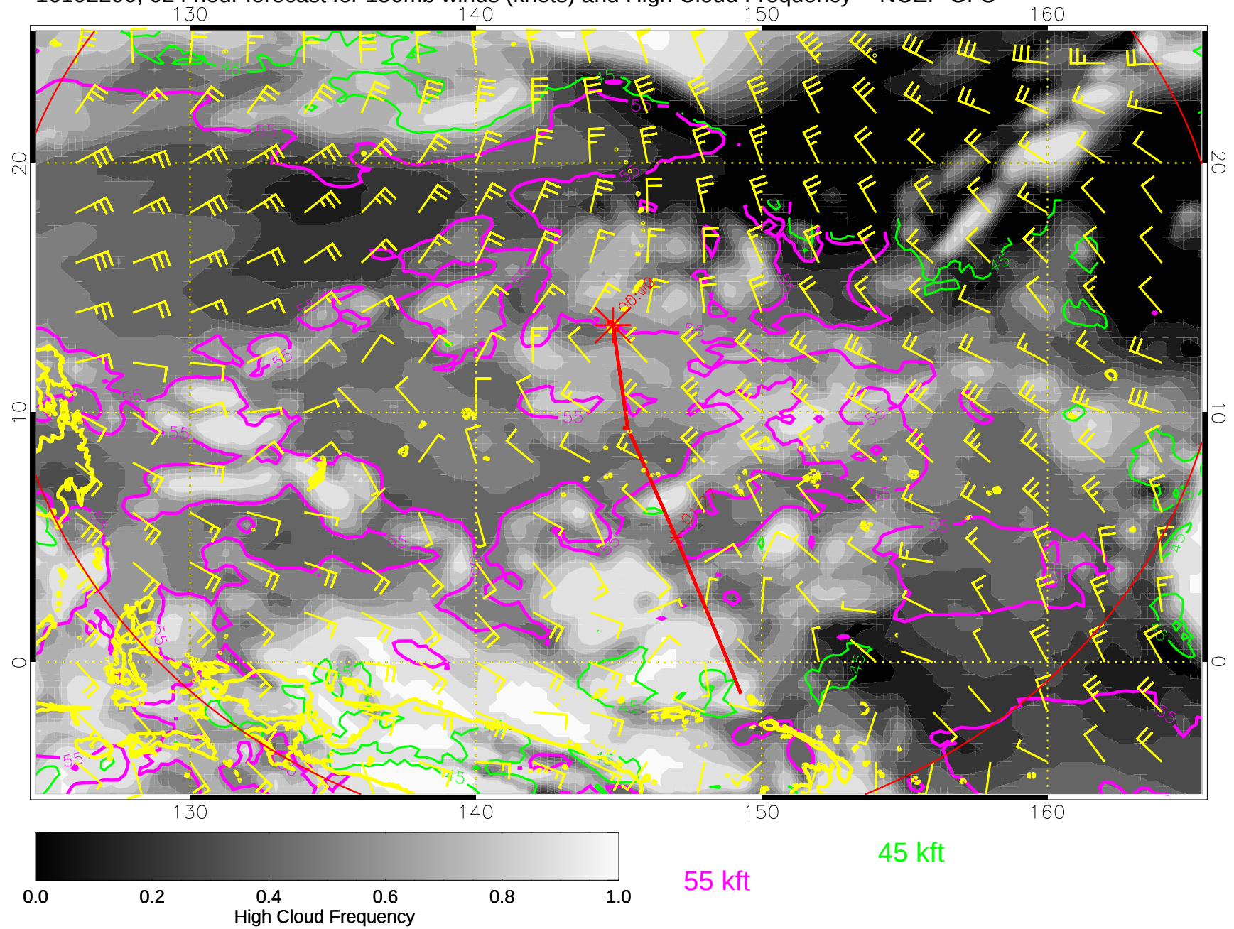
16102200, 024 hour forecast for 150mb winds (knots) and High Cloud Frequency -- NCEP GFS
