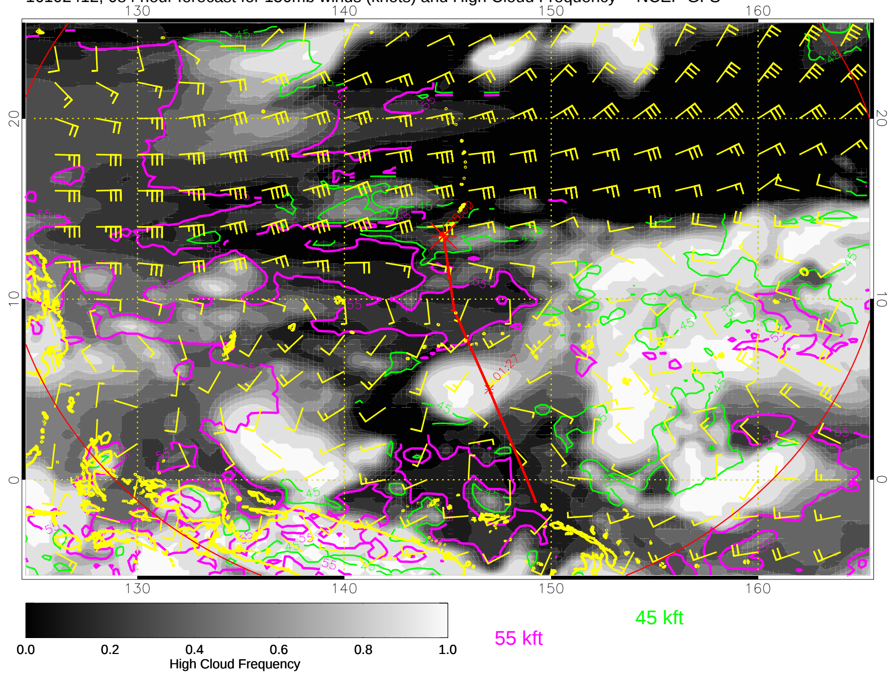
16102412, 084 hour forecast for 150mb winds (knots) and High Cloud Frequency -- NCEP GFS
