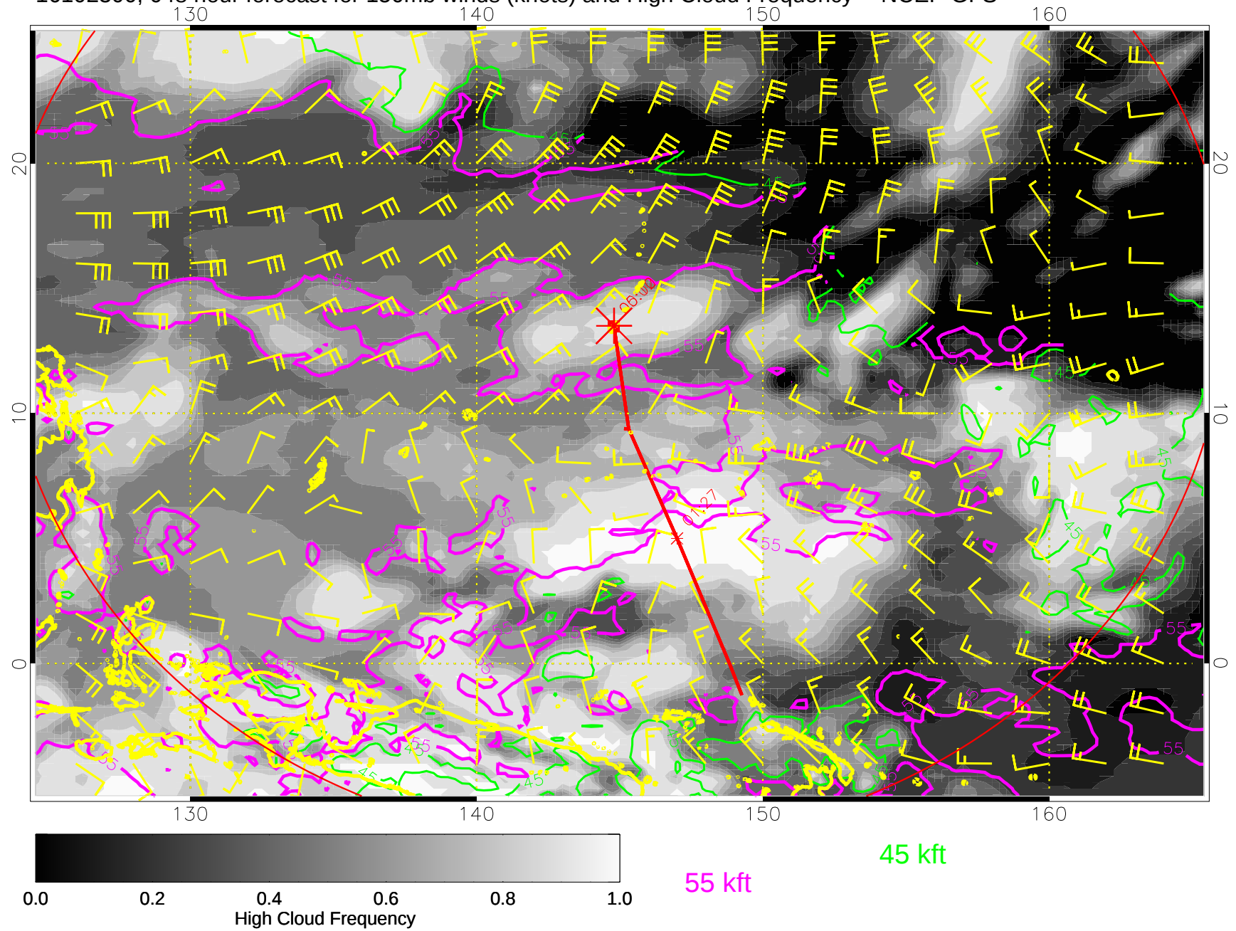
16102300, 048 hour forecast for 150mb winds (knots) and High Cloud Frequency -- NCEP GFS
