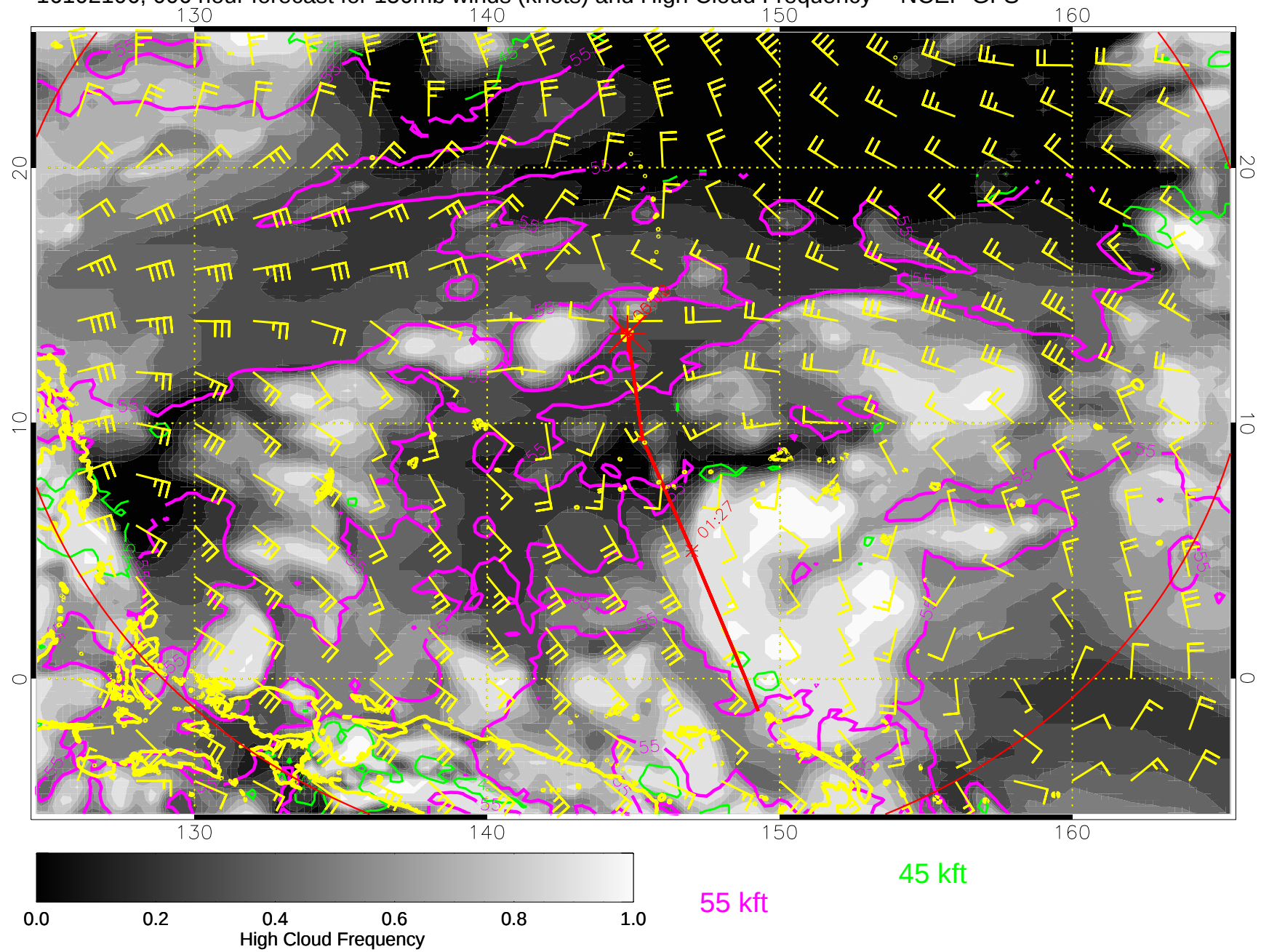
16102106, 006 hour forecast for 150mb winds (knots) and High Cloud Frequency -- NCEP GFS
