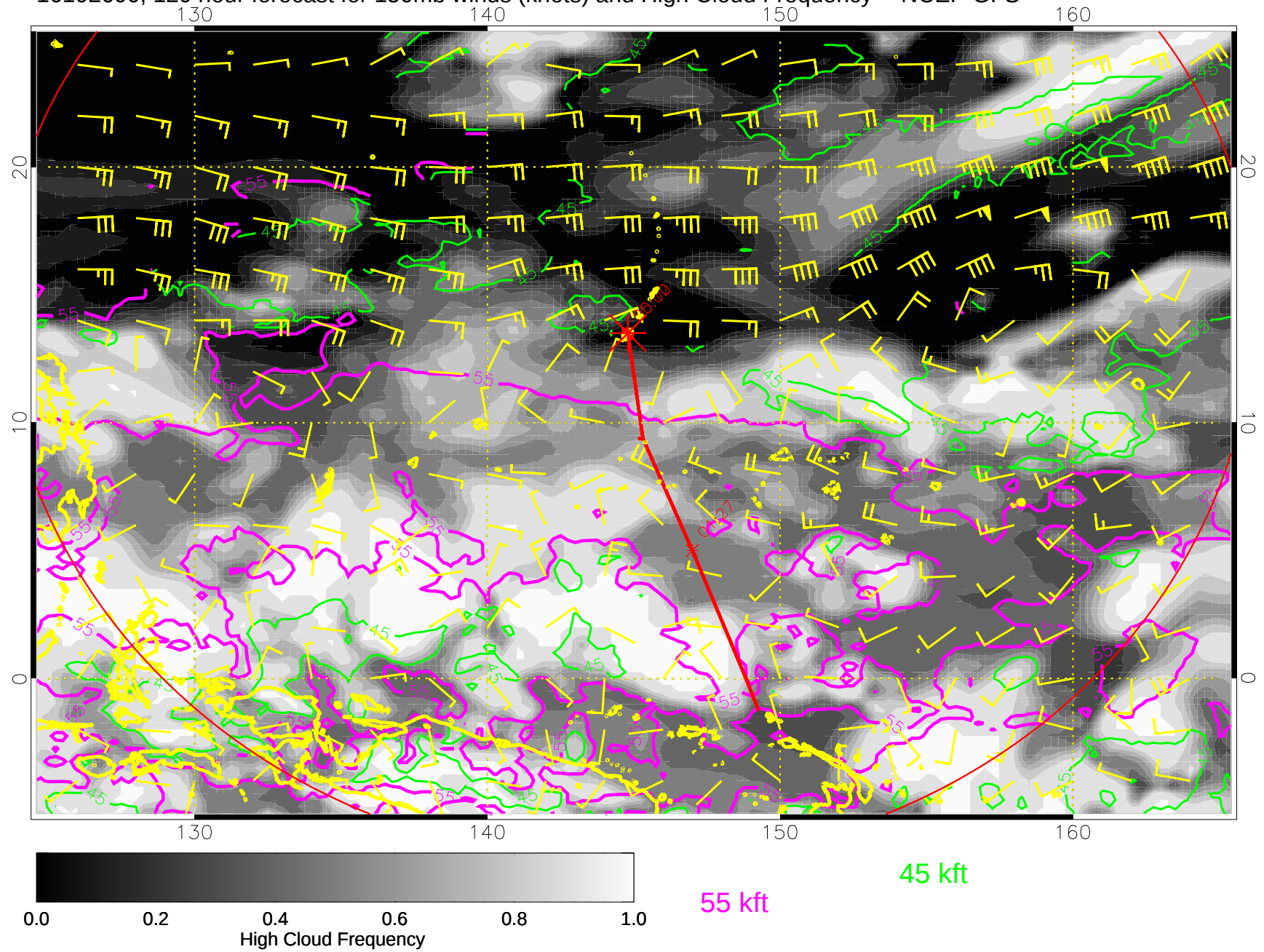
16102600, 120 hour forecast for 150mb winds (knots) and High Cloud Frequency -- NCEP GFS
