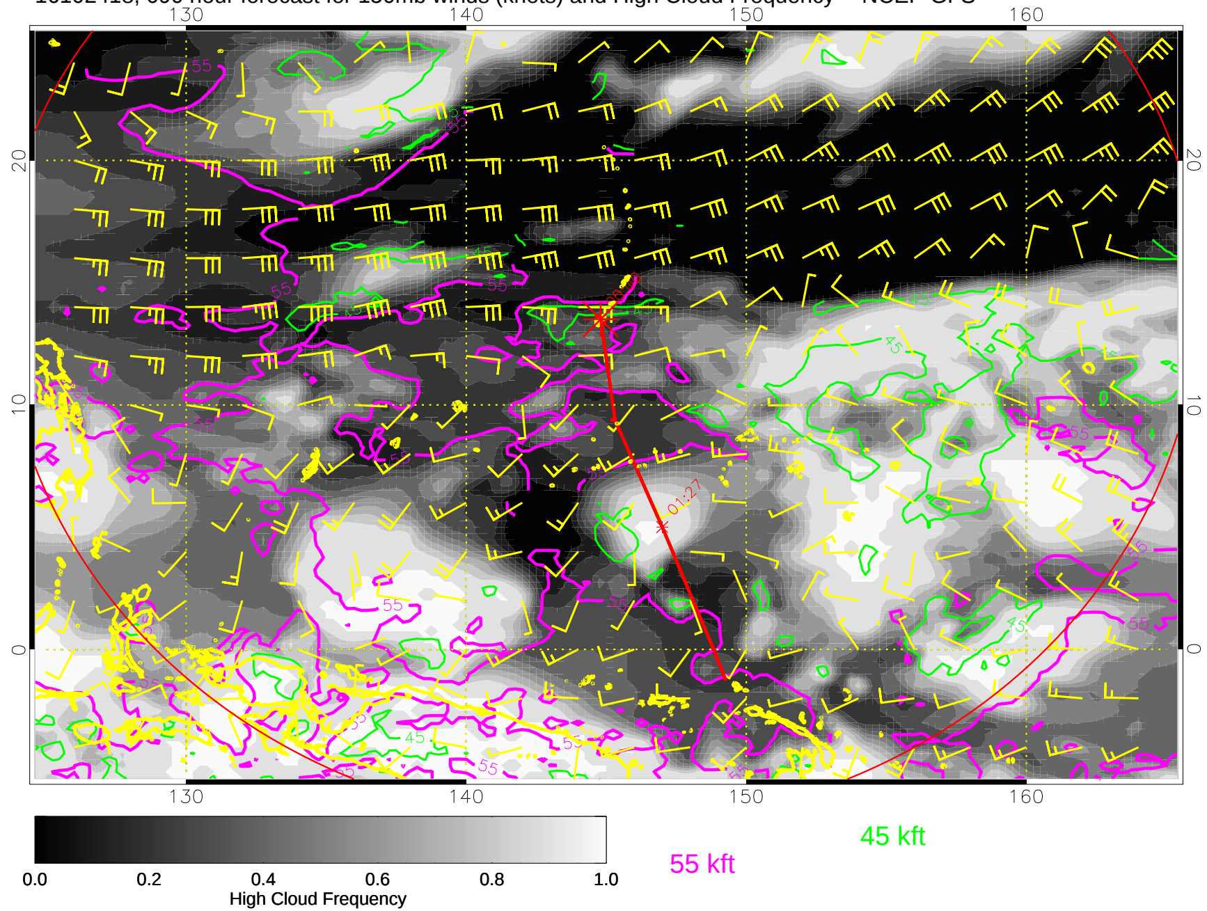
16102418, 090 hour forecast for 150mb winds (knots) and High Cloud Frequency -- NCEP GFS
