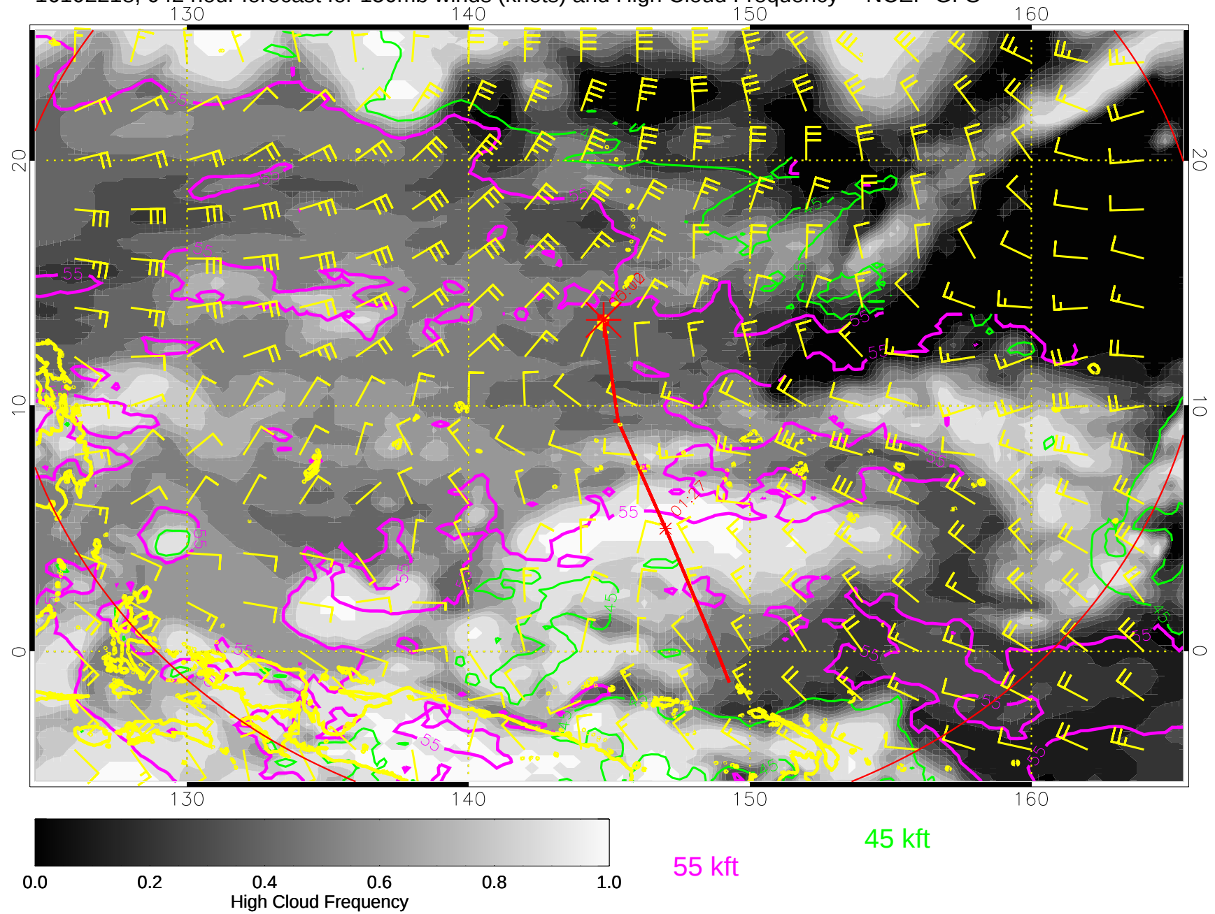
16102218, 042 hour forecast for 150mb winds (knots) and High Cloud Frequency -- NCEP GFS
