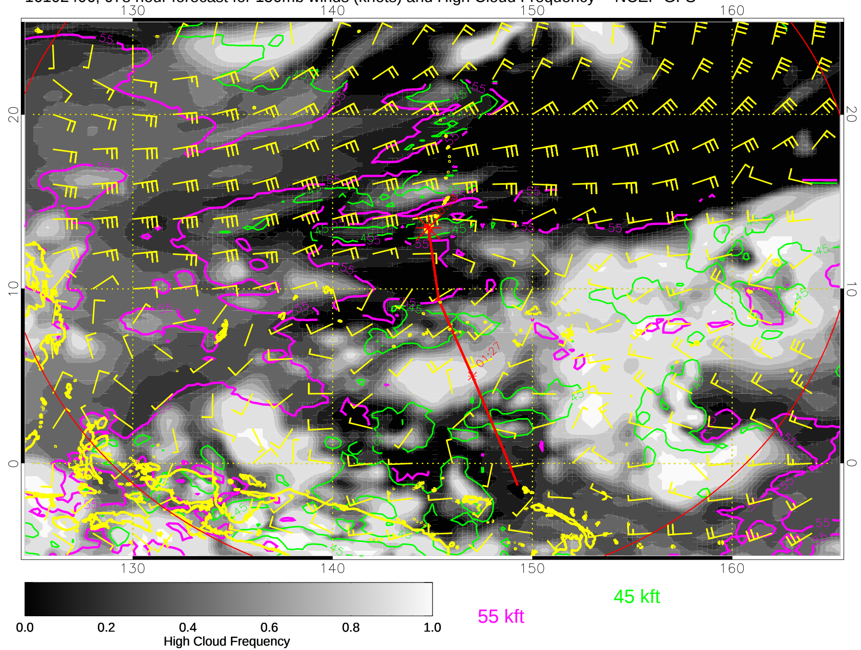
16102406, 078 hour forecast for 150mb winds (knots) and High Cloud Frequency -- NCEP GFS
