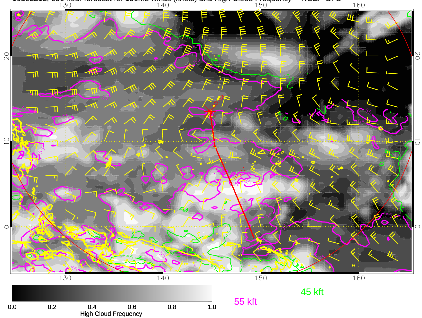
16102212, 036 hour forecast for 150mb winds (knots) and High Cloud Frequency -- NCEP GFS
