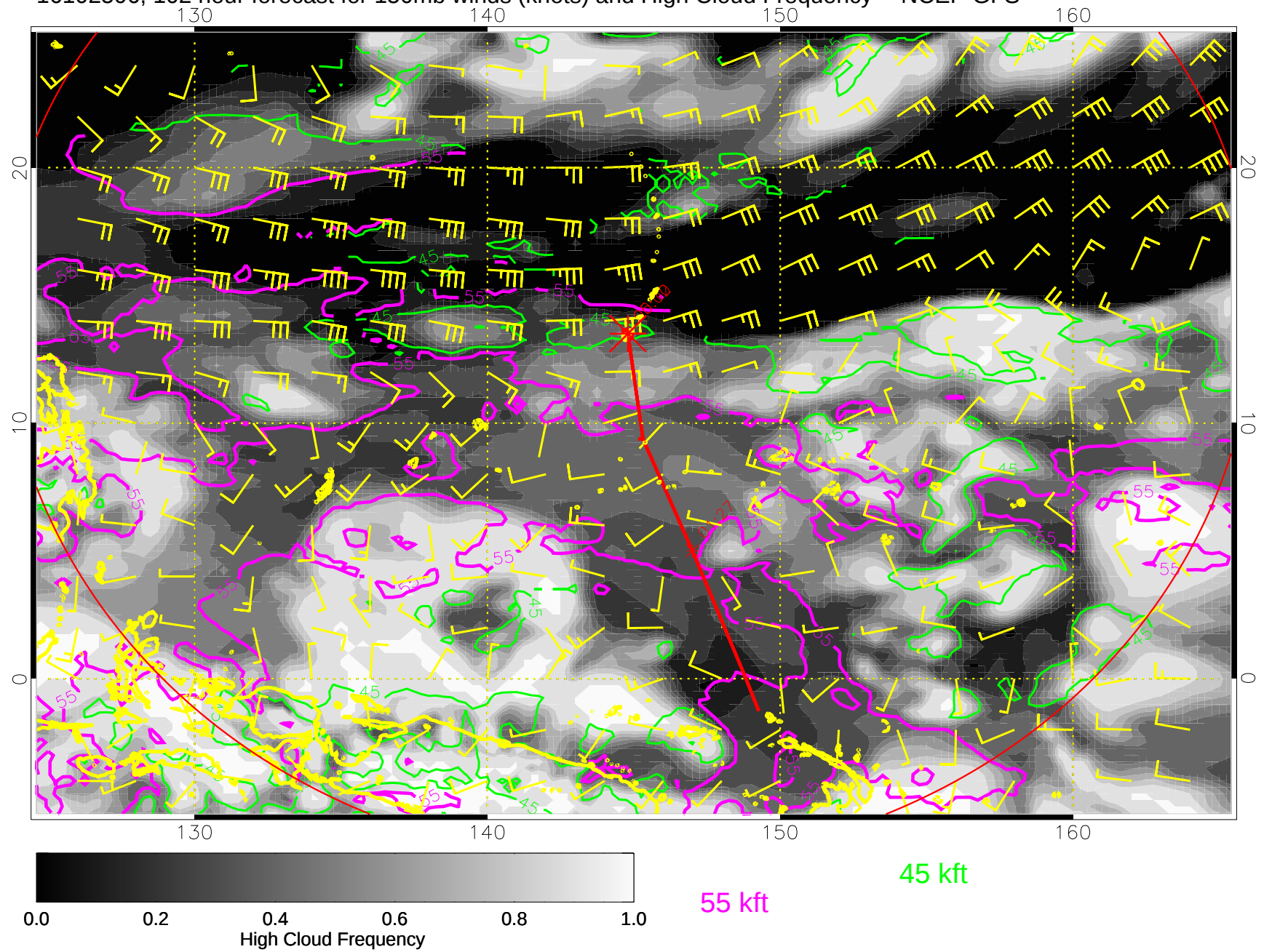
16102506, 102 hour forecast for 150mb winds (knots) and High Cloud Frequency -- NCEP GFS
