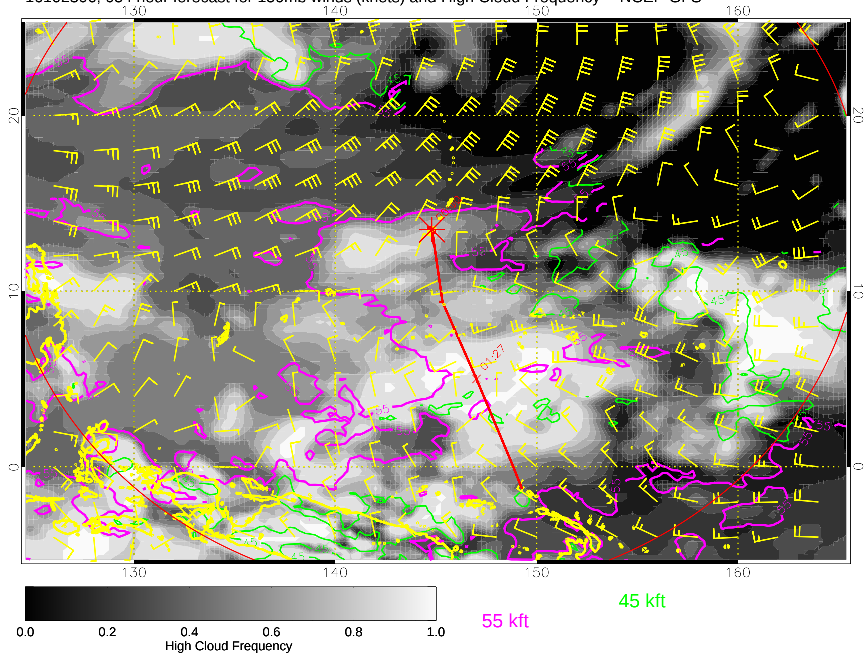
16102306, 054 hour forecast for 150mb winds (knots) and High Cloud Frequency -- NCEP GFS
