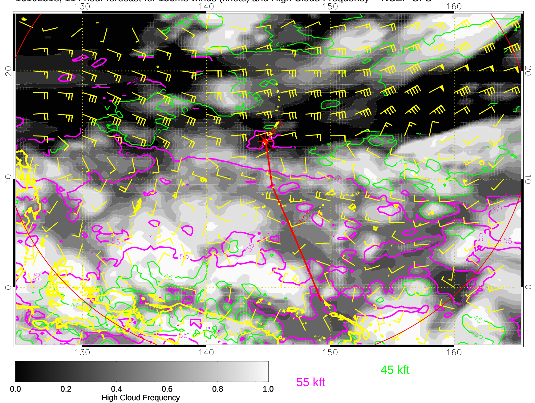
16102518, 114 hour forecast for 150mb winds (knots) and High Cloud Frequency -- NCEP GFS
