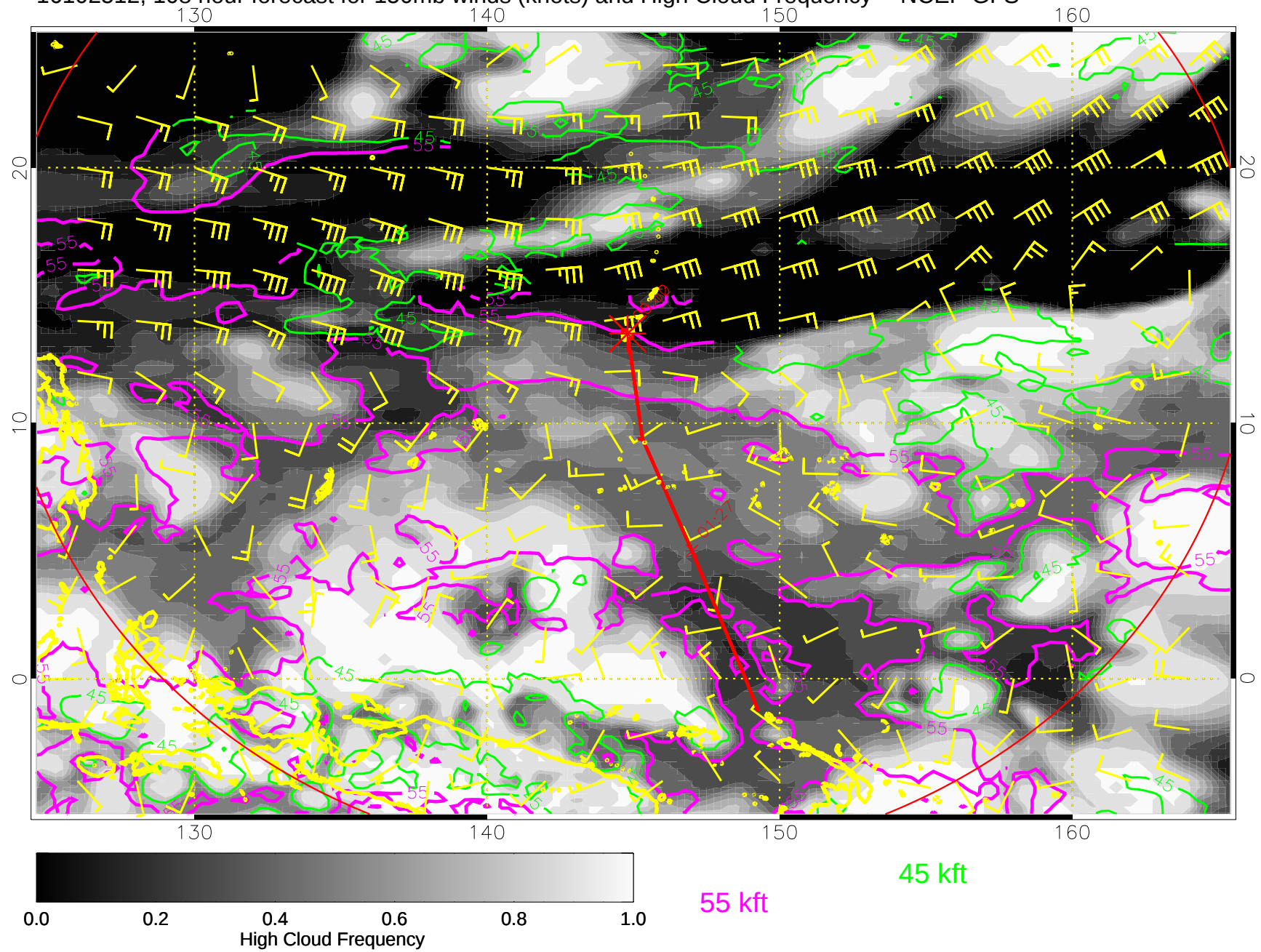
16102512, 108 hour forecast for 150mb winds (knots) and High Cloud Frequency -- NCEP GFS
