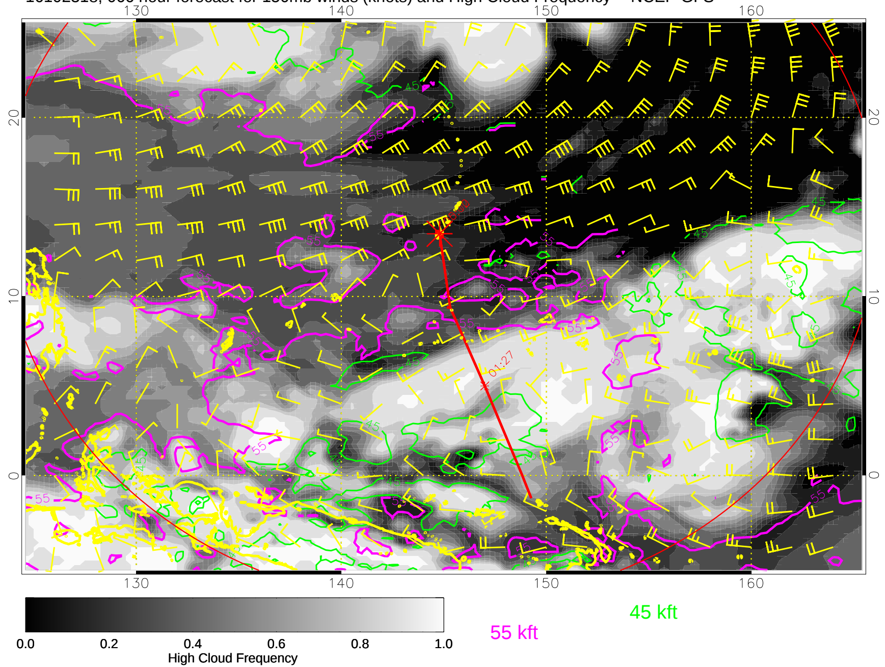
16102318, 066 hour forecast for 150mb winds (knots) and High Cloud Frequency -- NCEP GFS
