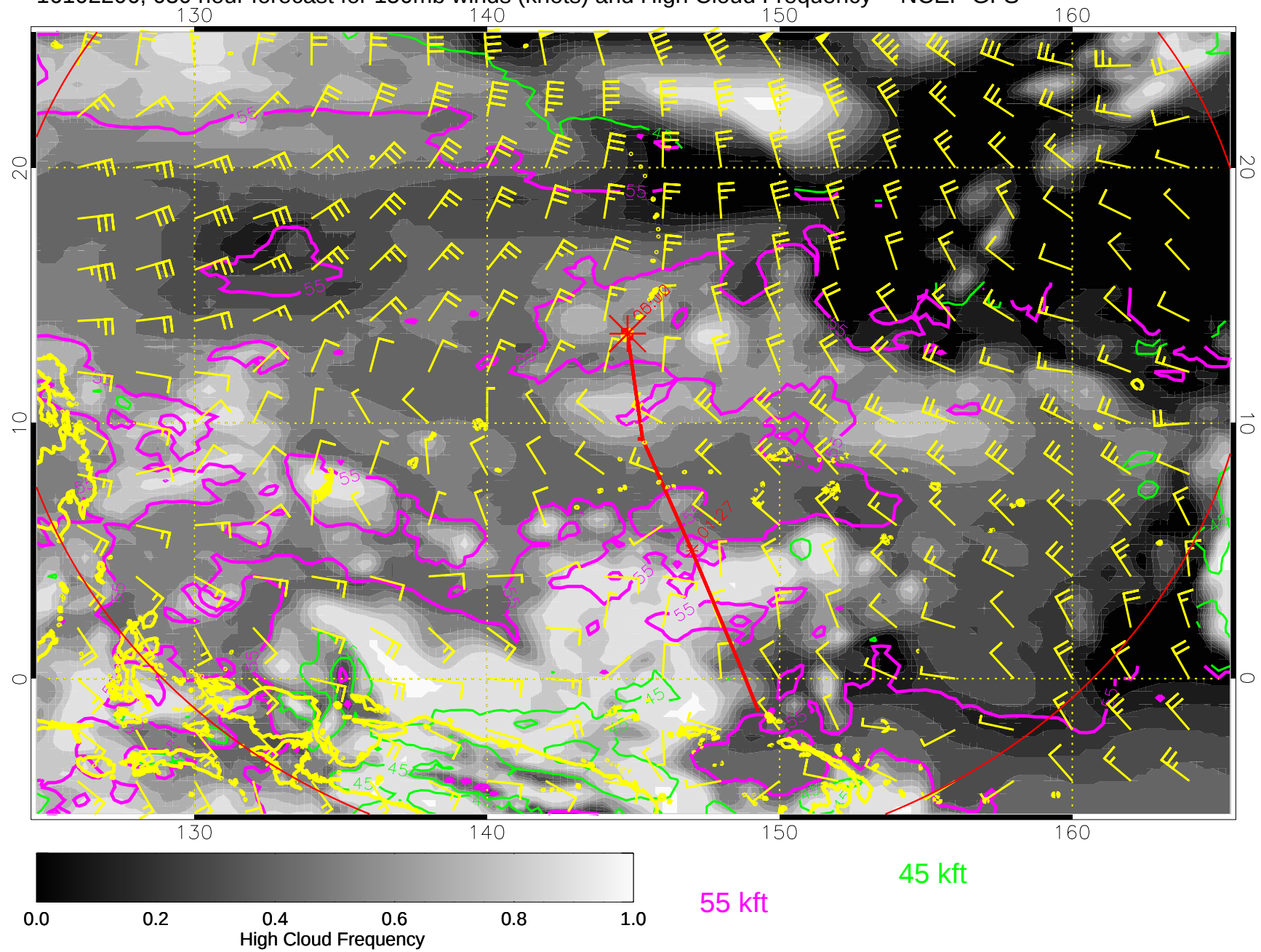
16102206, 030 hour forecast for 150mb winds (knots) and High Cloud Frequency -- NCEP GFS
