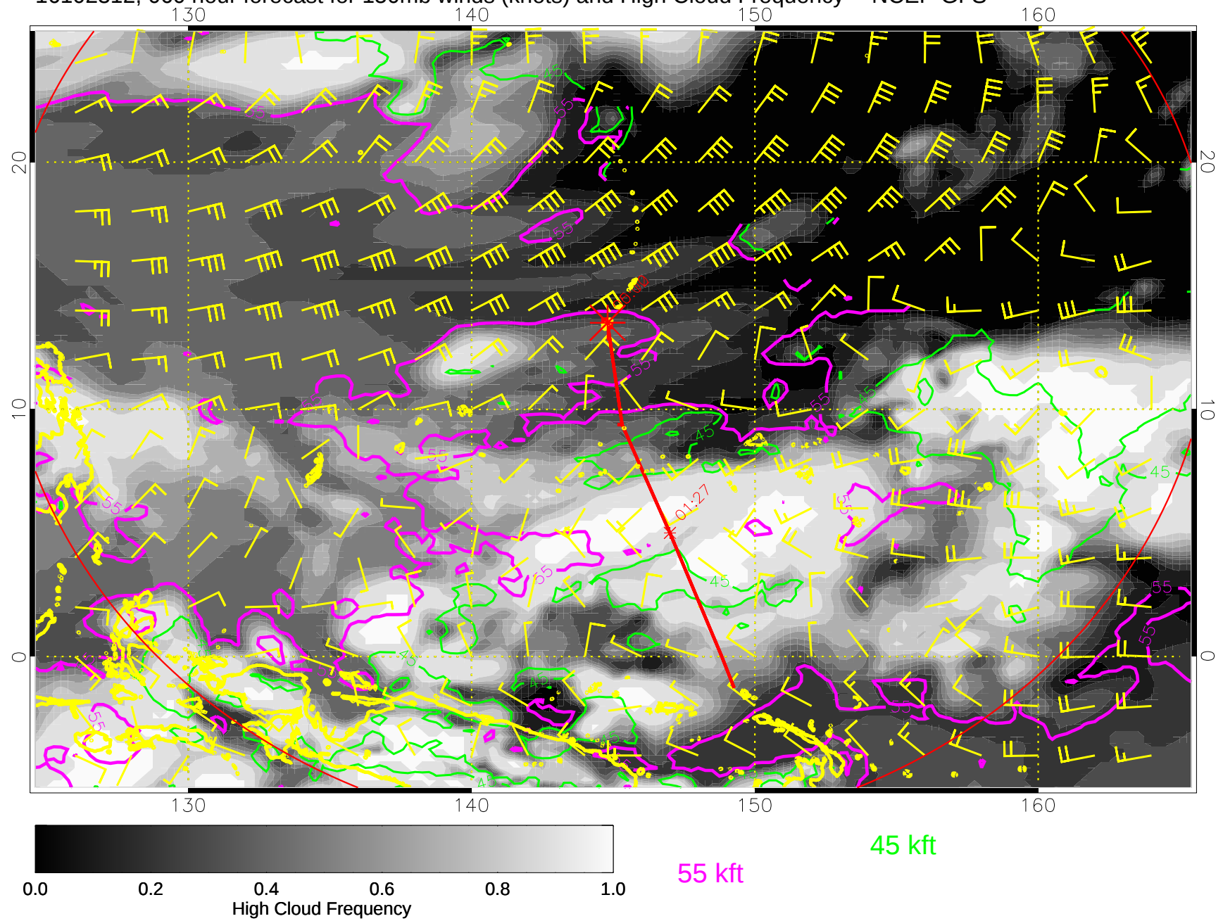
16102312, 060 hour forecast for 150mb winds (knots) and High Cloud Frequency -- NCEP GFS
