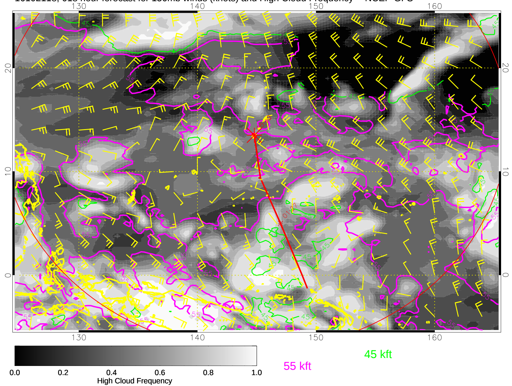
16102118, 018 hour forecast for 150mb winds (knots) and High Cloud Frequency -- NCEP GFS
