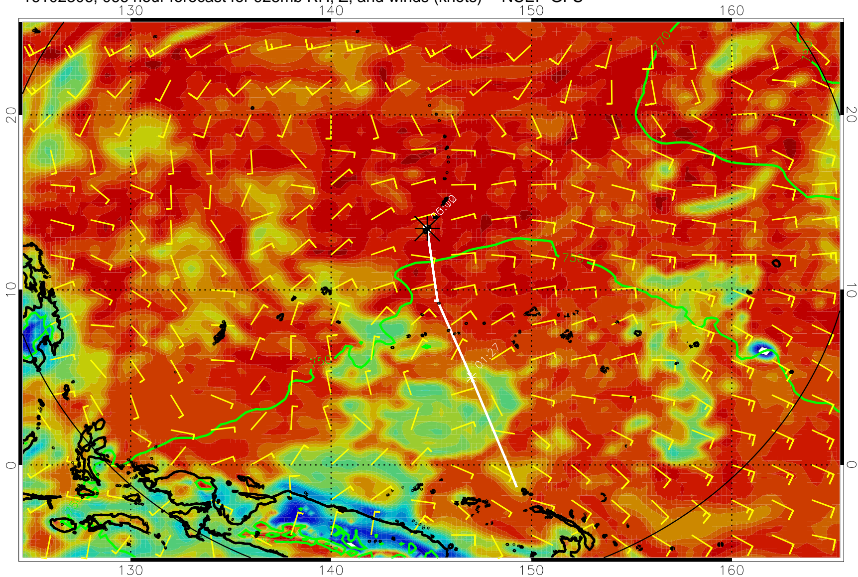
16102306, 066 hour forecast for 925mb RH, Z, and winds (knots) -- NCEP GFS
