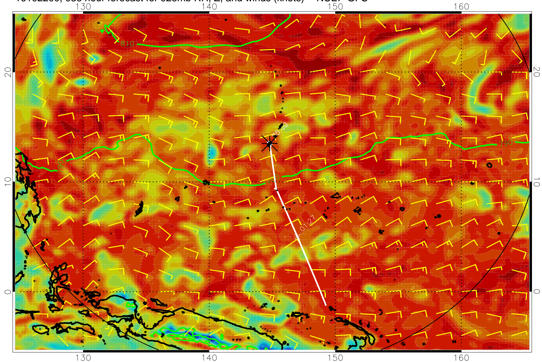
16102200, 036 hour forecast for 925mb RH, Z, and winds (knots) -- NCEP GFS
