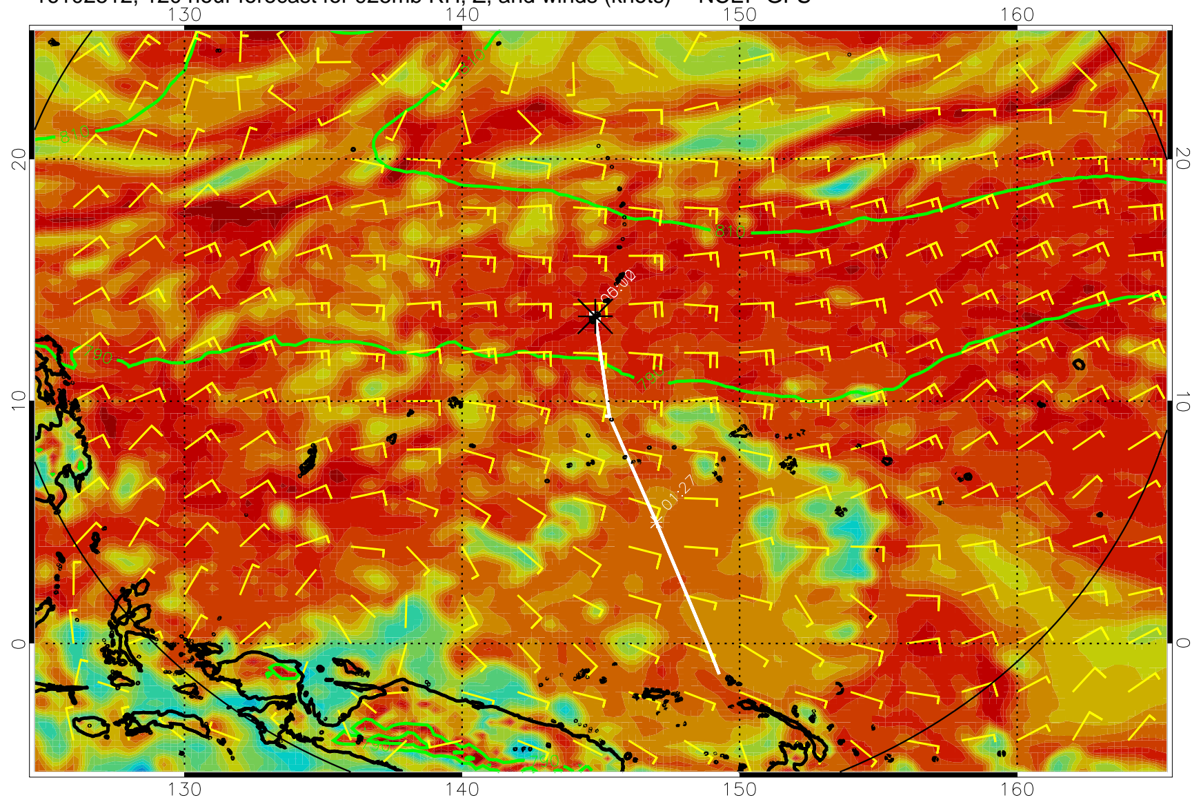
16102512, 120 hour forecast for 925mb RH, Z, and winds (knots) -- NCEP GFS
