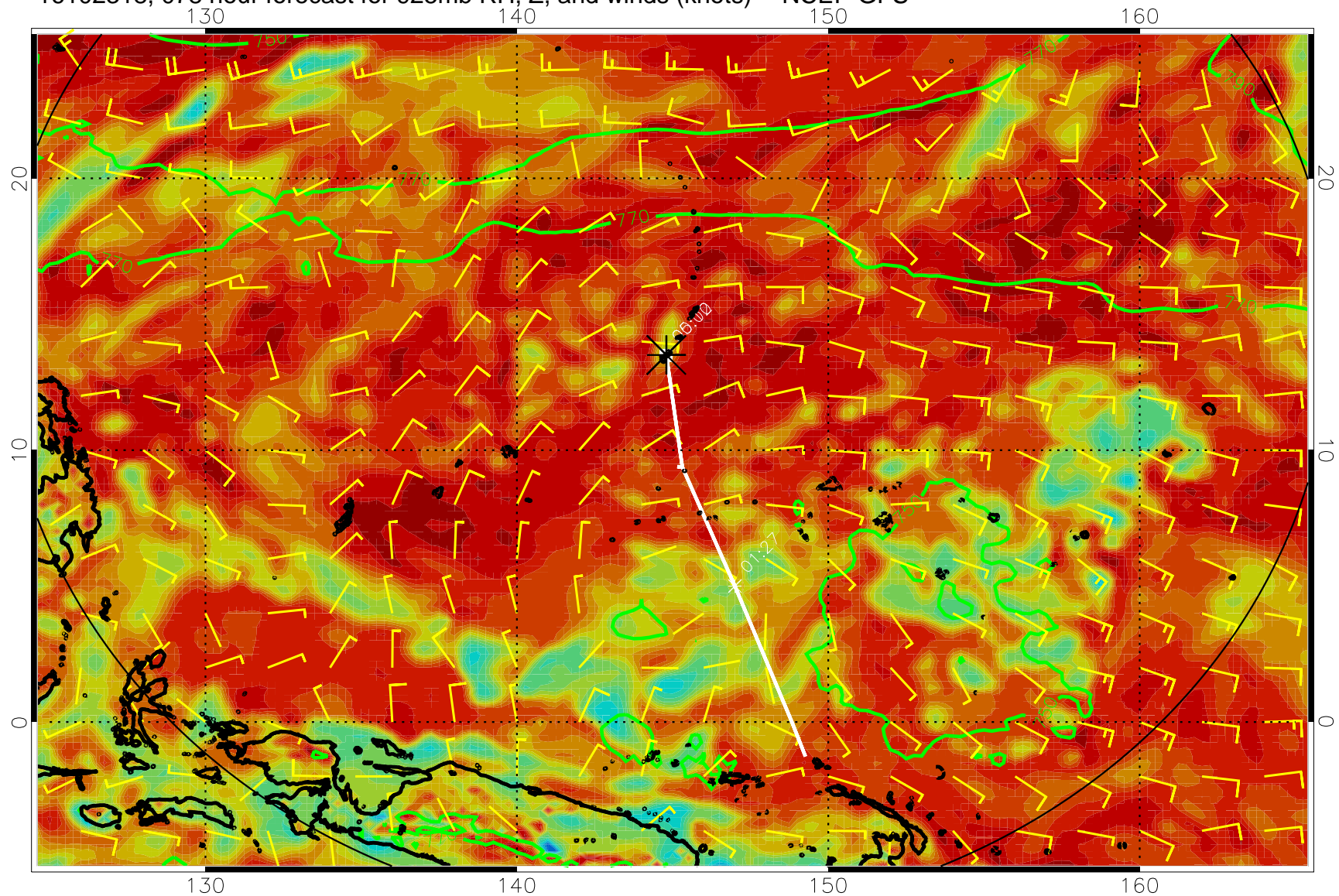
16102318, 078 hour forecast for 925mb RH, Z, and winds (knots) -- NCEP GFS
