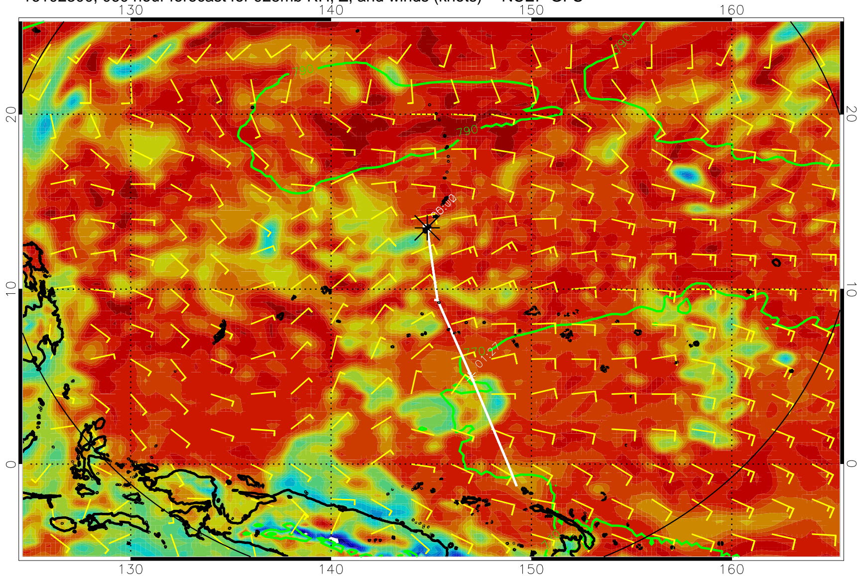
16102300, 060 hour forecast for 925mb RH, Z, and winds (knots) -- NCEP GFS
