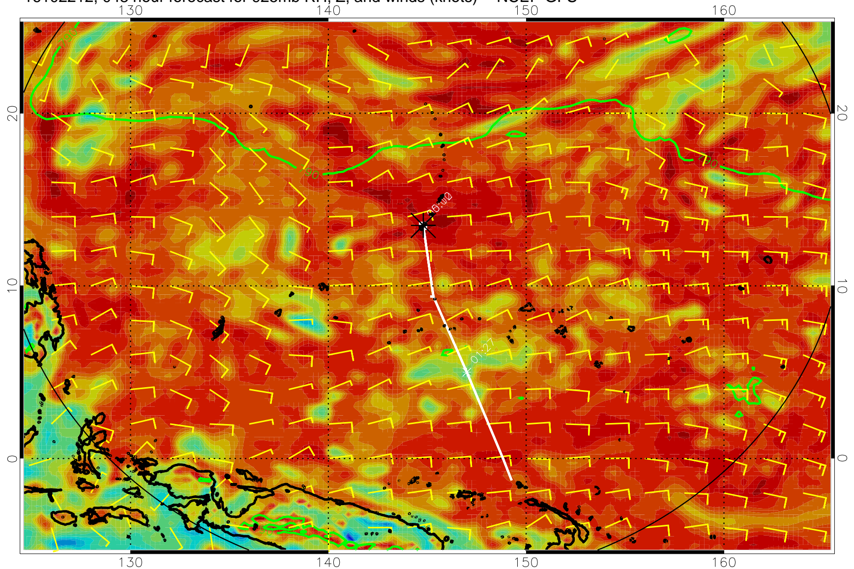
16102212, 048 hour forecast for 925mb RH, Z, and winds (knots) -- NCEP GFS
