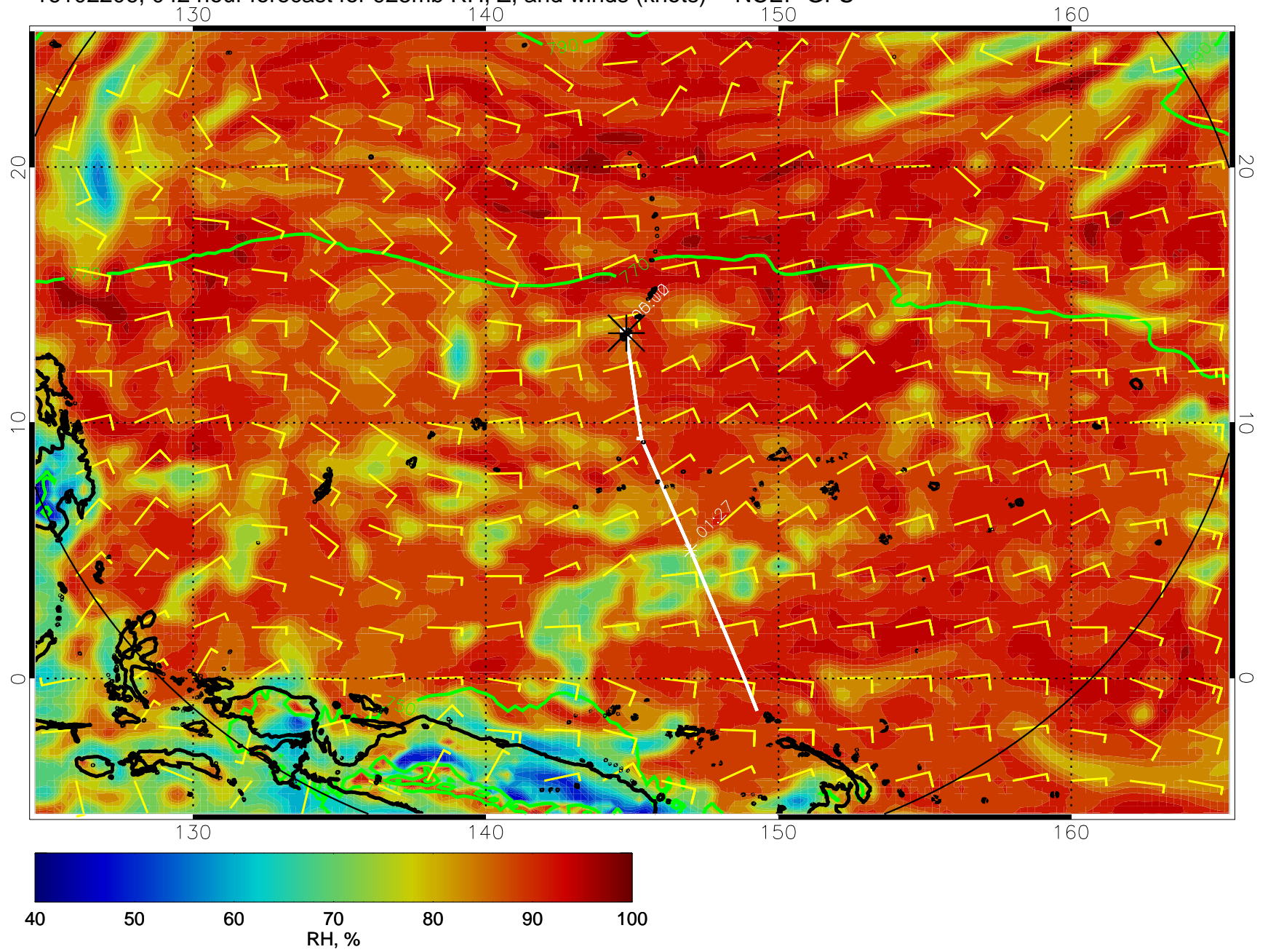
16102206, 042 hour forecast for 925mb RH, Z, and winds (knots) -- NCEP GFS
