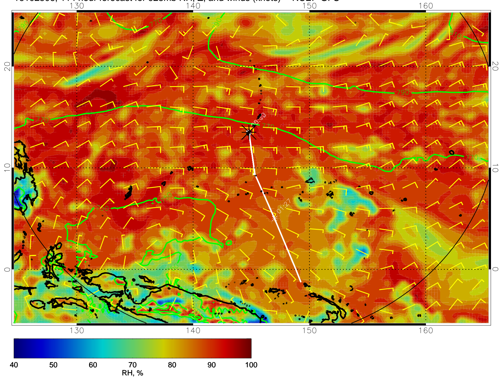
16102506, 114 hour forecast for 925mb RH, Z, and winds (knots) -- NCEP GFS
