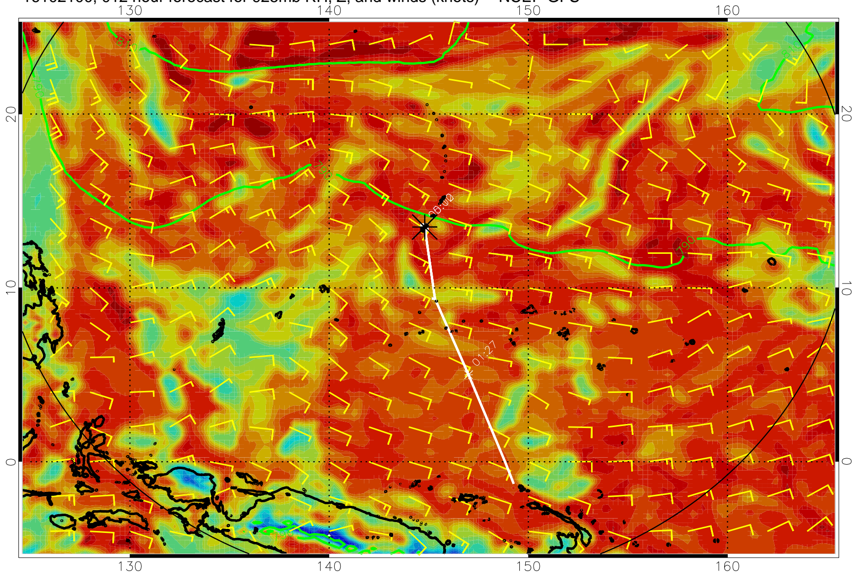
16102100, 012 hour forecast for 925mb RH, Z, and winds (knots) -- NCEP GFS
