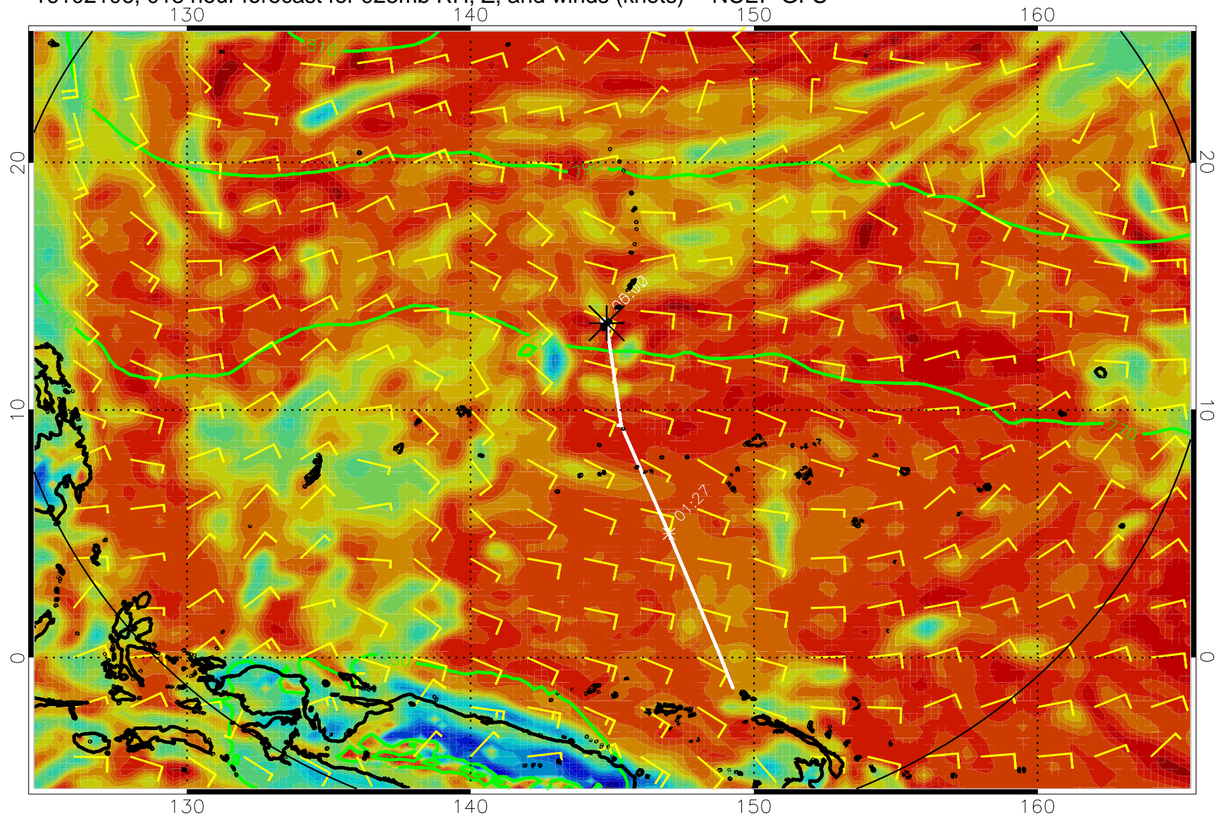
16102106, 018 hour forecast for 925mb RH, Z, and winds (knots) -- NCEP GFS
