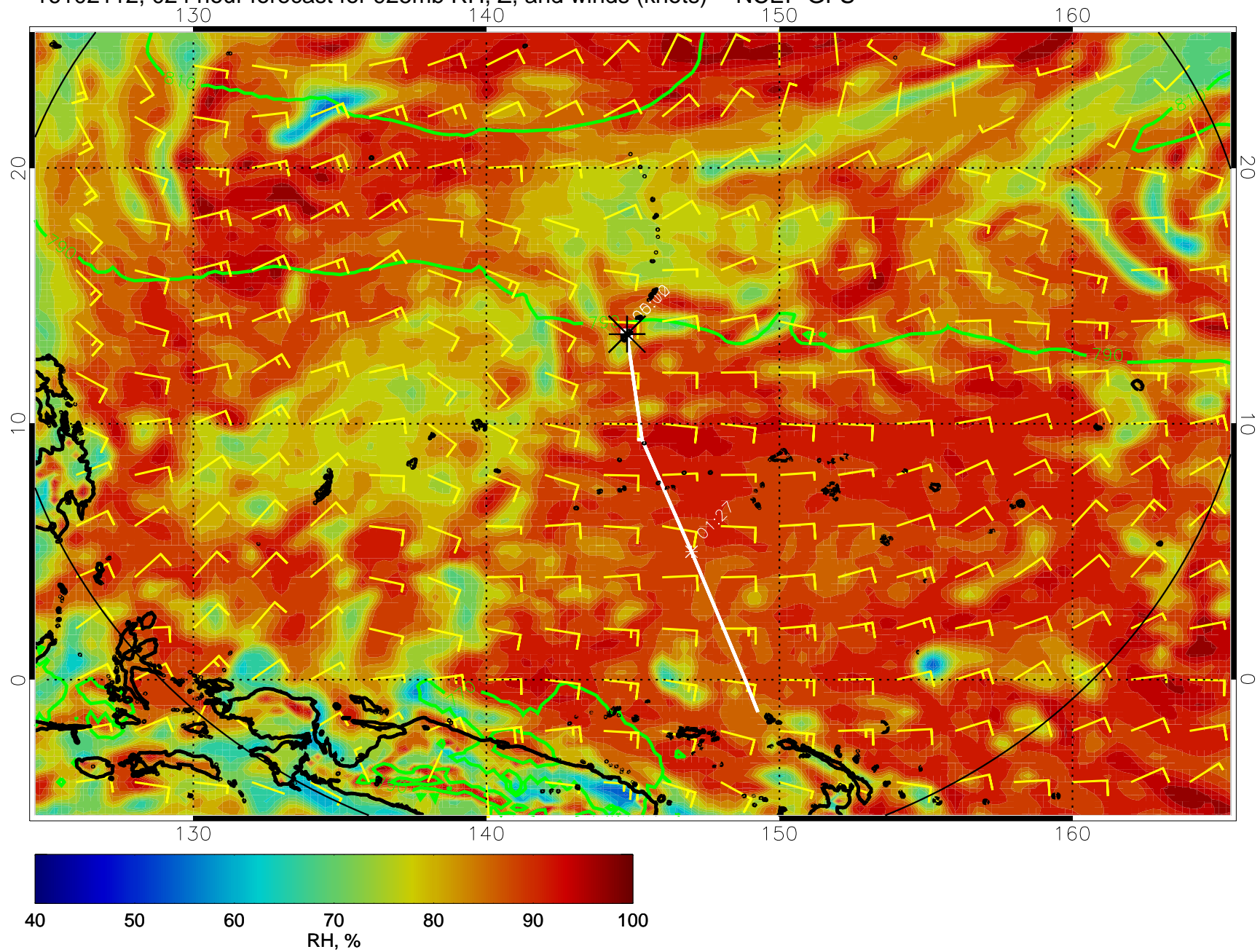
16102112, 024 hour forecast for 925mb RH, Z, and winds (knots) -- NCEP GFS
