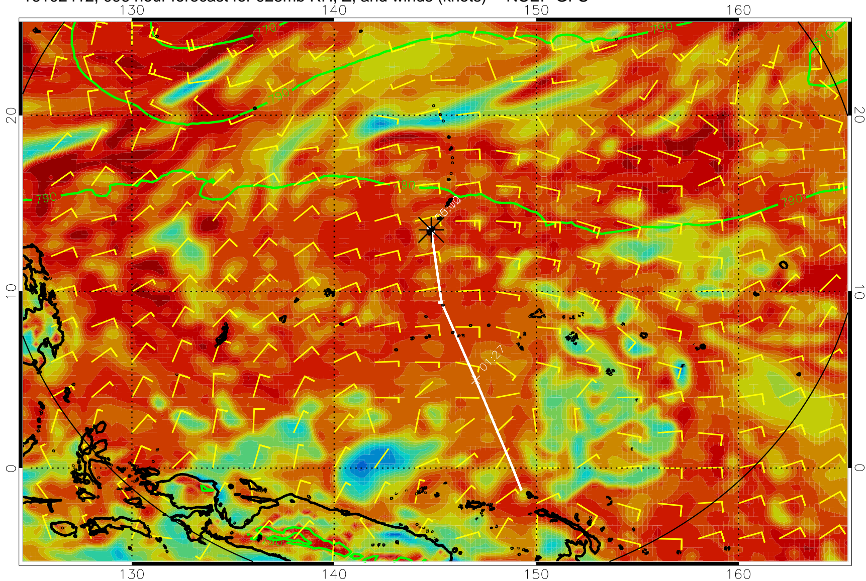
16102412, 096 hour forecast for 925mb RH, Z, and winds (knots) -- NCEP GFS
