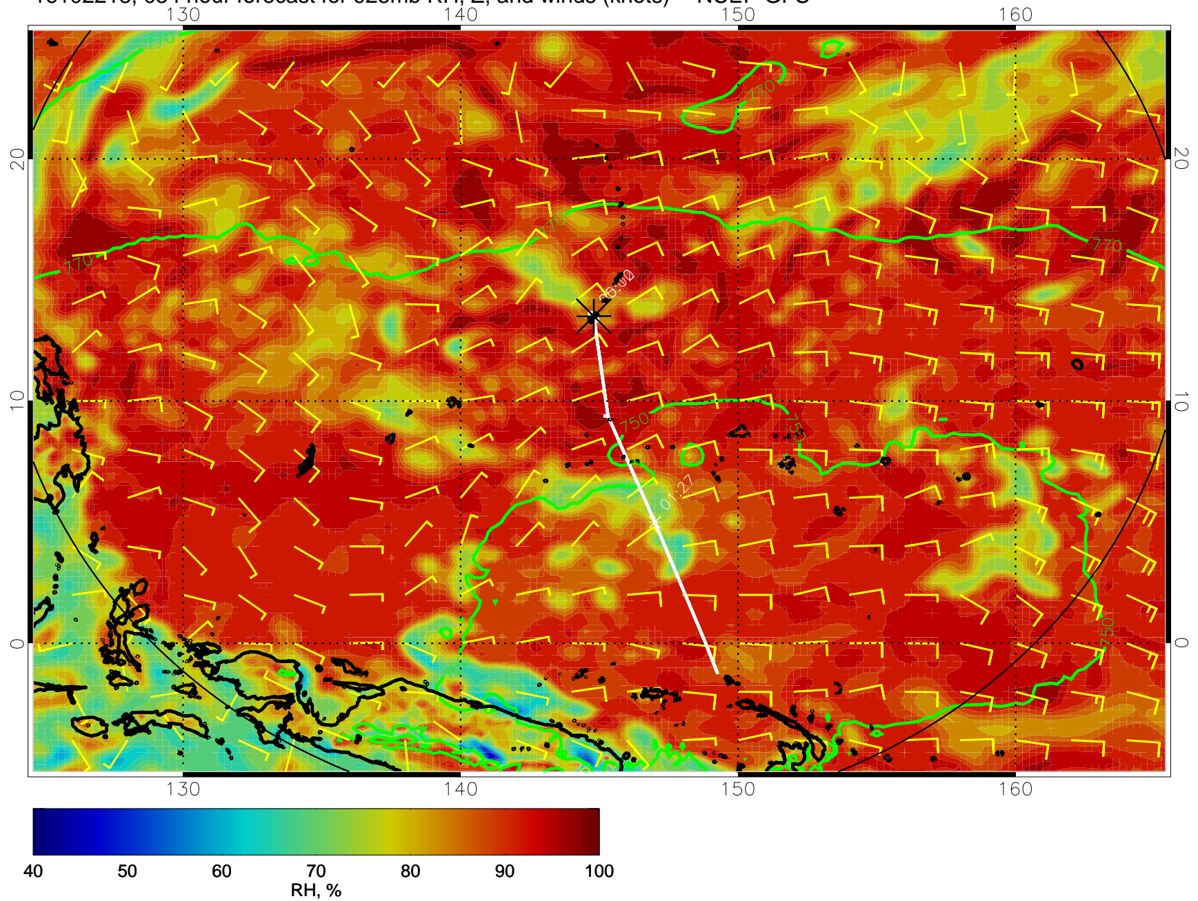
16102218, 054 hour forecast for 925mb RH, Z, and winds (knots) -- NCEP GFS
