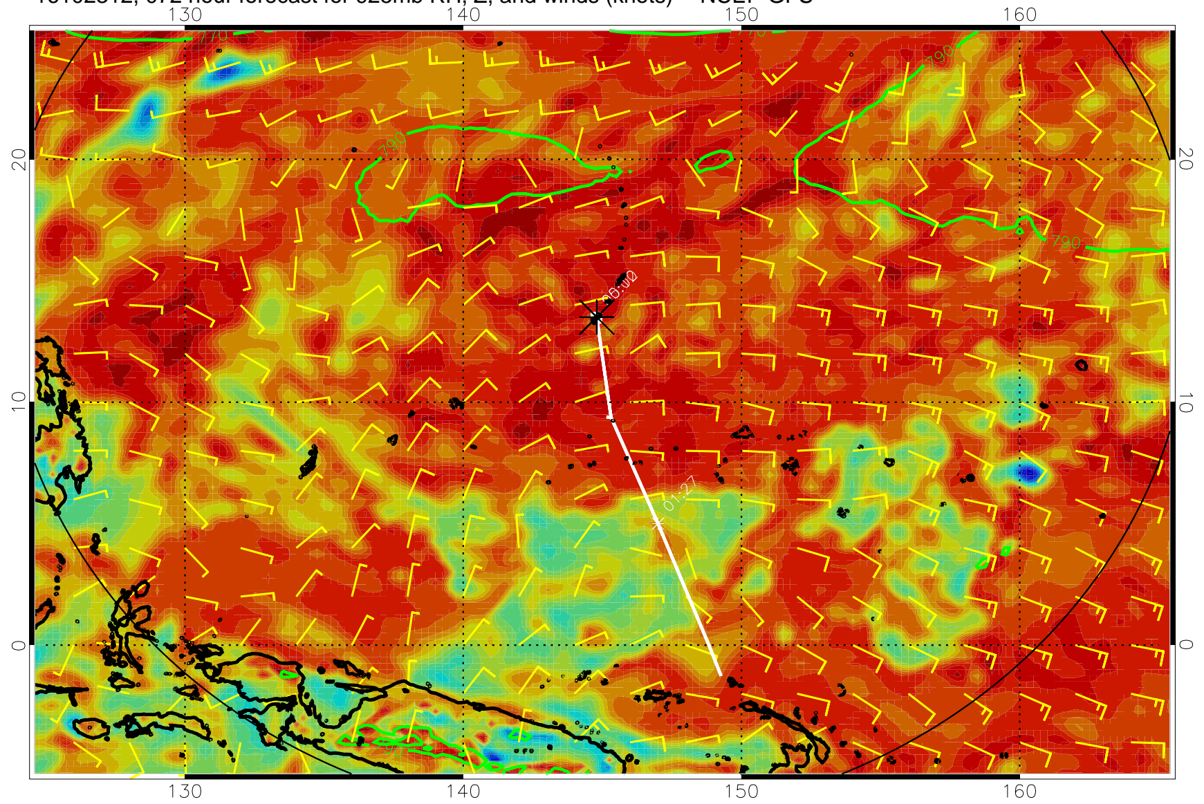
16102312, 072 hour forecast for 925mb RH, Z, and winds (knots) -- NCEP GFS
