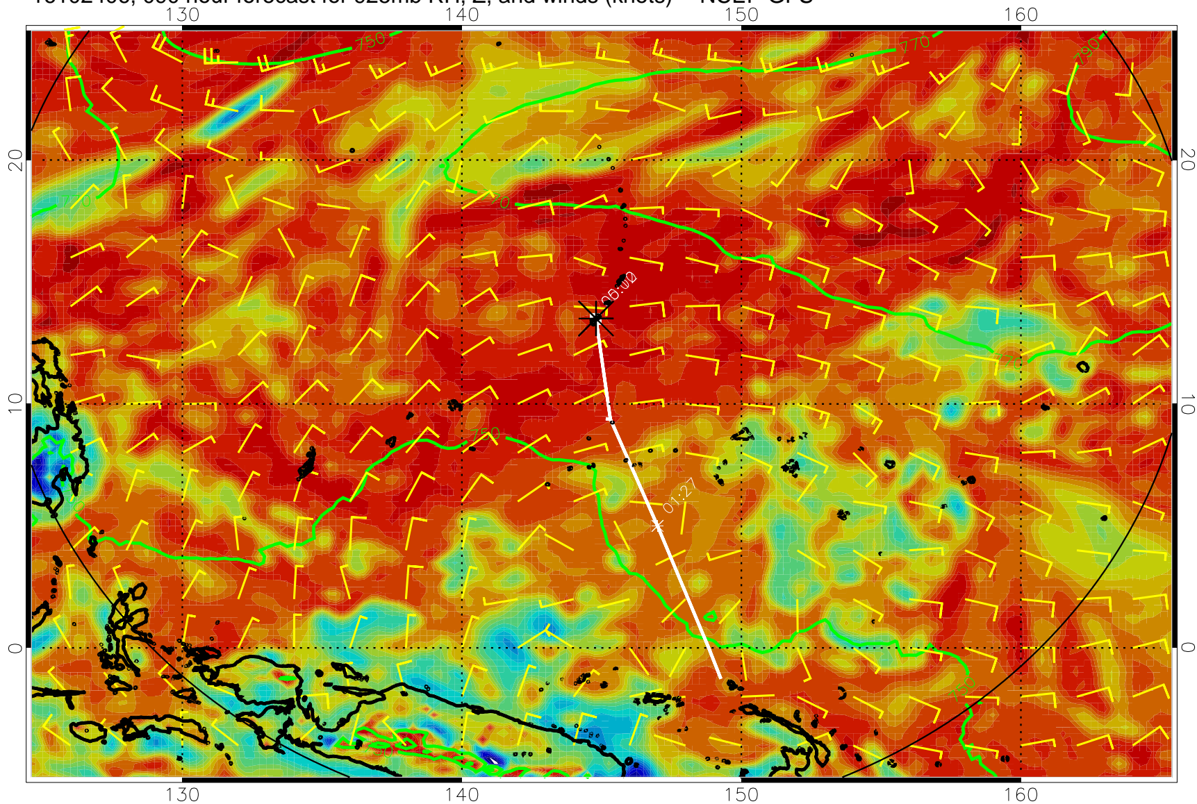
16102406, 090 hour forecast for 925mb RH, Z, and winds (knots) -- NCEP GFS
