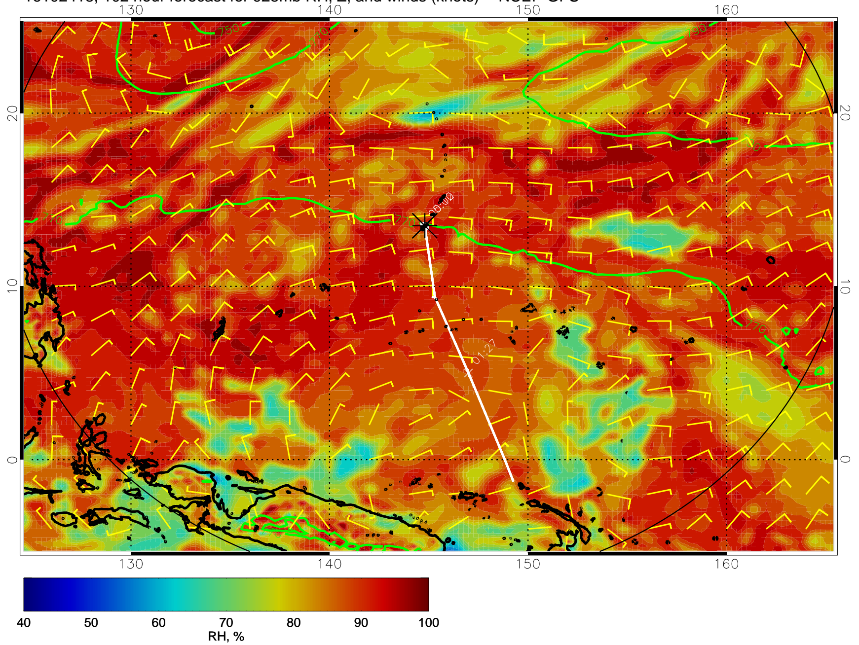
16102418, 102 hour forecast for 925mb RH, Z, and winds (knots) -- NCEP GFS
