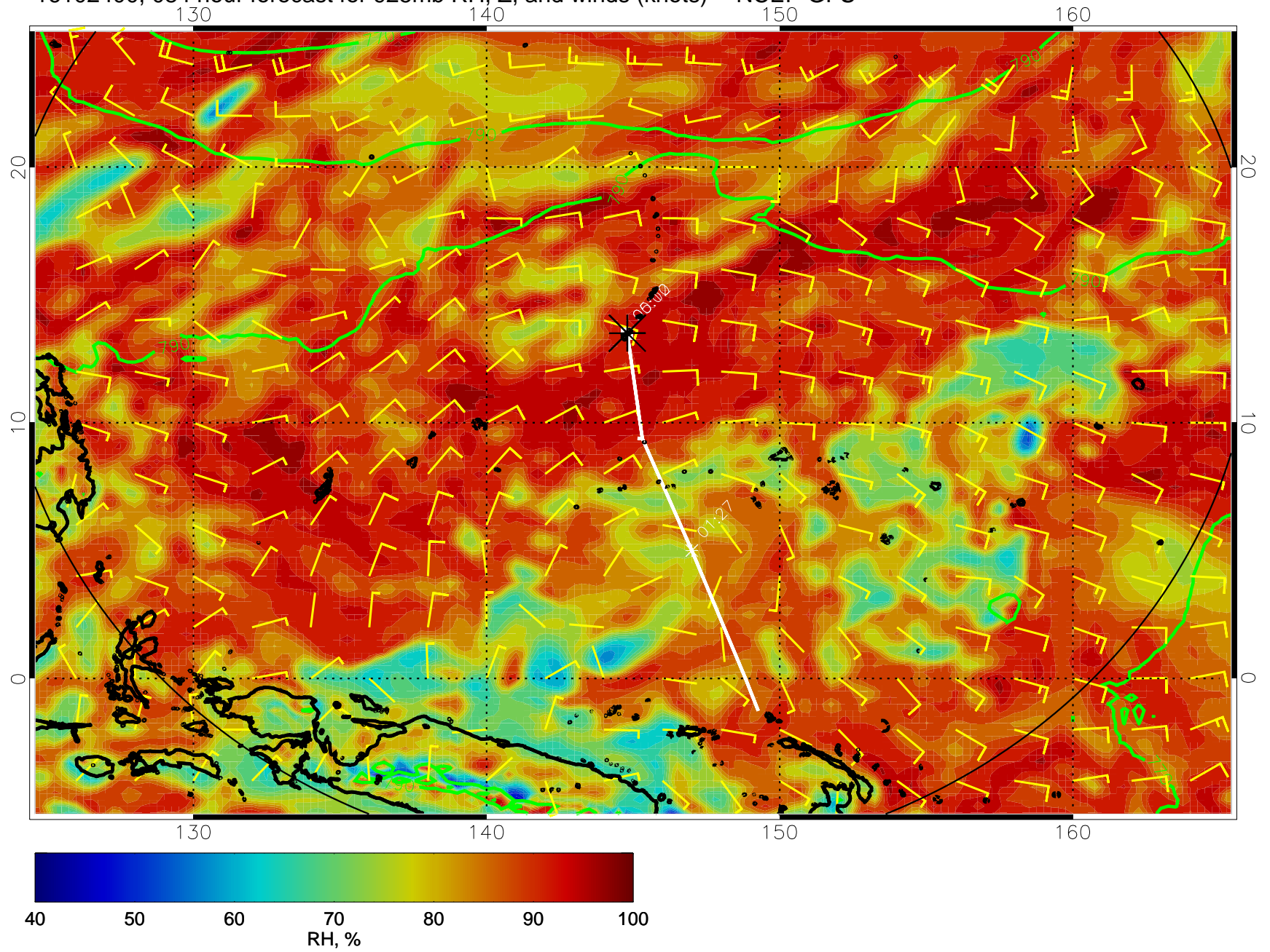
16102400, 084 hour forecast for 925mb RH, Z, and winds (knots) -- NCEP GFS
