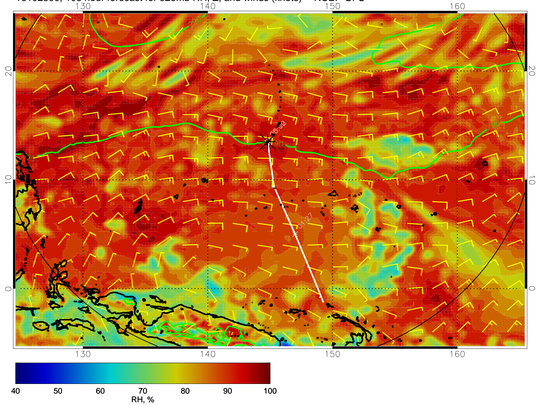
16102500, 108 hour forecast for 925mb RH, Z, and winds (knots) -- NCEP GFS
