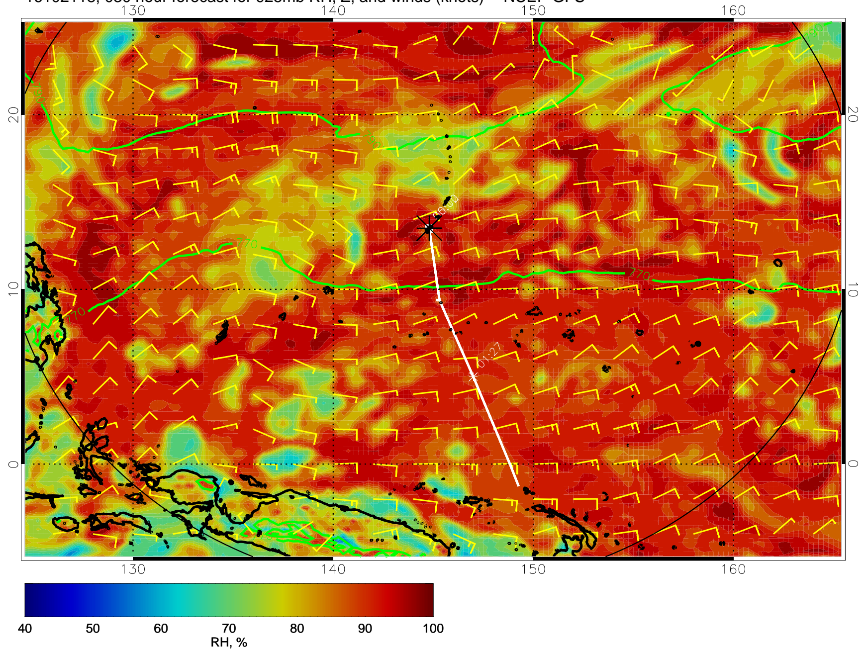
16102118, 030 hour forecast for 925mb RH, Z, and winds (knots) -- NCEP GFS
