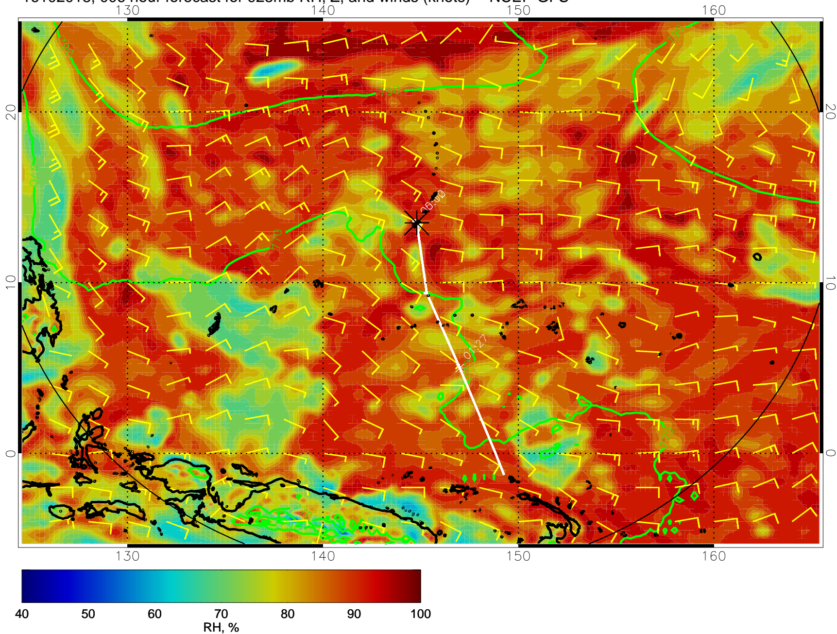
16102018, 006 hour forecast for 925mb RH, Z, and winds (knots) -- NCEP GFS
