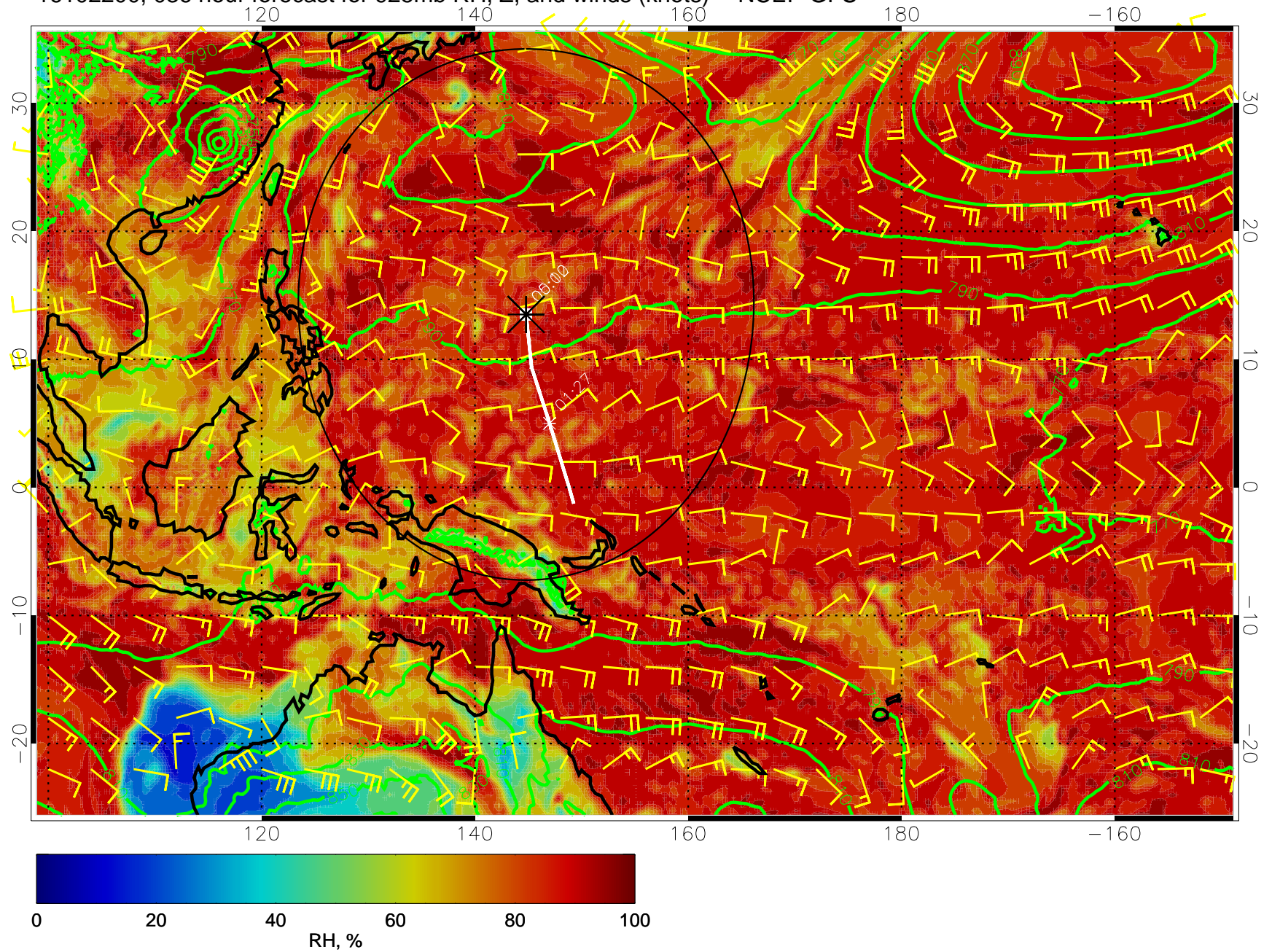
16102200, 036 hour forecast for 925mb RH, Z, and winds (knots) -- NCEP GFS
