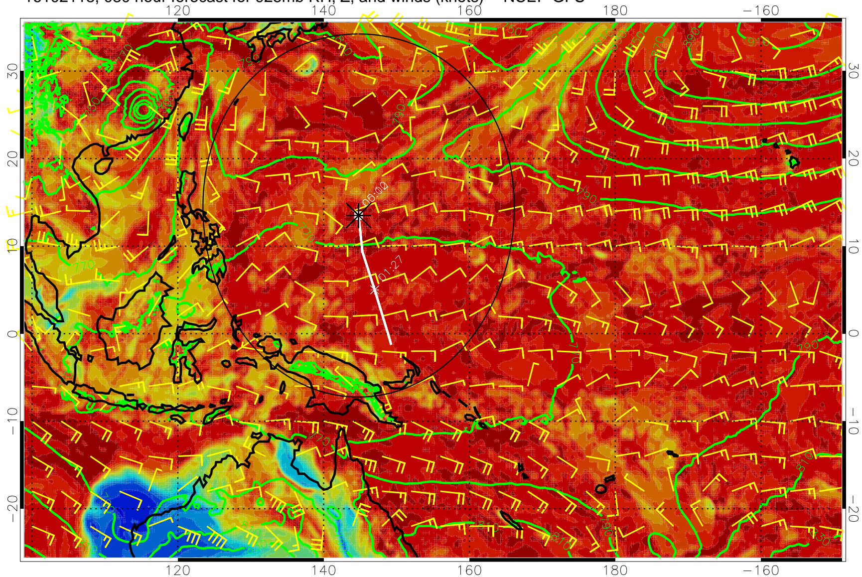
16102118, 030 hour forecast for 925mb RH, Z, and winds (knots) -- NCEP GFS
