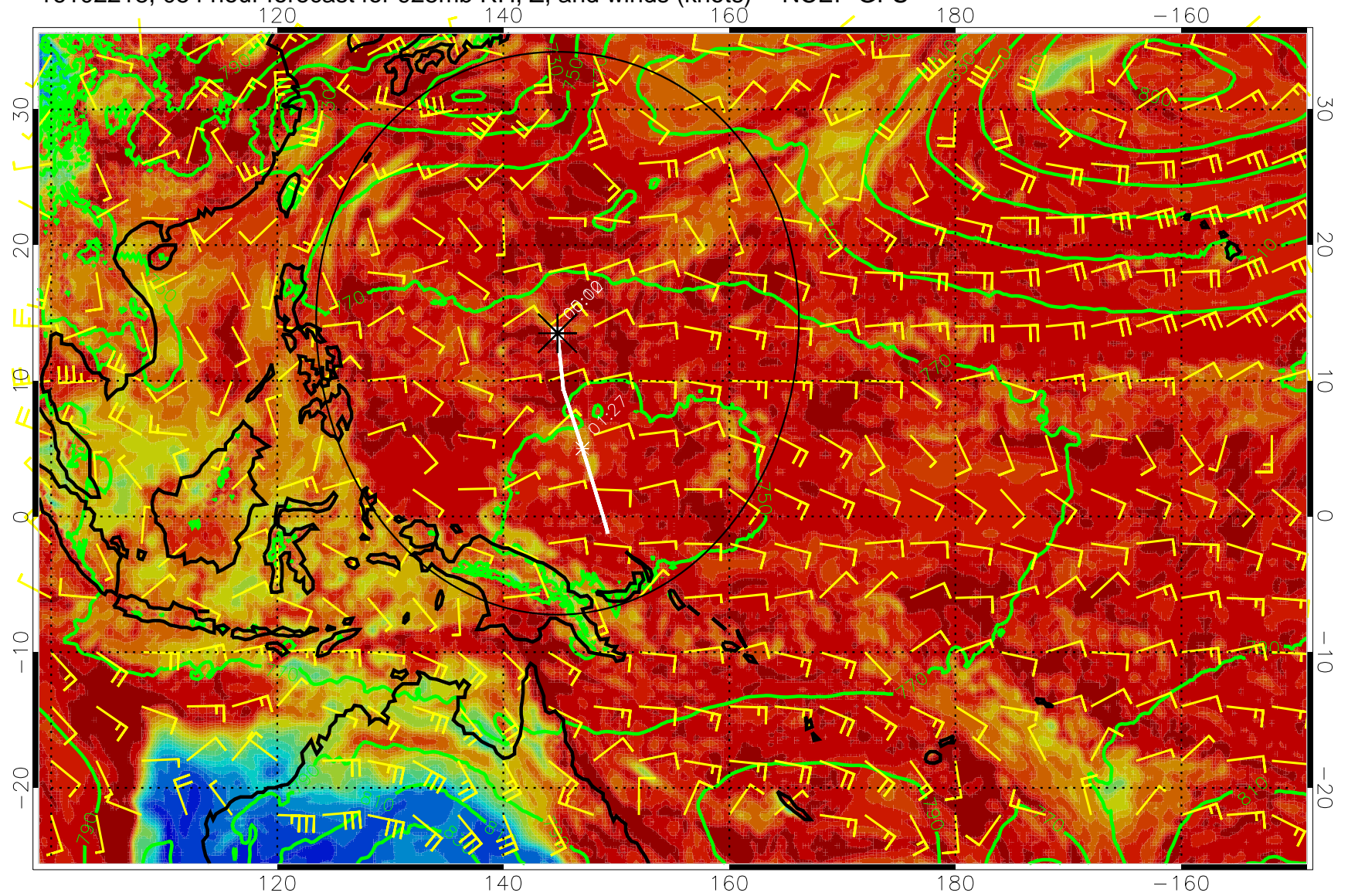
16102218, 054 hour forecast for 925mb RH, Z, and winds (knots) -- NCEP GFS
