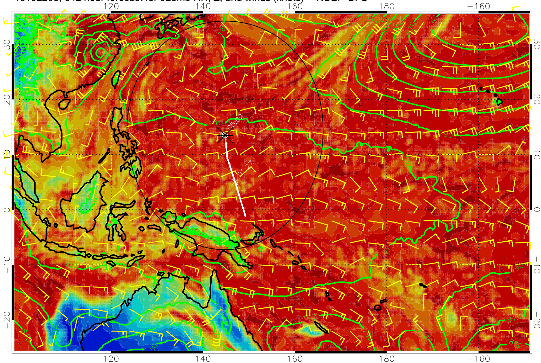
16102206, 042 hour forecast for 925mb RH, Z, and winds (knots) -- NCEP GFS
