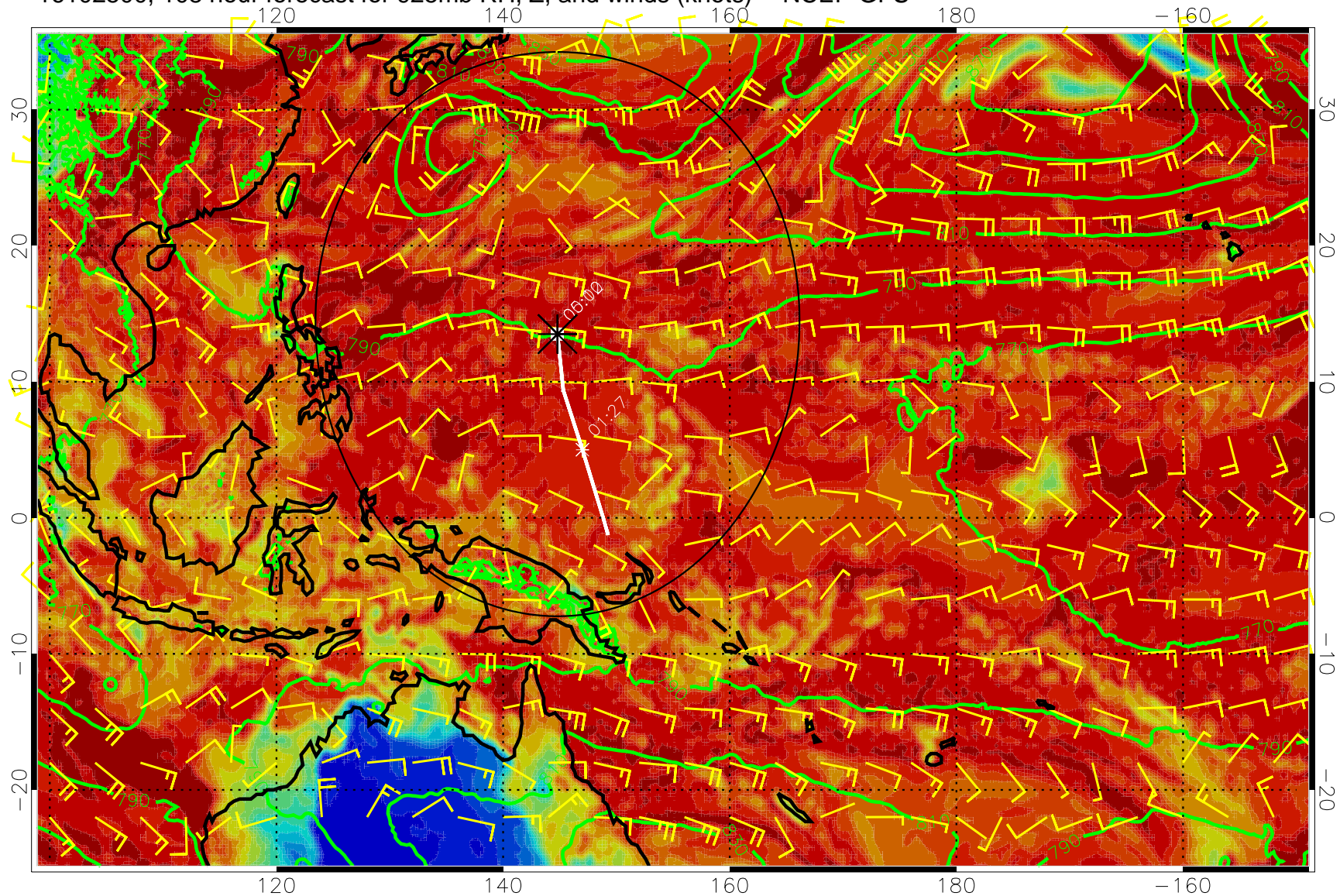
16102500, 108 hour forecast for 925mb RH, Z, and winds (knots) -- NCEP GFS
