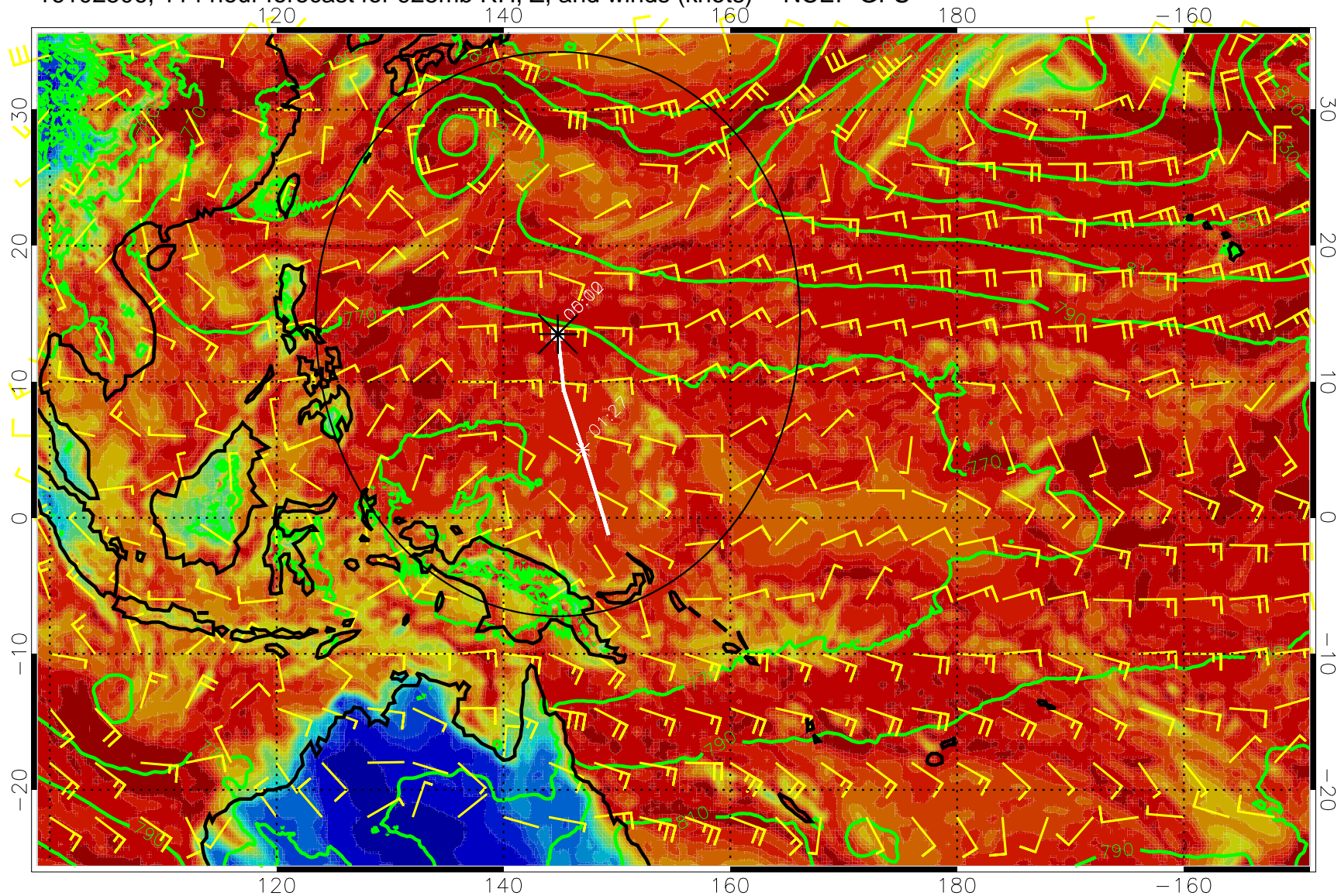
16102506, 114 hour forecast for 925mb RH, Z, and winds (knots) -- NCEP GFS
