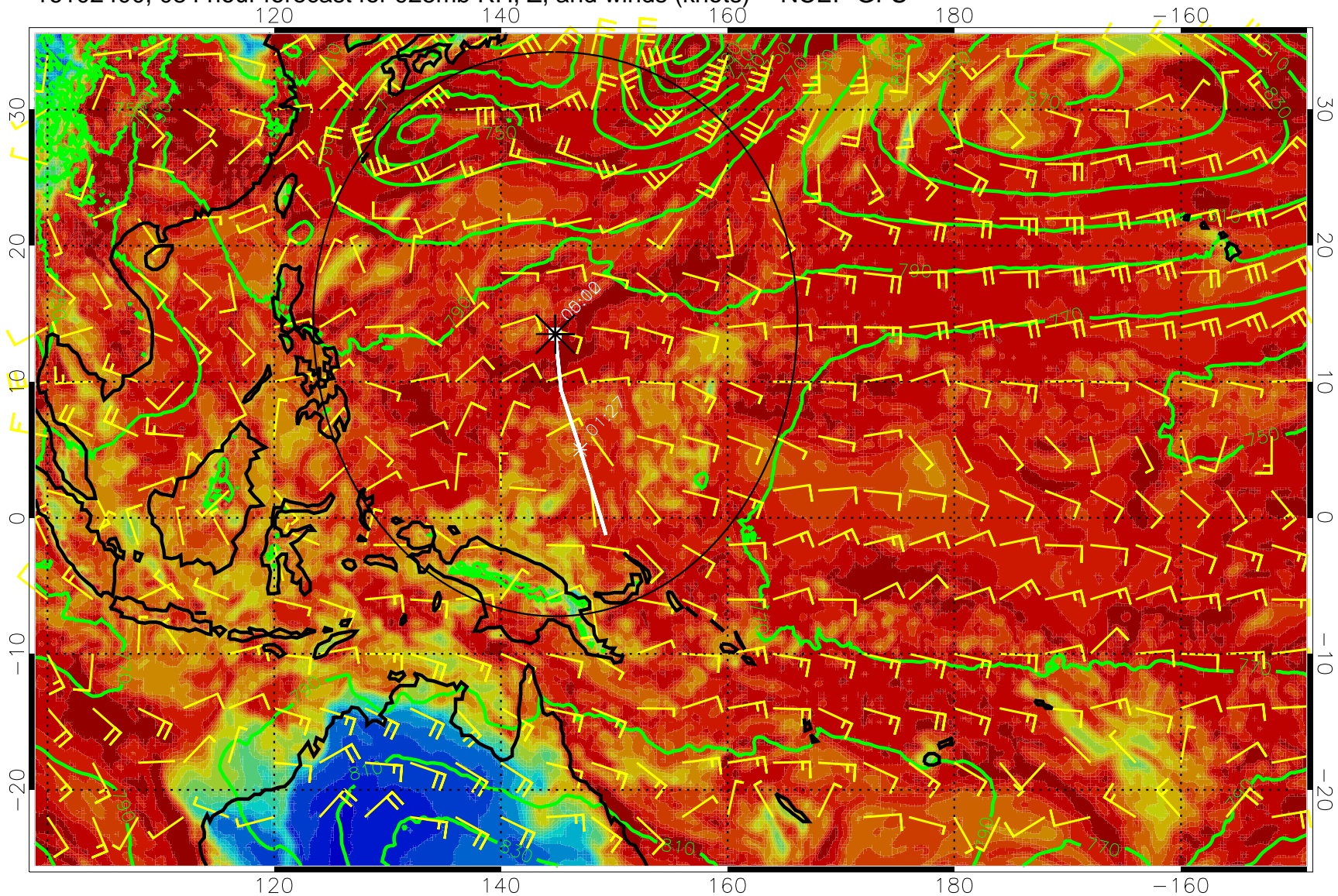
16102400, 084 hour forecast for 925mb RH, Z, and winds (knots) -- NCEP GFS
