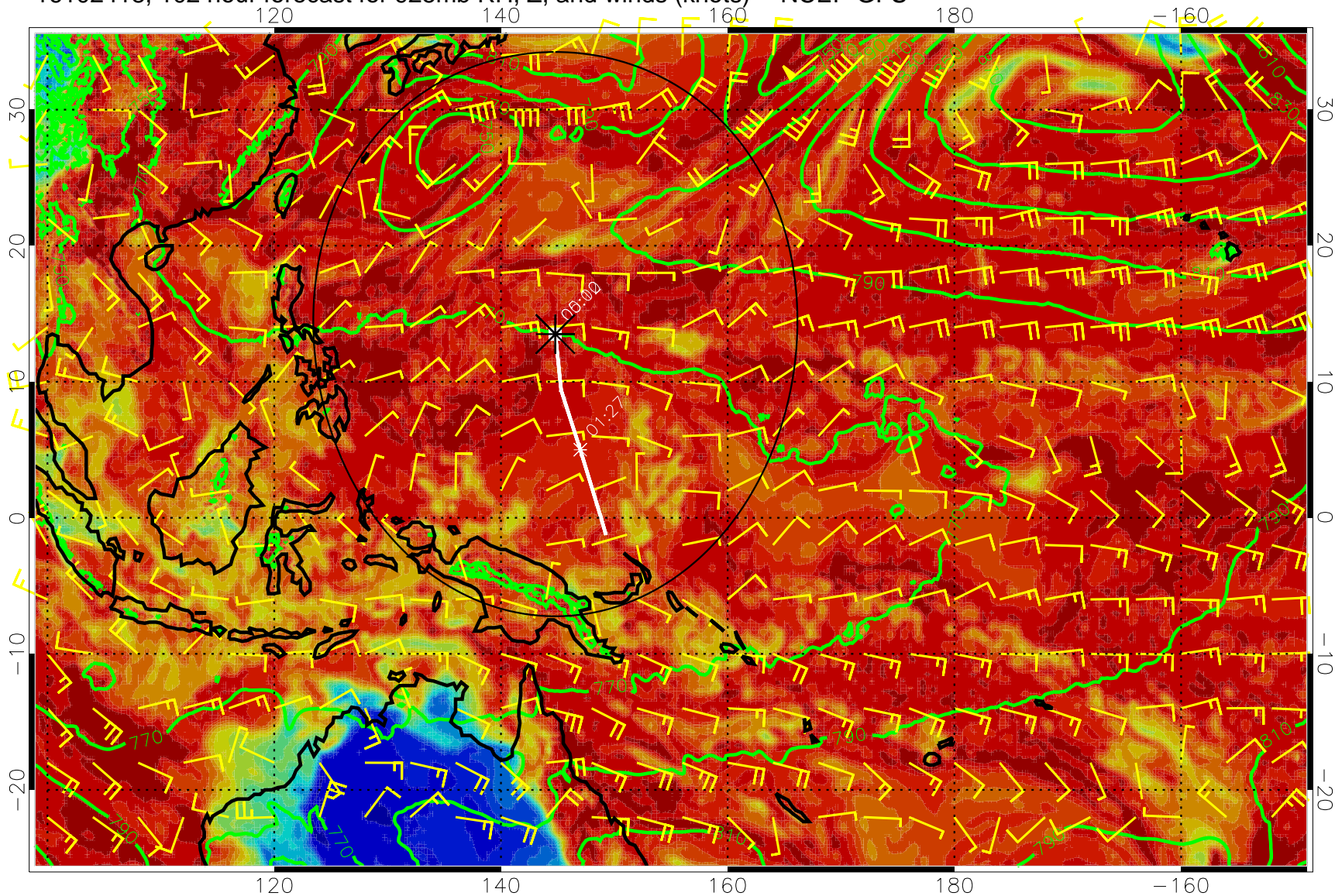
16102418, 102 hour forecast for 925mb RH, Z, and winds (knots) -- NCEP GFS
