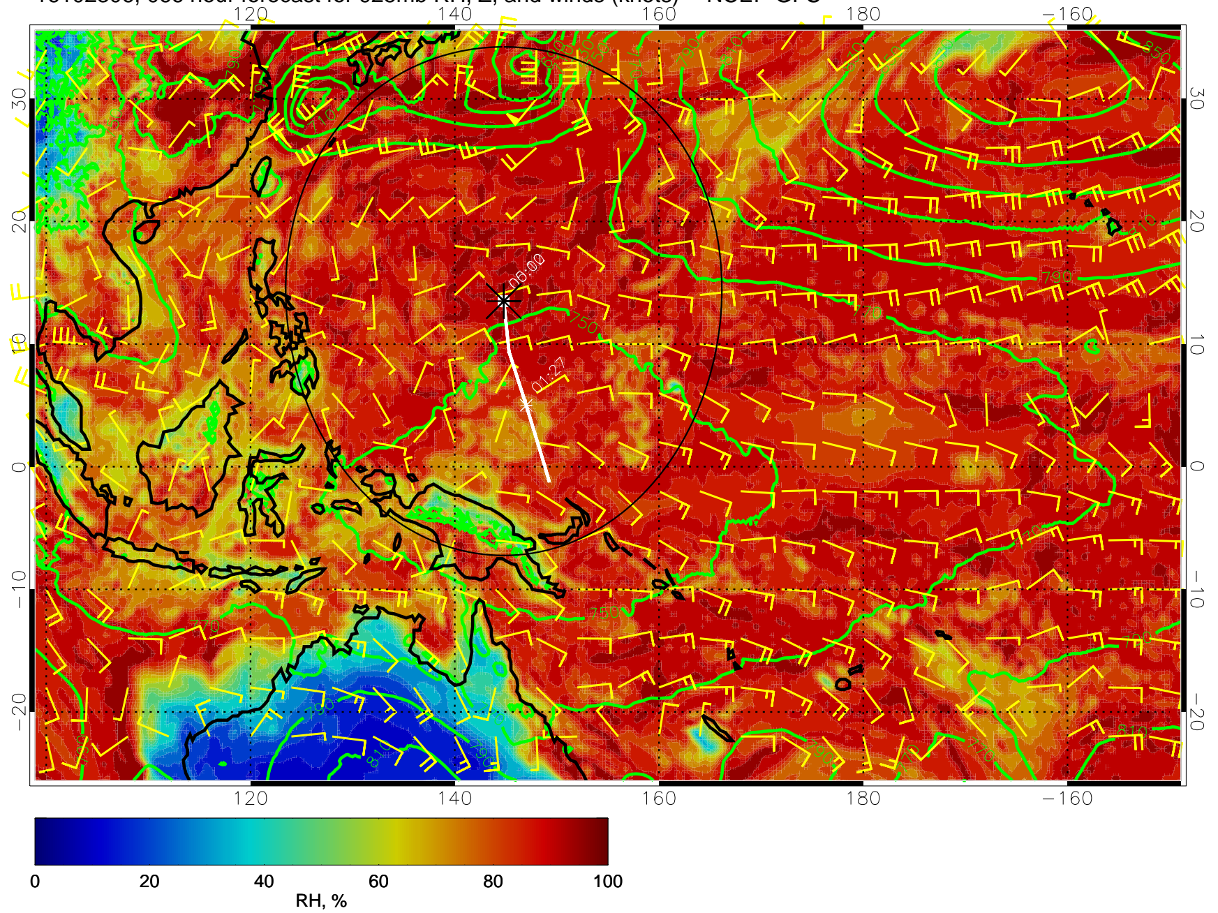
16102306, 066 hour forecast for 925mb RH, Z, and winds (knots) -- NCEP GFS
