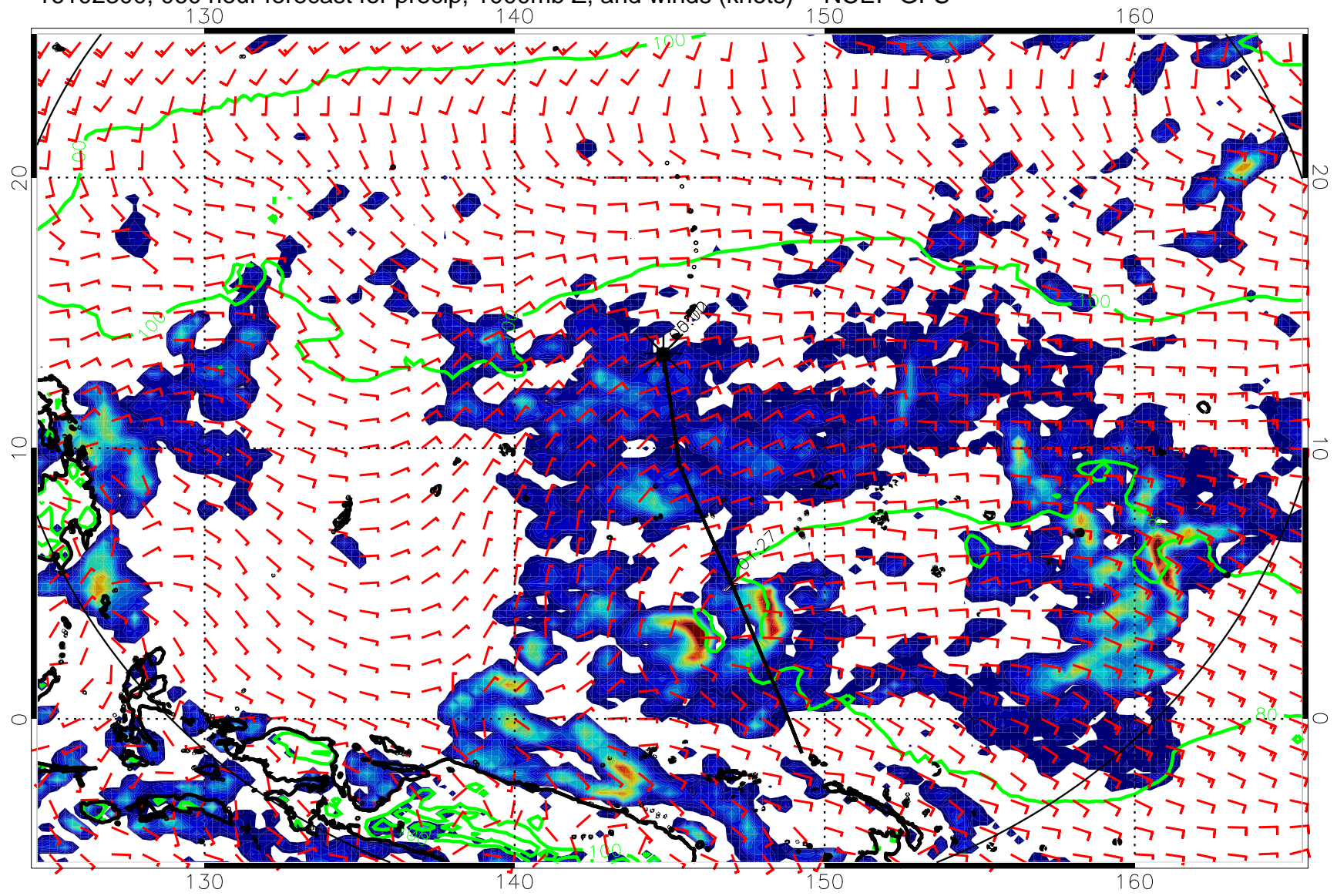
16102300, 060 hour forecast for precip, 1000mb Z, and winds (knots) -- NCEP GFS
