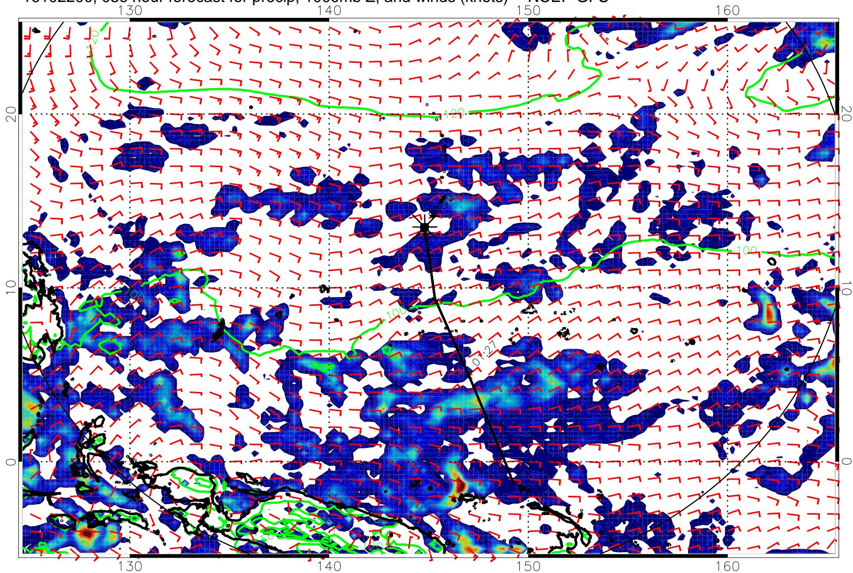
16102200, 036 hour forecast for precip, 1000mb Z, and winds (knots) -- NCEP GFS
