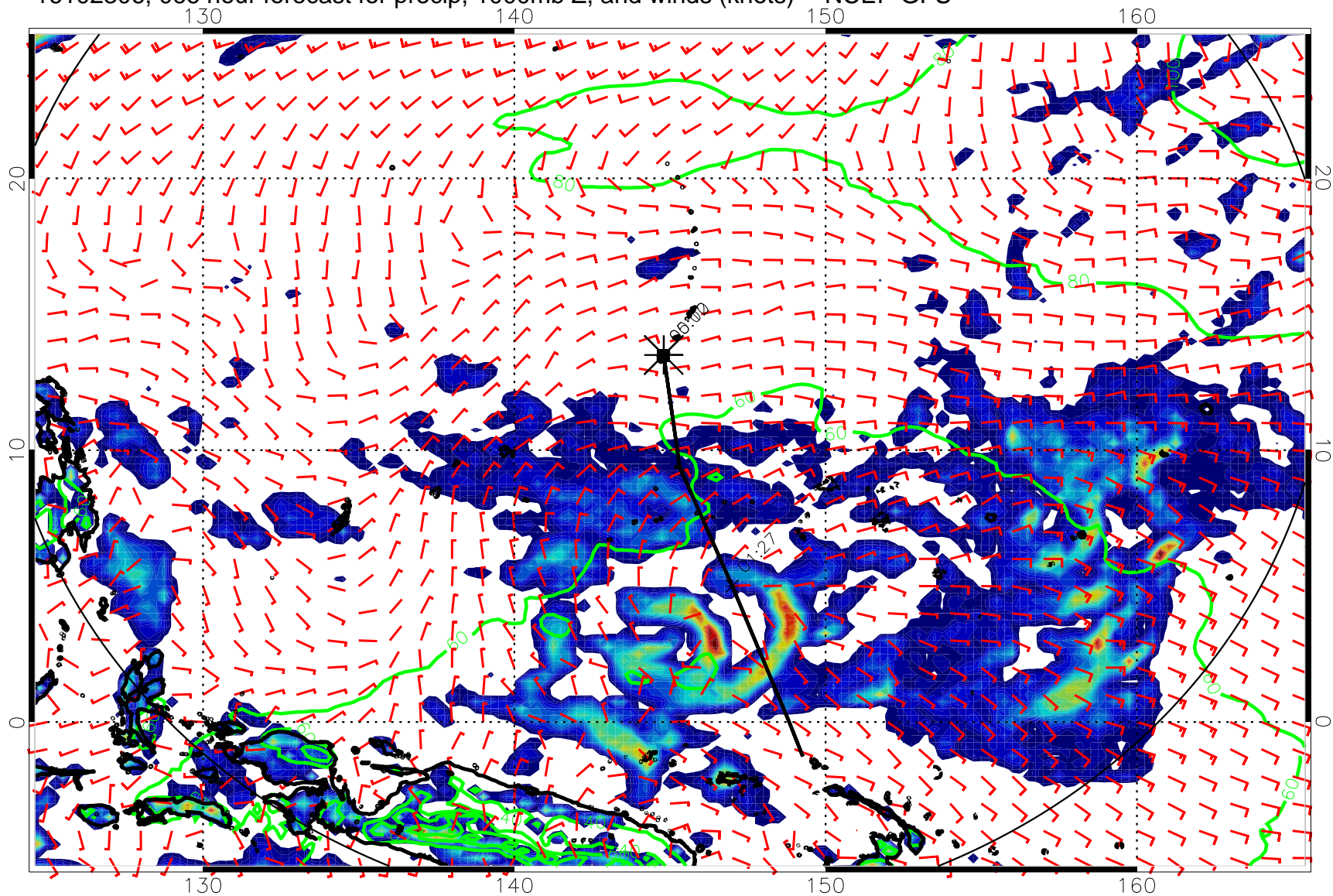
16102306, 066 hour forecast for precip, 1000mb Z, and winds (knots) -- NCEP GFS
