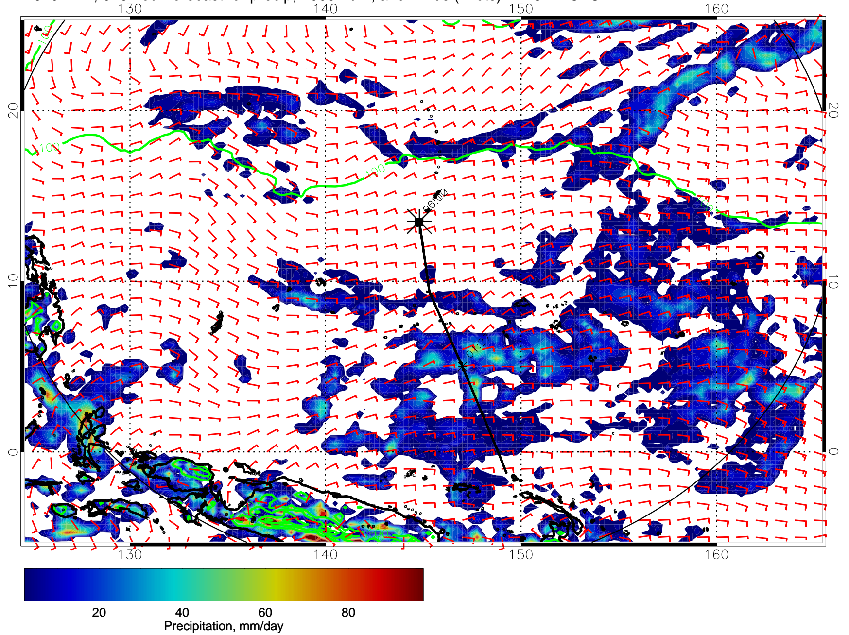
16102212, 048 hour forecast for precip, 1000mb Z, and winds (knots) -- NCEP GFS
