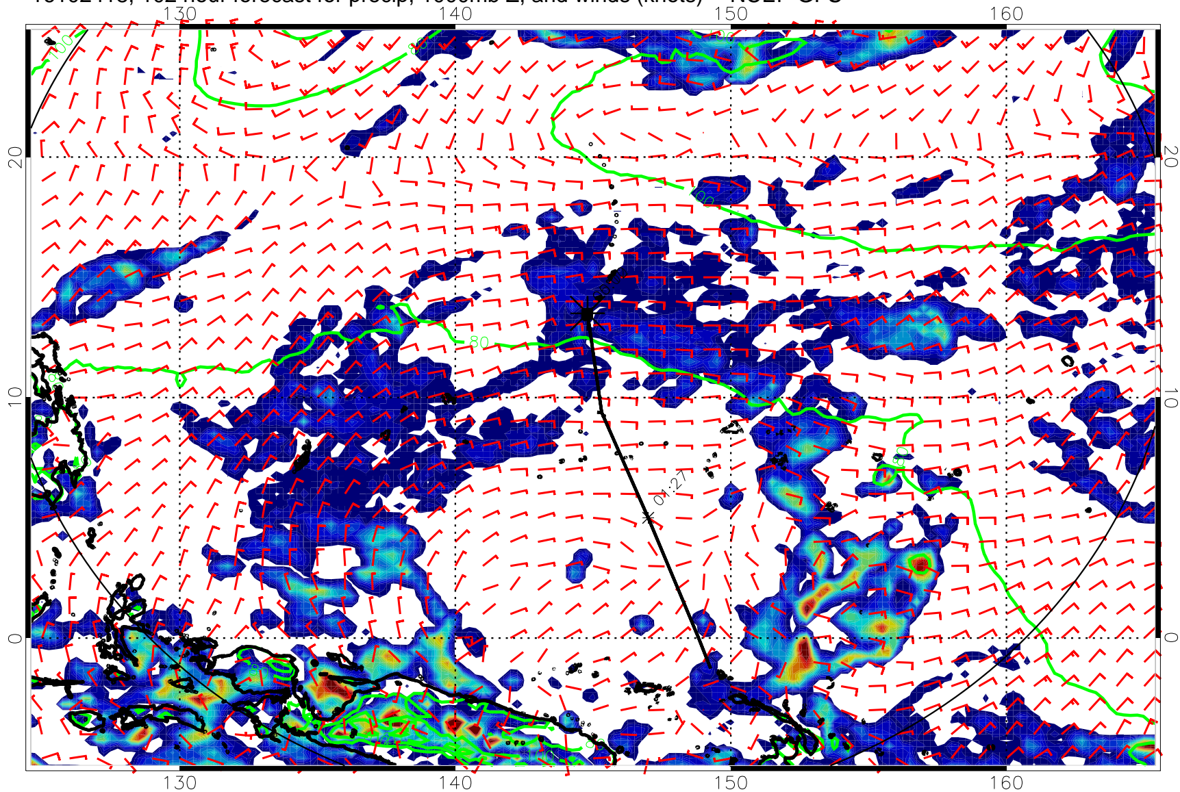
16102418, 102 hour forecast for precip, 1000mb Z, and winds (knots) -- NCEP GFS
