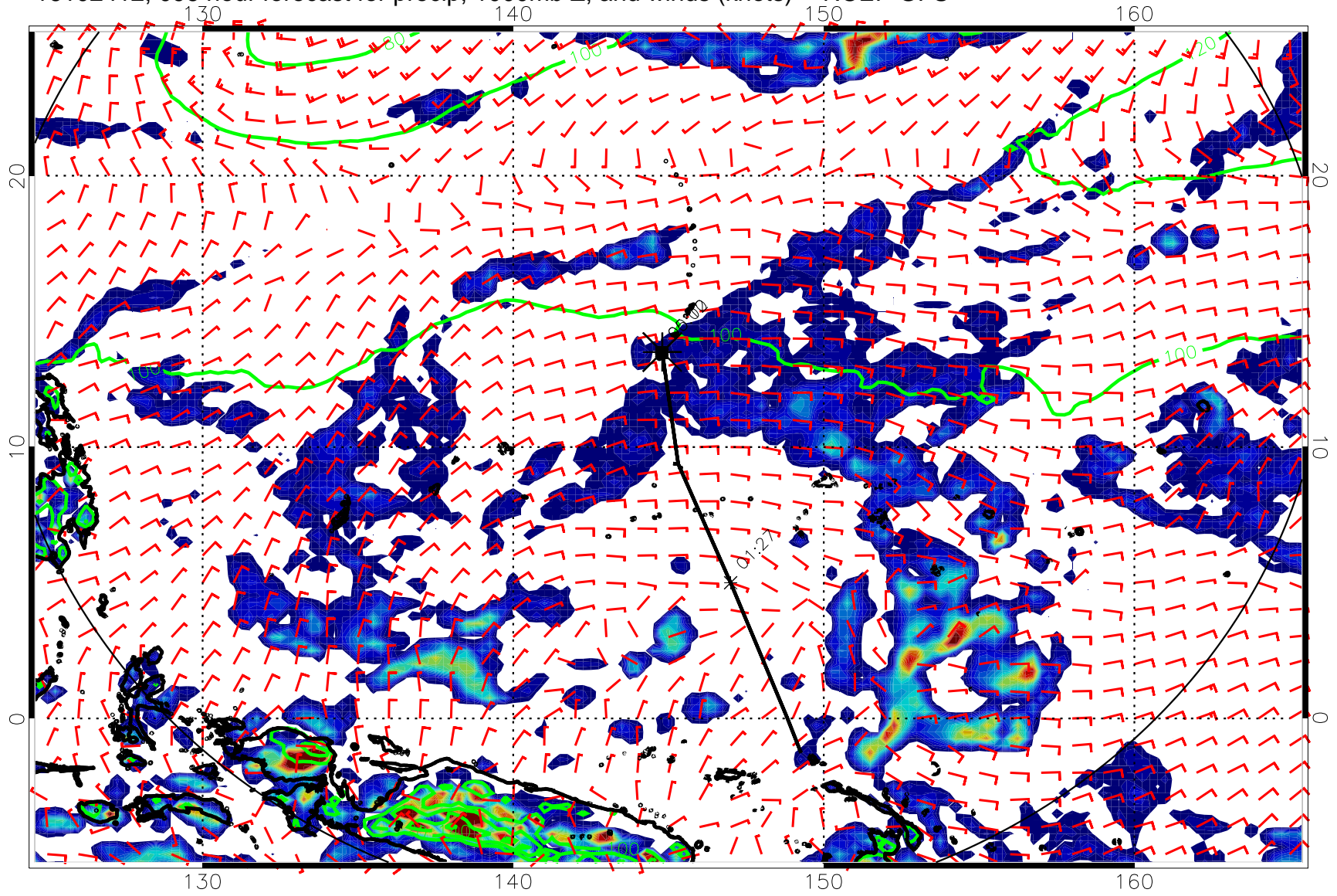
16102412, 096 hour forecast for precip, 1000mb Z, and winds (knots) -- NCEP GFS
