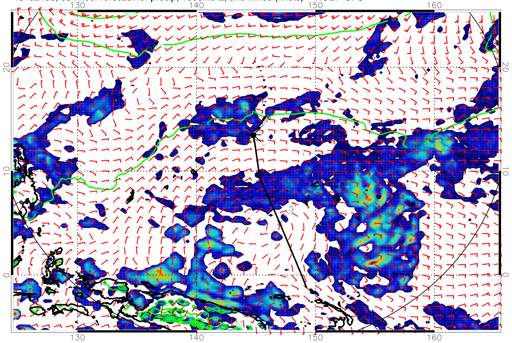
16102400, 084 hour forecast for precip, 1000mb Z, and winds (knots) -- NCEP GFS
