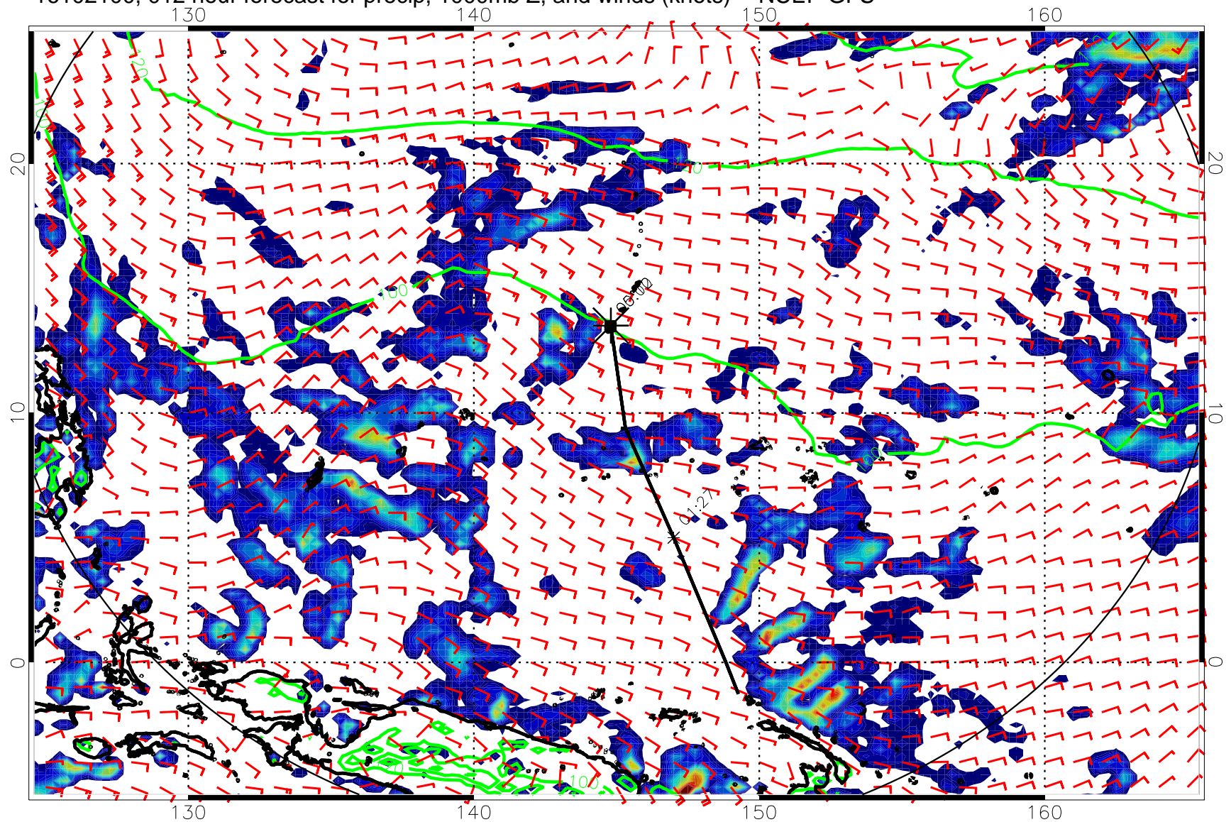
16102100, 012 hour forecast for precip, 1000mb Z, and winds (knots) -- NCEP GFS
