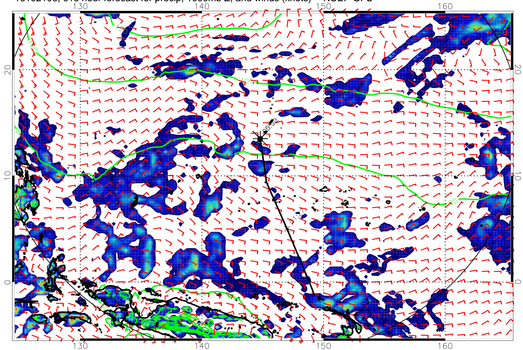
16102106, 018 hour forecast for precip, 1000mb Z, and winds (knots) -- NCEP GFS
