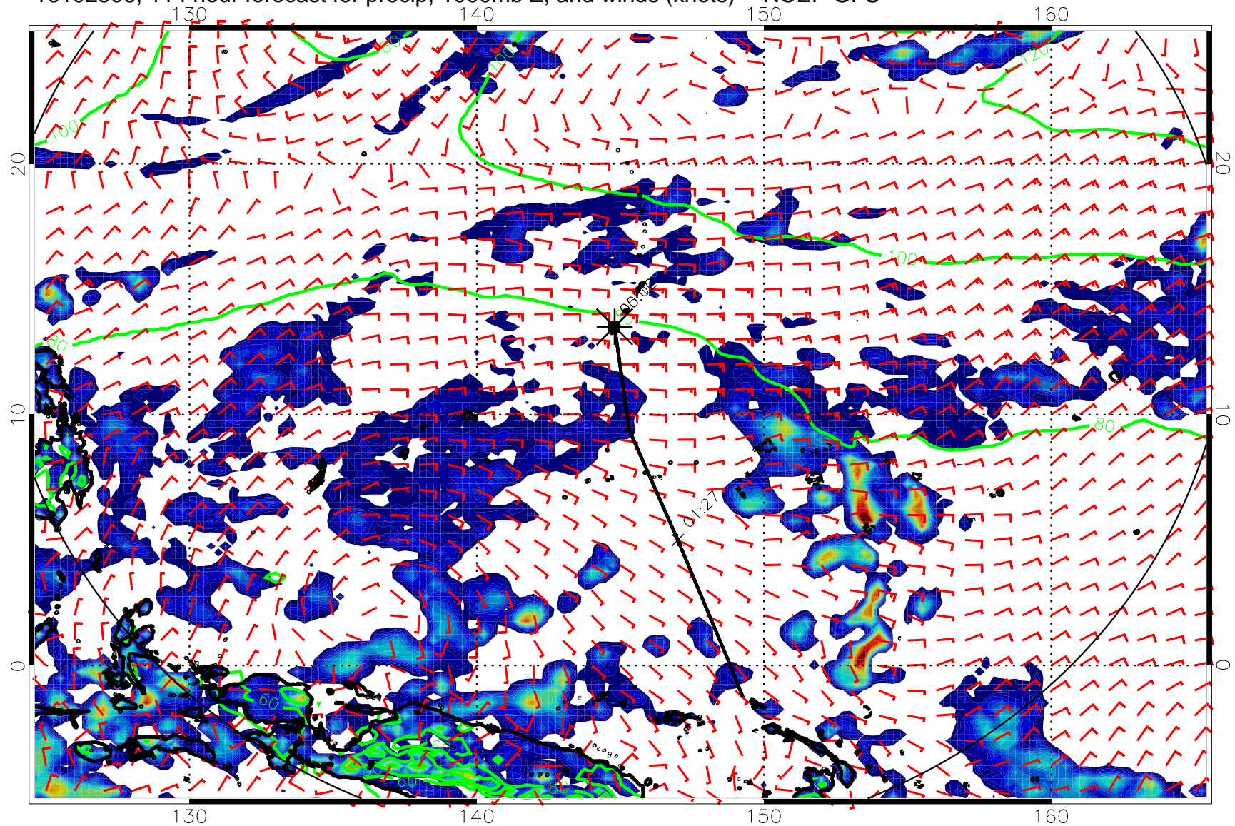
16102506, 114 hour forecast for precip, 1000mb Z, and winds (knots) -- NCEP GFS
