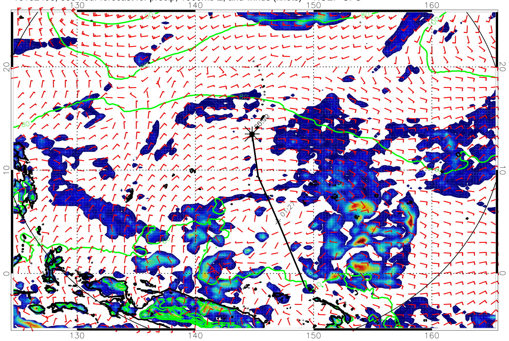
16102406, 090 hour forecast for precip, 1000mb Z, and winds (knots) -- NCEP GFS
