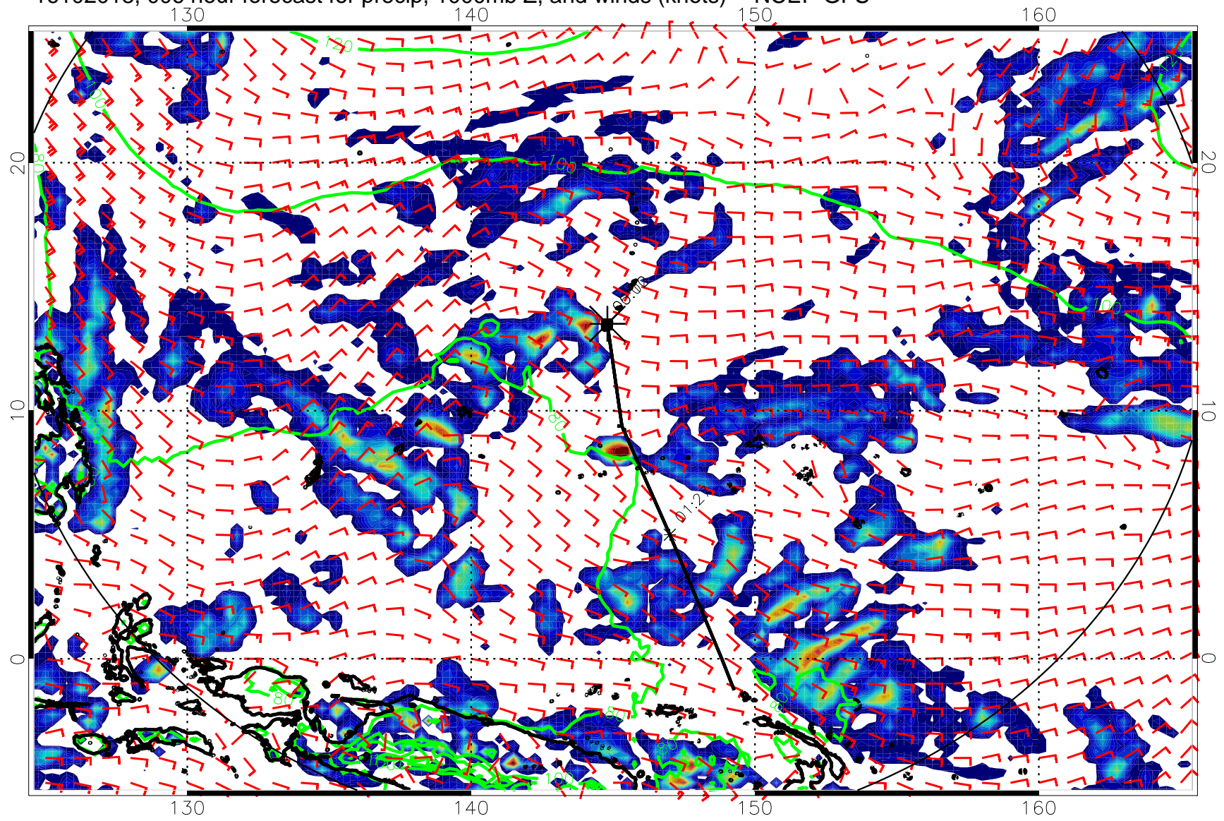
16102018, 006 hour forecast for precip, 1000mb Z, and winds (knots) -- NCEP GFS
