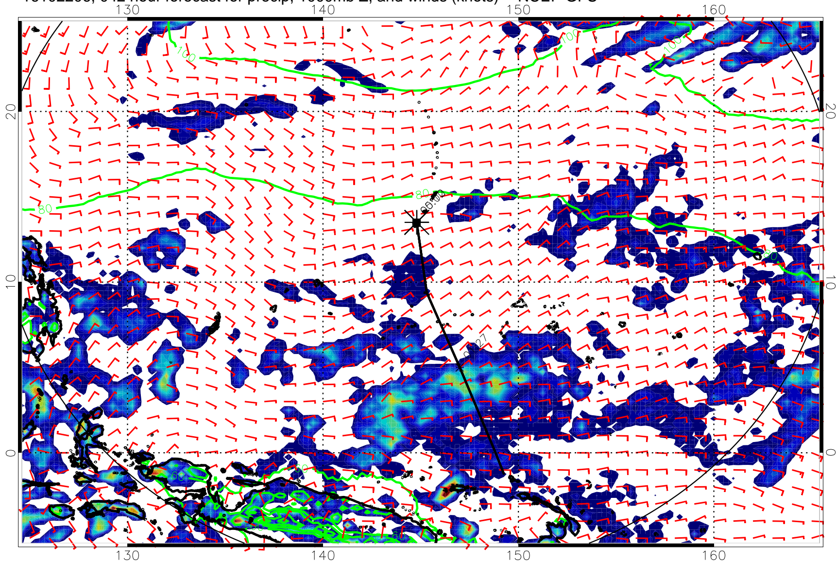
16102206, 042 hour forecast for precip, 1000mb Z, and winds (knots) -- NCEP GFS
