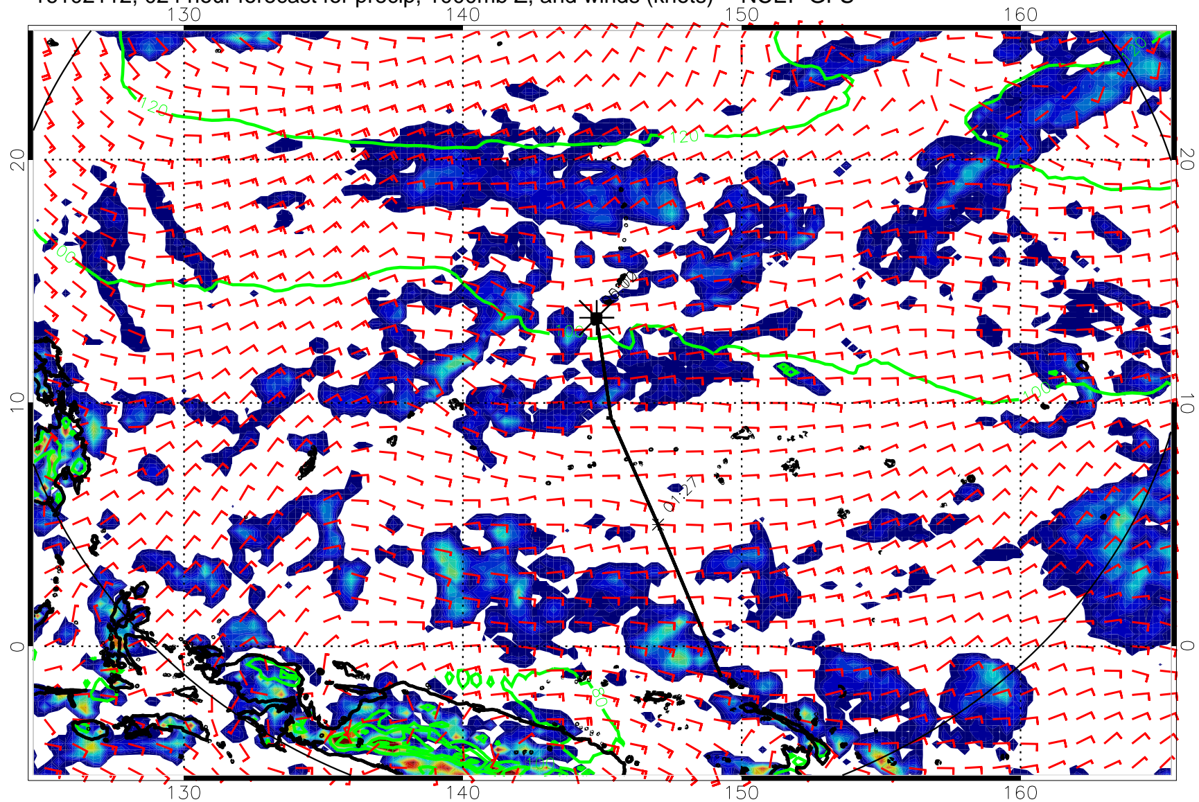
16102112, 024 hour forecast for precip, 1000mb Z, and winds (knots) -- NCEP GFS
