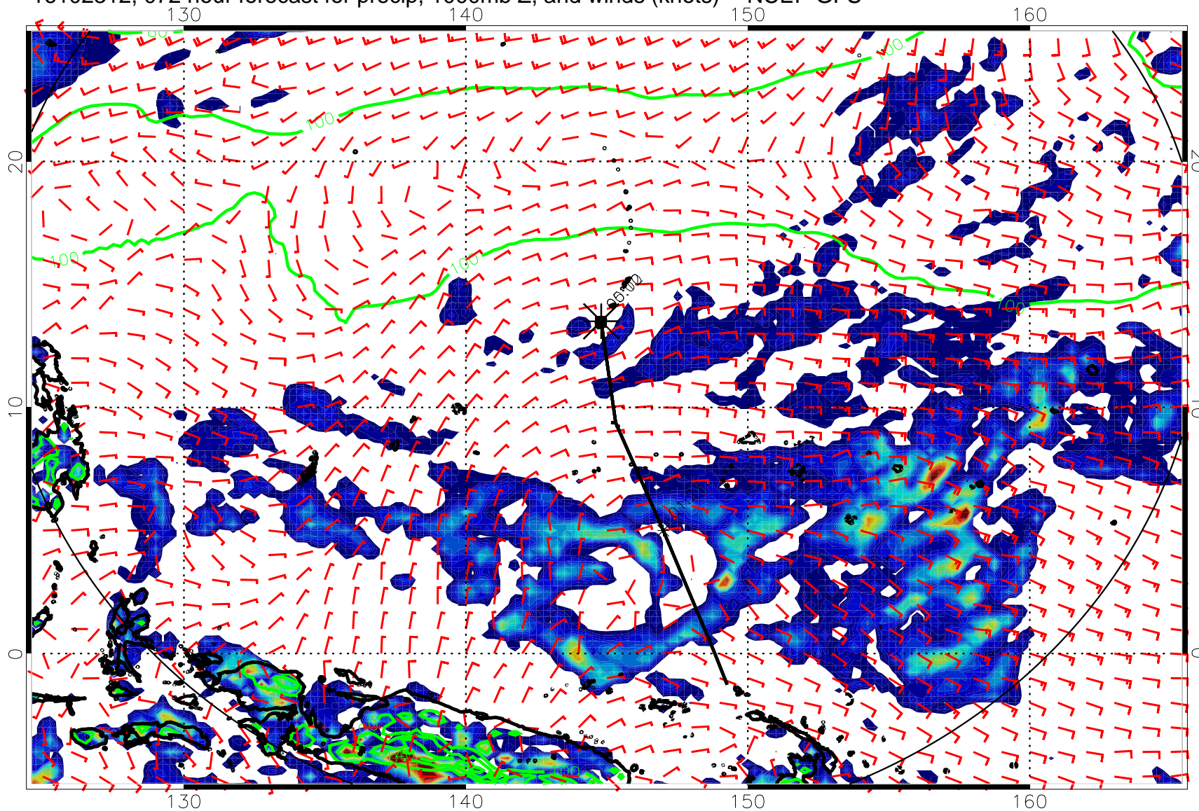
16102312, 072 hour forecast for precip, 1000mb Z, and winds (knots) -- NCEP GFS
