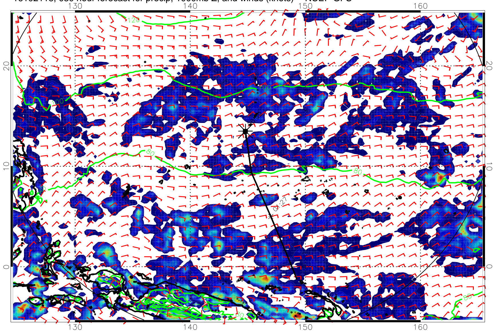
16102118, 030 hour forecast for precip, 1000mb Z, and winds (knots) -- NCEP GFS
