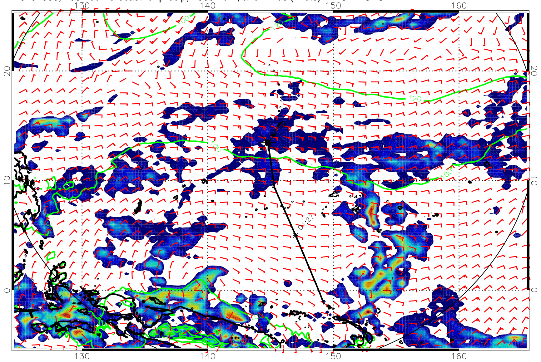
16102500, 108 hour forecast for precip, 1000mb Z, and winds (knots) -- NCEP GFS
