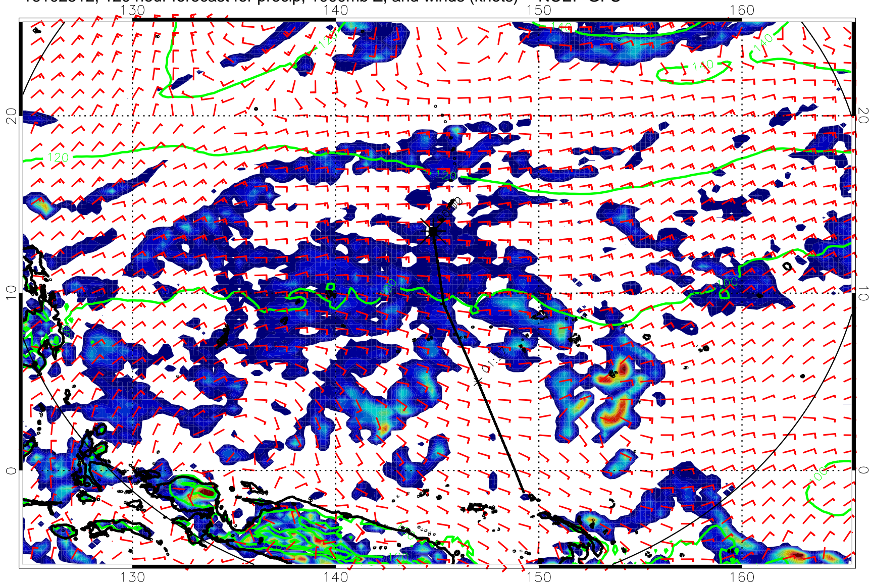
16102512, 120 hour forecast for precip, 1000mb Z, and winds (knots) -- NCEP GFS
