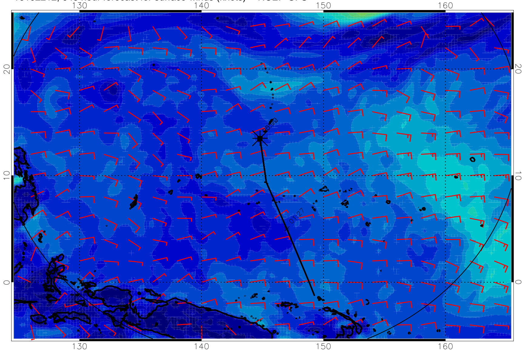
16102212, 048 hour forecast for surface winds (knots) -- NCEP GFS
