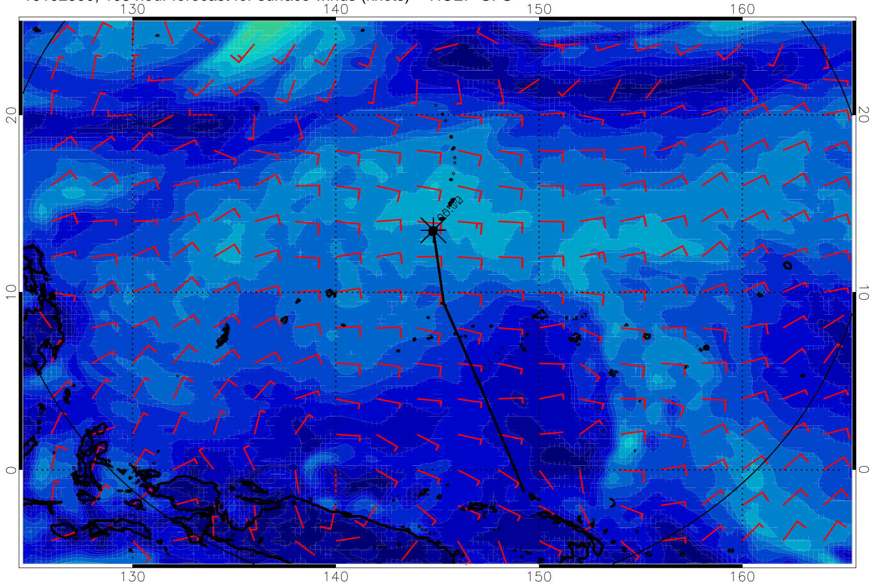
16102500, 108 hour forecast for surface winds (knots) -- NCEP GFS
