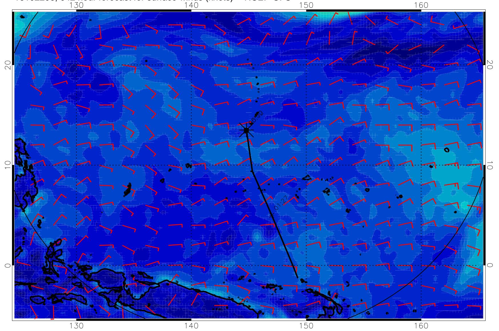
16102206, 042 hour forecast for surface winds (knots) -- NCEP GFS
