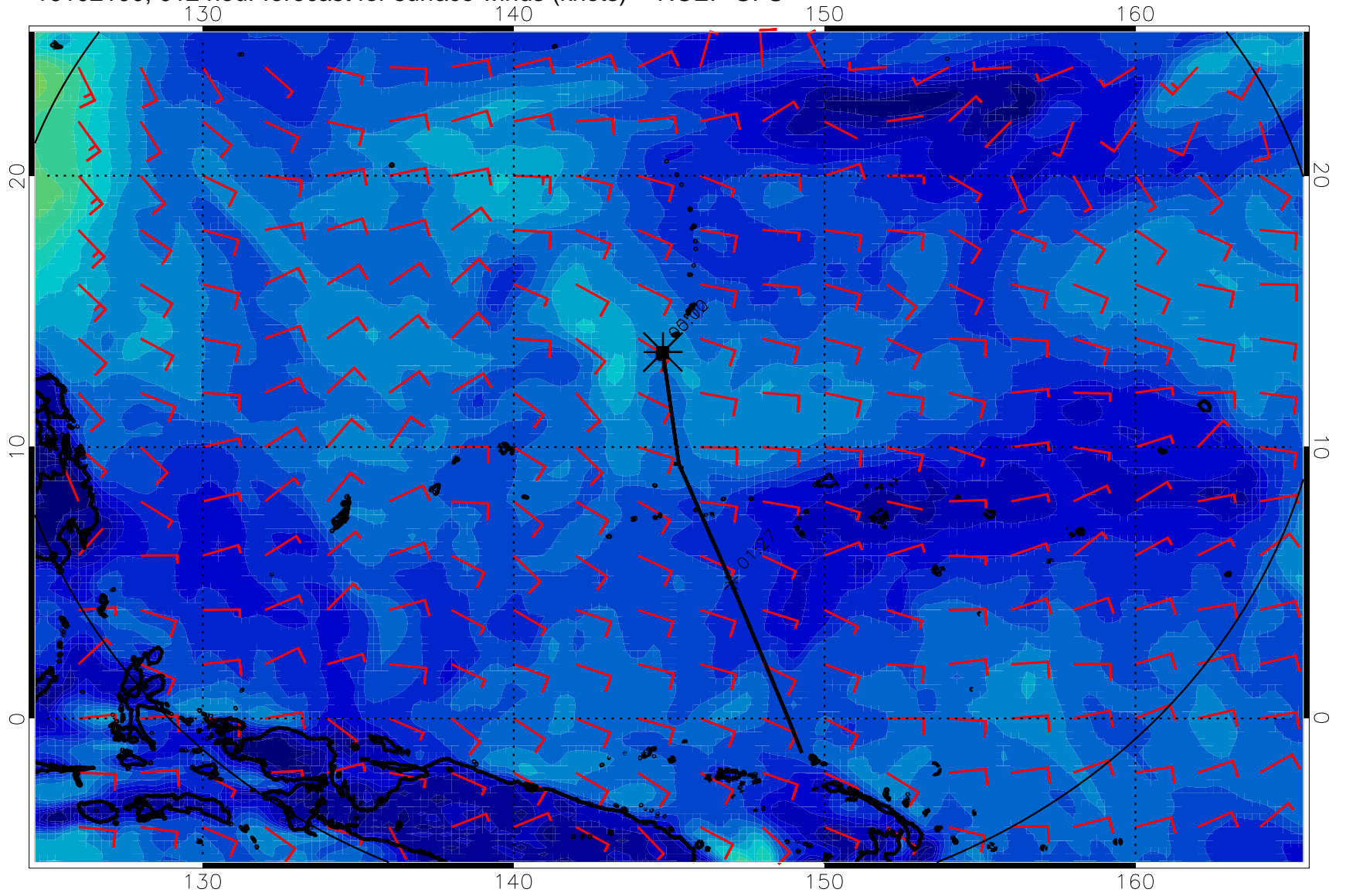
16102100, 012 hour forecast for surface winds (knots) -- NCEP GFS
