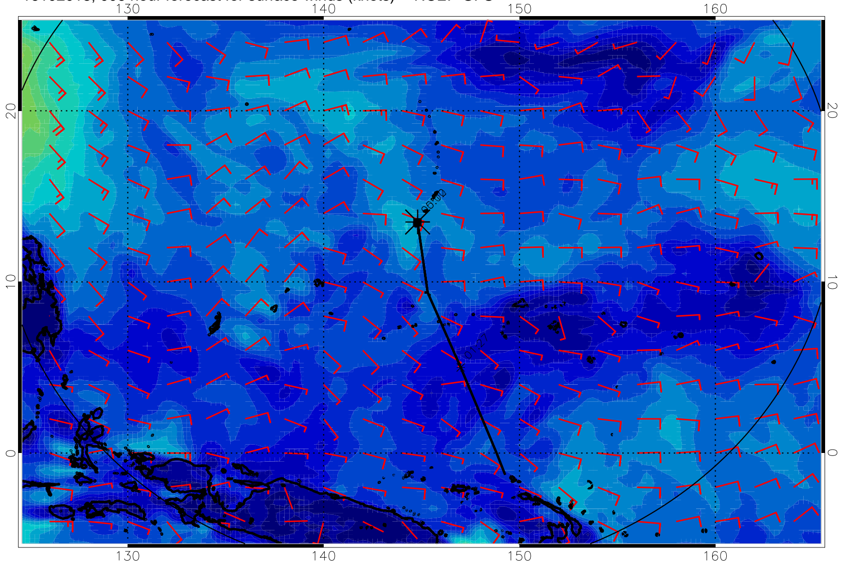
16102018, 006 hour forecast for surface winds (knots) -- NCEP GFS
