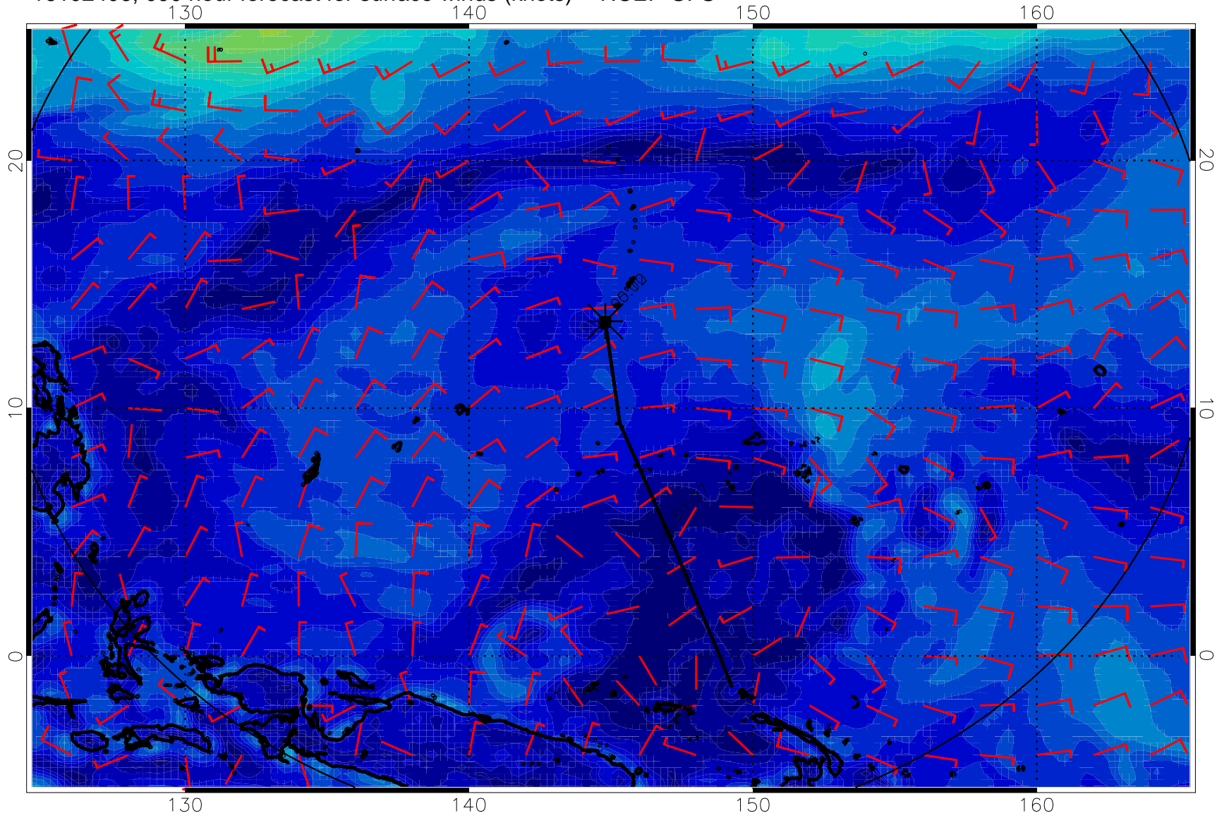
16102406, 090 hour forecast for surface winds (knots) -- NCEP GFS
