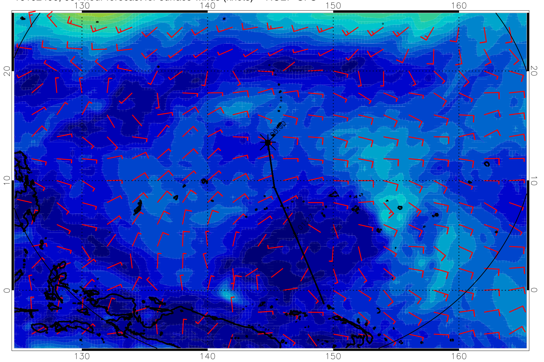
16102400, 084 hour forecast for surface winds (knots) -- NCEP GFS
