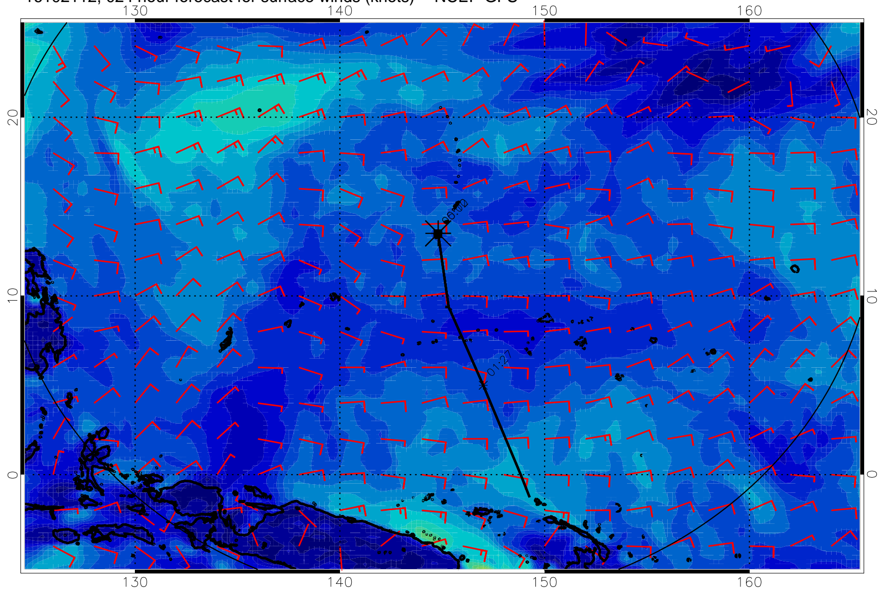
16102112, 024 hour forecast for surface winds (knots) -- NCEP GFS
