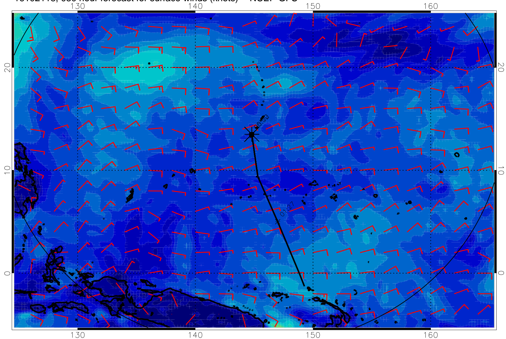
16102118, 030 hour forecast for surface winds (knots) -- NCEP GFS
