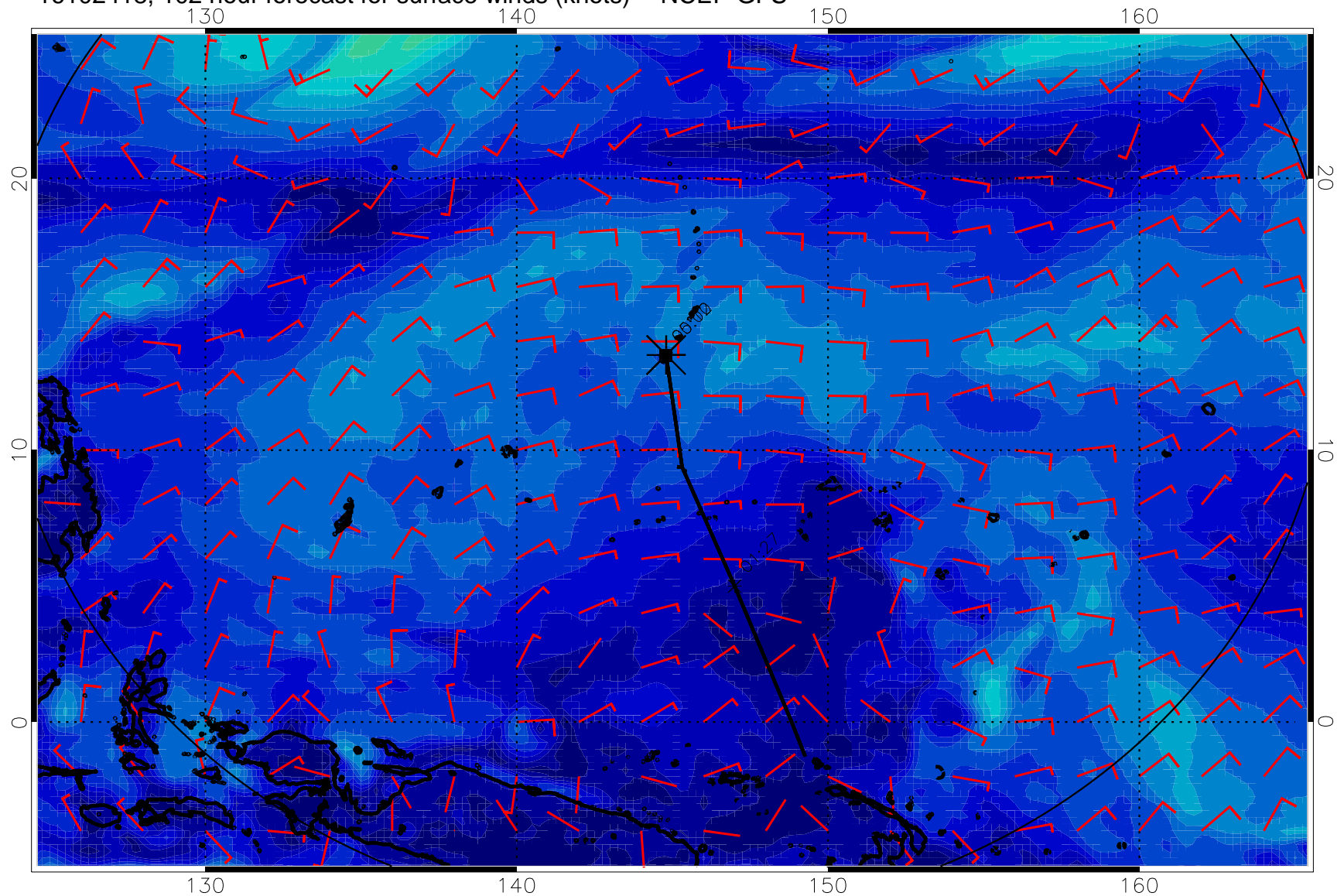
16102418, 102 hour forecast for surface winds (knots) -- NCEP GFS
