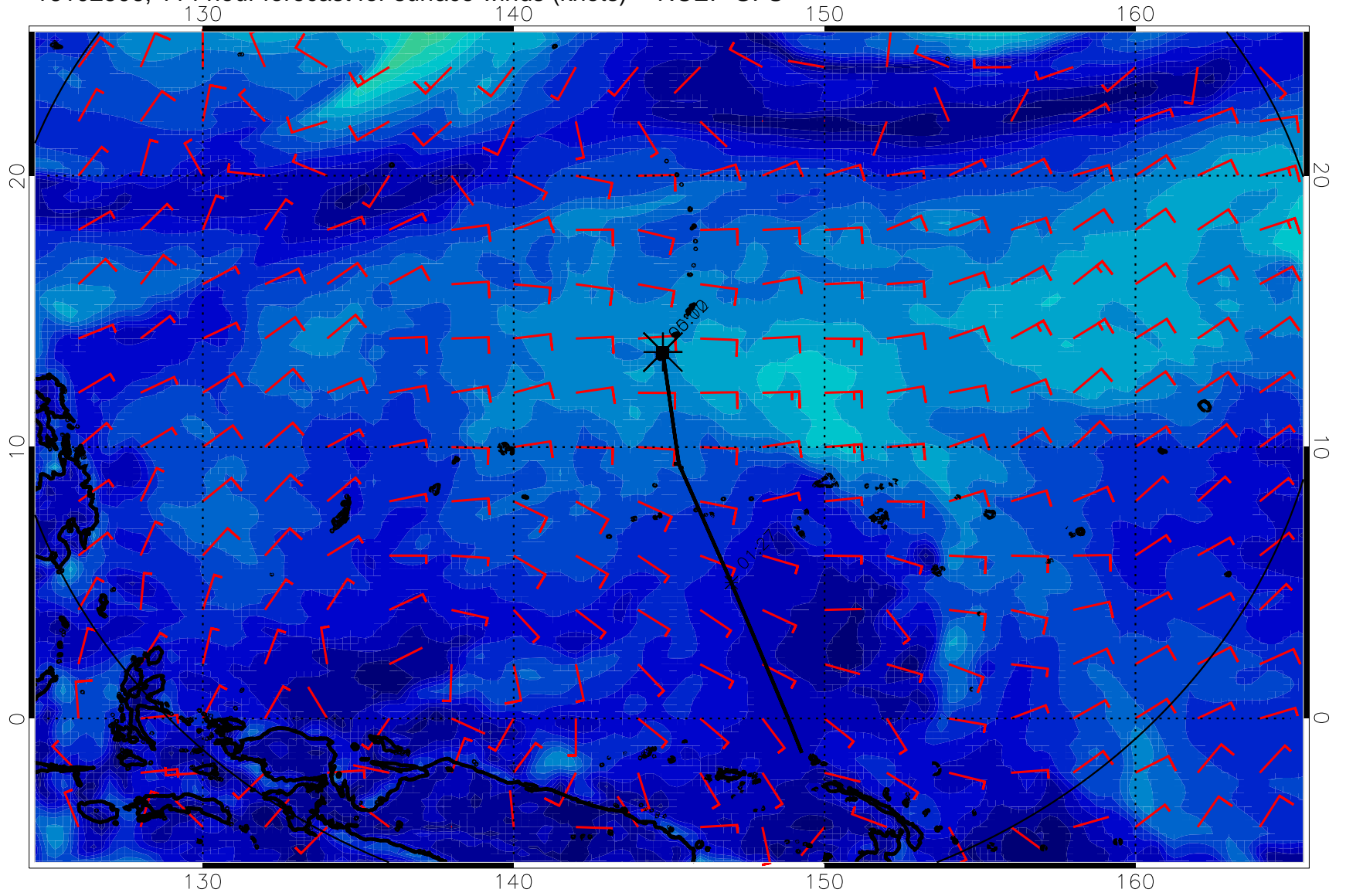
16102506, 114 hour forecast for surface winds (knots) -- NCEP GFS
