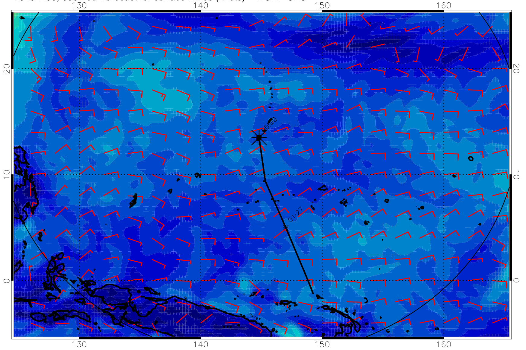
16102200, 036 hour forecast for surface winds (knots) -- NCEP GFS
