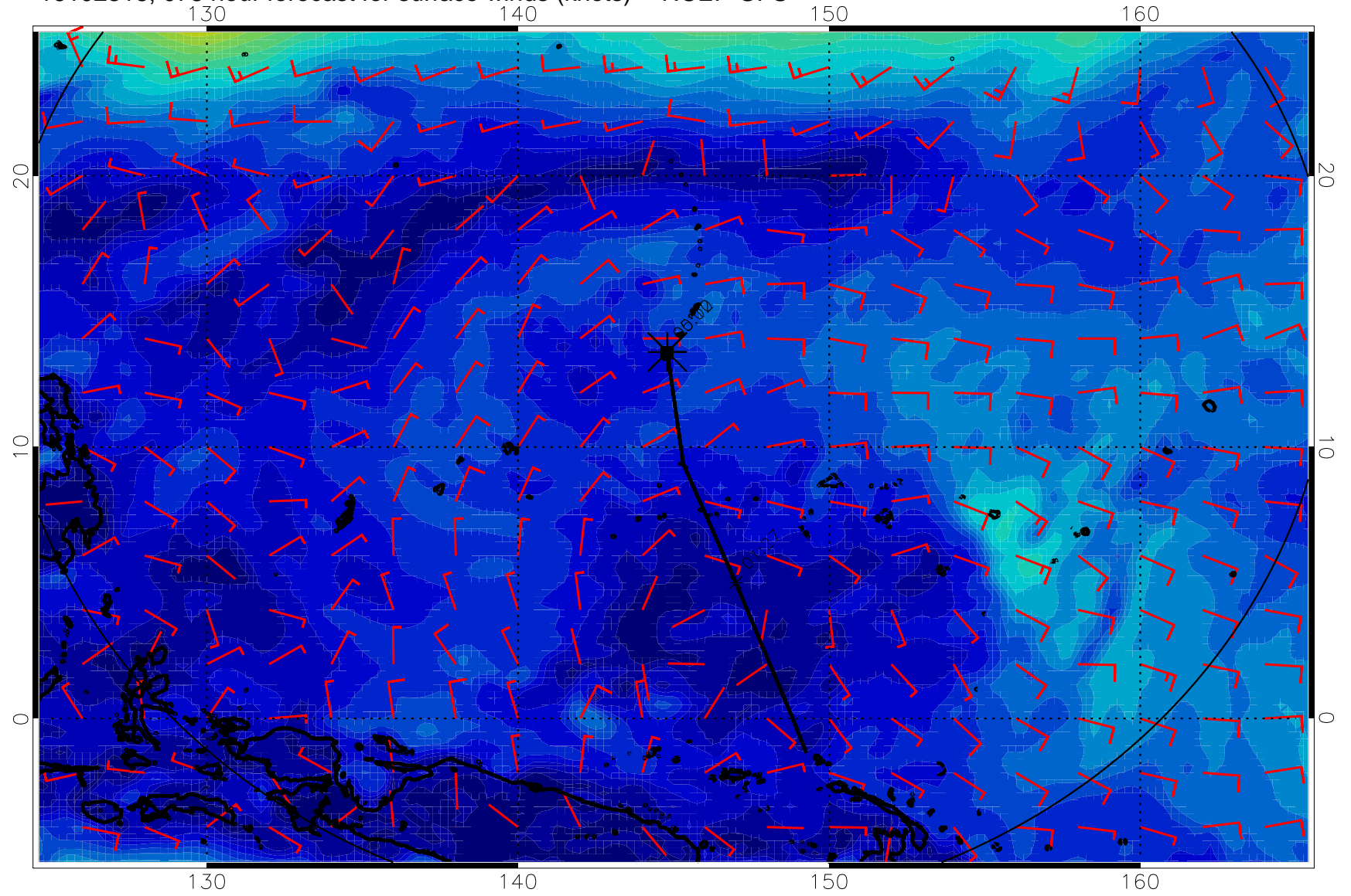
16102318, 078 hour forecast for surface winds (knots) -- NCEP GFS
