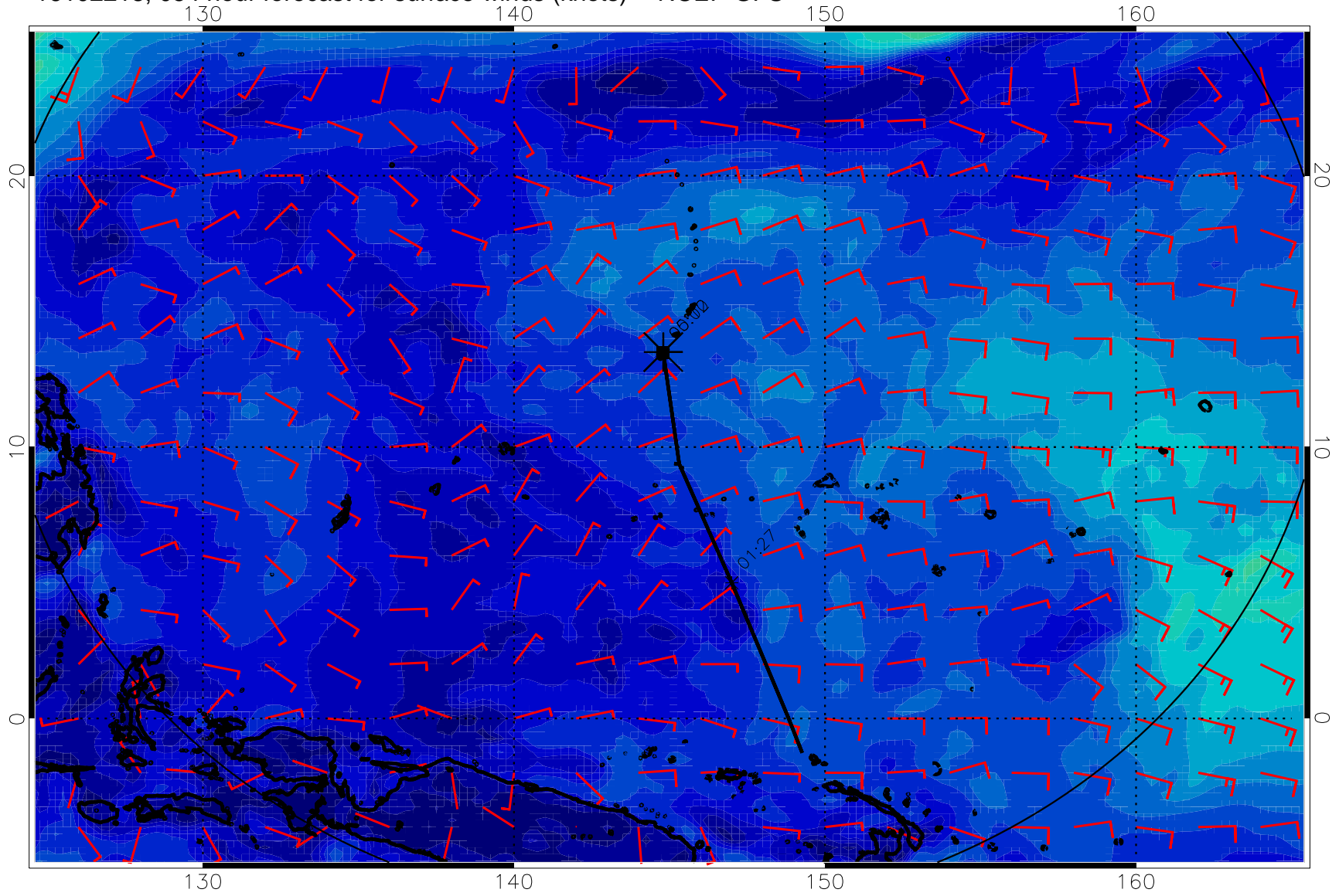
16102218, 054 hour forecast for surface winds (knots) -- NCEP GFS
