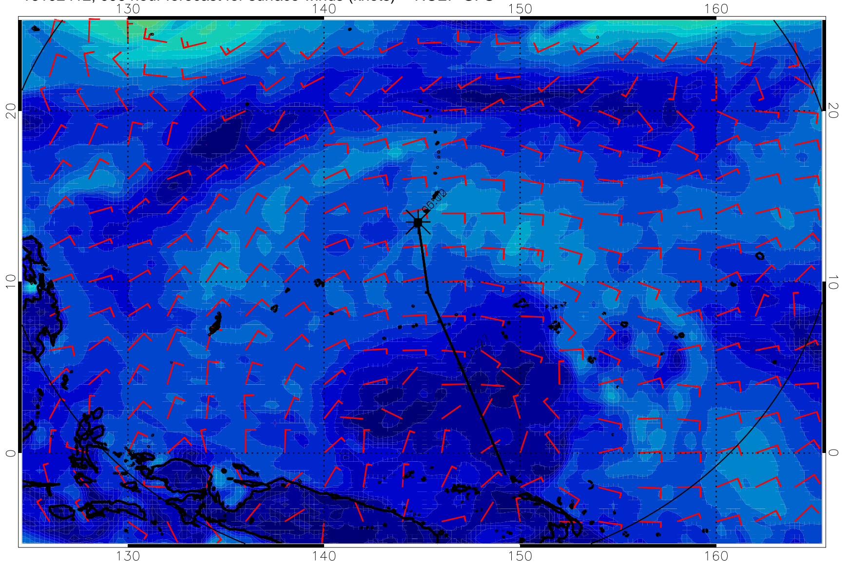
16102412, 096 hour forecast for surface winds (knots) -- NCEP GFS
