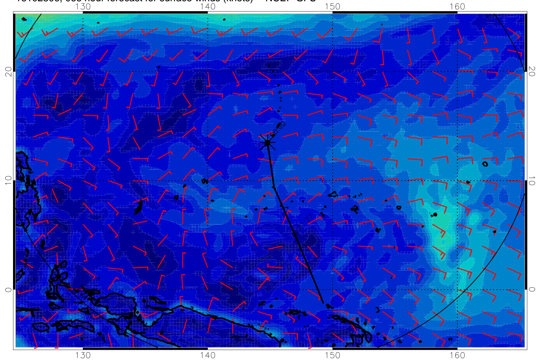
16102306, 066 hour forecast for surface winds (knots) -- NCEP GFS
