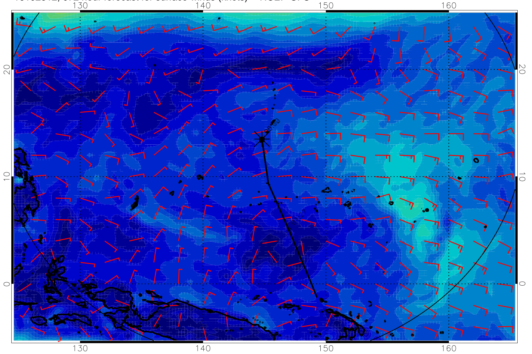
16102312, 072 hour forecast for surface winds (knots) -- NCEP GFS
