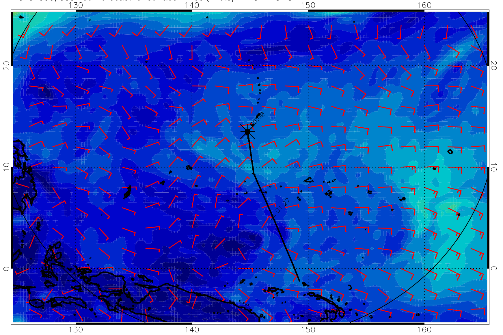
16102300, 060 hour forecast for surface winds (knots) -- NCEP GFS
