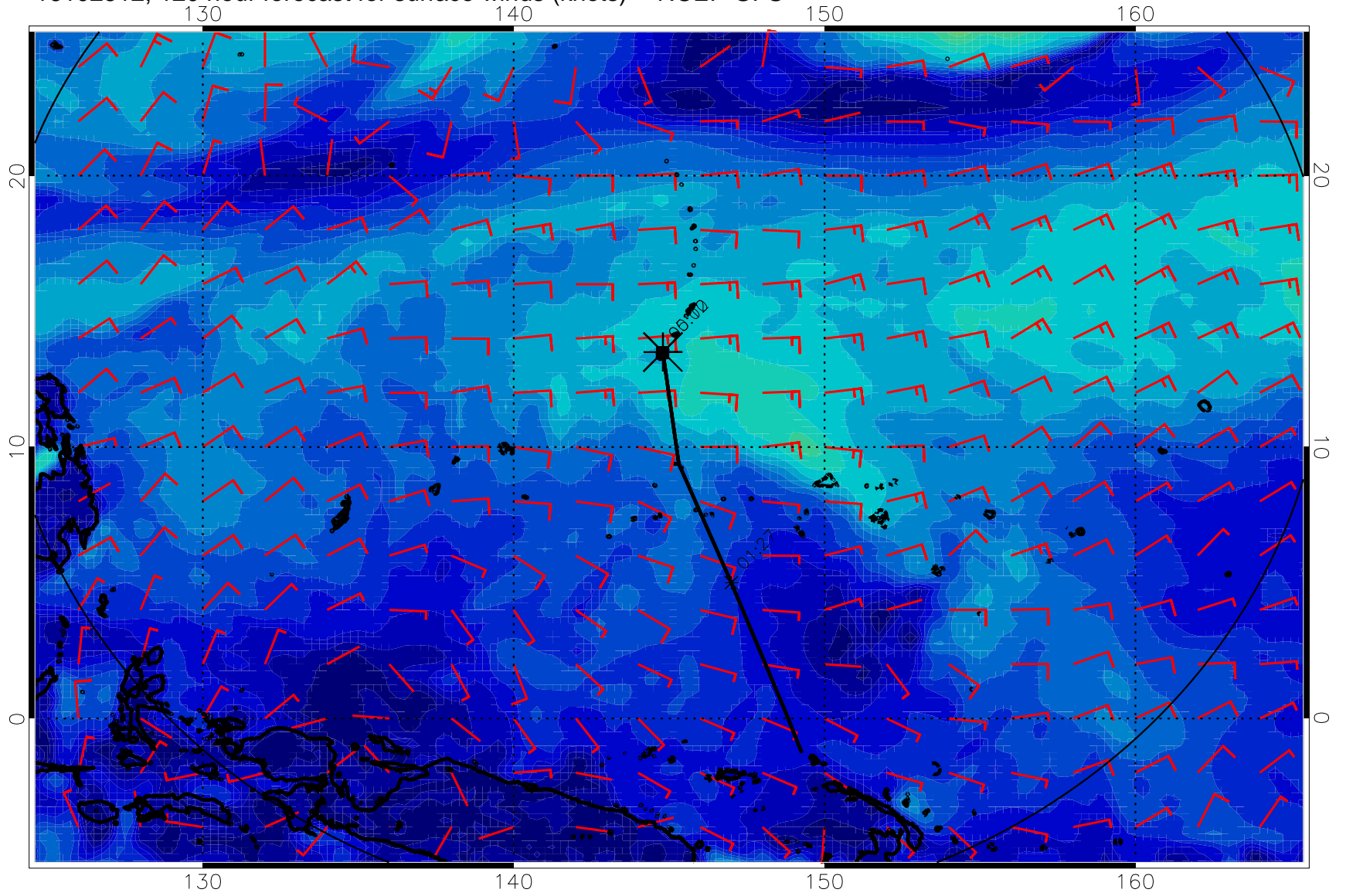
16102512, 120 hour forecast for surface winds (knots) -- NCEP GFS
