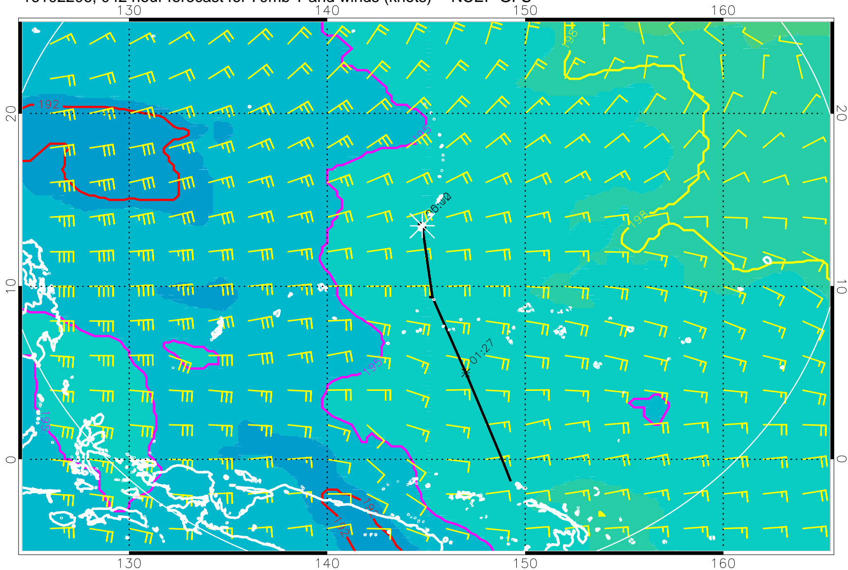
16102206, 04Z hour forecast for 70mb T and winds (knots) -- NCEP GFS
