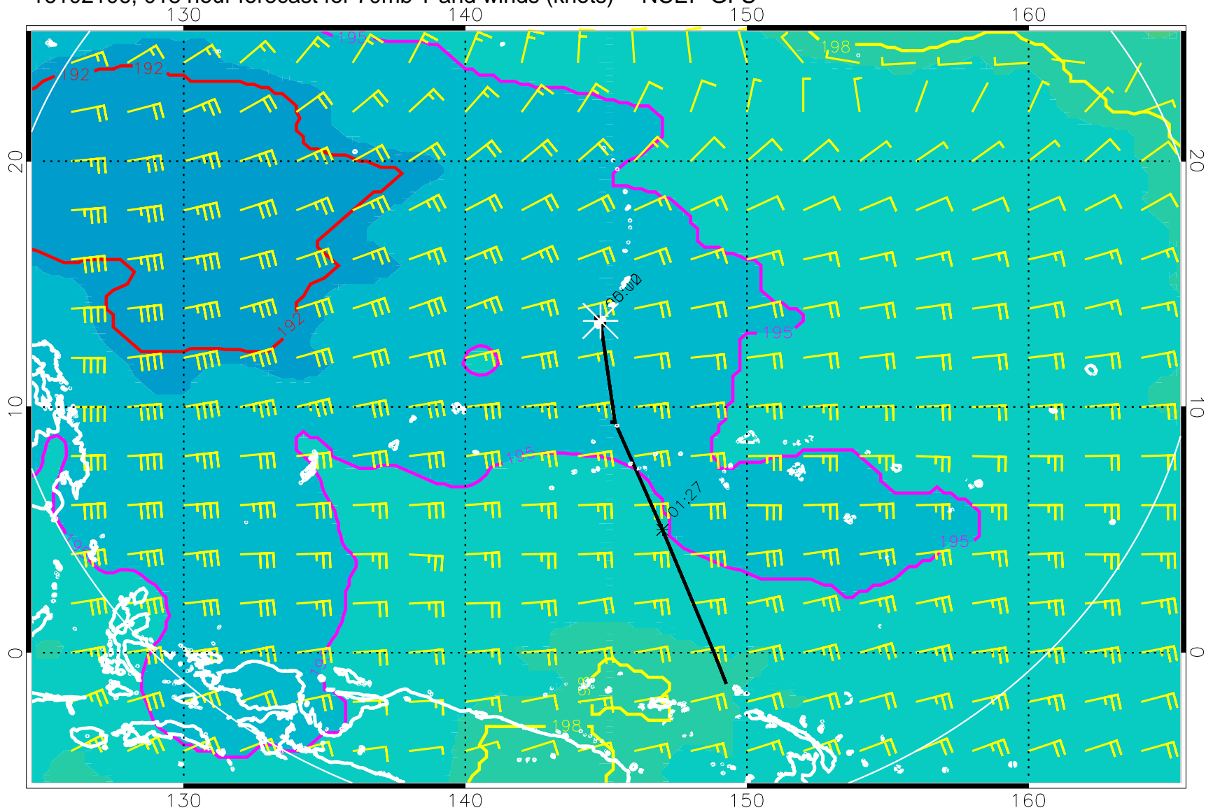
16102106, 018 hour forecast for 70mb T and winds (knots) -- NCEP GFS
