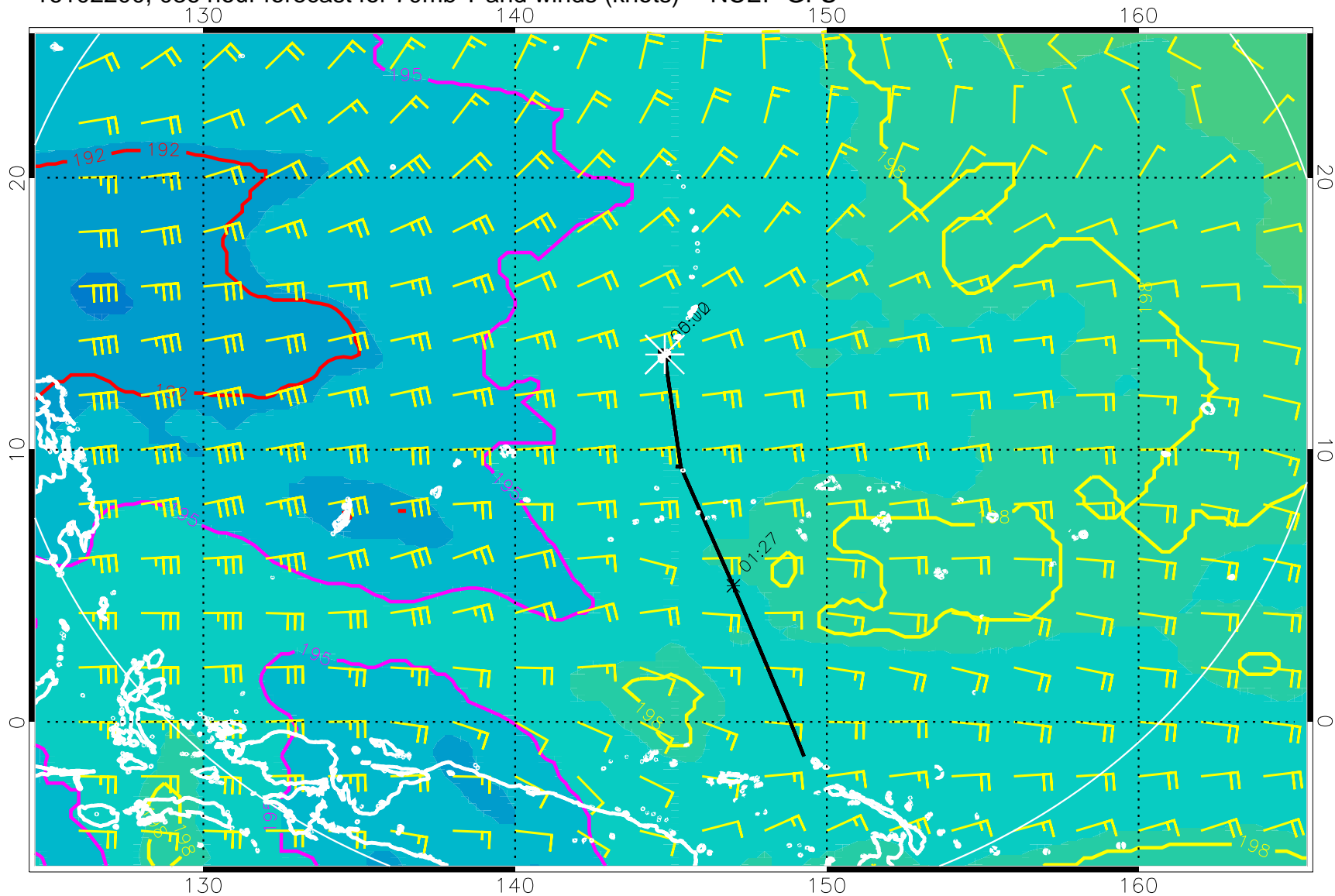
16102200, 036 hour forecast for 70mb T and winds (knots) -- NCEP GFS
