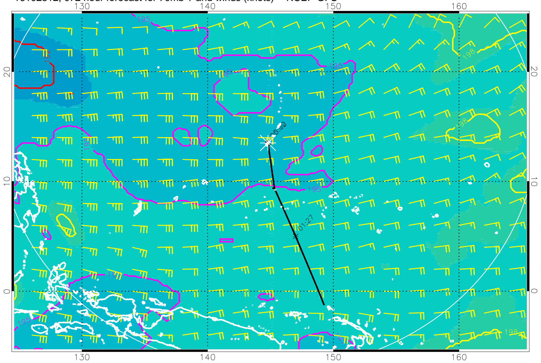
16102312, 072 hour forecast for 70mb T and winds (knots) -- NCEP GFS
