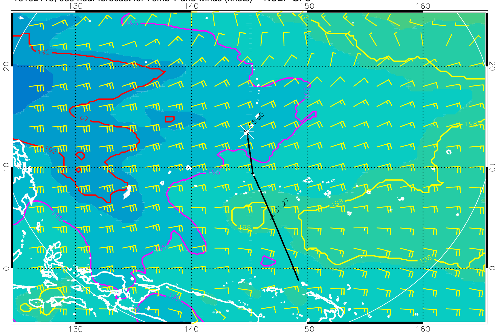
16102118, 030 hour forecast for 70mb T and winds (knots) -- NCEP GFS
