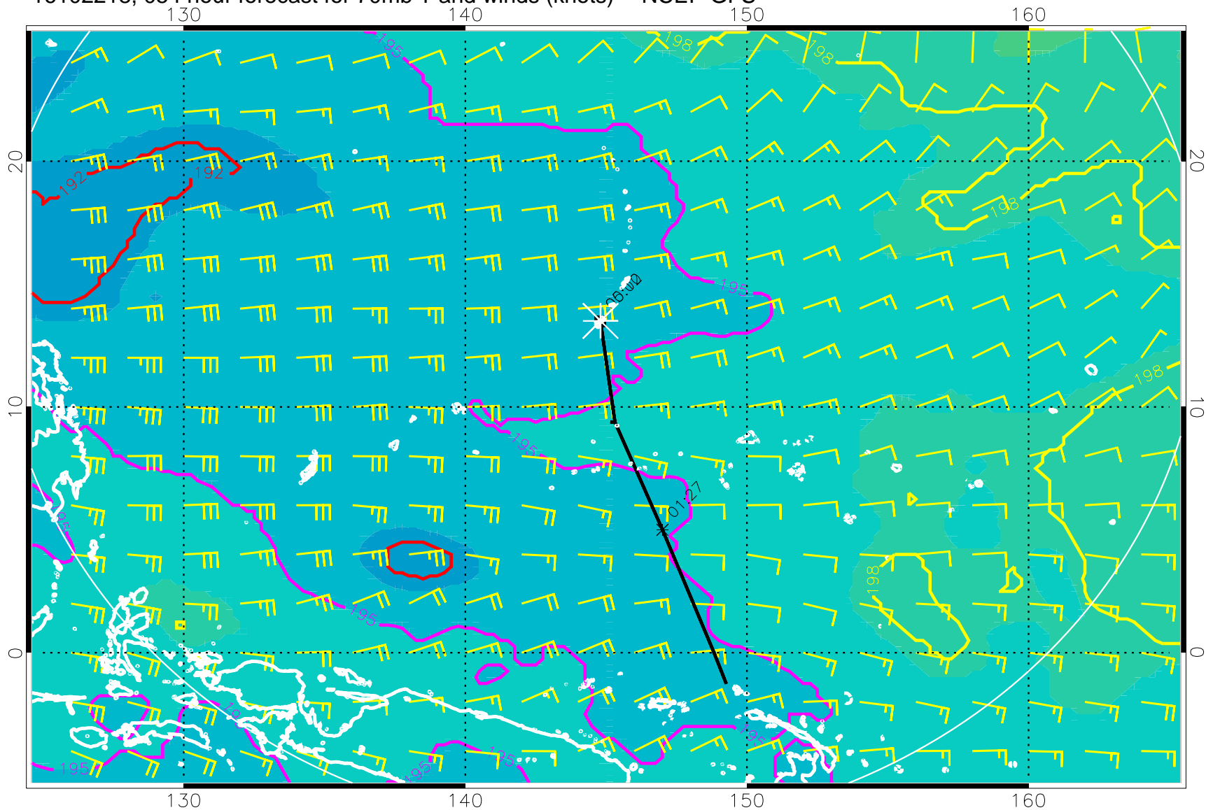
16102218, 054 hour forecast for 70mb T and winds (knots) -- NCEP GFS
