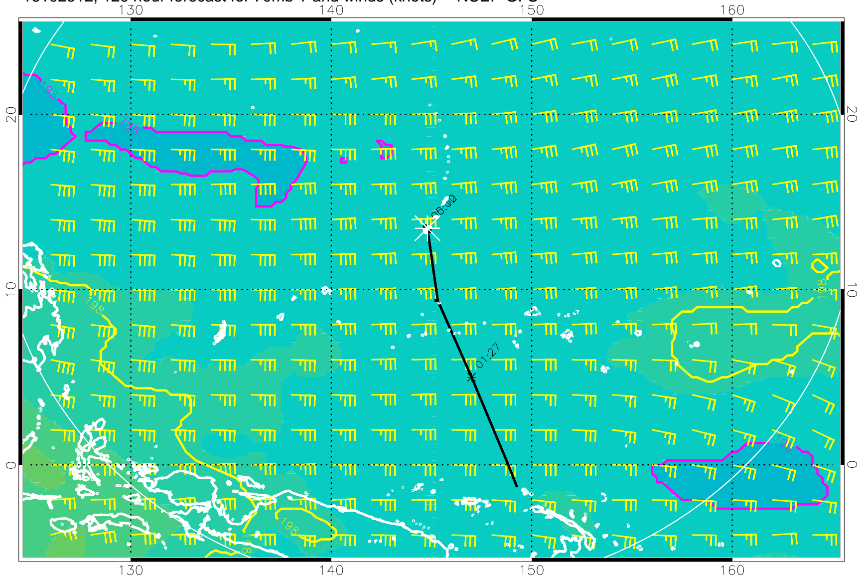
16102512, 120 hour forecast for 70mb T and winds (knots) -- NCEP GFS
