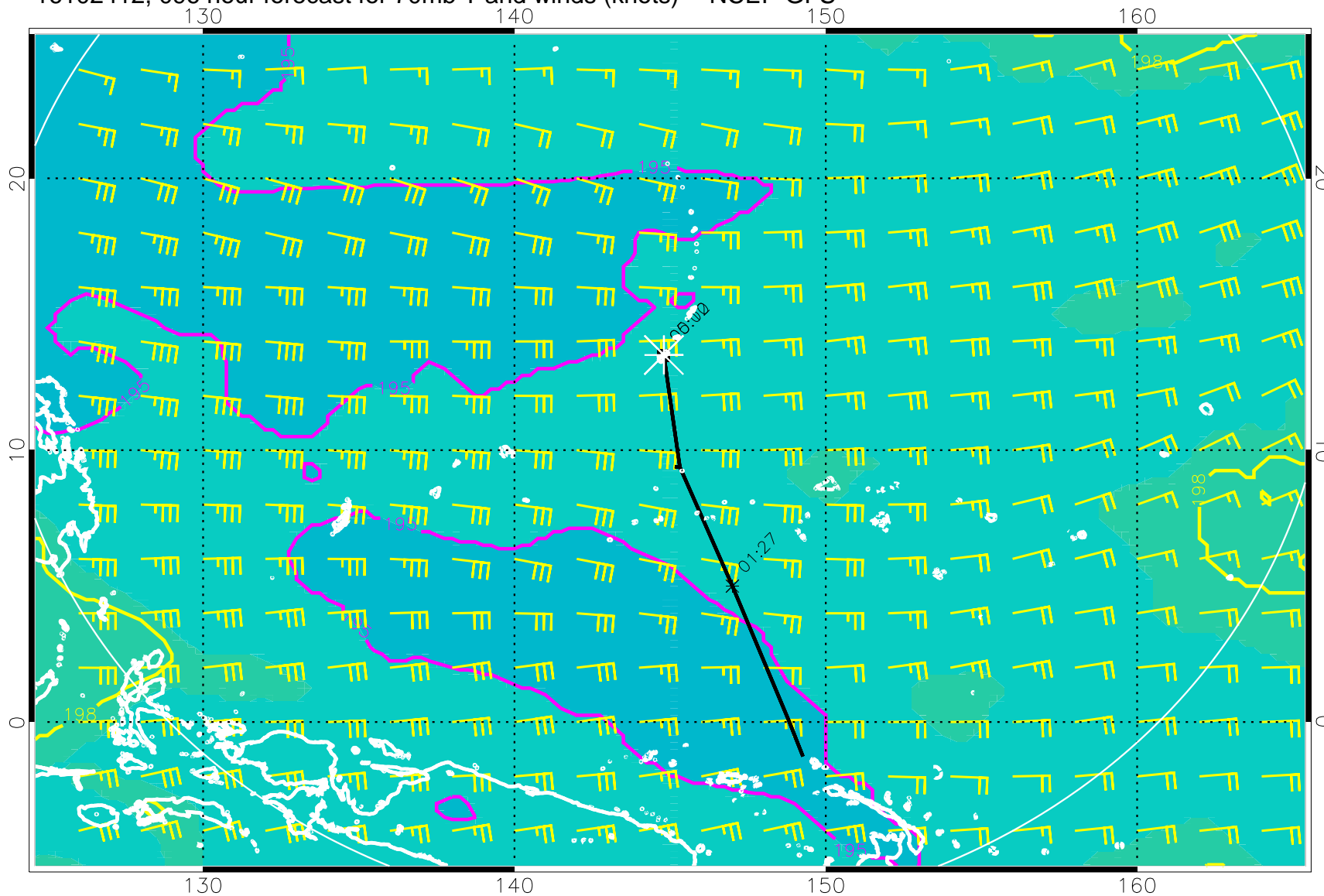
16102412, 096 hour forecast for 70mb T and winds (knots) -- NCEP GFS
