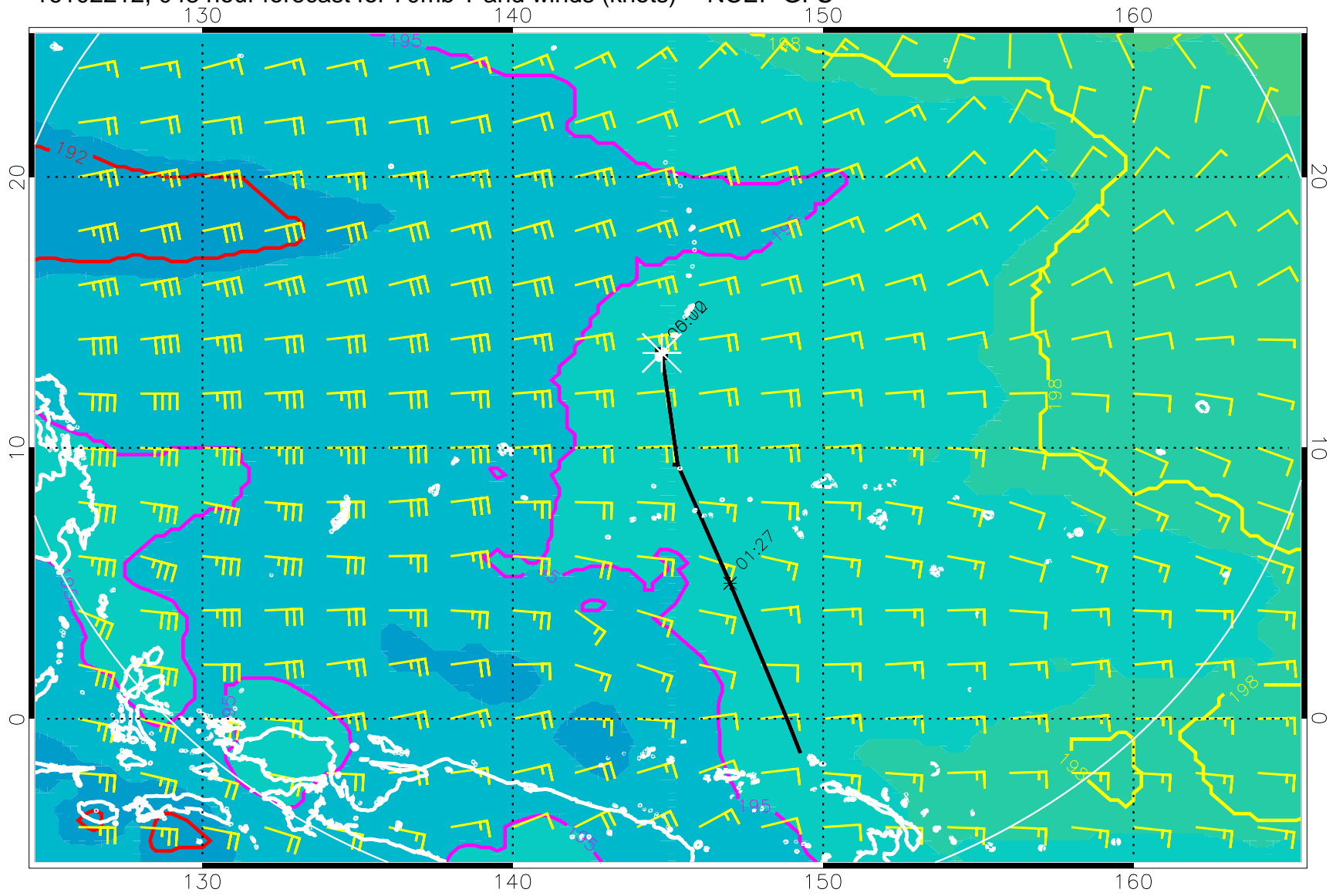
16102212, 048 hour forecast for 70mb T and winds (knots) -- NCEP GFS
