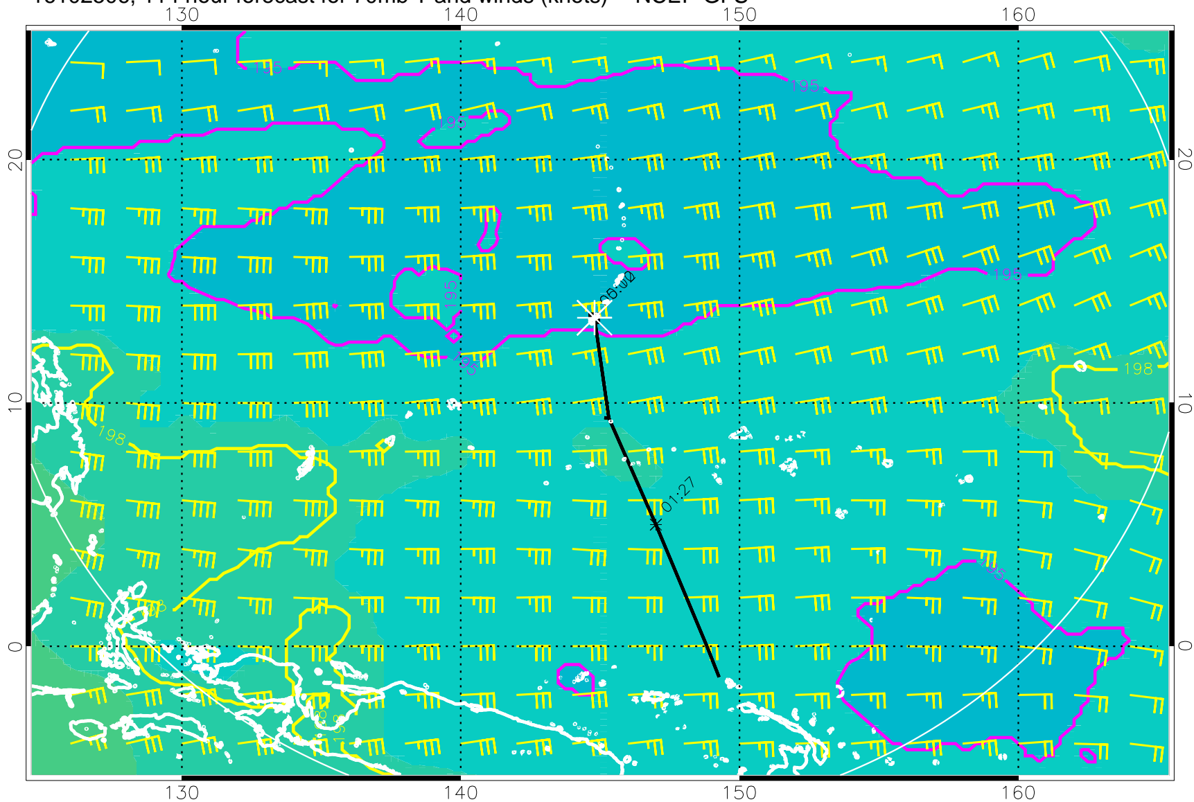
16102506, 114 hour forecast for 70mb T and winds (knots) -- NCEP GFS
