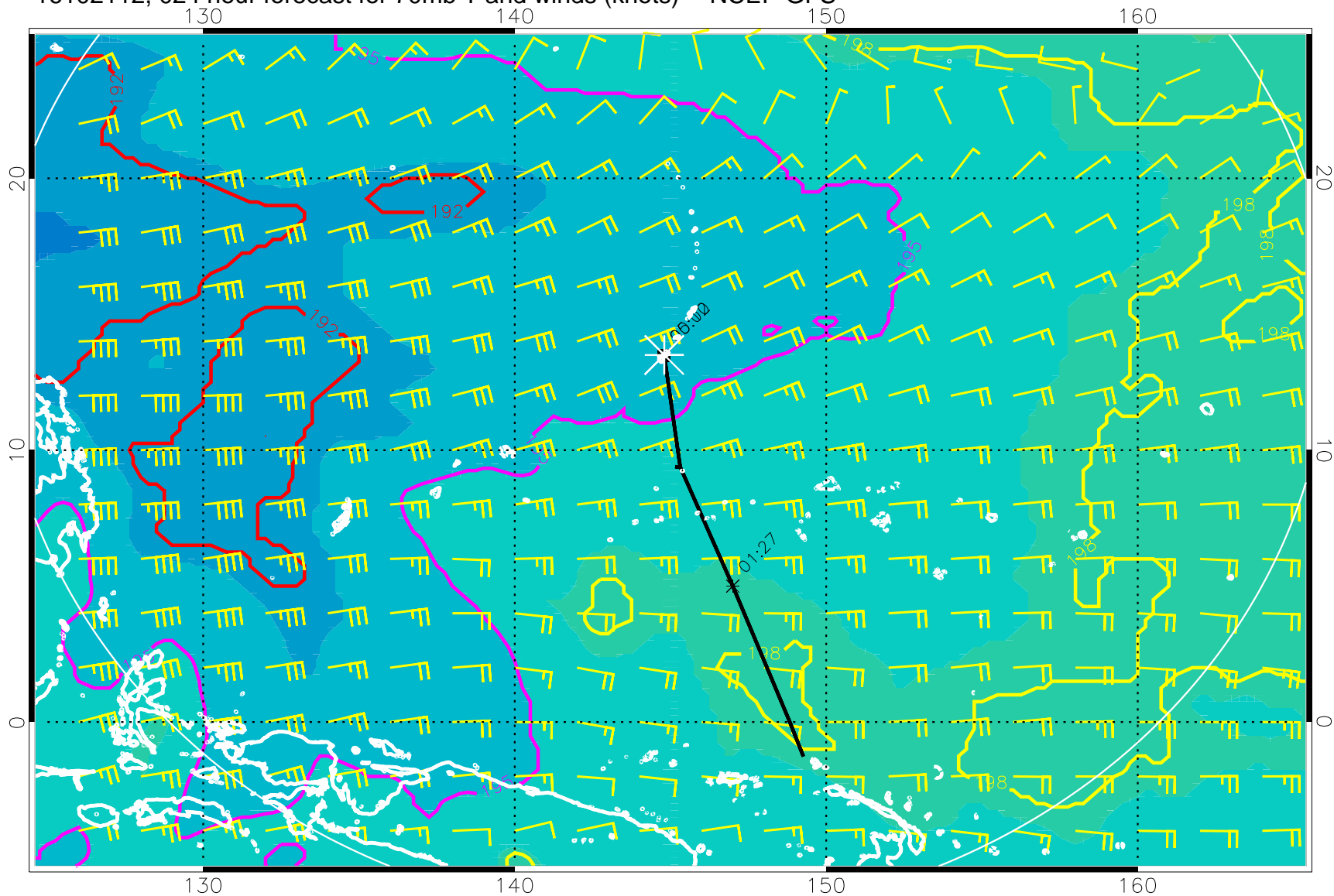
16102112, 024 hour forecast for 70mb T and winds (knots) -- NCEP GFS
