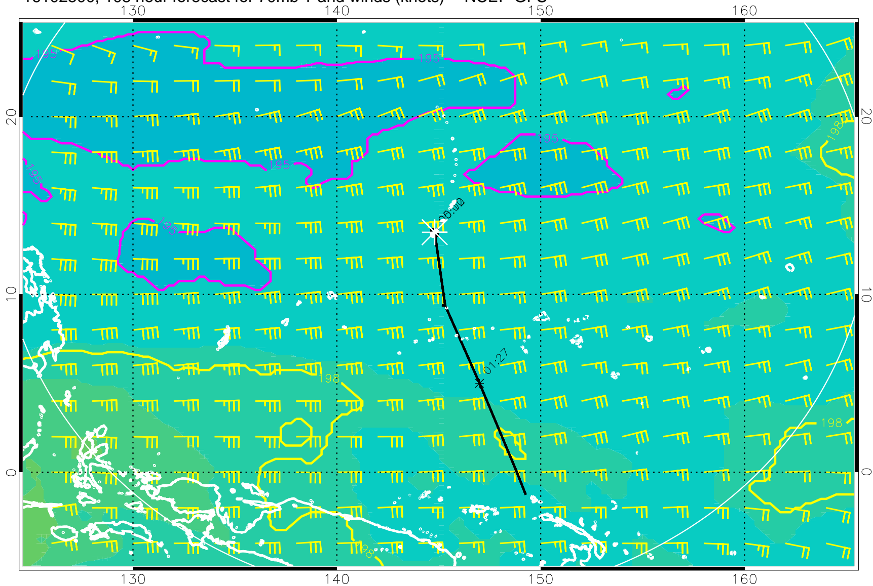
16102500, 108 hour forecast for 70mb T and winds (knots) -- NCEP GFS
