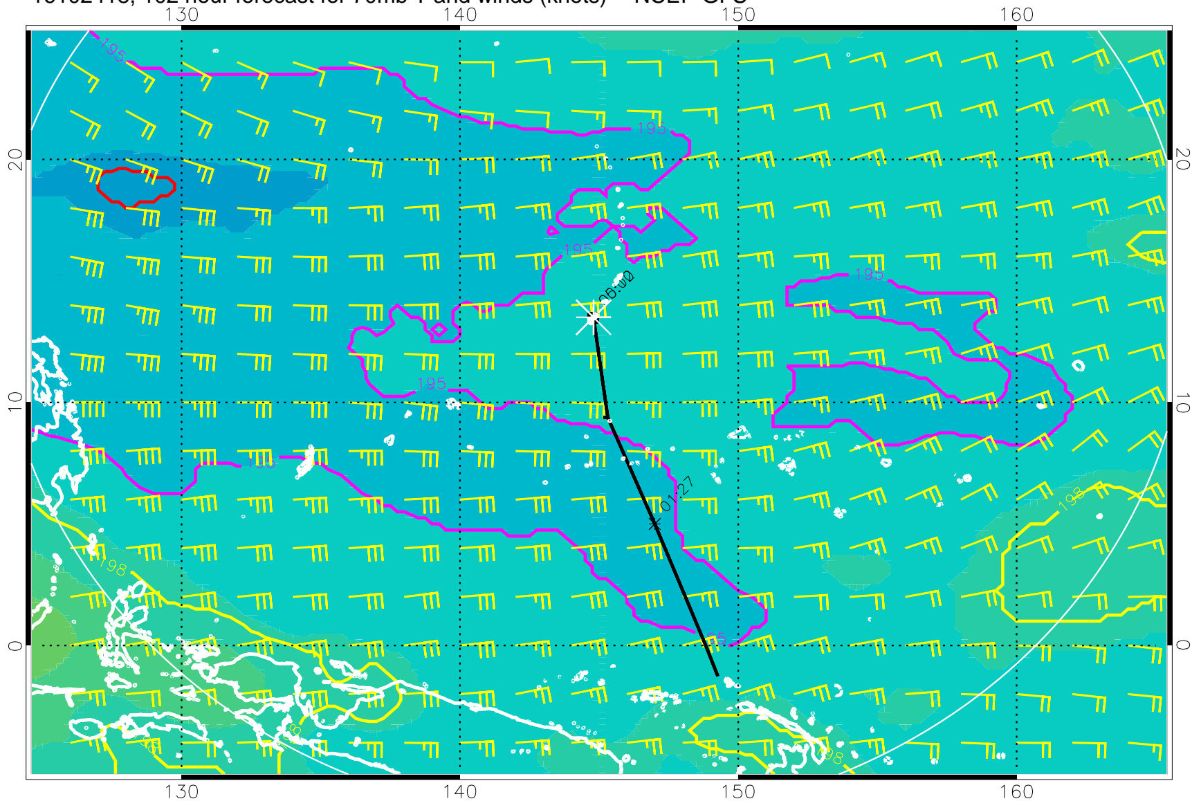
16102418, 102 hour forecast for 70mb T and winds (knots) -- NCEP GFS
