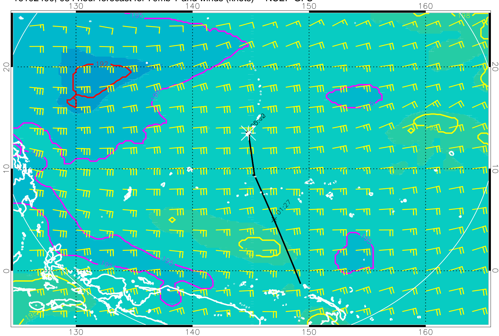
16102400, 084 hour forecast for 70mb T and winds (knots) -- NCEP GFS
