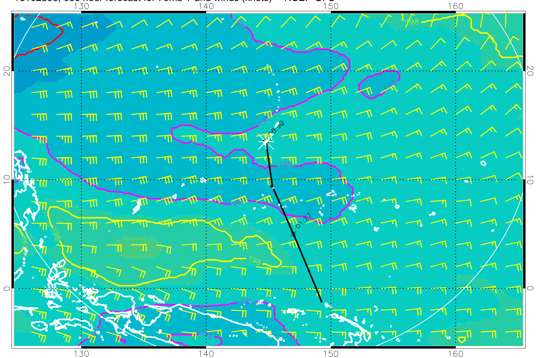
16102306, 066 hour forecast for 70mb T and winds (knots) -- NCEP GFS
