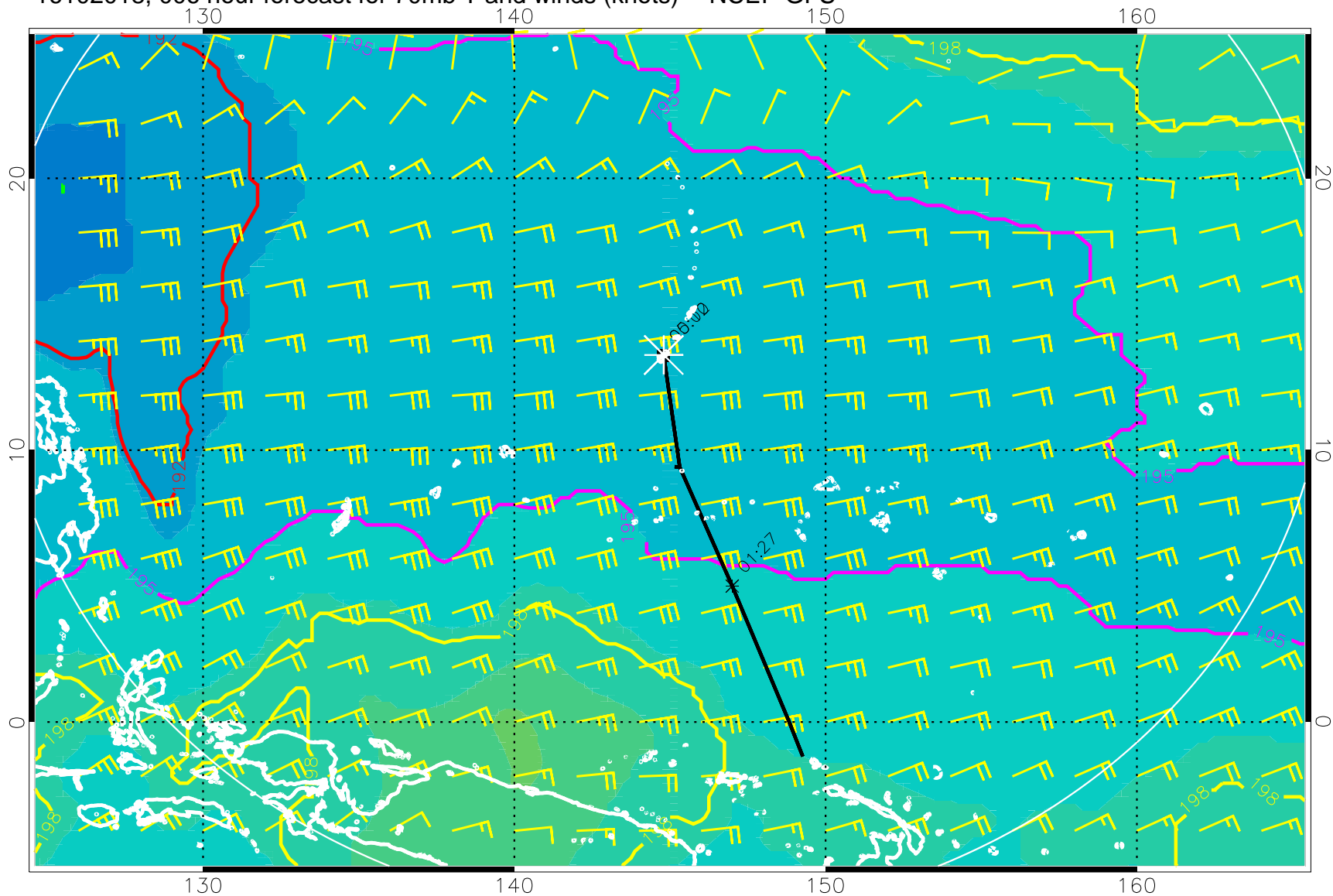
16102018, 006 hour forecast for 70mb T and winds (knots) -- NCEP GFS
