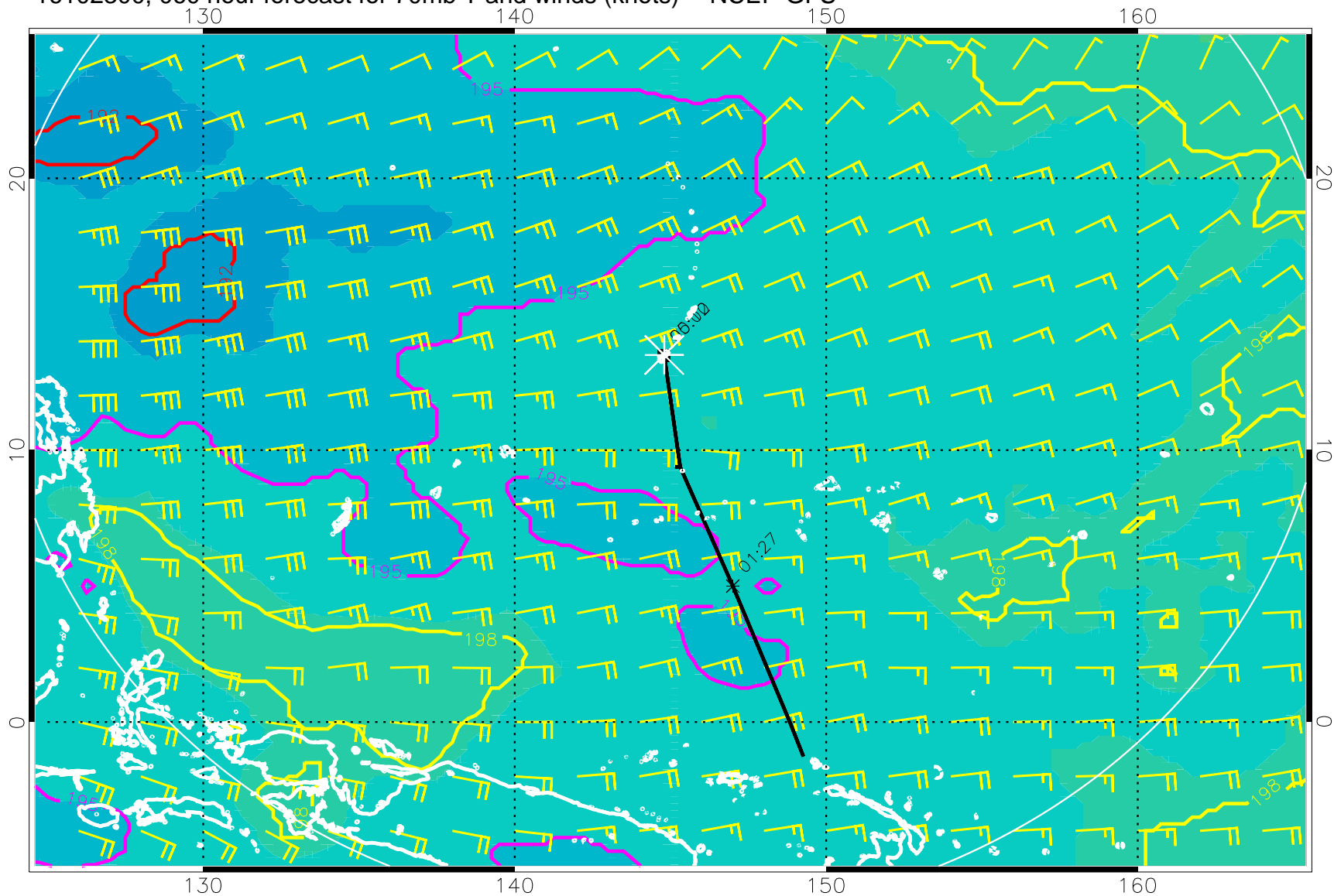
16102300, 060 hour forecast for 70mb T and winds (knots) -- NCEP GFS
