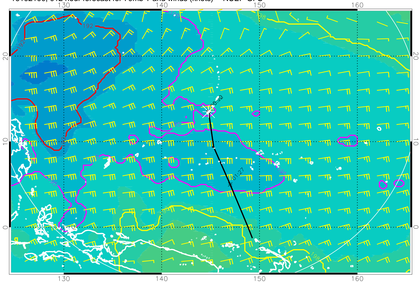
16102100, 012 hour forecast for 70mb T and winds (knots) -- NCEP GFS
