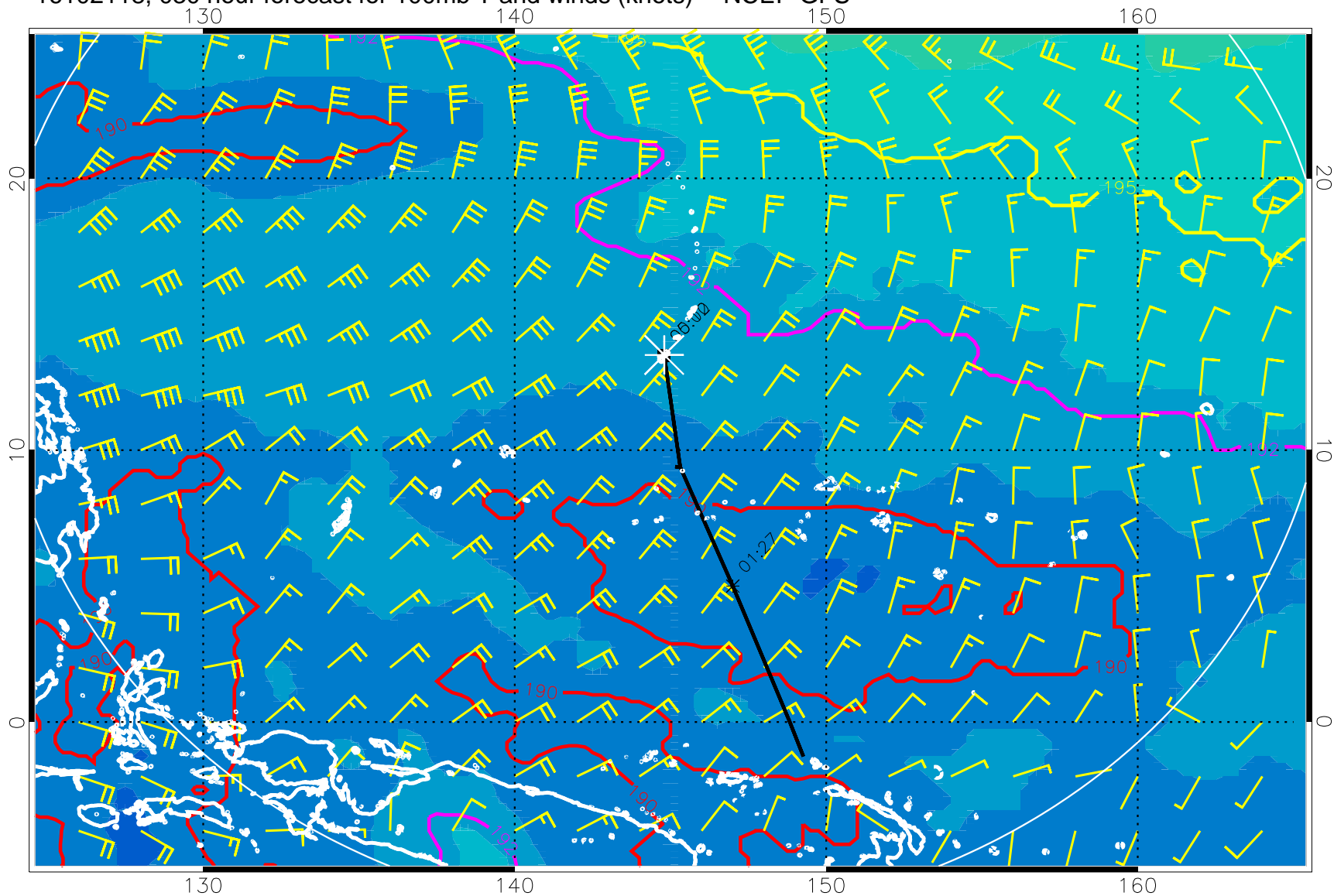
16102118, 030 hour forecast for 100mb T and winds (knots) -- NCEP GFS
