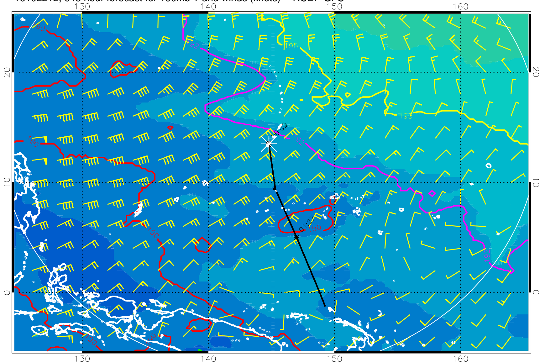
16102212, 048 hour forecast for 100mb T and winds (knots) -- NCEP GFS
