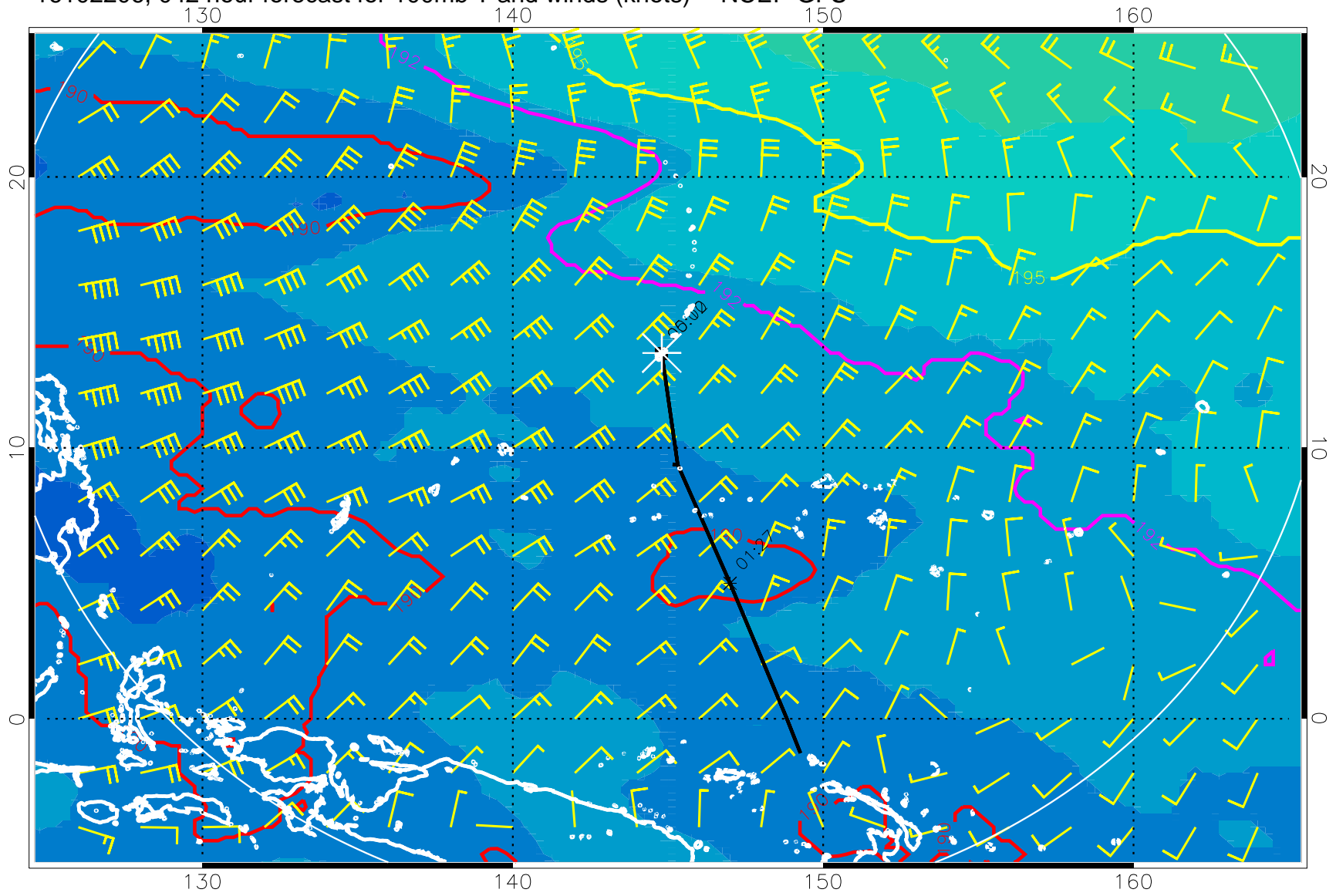
16102206, 042 hour forecast for 100mb T and winds (knots) -- NCEP GFS
