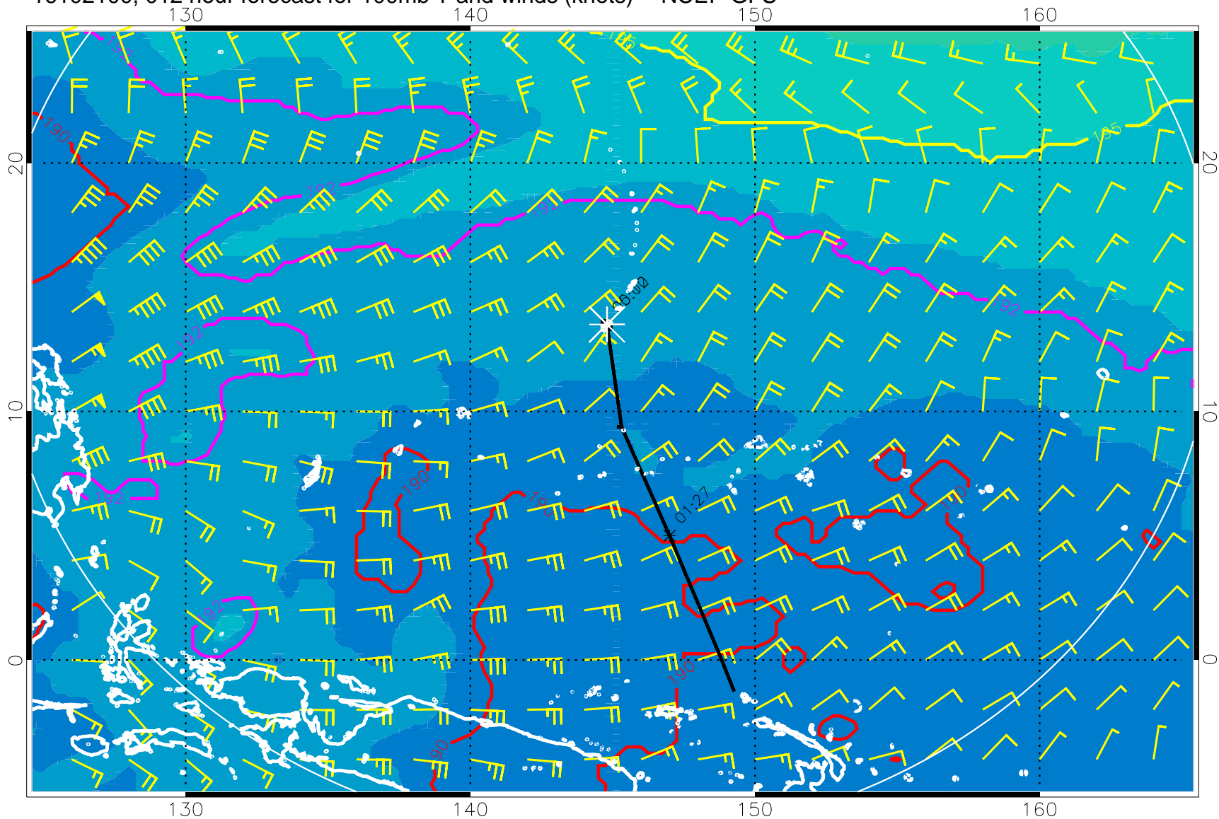
16102100, 012 hour forecast for 100mb T and winds (knots) -- NCEP GFS
