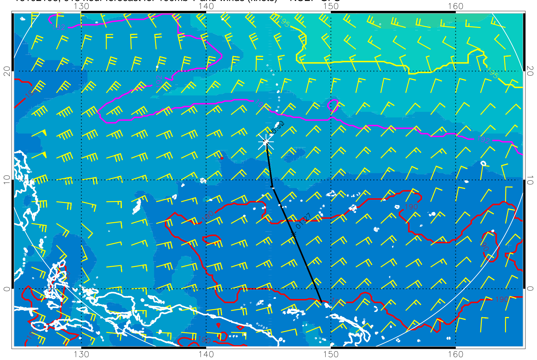
16102106, 018 hour forecast for 100mb T and winds (knots) -- NCEP GFS
