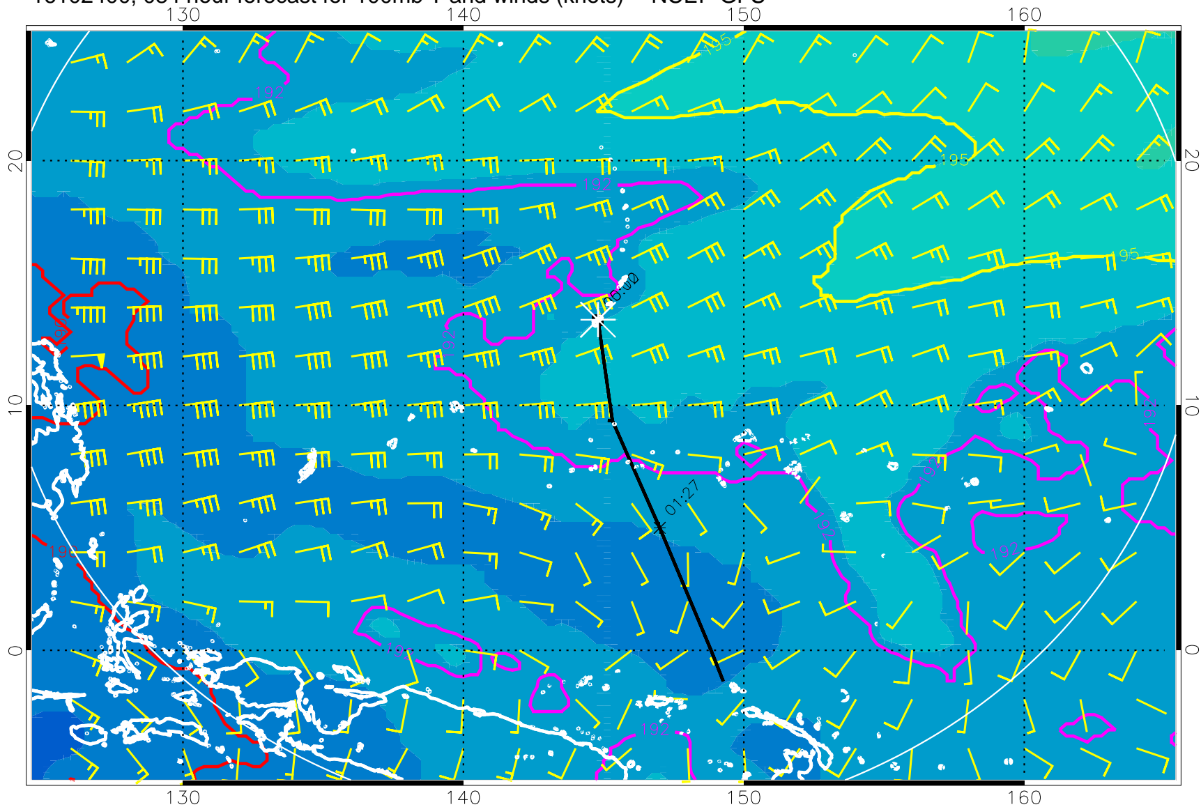
16102400, 084 hour forecast for 100mb T and winds (knots) -- NCEP GFS
