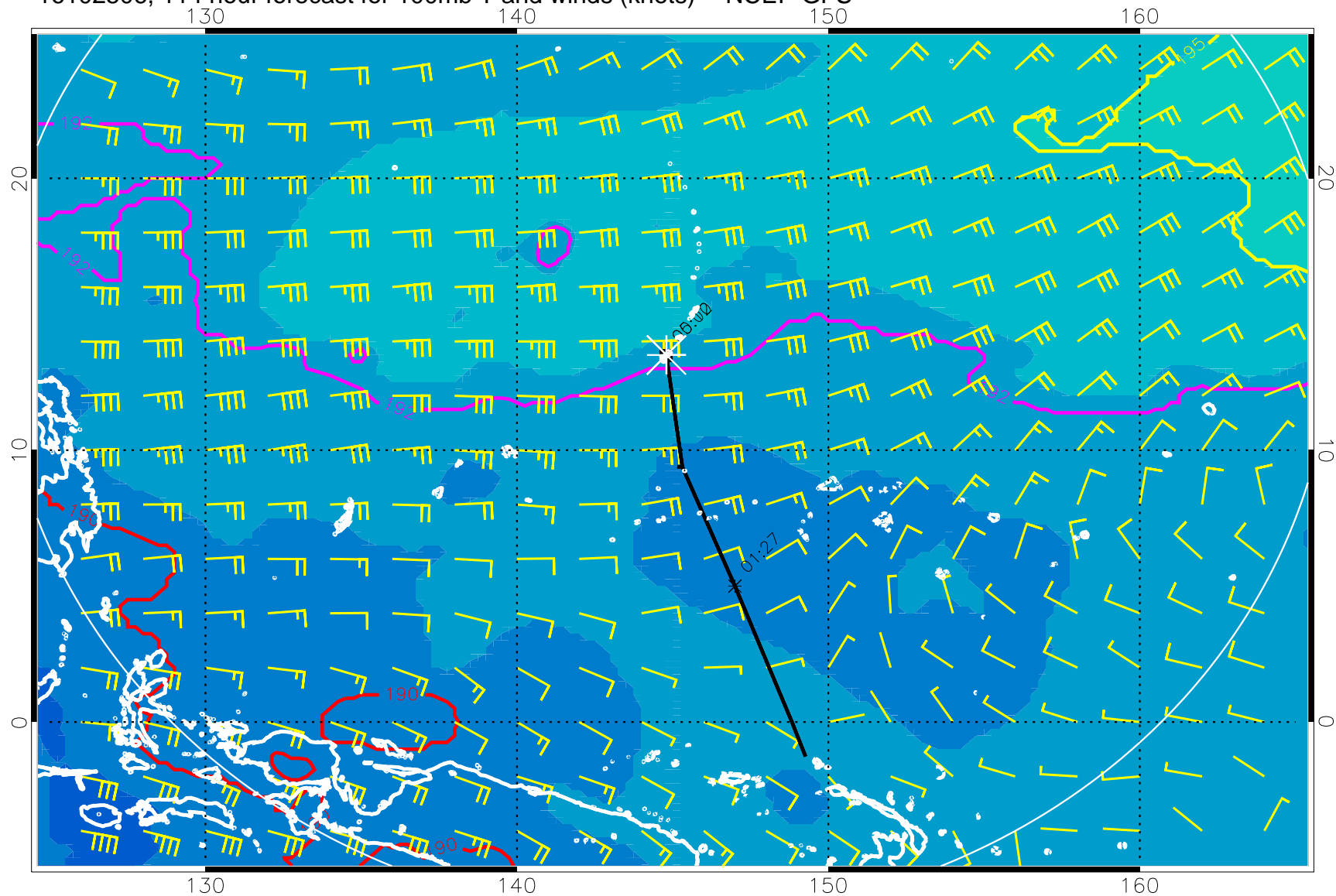
16102506, 114 hour forecast for 100mb T and winds (knots) -- NCEP GFS
