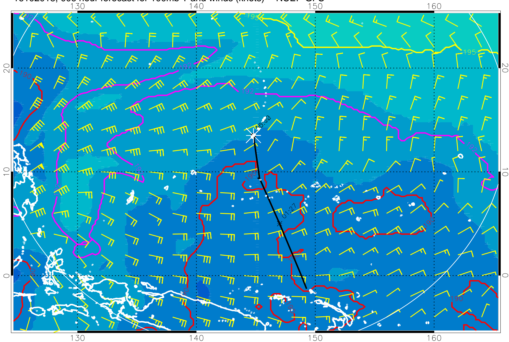
16102018, 006 hour forecast for 100mb T and winds (knots) -- NCEP GFS
