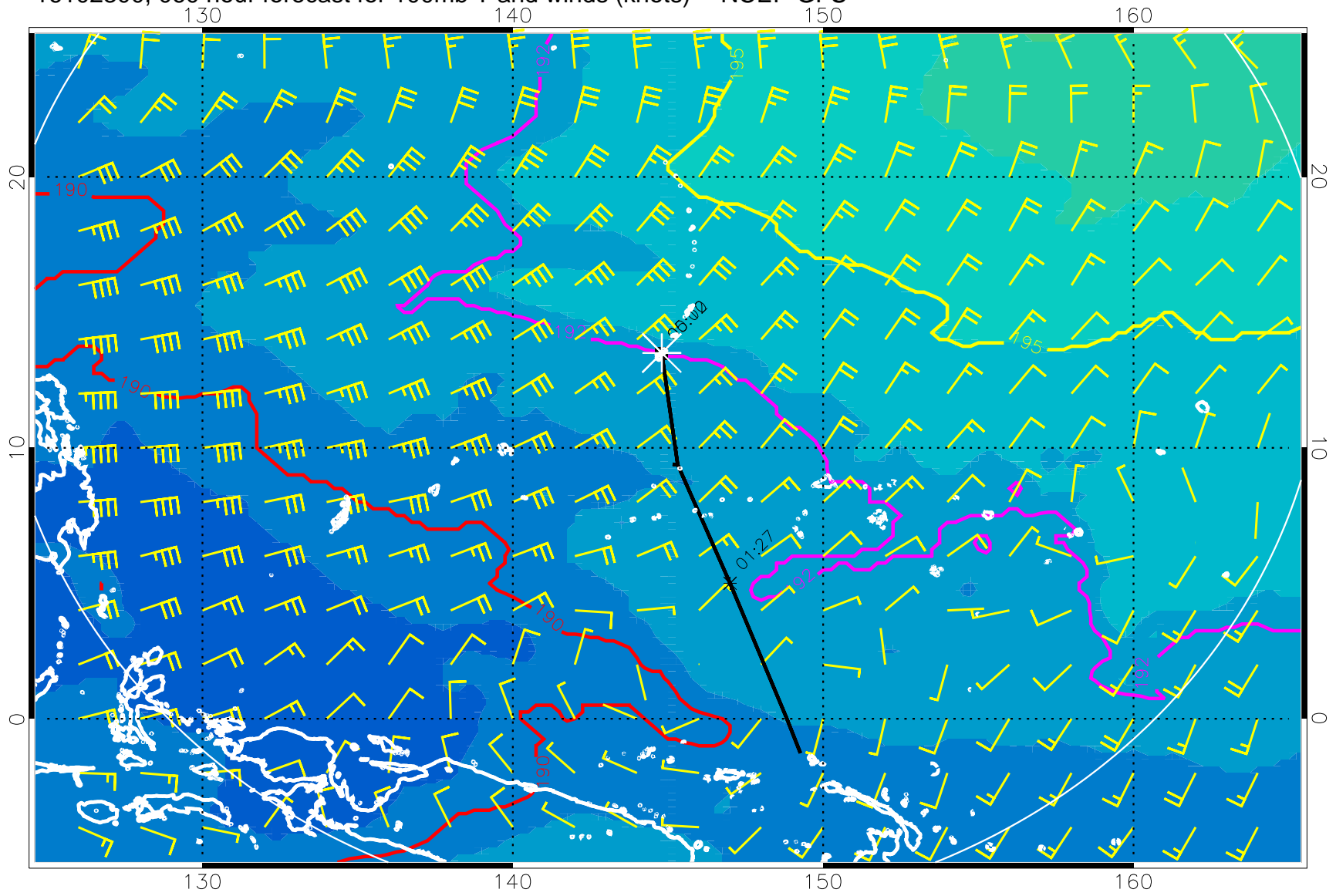
16102300, 060 hour forecast for 100mb T and winds (knots) -- NCEP GFS
