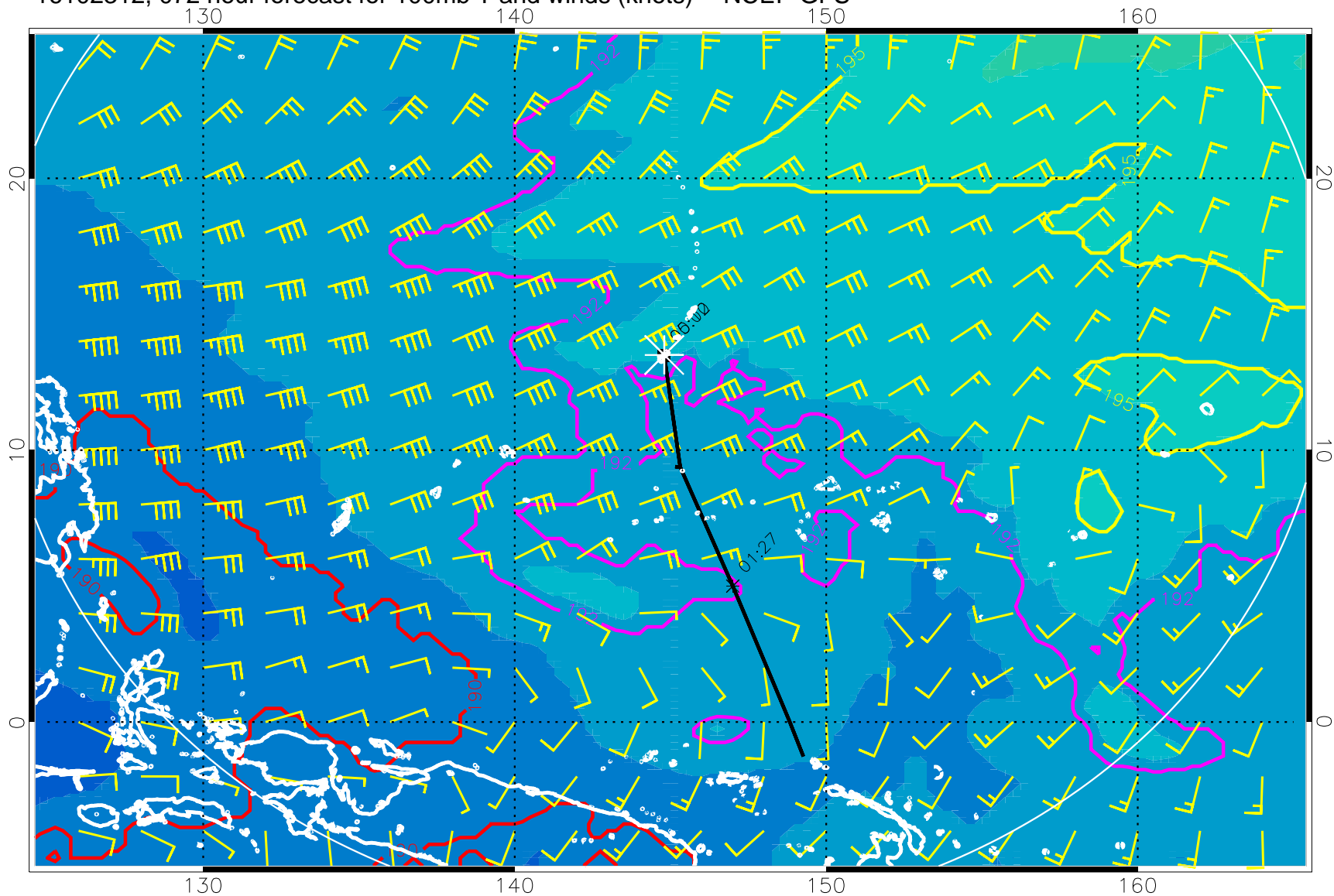
16102312, 072 hour forecast for 100mb T and winds (knots) -- NCEP GFS
