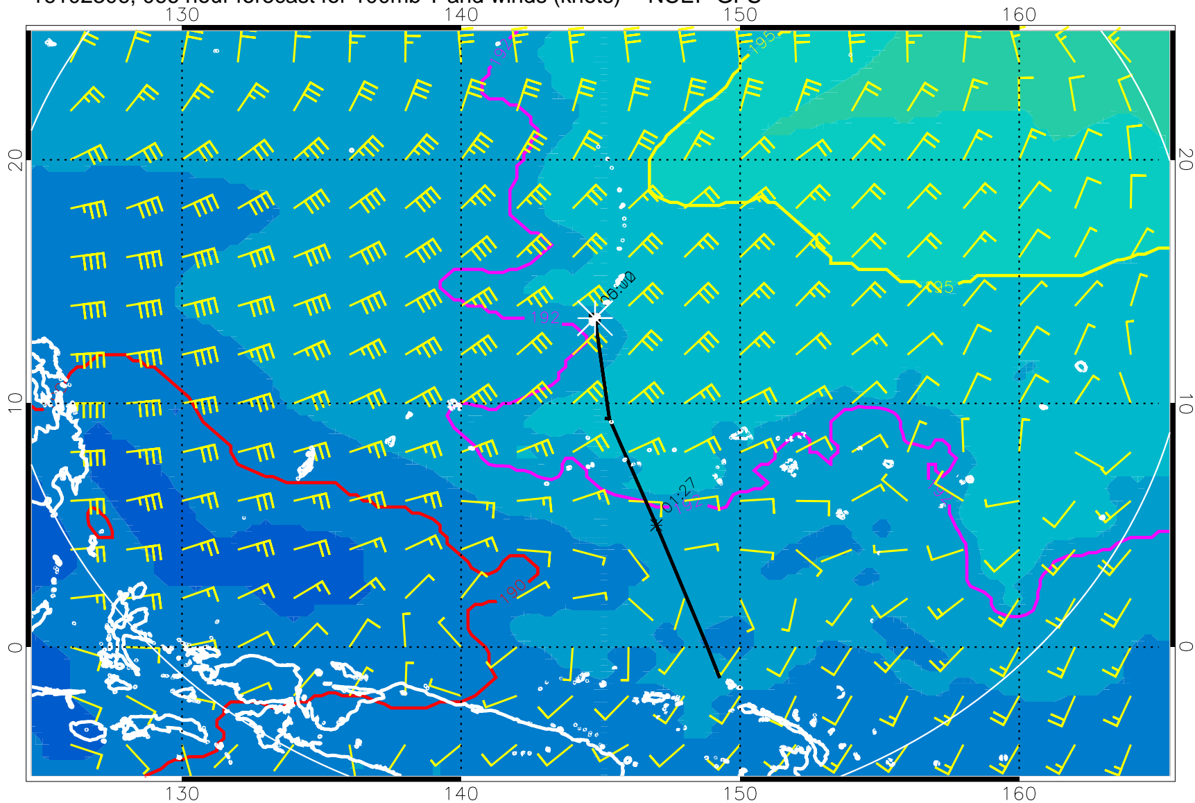
16102306, 066 hour forecast for 100mb T and winds (knots) -- NCEP GFS
