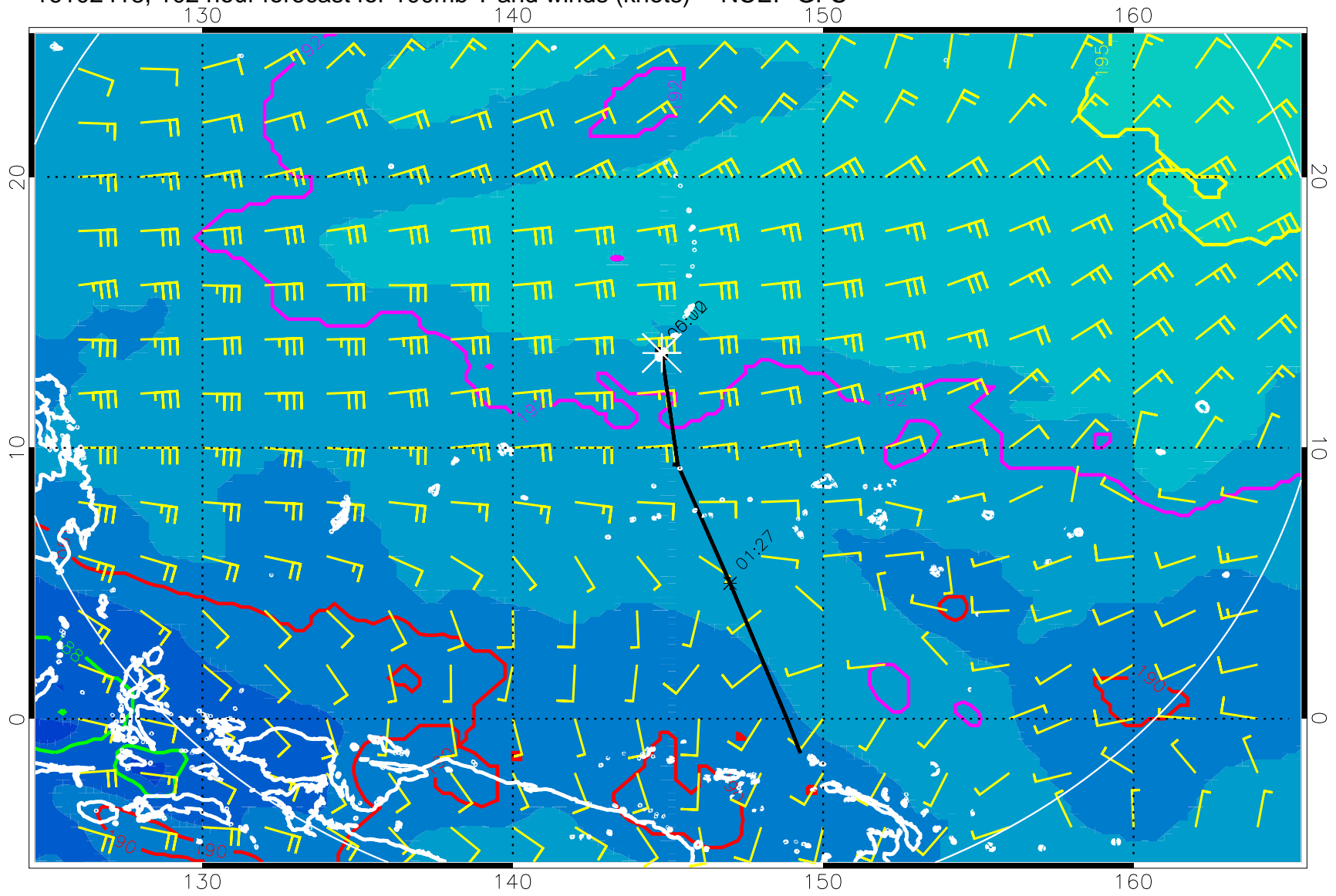
16102418, 102 hour forecast for 100mb T and winds (knots) -- NCEP GFS
