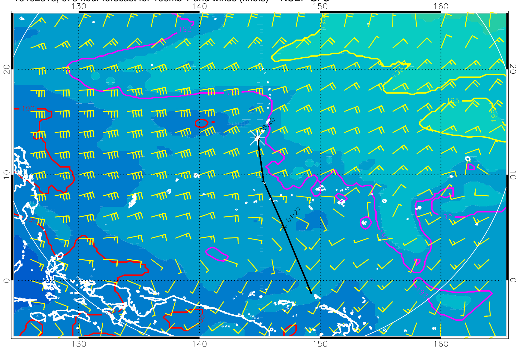
16102318, 078 hour forecast for 100mb T and winds (knots) -- NCEP GFS
