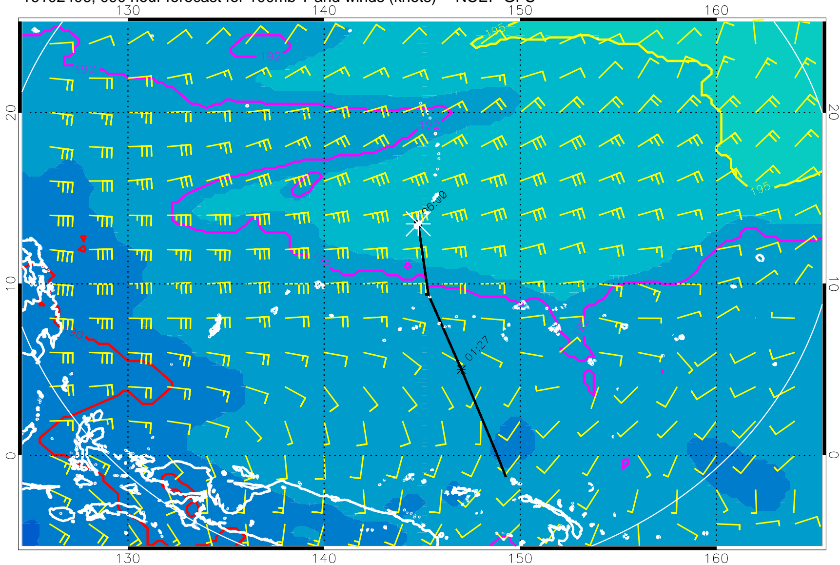
16102406, 090 hour forecast for 100mb T and winds (knots) -- NCEP GFS
