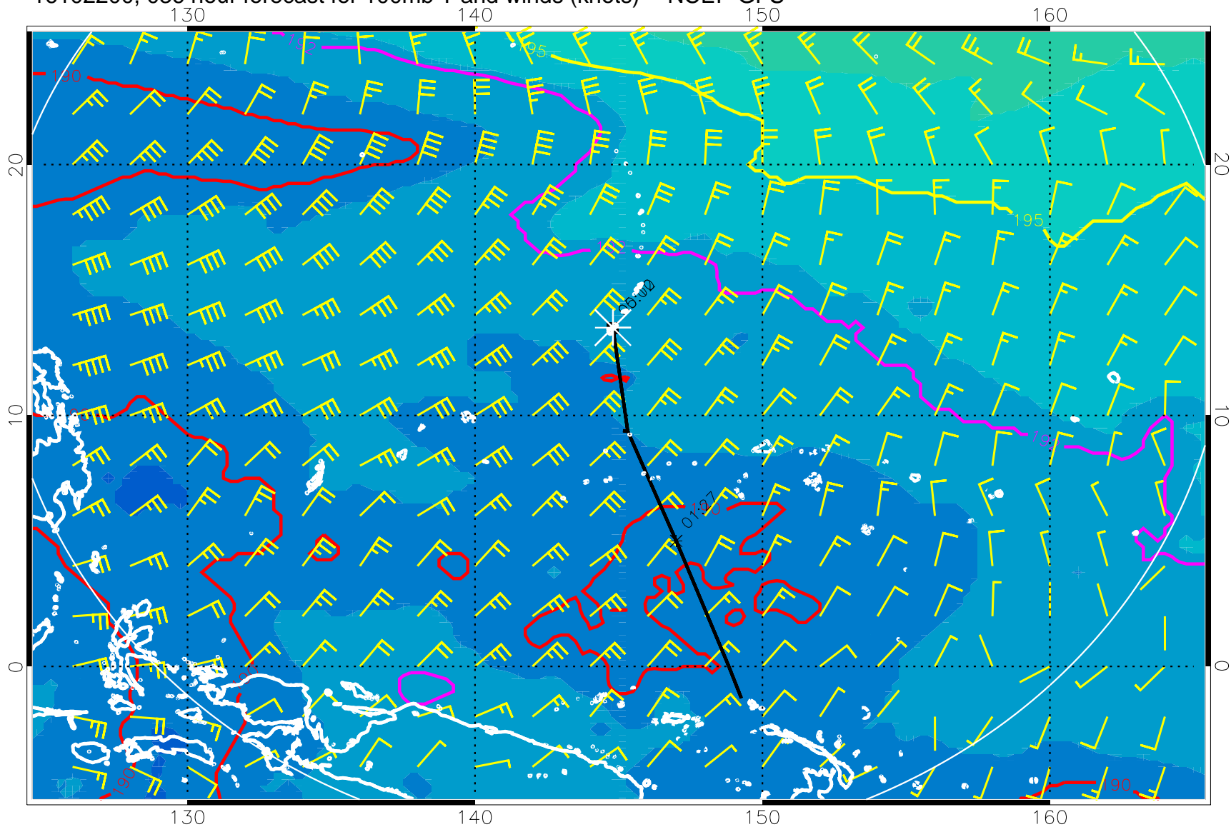
16102200, 036 hour forecast for 100mb T and winds (knots) -- NCEP GFS
