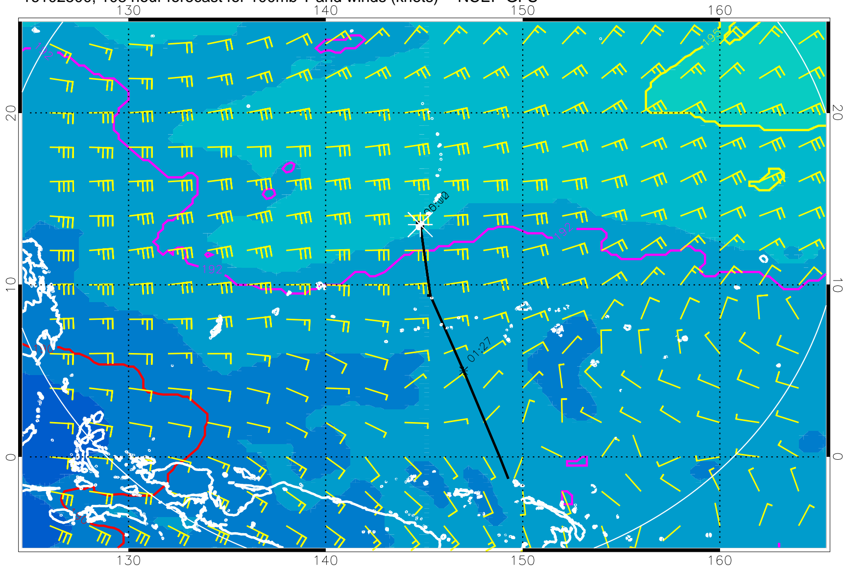
16102500, 108 hour forecast for 100mb T and winds (knots) -- NCEP GFS
