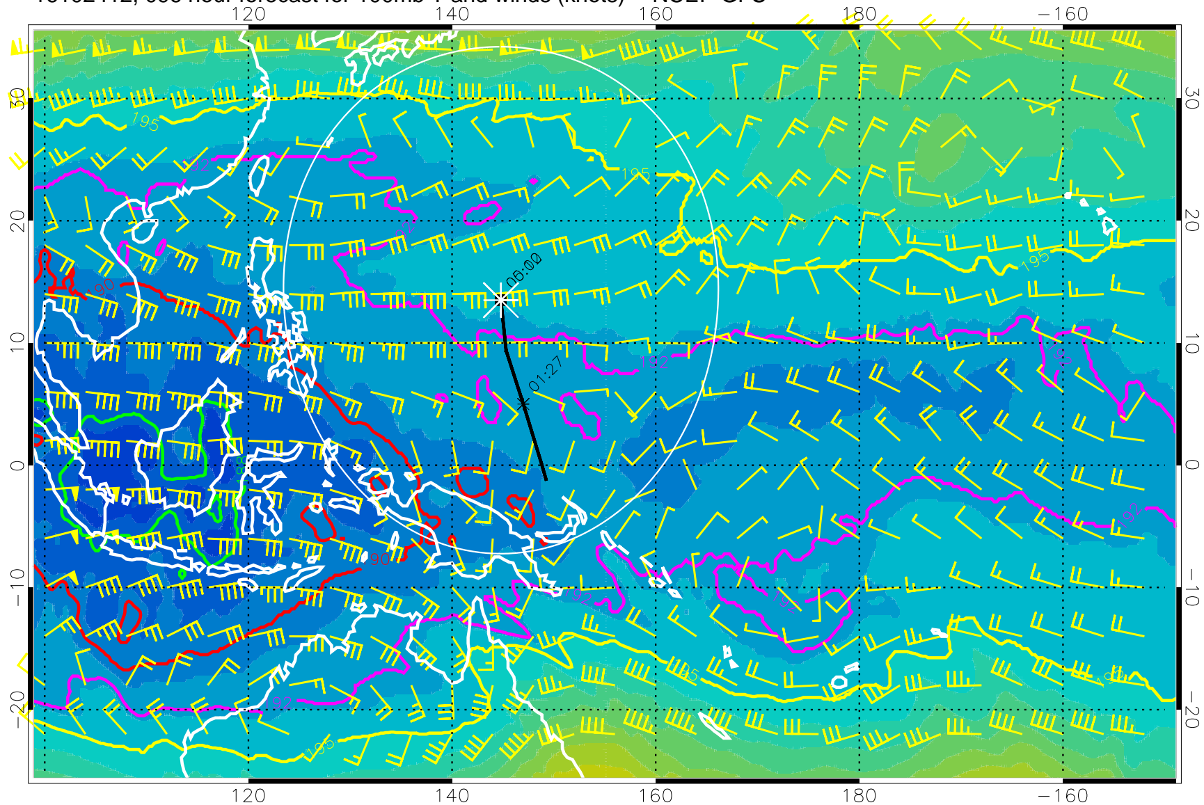
16102412, 096 hour forecast for 100mb T and winds (knots) -- NCEP GFS
