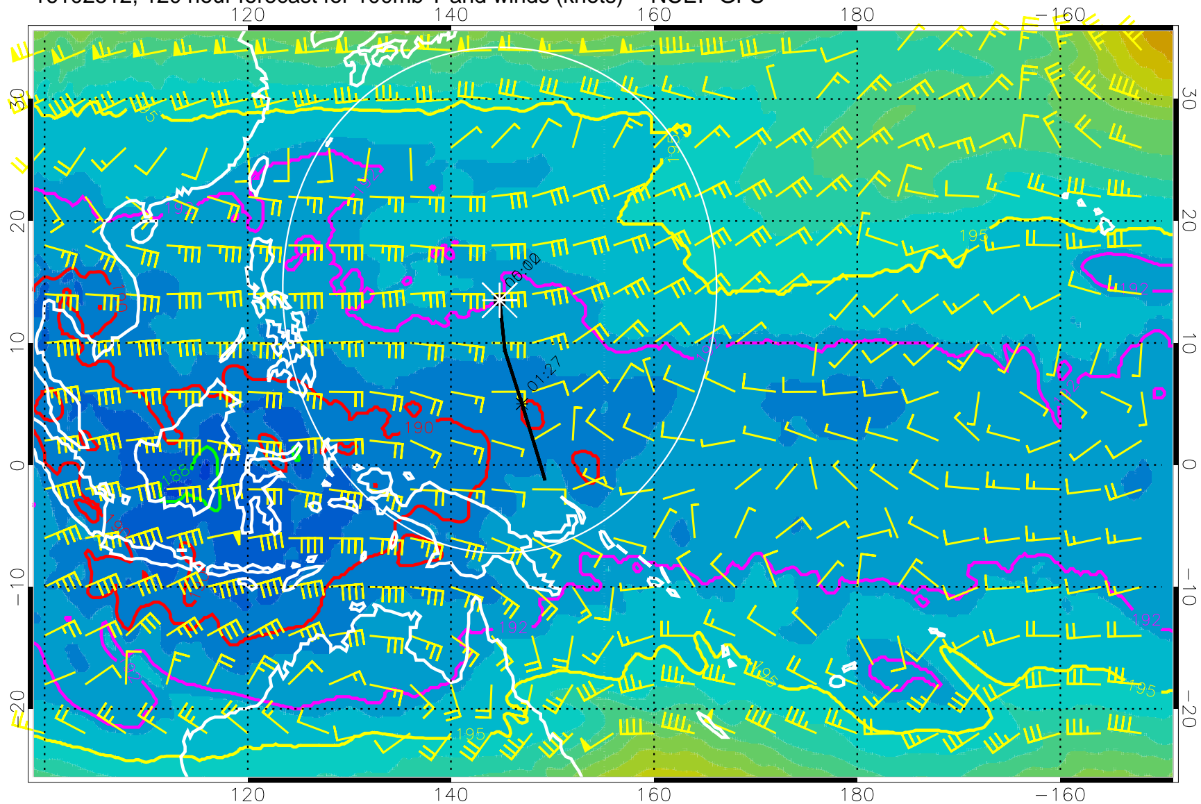
16102512, 120 hour forecast for 100mb T and winds (knots) -- NCEP GFS
