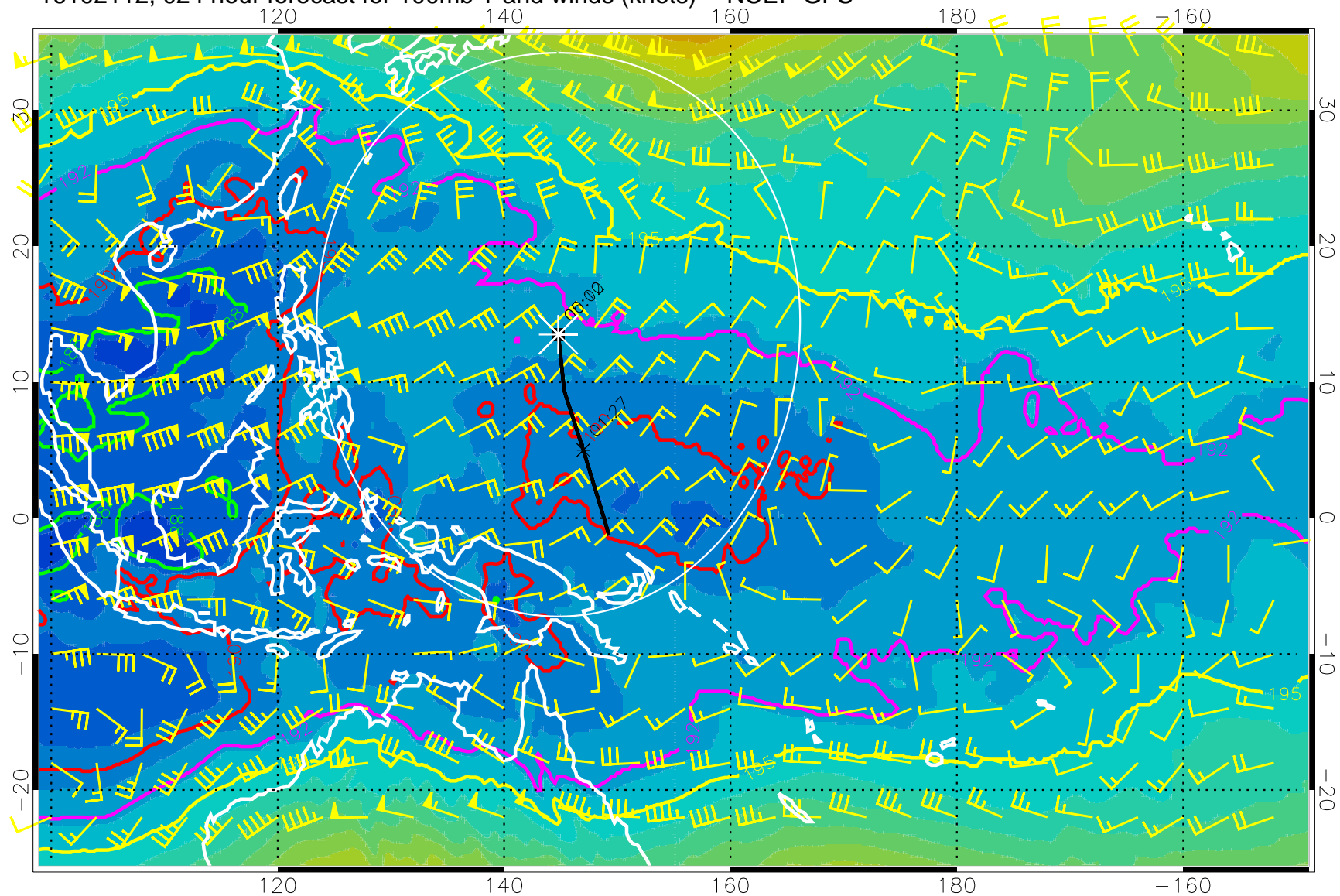
16102112, 024 hour forecast for 100mb T and winds (knots) -- NCEP GFS
