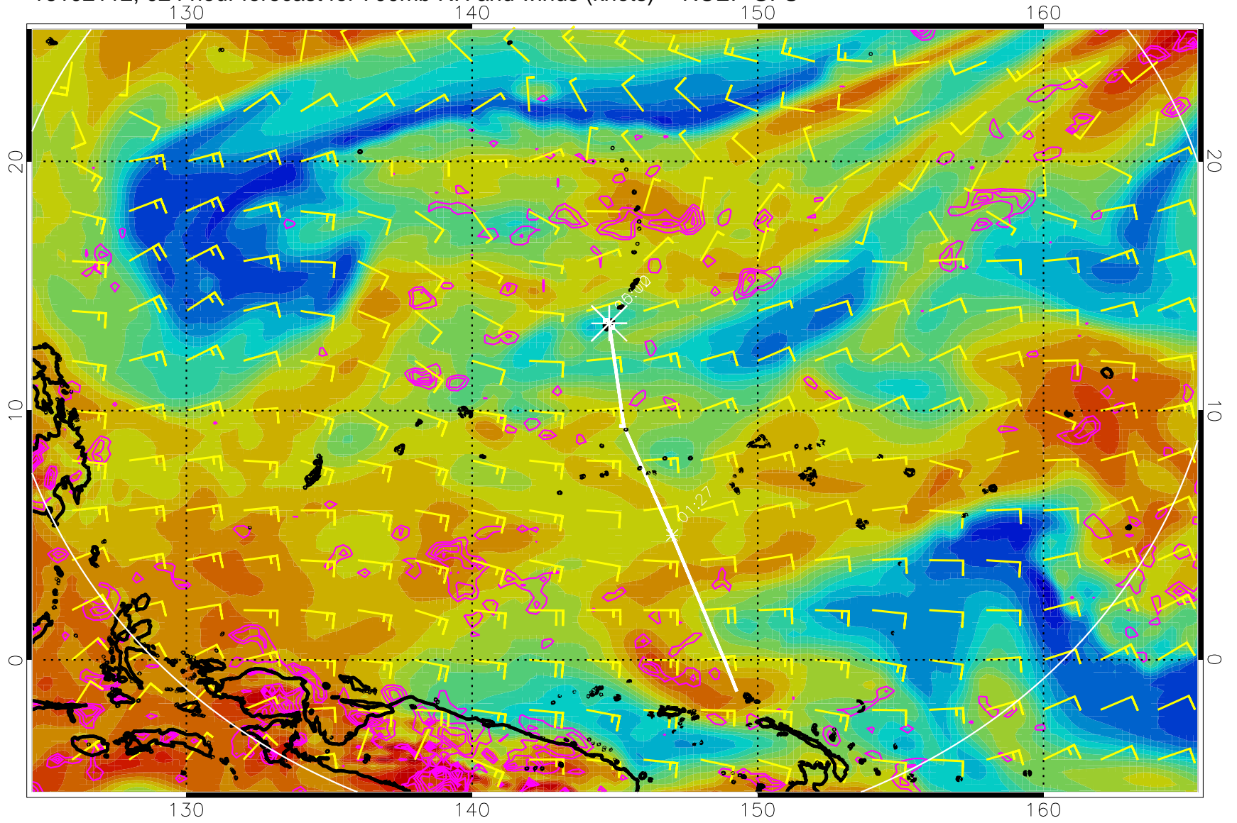
16102112, 024 hour forecast for 700mb RH and winds (knots) -- NCEP GFS
