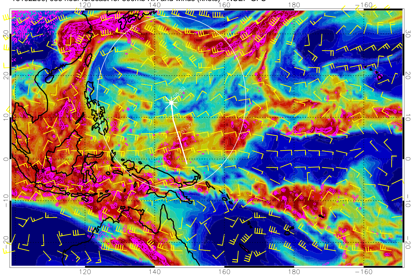
16102200, 036 hour forecast for 500mb RH and winds (knots) - NCEP GFS
