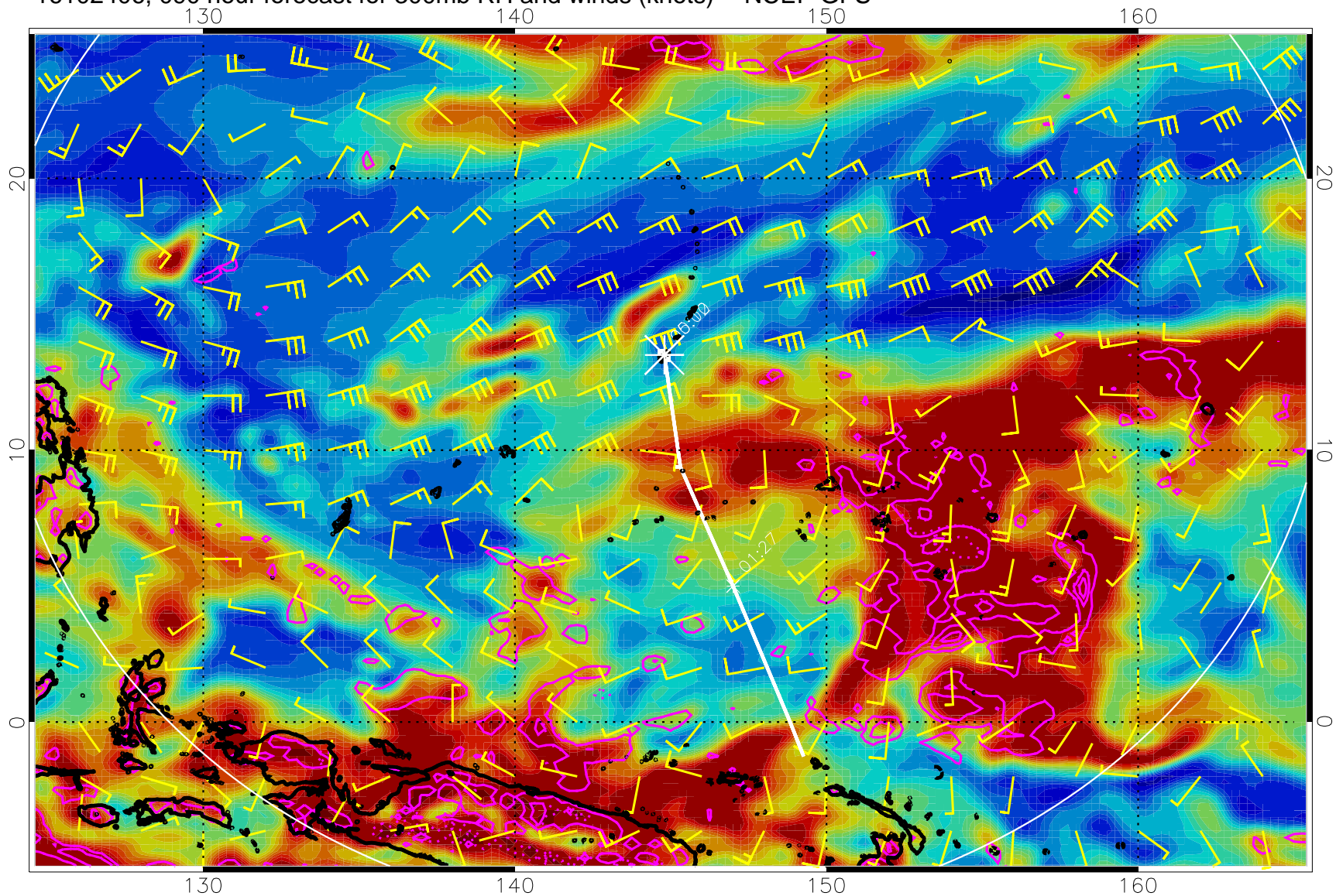
16102406, 090 hour forecast for 300mb RH and winds (knots) -- NCEP GFS
