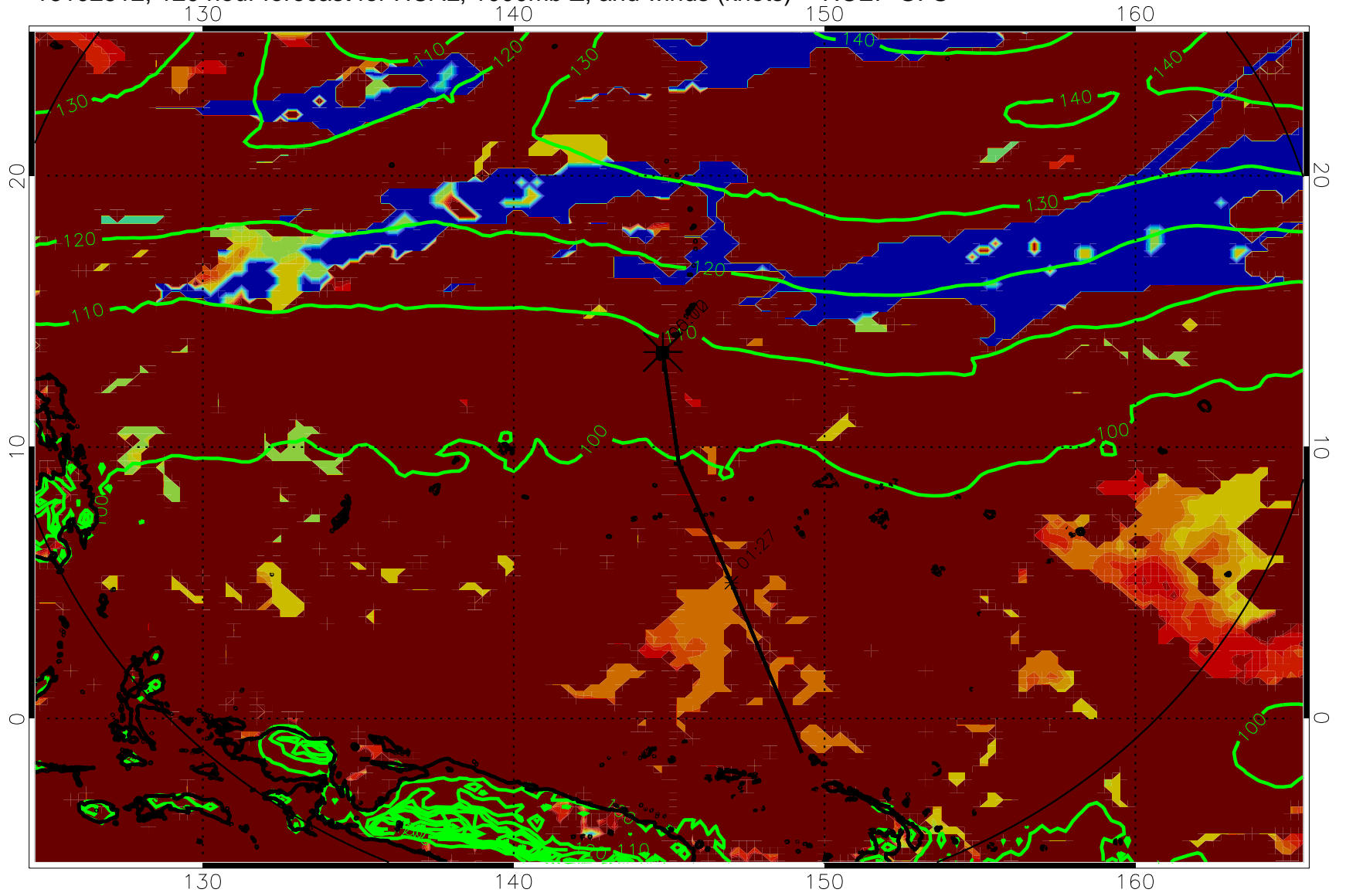
16102512, 120 hour forecast for HCAL, 1000mb Z, and winds (knots) -- NCEP GFS
