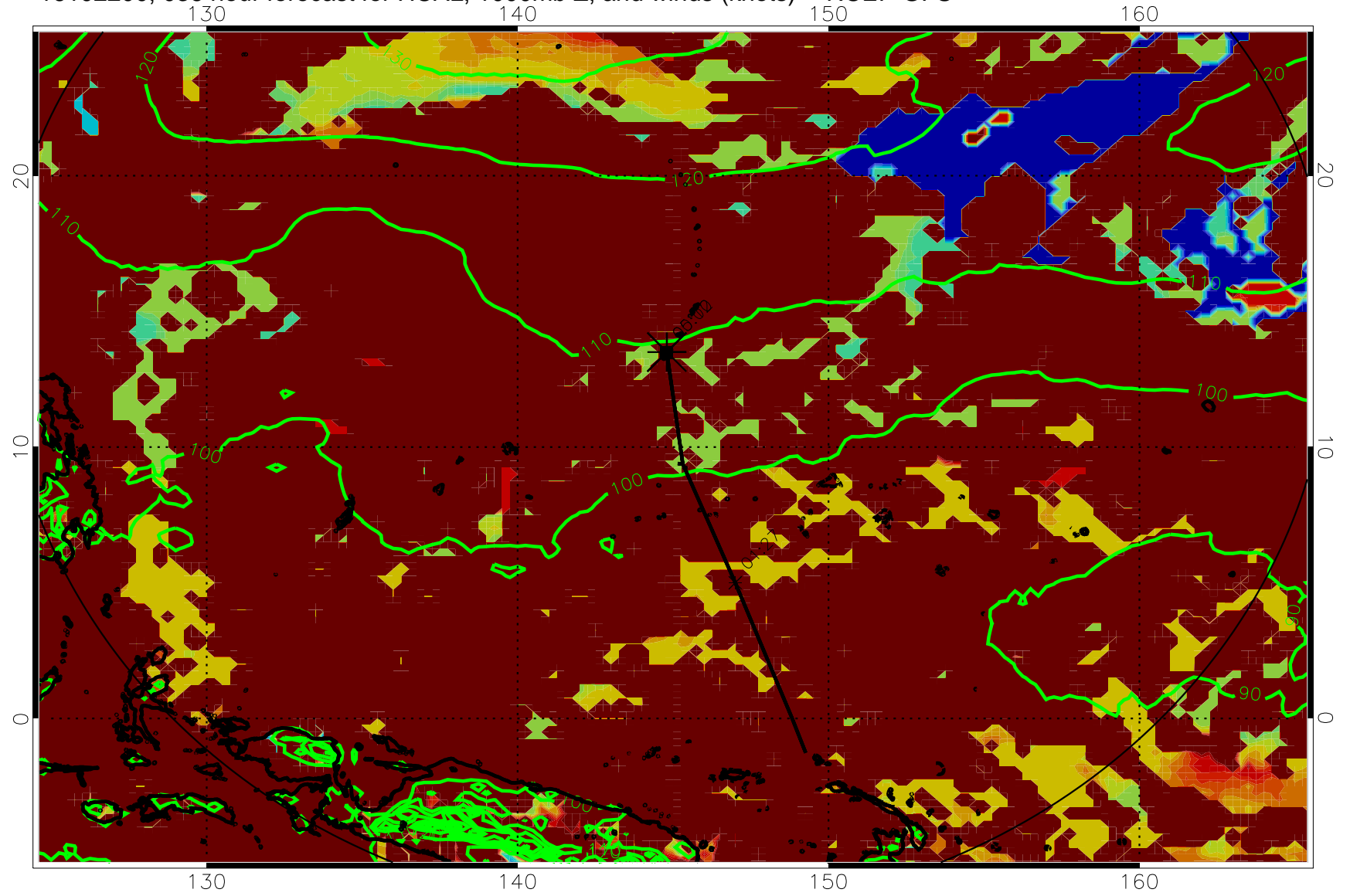
16102200, 036 hour forecast for HCAL, 1000mb Z, and winds (knots) -- NCEP GFS
