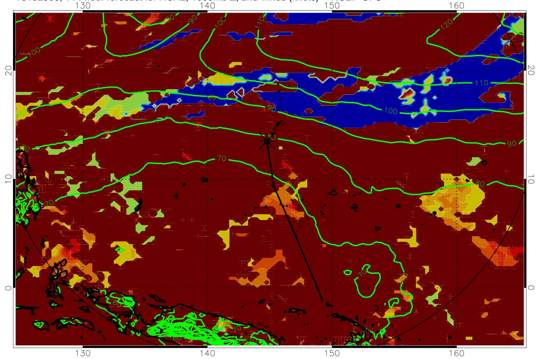
16102506, 114 hour forecast for HCAL, 1000mb Z, and winds (knots) -- NCEP GFS
