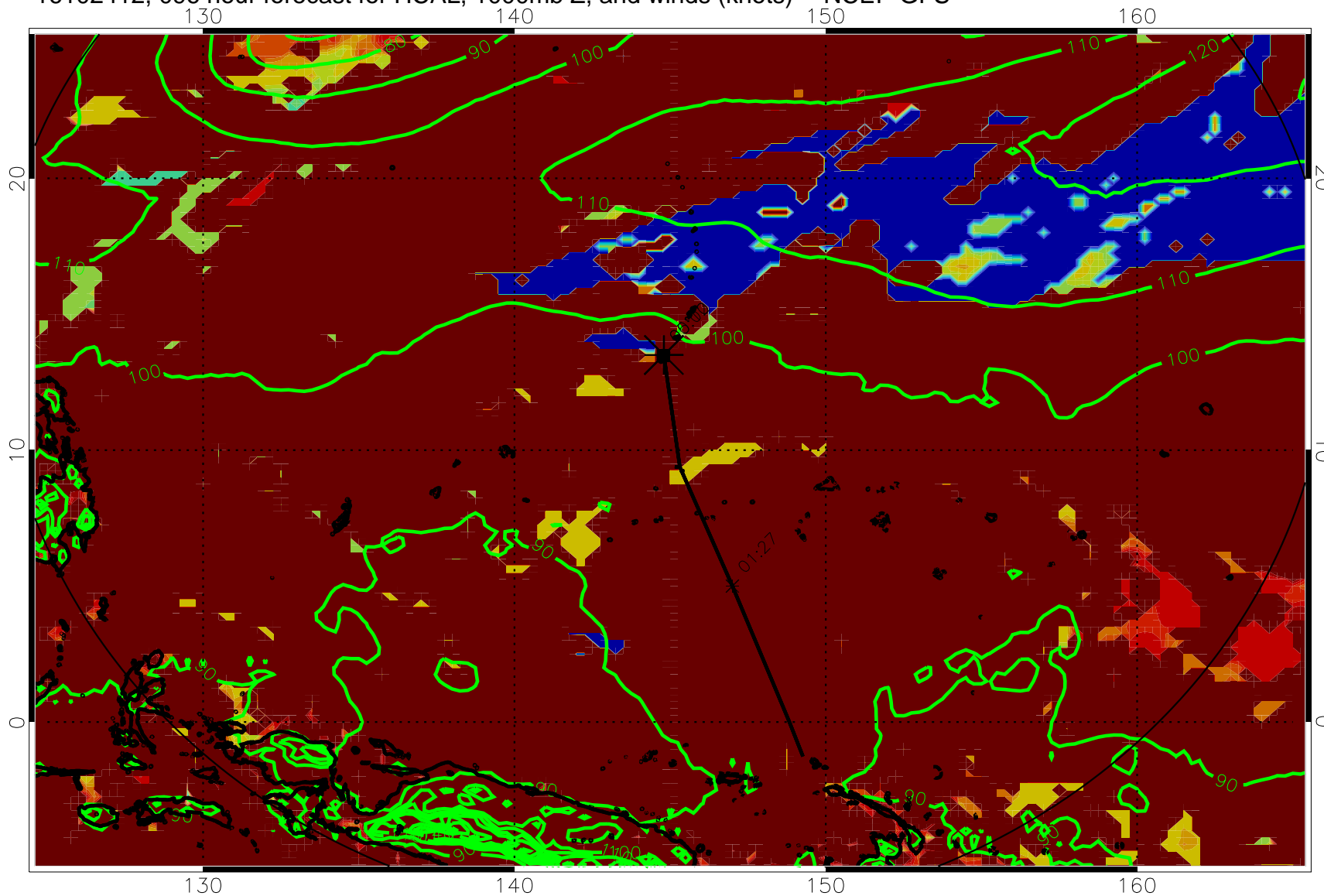
16102412, 096 hour forecast for HCAL, 1000mb Z, and winds (knots) -- NCEP GFS
