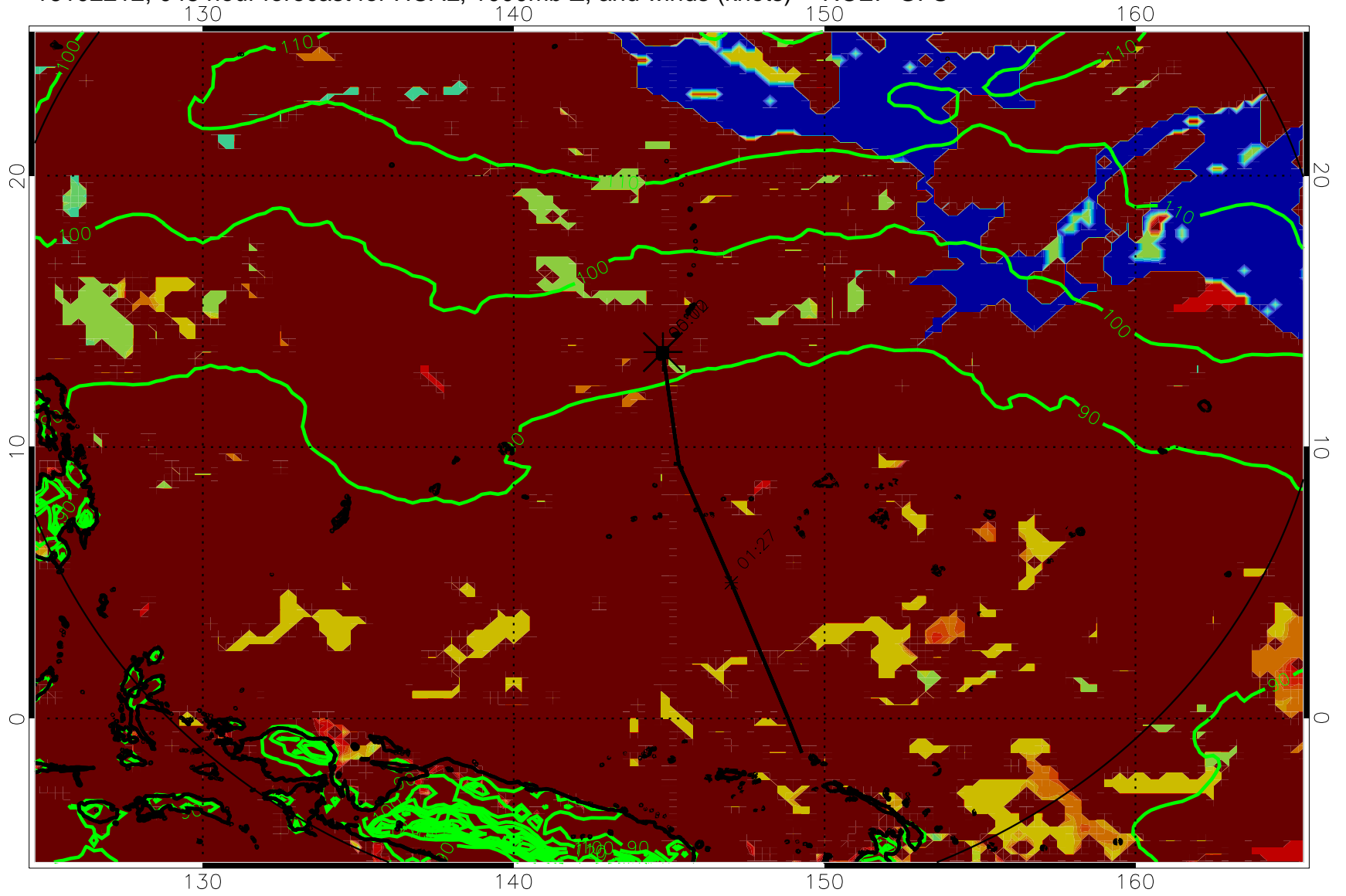
16102212, 048 hour forecast for HCAL, 1000mb Z, and winds (knots) -- NCEP GFS
