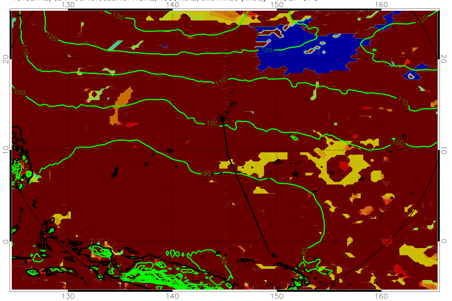
16102112, 024 hour forecast for HCAL, 1000mb Z, and winds (knots) -- NCEP GFS
