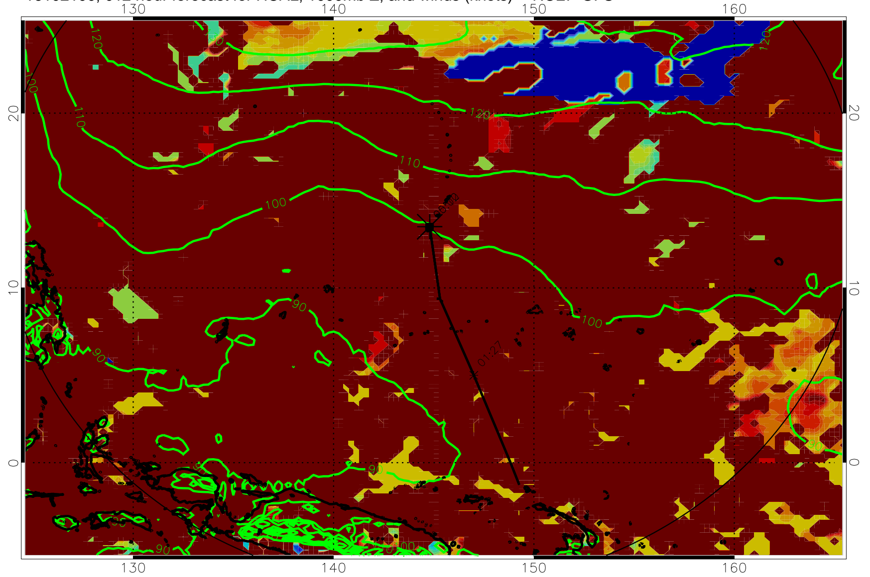
16102100, 012 hour forecast for HCAL, 1000mb Z, and winds (knots) -- NCEP GFS
