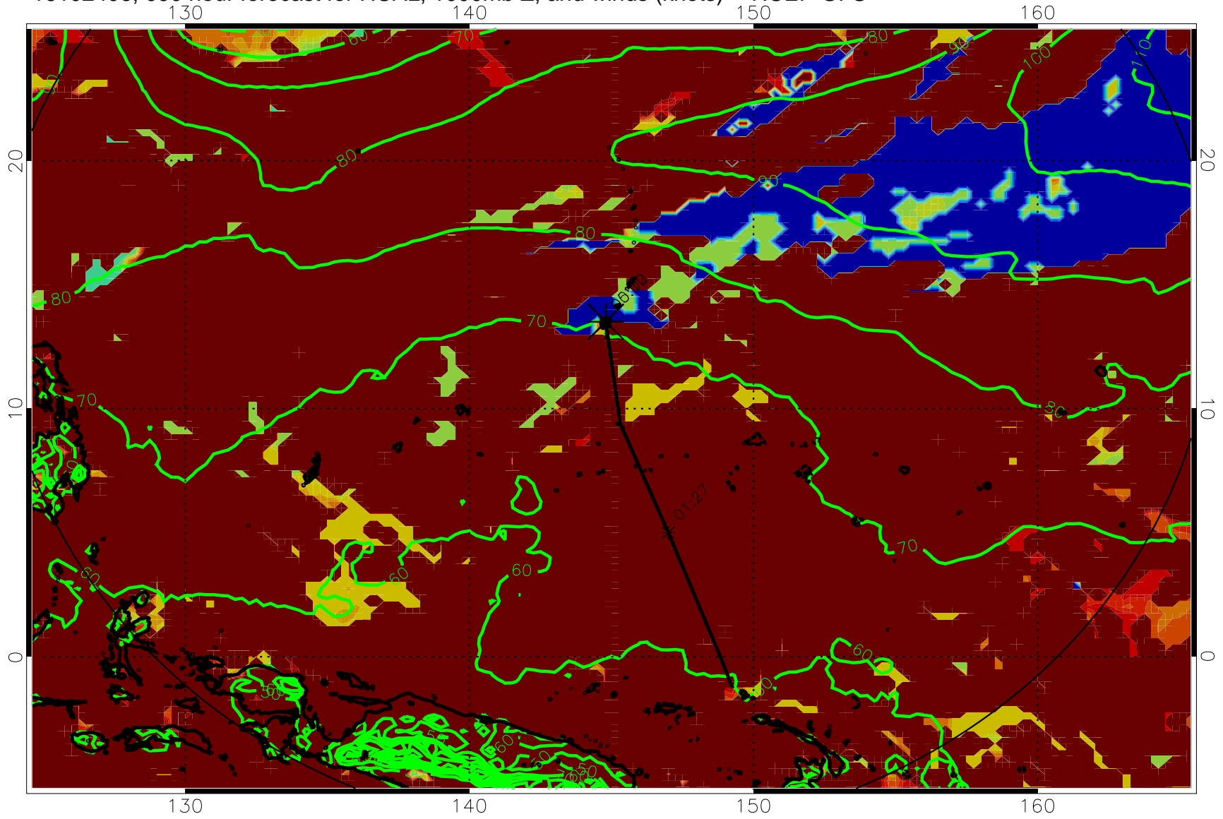
16102406, 090 hour forecast for HCAL, 1000mb Z, and winds (knots) -- NCEP GFS
