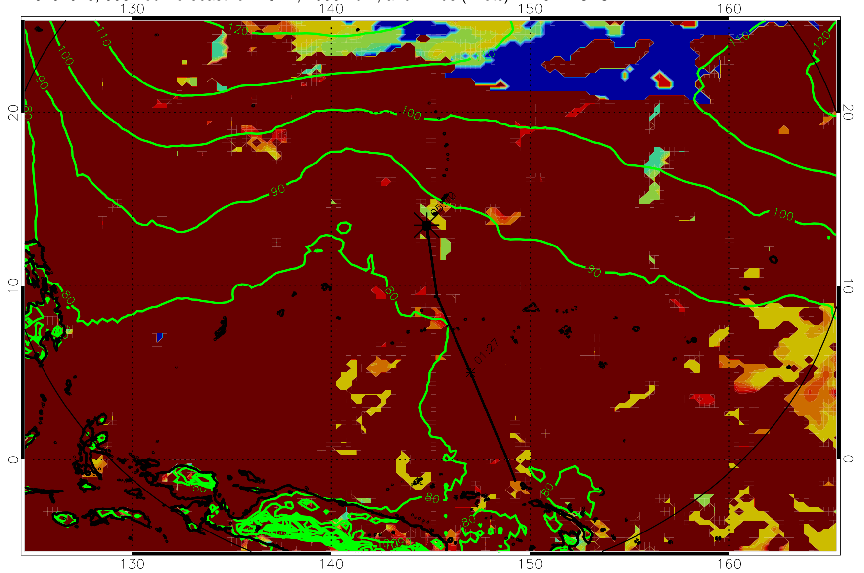
16102018, 006 hour forecast for HCAL, 1000mb Z, and winds (knots) -- NCEP GFS
