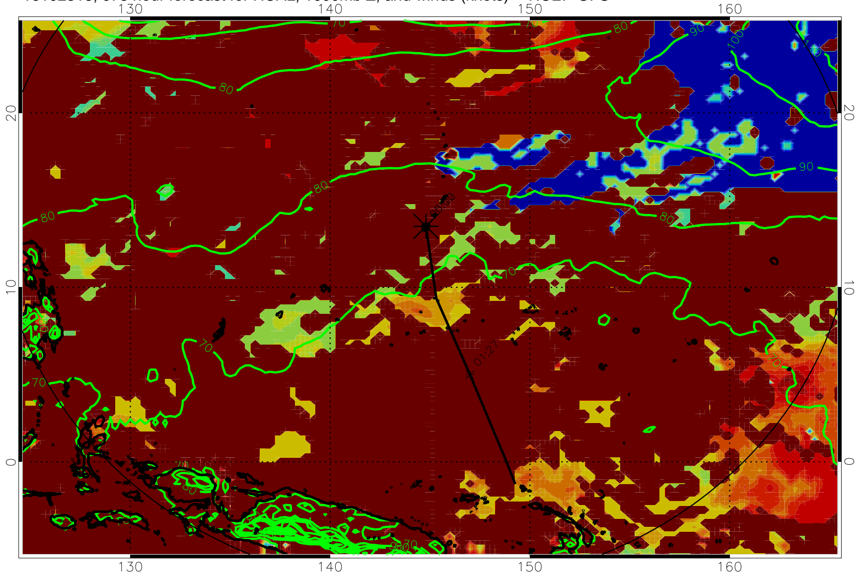
16102318, 078 hour forecast for HCAL, 1000mb Z, and winds (knots) -- NCEP GFS
