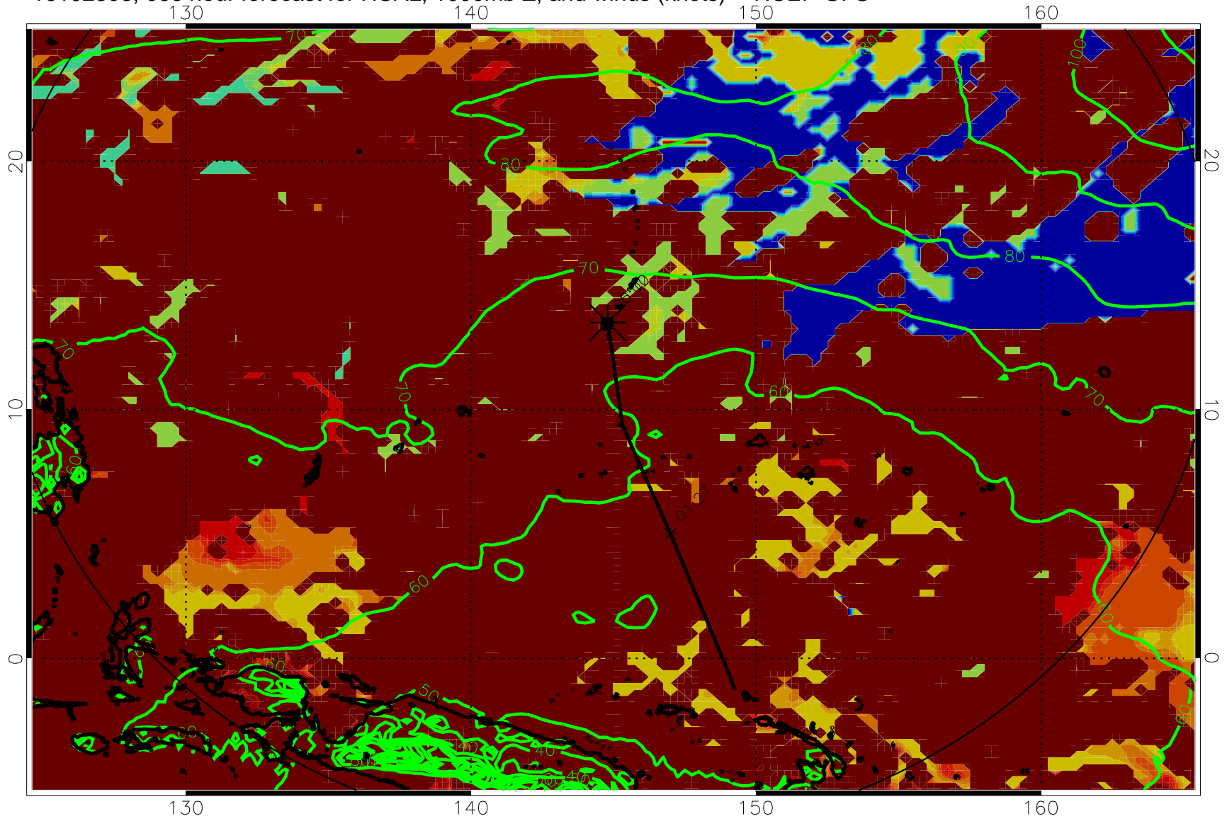
16102306, 066 hour forecast for HCAL, 1000mb Z, and winds (knots) -- NCEP GFS
