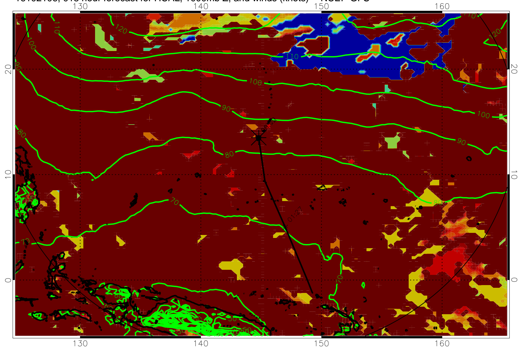
16102106, 018 hour forecast for HCAL, 1000mb Z, and winds (knots) -- NCEP GFS
