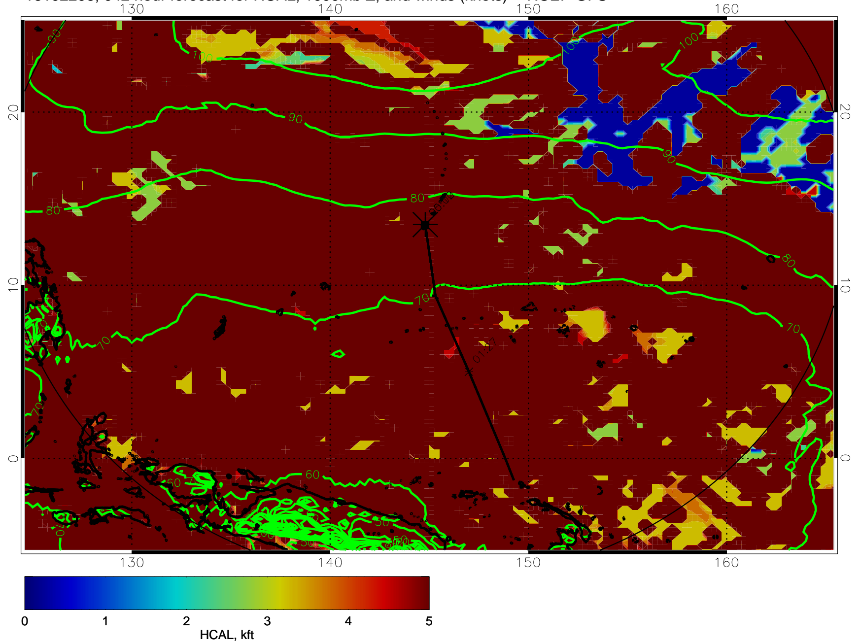
16102206, 042 hour forecast for HCAL, 1000mb Z, and winds (knots) -- NCEP GFS
