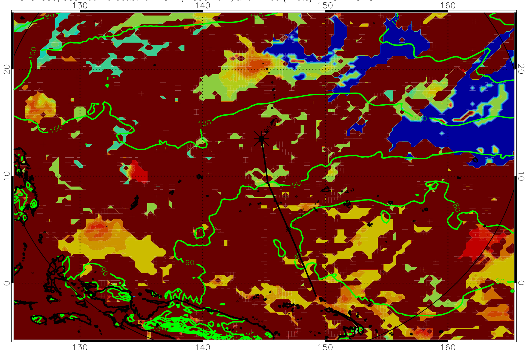
16102300, 060 hour forecast for HCAL, 1000mb Z, and winds (knots) -- NCEP GFS
