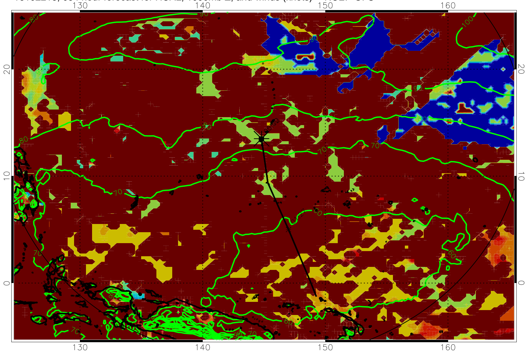
16102218, 054 hour forecast for HCAL, 1000mb Z, and winds (knots) -- NCEP GFS
