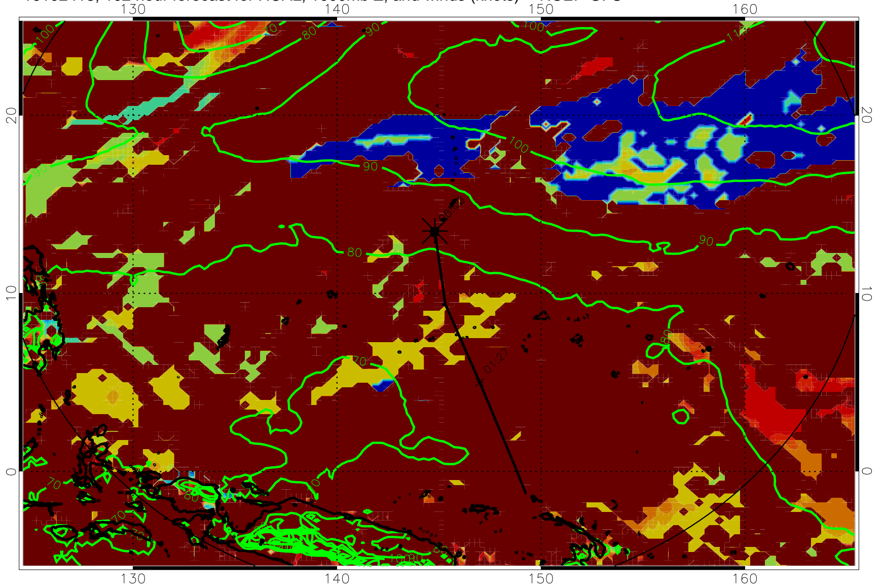
16102418, 102 hour forecast for HCAL, 1000mb Z, and winds (knots) -- NCEP GFS
