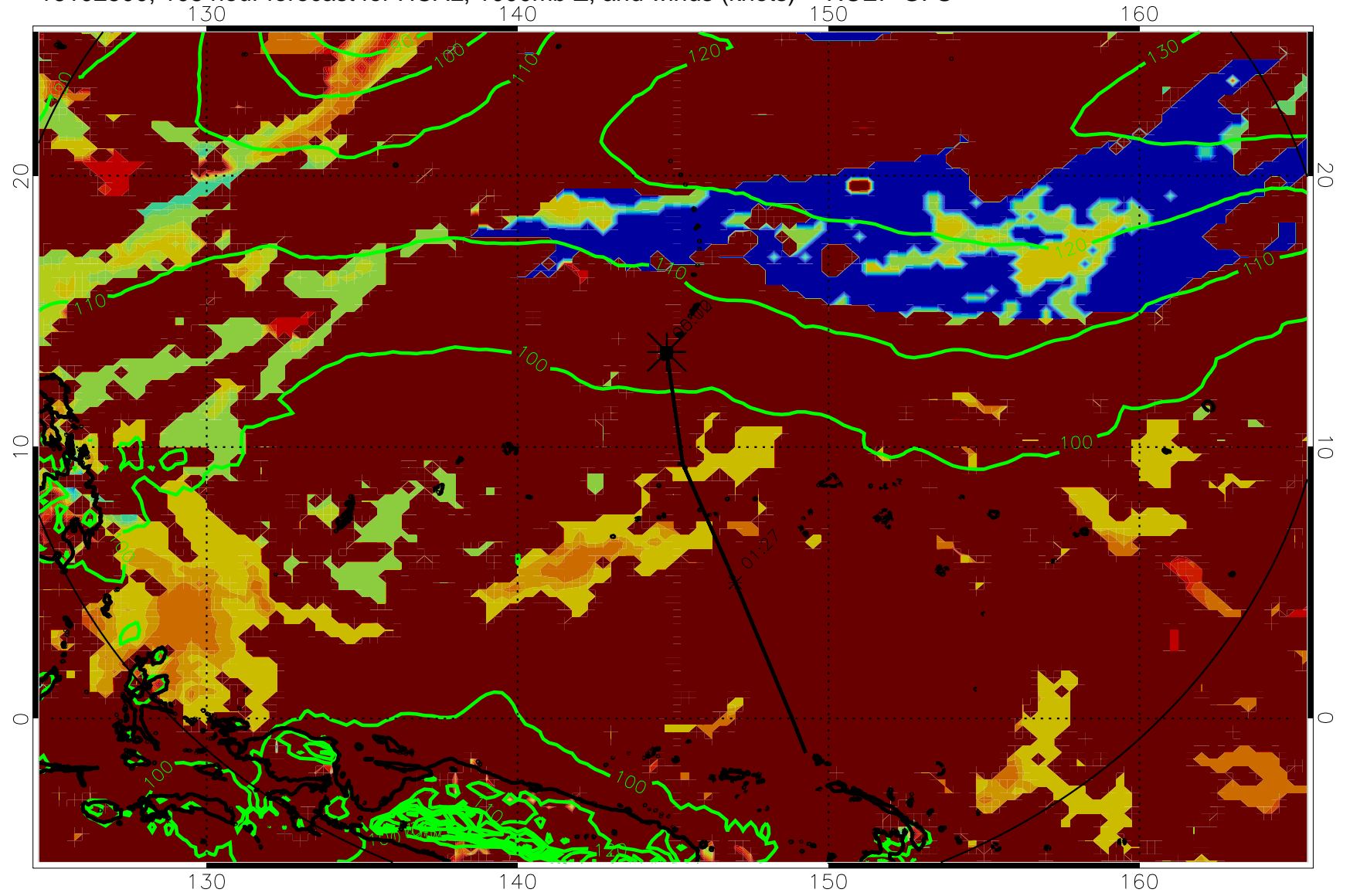
16102500, 108 hour forecast for HCAL, 1000mb Z, and winds (knots) -- NCEP GFS
