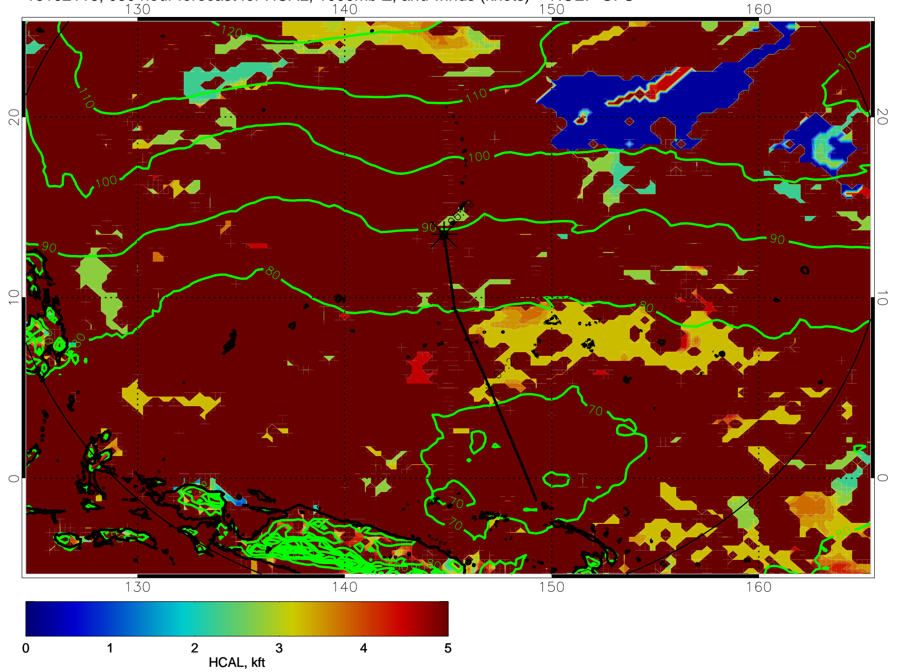
16102118, 030 hour forecast for HCAL, 1000mb Z, and winds (knots) -- NCEP GFS
