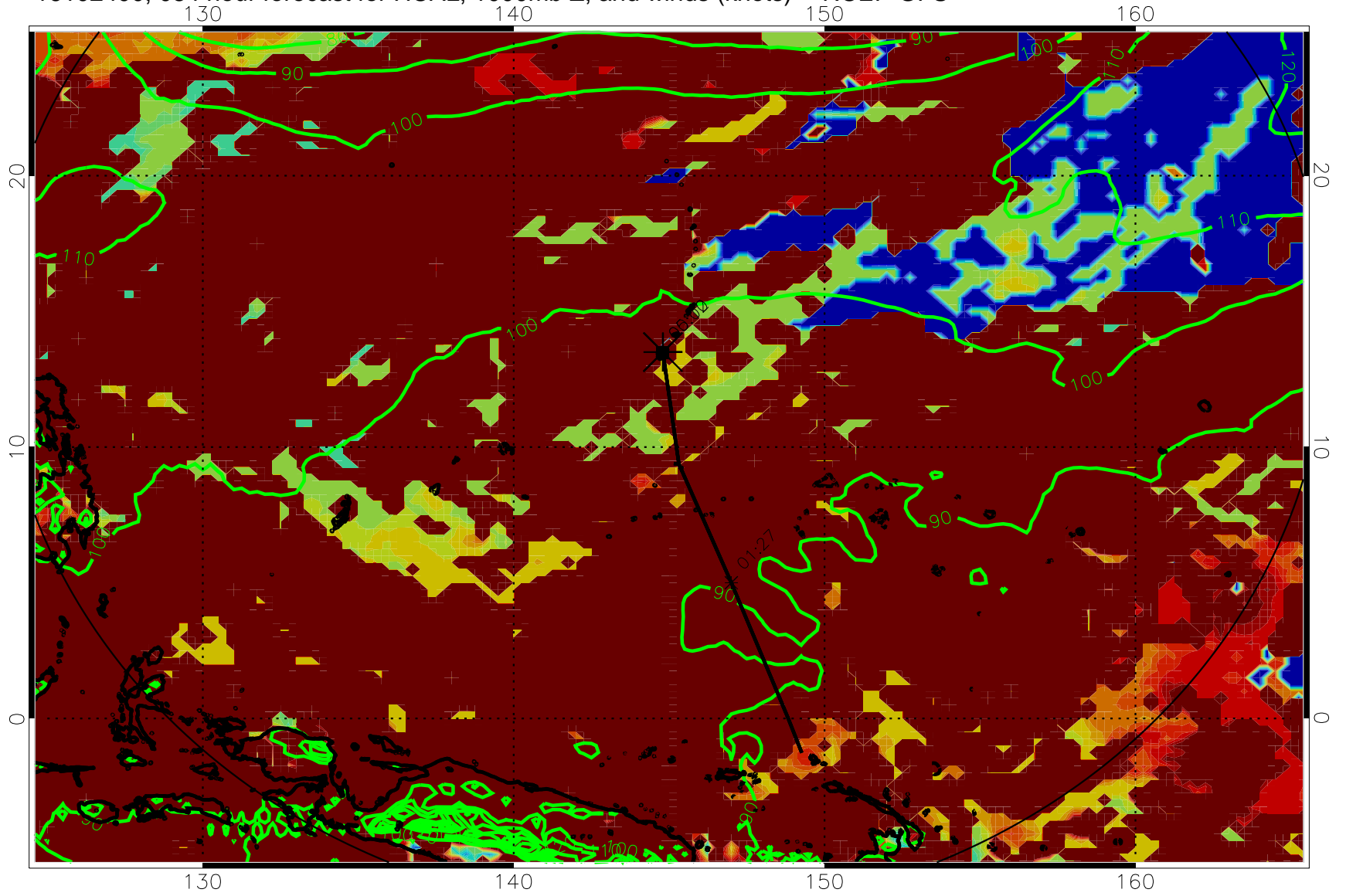
16102400, 084 hour forecast for HCAL, 1000mb Z, and winds (knots) -- NCEP GFS
