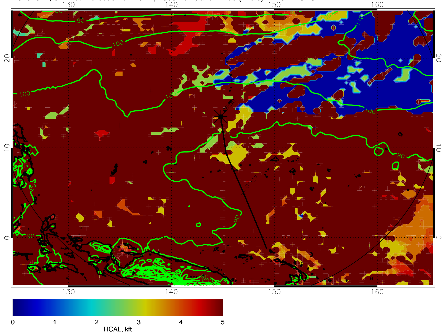
16102312, 072 hour forecast for HCAL, 1000mb Z, and winds (knots) -- NCEP GFS
