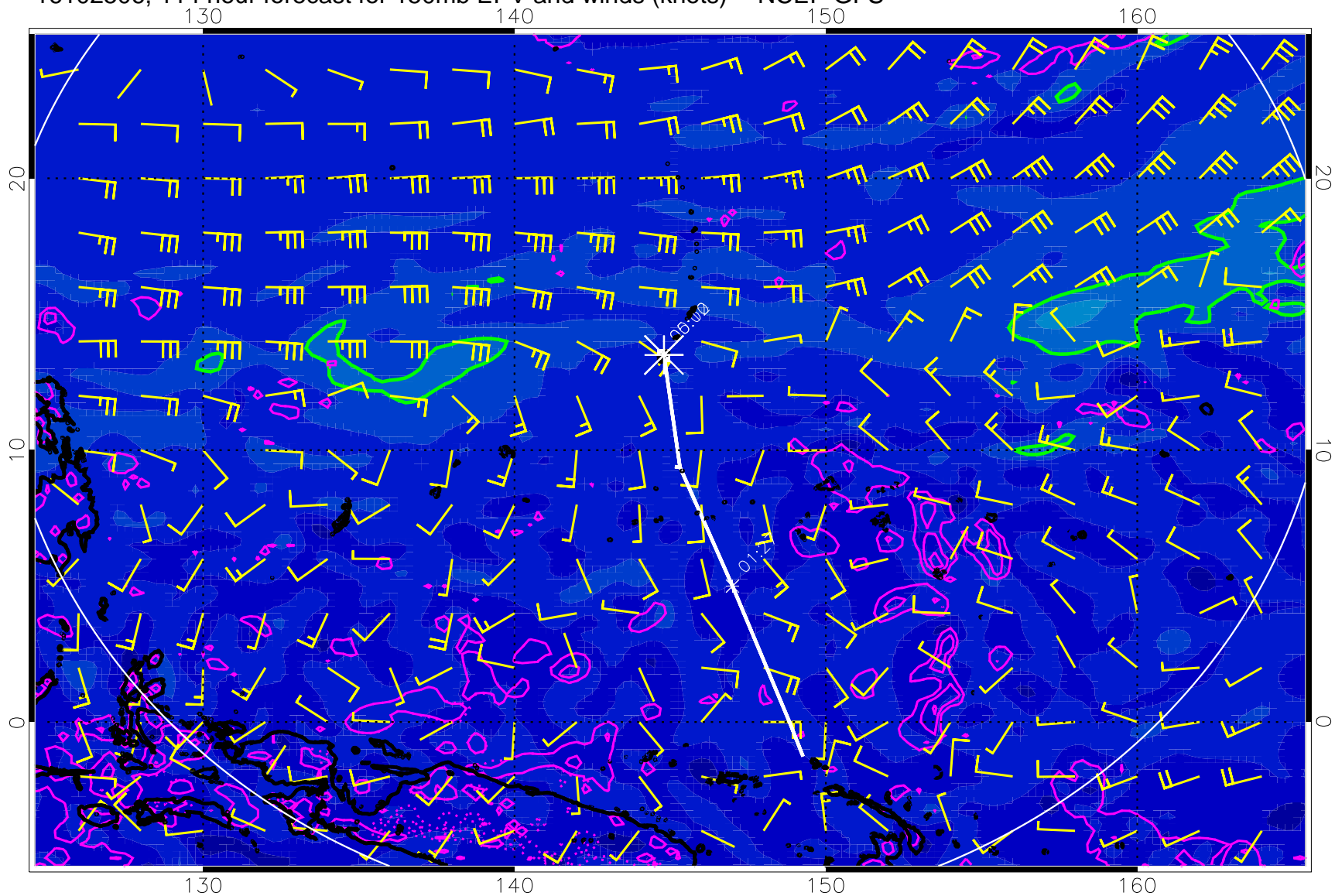
16102506, 114 hour forecast for 150mb EPV and winds (knots) -- NCEP GFS
