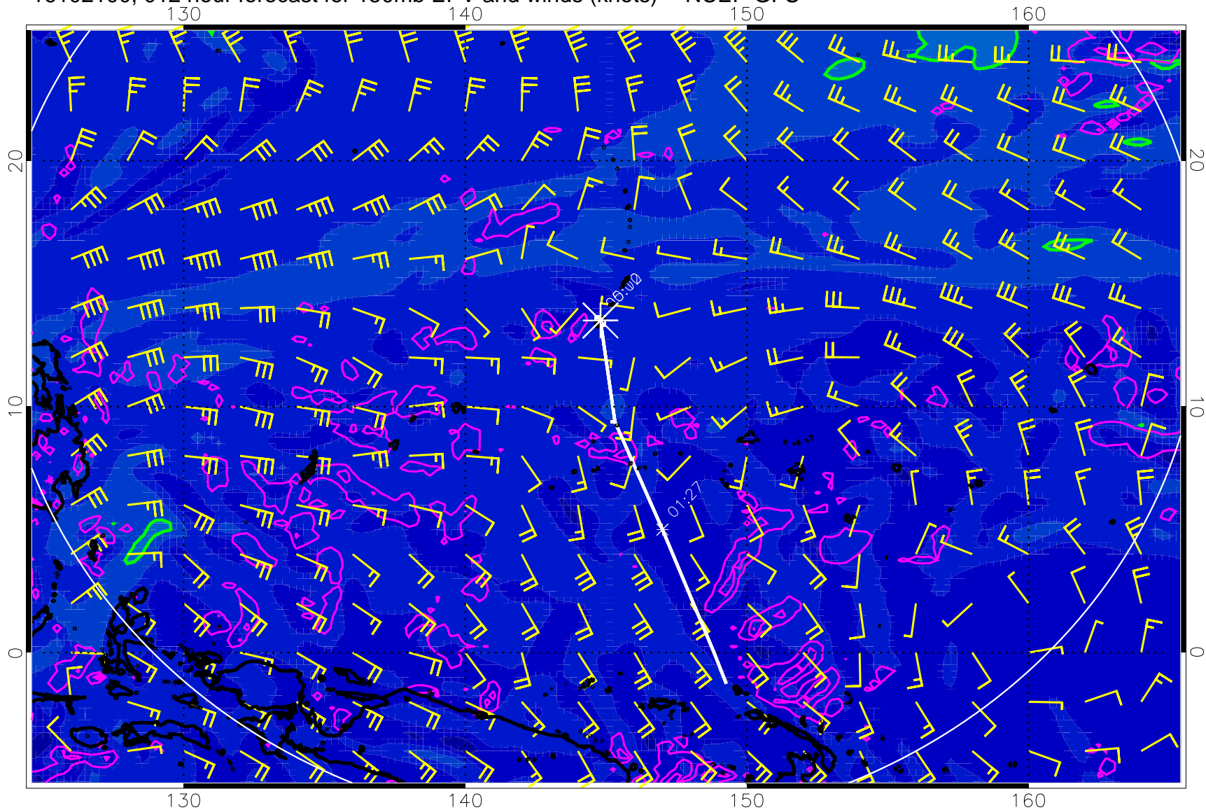
16102100, 012 hour forecast for 150mb EPV and winds (knots) -- NCEP GFS
