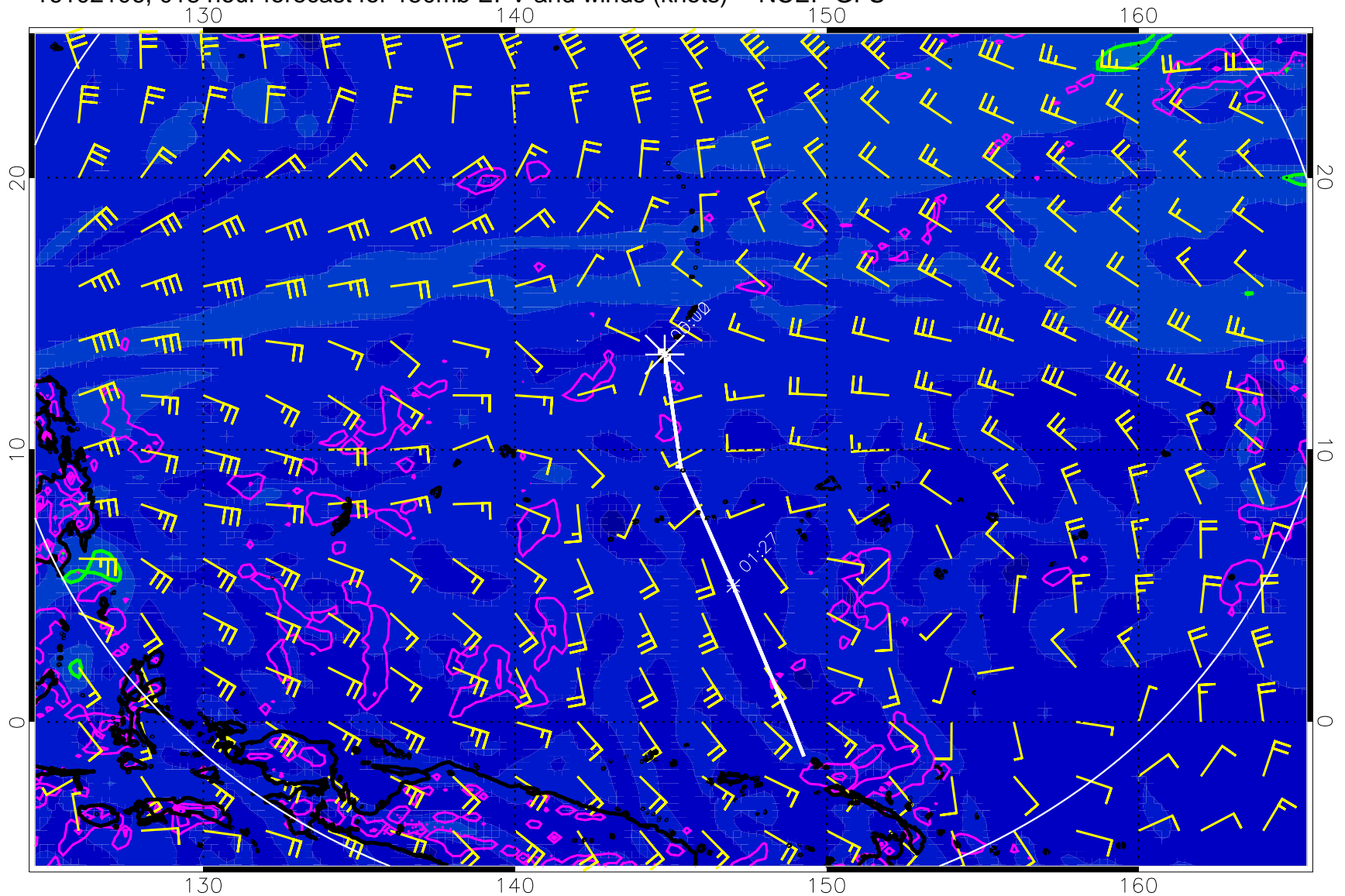
16102106, 018 hour forecast for 150mb EPV and winds (knots) -- NCEP GFS
