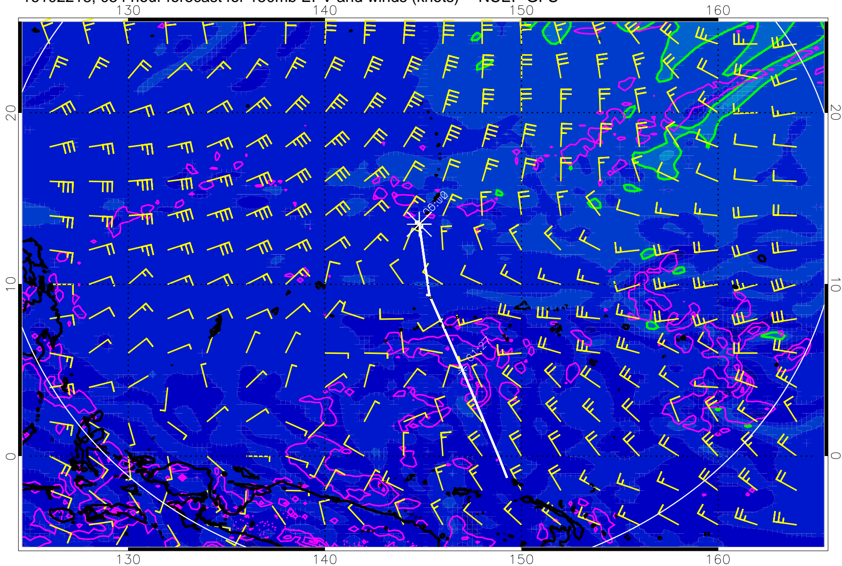
16102218, 054 hour forecast for 150mb EPV and winds (knots) -- NCEP GFS
