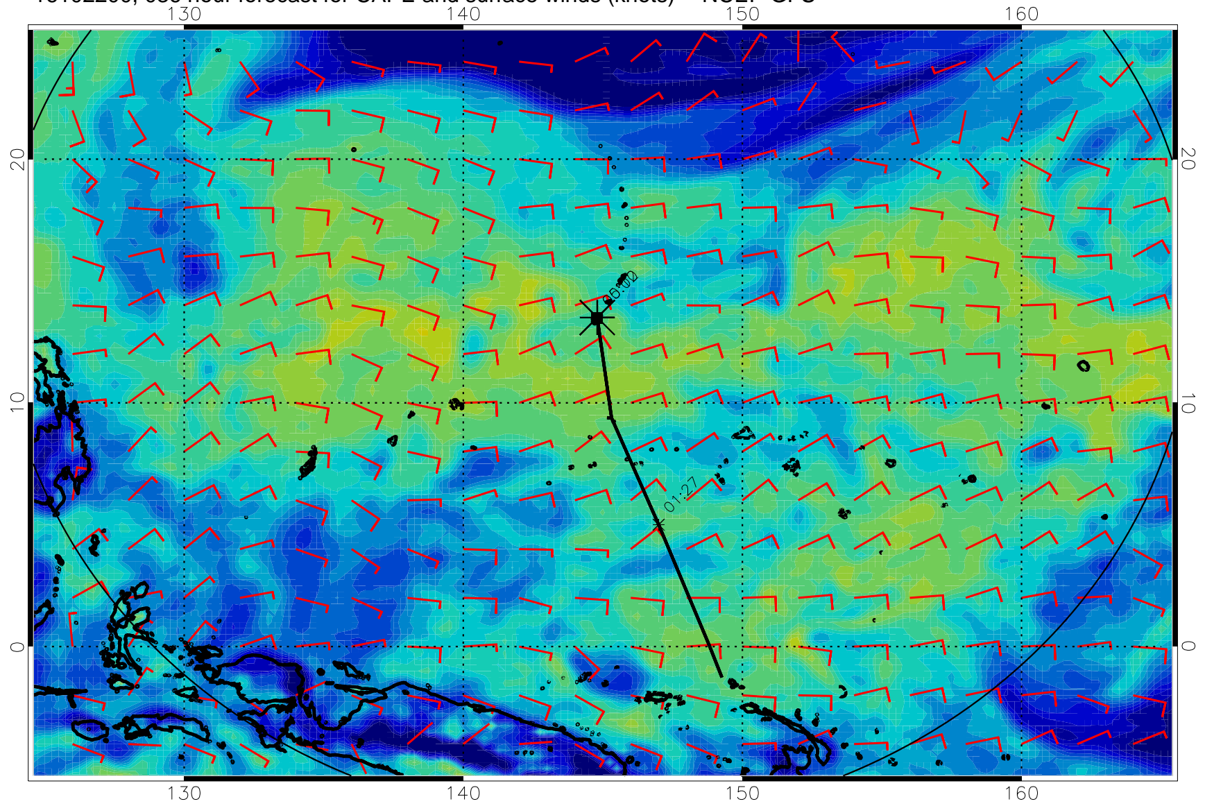
16102200, 036 hour forecast for CAPE and surface winds (knots) -- NCEP GFS
