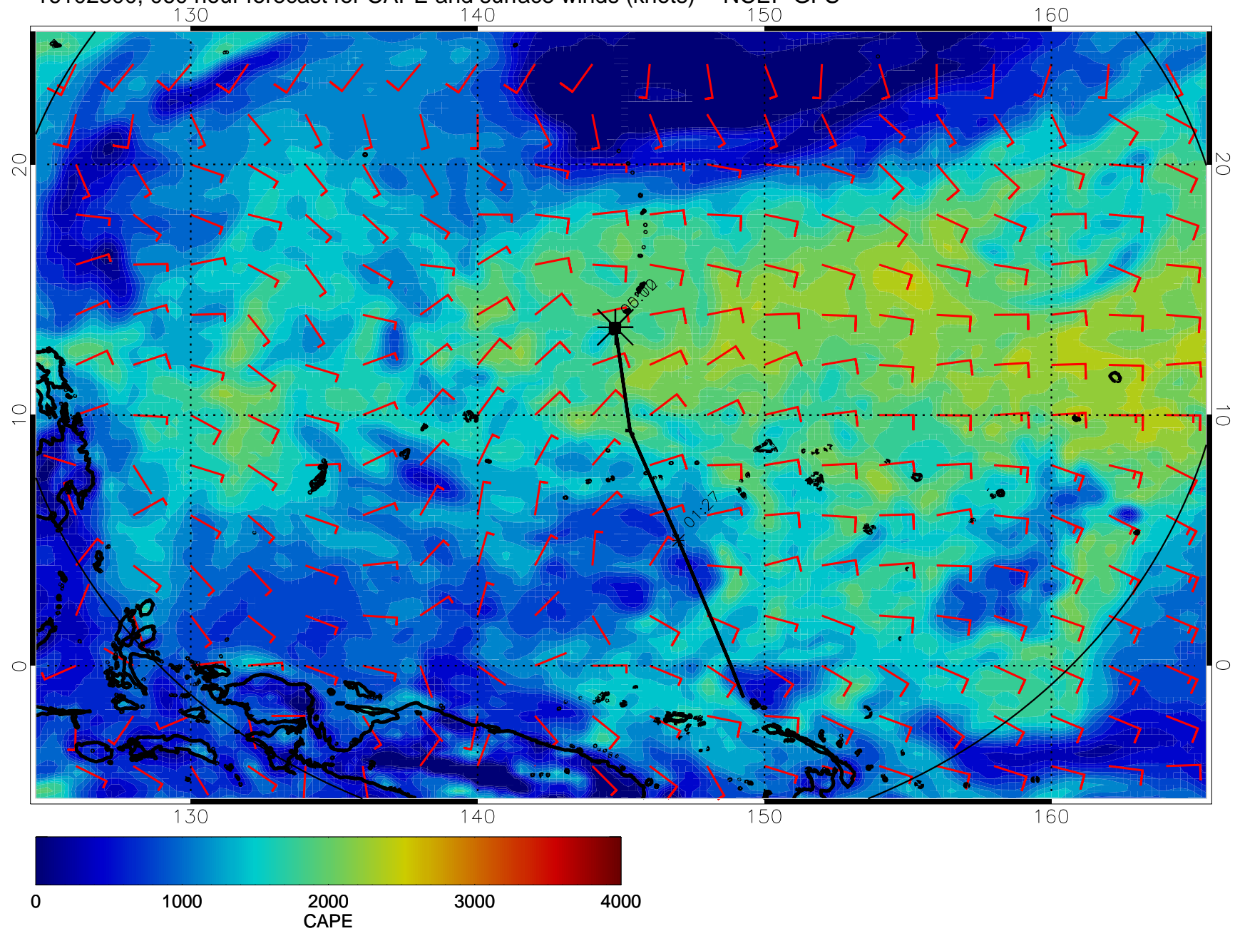
16102300, 060 hour forecast for CAPE and surface winds (knots) -- NCEP GFS
