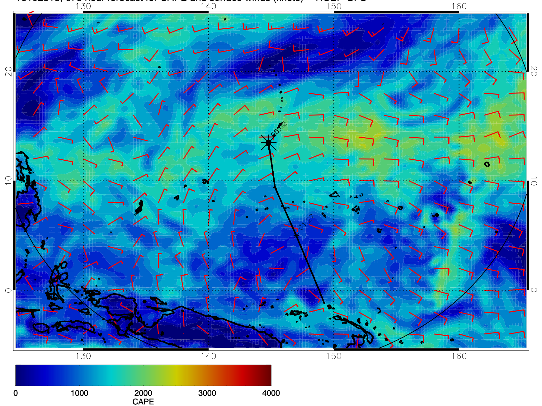
16102318, 078 hour forecast for CAPE and surface winds (knots) -- NCEP GFS
