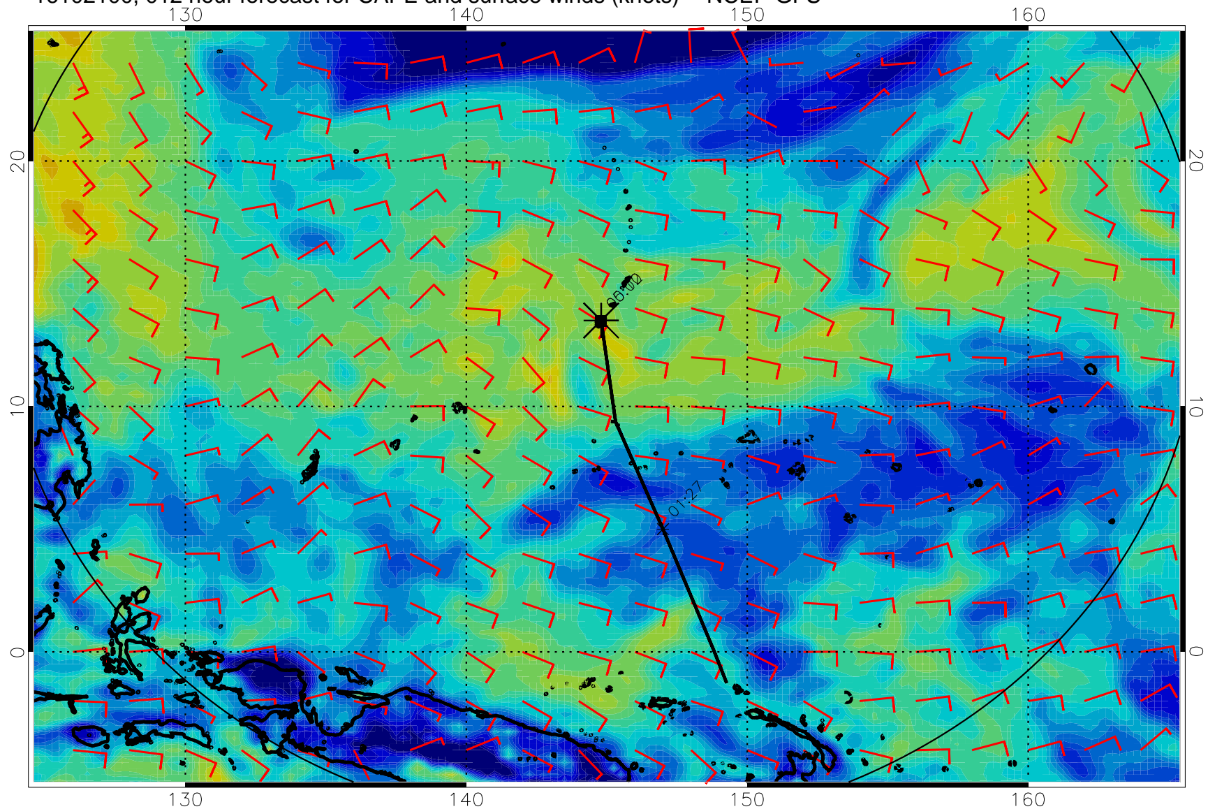
16102100, 012 hour forecast for CAPE and surface winds (knots) -- NCEP GFS
