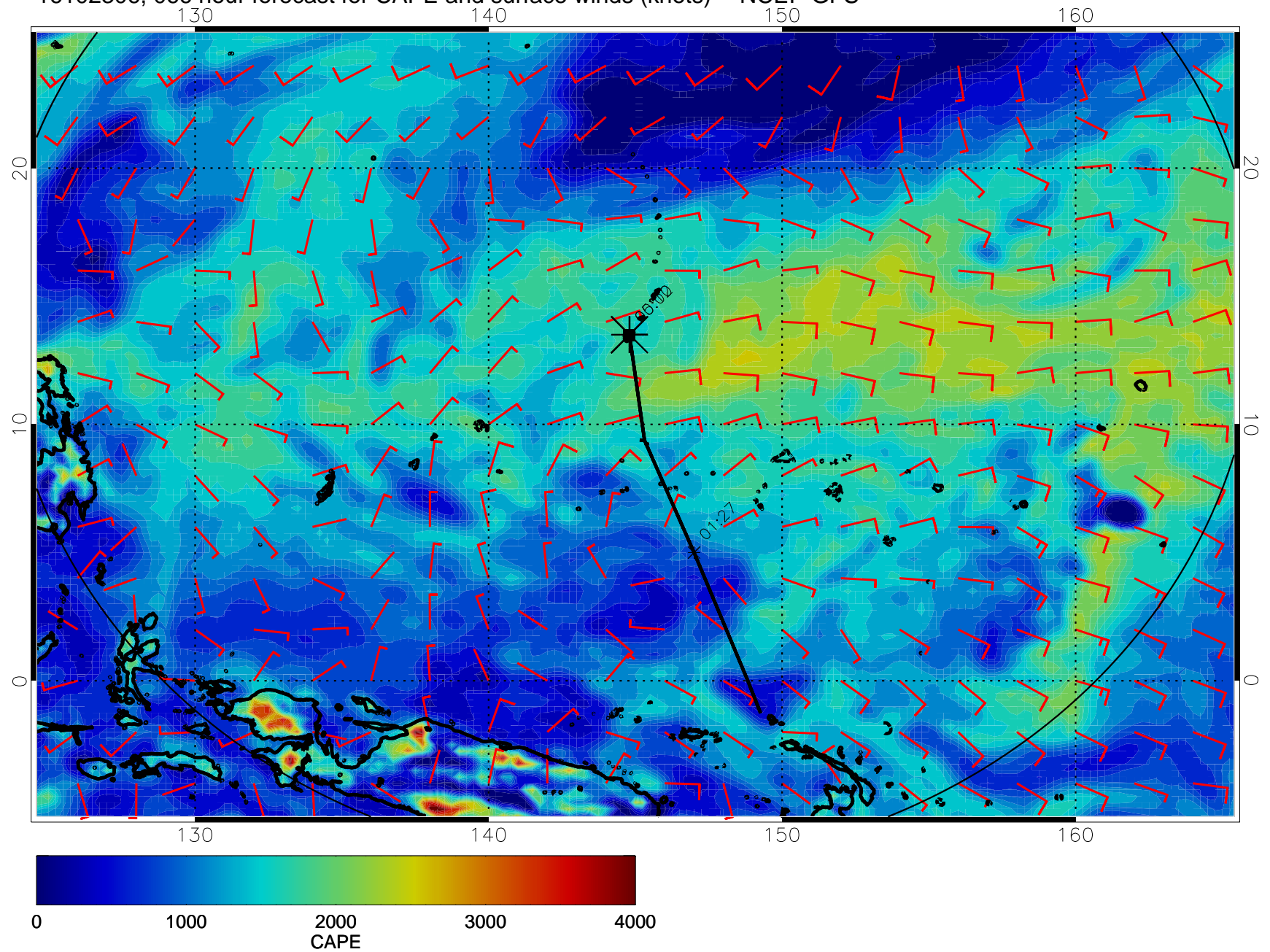
16102306, 066 hour forecast for CAPE and surface winds (knots) -- NCEP GFS
