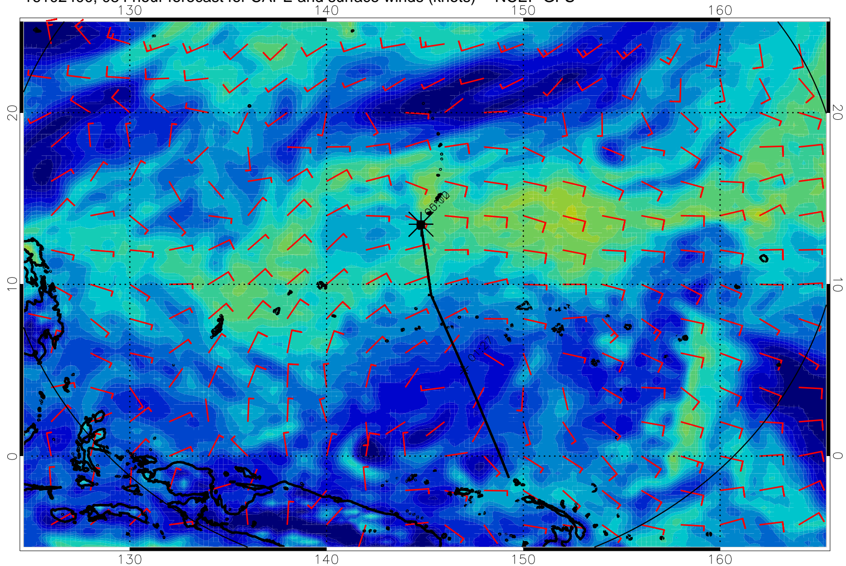
16102400, 084 hour forecast for CAPE and surface winds (knots) -- NCEP GFS
