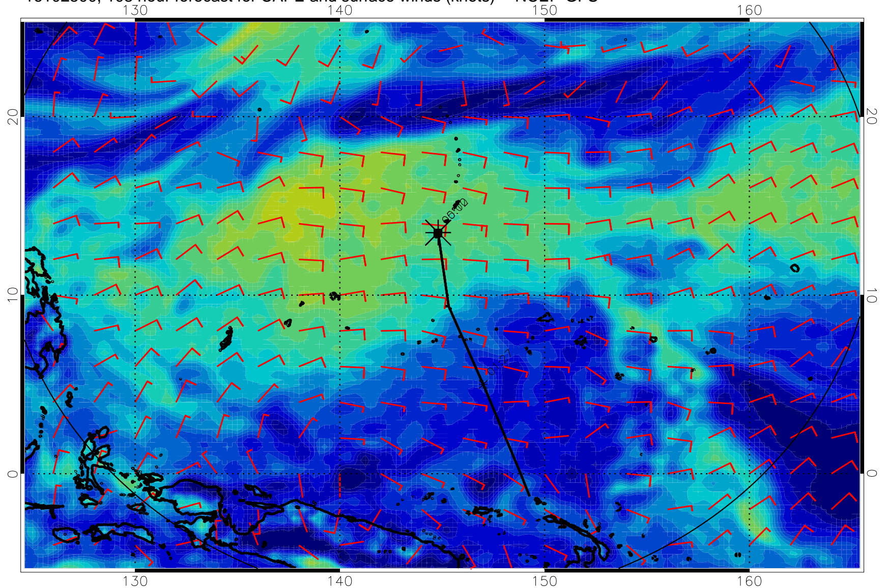
16102500, 108 hour forecast for CAPE and surface winds (knots) -- NCEP GFS
