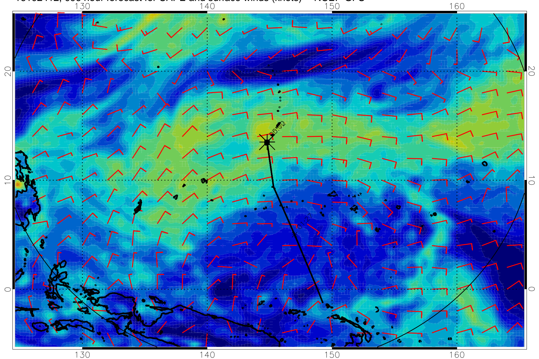
16102412, 096 hour forecast for CAPE and surface winds (knots) -- NCEP GFS
