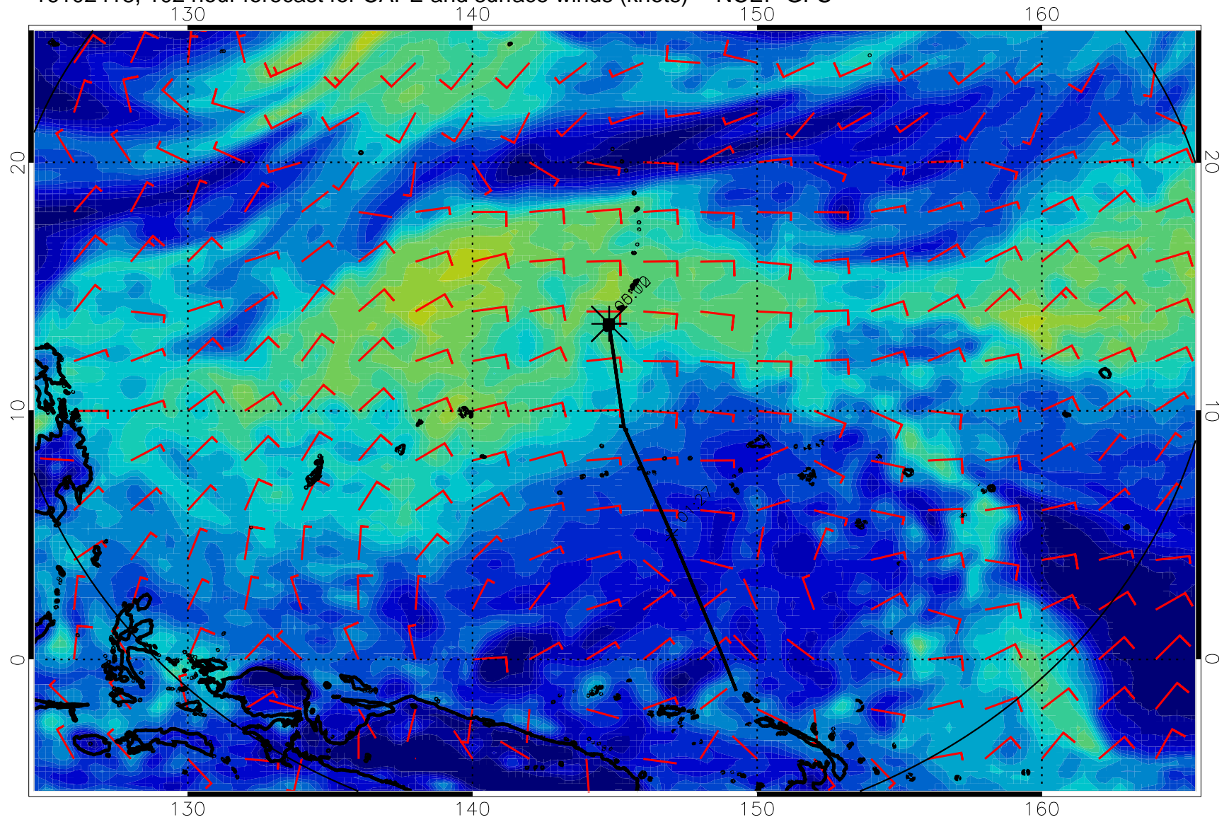
16102418, 102 hour forecast for CAPE and surface winds (knots) -- NCEP GFS
