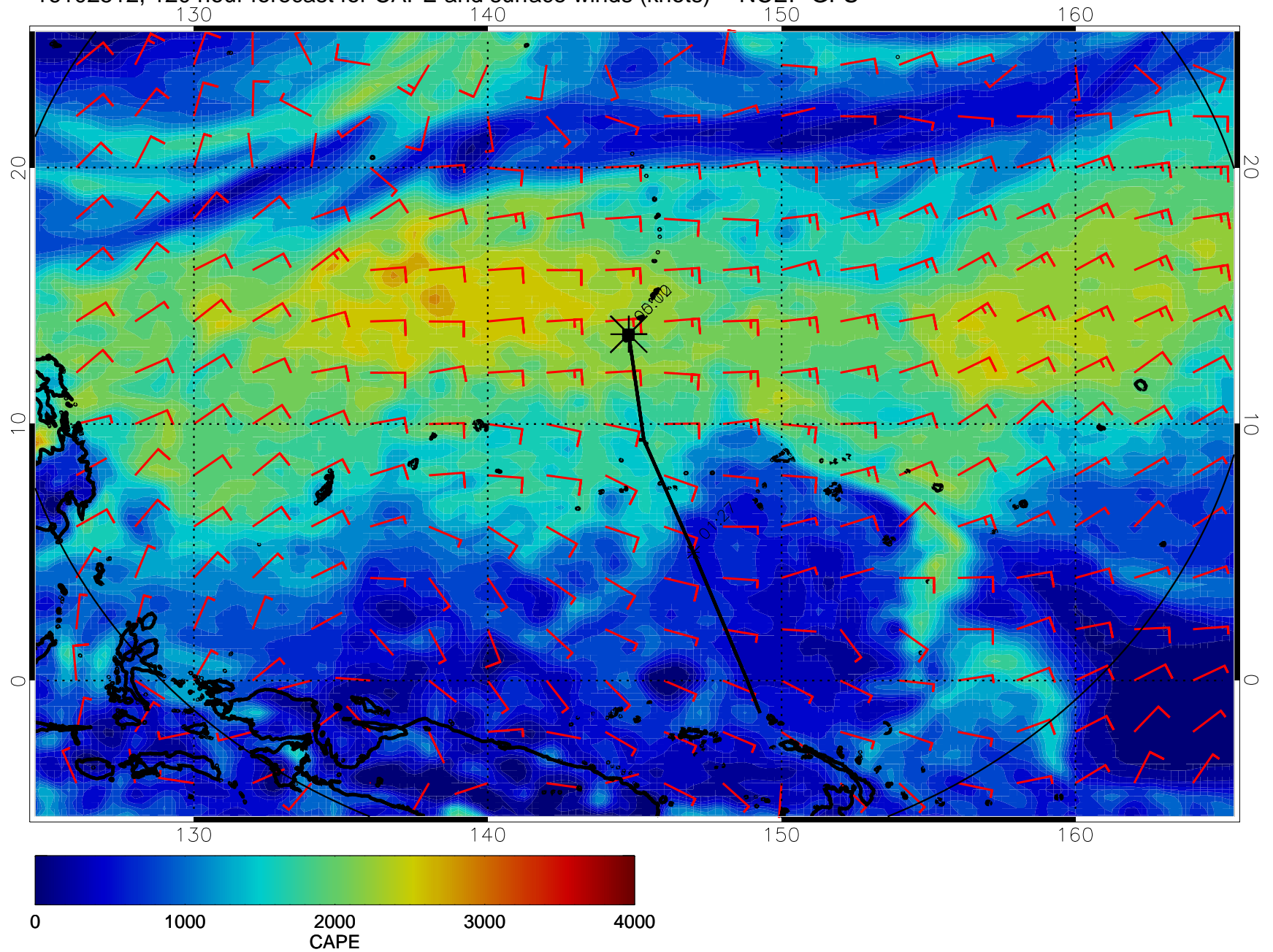
16102512, 120 hour forecast for CAPE and surface winds (knots) -- NCEP GFS
