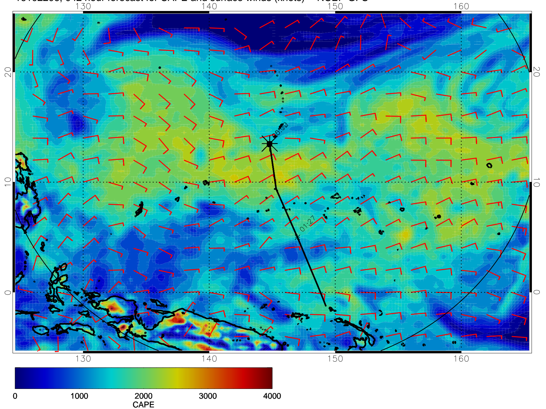
16102206, 042 hour forecast for CAPE and surface winds (knots) -- NCEP GFS
