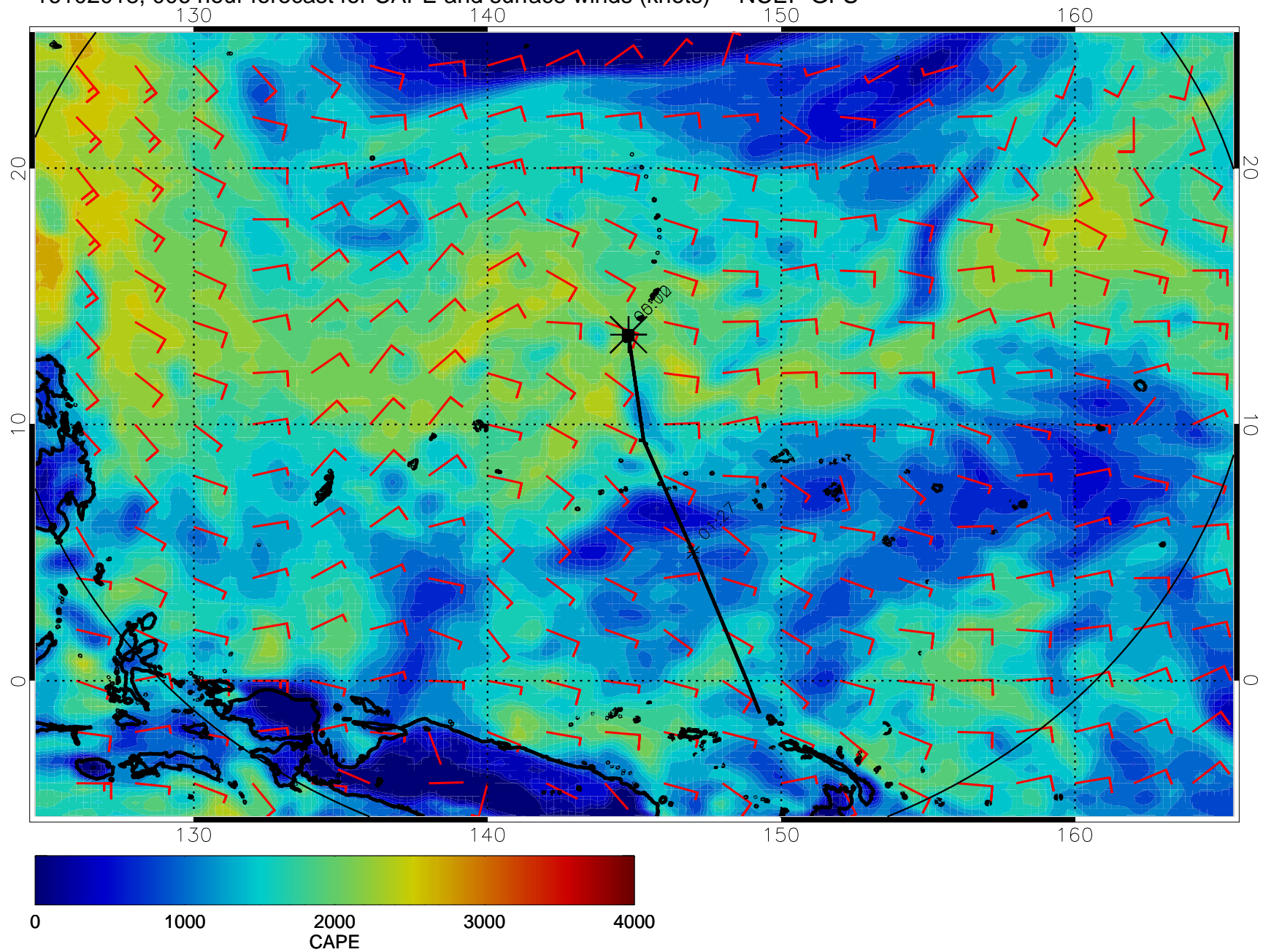
16102018, 006 hour forecast for CAPE and surface winds (knots) -- NCEP GFS
