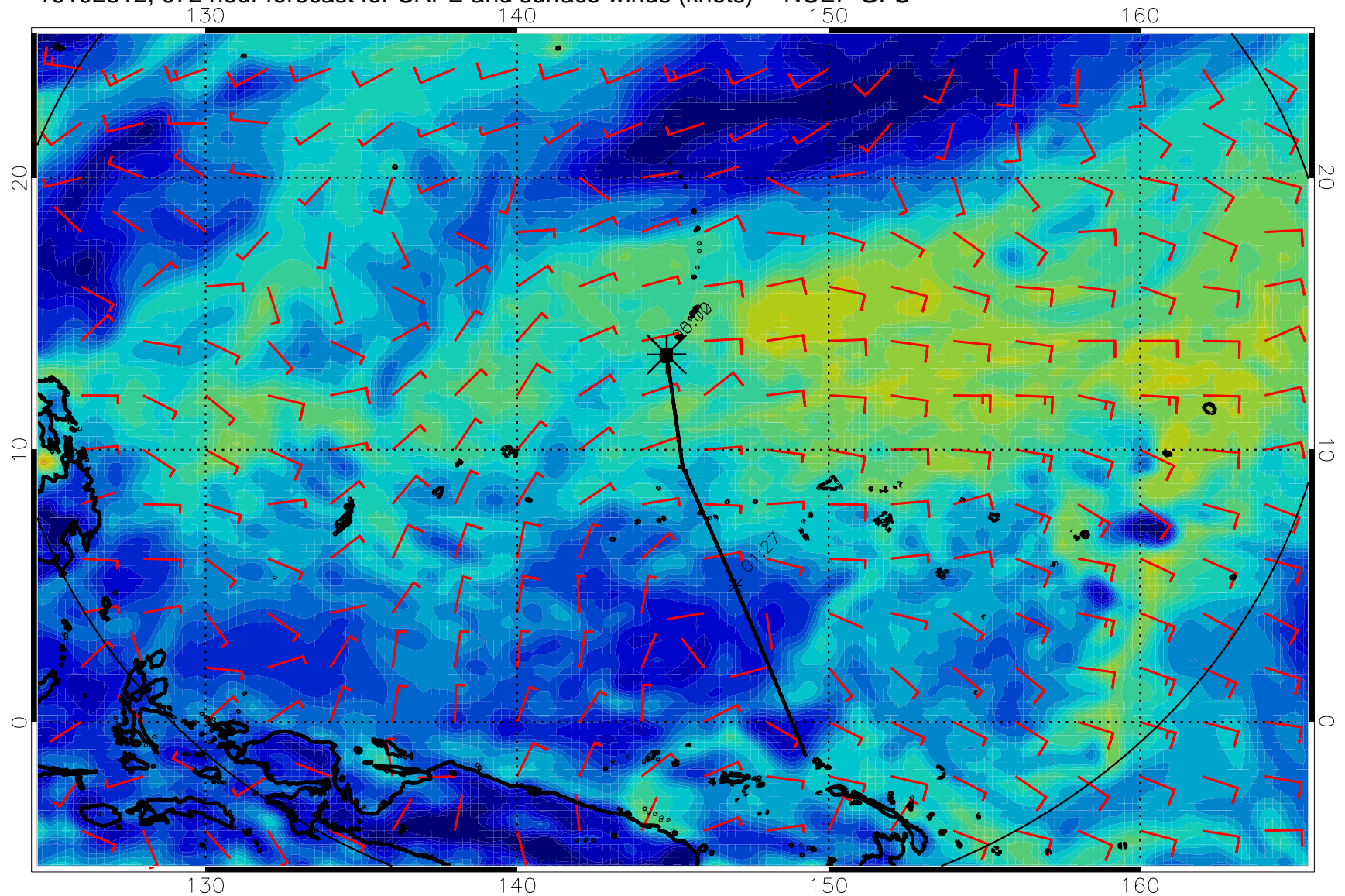
16102312, 072 hour forecast for CAPE and surface winds (knots) -- NCEP GFS
