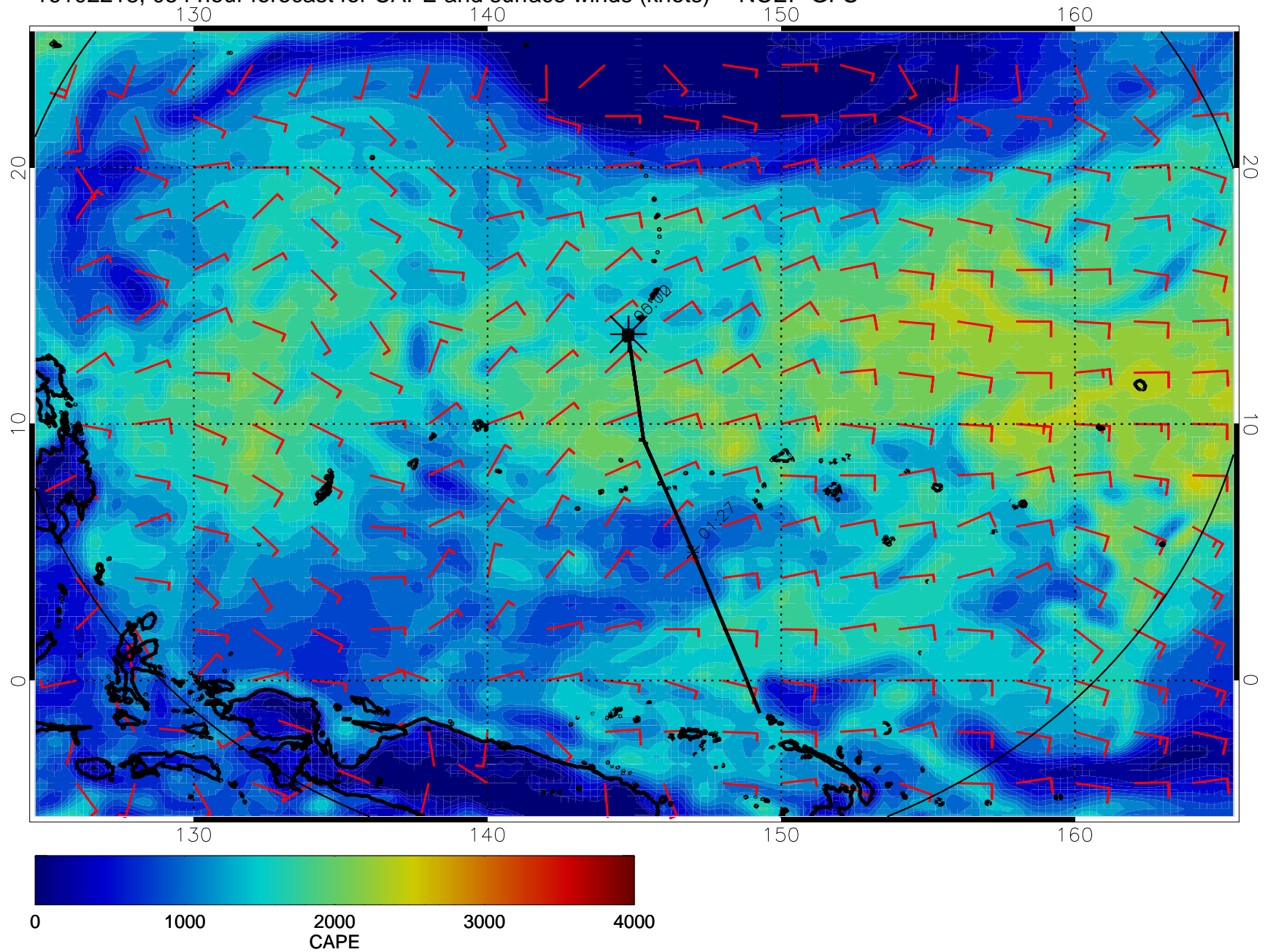
16102218, 054 hour forecast for CAPE and surface winds (knots) -- NCEP GFS
