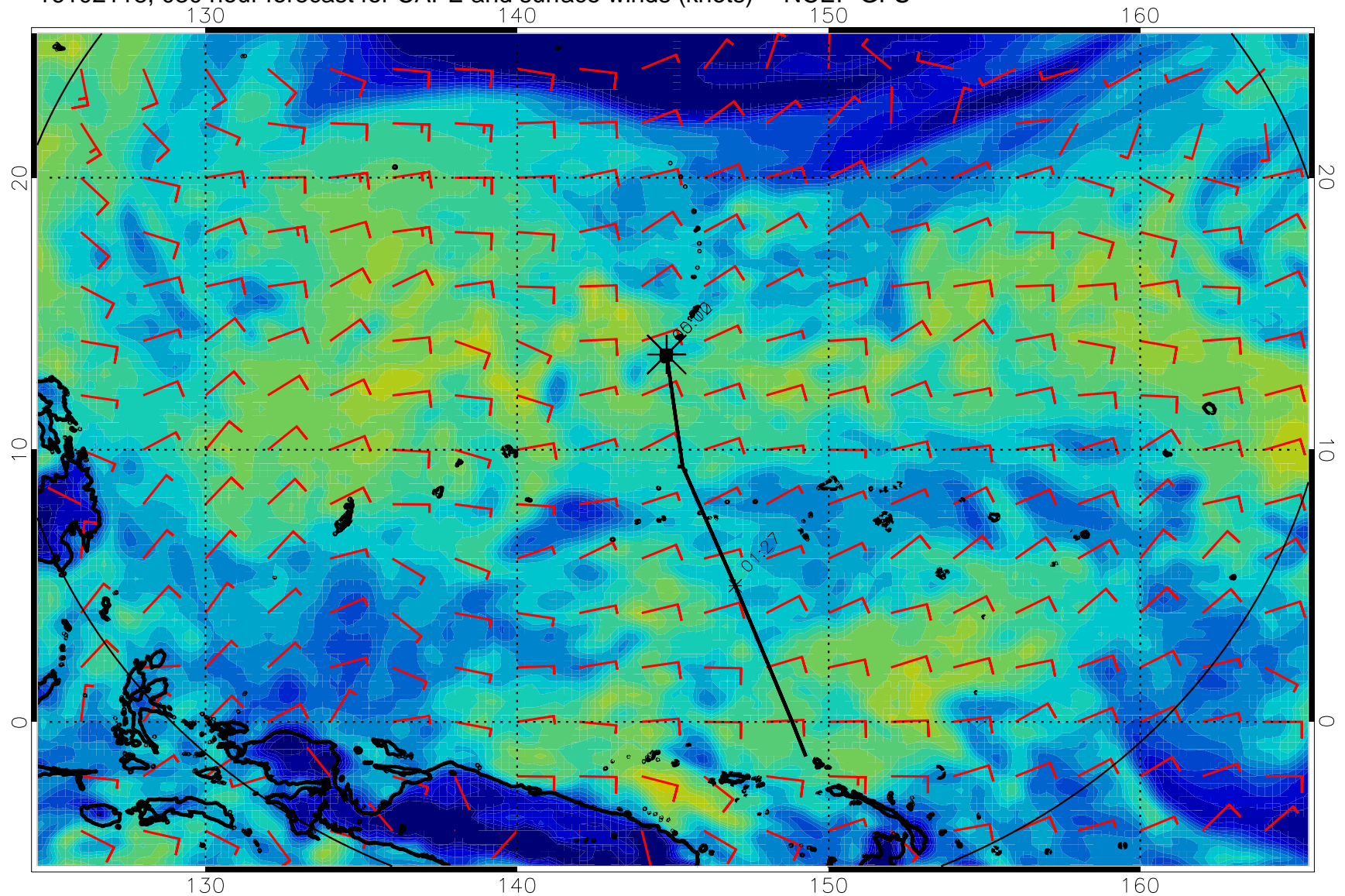
16102118, 030 hour forecast for CAPE and surface winds (knots) -- NCEP GFS
