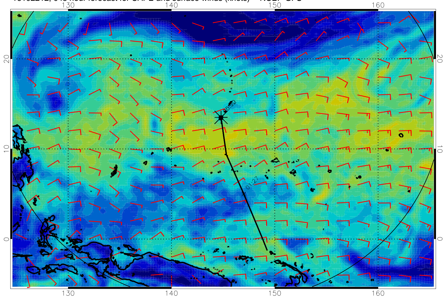
16102212, 048 hour forecast for CAPE and surface winds (knots) -- NCEP GFS
