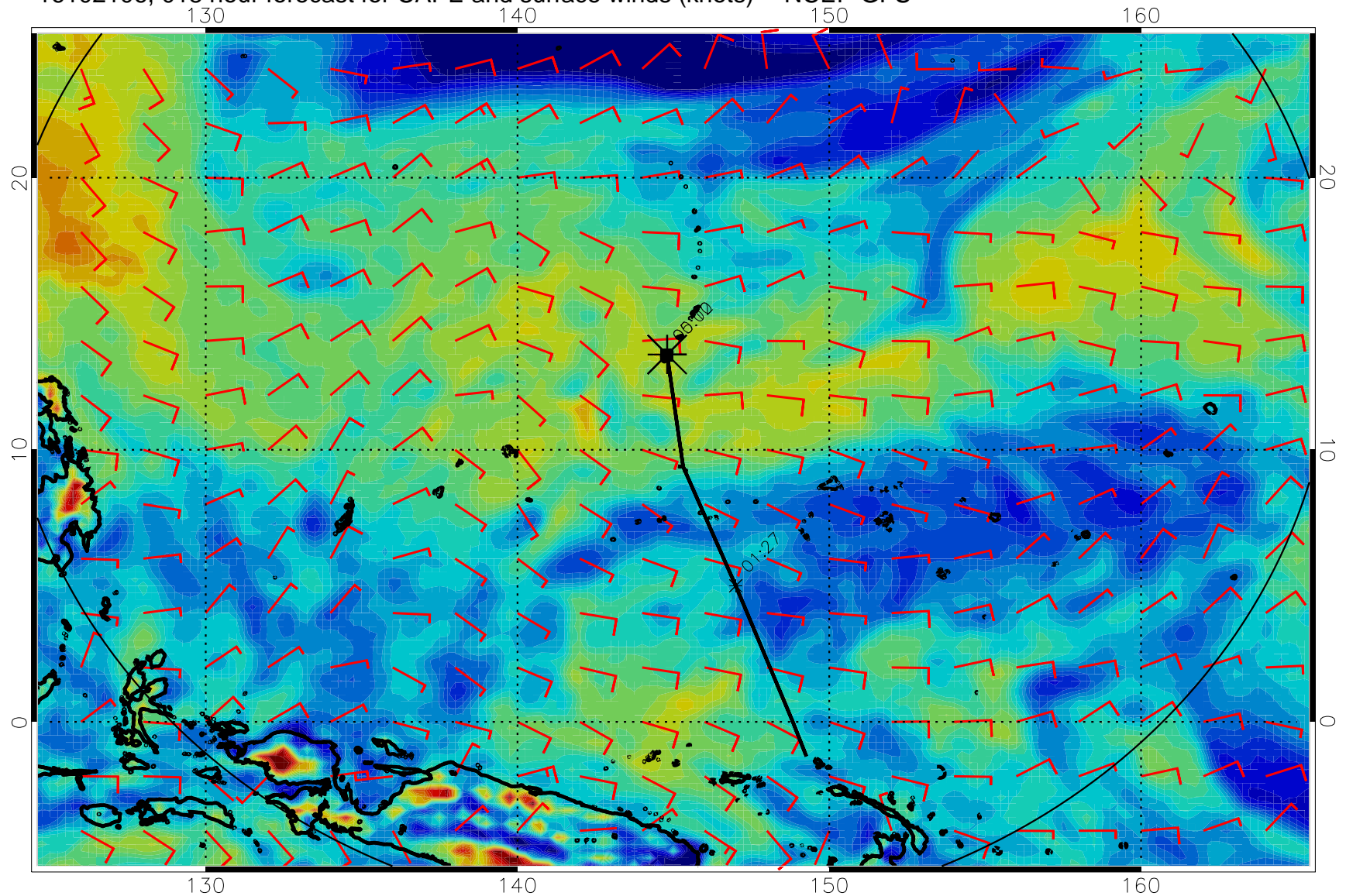
16102106, 018 hour forecast for CAPE and surface winds (knots) -- NCEP GFS
