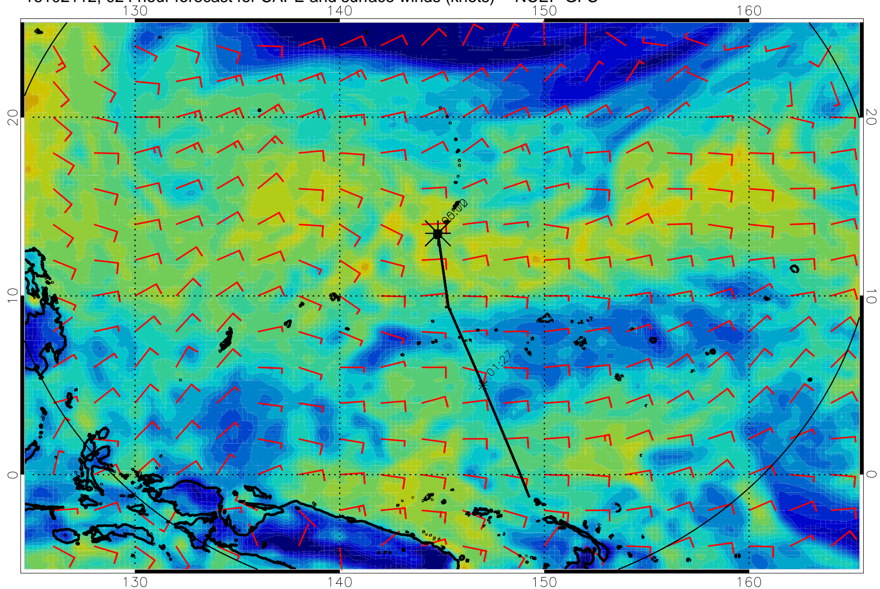
16102112, 024 hour forecast for CAPE and surface winds (knots) -- NCEP GFS
