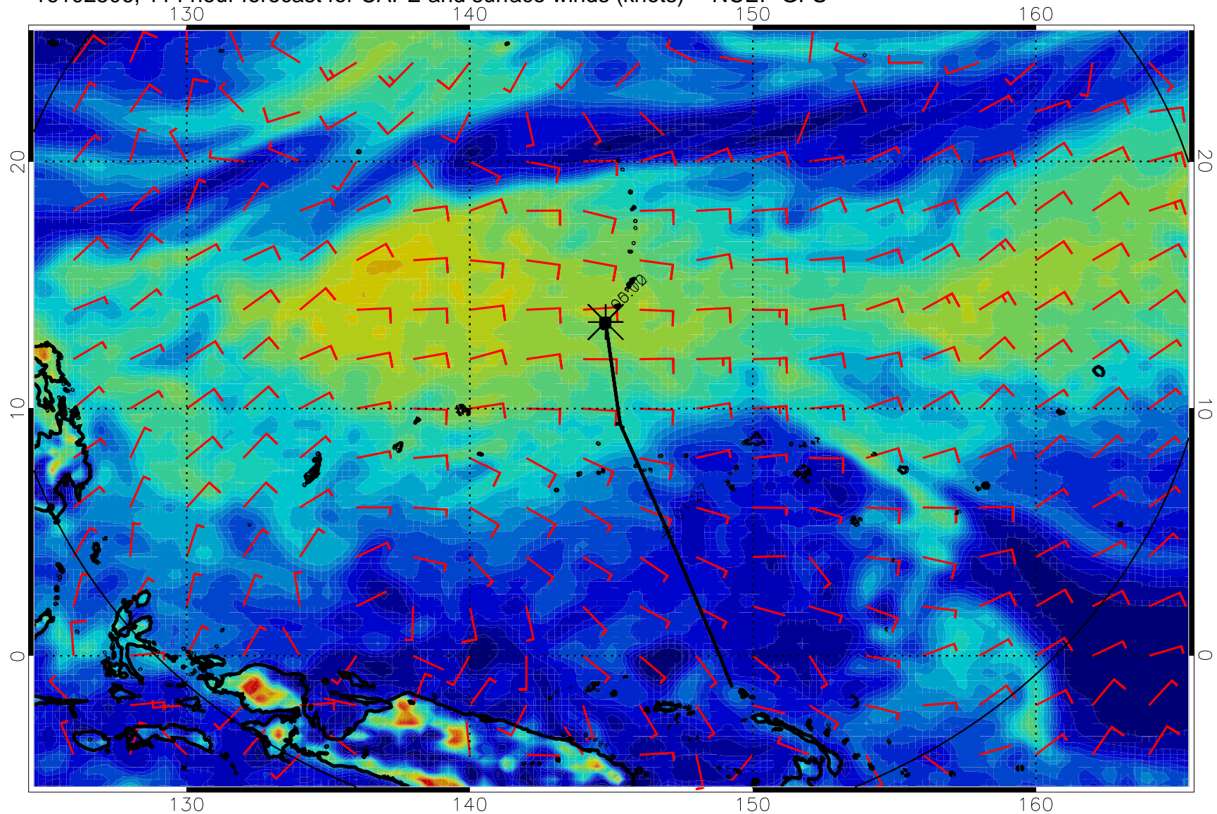
16102506, 114 hour forecast for CAPE and surface winds (knots) -- NCEP GFS
