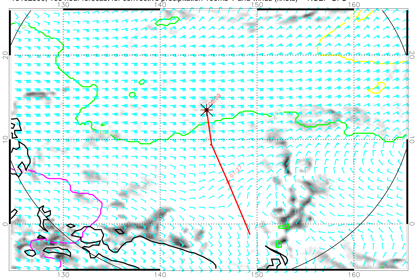
16102500, 108 hour forecast for convective precipitation 100mb T and winds (knots) -- NCEP GFS
