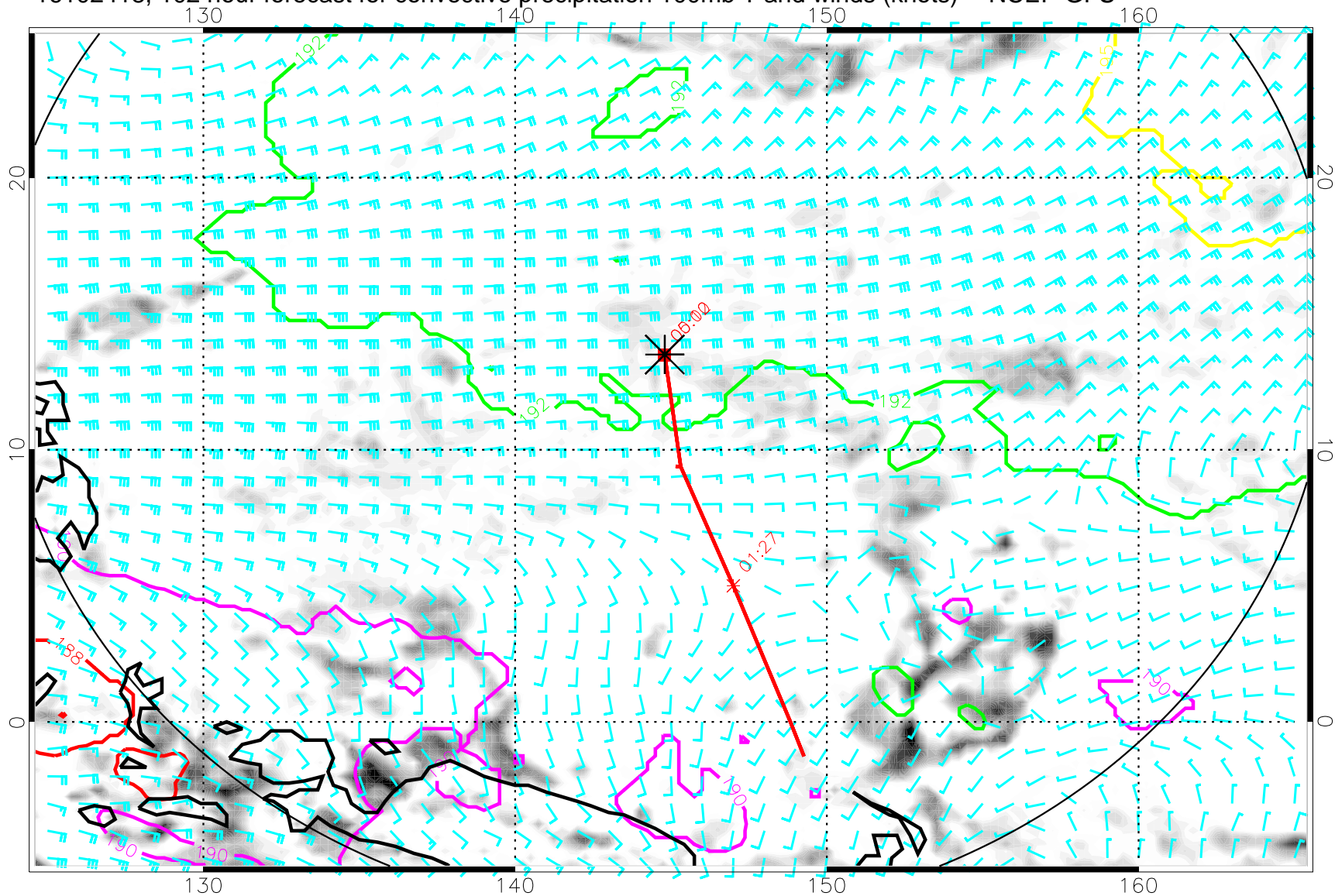
16102418, 102 hour forecast for convective precipitation 100mb T and winds (knots) -- NCEP GFS
