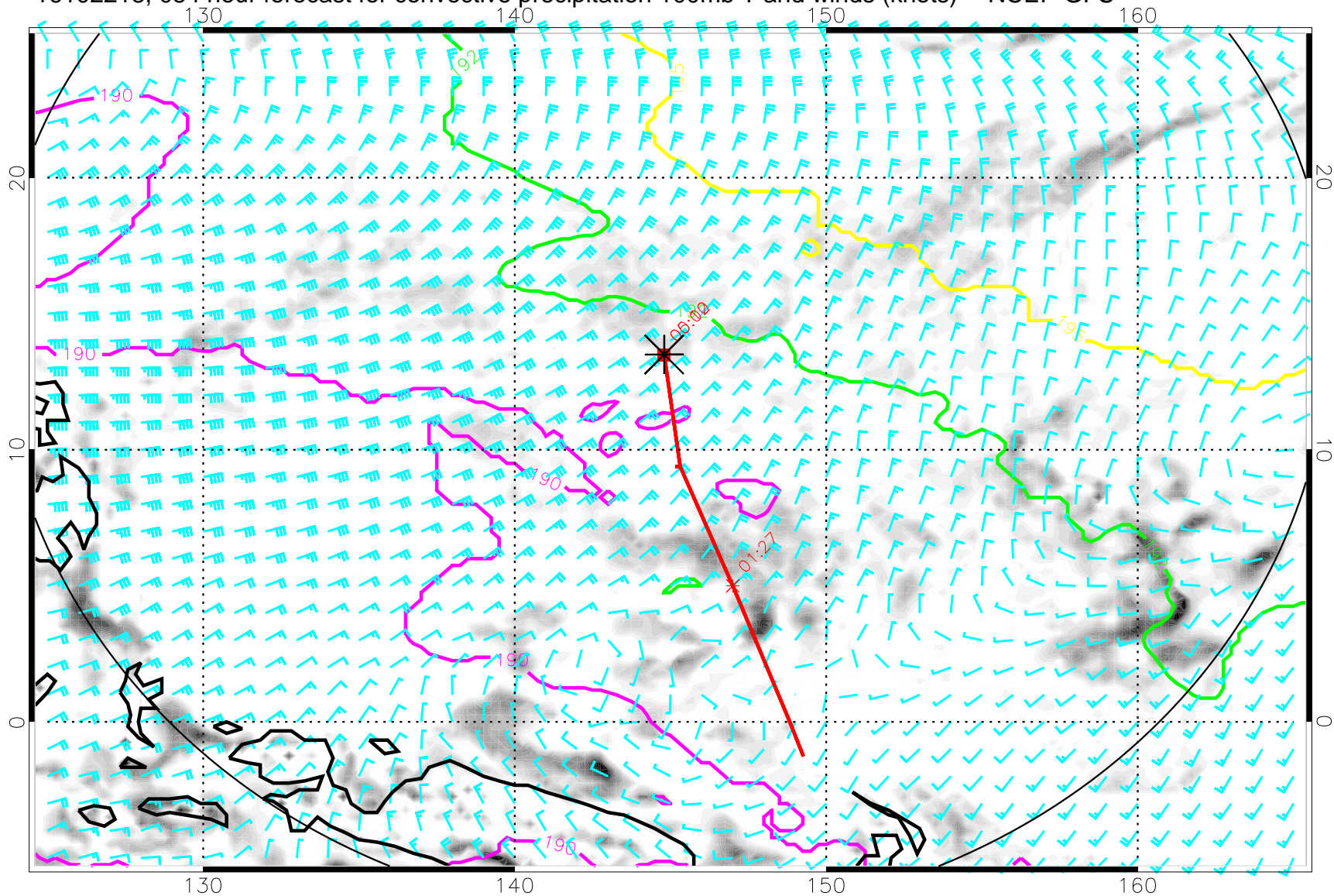
16102218, 054 hour forecast for convective precipitation 100mb T and winds (knots) -- NCEP GFS
