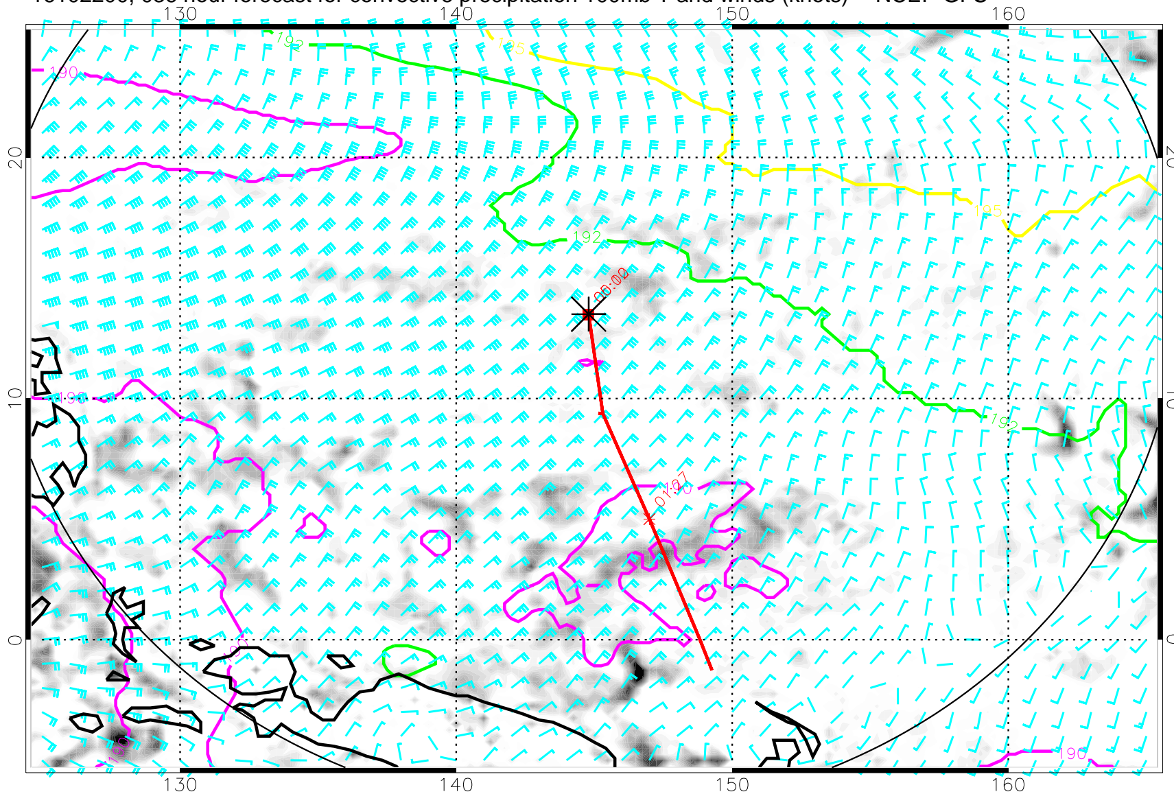
16102200, 036 hour forecast for convective precipitation 100mb T and winds (knots) -- NCEP GFS
