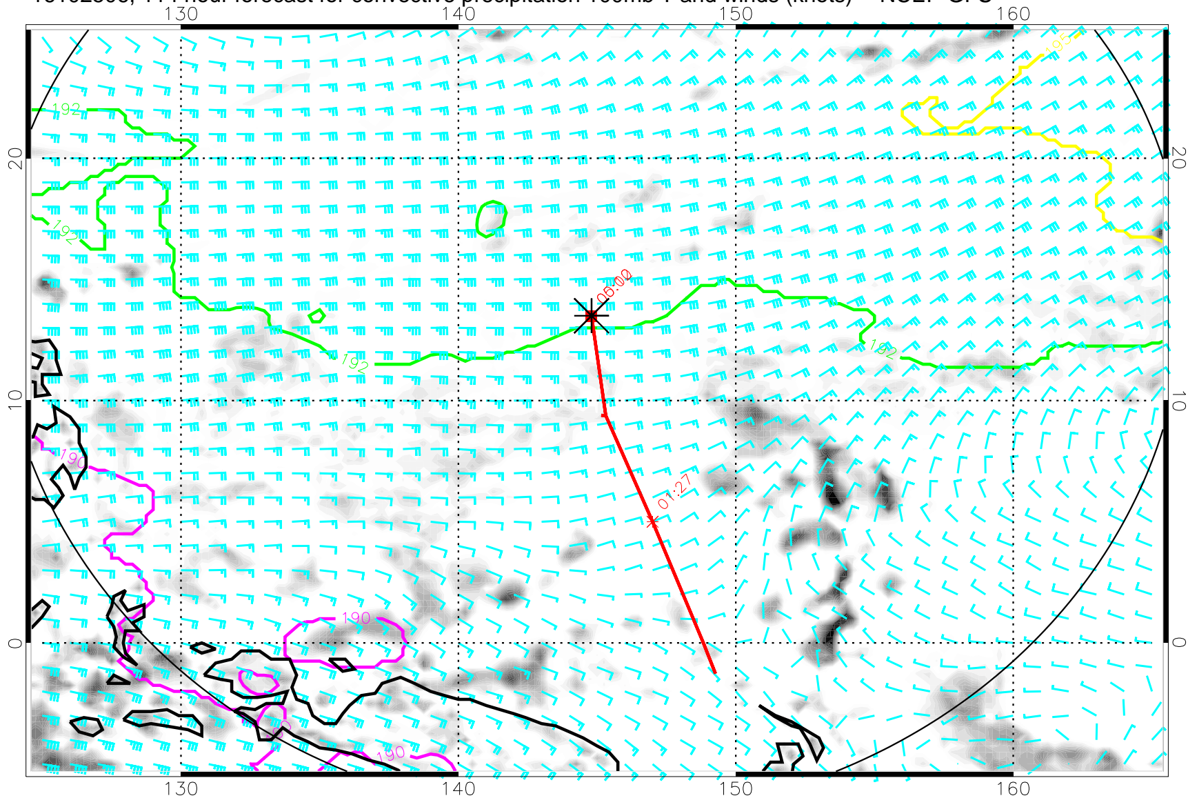
16102506, 114 hour forecast for convective precipitation 100mb T and winds (knots) -- NCEP GFS
