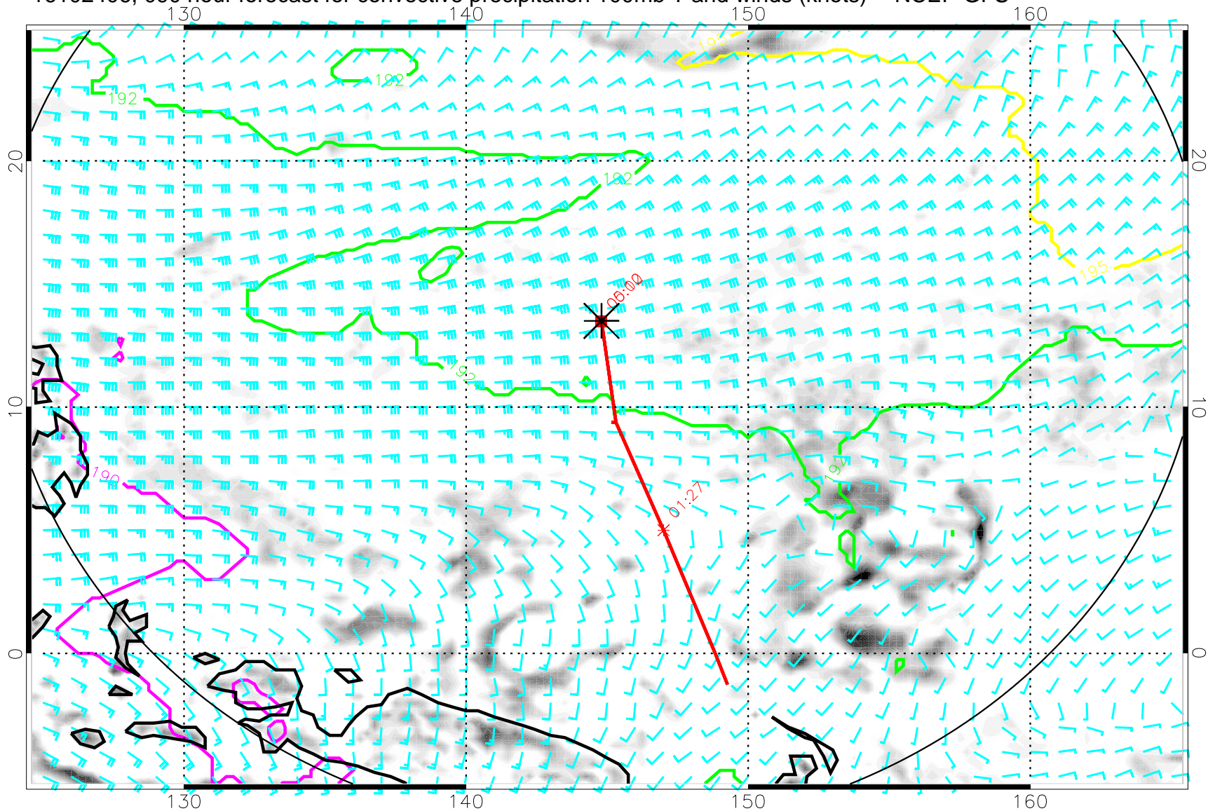
16102406, 090 hour forecast for convective precipitation 100mb T and winds (knots) -- NCEP GFS
