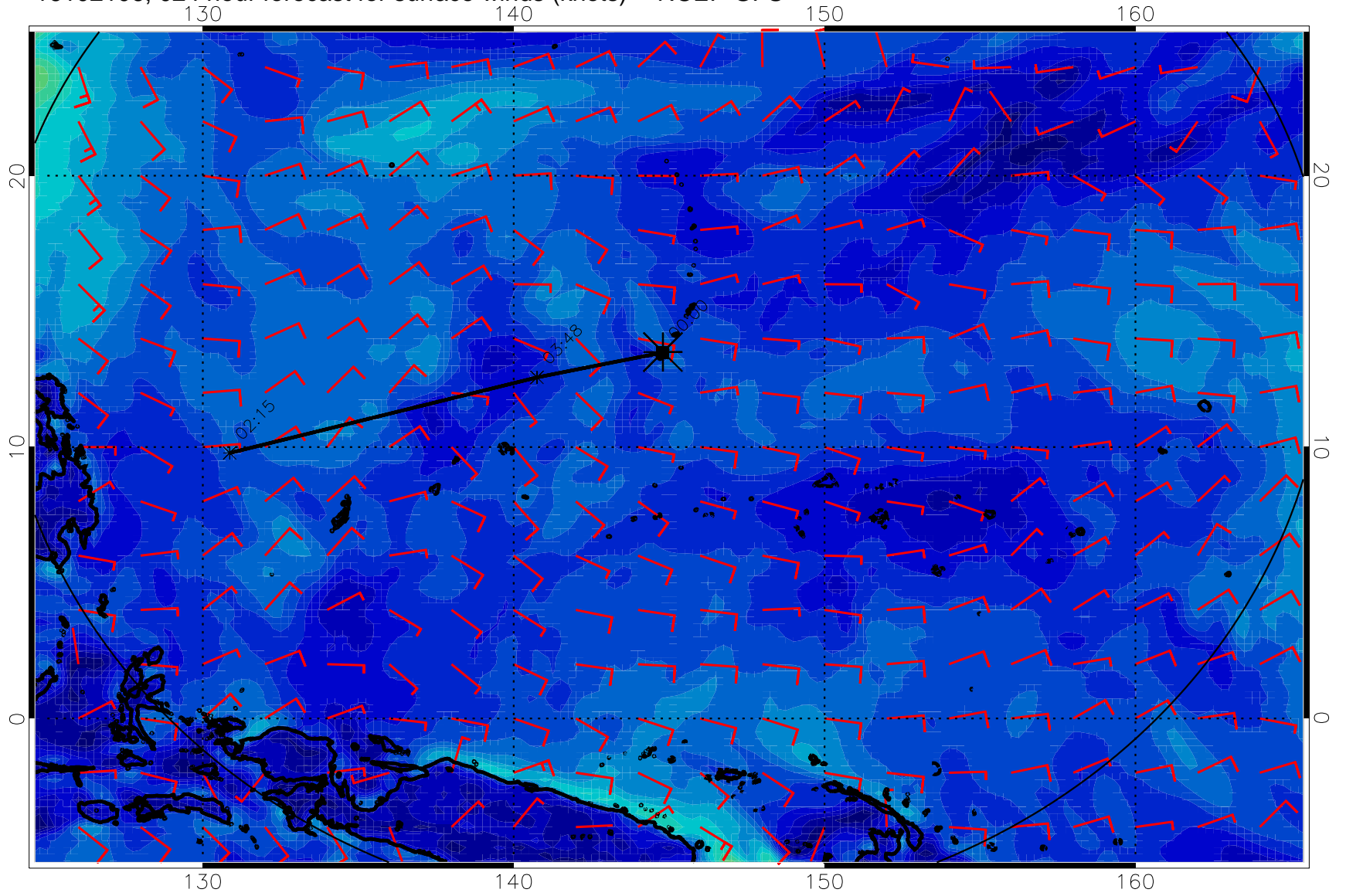
16102106, 024 hour forecast for surface winds (knots) -- NCEP GFS
