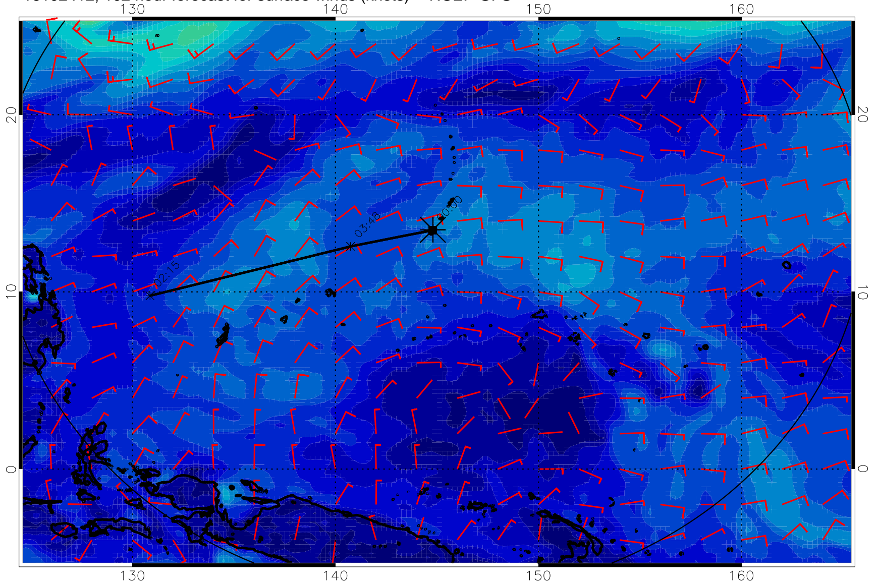
16102412, 102 hour forecast for surface winds (knots) -- NCEP GFS
