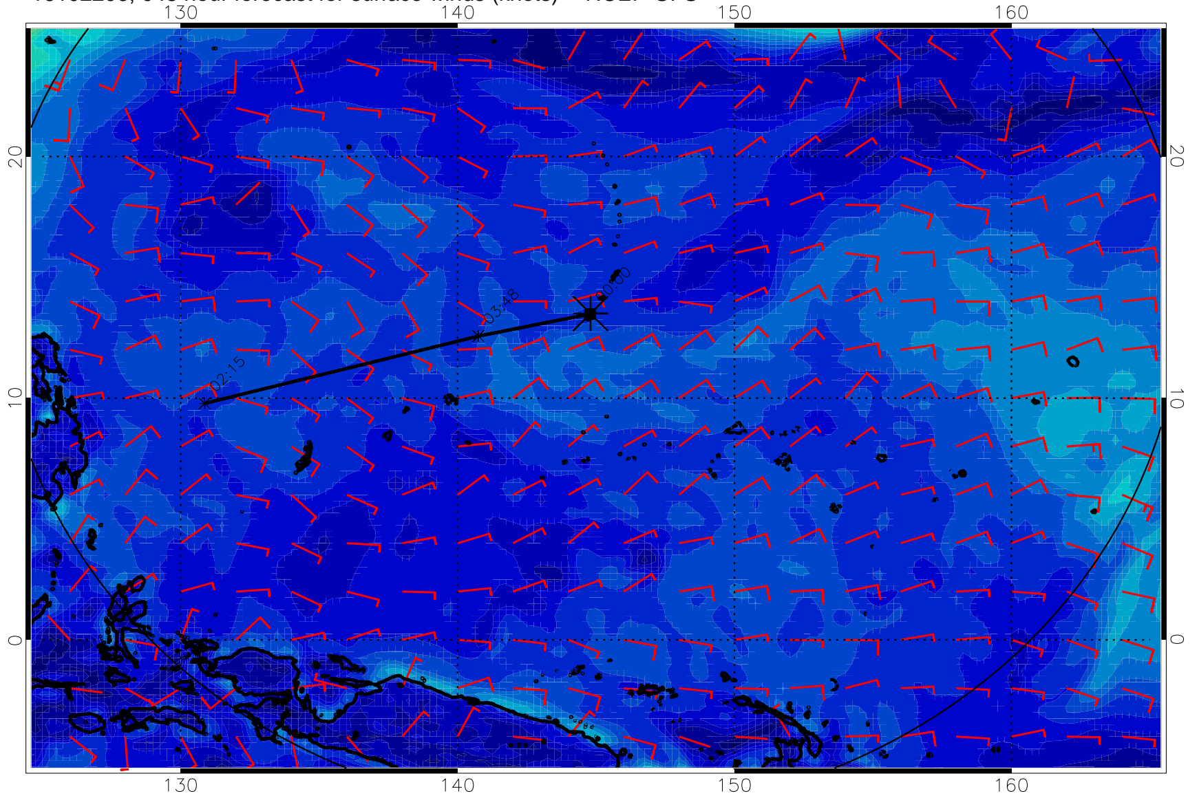
16102206, 048 hour forecast for surface winds (knots) -- NCEP GFS
