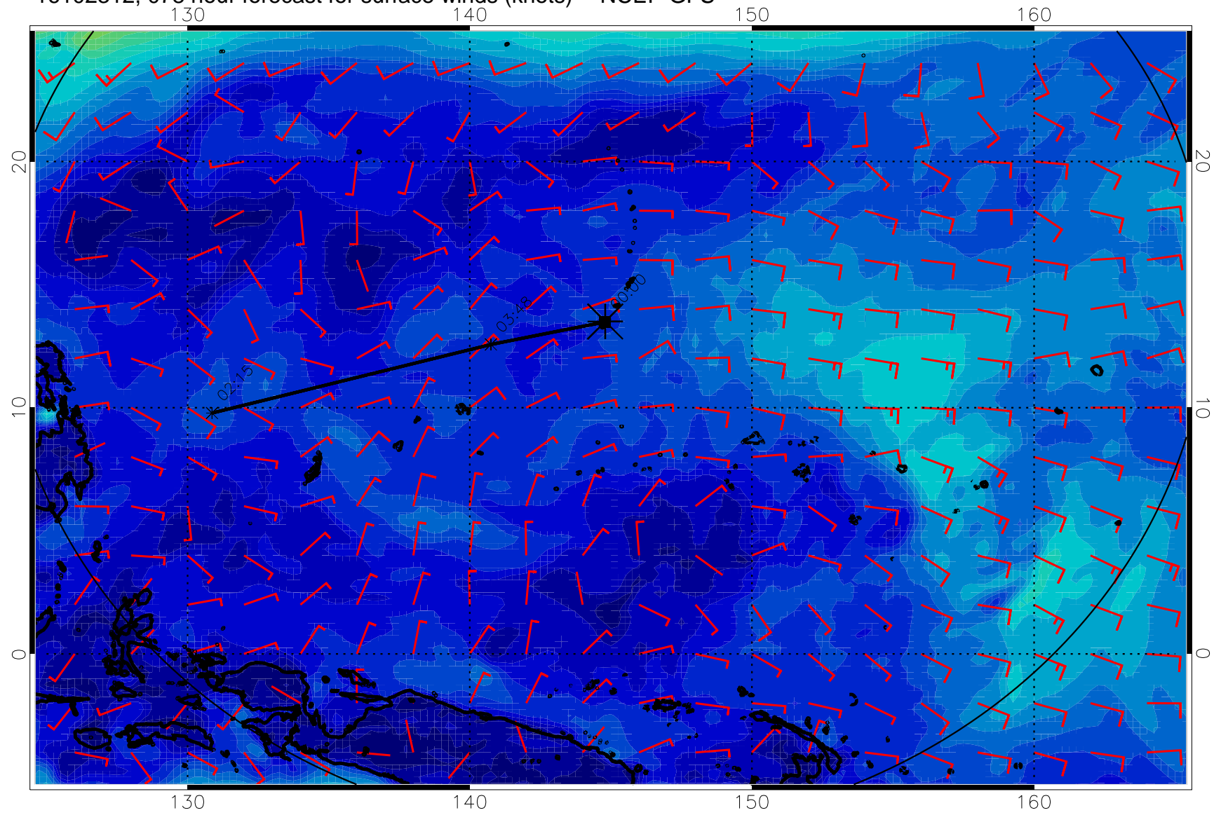
16102312, 078 hour forecast for surface winds (knots) -- NCEP GFS
