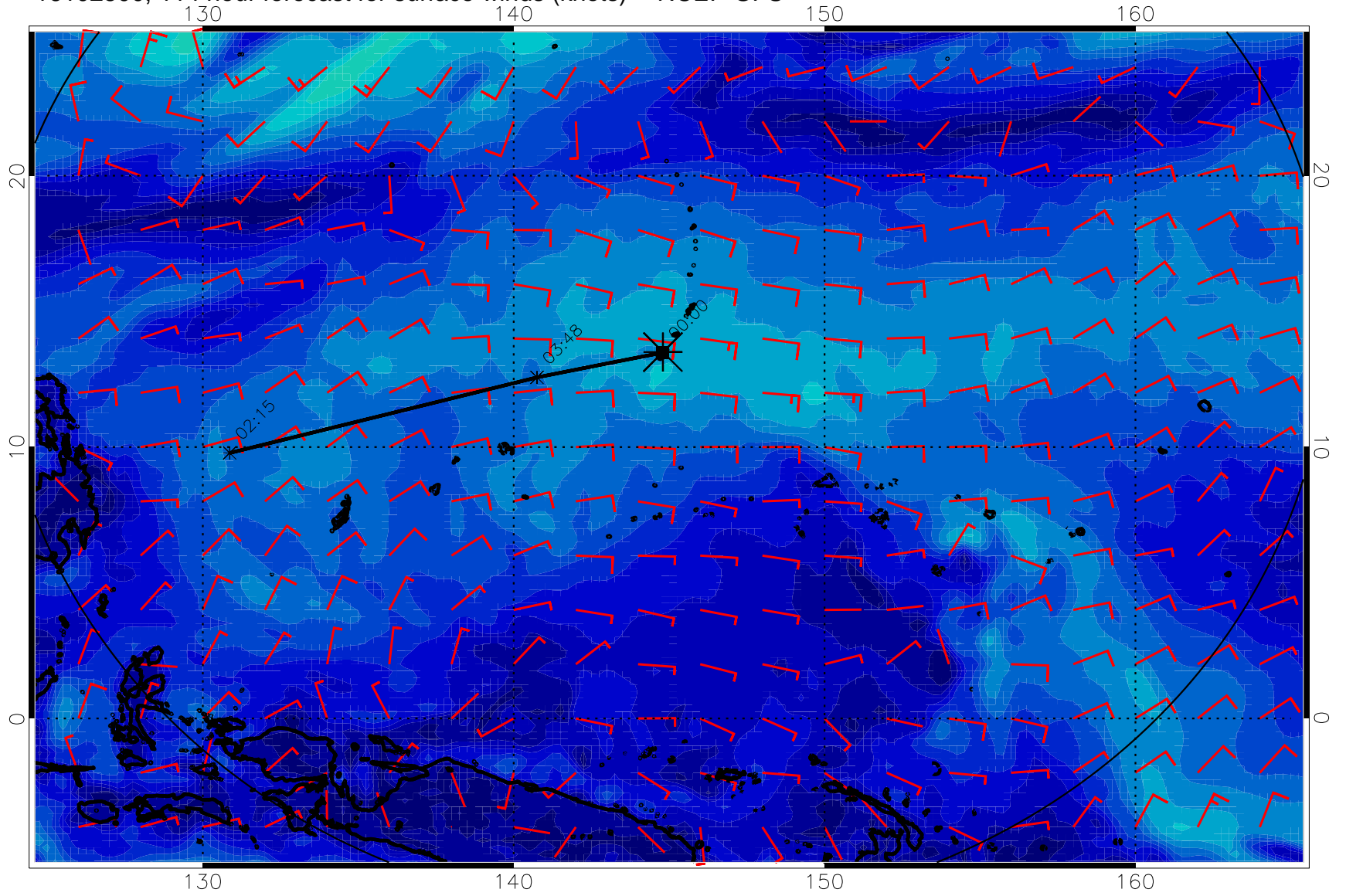
16102500, 114 hour forecast for surface winds (knots) -- NCEP GFS
