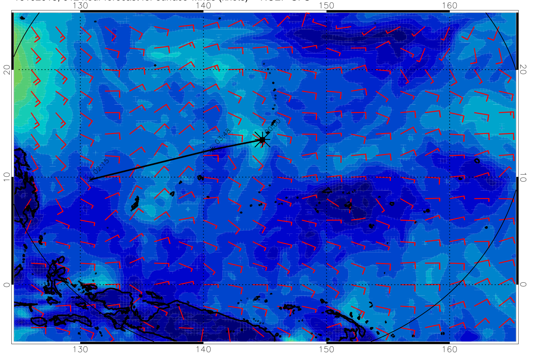
16102018, 012 hour forecast for surface winds (knots) -- NCEP GFS
