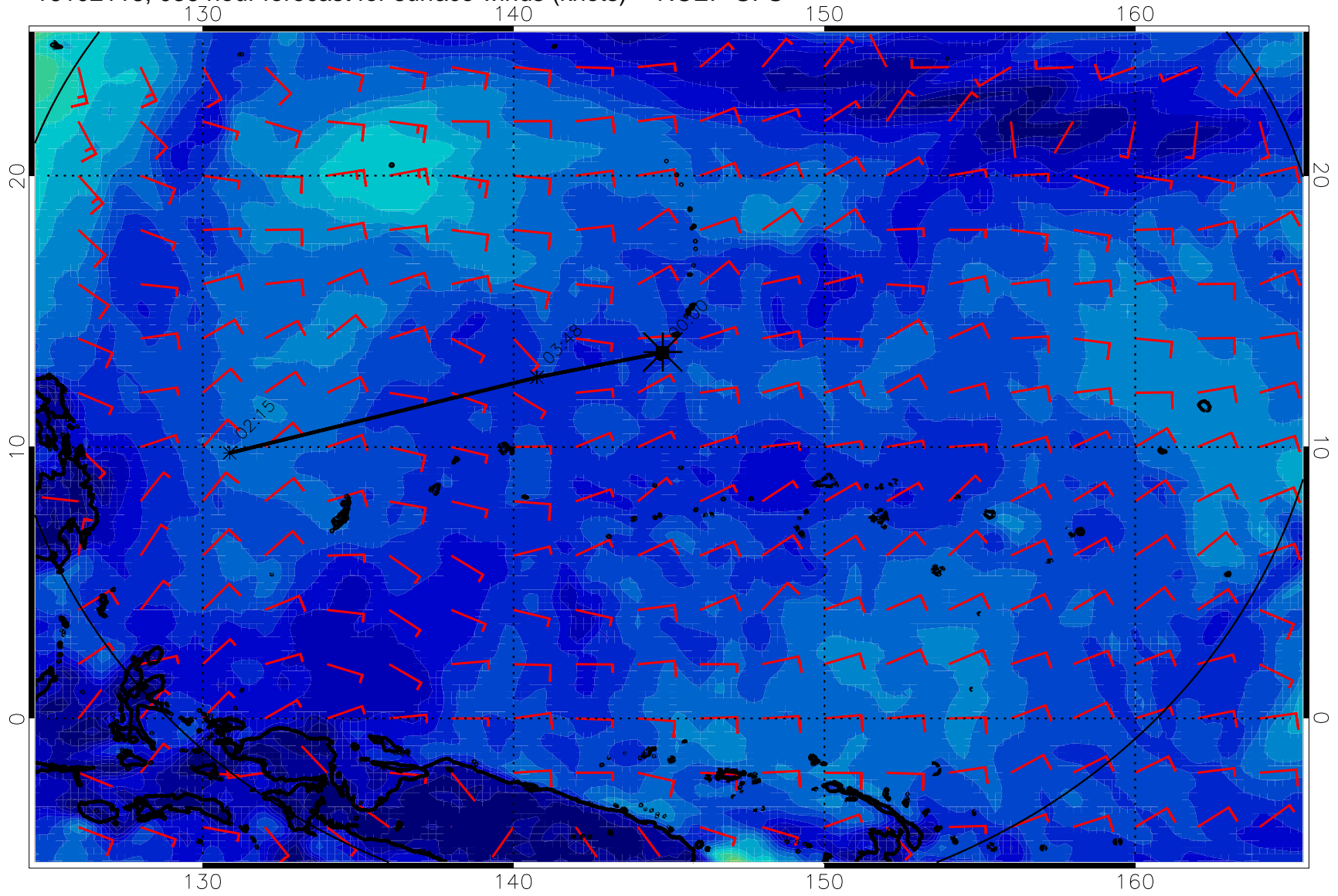
16102118, 036 hour forecast for surface winds (knots) -- NCEP GFS
