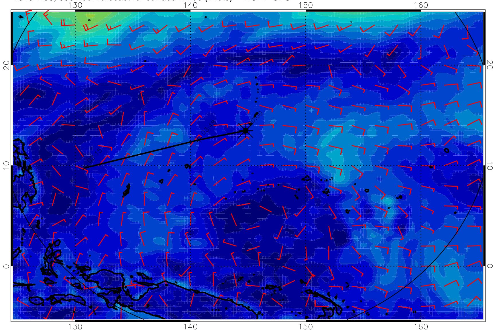
16102406, 096 hour forecast for surface winds (knots) -- NCEP GFS
