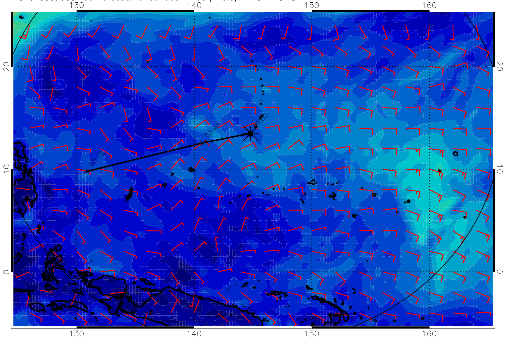
16102300, 066 hour forecast for surface winds (knots) -- NCEP GFS
