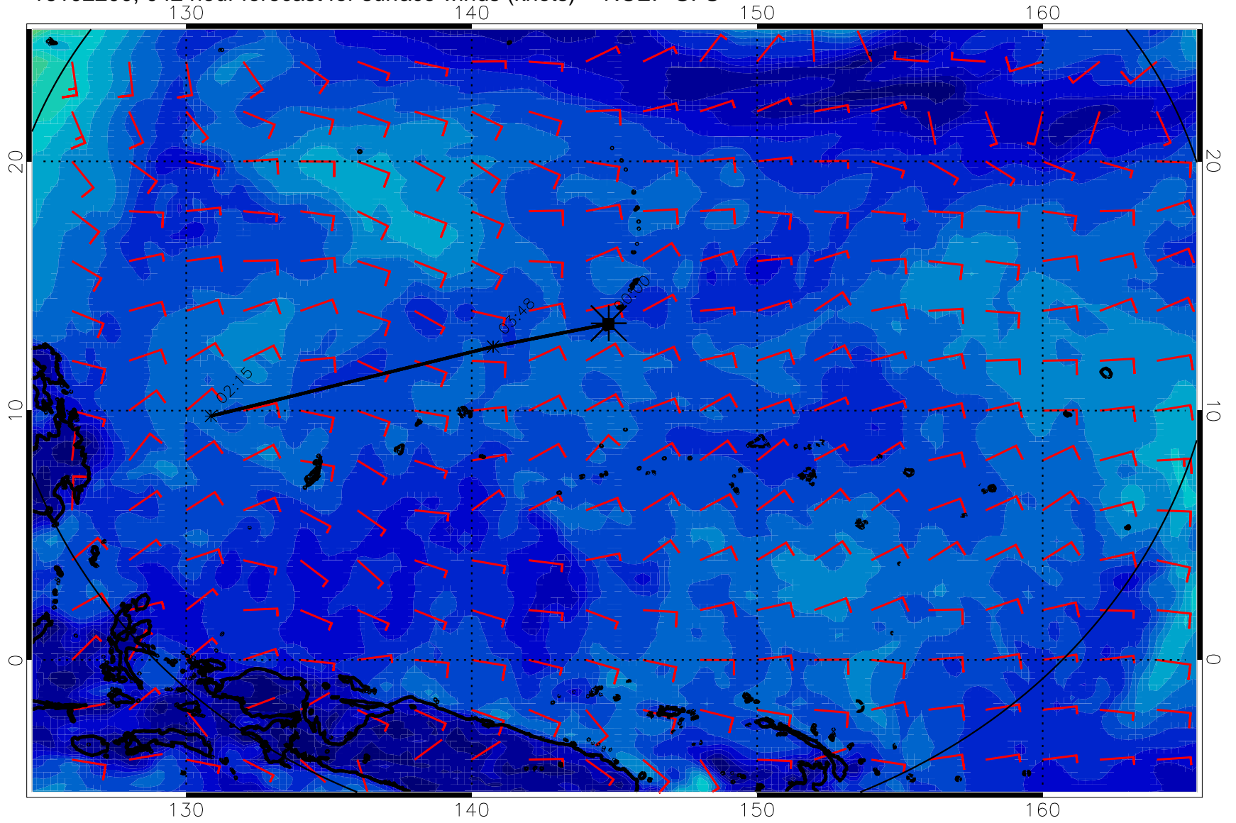
16102200, 042 hour forecast for surface winds (knots) -- NCEP GFS
