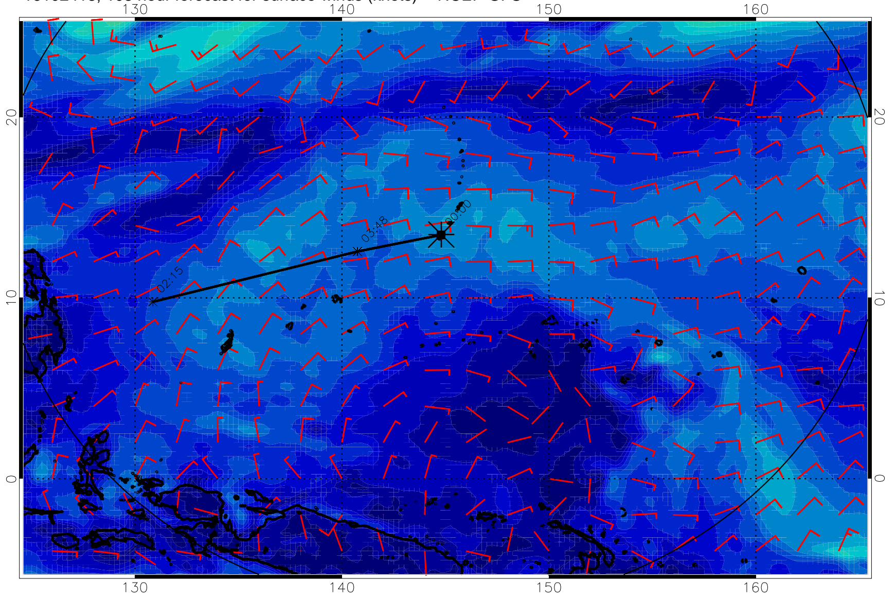
16102418, 108 hour forecast for surface winds (knots) -- NCEP GFS
