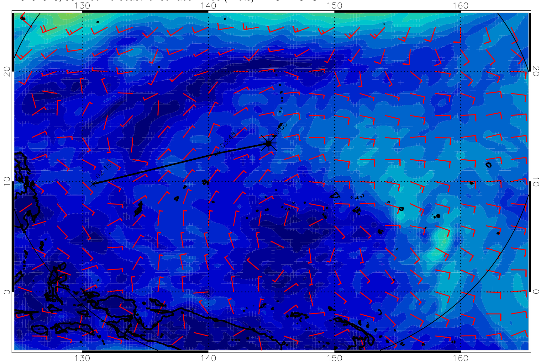
16102318, 084 hour forecast for surface winds (knots) -- NCEP GFS
