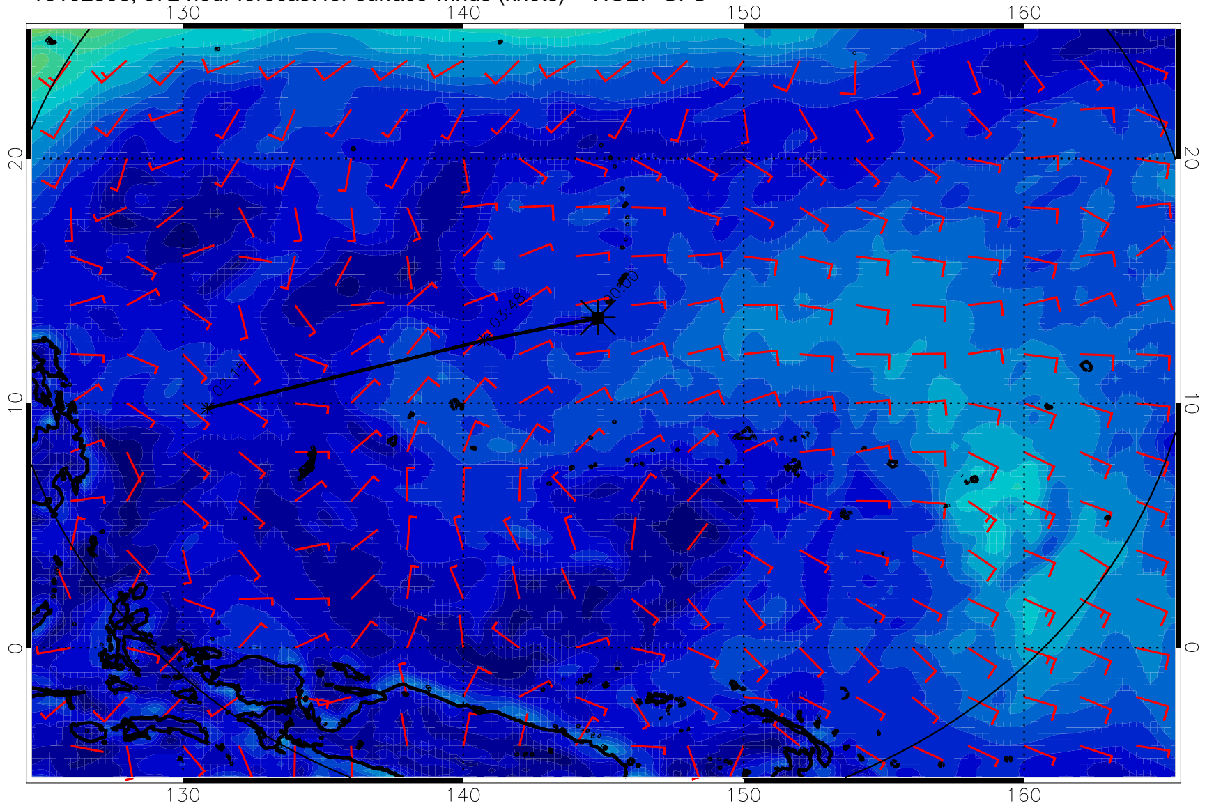
16102306, 072 hour forecast for surface winds (knots) -- NCEP GFS
