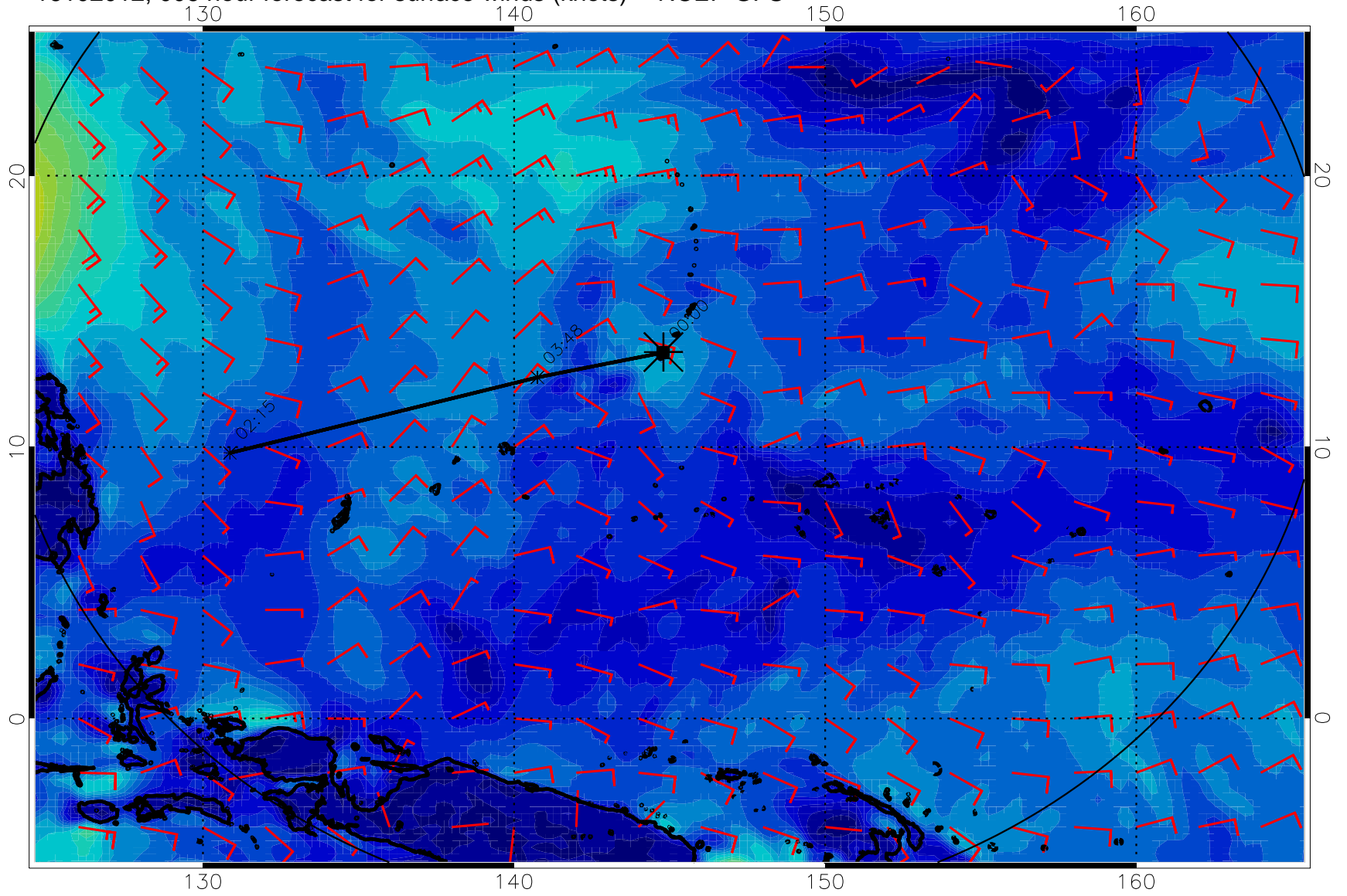
16102012, 006 hour forecast for surface winds (knots) -- NCEP GFS
