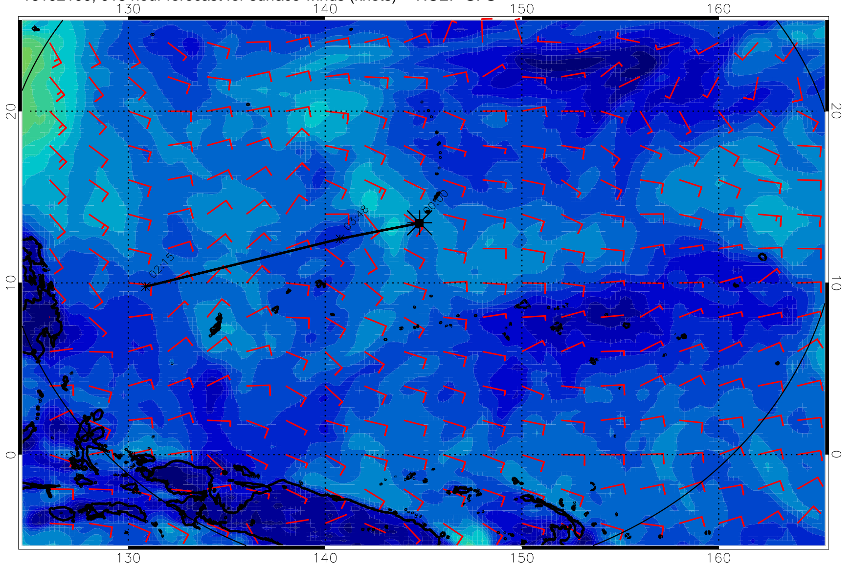
16102100, 018 hour forecast for surface winds (knots) -- NCEP GFS
