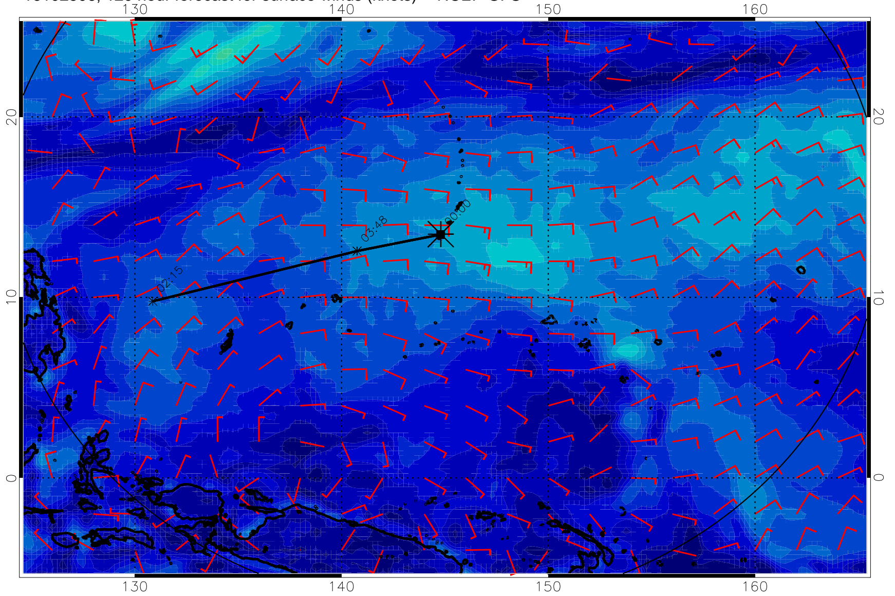
16102506, 120 hour forecast for surface winds (knots) -- NCEP GFS
