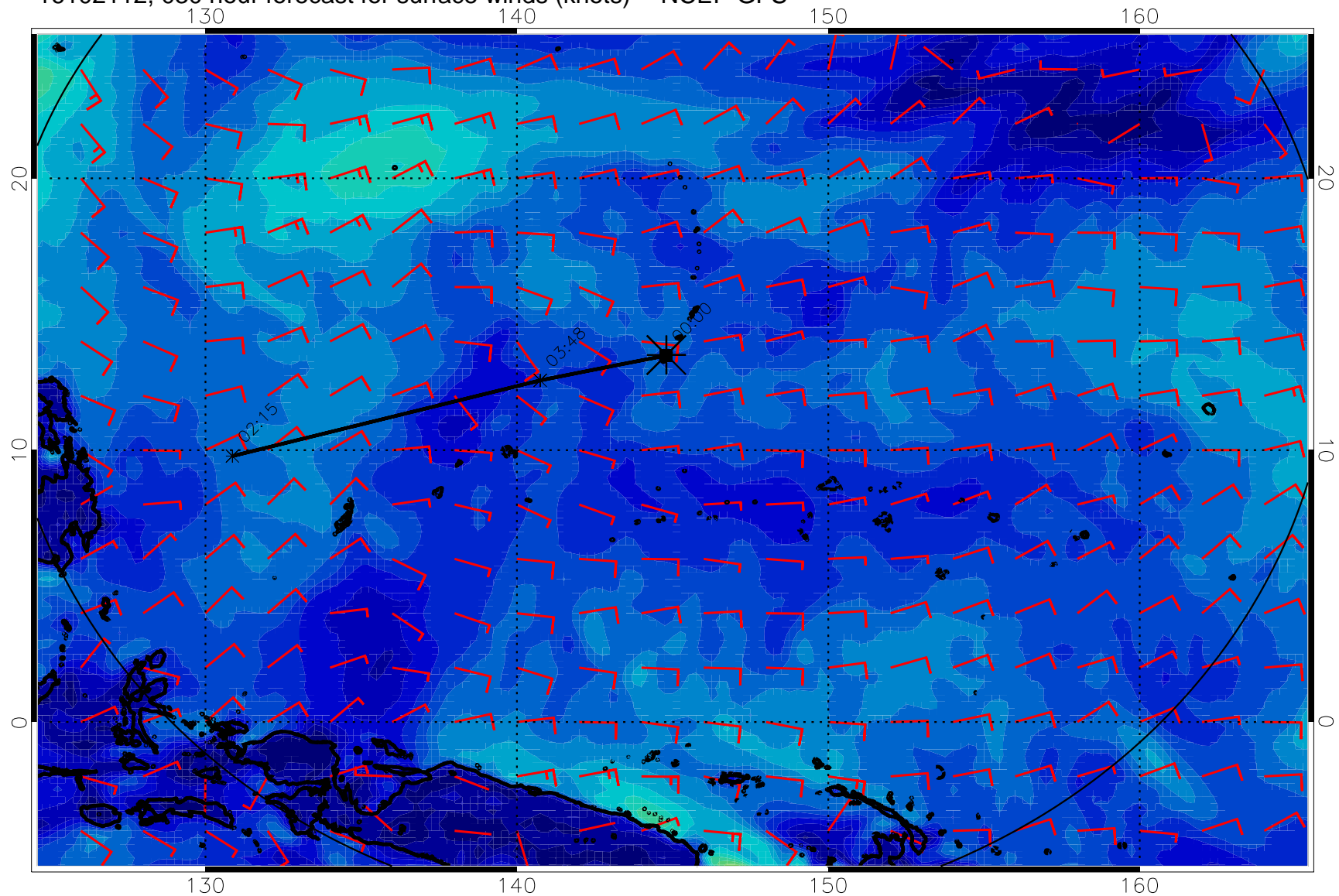
16102112, 030 hour forecast for surface winds (knots) -- NCEP GFS
