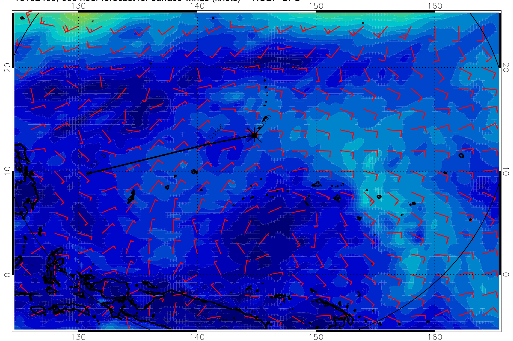
16102400, 090 hour forecast for surface winds (knots) -- NCEP GFS
