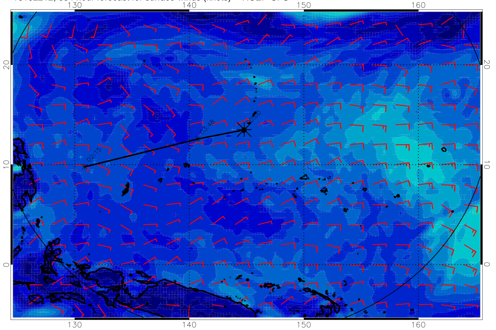
16102212, 054 hour forecast for surface winds (knots) -- NCEP GFS
