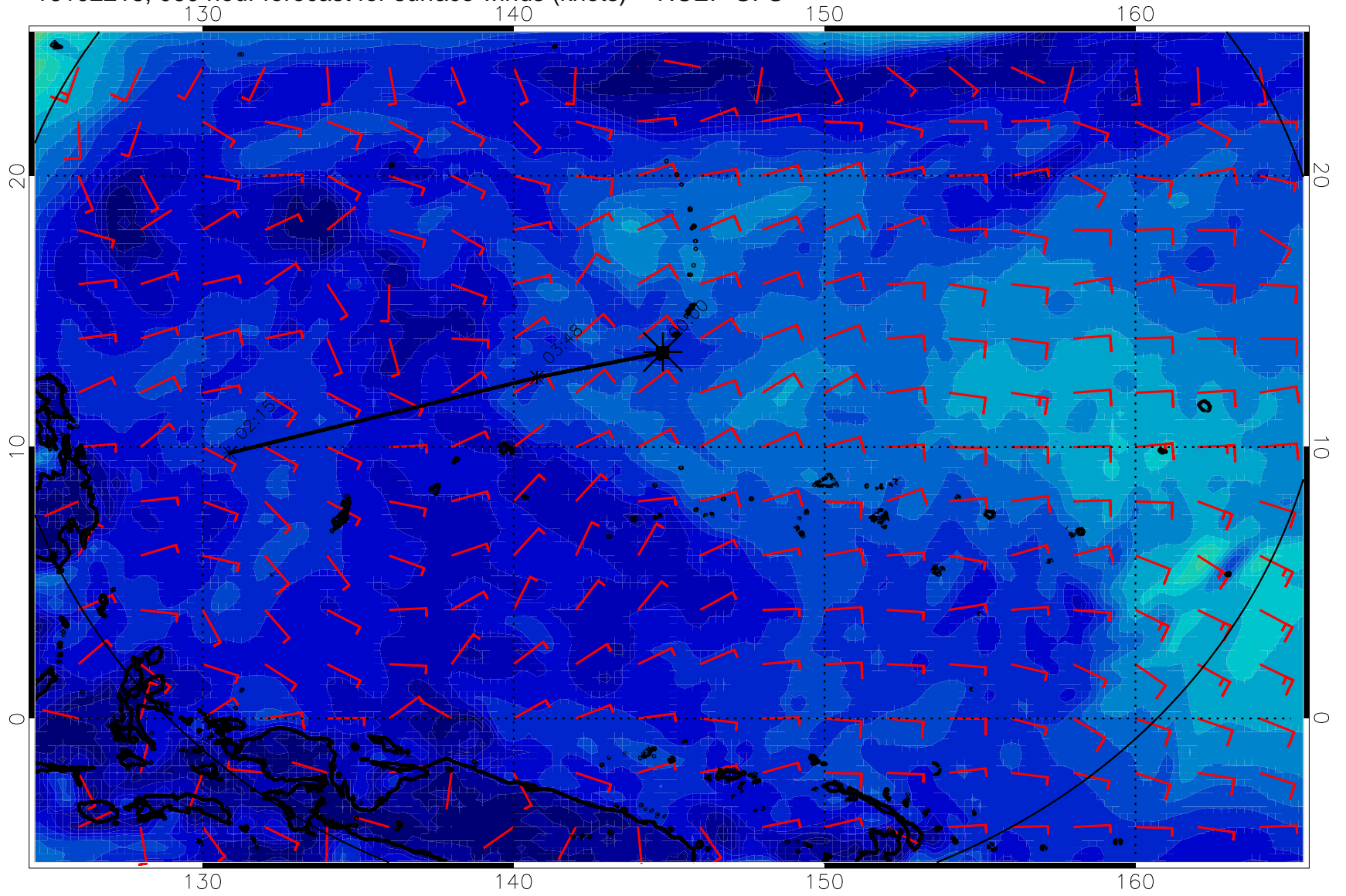
16102218, 060 hour forecast for surface winds (knots) -- NCEP GFS
