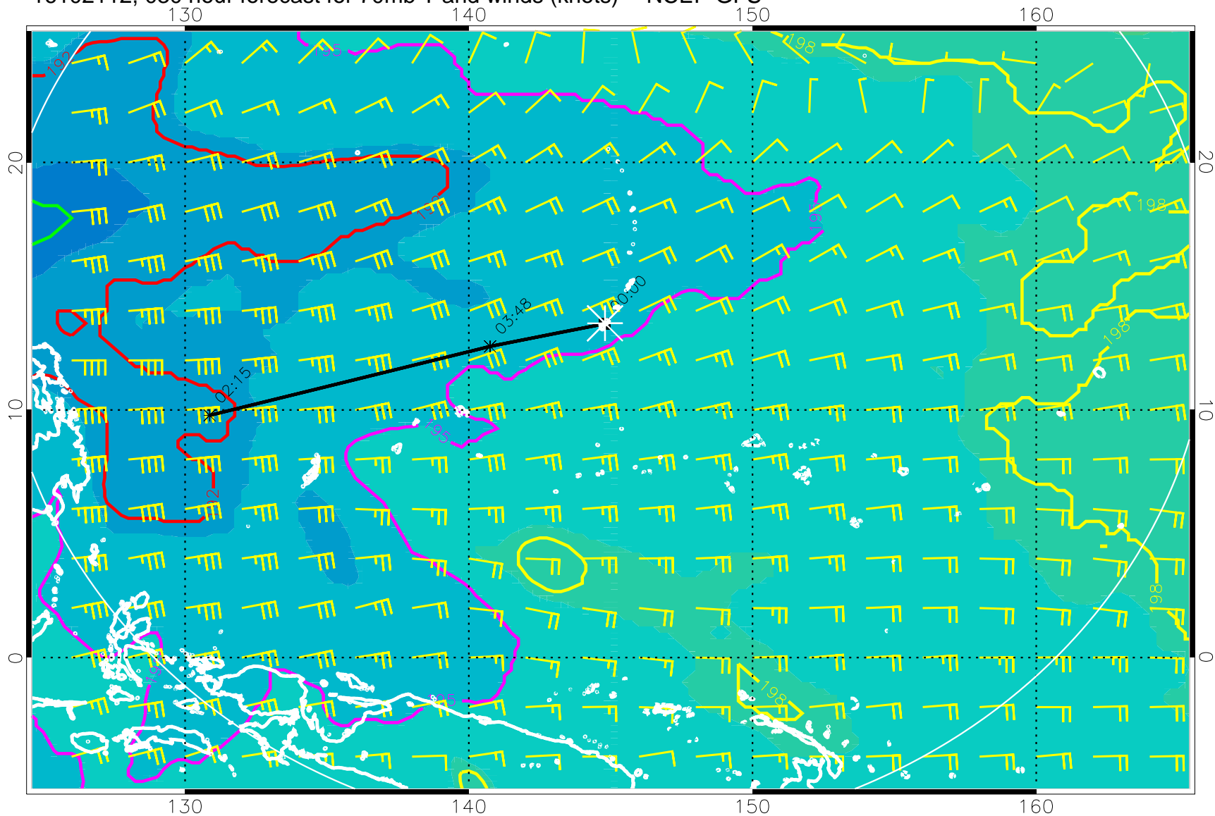
16102112, 030 hour forecast for 70mb T and winds (knots) -- NCEP GFS
