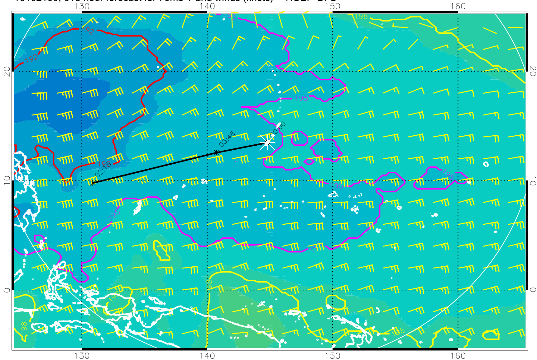
16102100, 018 hour forecast for 70mb T and winds (knots) -- NCEP GFS
