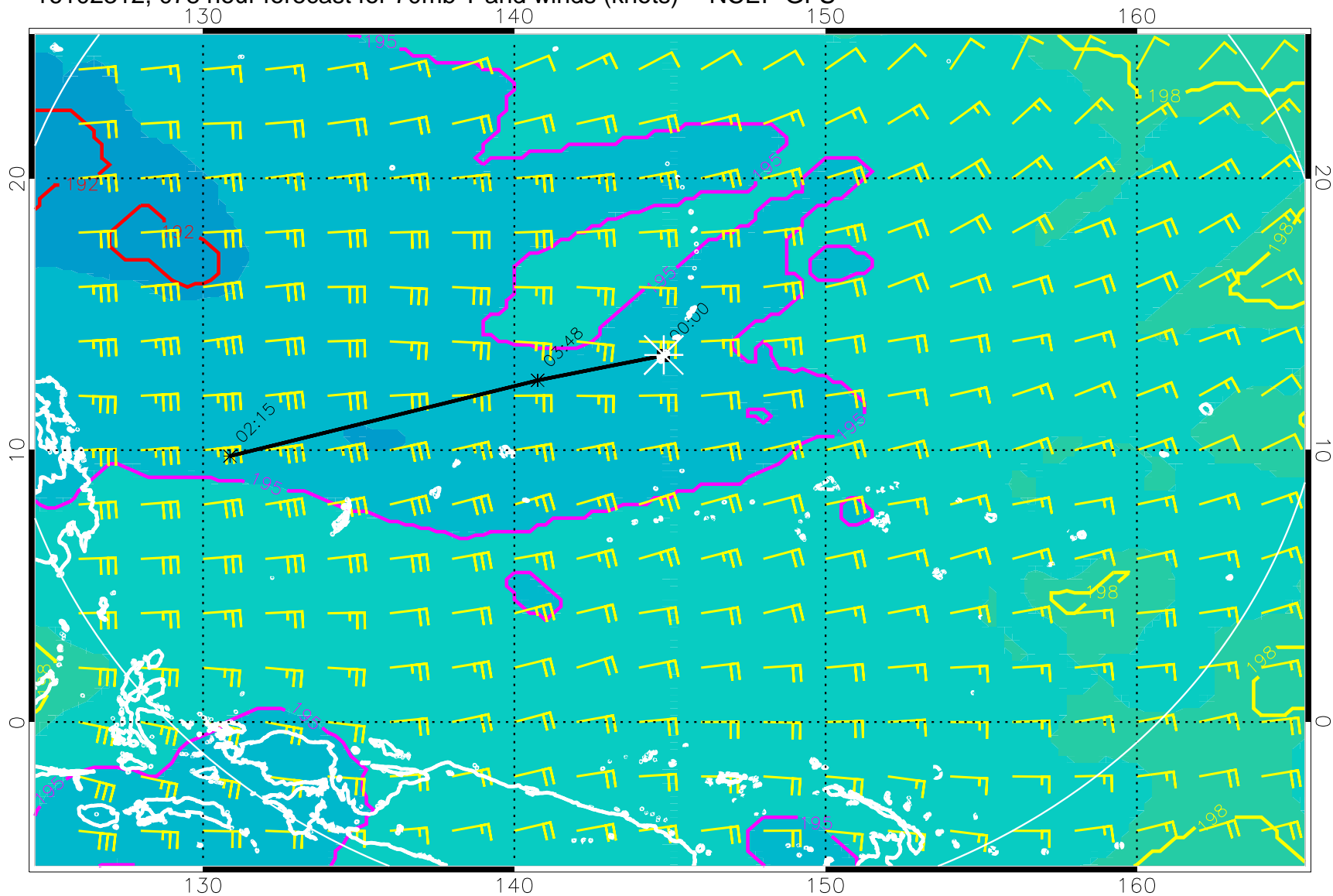
16102312, 078 hour forecast for 70mb T and winds (knots) -- NCEP GFS
