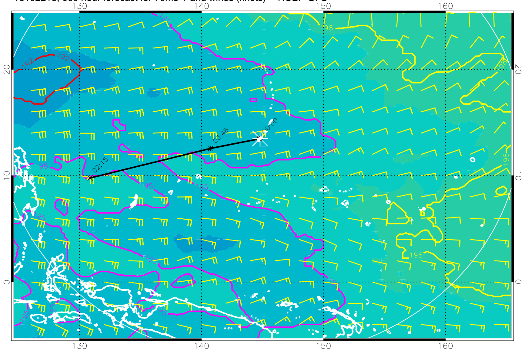
16102218, 060 hour forecast for 70mb T and winds (knots) -- NCEP GFS
