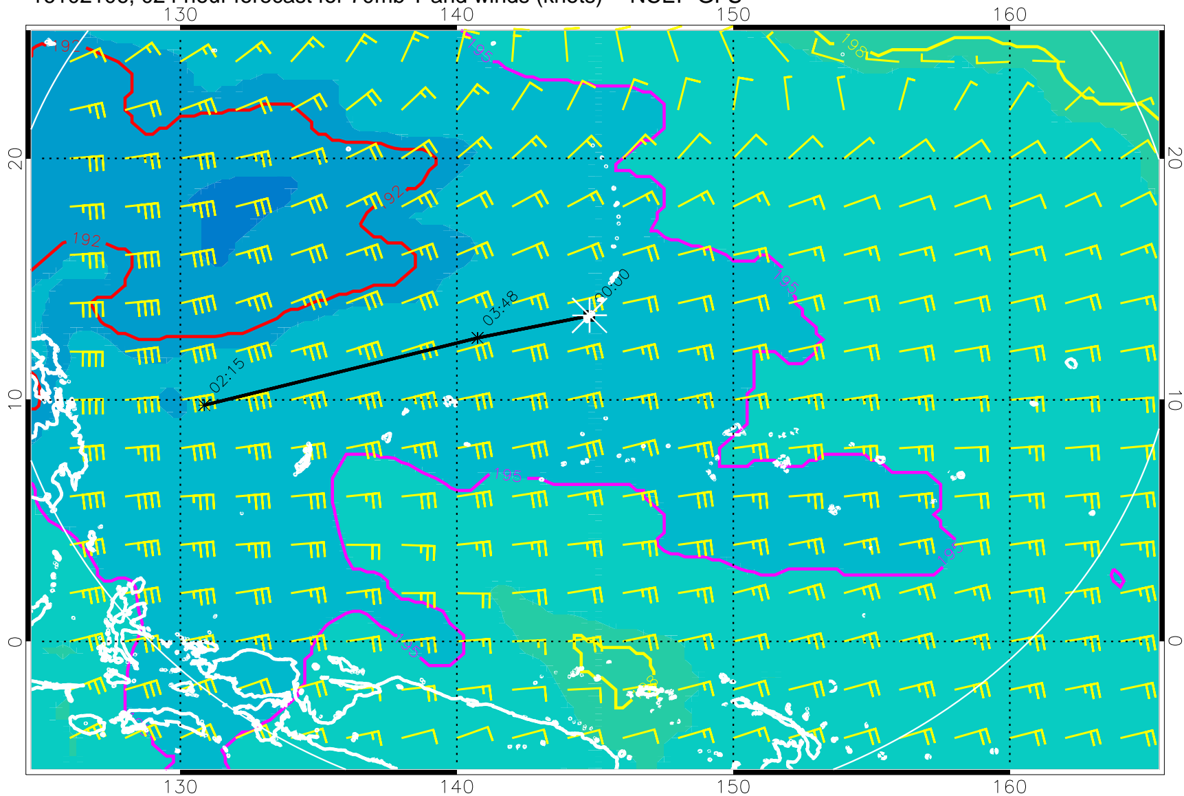
16102106, 024 hour forecast for 70mb T and winds (knots) -- NCEP GFS
