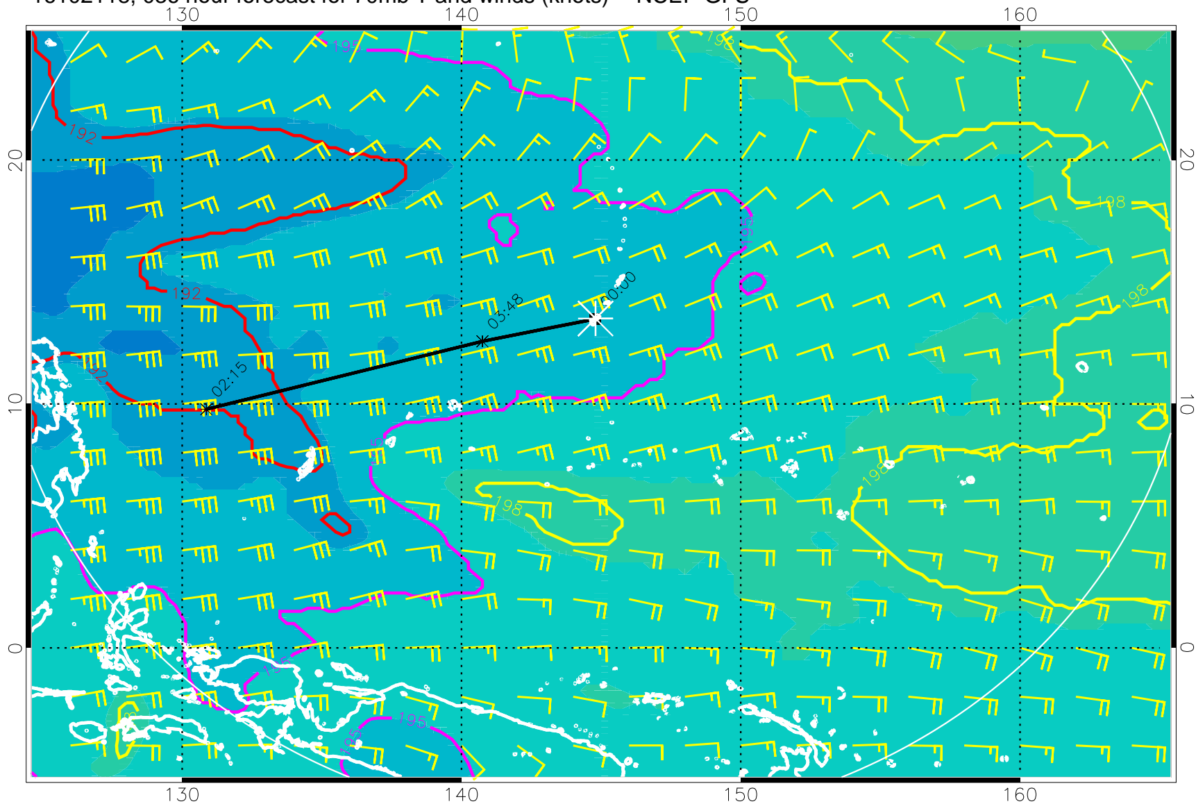
16102118, 036 hour forecast for 70mb T and winds (knots) -- NCEP GFS
