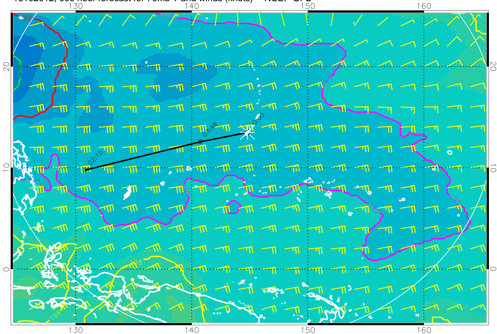
16102012, 006 hour forecast for 70mb T and winds (knots) -- NCEP GFS
