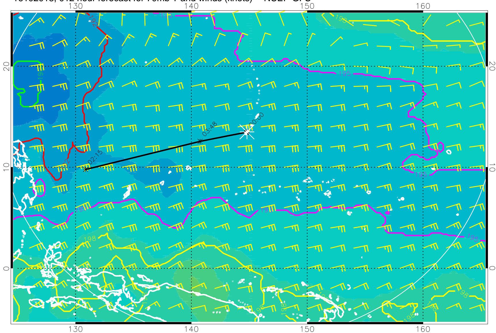
16102018, 012 hour forecast for 70mb T and winds (knots) -- NCEP GFS
