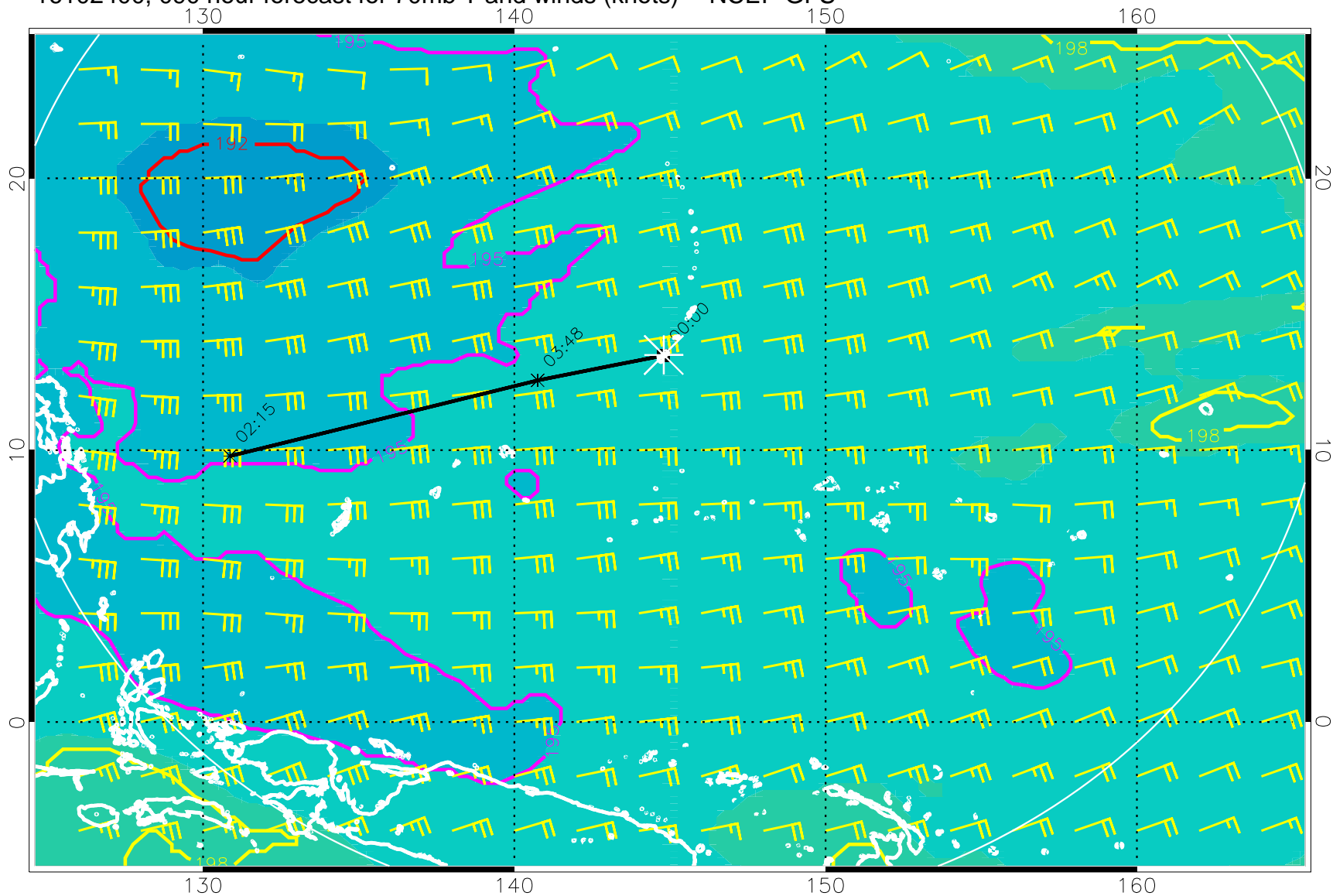
16102400, 090 hour forecast for 70mb T and winds (knots) -- NCEP GFS
