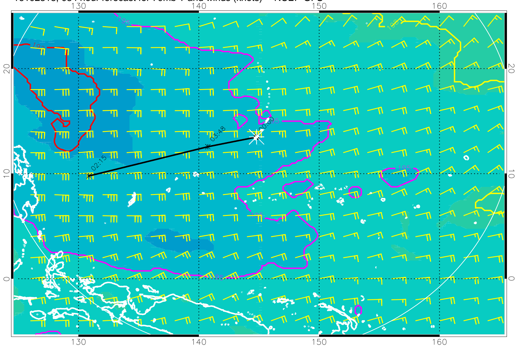
16102318, 084 hour forecast for 70mb T and winds (knots) -- NCEP GFS
