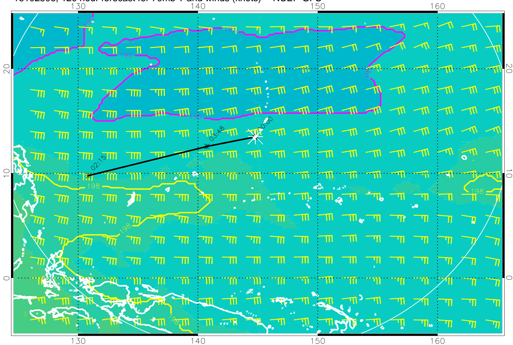
16102506, 120 hour forecast for 70mb T and winds (knots) -- NCEP GFS
