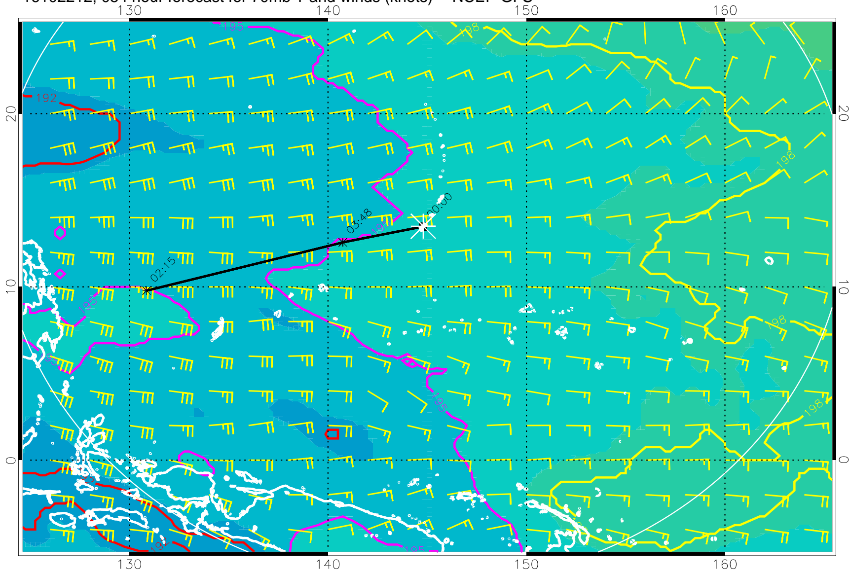
16102212, 054 hour forecast for 70mb T and winds (knots) -- NCEP GFS
