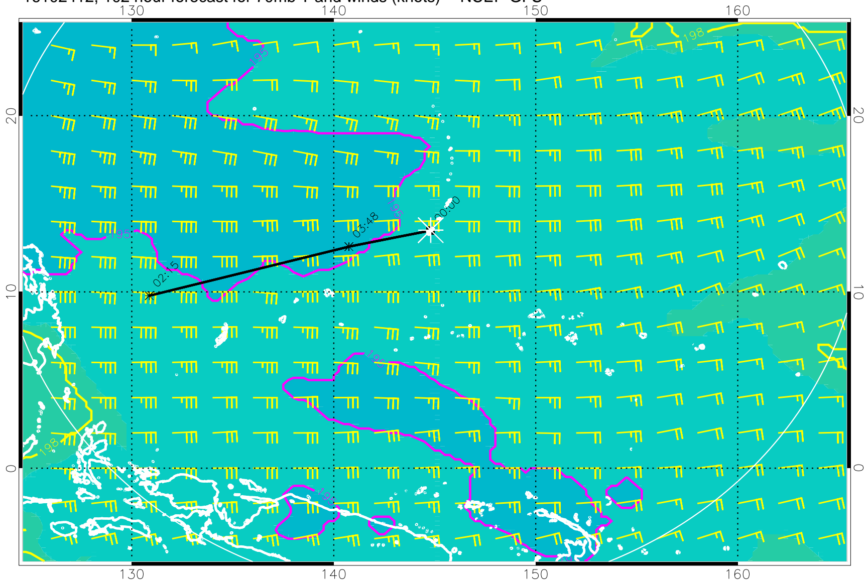
16102412, 102 hour forecast for 70mb T and winds (knots) -- NCEP GFS
