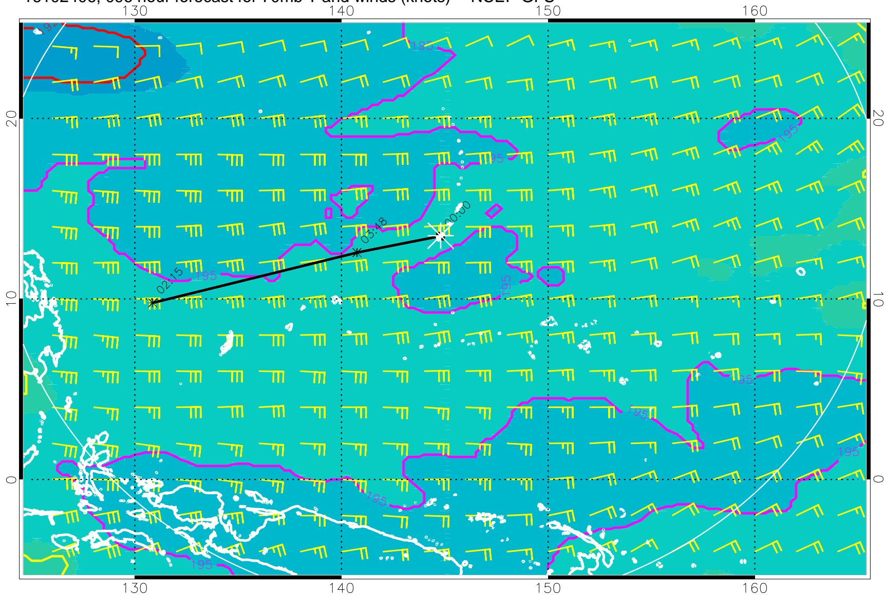
16102406, 096 hour forecast for 70mb T and winds (knots) -- NCEP GFS
