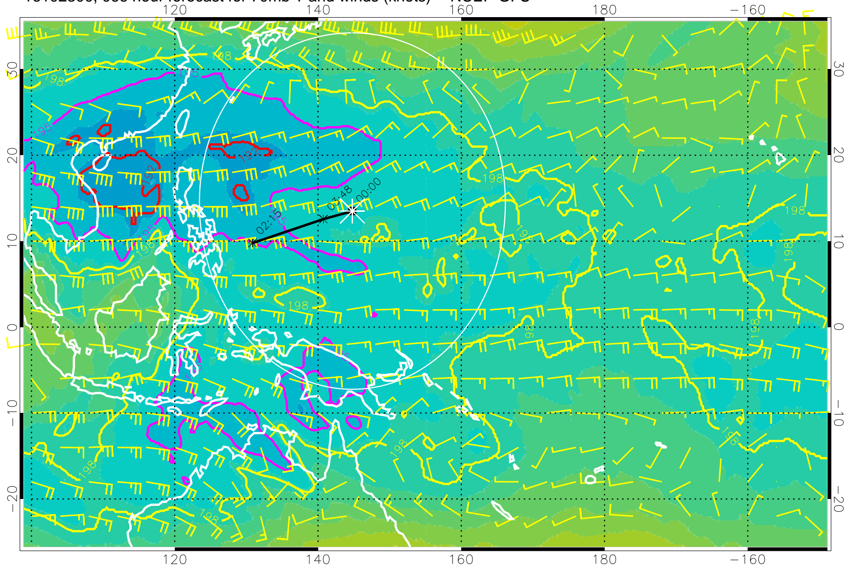
16102300, 066 hour forecast for 70mb T and winds (knots) -- NCEP GFS
