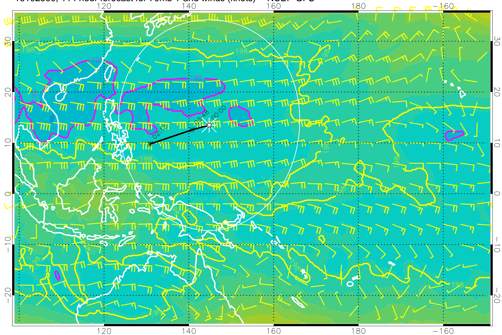
16102500, 114 hour forecast for 70mb T and winds (knots) -- NCEP GFS
