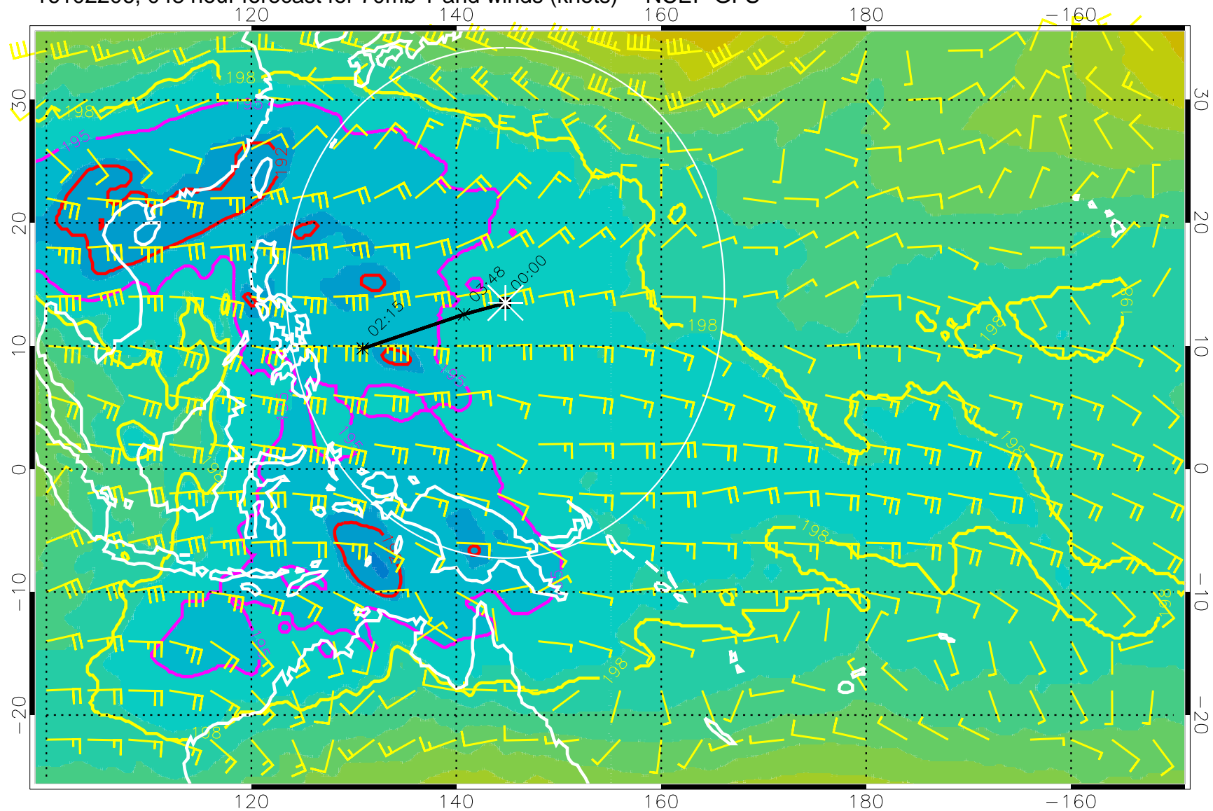
16102206, 048 hour forecast for 70mb T and winds (knots) -- NCEP GFS
