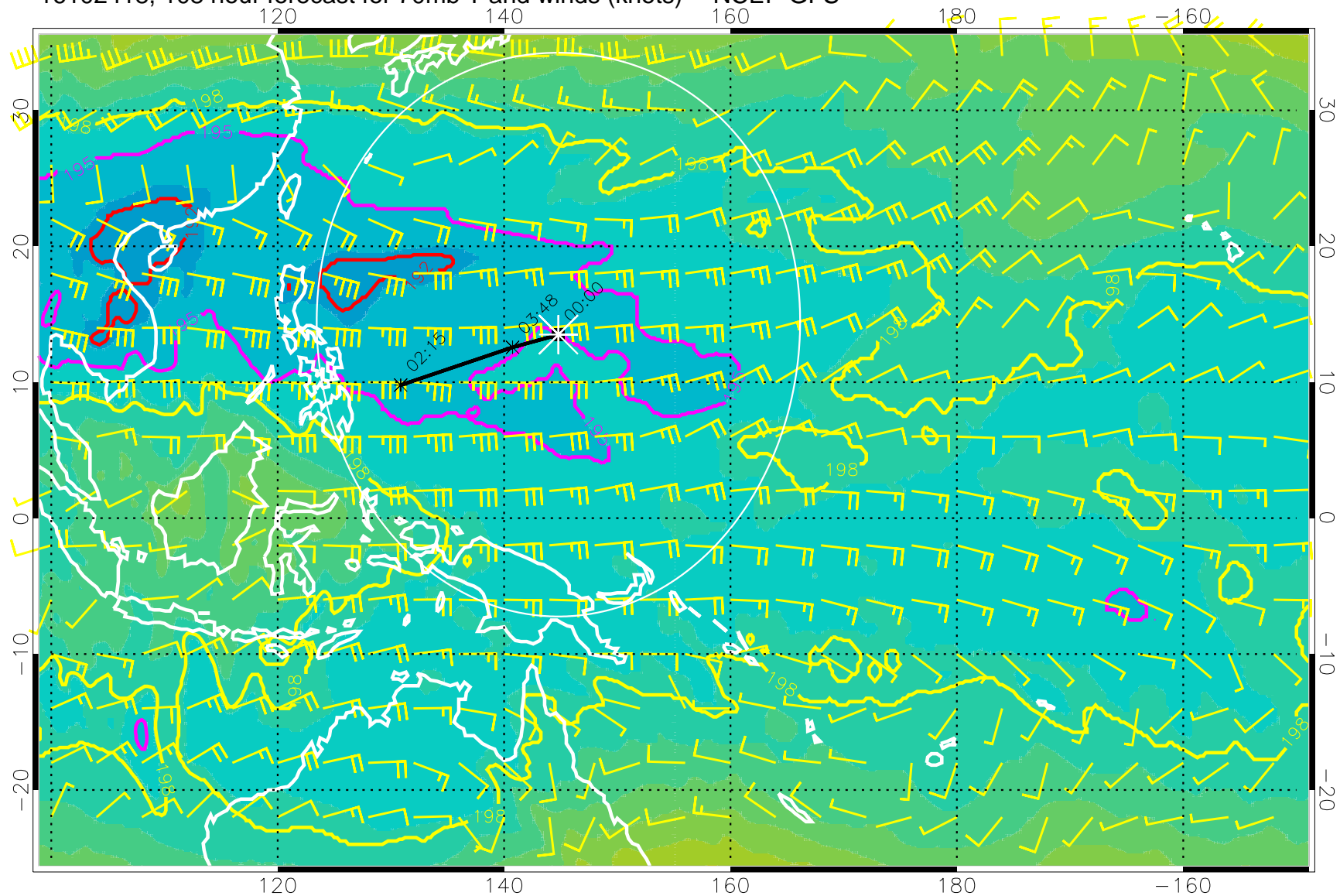
16102418, 108 hour forecast for 70mb T and winds (knots) -- NCEP GFS
