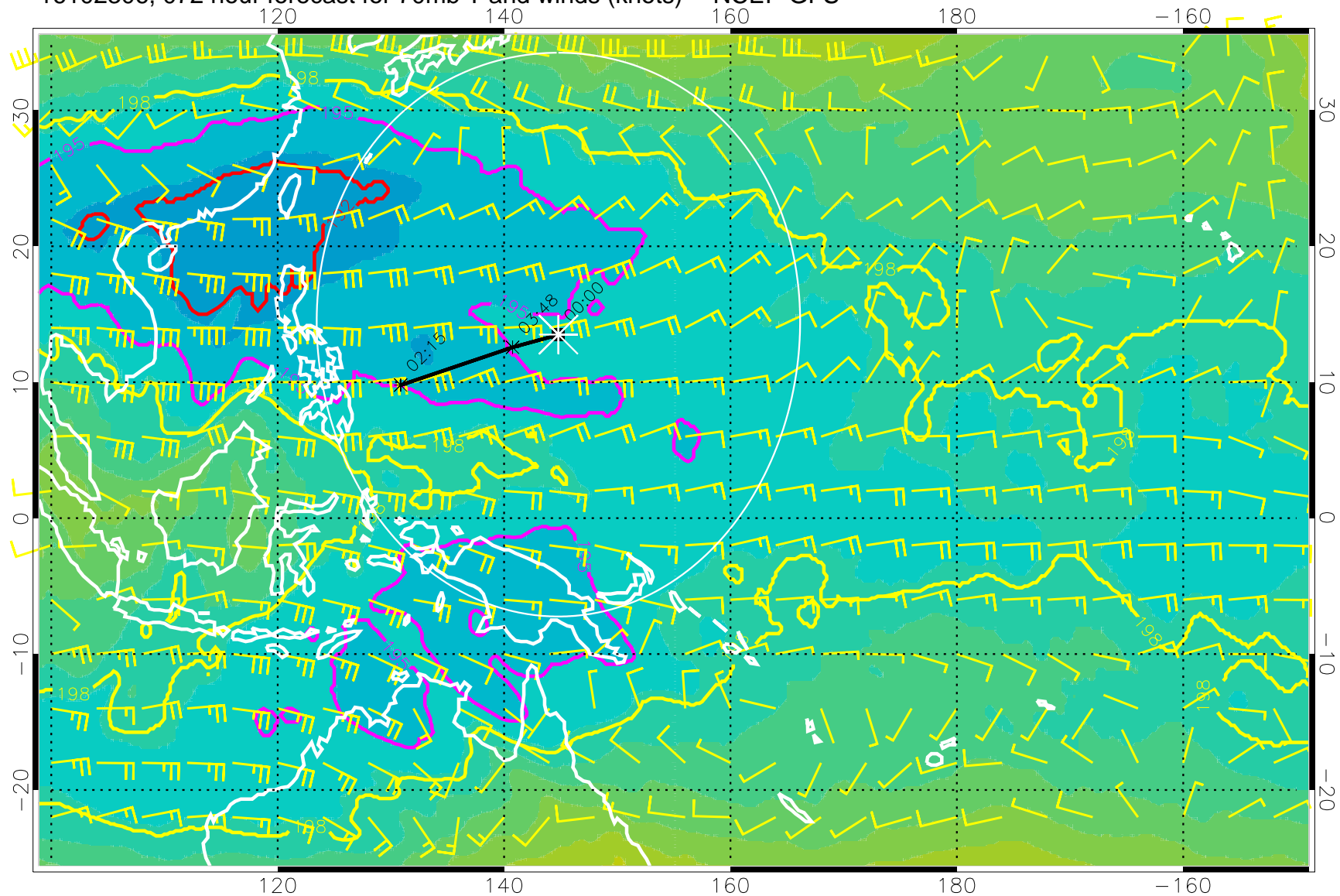
16102306, 072 hour forecast for 70mb T and winds (knots) -- NCEP GFS
