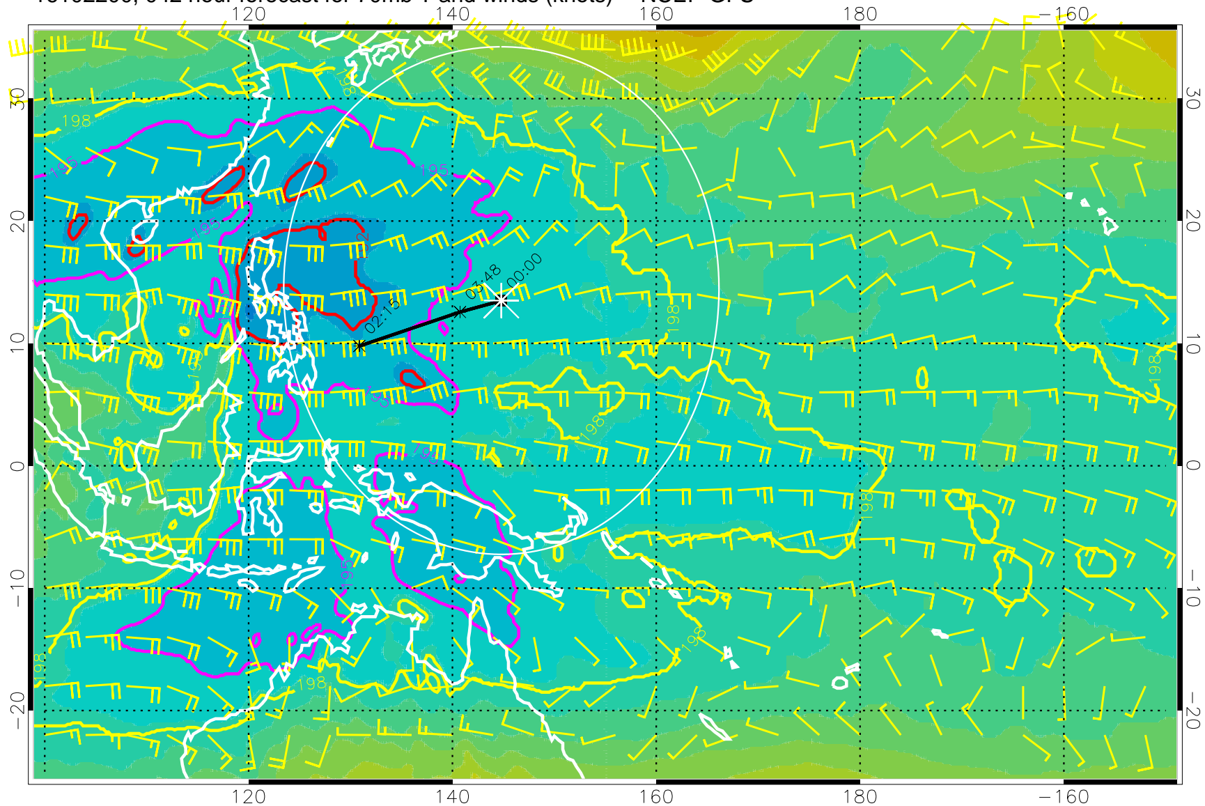
16102200, 042 hour forecast for 70mb T and winds (knots) -- NCEP GFS
