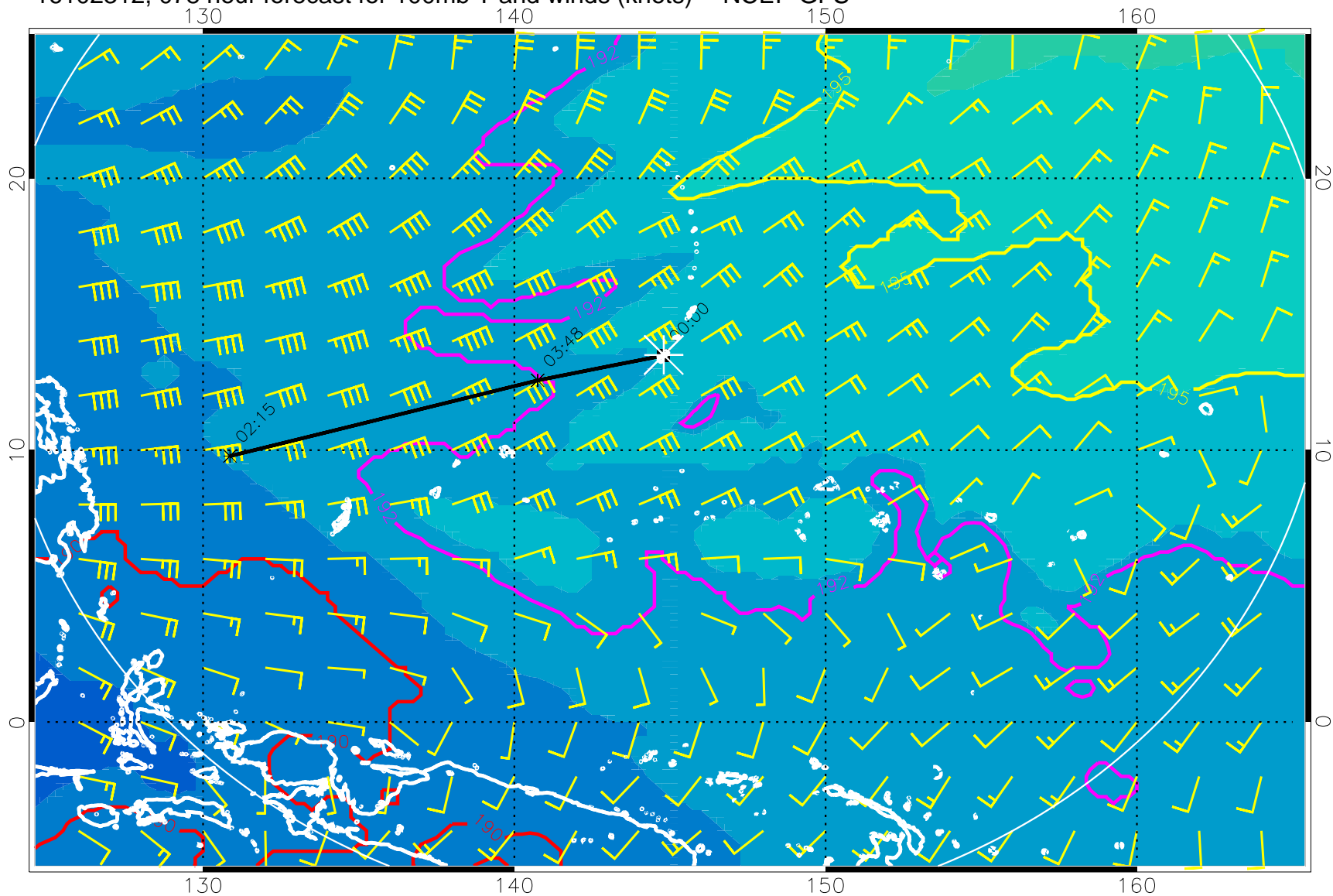
16102312, 078 hour forecast for 100mb T and winds (knots) -- NCEP GFS
