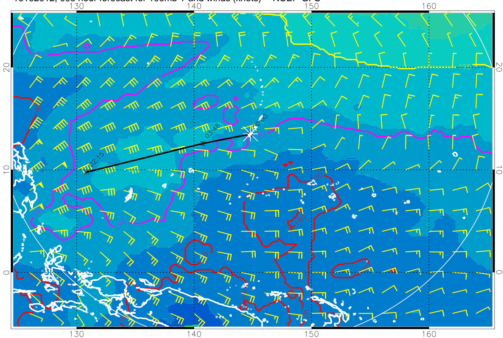
16102012, 006 hour forecast for 100mb T and winds (knots) -- NCEP GFS
