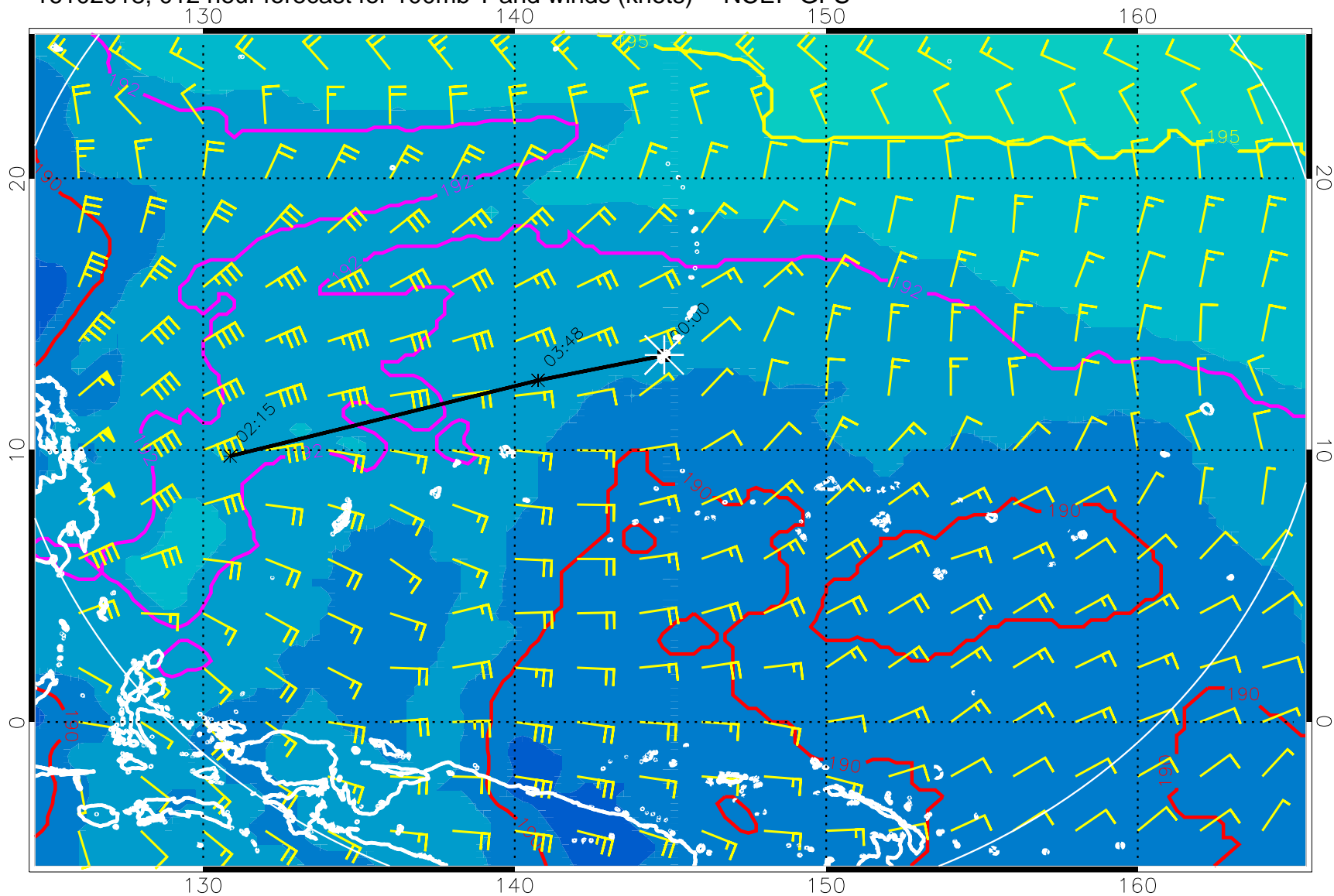
16102018, 012 hour forecast for 100mb T and winds (knots) -- NCEP GFS
