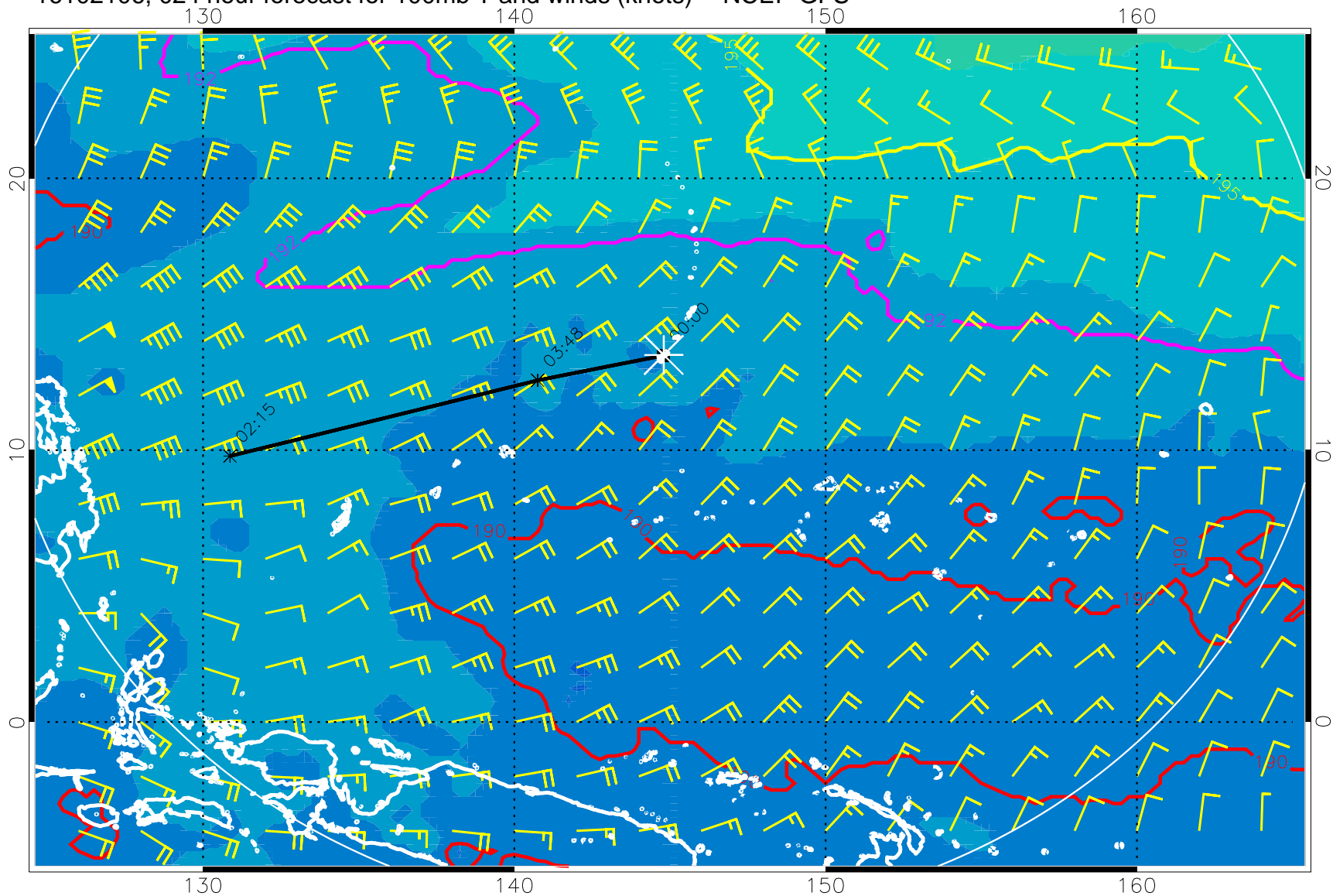
16102106, 024 hour forecast for 100mb T and winds (knots) -- NCEP GFS
