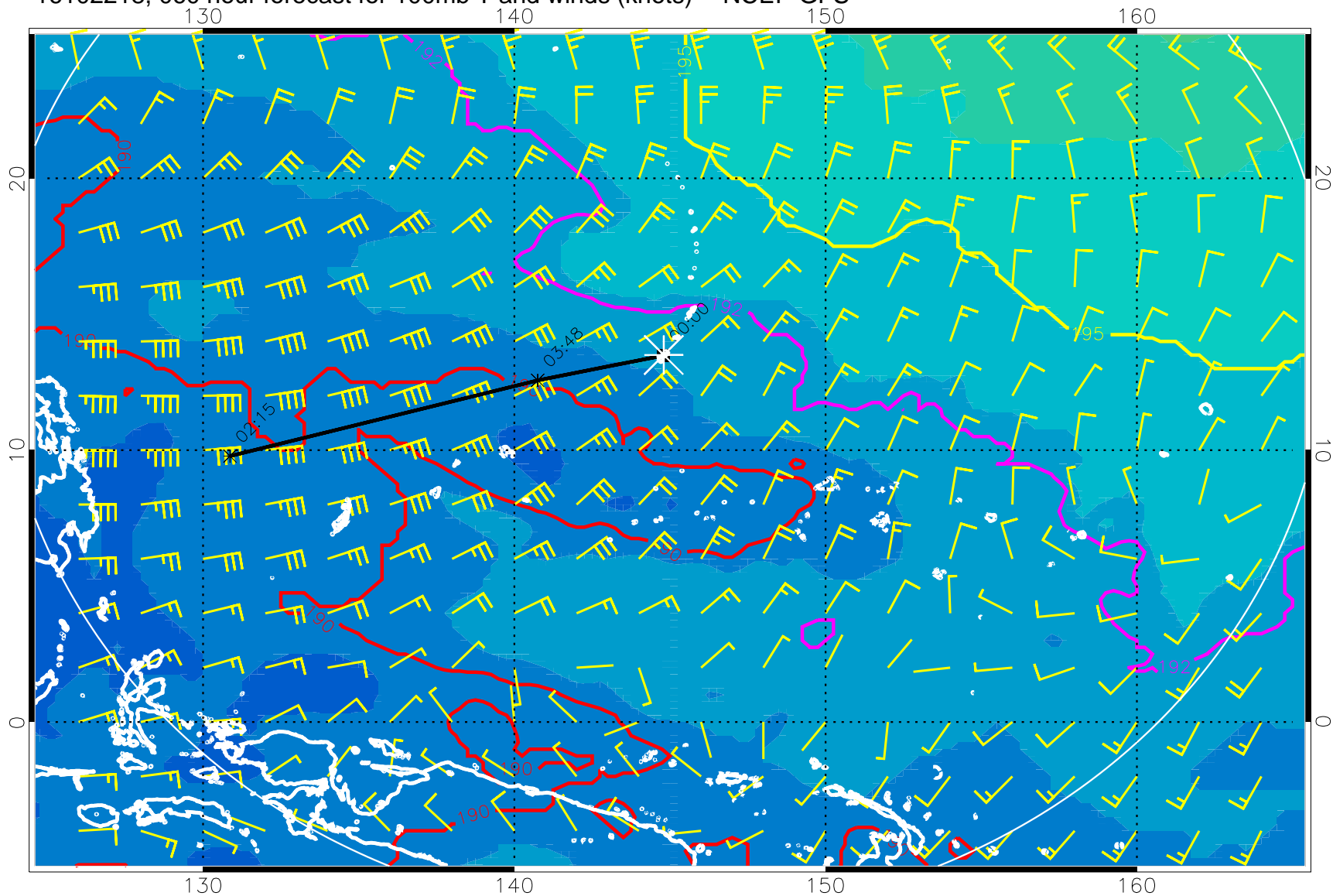
16102218, 060 hour forecast for 100mb T and winds (knots) -- NCEP GFS
