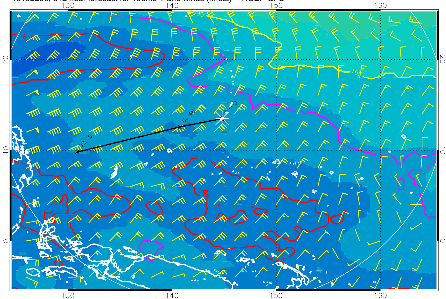
16102200, 042 hour forecast for 100mb T and winds (knots) -- NCEP GFS
