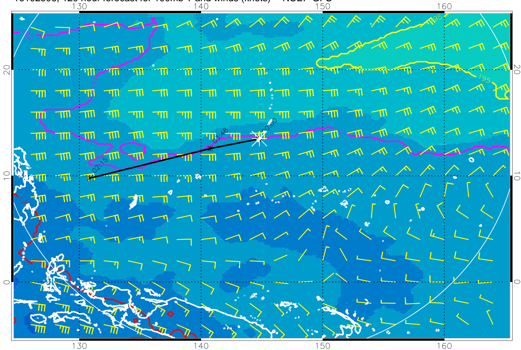
16102506, 120 hour forecast for 100mb T and winds (knots) -- NCEP GFS
