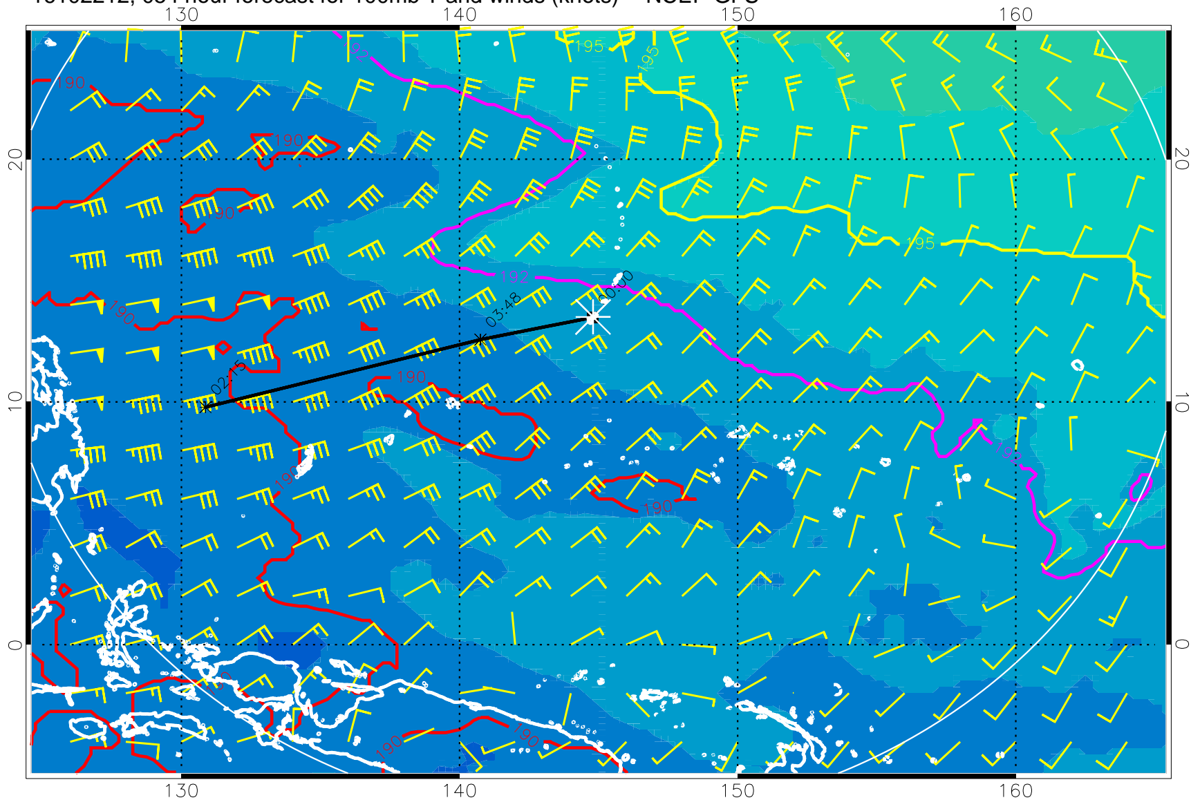
16102212, 054 hour forecast for 100mb T and winds (knots) -- NCEP GFS
