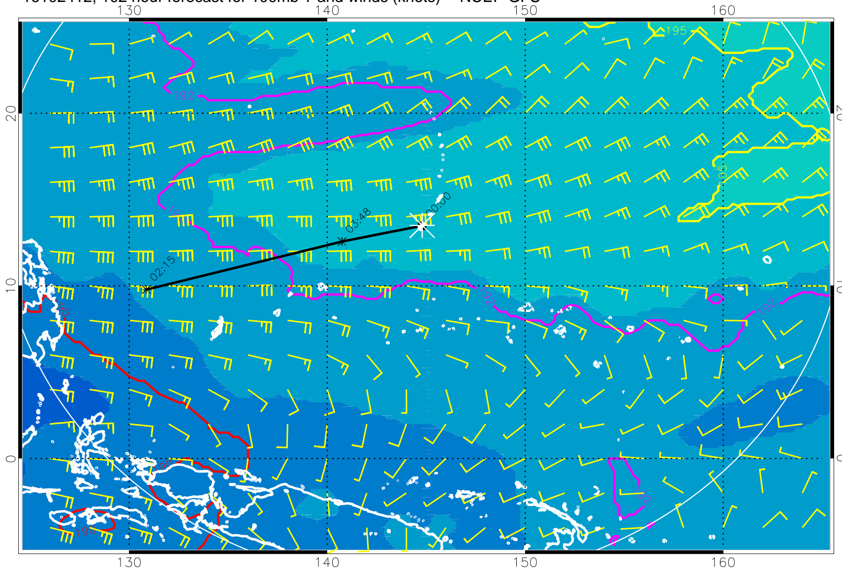
16102412, 102 hour forecast for 100mb T and winds (knots) -- NCEP GFS
