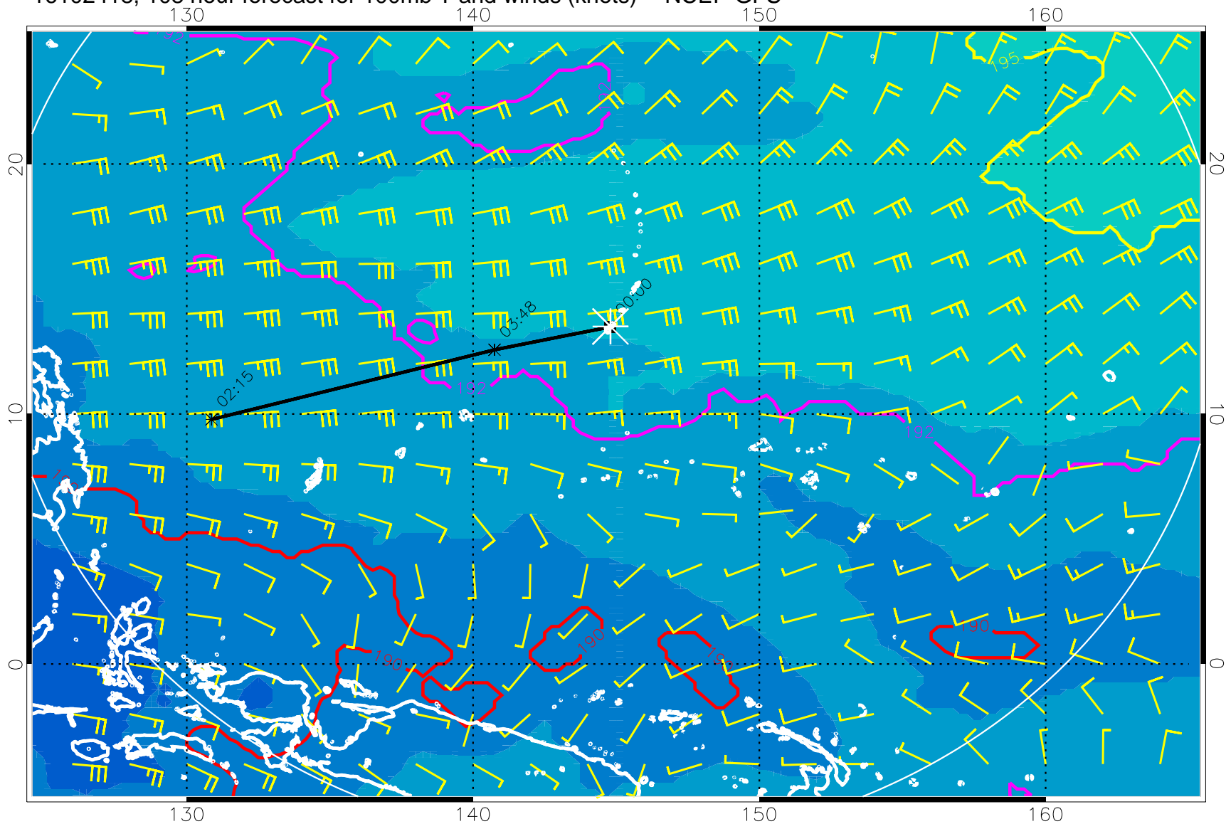
16102418, 108 hour forecast for 100mb T and winds (knots) -- NCEP GFS
