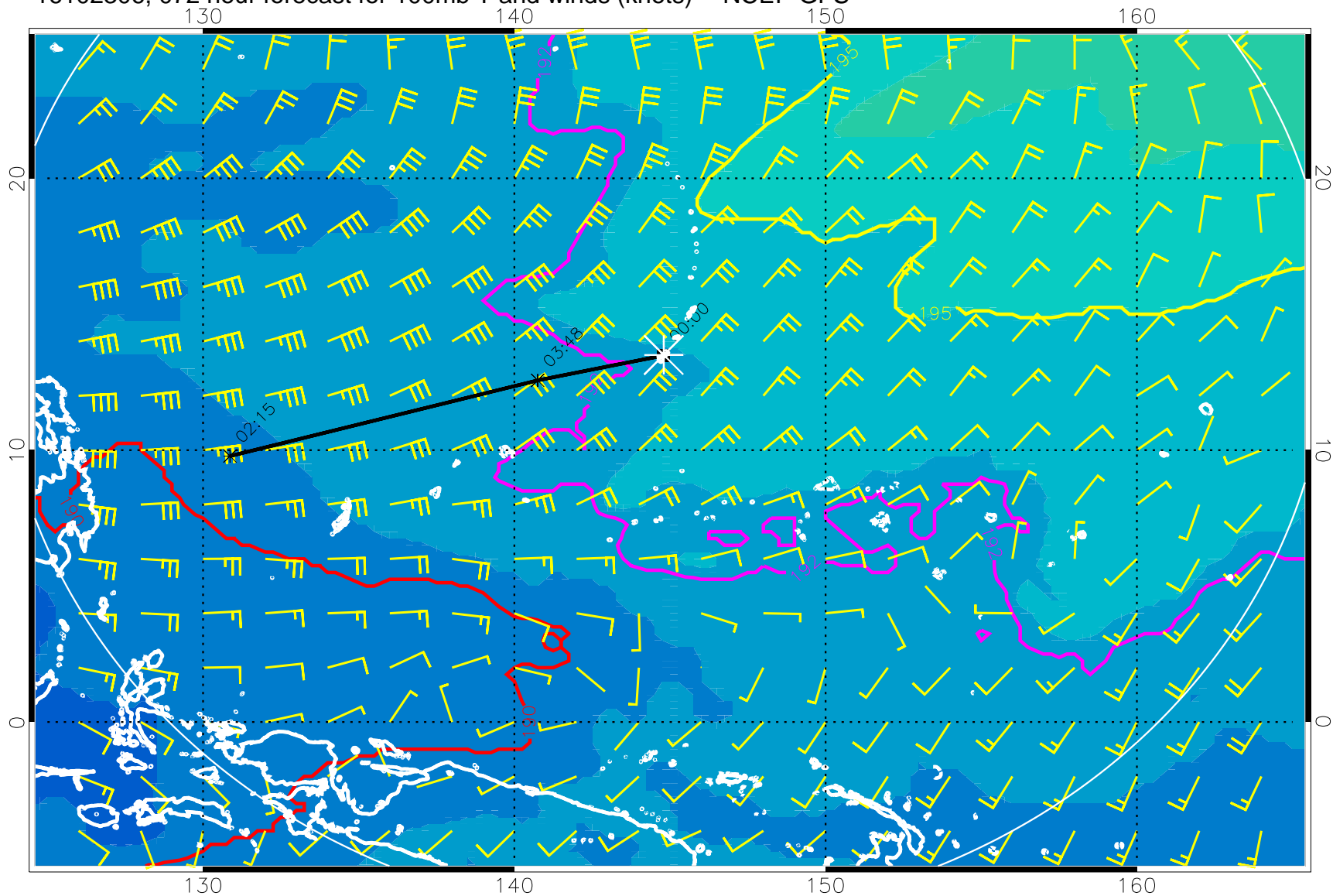
16102306, 072 hour forecast for 100mb T and winds (knots) -- NCEP GFS
