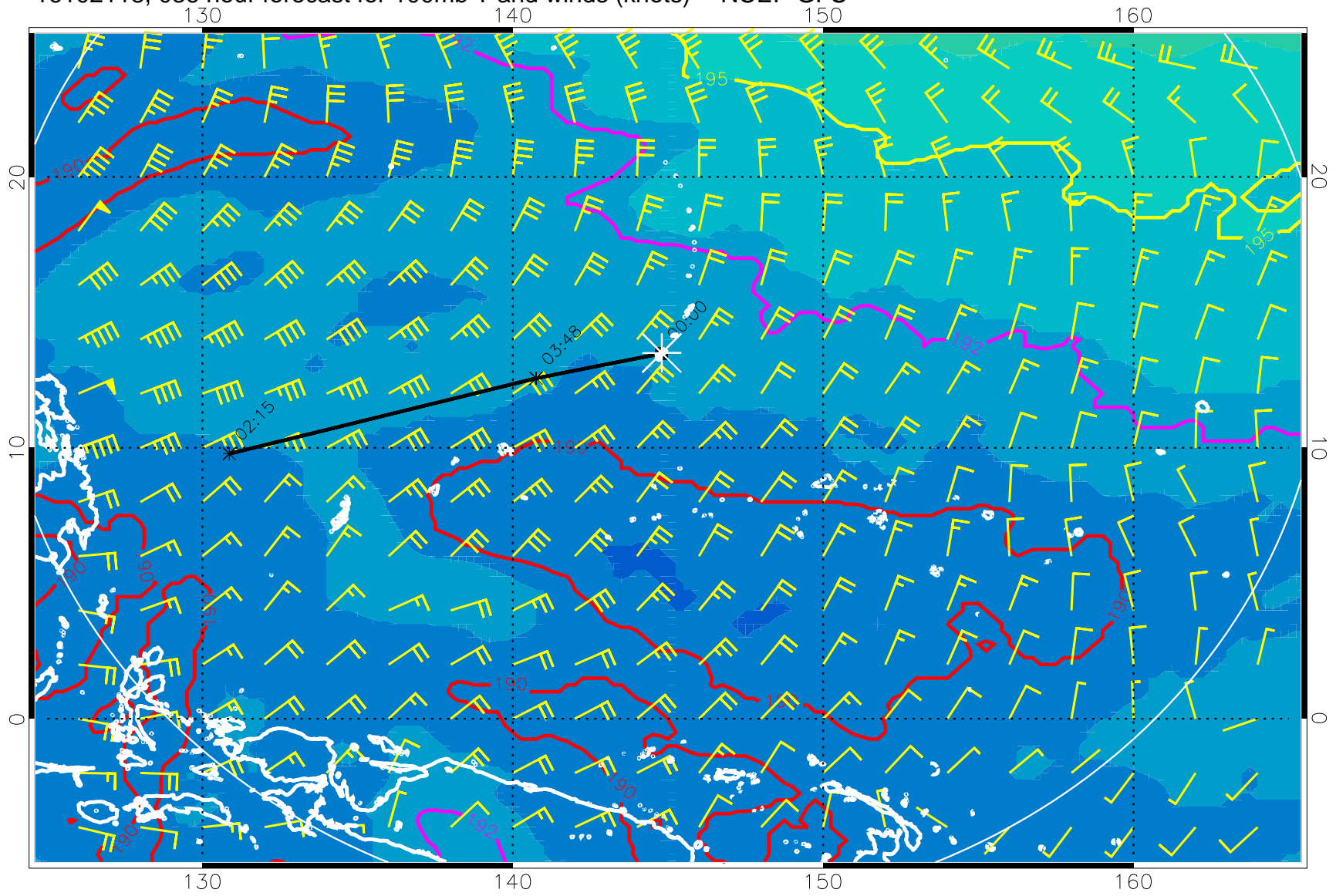
16102118, 036 hour forecast for 100mb T and winds (knots) -- NCEP GFS
