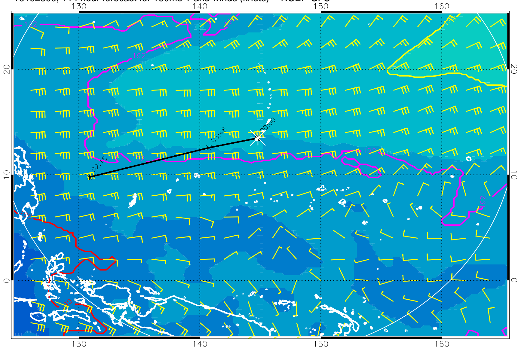
16102500, 114 hour forecast for 100mb T and winds (knots) -- NCEP GFS
