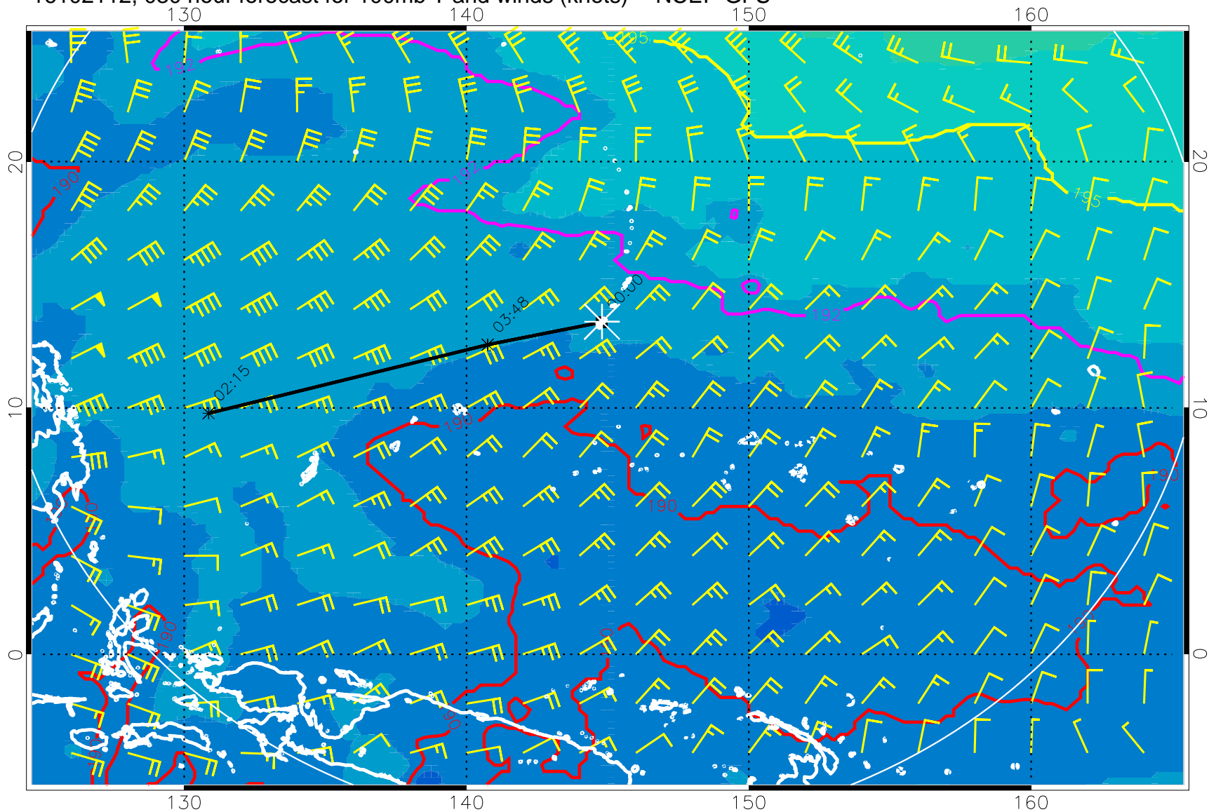
16102112, 030 hour forecast for 100mb T and winds (knots) -- NCEP GFS
