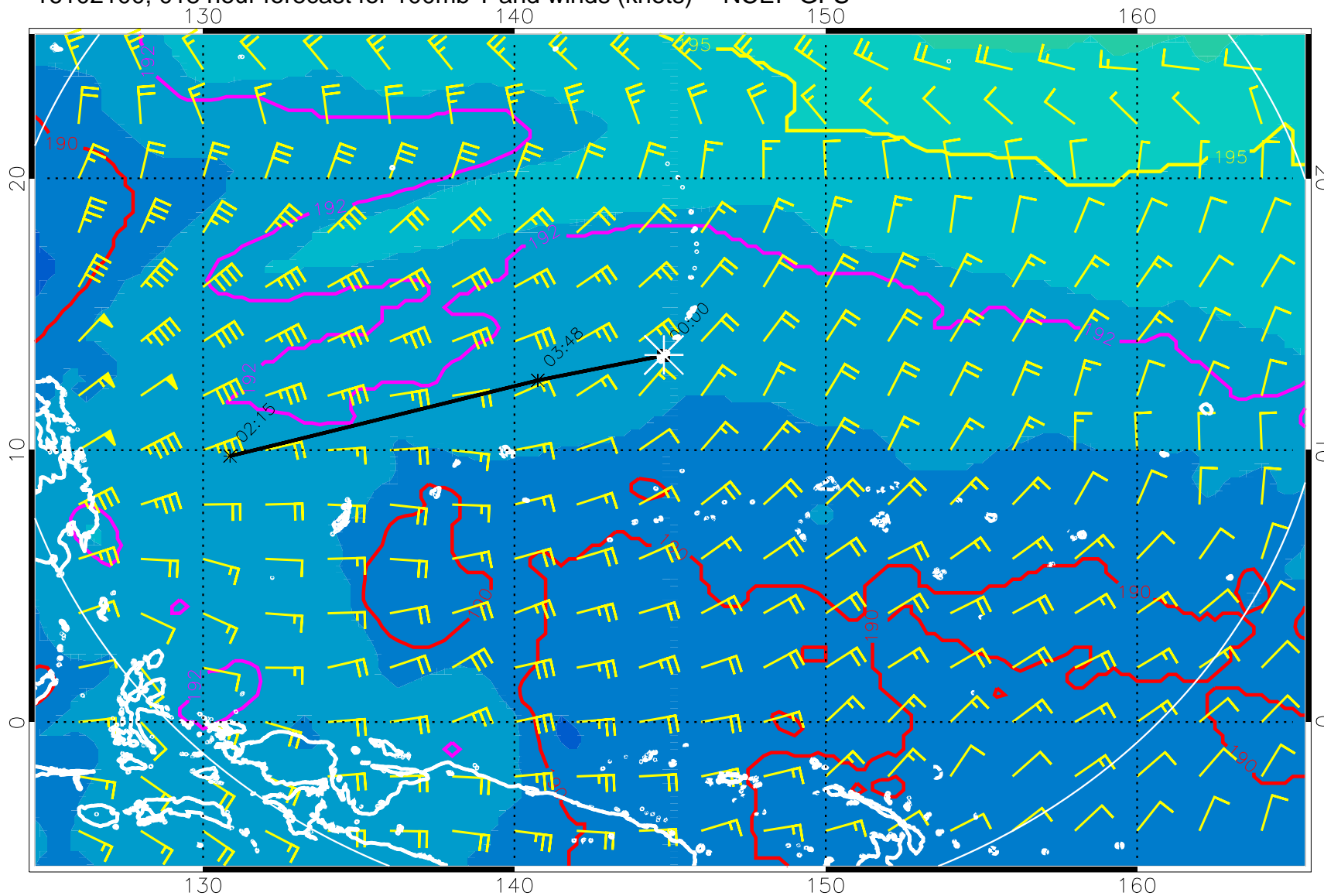
16102100, 018 hour forecast for 100mb T and winds (knots) -- NCEP GFS
