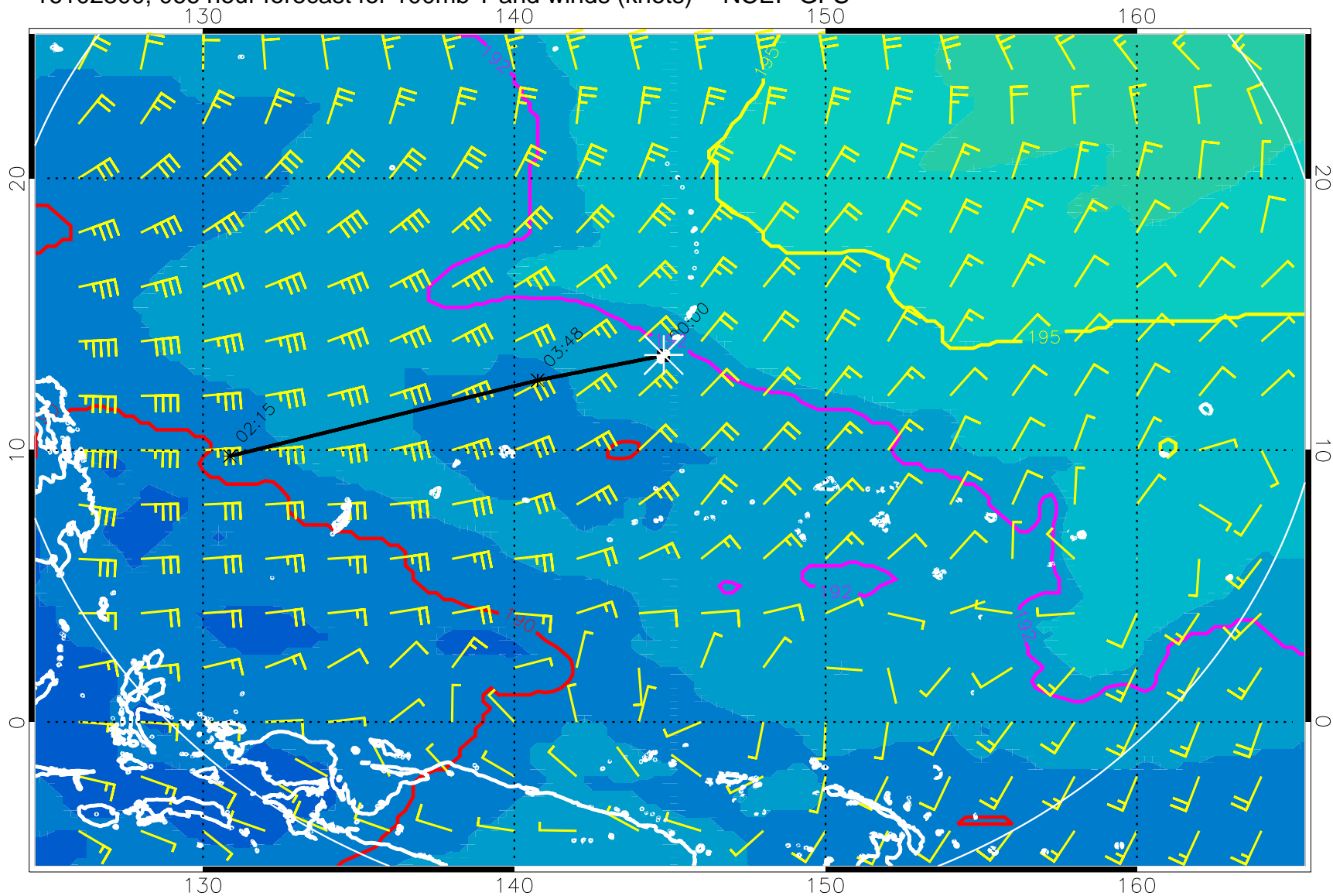
16102300, 066 hour forecast for 100mb T and winds (knots) -- NCEP GFS
