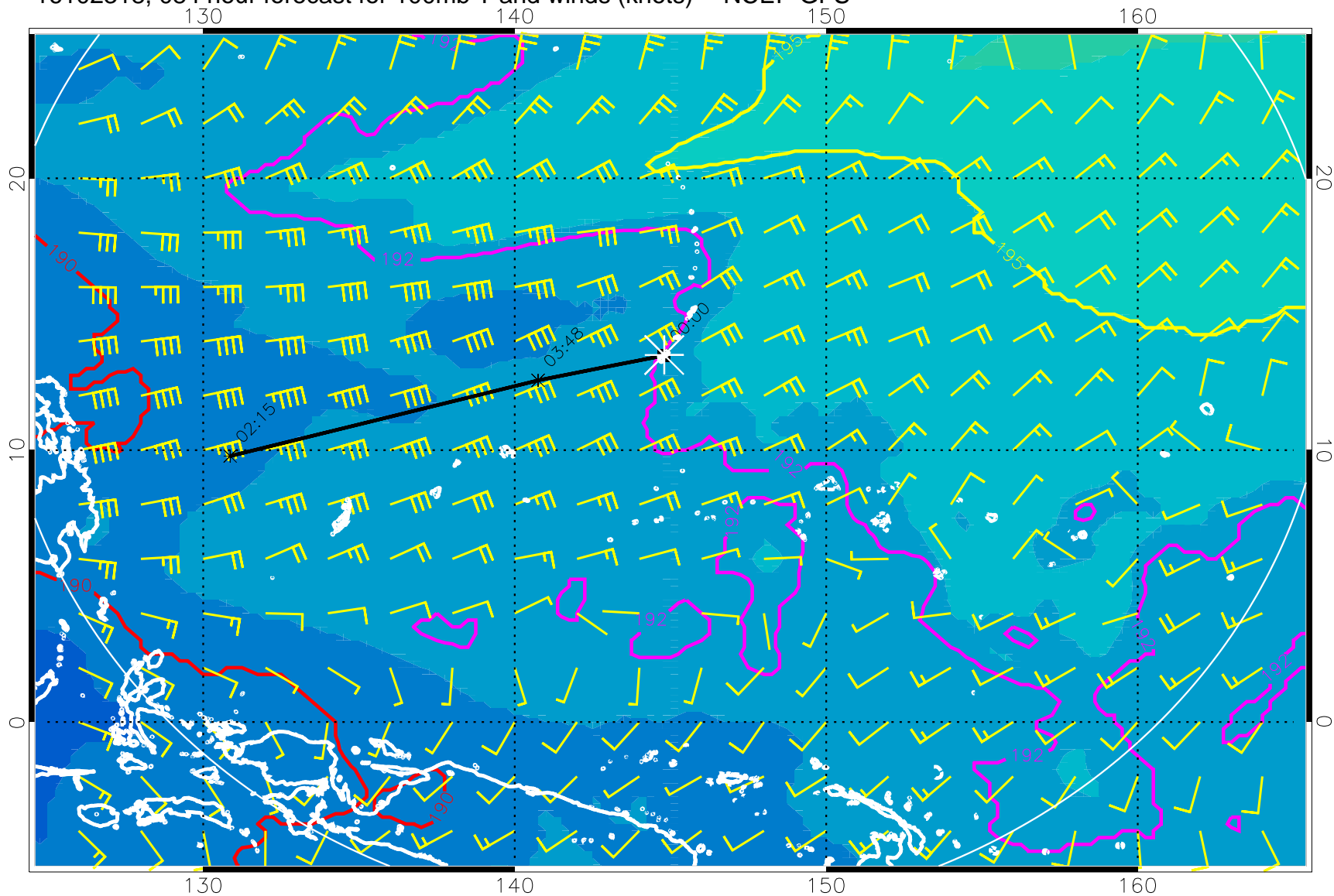
16102318, 084 hour forecast for 100mb T and winds (knots) -- NCEP GFS
