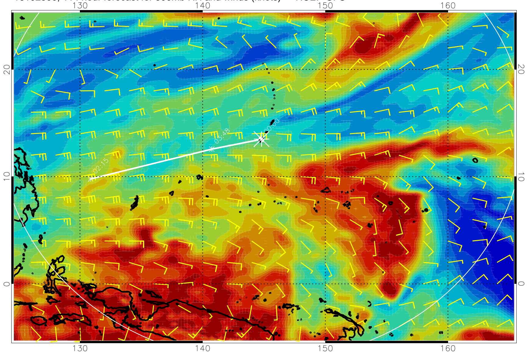
16102500, 114 hour forecast for 500mb RH and winds (knots) -- NCEP GFS
