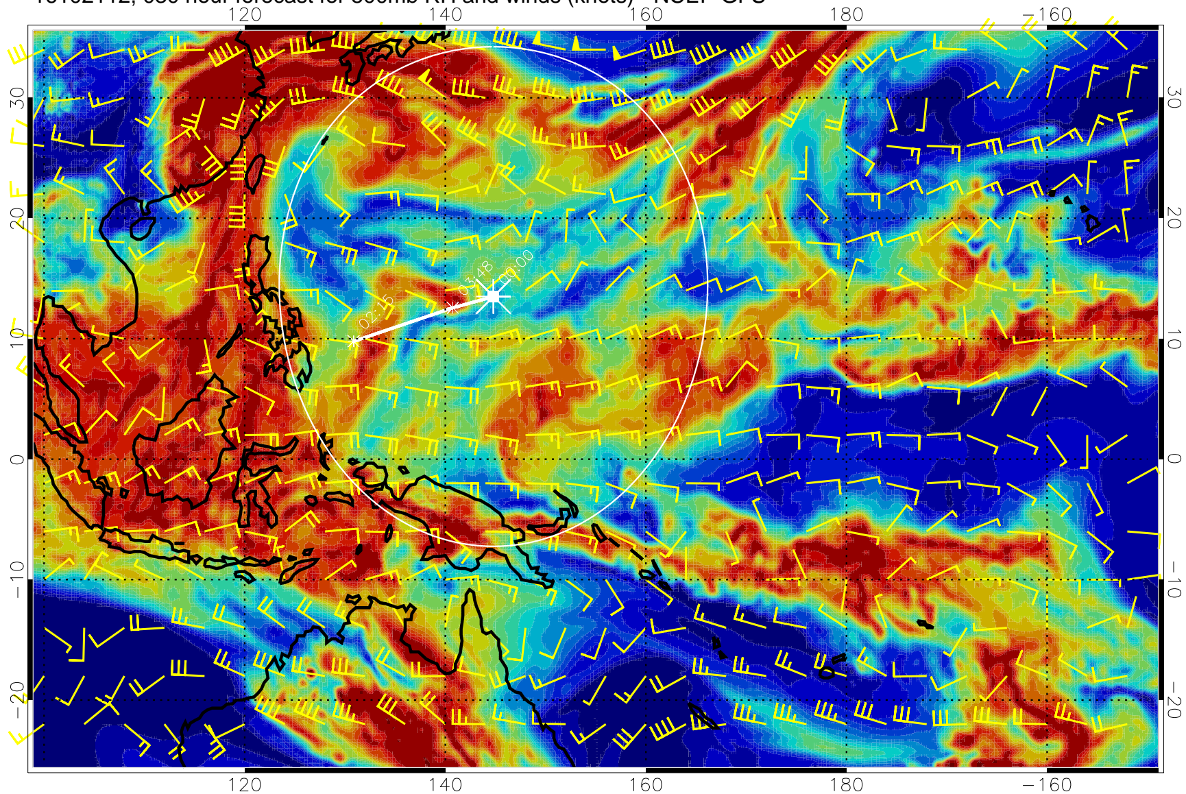
16102112, 030 hour forecast for 500mb RH and winds (knots) - NCEP GFS
