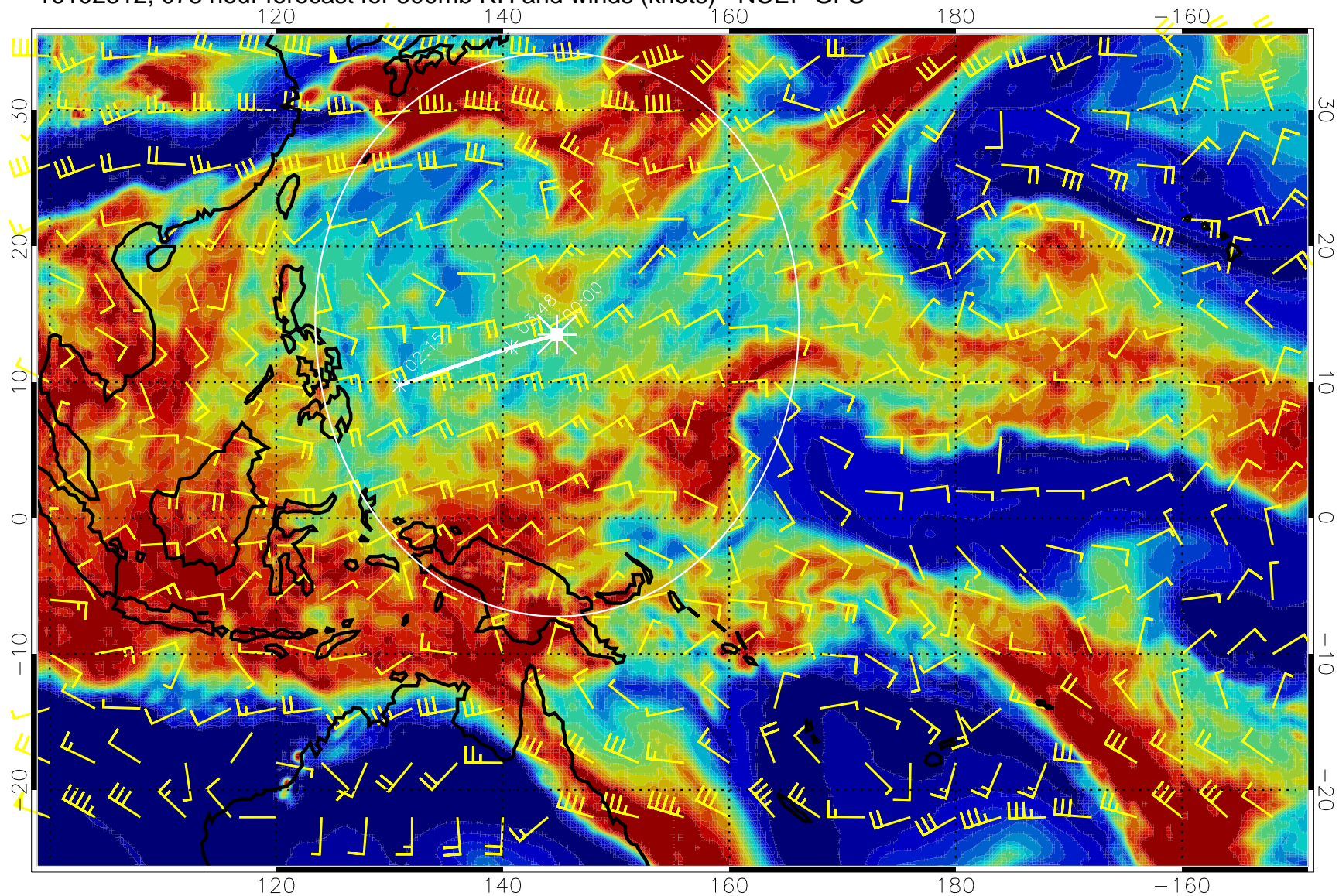
16102312, 078 hour forecast for 500mb RH and winds (knots) - NCEP GFS
