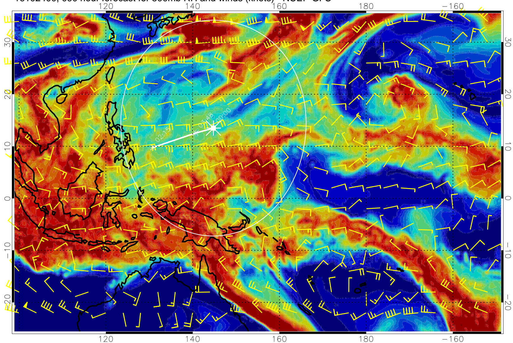
16102400, 090 hour forecast for 500mb RH and winds (knots) - NCEP GFS
