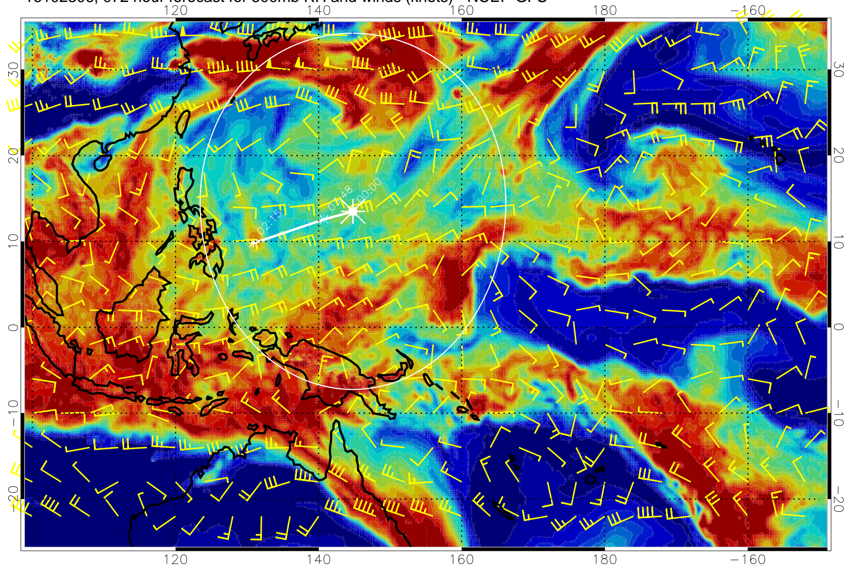
16102306, 072 hour forecast for 500mb RH and winds (knots) - NCEP GFS
