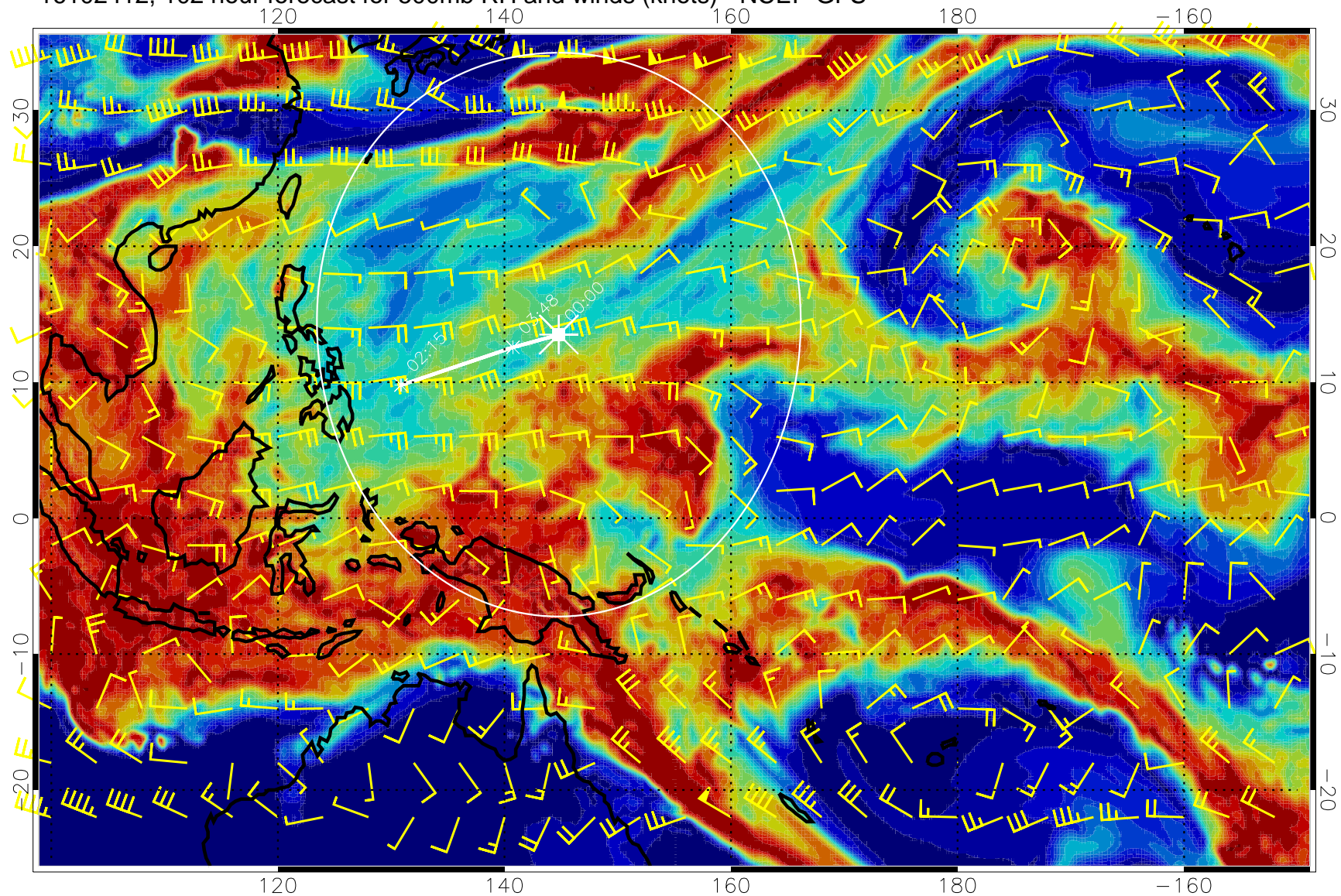
16102412, 102 hour forecast for 500mb RH and winds (knots) - NCEP GFS
