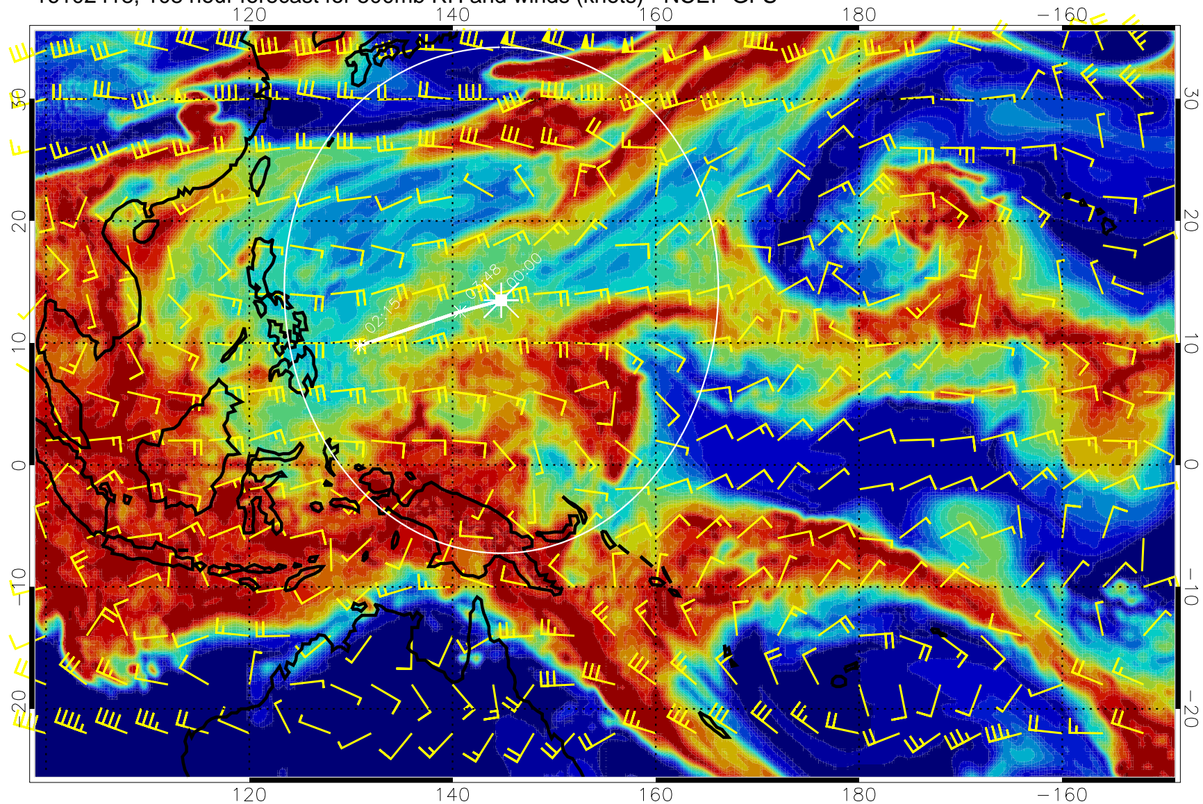
16102418, 108 hour forecast for 500mb RH and winds (knots) - NCEP GFS
