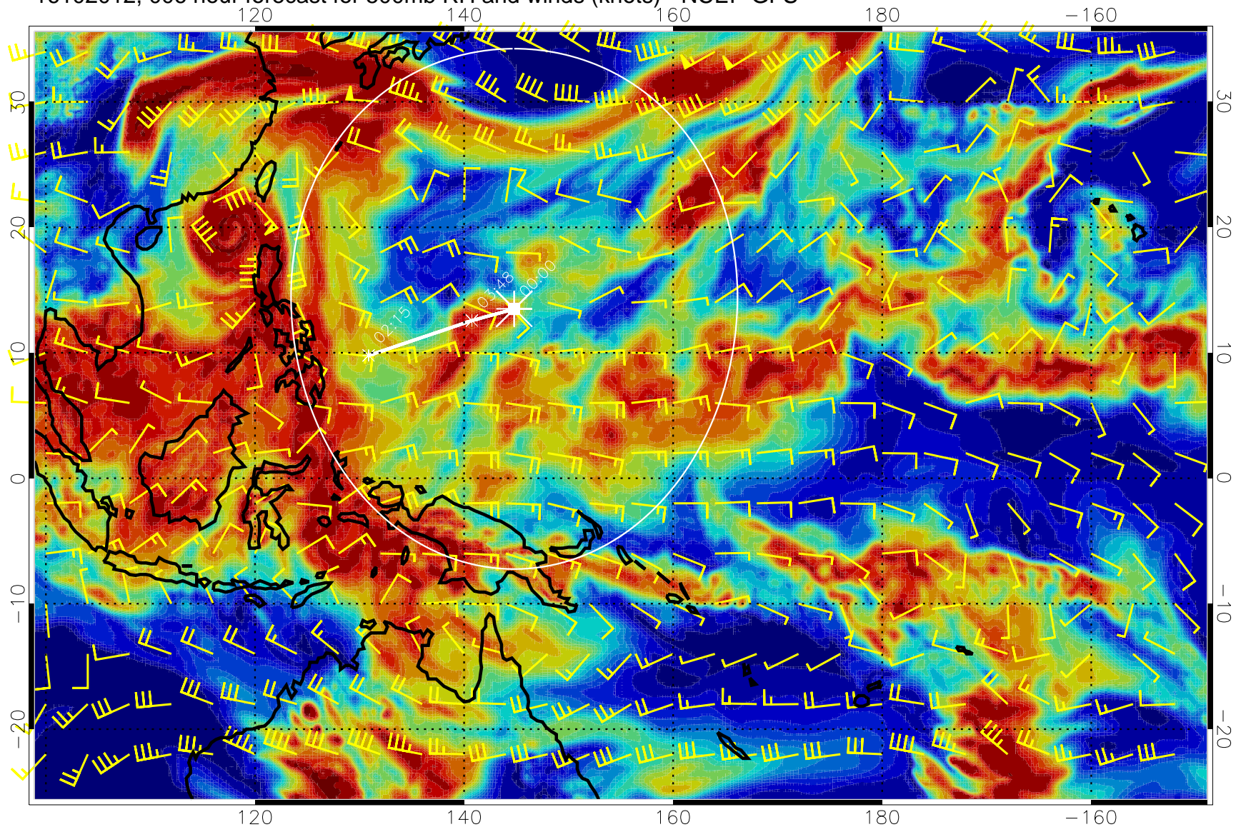
16102012, 006 hour forecast for 500mb RH and winds (knots) - NCEP GFS
