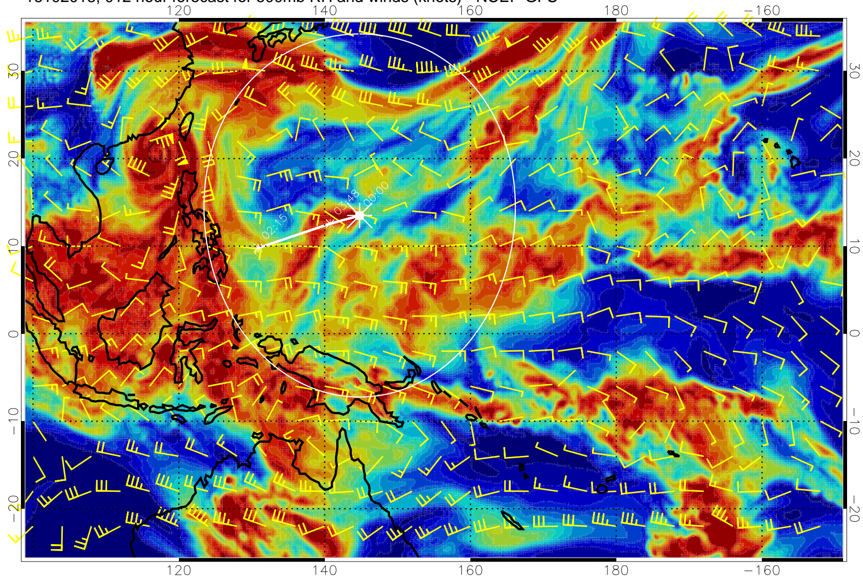
16102018, 012 hour forecast for 500mb RH and winds (knots) - NCEP GFS
