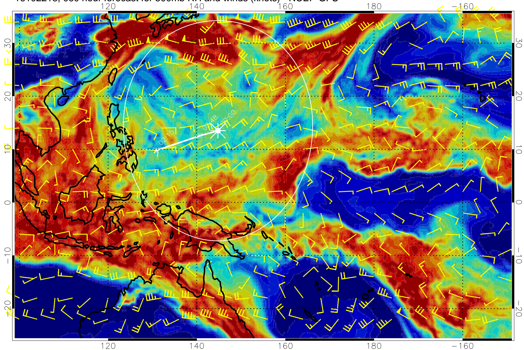
16102218, 060 hour forecast for 500mb RH and winds (knots) - NCEP GFS
