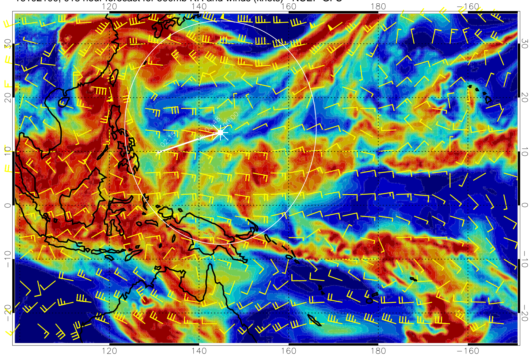
16102100, 018 hour forecast for 500mb RH and winds (knots) - NCEP GFS
