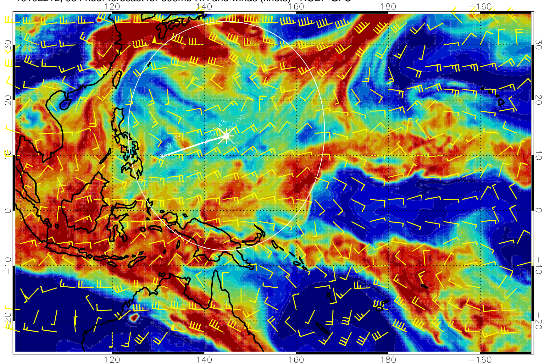
16102212, 054 hour forecast for 500mb RH and winds (knots) - NCEP GFS
