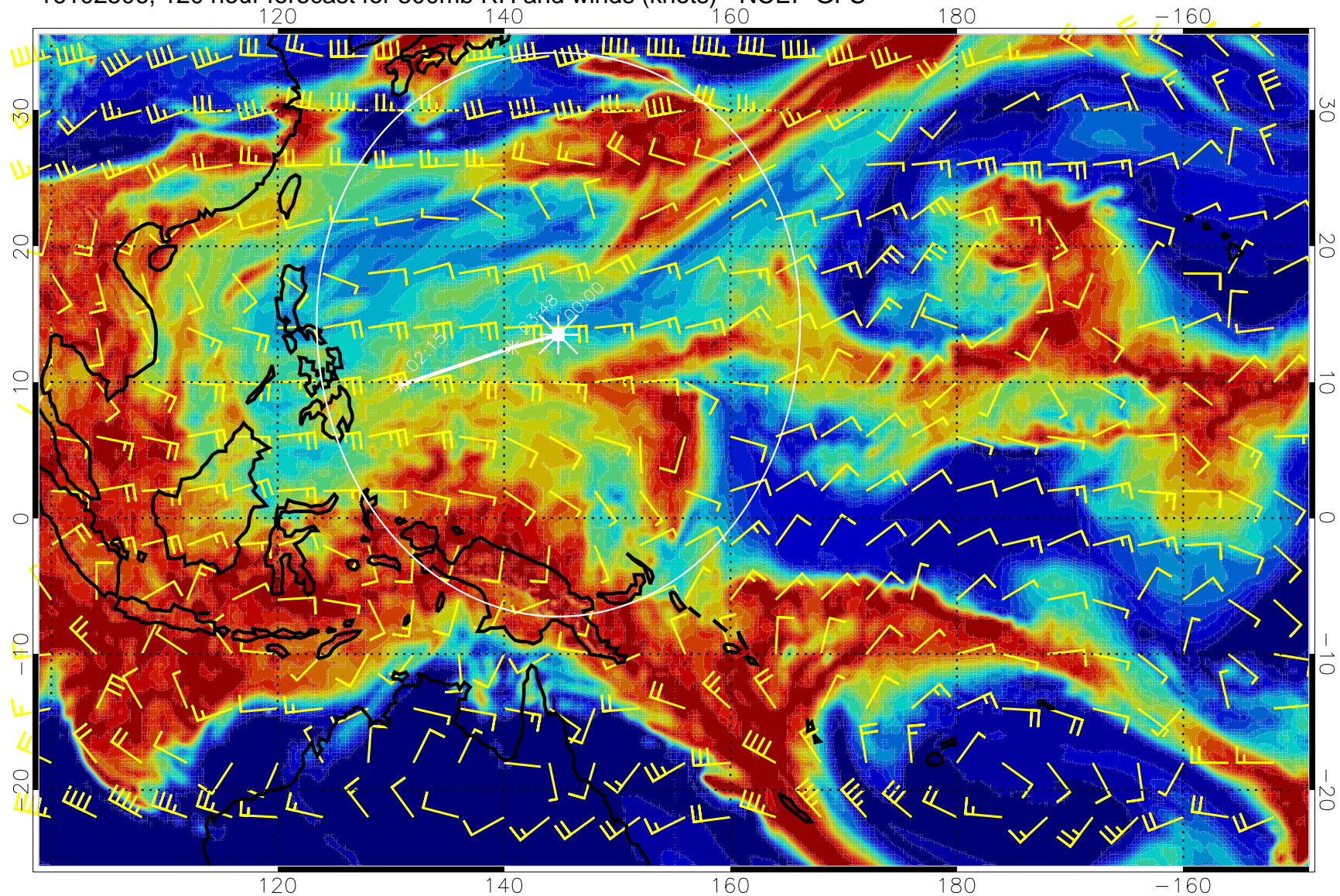
16102506, 120 hour forecast for 500mb RH and winds (knots) - NCEP GFS
