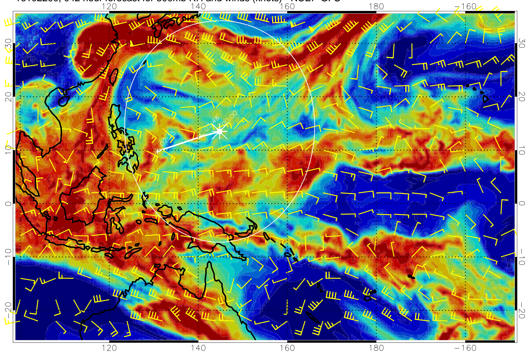
16102200, 042 hour forecast for 500mb RH and winds (knots) - NCEP GFS
