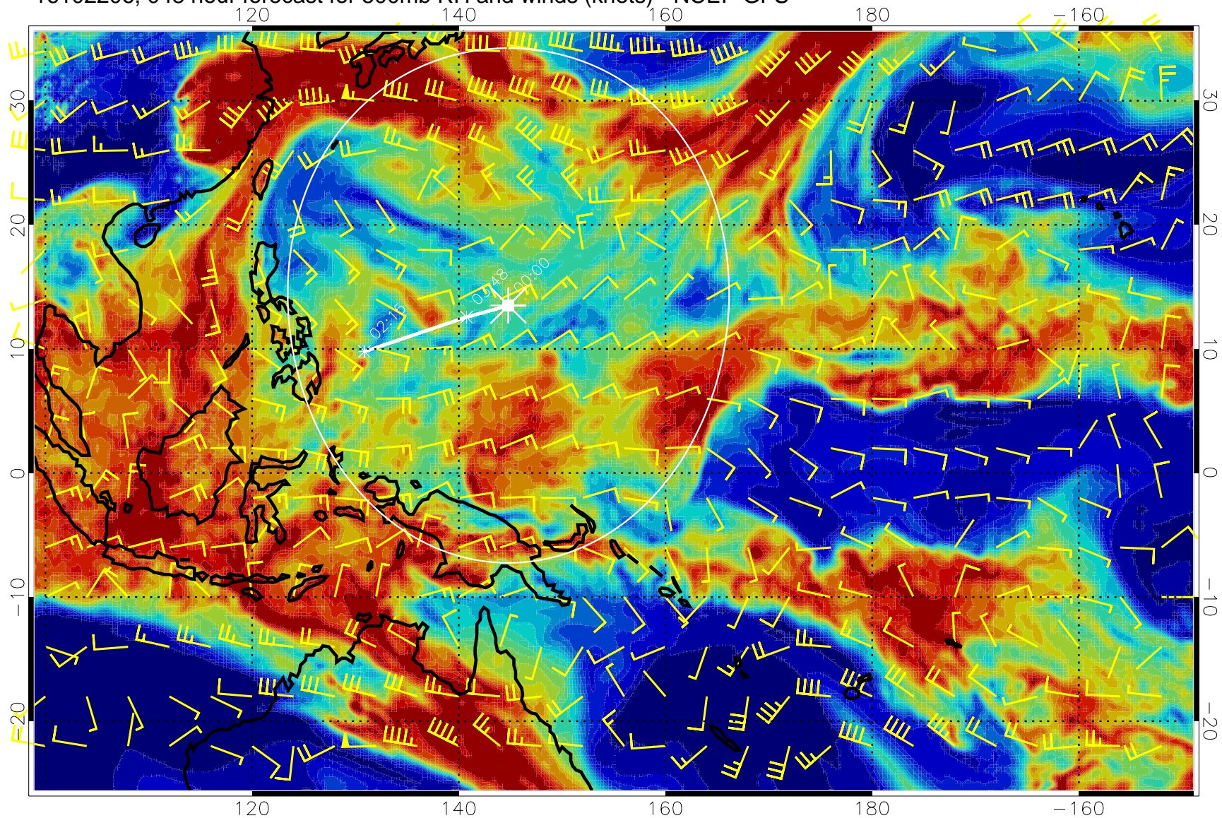
16102206, 048 hour forecast for 500mb RH and winds (knots) - NCEP GFS
