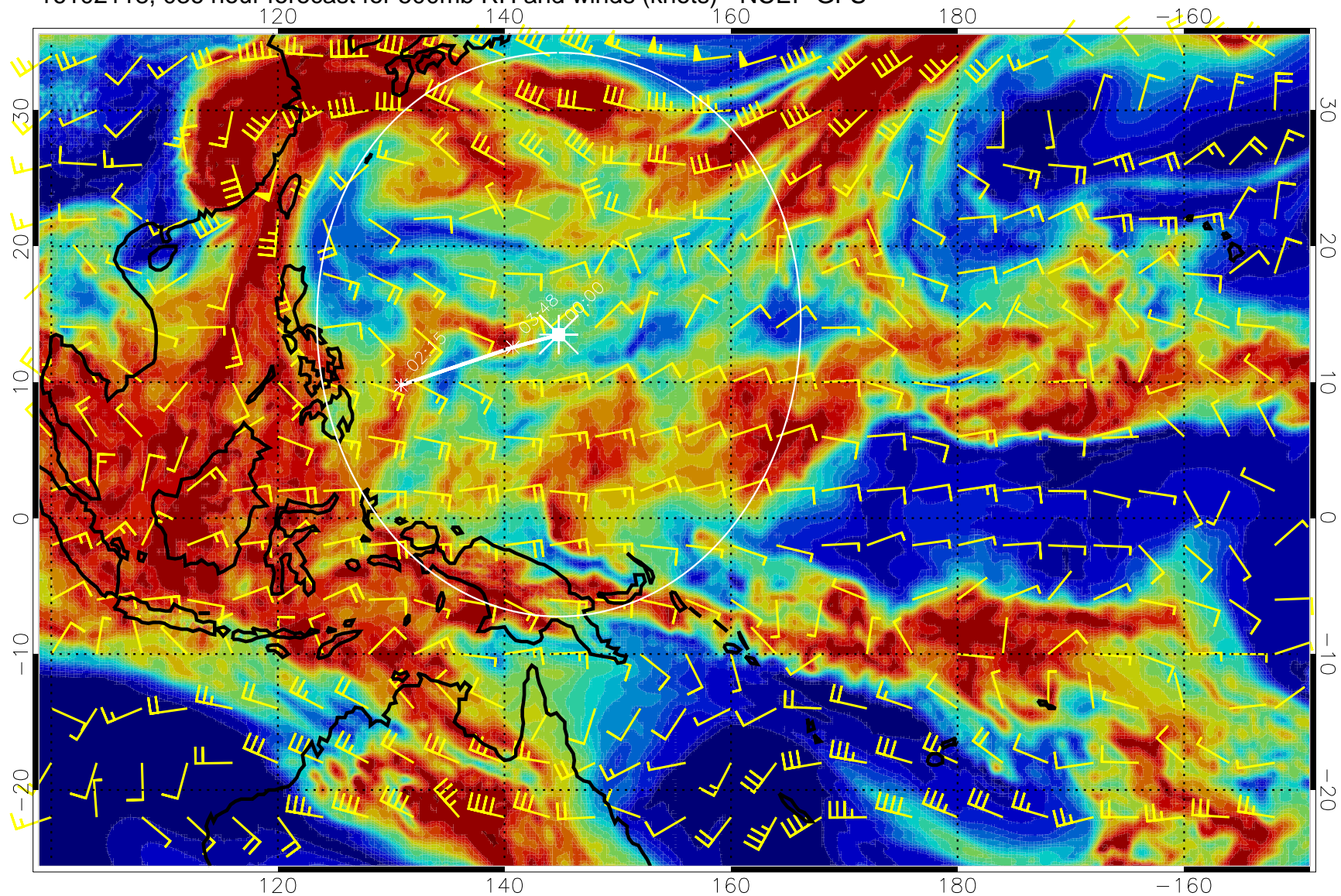
16102118, 036 hour forecast for 500mb RH and winds (knots) - NCEP GFS
