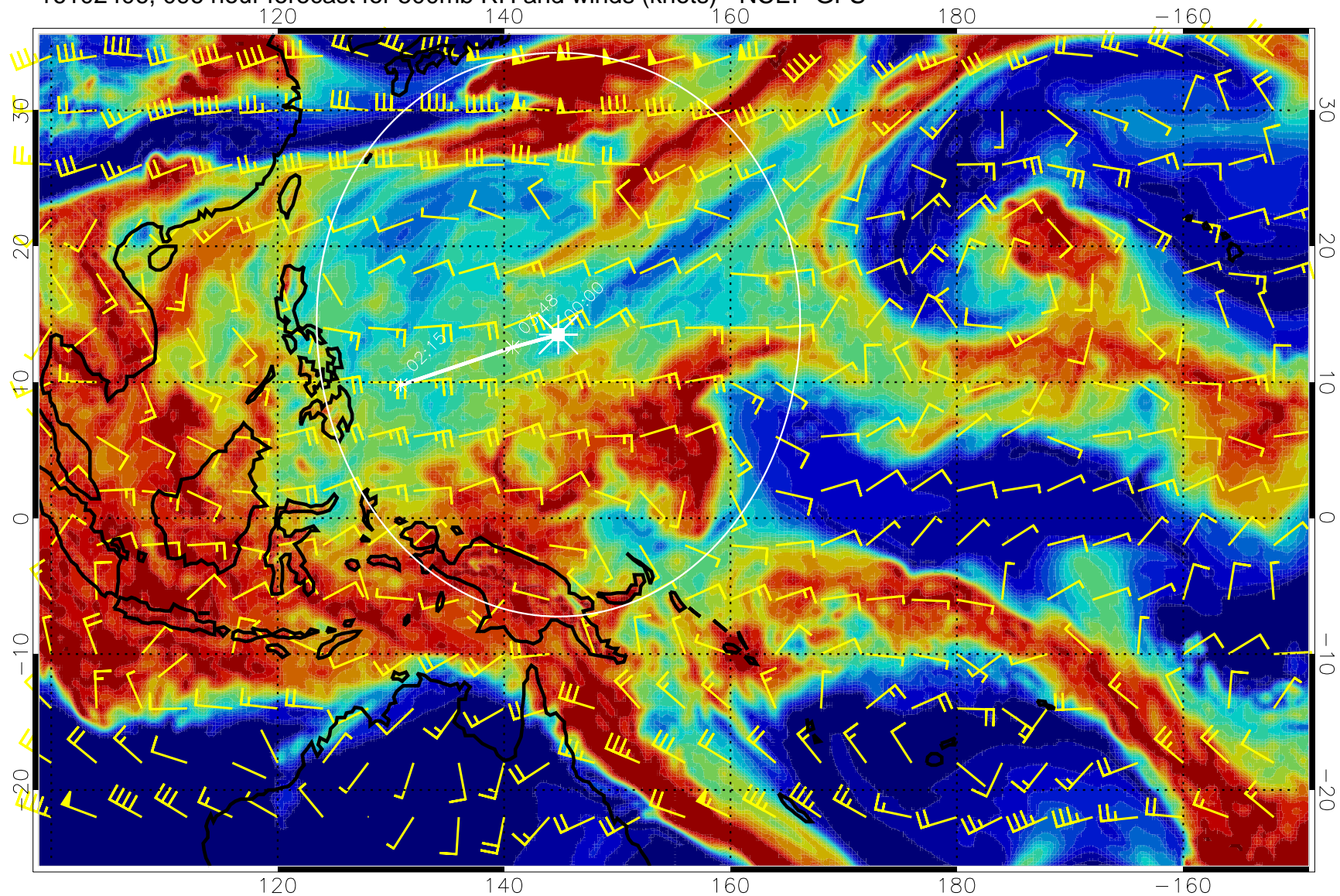
16102406, 096 hour forecast for 500mb RH and winds (knots) - NCEP GFS
