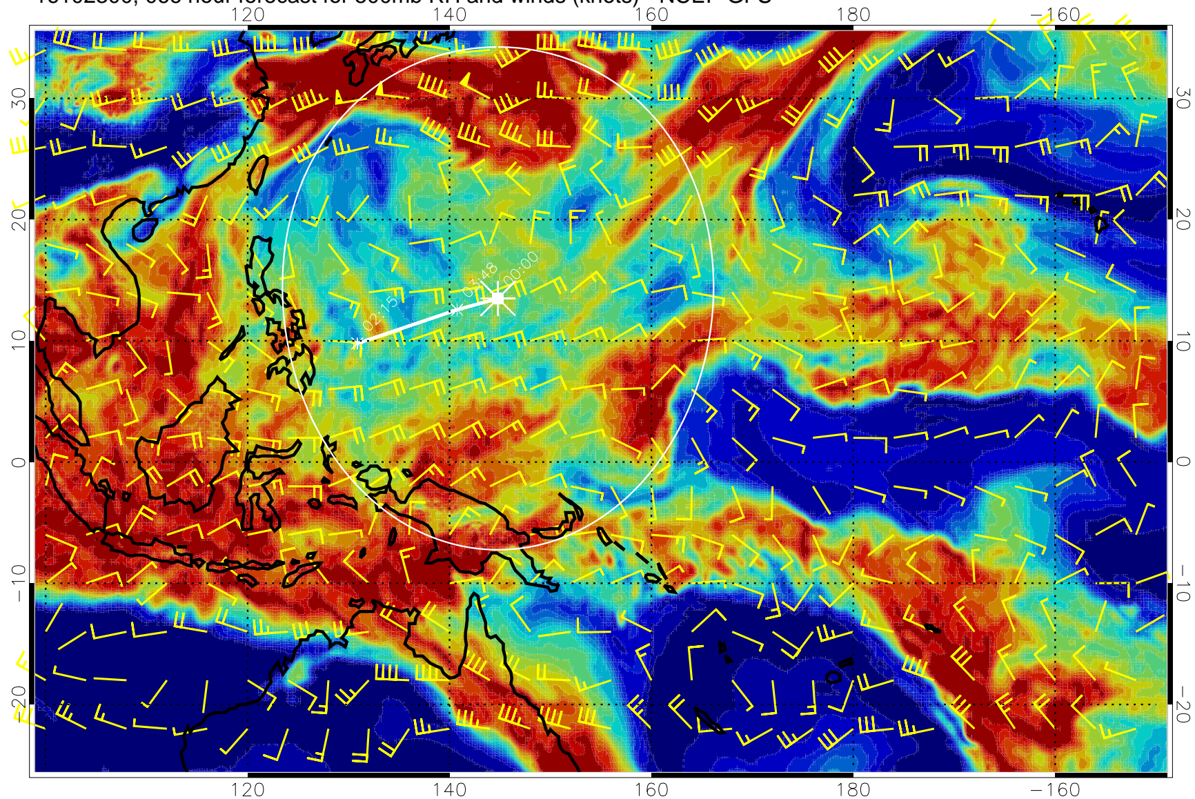
16102300, 066 hour forecast for 500mb RH and winds (knots) - NCEP GFS
