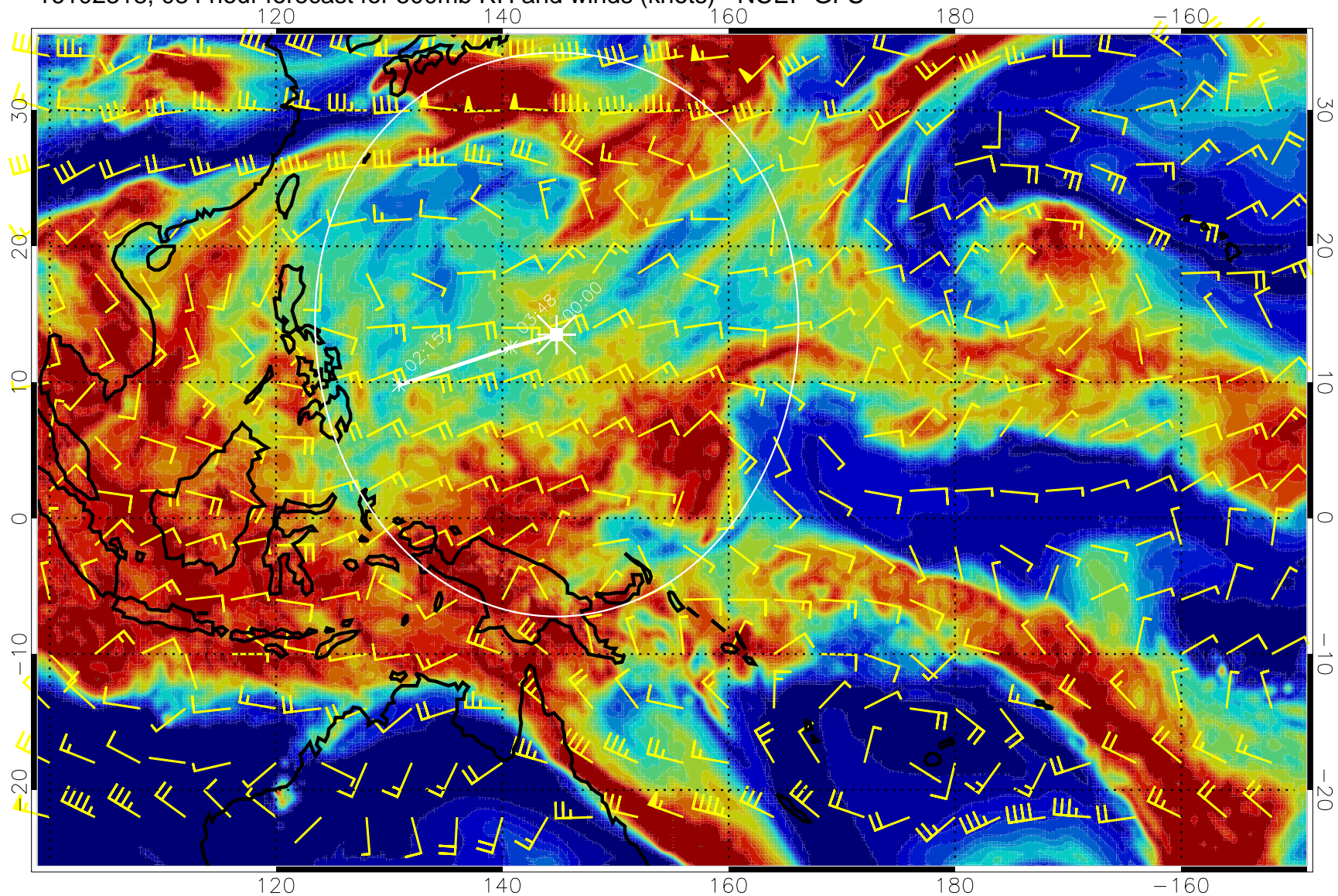
16102318, 084 hour forecast for 500mb RH and winds (knots) - NCEP GFS
