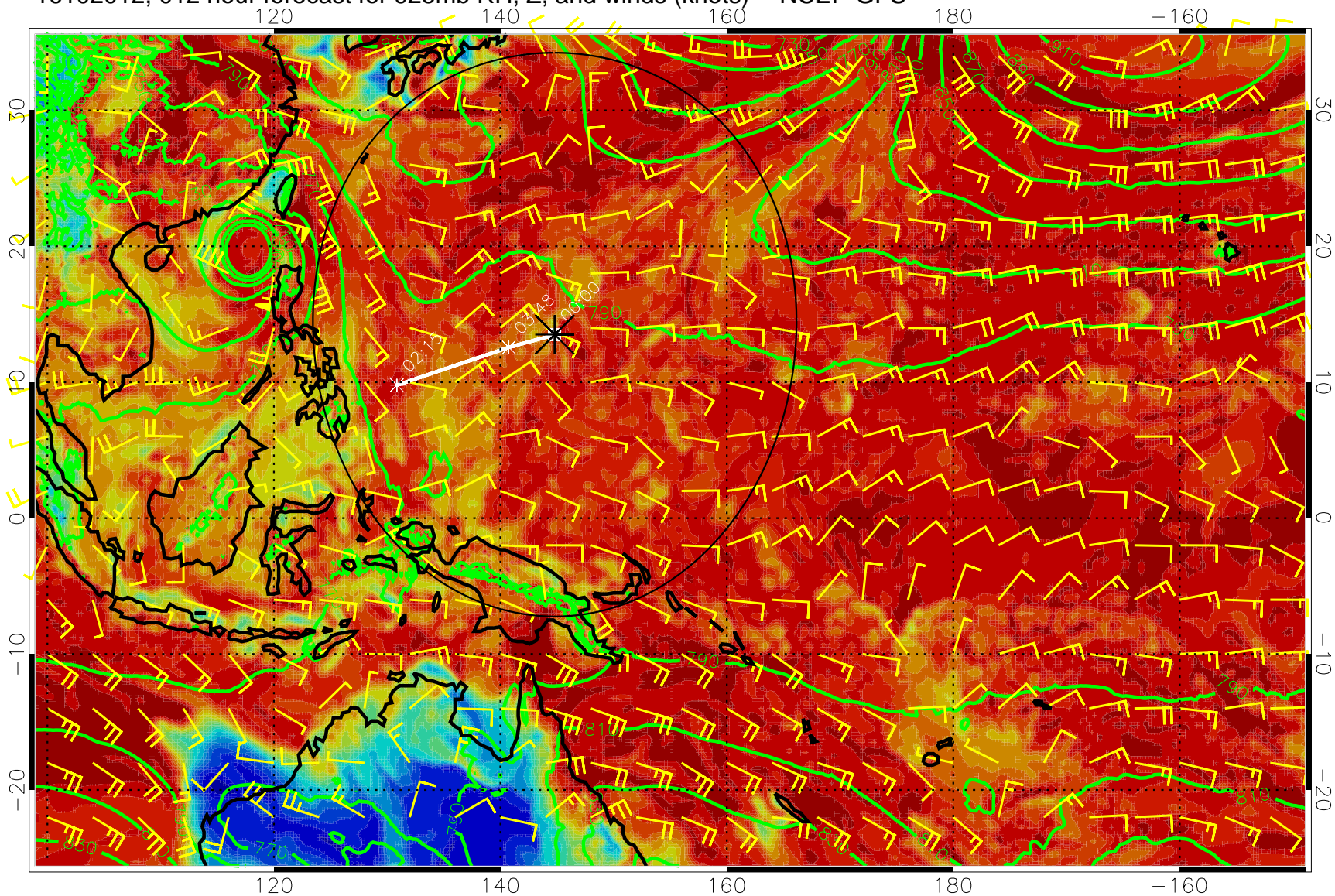
16102012, 012 hour forecast for 925mb RH, Z, and winds (knots) -- NCEP GFS
