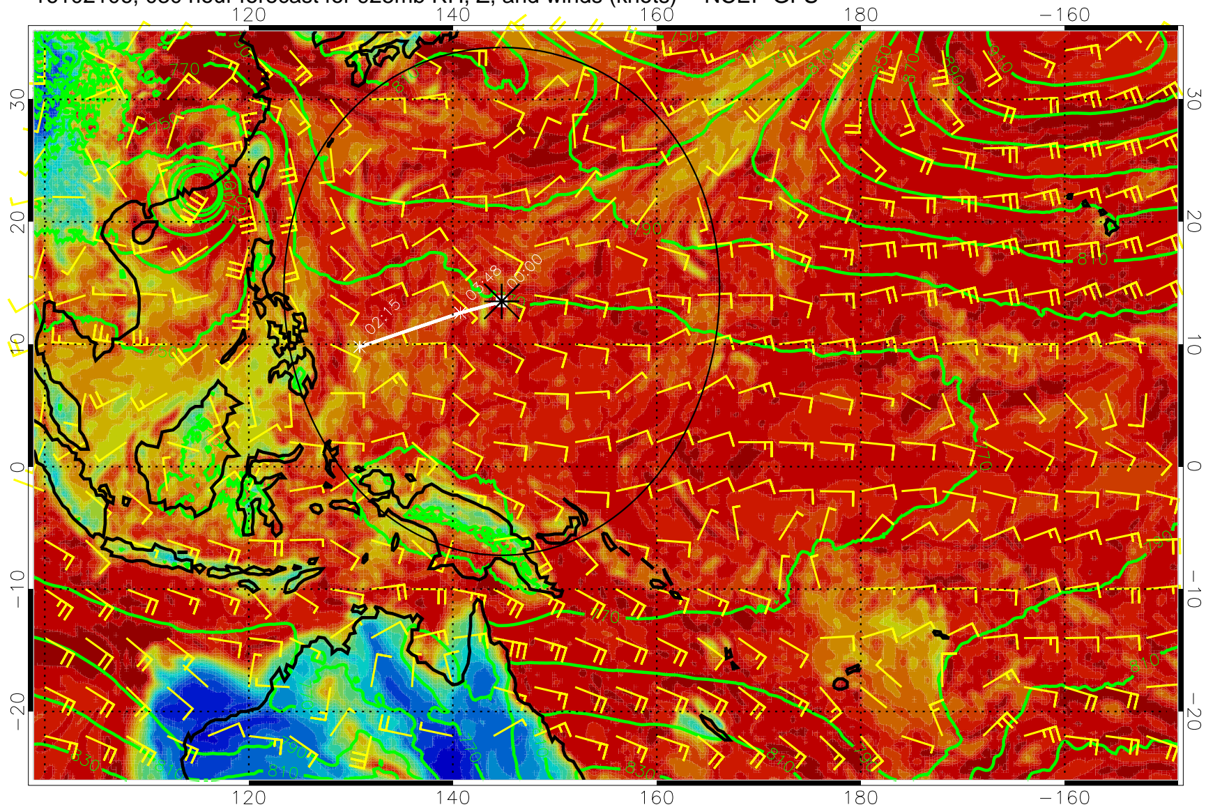
16102106, 030 hour forecast for 925mb RH, Z, and winds (knots) -- NCEP GFS
