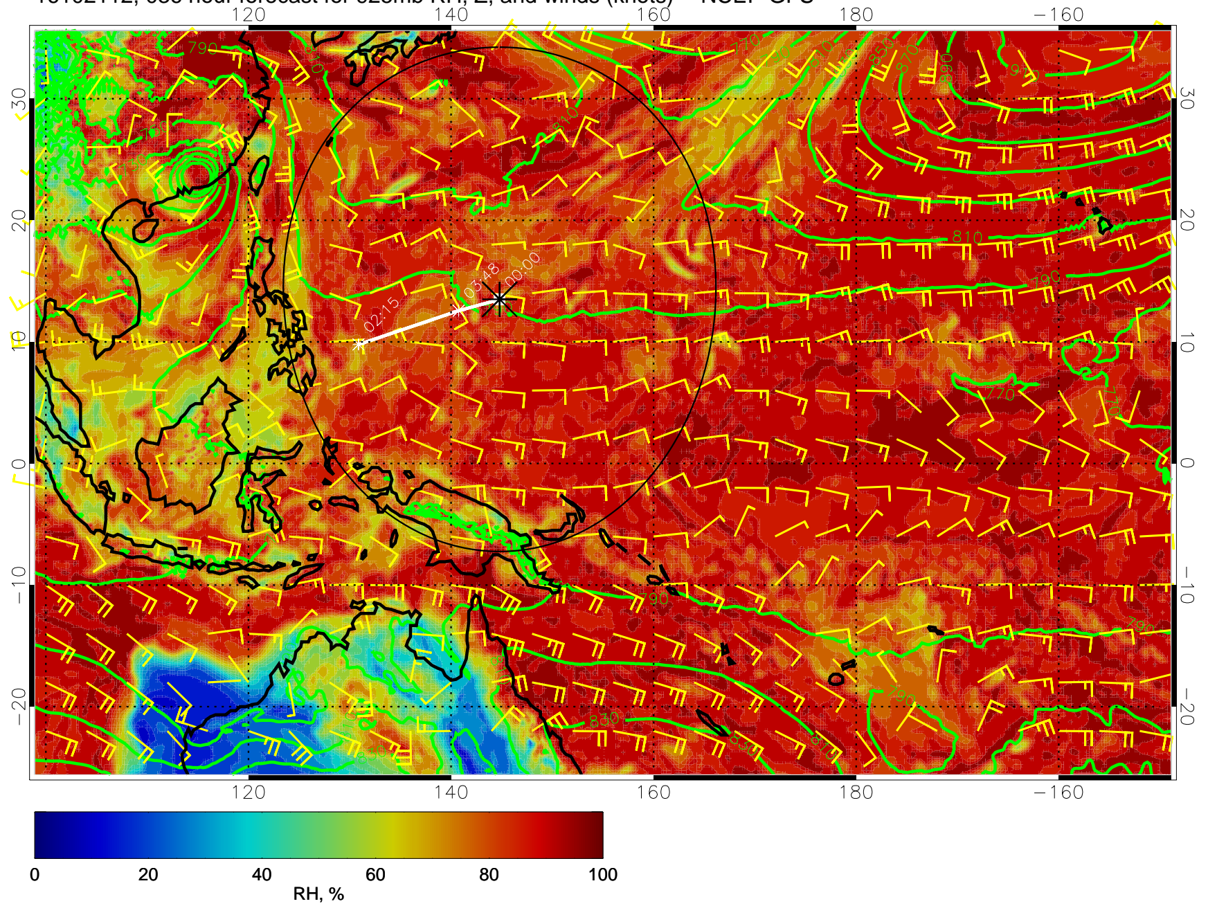
16102112, 036 hour forecast for 925mb RH, Z, and winds (knots) -- NCEP GFS
