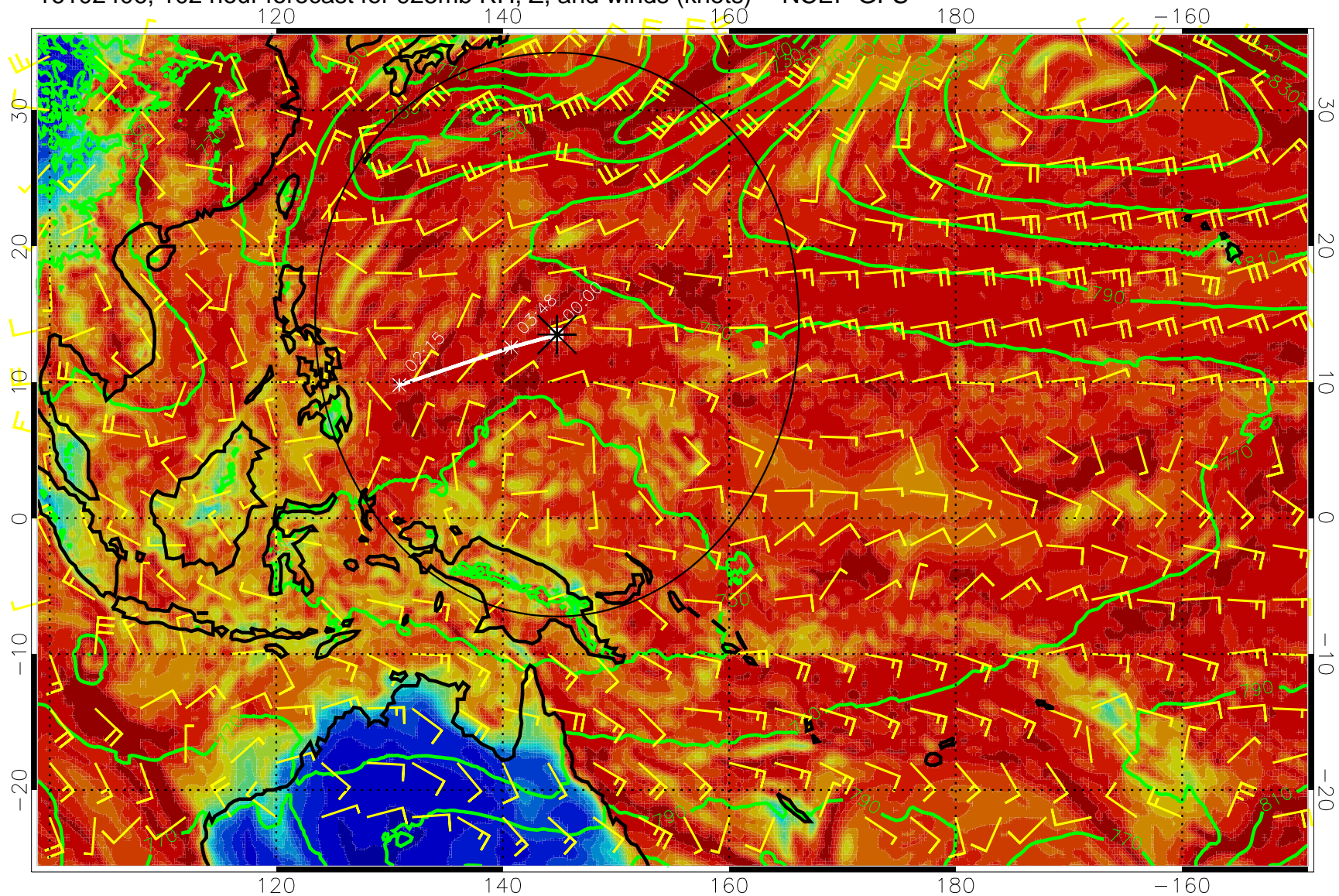
16102406, 102 hour forecast for 925mb RH, Z, and winds (knots) -- NCEP GFS
