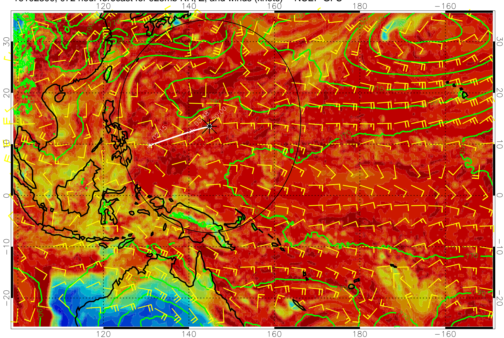
16102300, 072 hour forecast for 925mb RH, Z, and winds (knots) -- NCEP GFS
