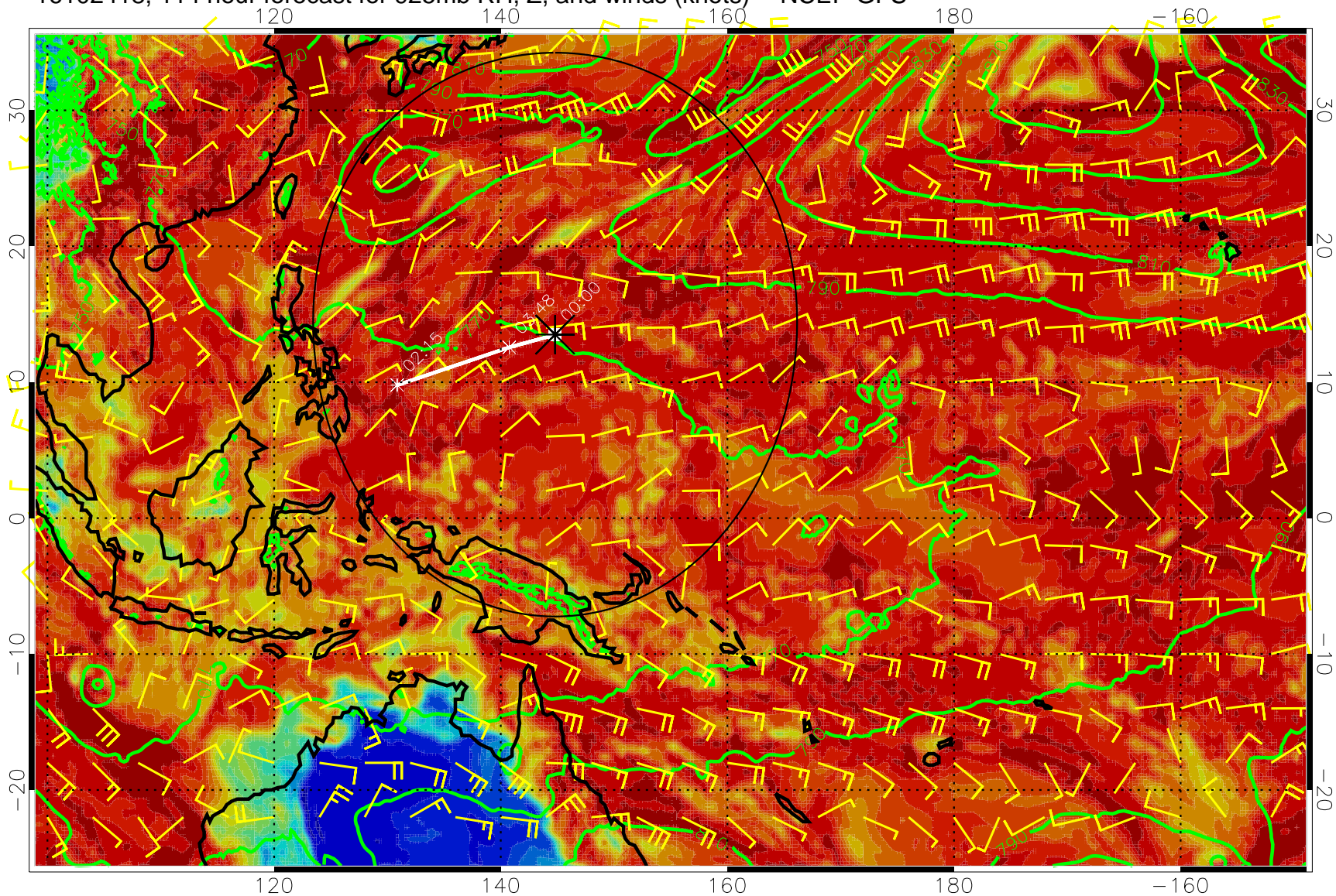
16102418, 114 hour forecast for 925mb RH, Z, and winds (knots) -- NCEP GFS
