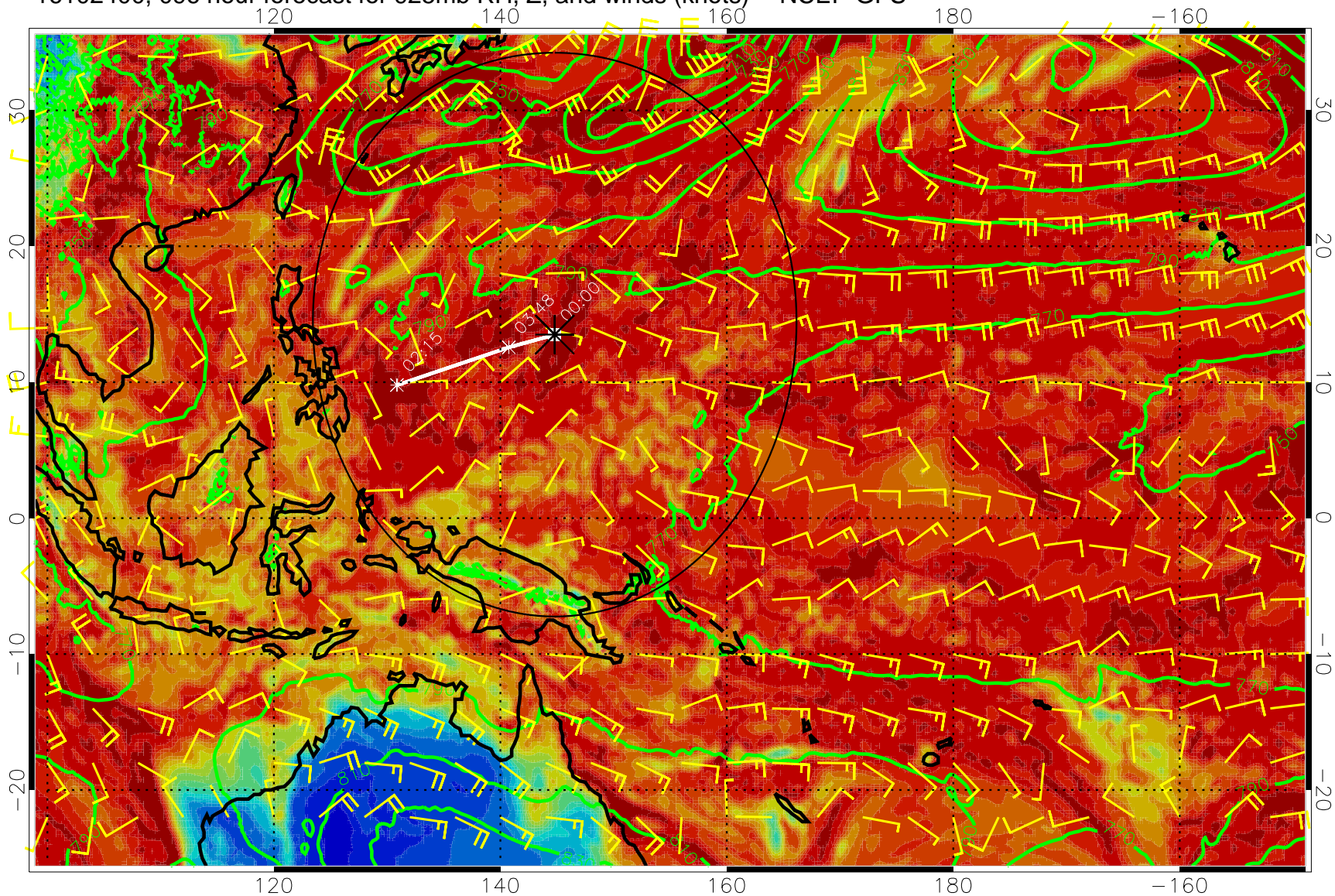
16102400, 096 hour forecast for 925mb RH, Z, and winds (knots) -- NCEP GFS
