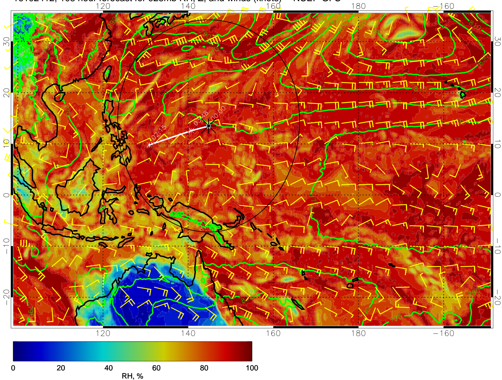
16102412, 108 hour forecast for 925mb RH, Z, and winds (knots) -- NCEP GFS
