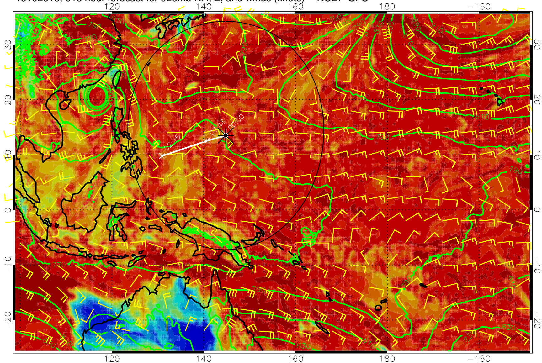
16102018, 018 hour forecast for 925mb RH, Z, and winds (knots) -- NCEP GFS
