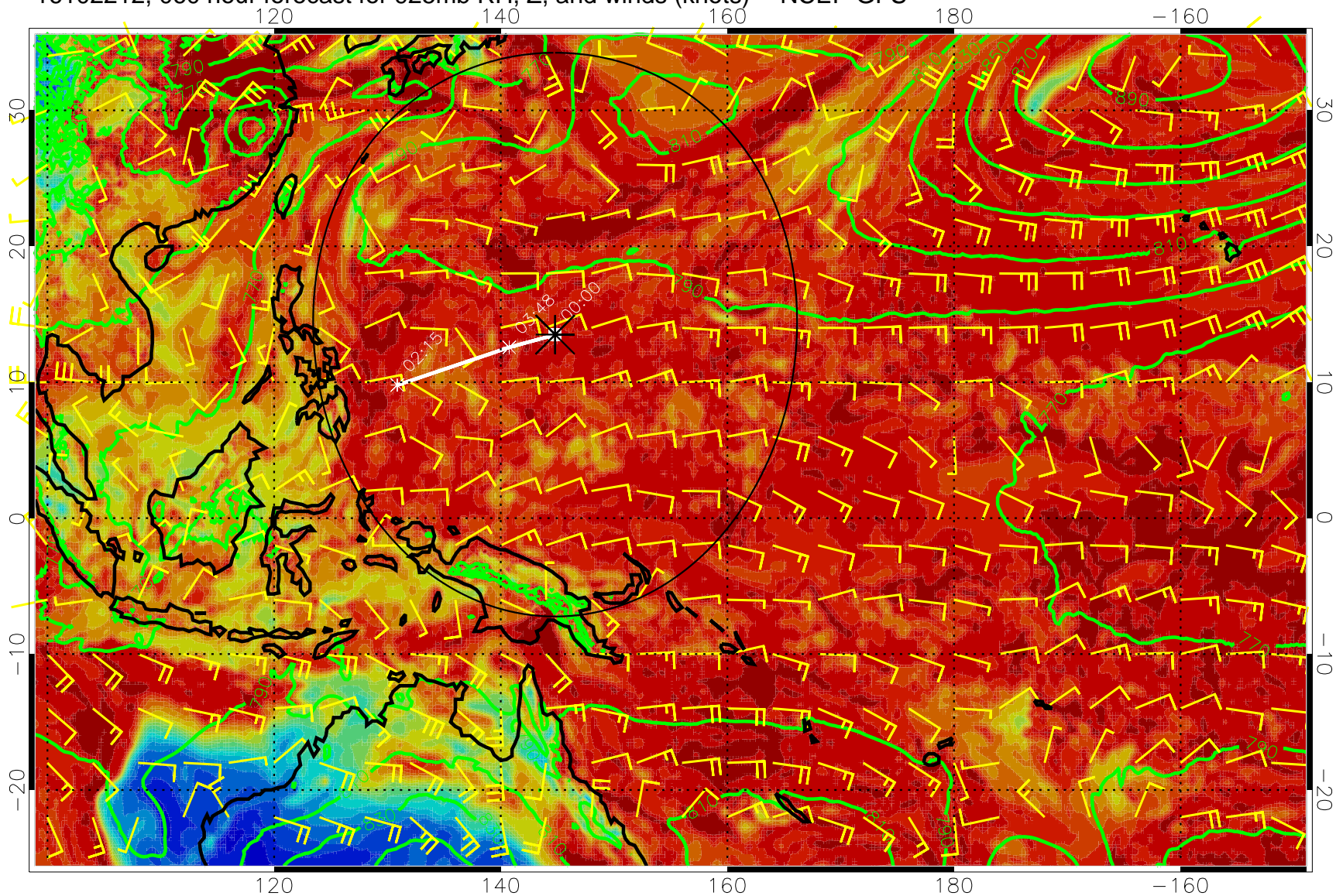
16102212, 060 hour forecast for 925mb RH, Z, and winds (knots) -- NCEP GFS
