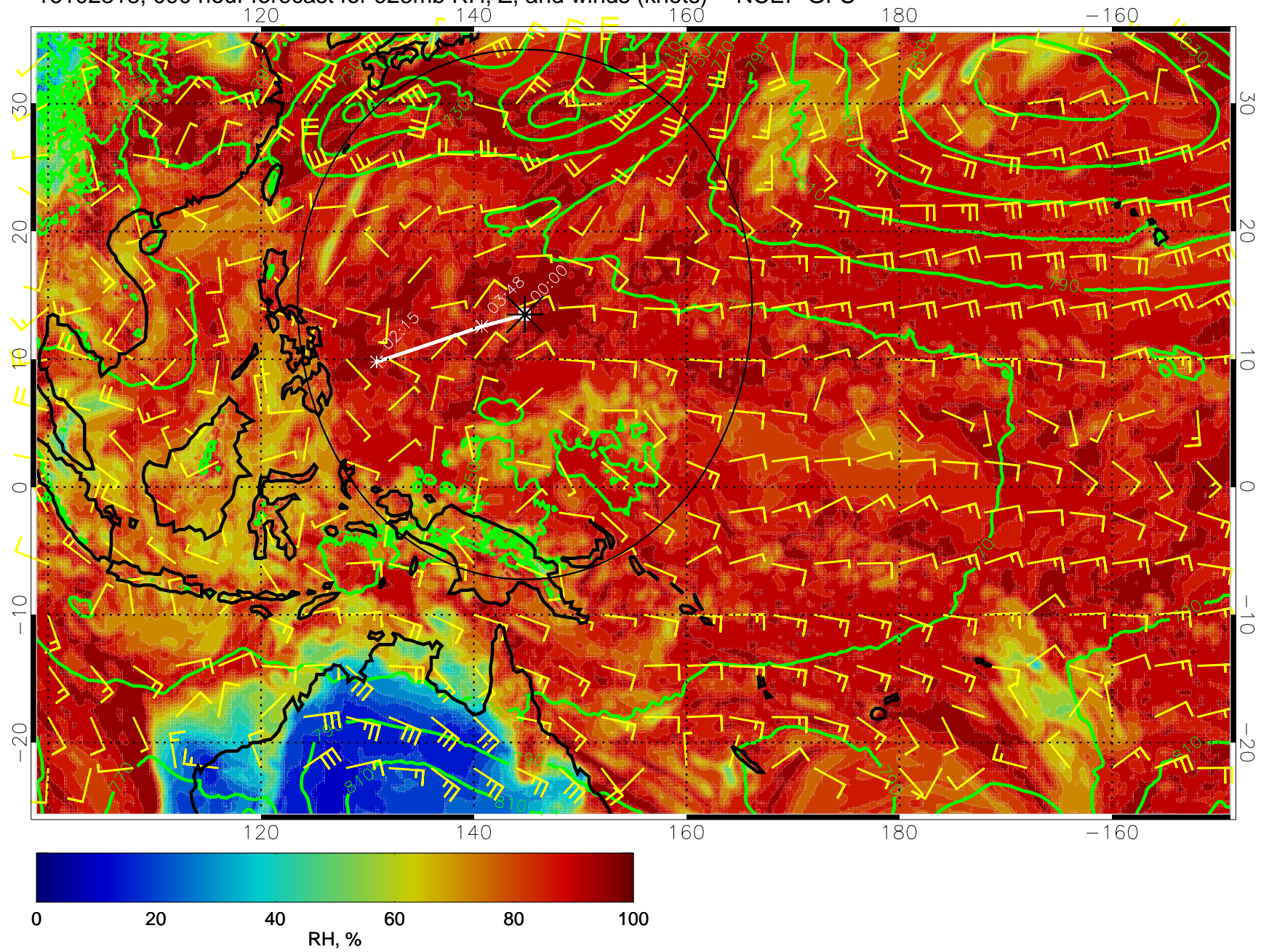
16102318, 090 hour forecast for 925mb RH, Z, and winds (knots) -- NCEP GFS
