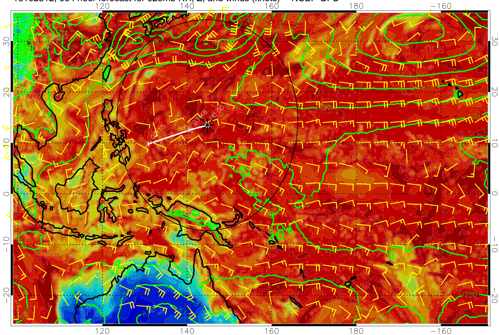
16102312, 084 hour forecast for 925mb RH, Z, and winds (knots) -- NCEP GFS
