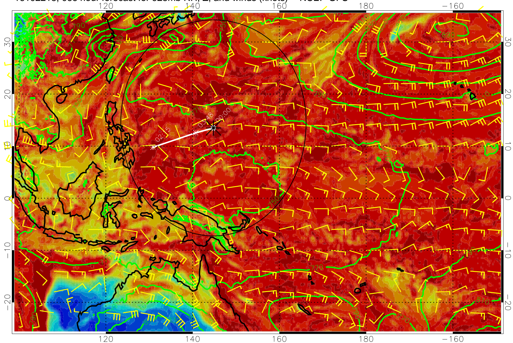
16102218, 066 hour forecast for 925mb RH, Z, and winds (knots) -- NCEP GFS
