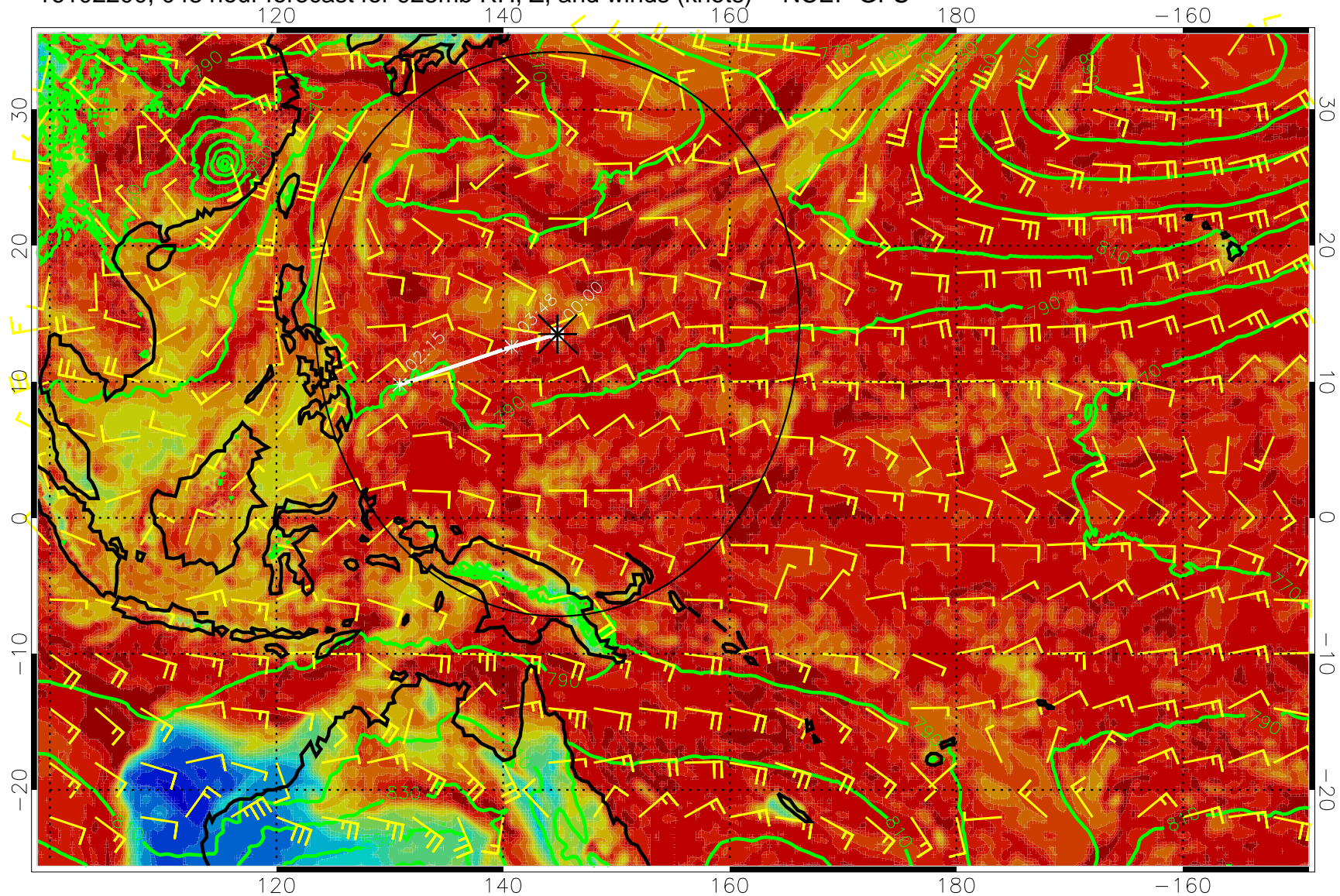
16102200, 048 hour forecast for 925mb RH, Z, and winds (knots) -- NCEP GFS
