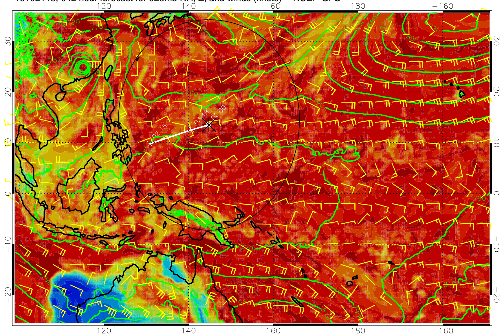
16102118, 042 hour forecast for 925mb RH, Z, and winds (knots) -- NCEP GFS
