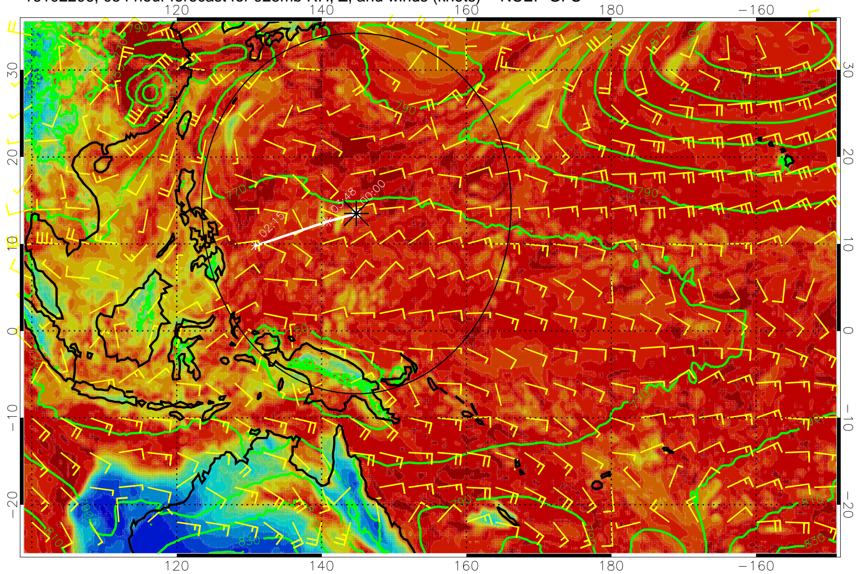
16102206, 054 hour forecast for 925mb RH, Z, and winds (knots) -- NCEP GFS
