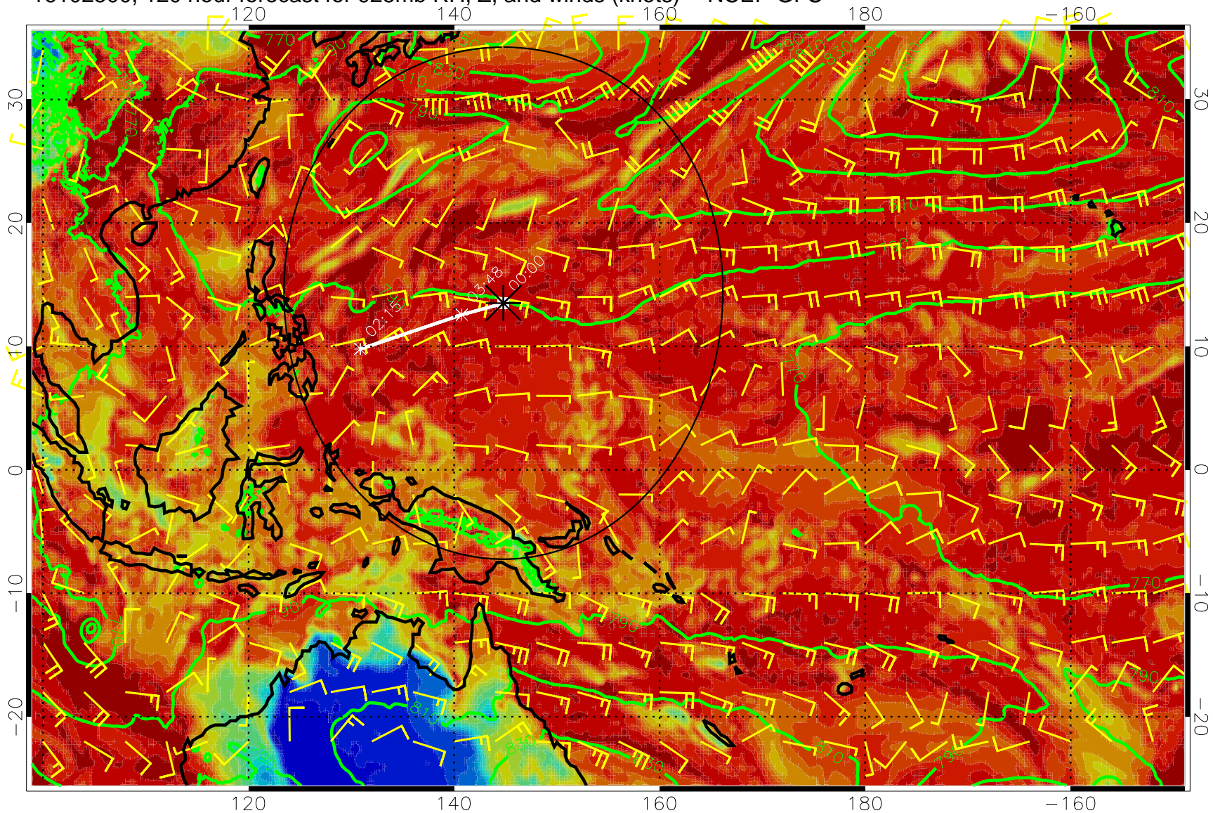
16102500, 120 hour forecast for 925mb RH, Z, and winds (knots) -- NCEP GFS
