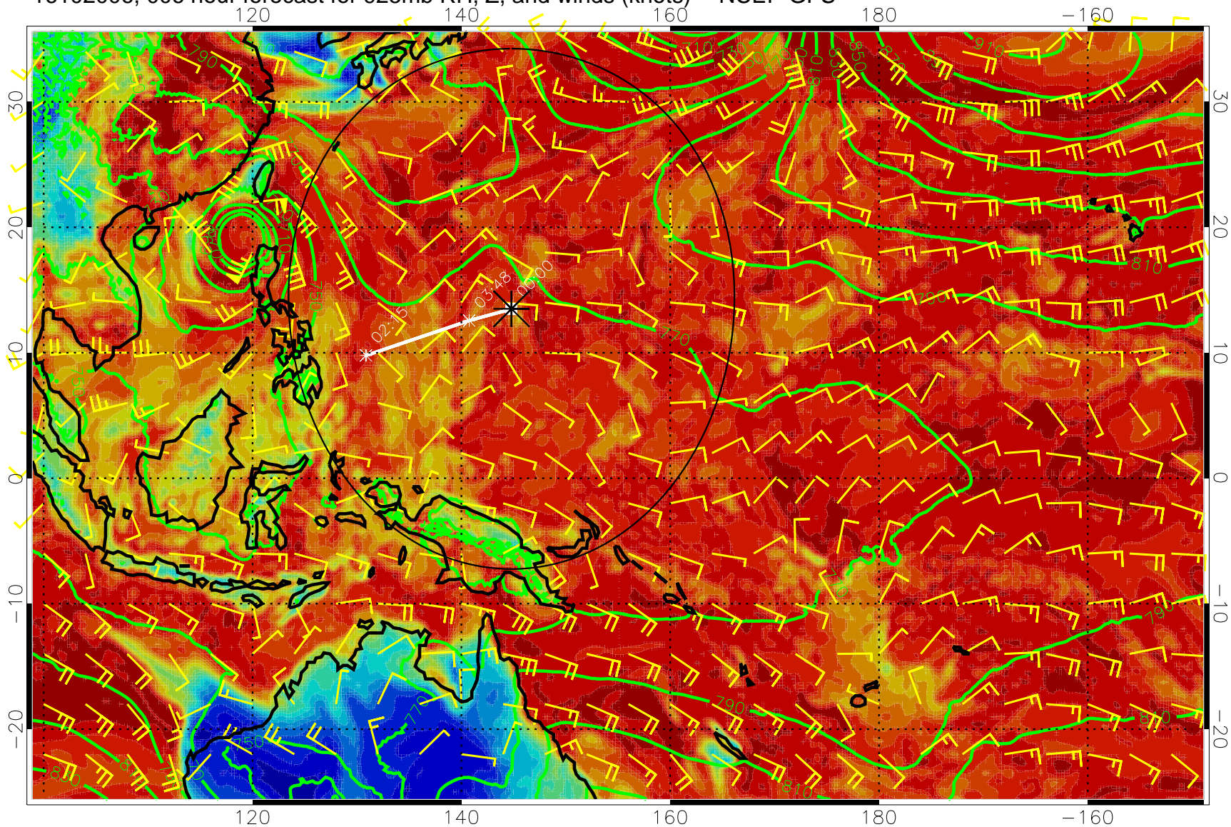
16102006, 006 hour forecast for 925mb RH, Z, and winds (knots) -- NCEP GFS
