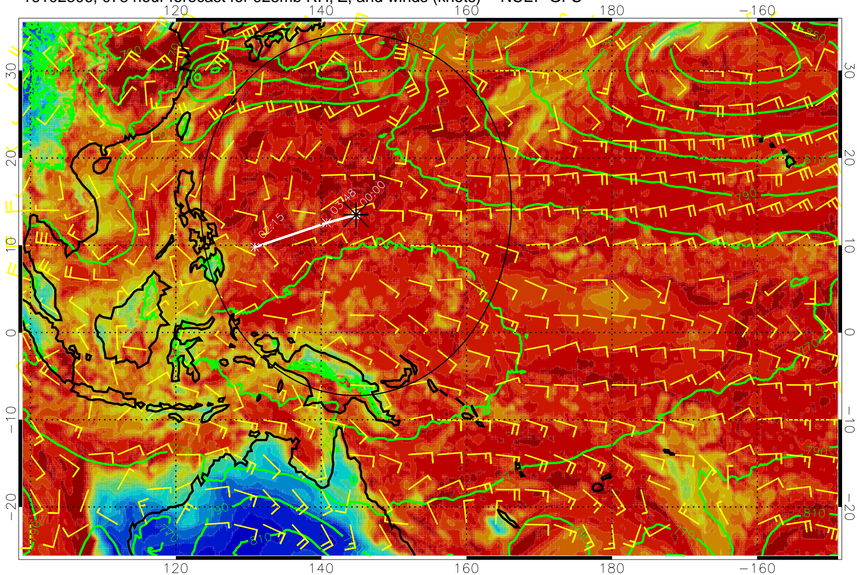
16102306, 078 hour forecast for 925mb RH, Z, and winds (knots) -- NCEP GFS
