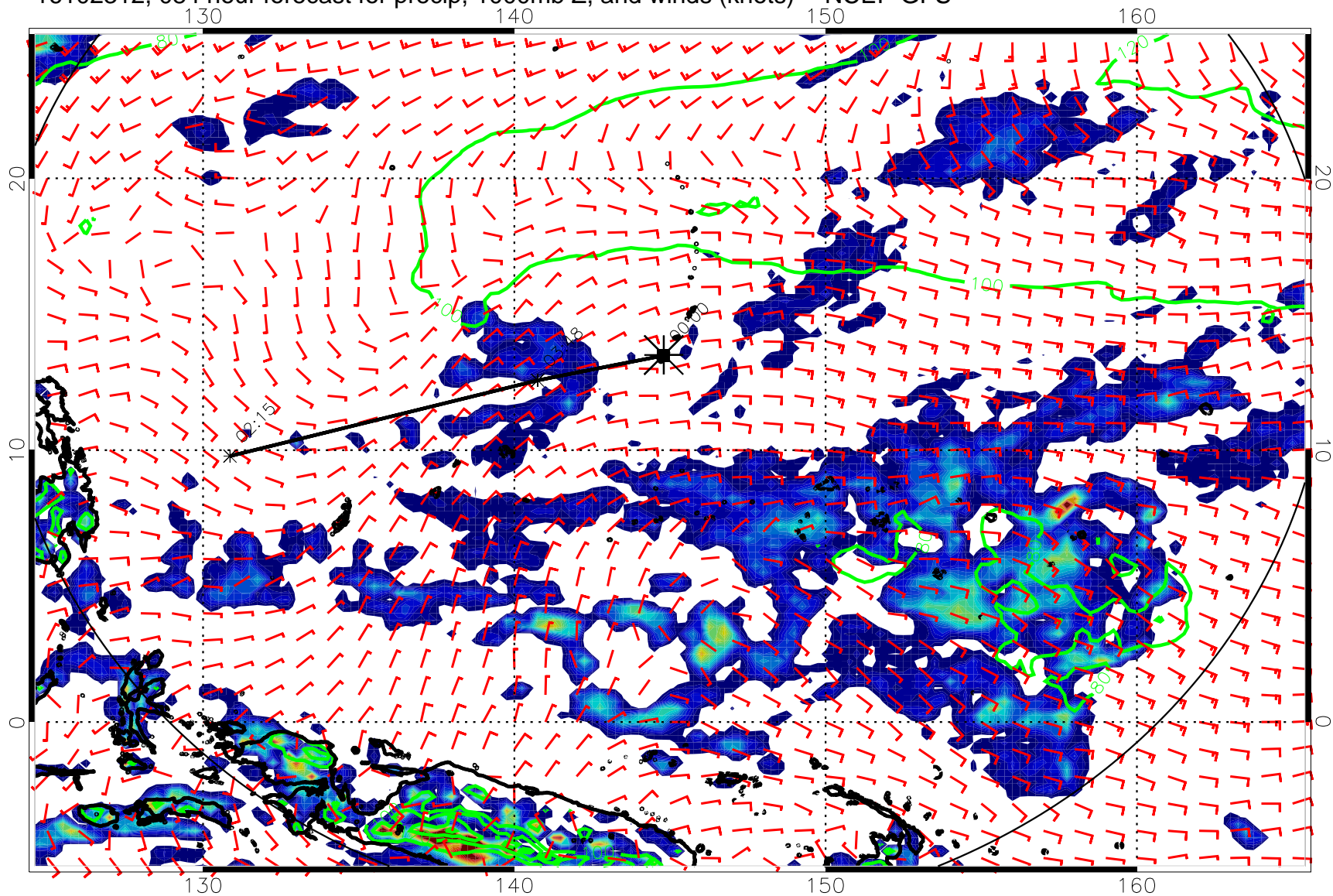
16102312, 084 hour forecast for precip, 1000mb Z, and winds (knots) -- NCEP GFS
