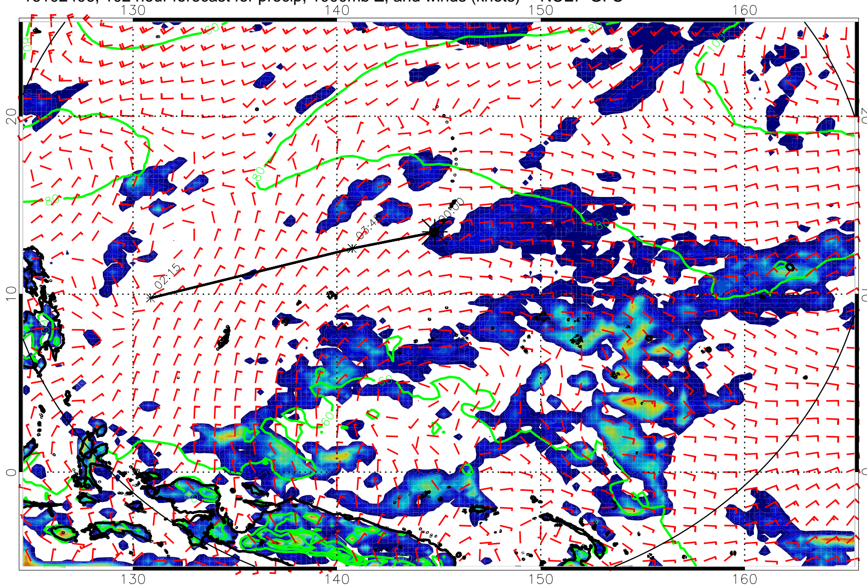
16102406, 102 hour forecast for precip, 1000mb Z, and winds (knots) -- NCEP GFS
