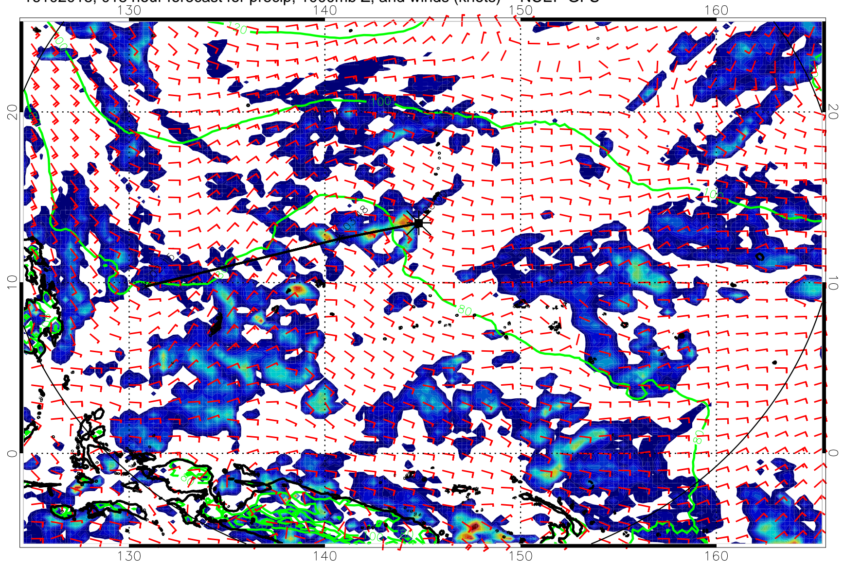
16102018, 018 hour forecast for precip, 1000mb Z, and winds (knots) -- NCEP GFS
