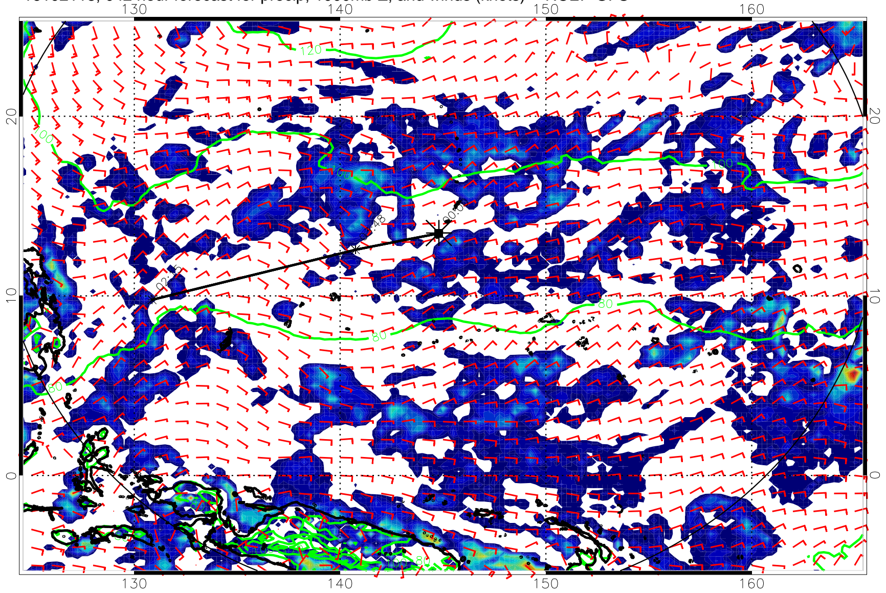
16102118, 042 hour forecast for precip, 1000mb Z, and winds (knots) -- NCEP GFS
