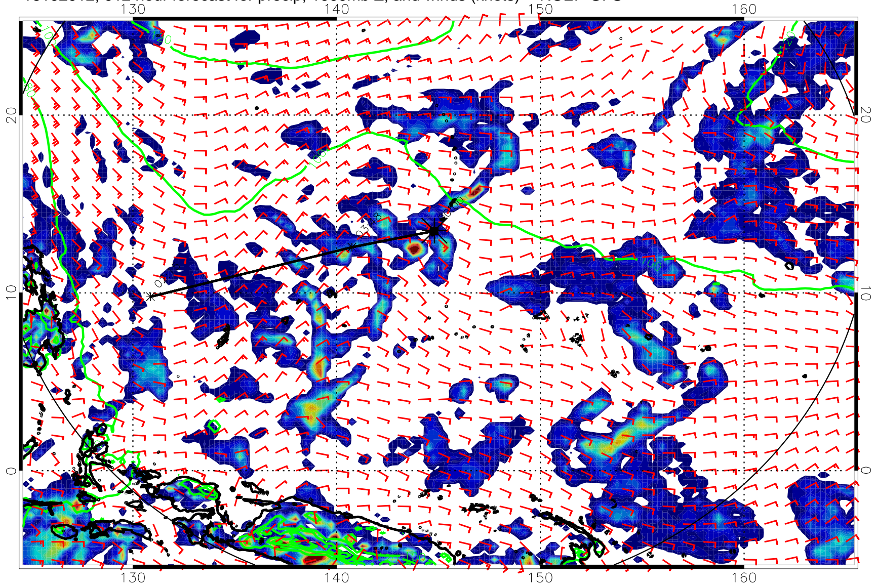
16102012, 012 hour forecast for precip, 1000mb Z, and winds (knots) -- NCEP GFS
