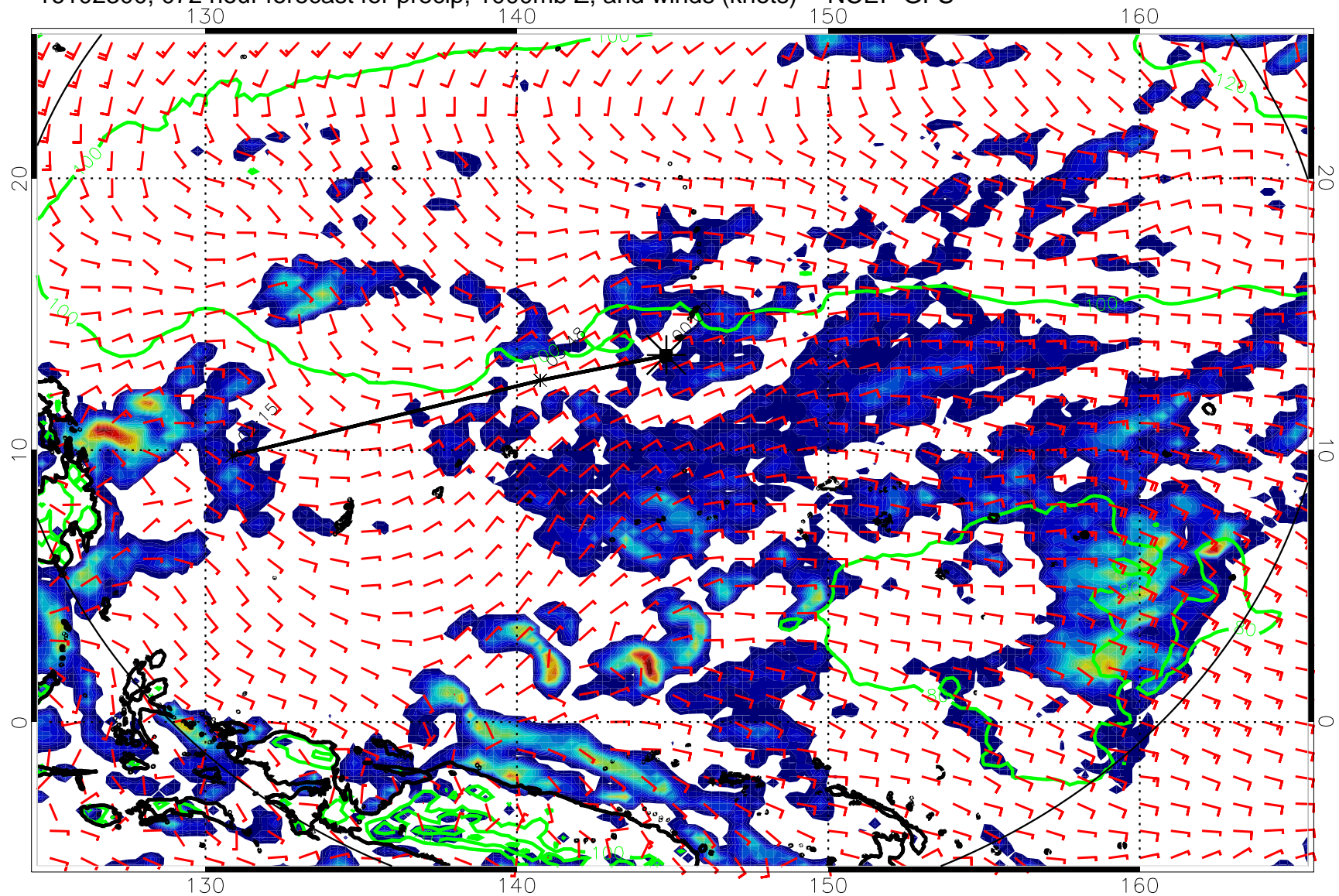
16102300, 072 hour forecast for precip, 1000mb Z, and winds (knots) -- NCEP GFS
