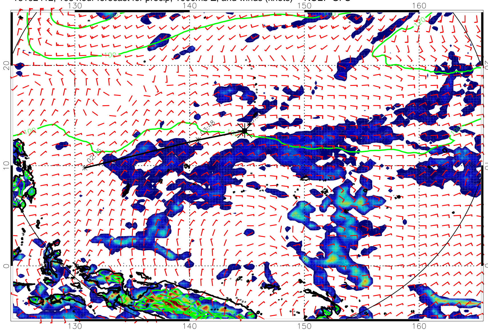
16102412, 108 hour forecast for precip, 1000mb Z, and winds (knots) -- NCEP GFS
