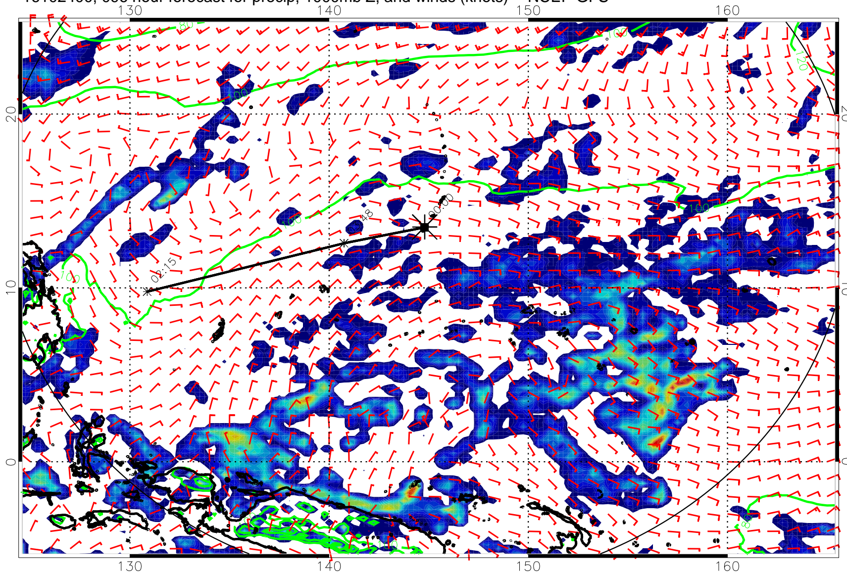
16102400, 096 hour forecast for precip, 1000mb Z, and winds (knots) -- NCEP GFS
