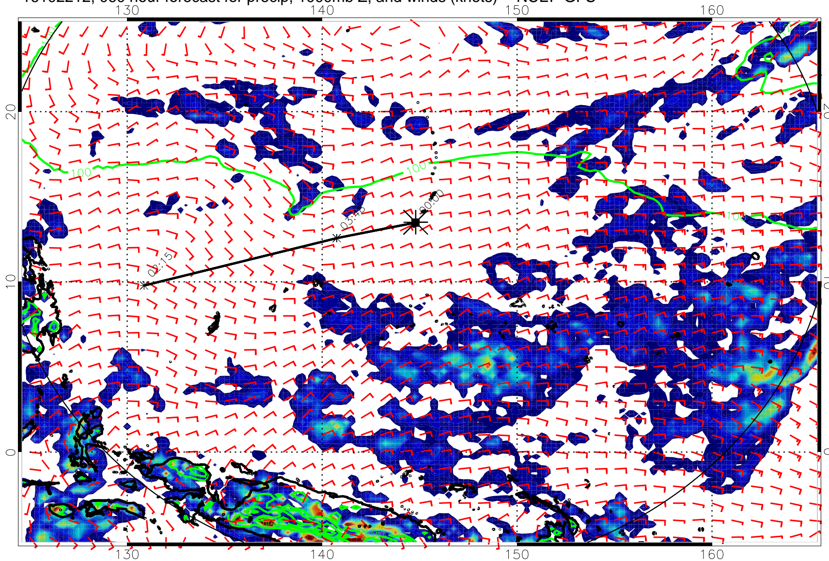
16102212, 060 hour forecast for precip, 1000mb Z, and winds (knots) -- NCEP GFS
