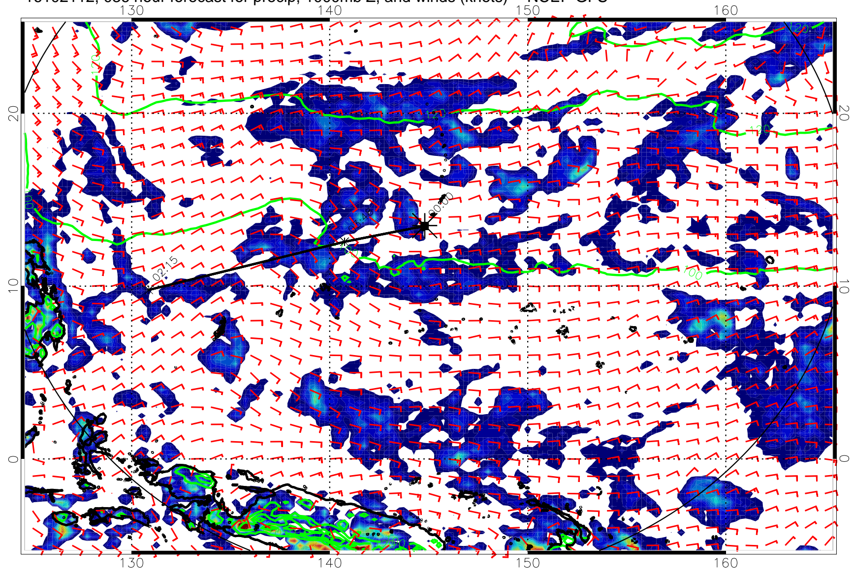
16102112, 036 hour forecast for precip, 1000mb Z, and winds (knots) -- NCEP GFS
