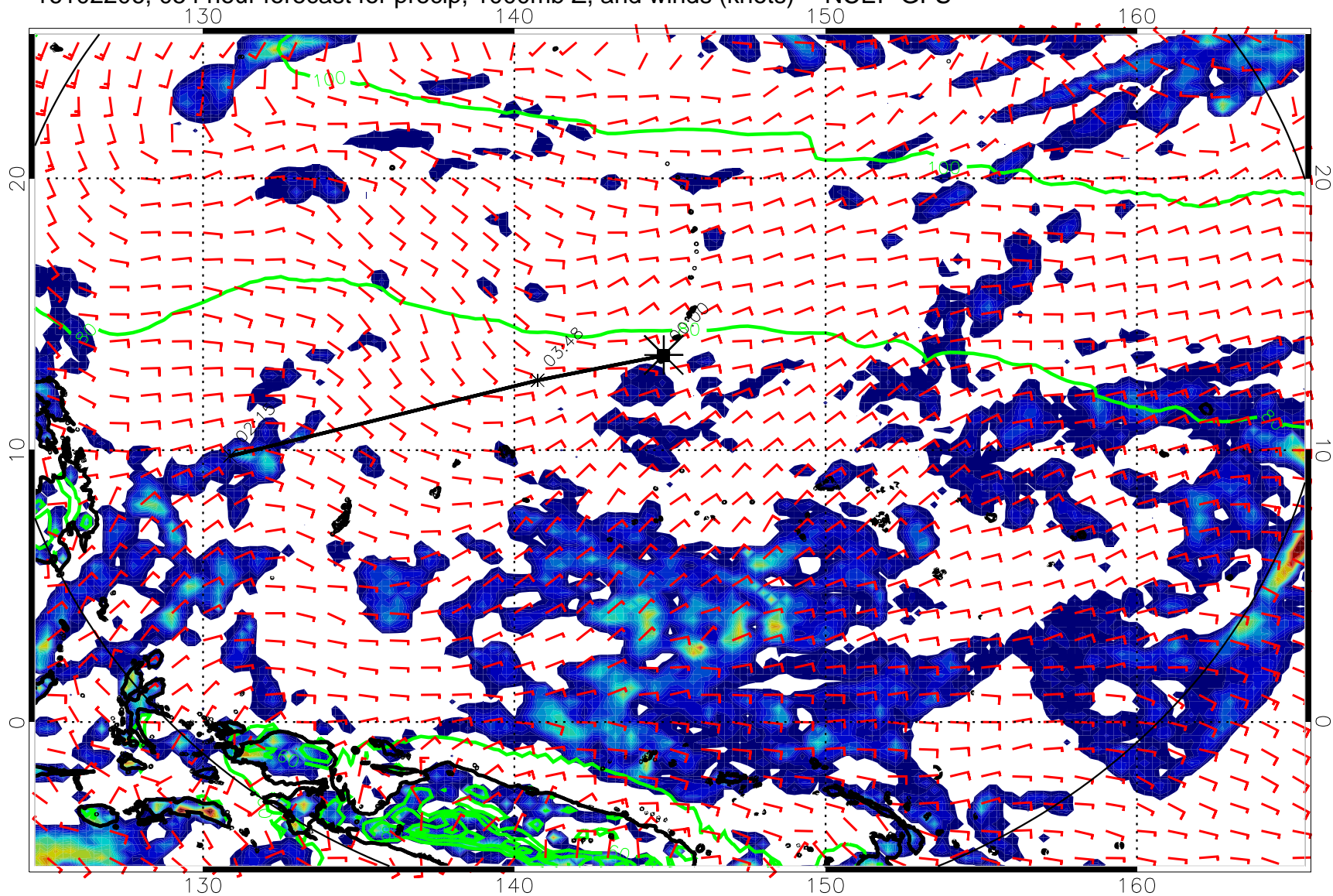
16102206, 054 hour forecast for precip, 1000mb Z, and winds (knots) -- NCEP GFS
