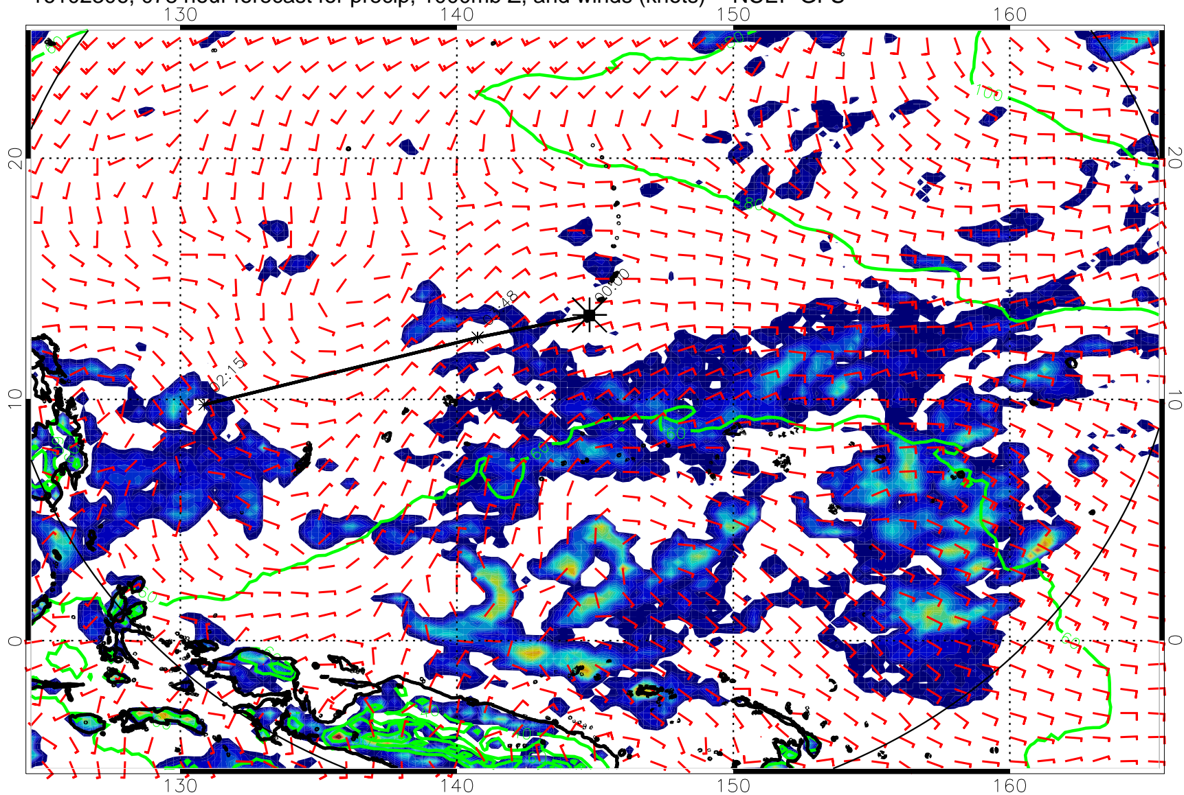
16102306, 078 hour forecast for precip, 1000mb Z, and winds (knots) -- NCEP GFS
