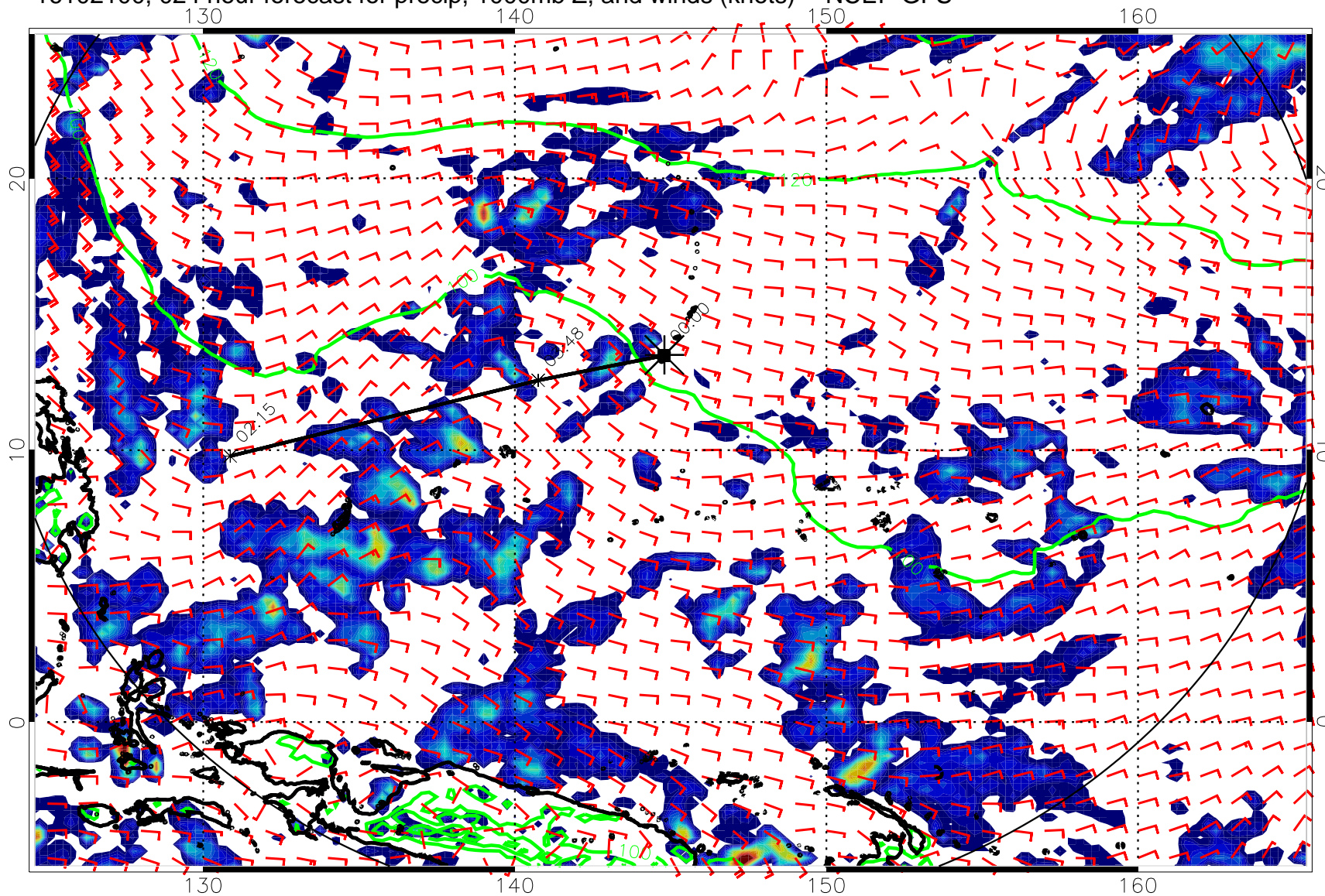
16102100, 024 hour forecast for precip, 1000mb Z, and winds (knots) -- NCEP GFS
