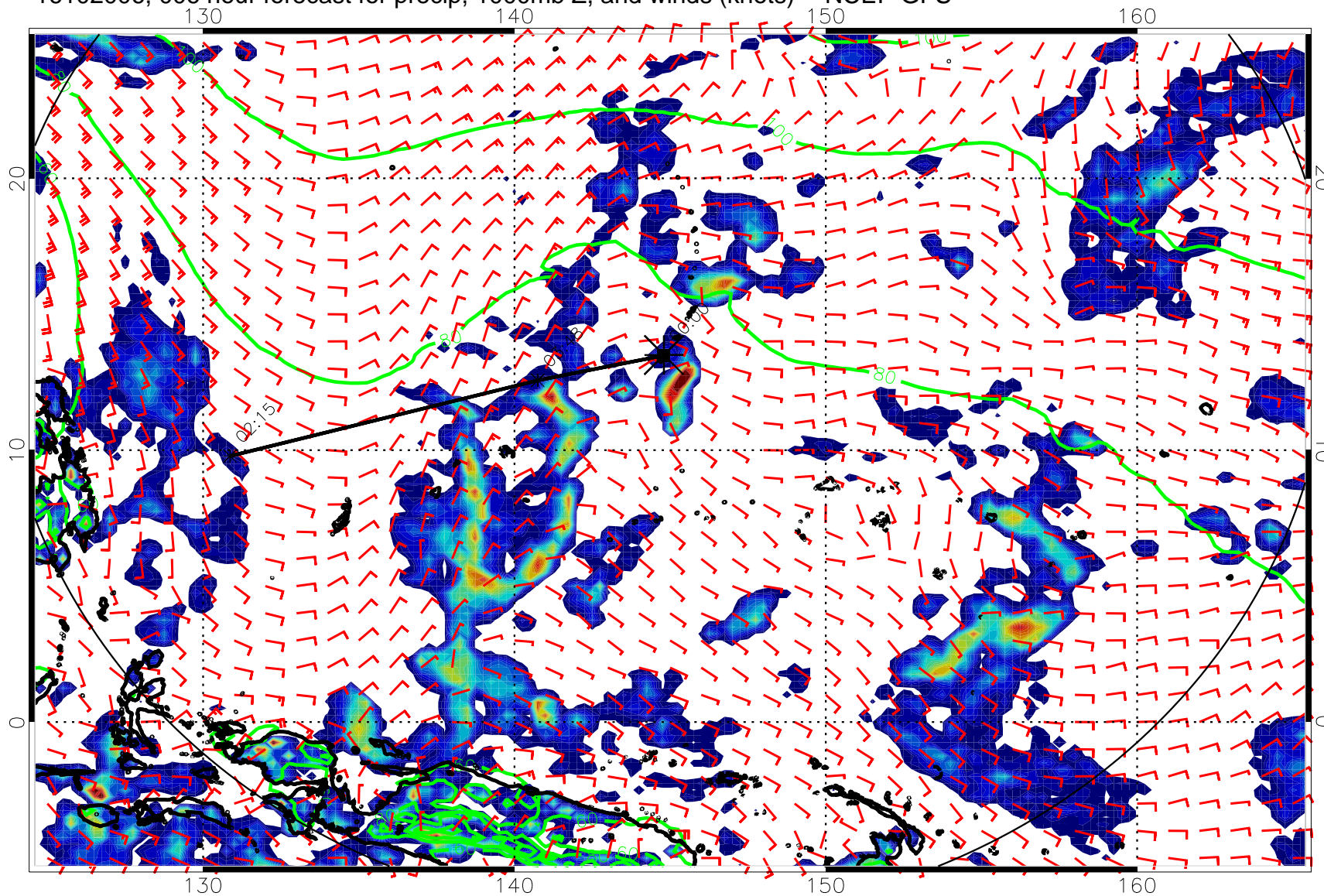
16102006, 006 hour forecast for precip, 1000mb Z, and winds (knots) -- NCEP GFS
