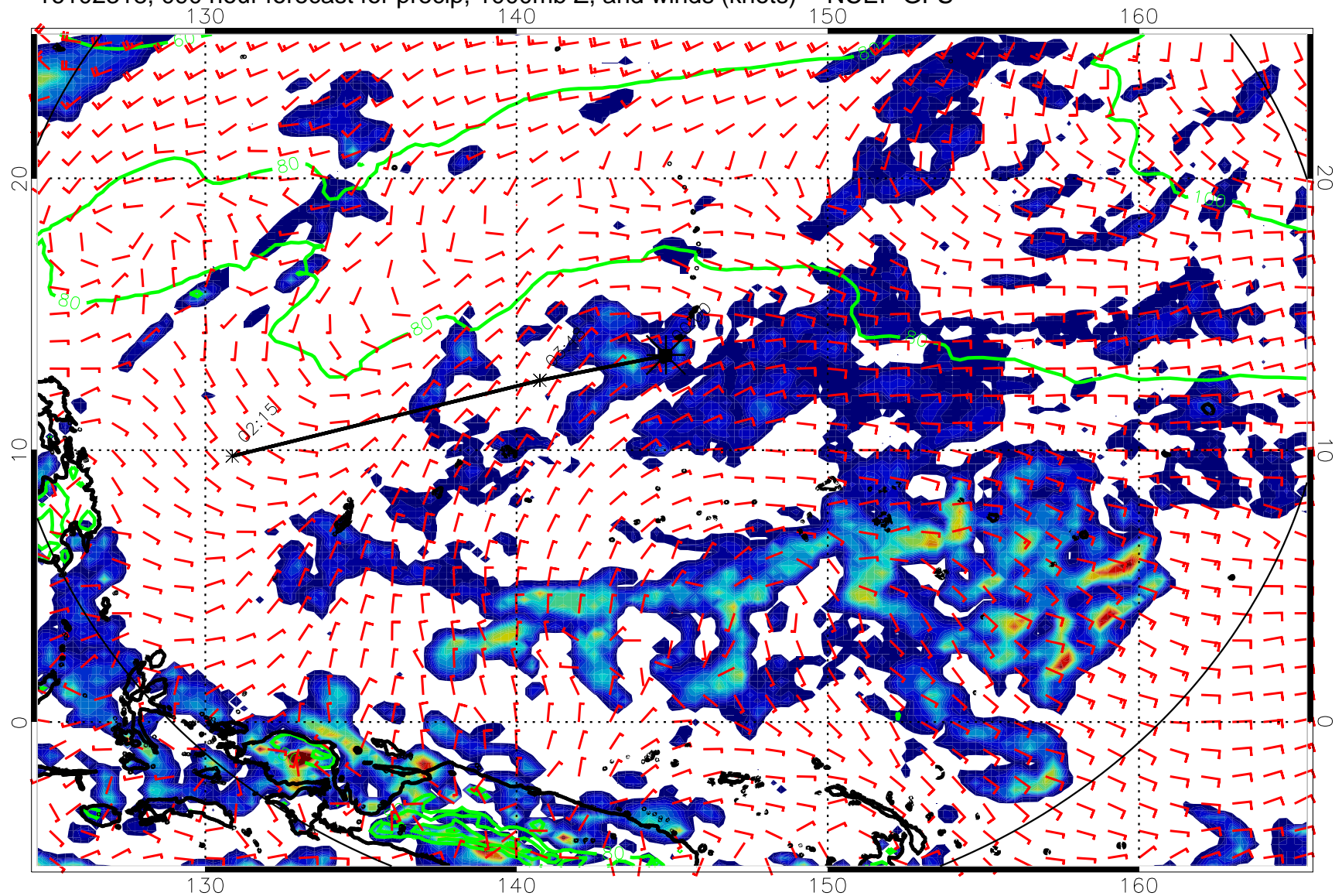
16102318, 090 hour forecast for precip, 1000mb Z, and winds (knots) -- NCEP GFS
