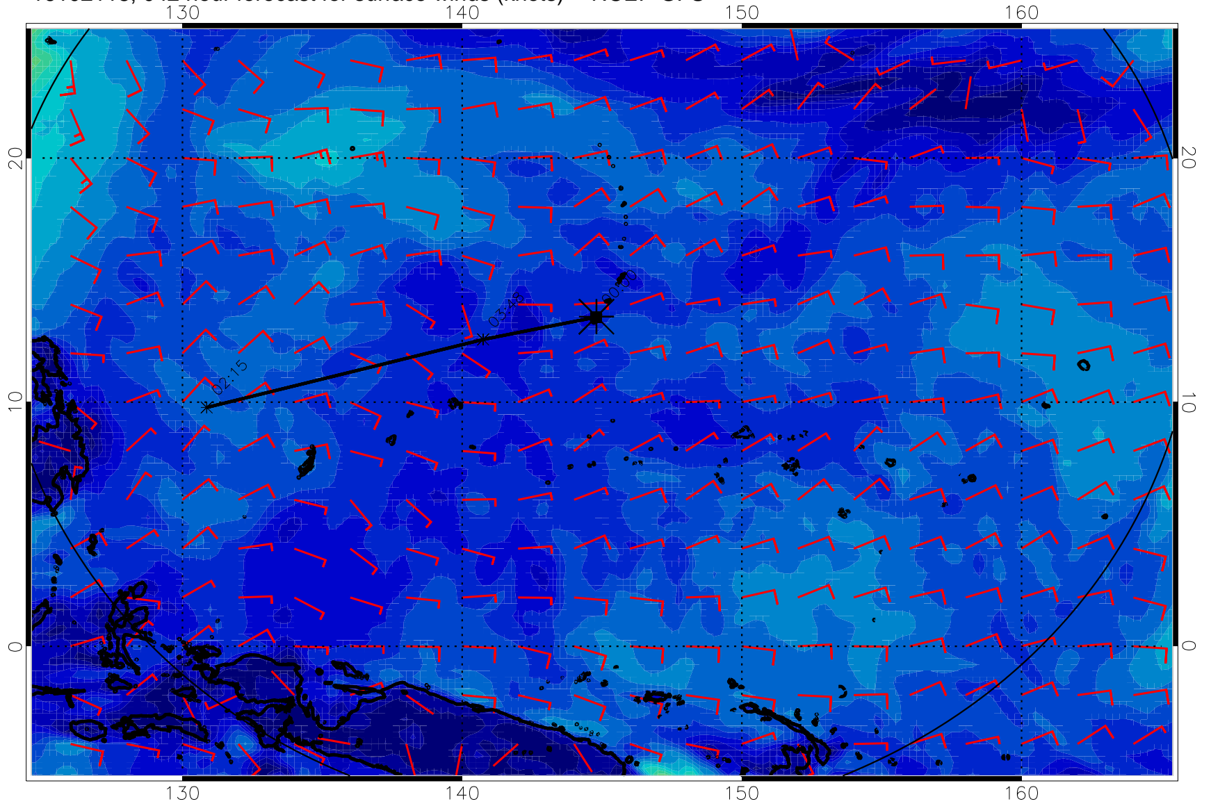
16102118, 042 hour forecast for surface winds (knots) -- NCEP GFS
