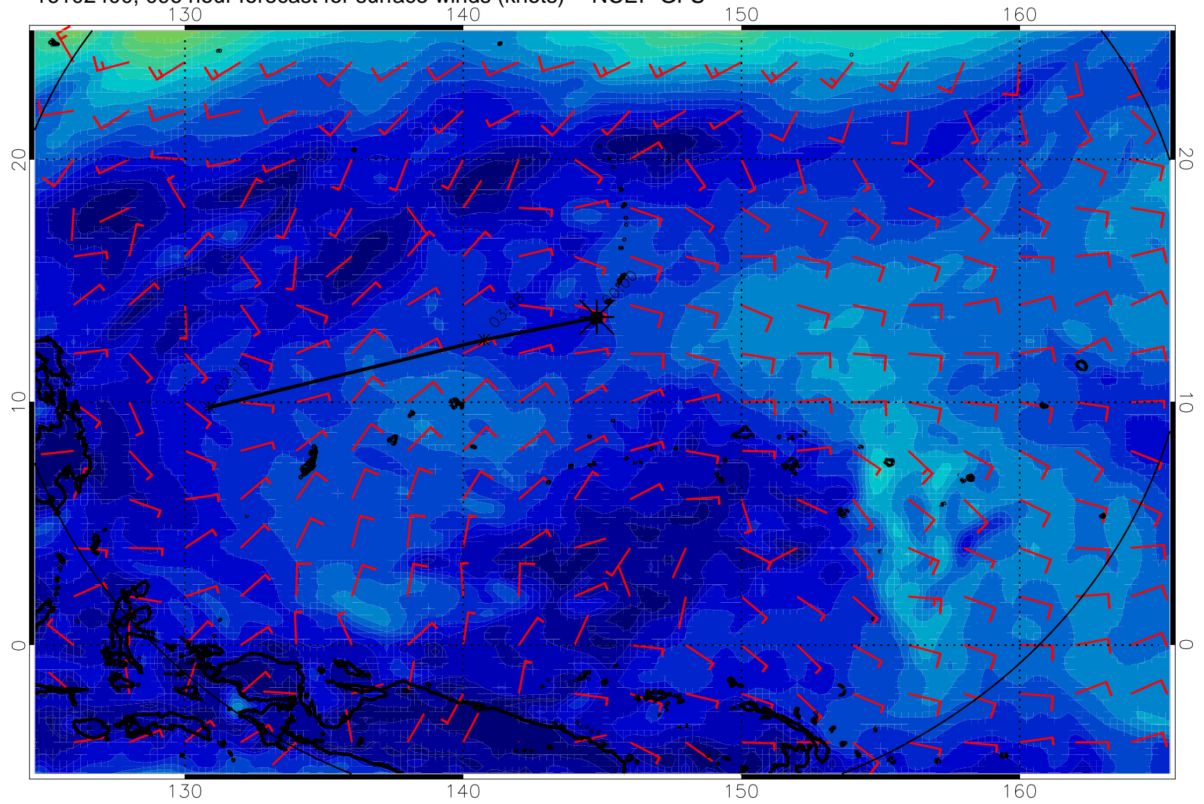
16102400, 096 hour forecast for surface winds (knots) -- NCEP GFS
