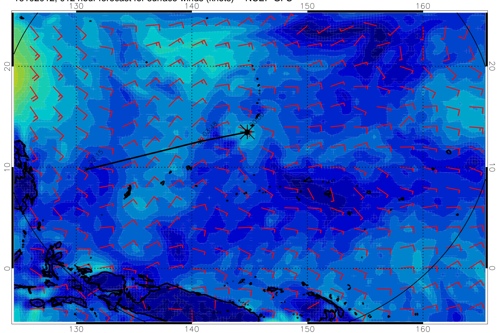
16102012, 012 hour forecast for surface winds (knots) -- NCEP GFS
