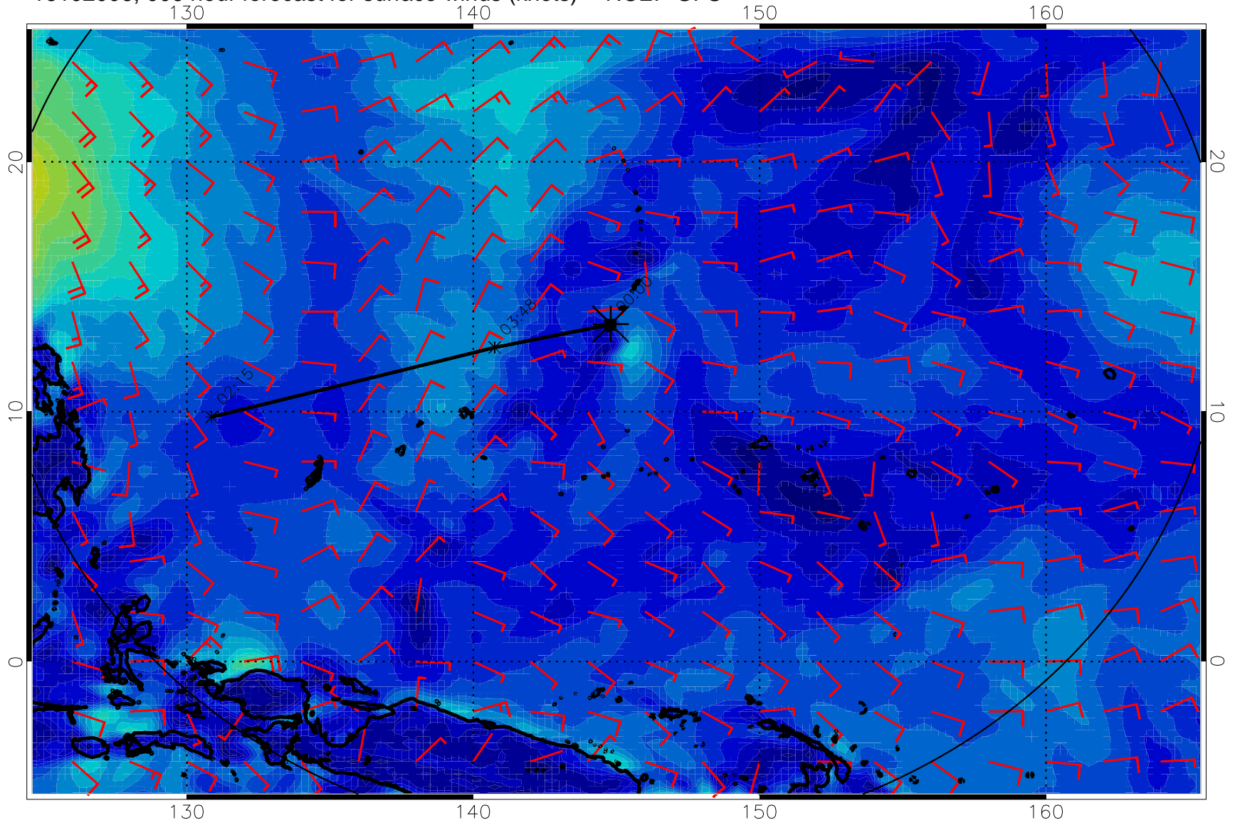
16102006, 006 hour forecast for surface winds (knots) -- NCEP GFS
