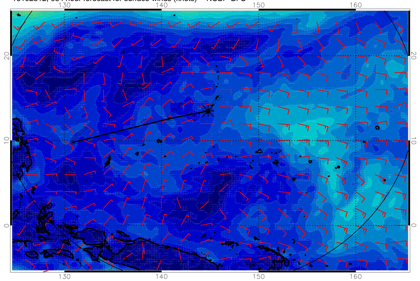
16102312, 084 hour forecast for surface winds (knots) -- NCEP GFS
