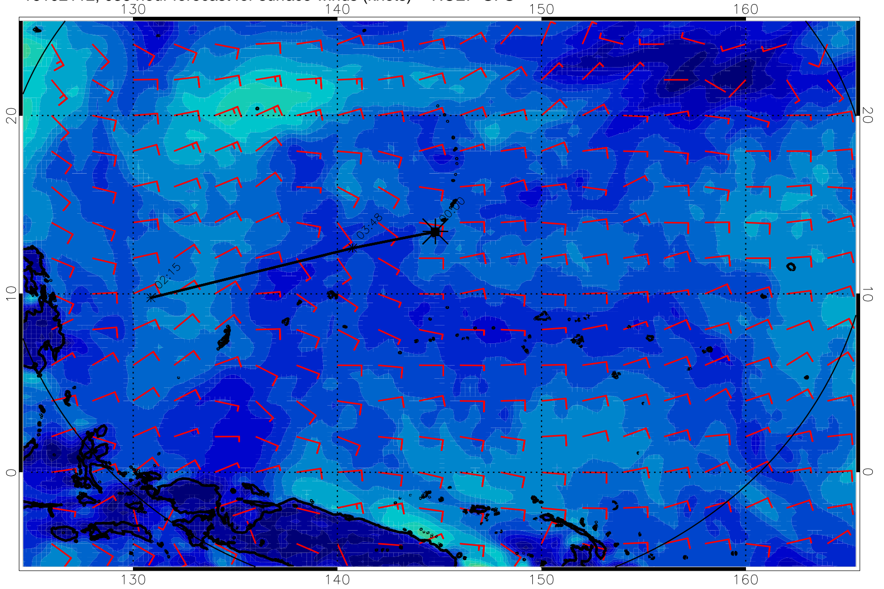
16102112, 036 hour forecast for surface winds (knots) -- NCEP GFS
