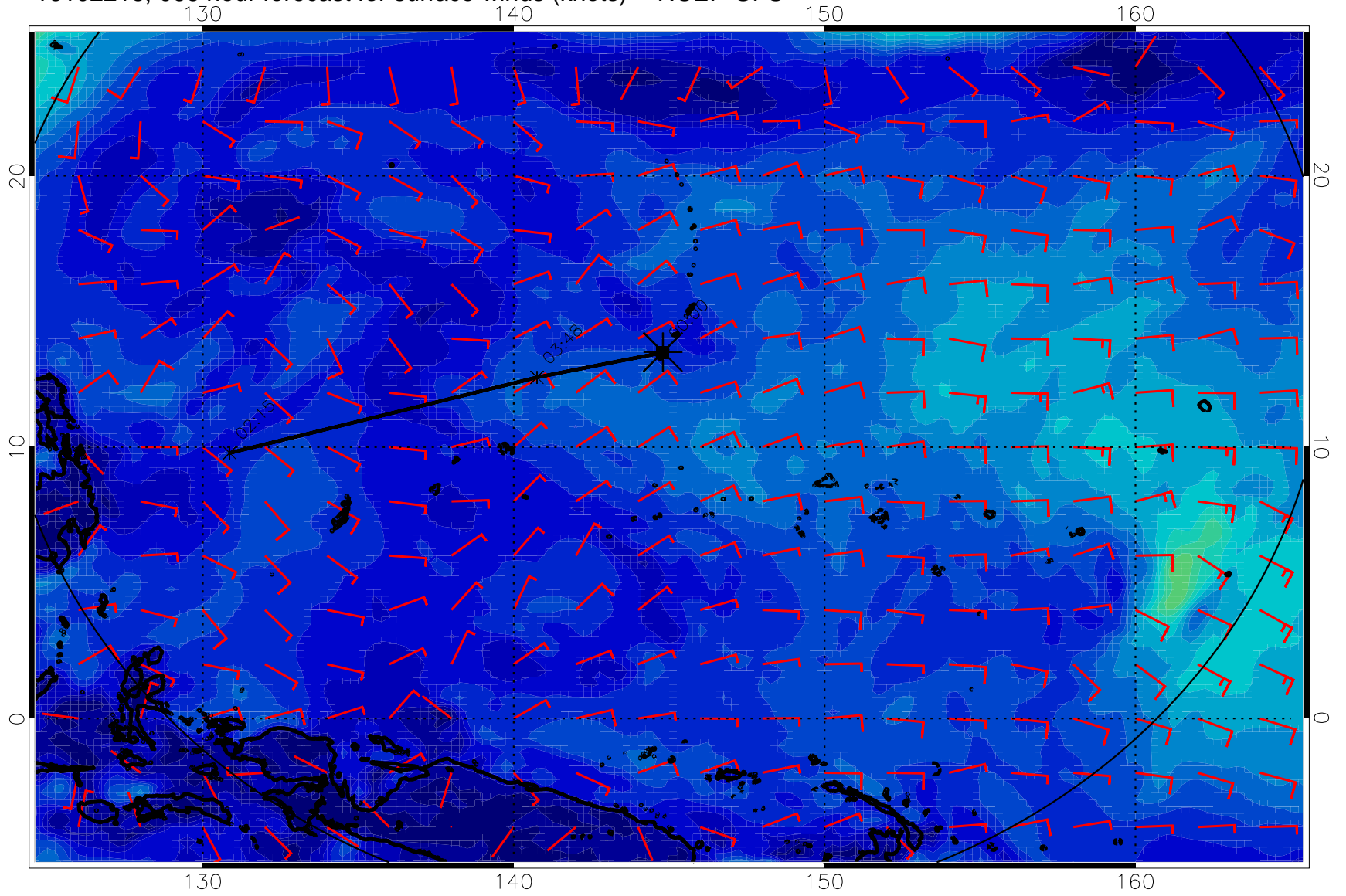
16102218, 066 hour forecast for surface winds (knots) -- NCEP GFS
