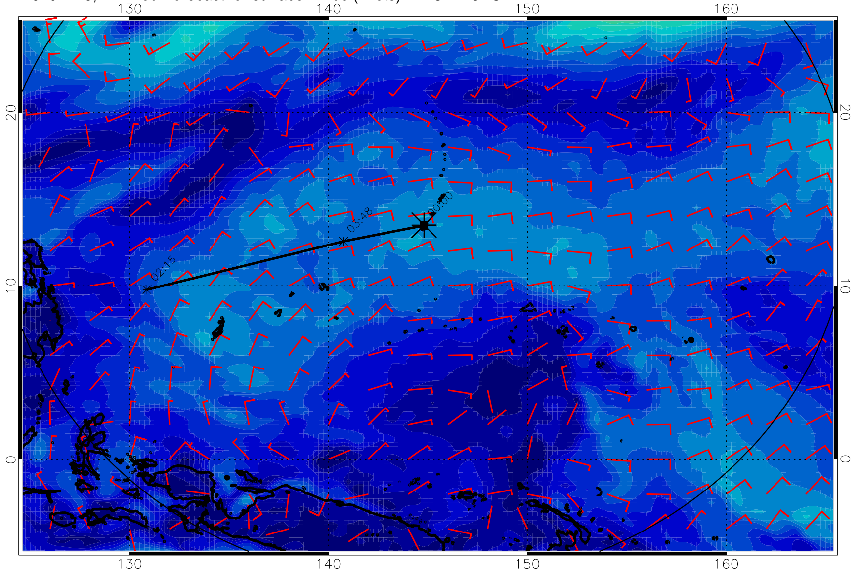
16102418, 114 hour forecast for surface winds (knots) -- NCEP GFS
