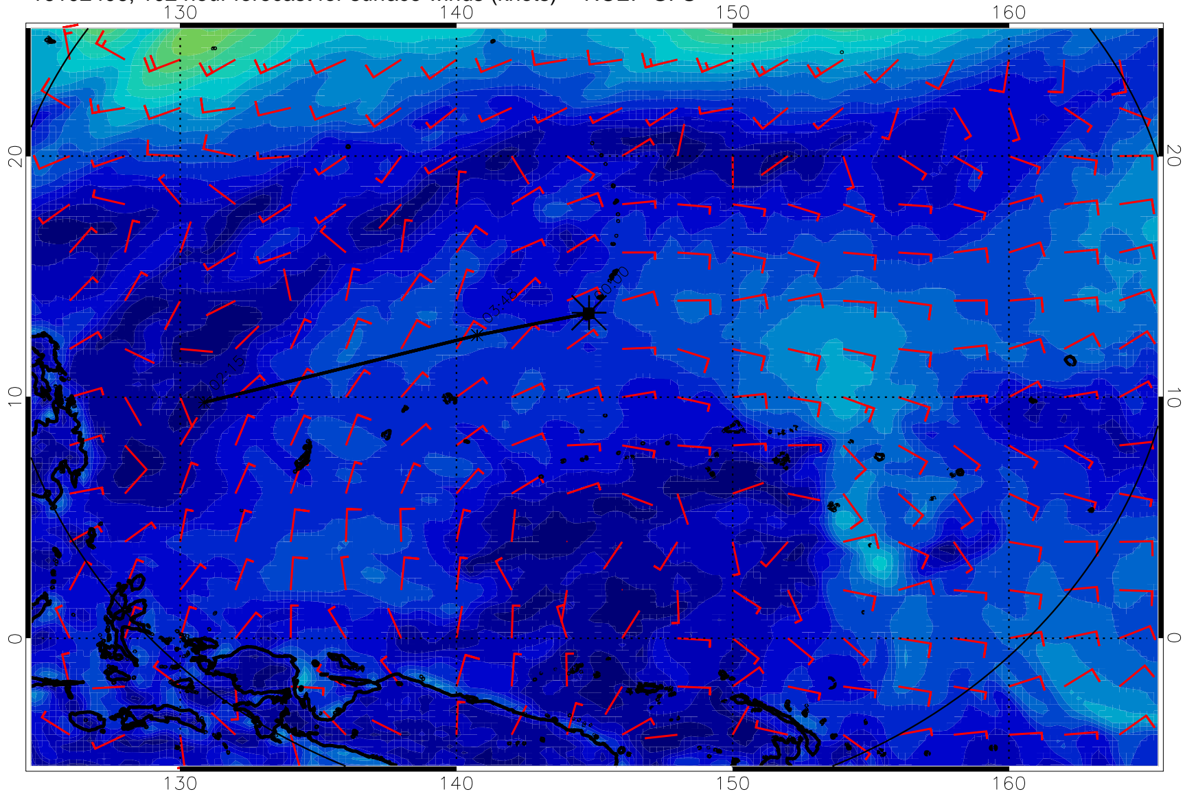
16102406, 102 hour forecast for surface winds (knots) -- NCEP GFS
