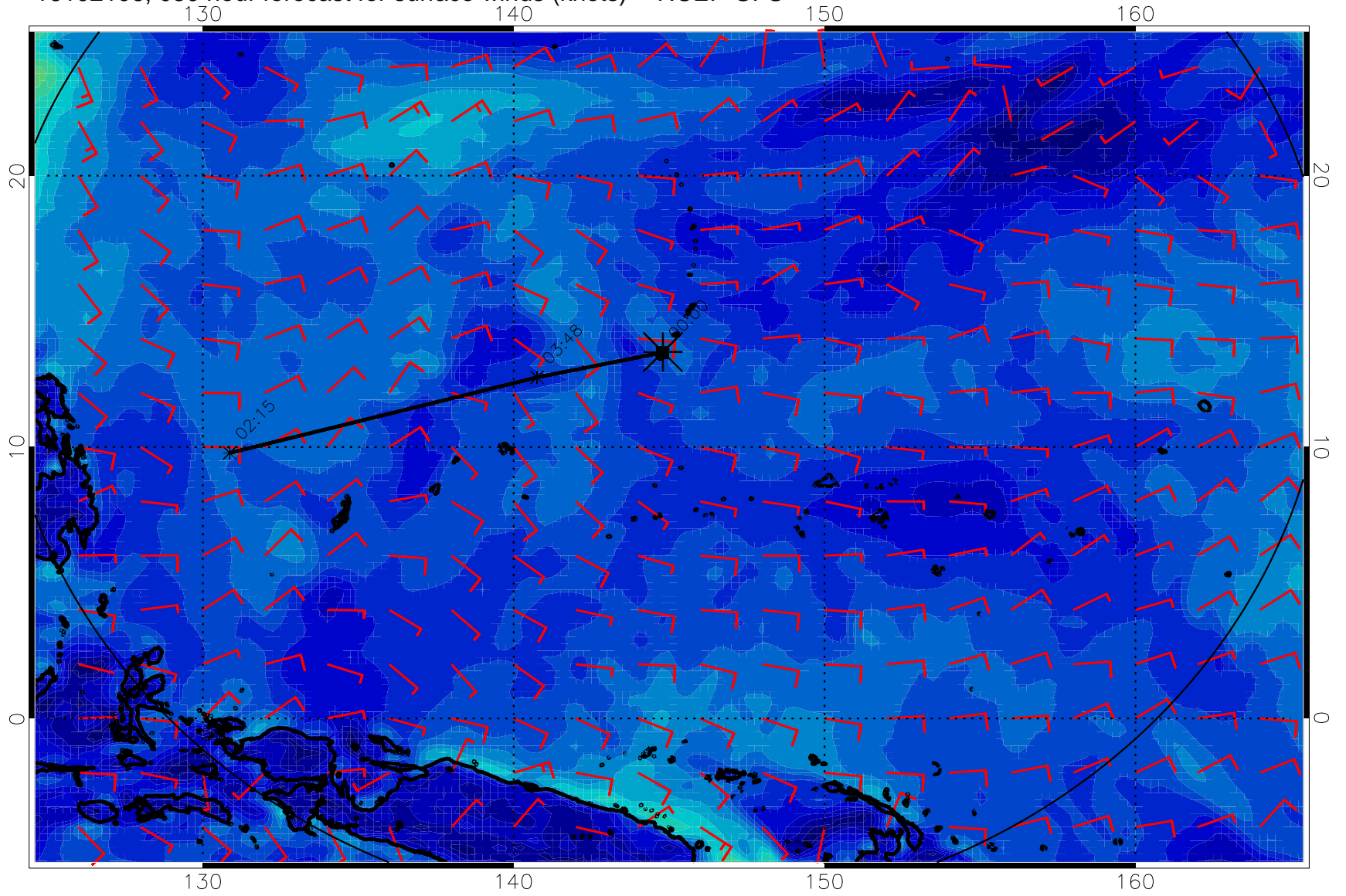
16102106, 030 hour forecast for surface winds (knots) -- NCEP GFS
