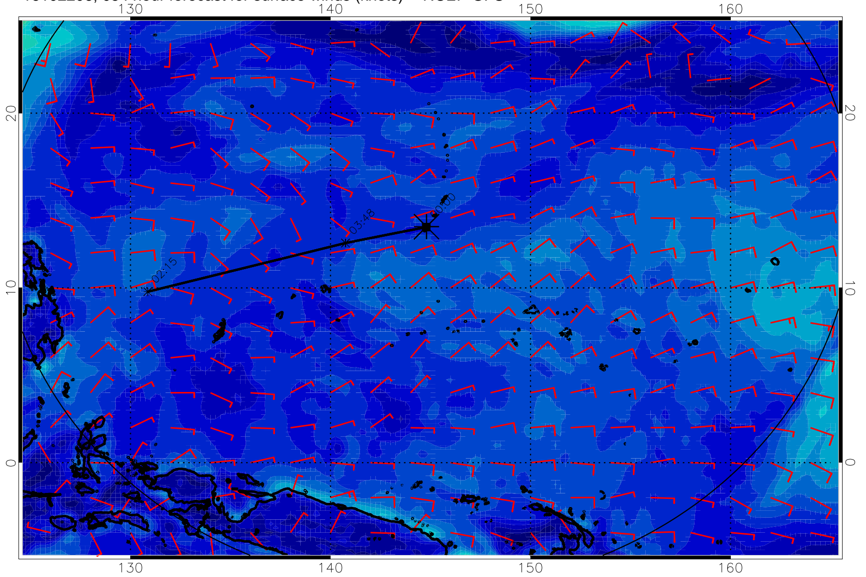
16102206, 054 hour forecast for surface winds (knots) -- NCEP GFS
