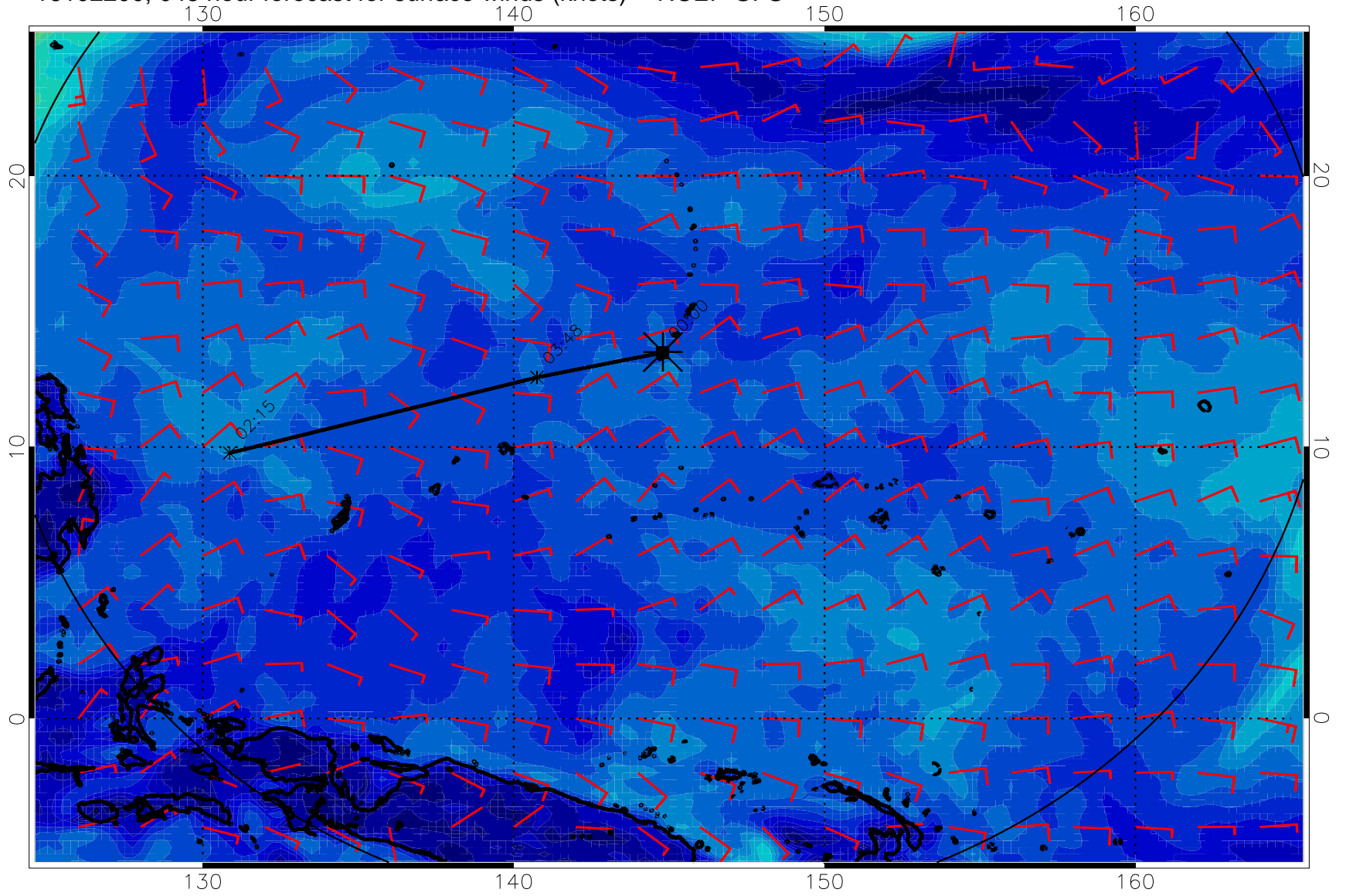
16102200, 048 hour forecast for surface winds (knots) -- NCEP GFS
