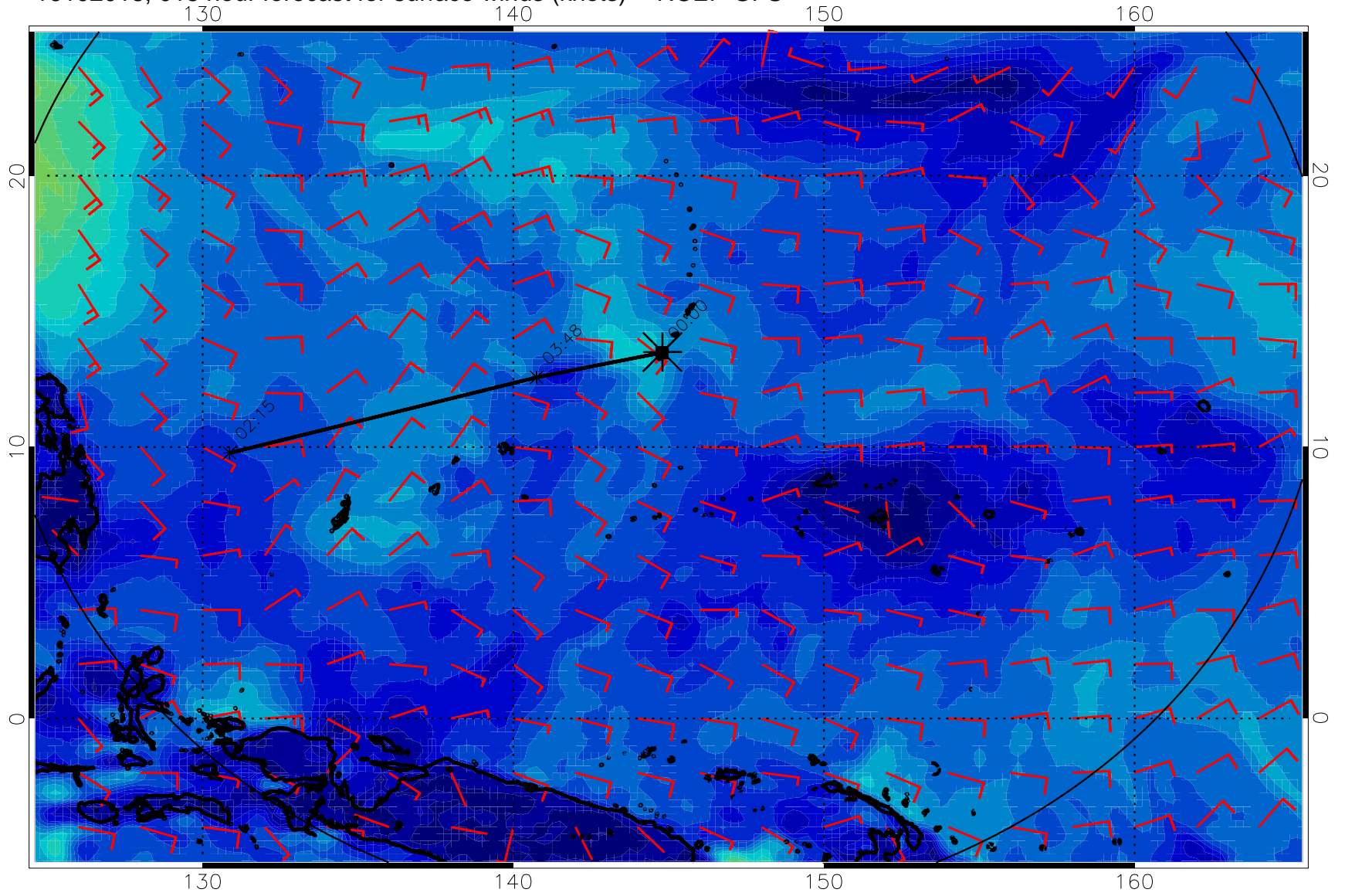
16102018, 018 hour forecast for surface winds (knots) -- NCEP GFS
