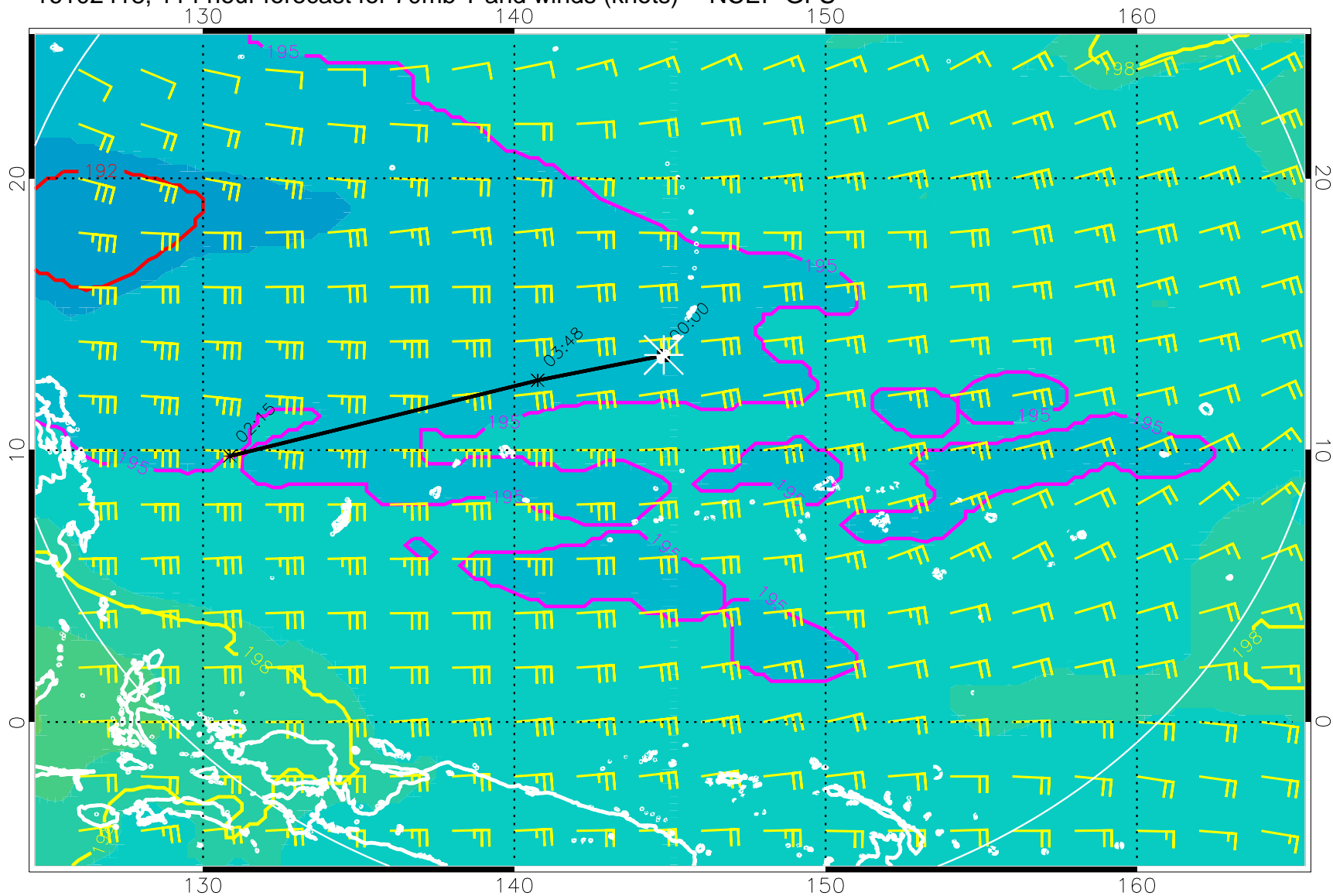
16102418, 114 hour forecast for 70mb T and winds (knots) -- NCEP GFS
