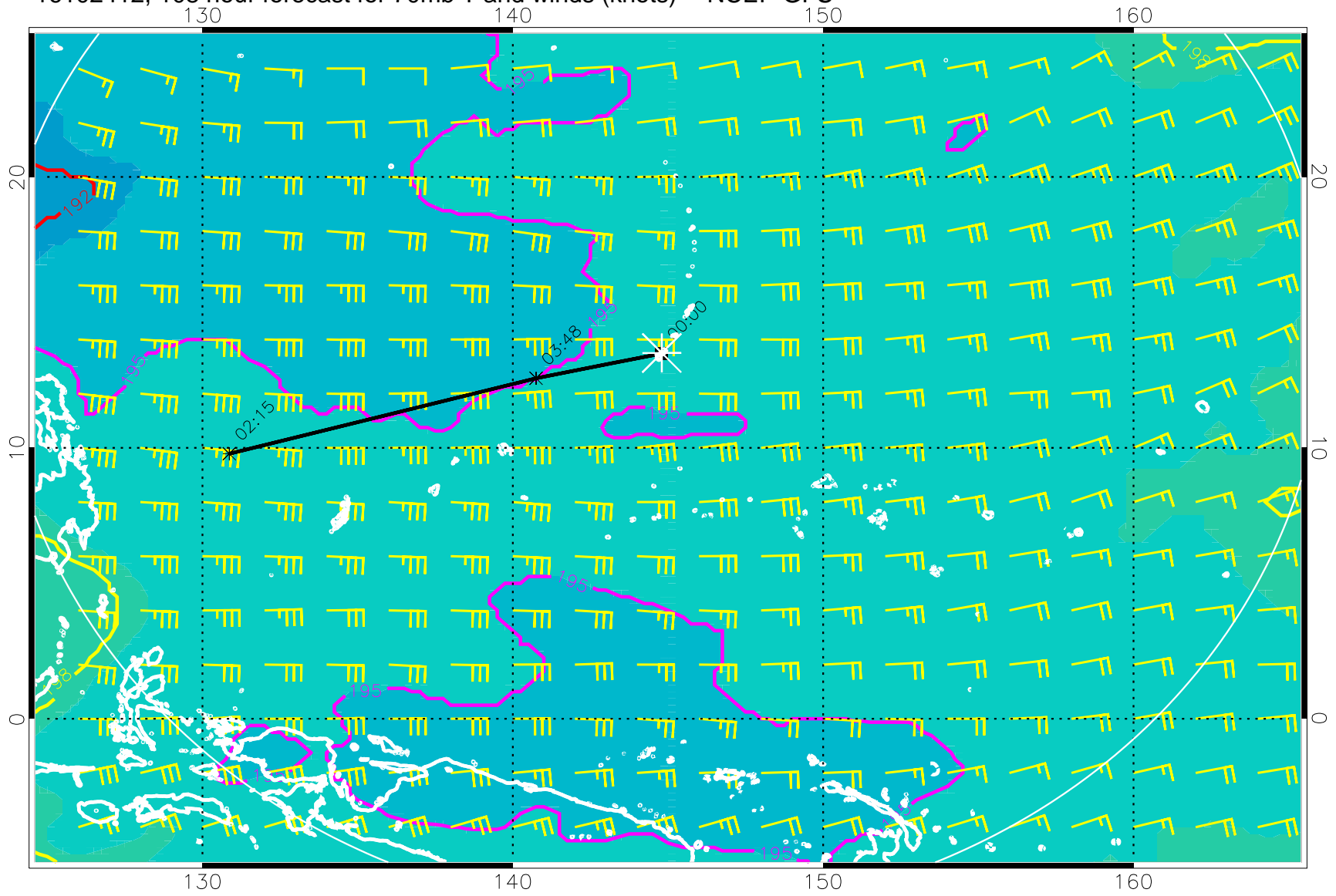
16102412, 108 hour forecast for 70mb T and winds (knots) -- NCEP GFS
