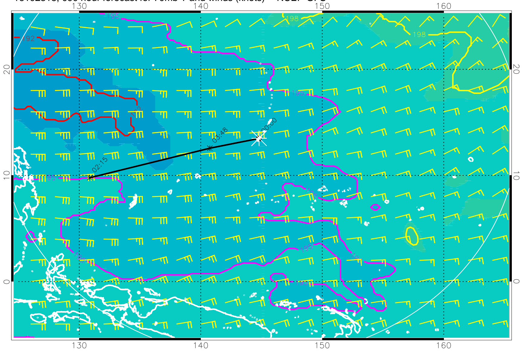
16102318, 090 hour forecast for 70mb T and winds (knots) -- NCEP GFS
