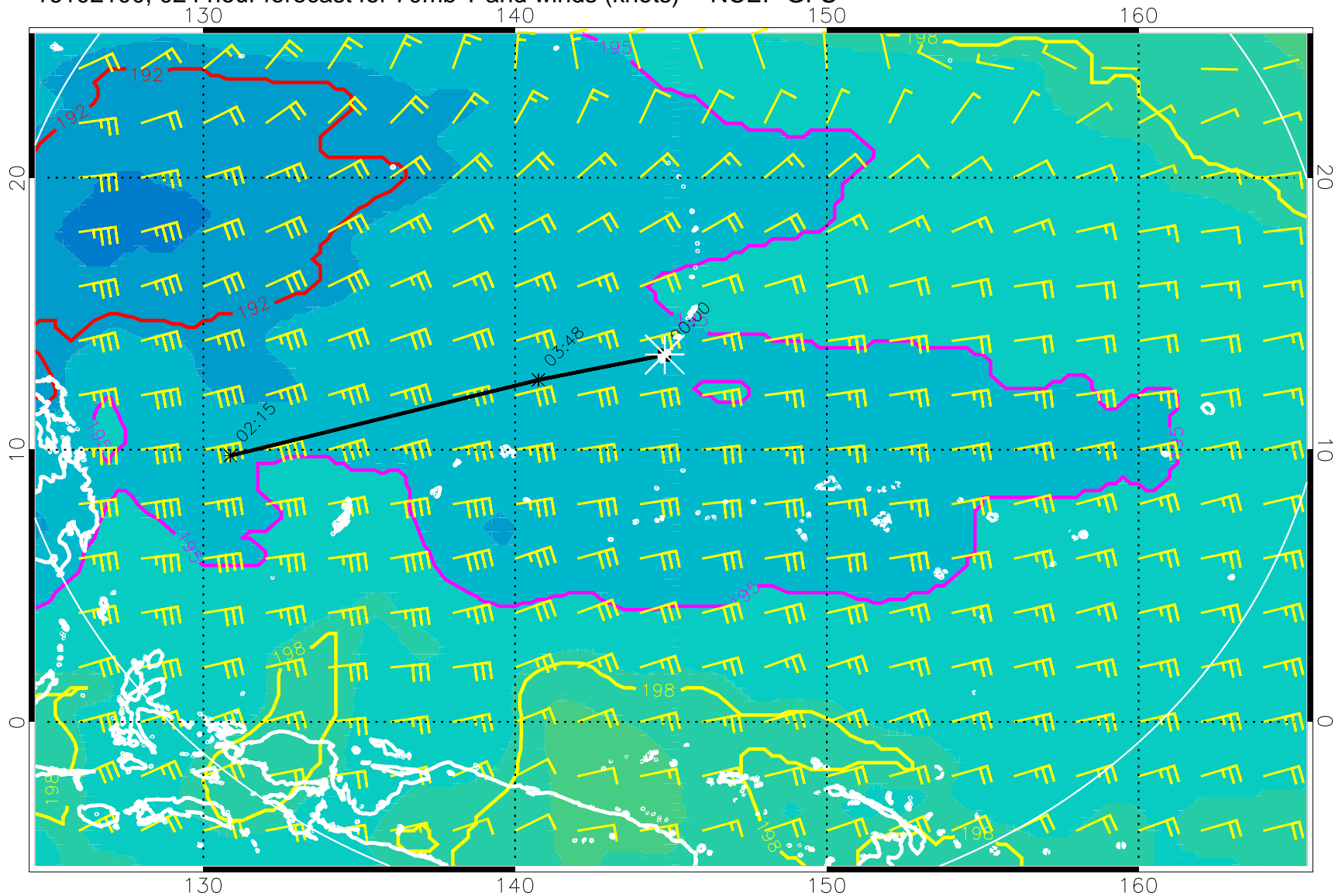
16102100, 024 hour forecast for 70mb T and winds (knots) -- NCEP GFS
