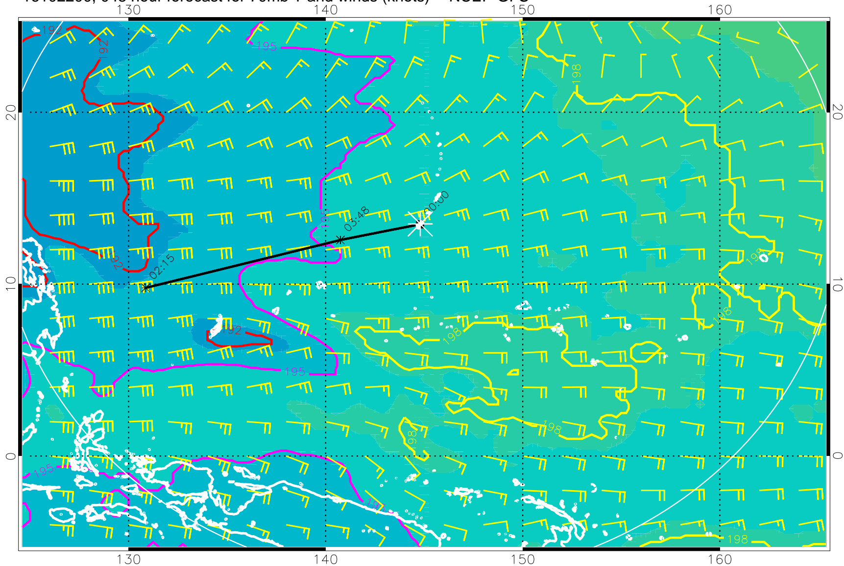
16102200, 048 hour forecast for 70mb T and winds (knots) -- NCEP GFS
