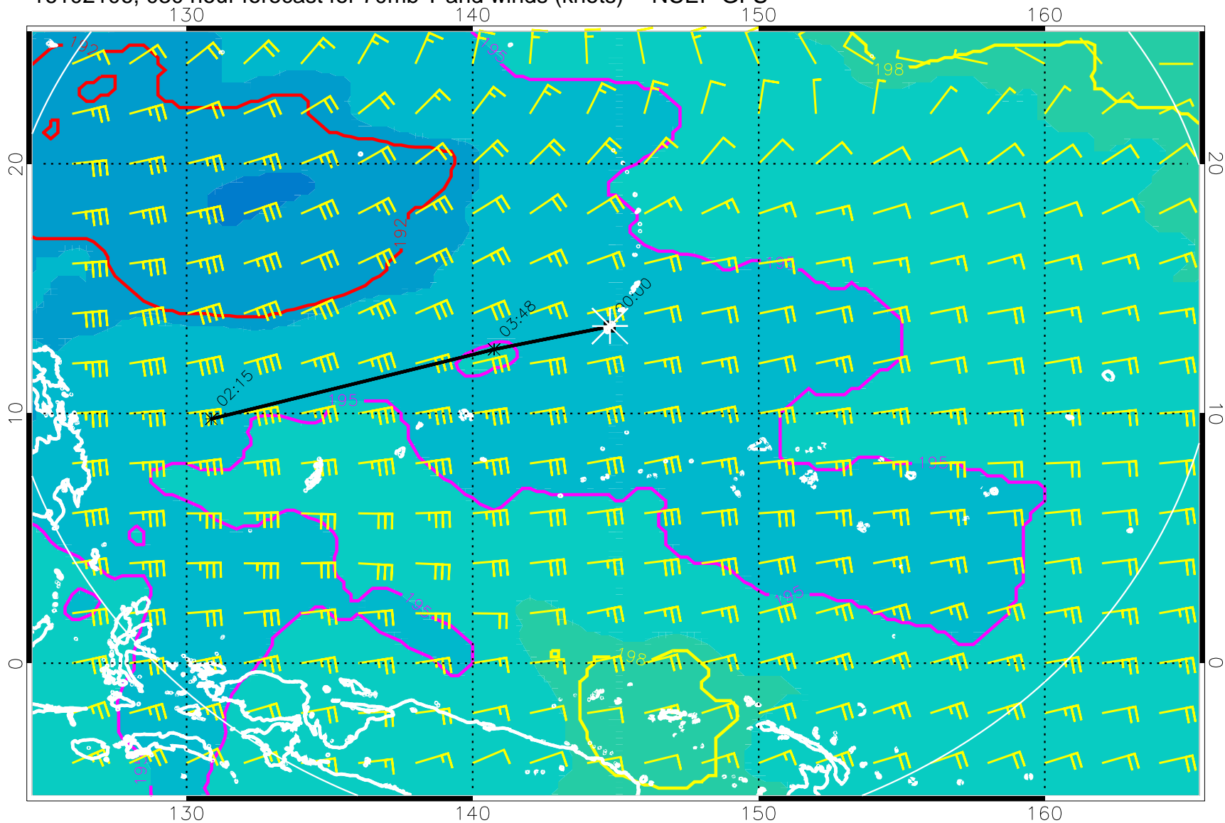
16102106, 030 hour forecast for 70mb T and winds (knots) -- NCEP GFS
