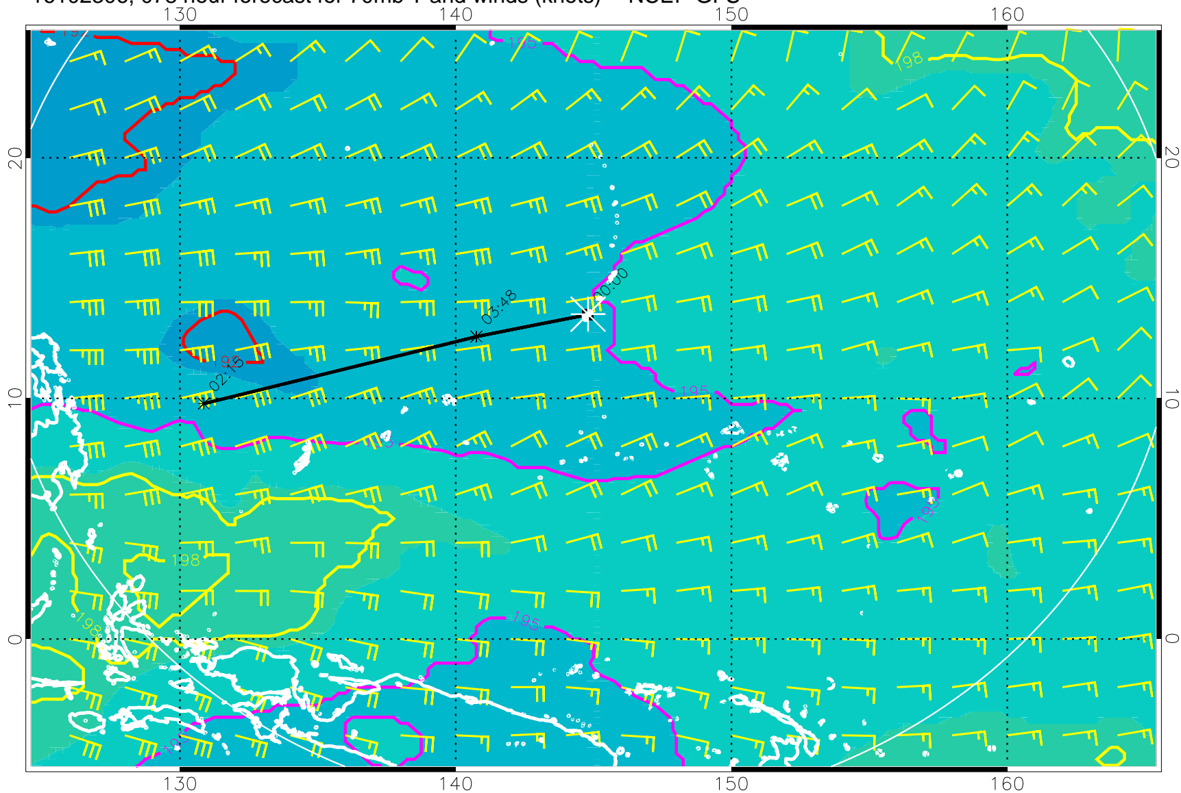
16102306, 078 hour forecast for 70mb T and winds (knots) -- NCEP GFS
