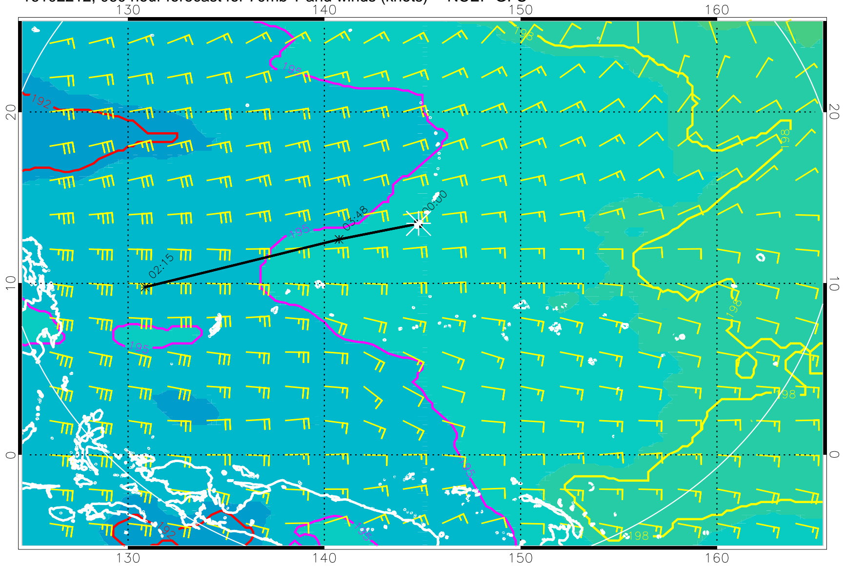
16102212, 060 hour forecast for 70mb T and winds (knots) -- NCEP GFS
