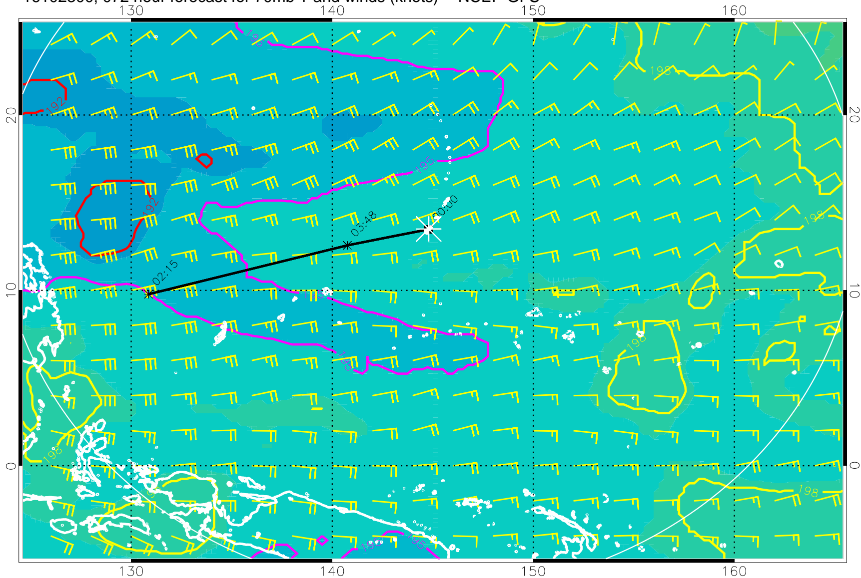
16102300, 072 hour forecast for 70mb T and winds (knots) -- NCEP GFS
