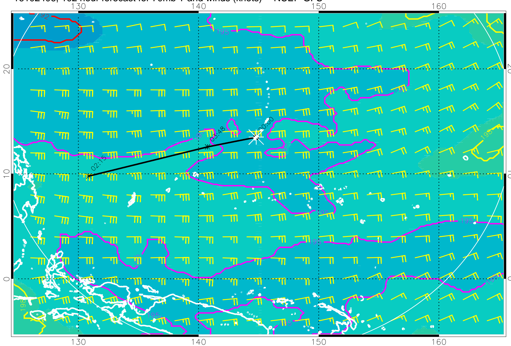
16102406, 102 hour forecast for 70mb T and winds (knots) -- NCEP GFS
