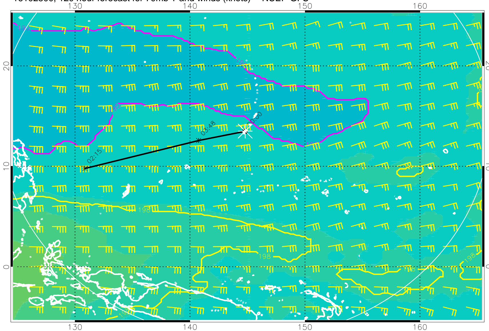
16102500, 120 hour forecast for 70mb T and winds (knots) -- NCEP GFS
