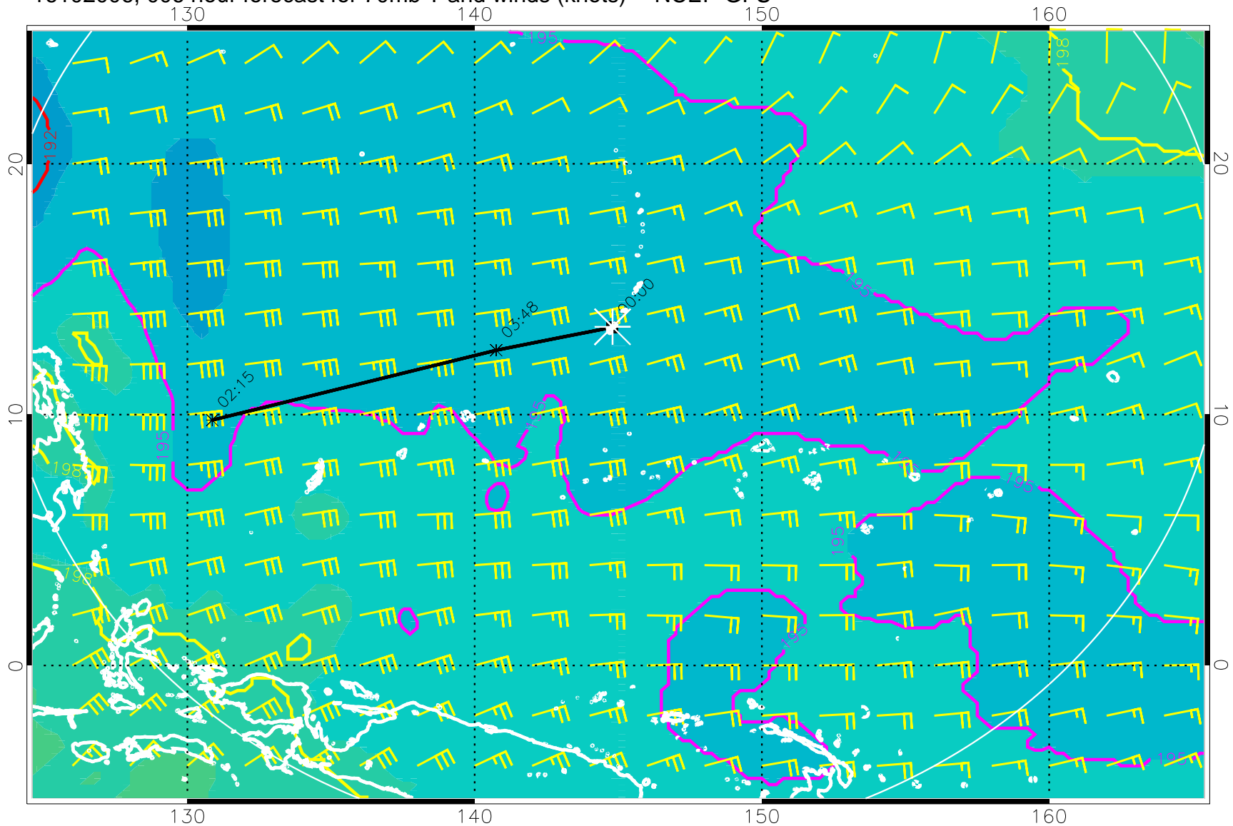
16102006, 006 hour forecast for 70mb T and winds (knots) -- NCEP GFS
