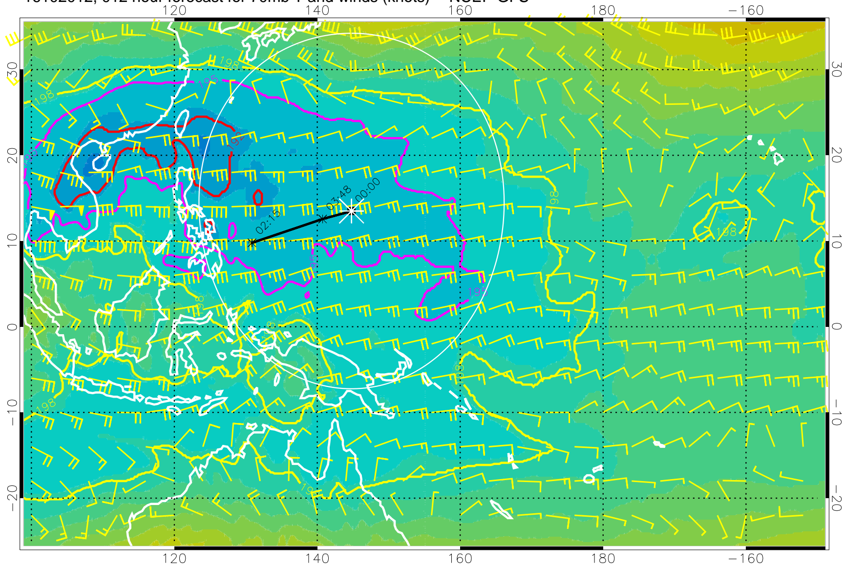
16102012, 012 hour forecast for 70mb T and winds (knots) -- NCEP GFS
