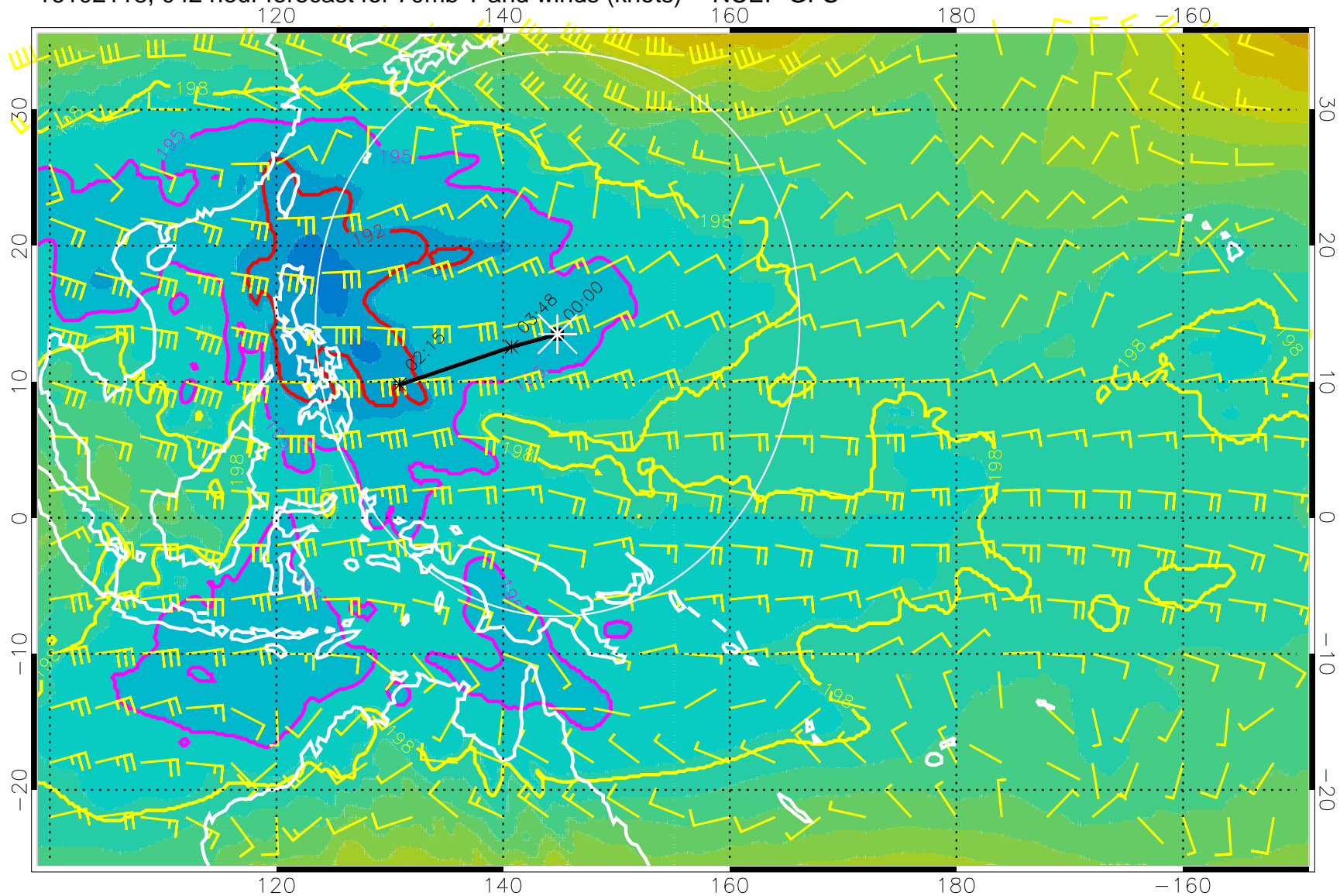
16102118, 042 hour forecast for 70mb T and winds (knots) -- NCEP GFS
