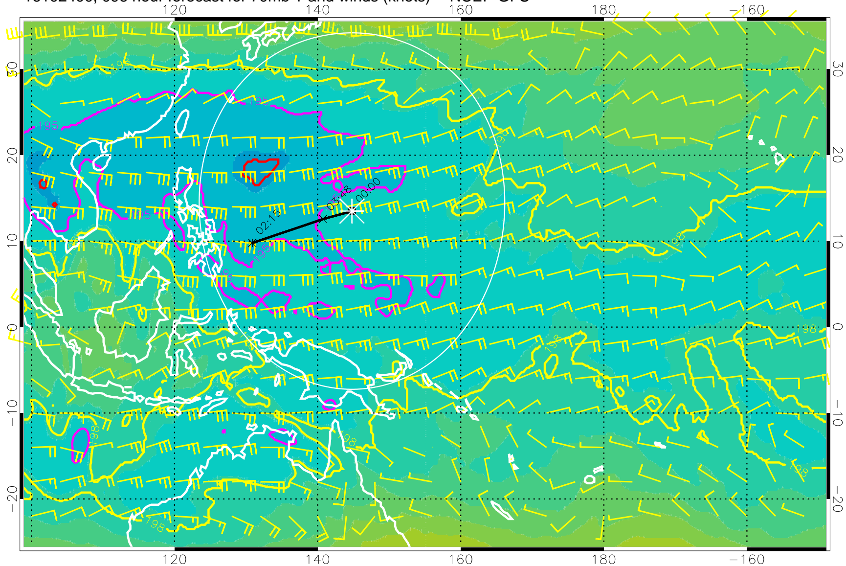
16102400, 096 hour forecast for 70mb T and winds (knots) -- NCEP GFS
