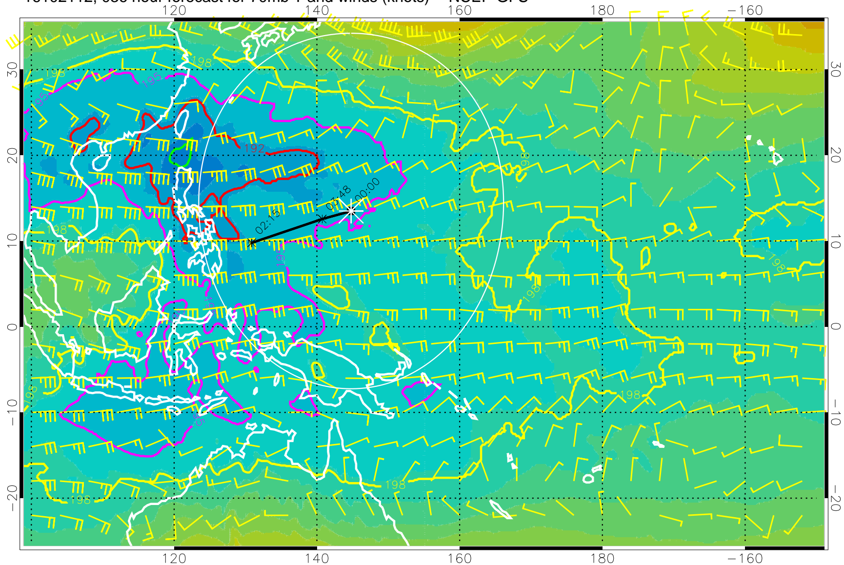
16102112, 036 hour forecast for 70mb T and winds (knots) -- NCEP GFS
