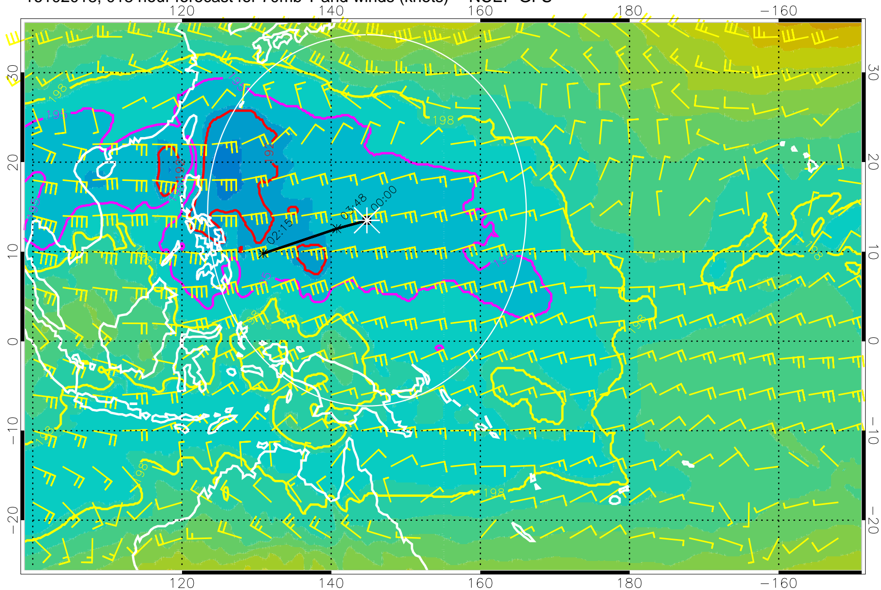
16102018, 018 hour forecast for 70mb T and winds (knots) -- NCEP GFS
