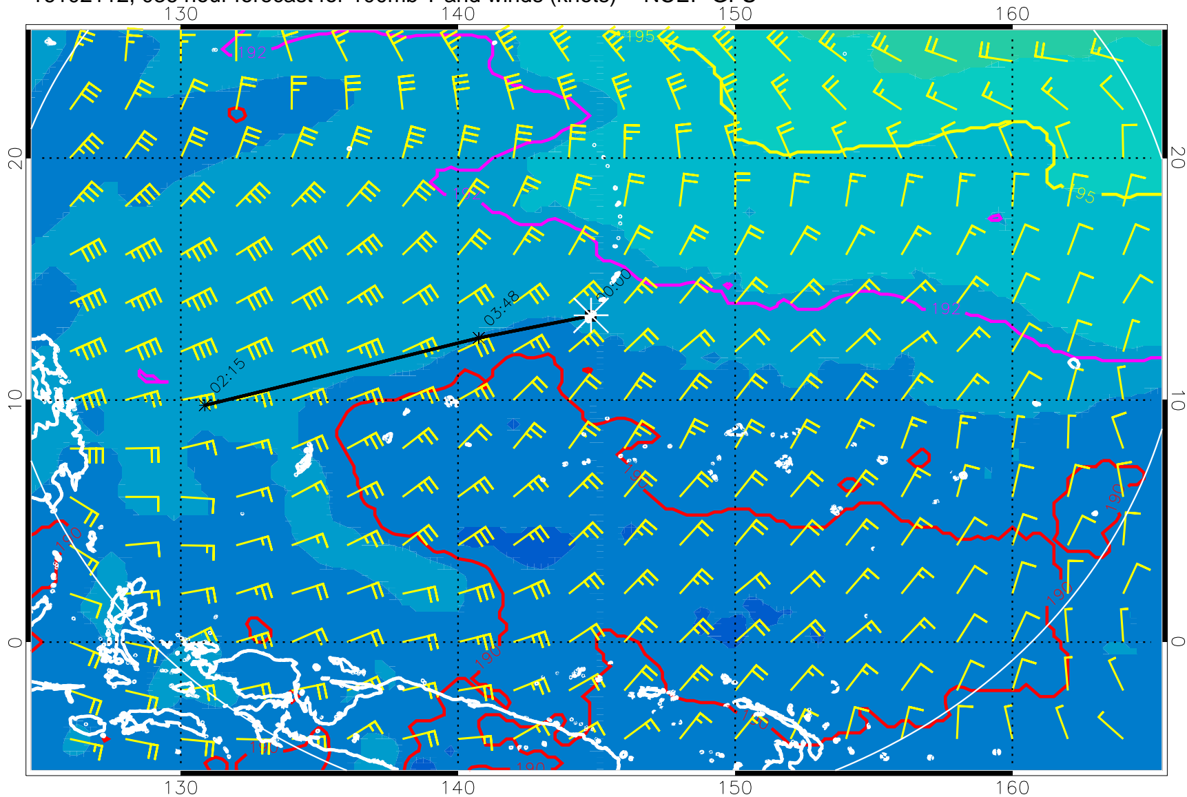
16102112, 036 hour forecast for 100mb T and winds (knots) -- NCEP GFS
