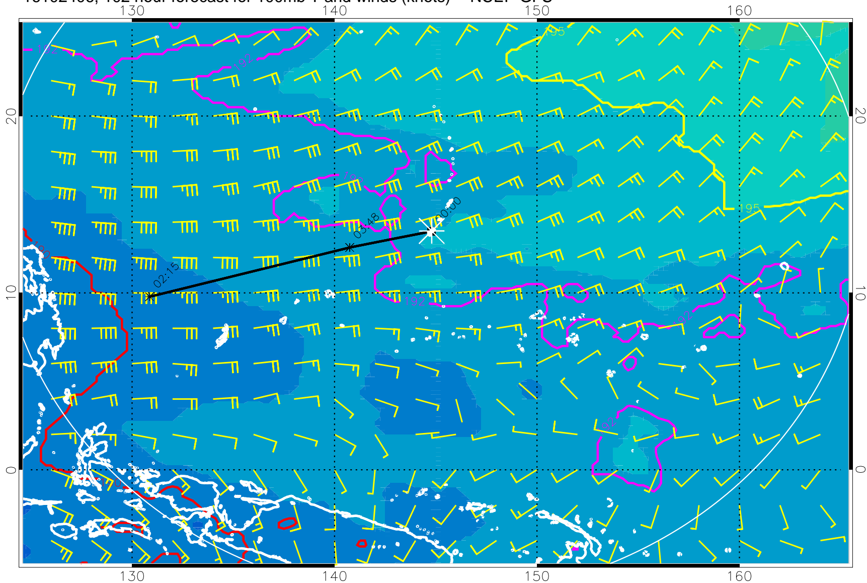
16102406, 102 hour forecast for 100mb T and winds (knots) -- NCEP GFS
