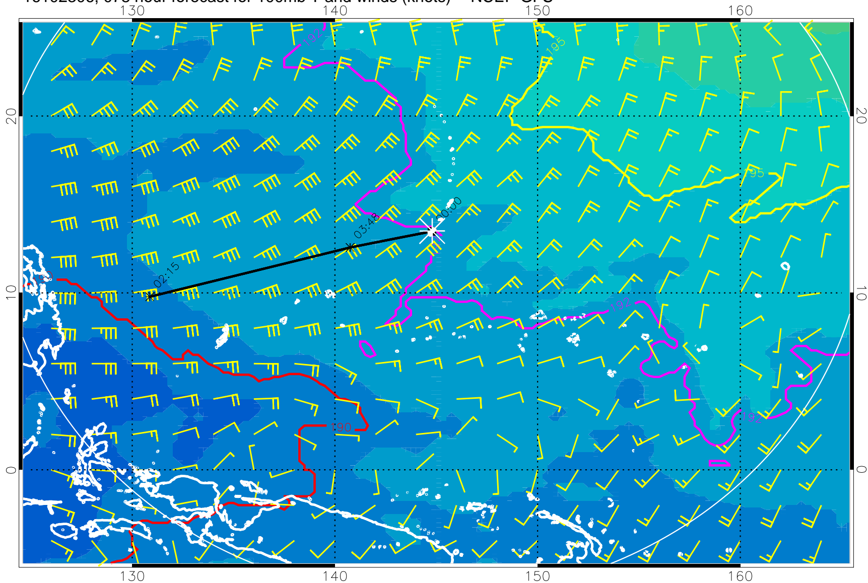
16102306, 078 hour forecast for 100mb T and winds (knots) -- NCEP GFS
