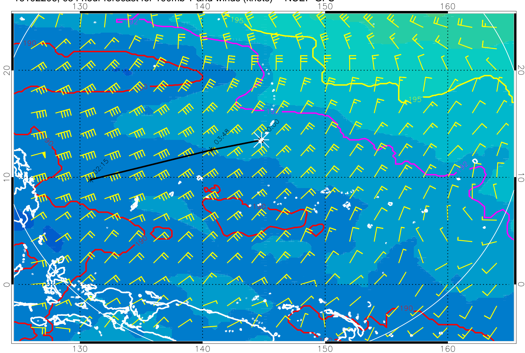
16102206, 054 hour forecast for 100mb T and winds (knots) -- NCEP GFS
