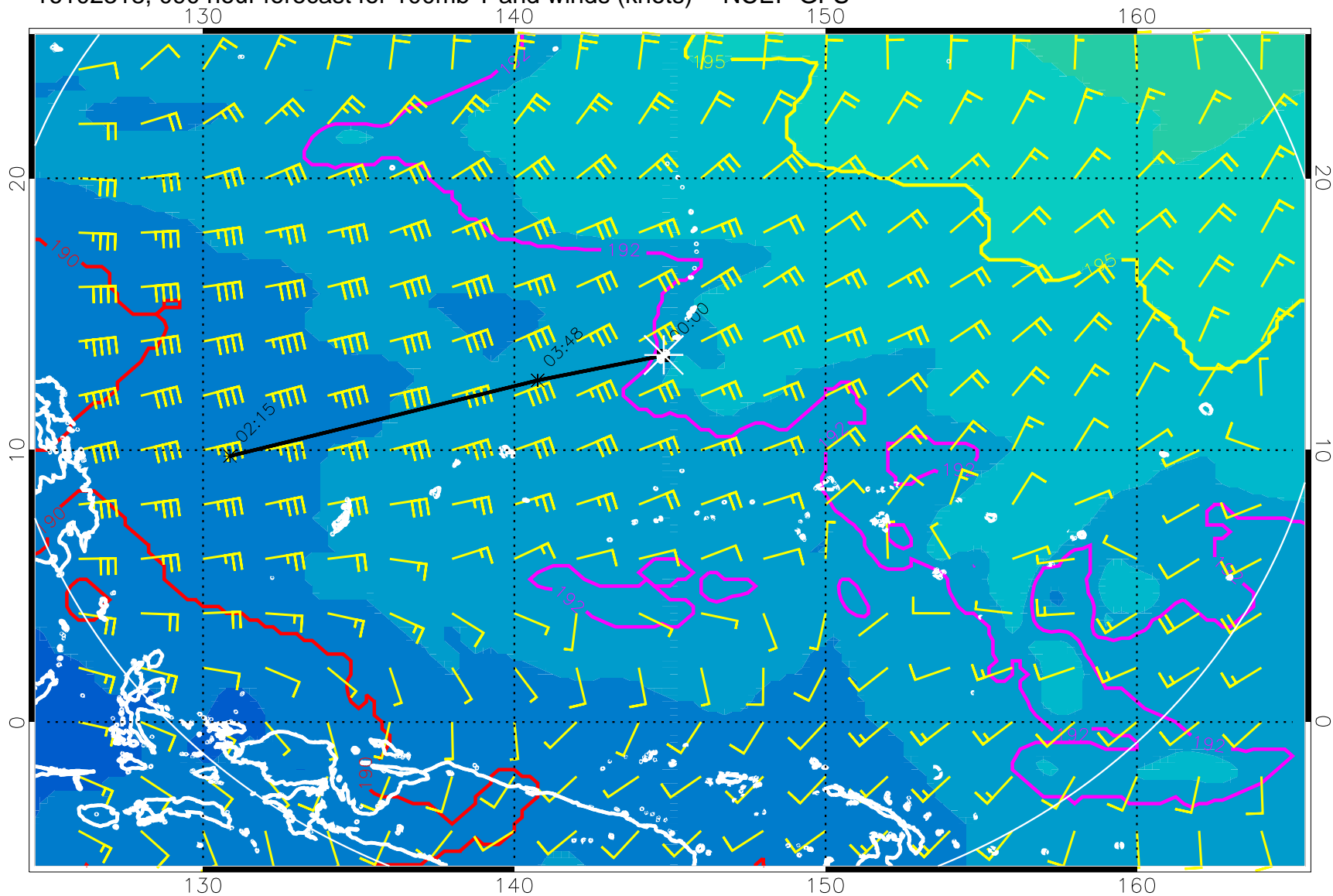
16102318, 090 hour forecast for 100mb T and winds (knots) -- NCEP GFS
