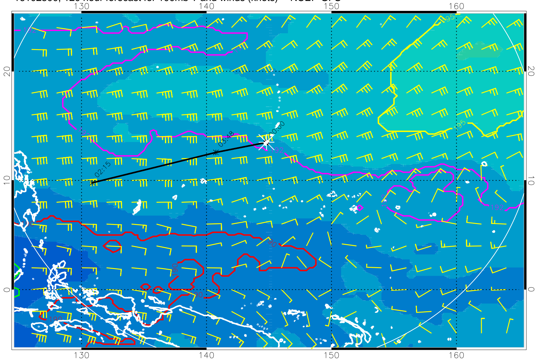
16102500, 120 hour forecast for 100mb T and winds (knots) -- NCEP GFS
