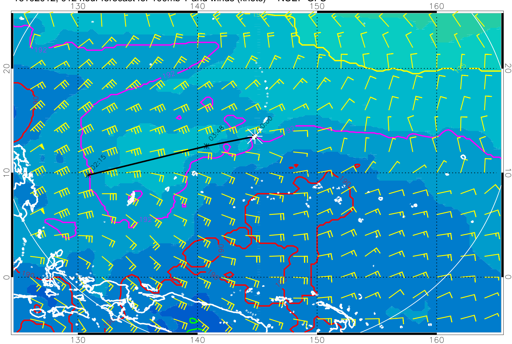
16102012, 012 hour forecast for 100mb T and winds (knots) -- NCEP GFS
