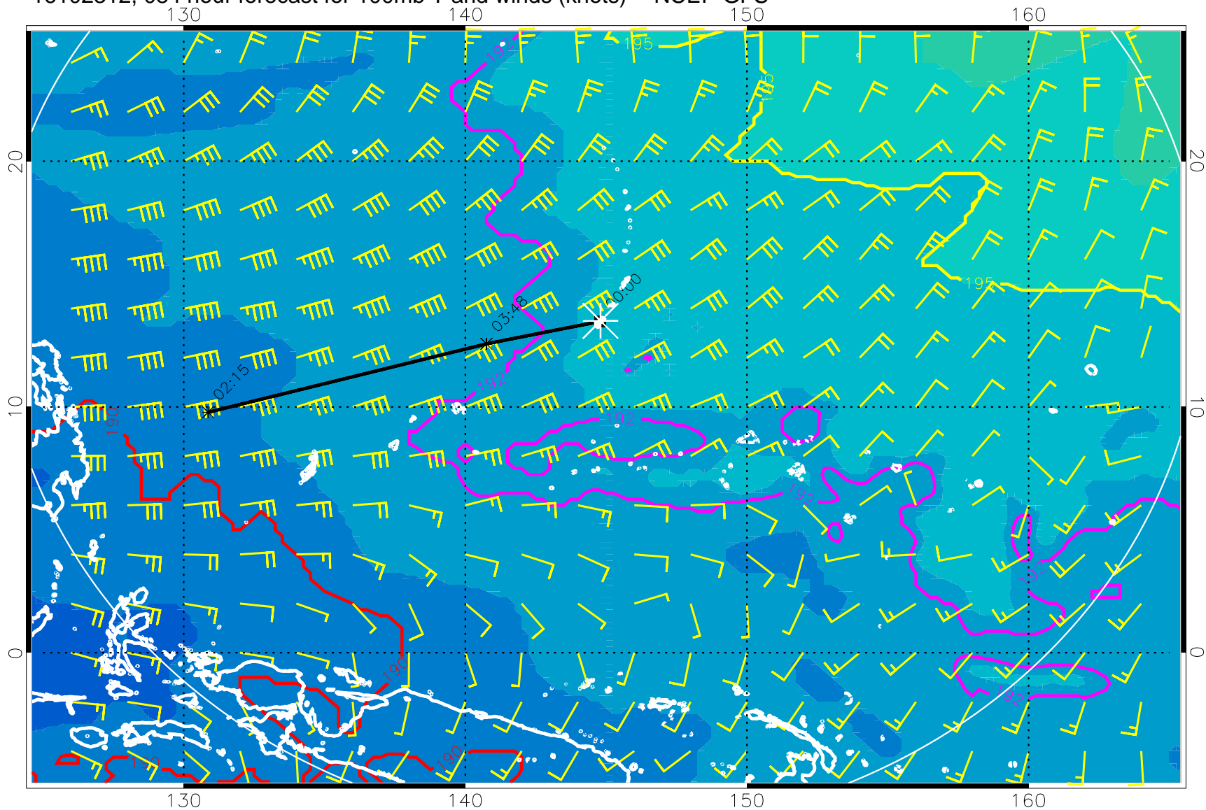
16102312, 084 hour forecast for 100mb T and winds (knots) -- NCEP GFS
