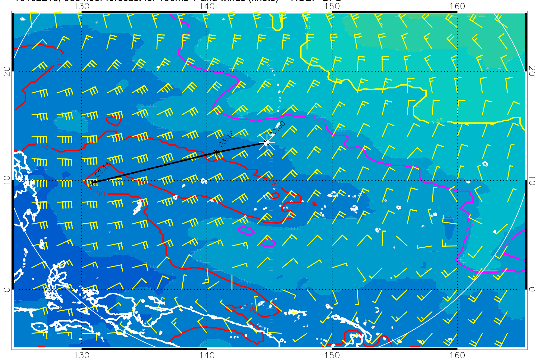
16102218, 066 hour forecast for 100mb T and winds (knots) -- NCEP GFS
