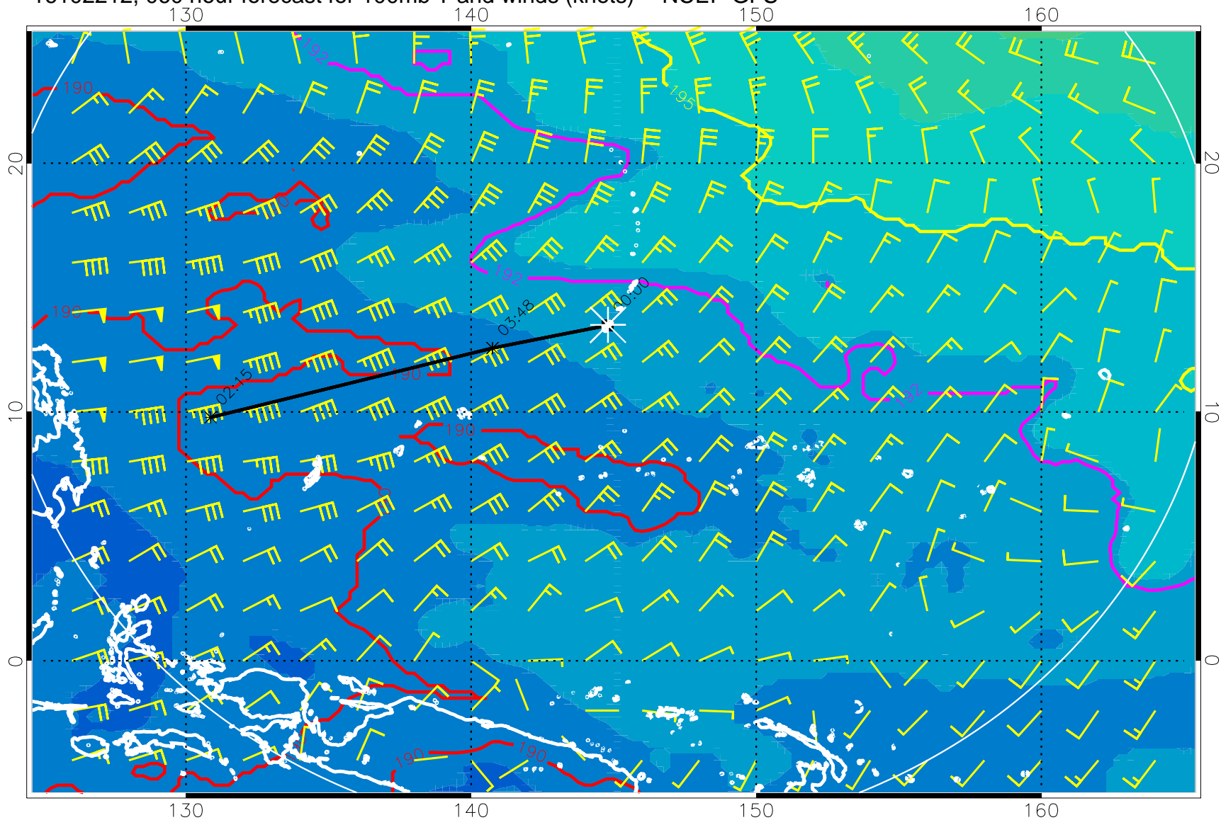
16102212, 060 hour forecast for 100mb T and winds (knots) -- NCEP GFS
