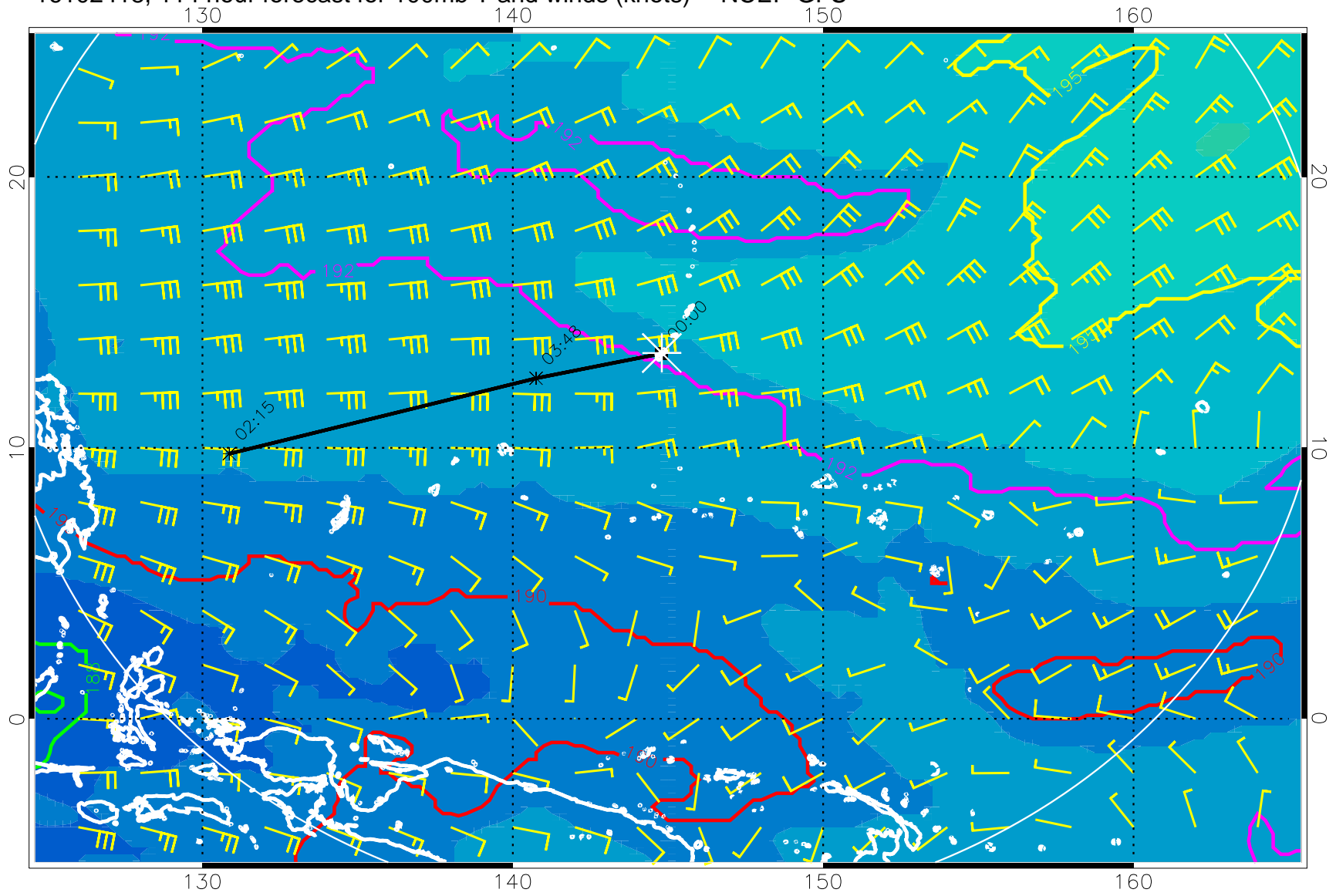
16102418, 114 hour forecast for 100mb T and winds (knots) -- NCEP GFS
