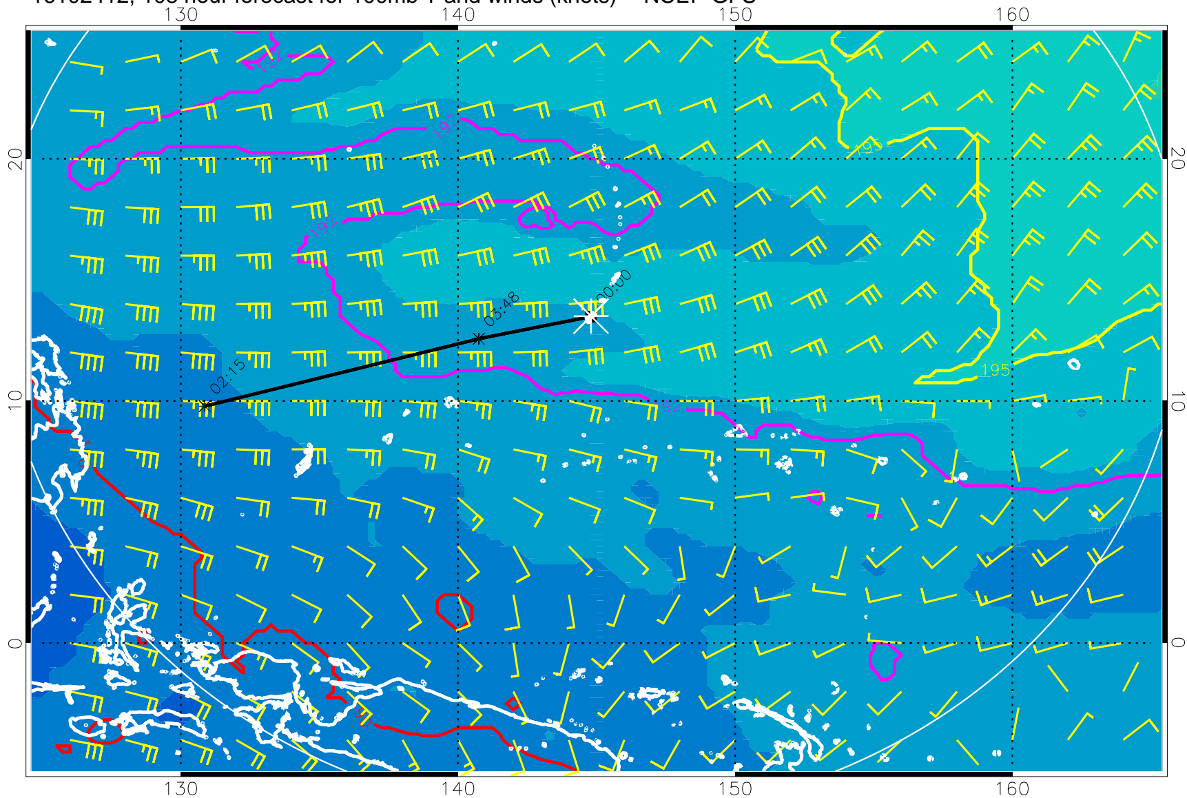
16102412, 108 hour forecast for 100mb T and winds (knots) -- NCEP GFS
