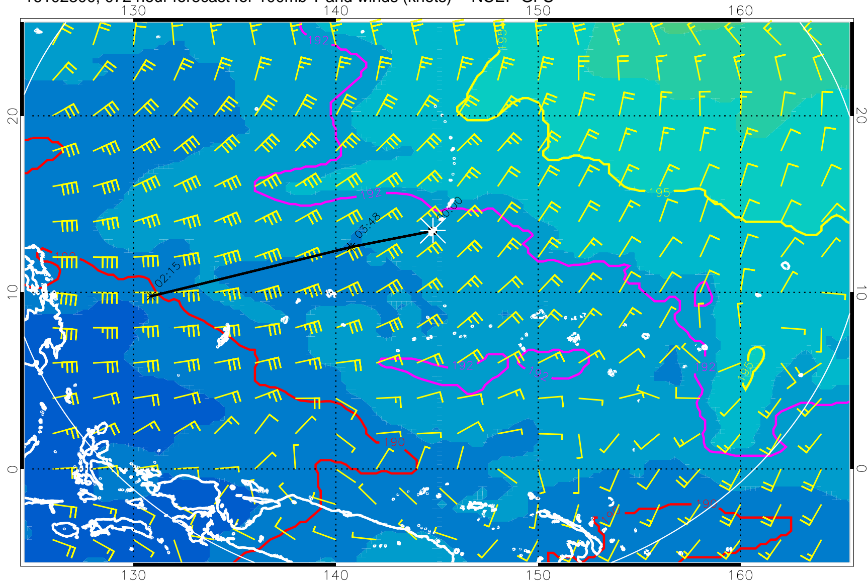
16102300, 072 hour forecast for 100mb T and winds (knots) -- NCEP GFS
