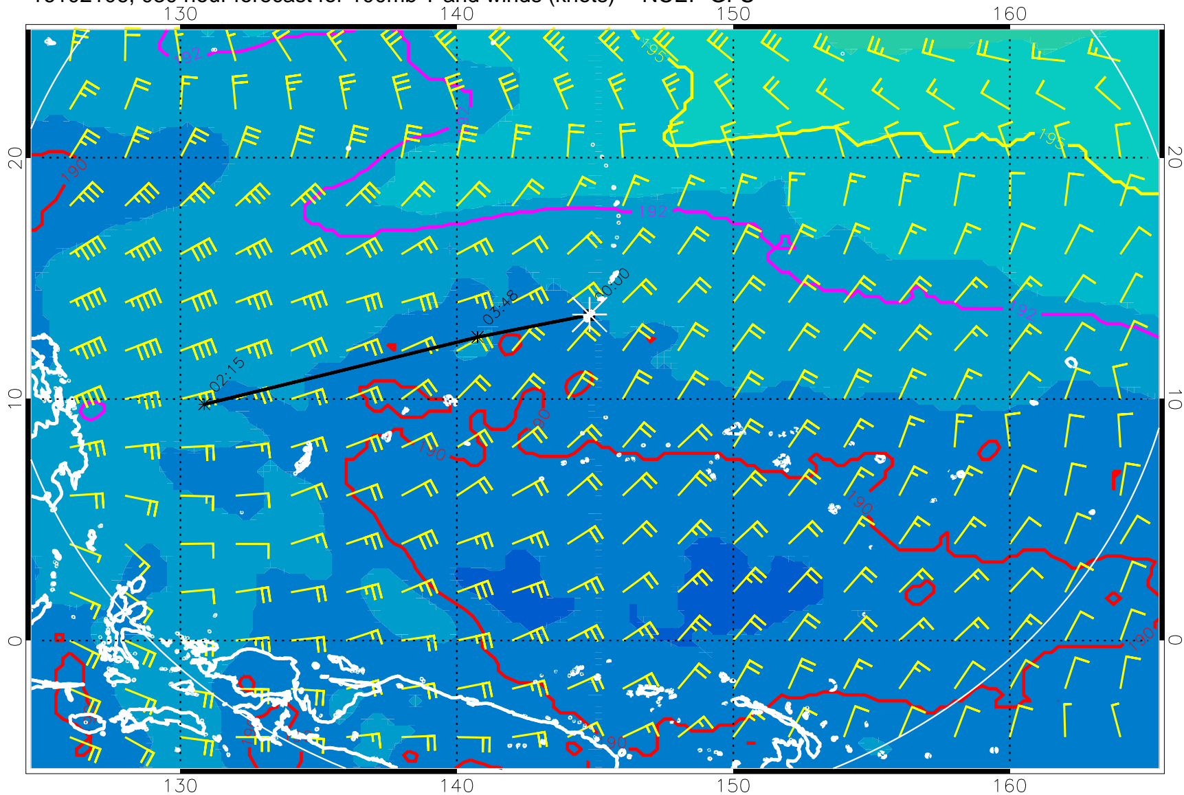
16102106, 030 hour forecast for 100mb T and winds (knots) -- NCEP GFS
