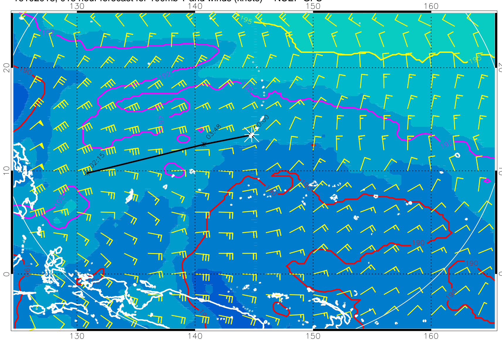
16102018, 018 hour forecast for 100mb T and winds (knots) -- NCEP GFS
