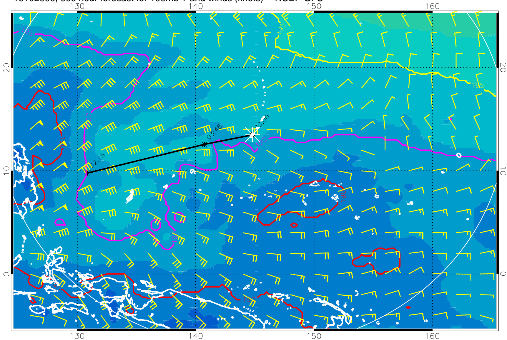
16102006, 006 hour forecast for 100mb T and winds (knots) -- NCEP GFS
