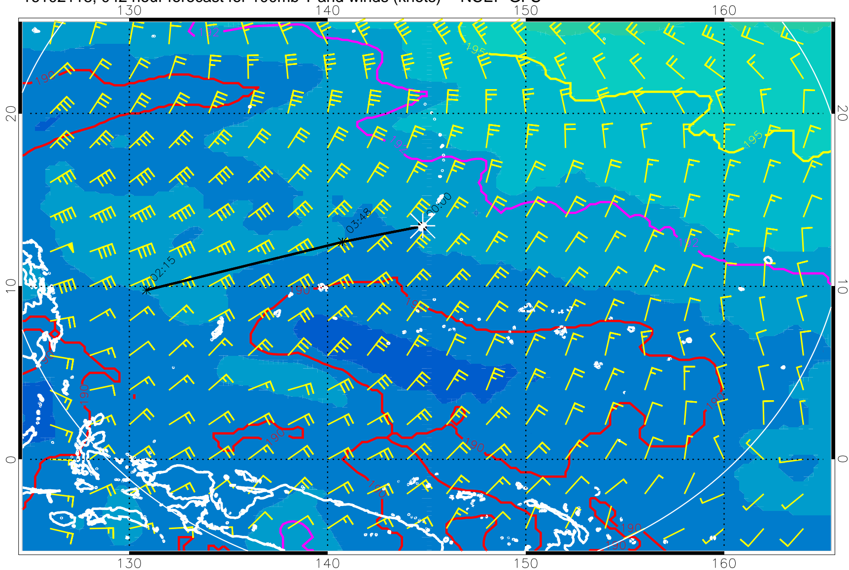
16102118, 042 hour forecast for 100mb T and winds (knots) -- NCEP GFS
