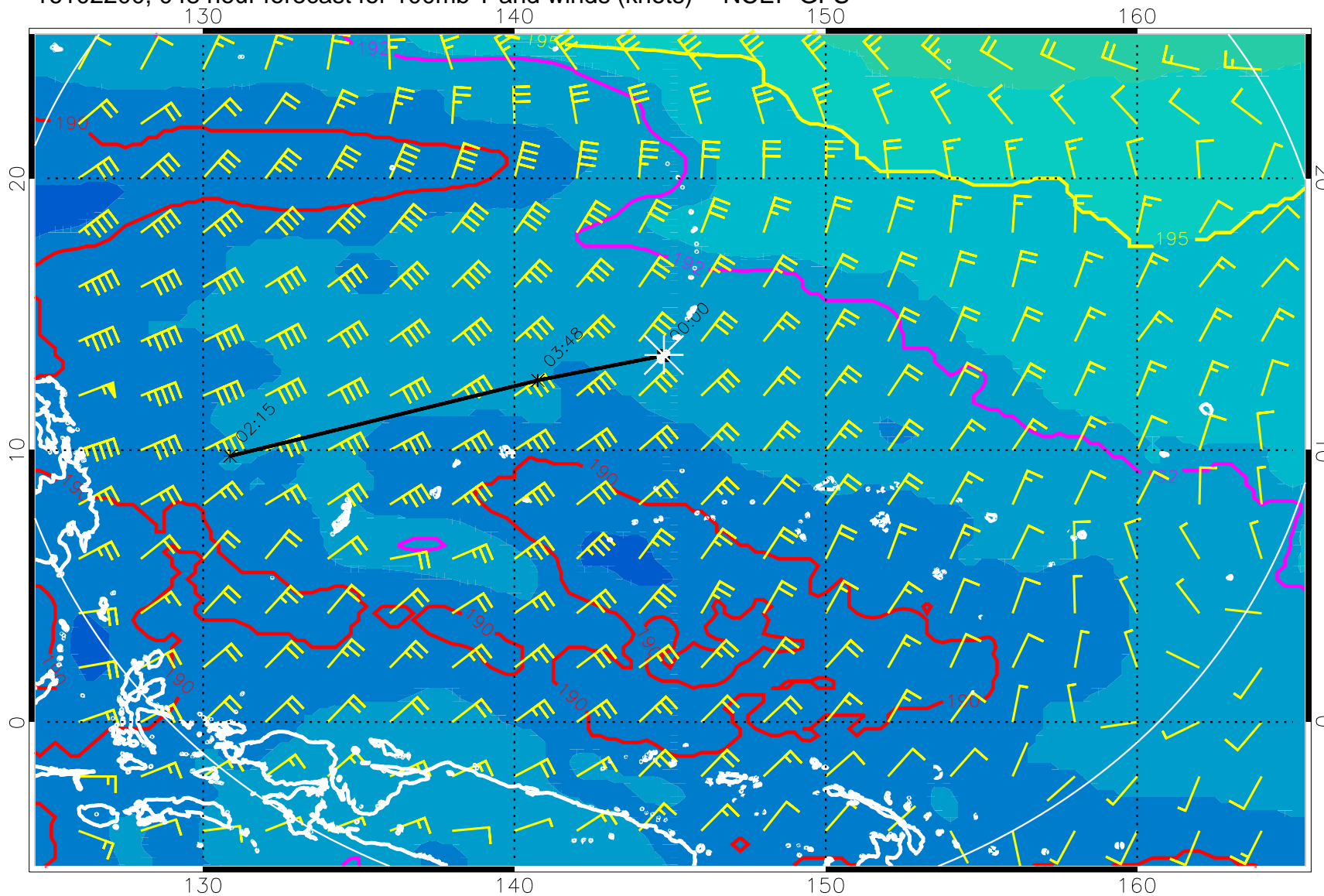
16102200, 048 hour forecast for 100mb T and winds (knots) -- NCEP GFS
