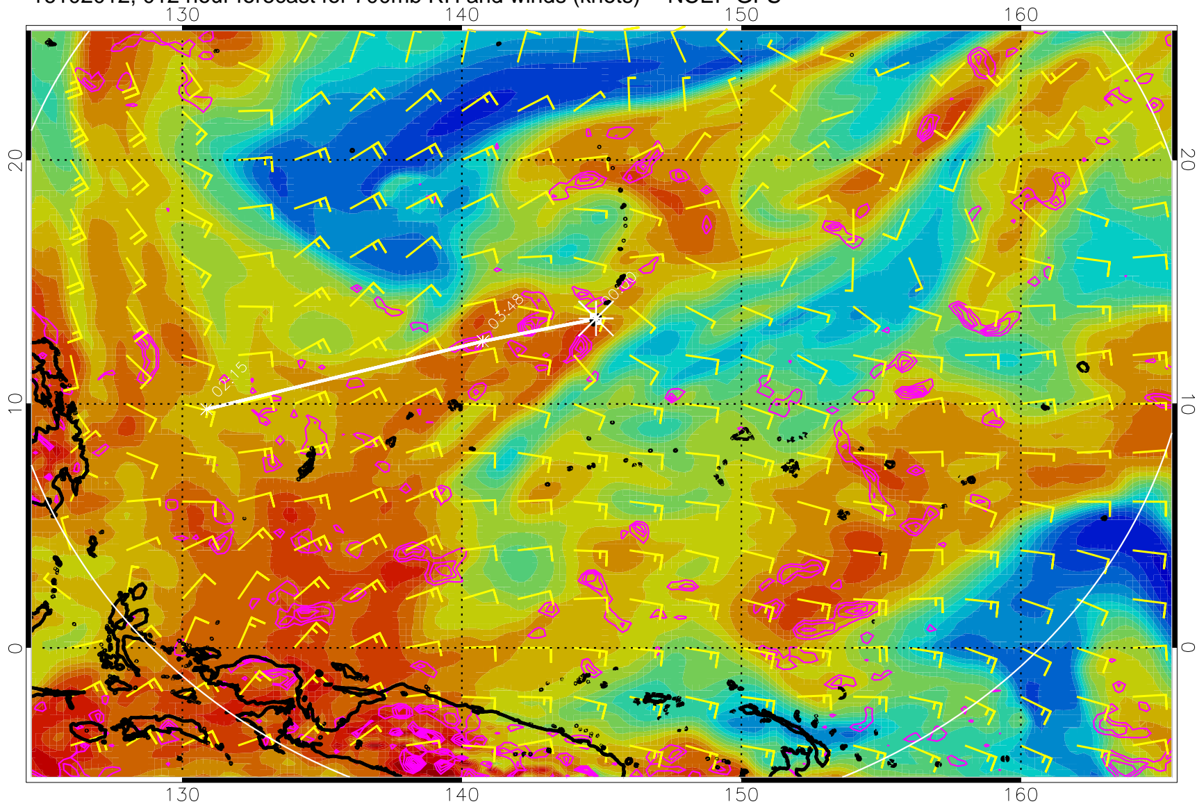
16102012, 012 hour forecast for 700mb RH and winds (knots) -- NCEP GFS
