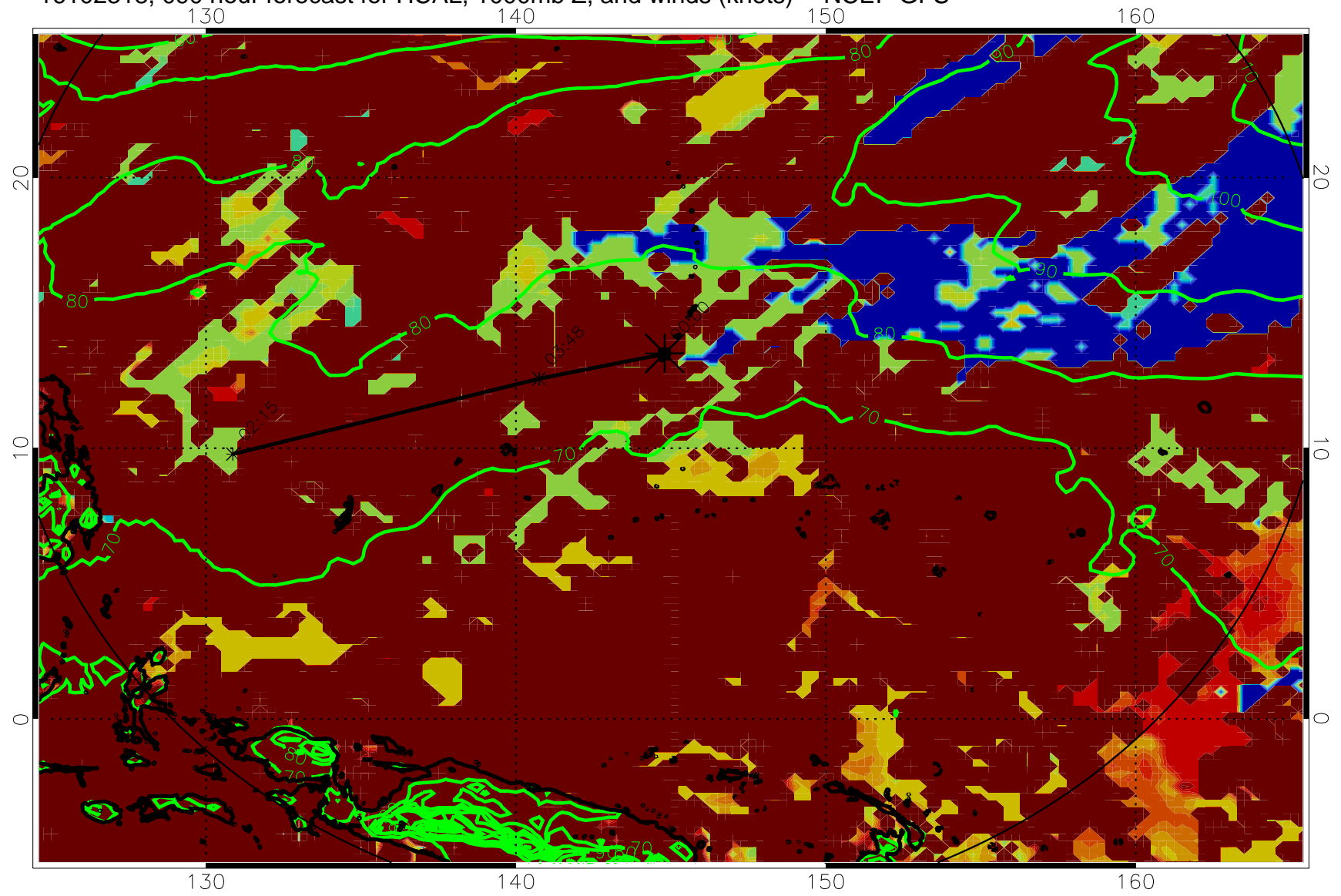
16102318, 090 hour forecast for HCAL, 1000mb Z, and winds (knots) -- NCEP GFS
