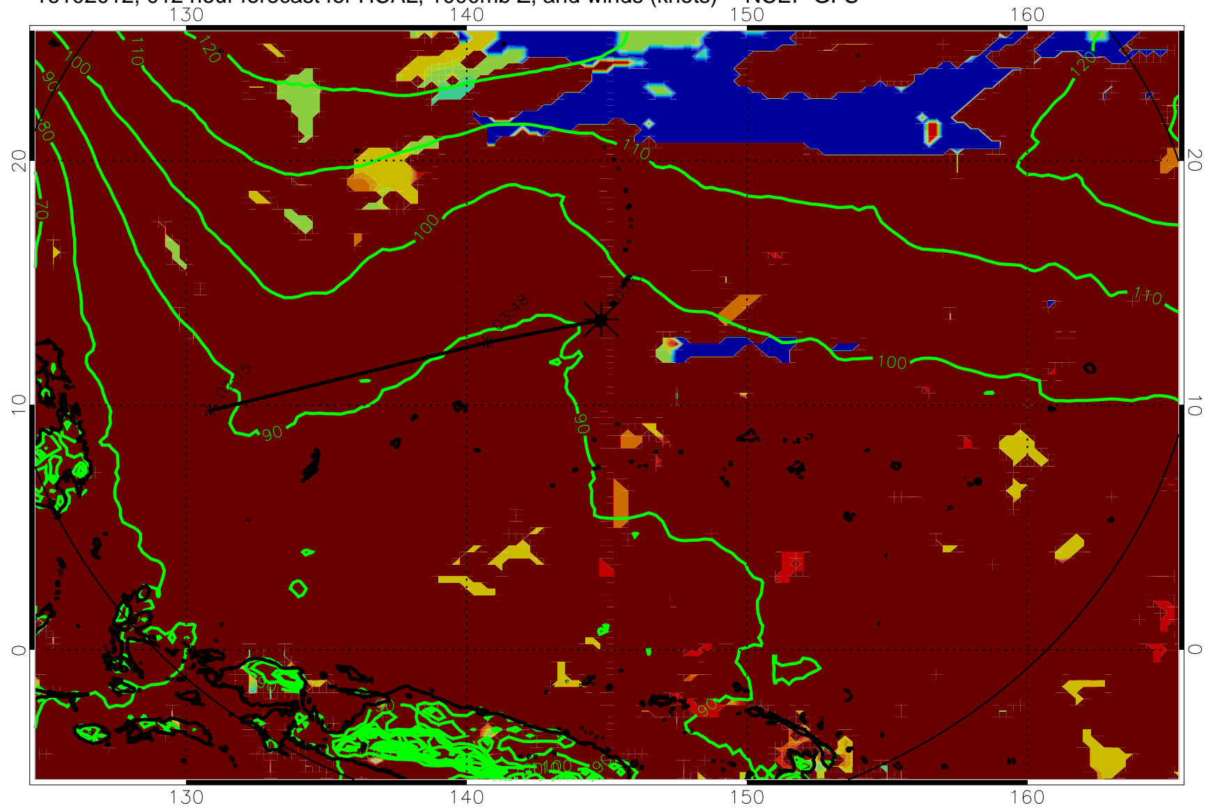
16102012, 012 hour forecast for HCAL, 1000mb Z, and winds (knots) -- NCEP GFS
