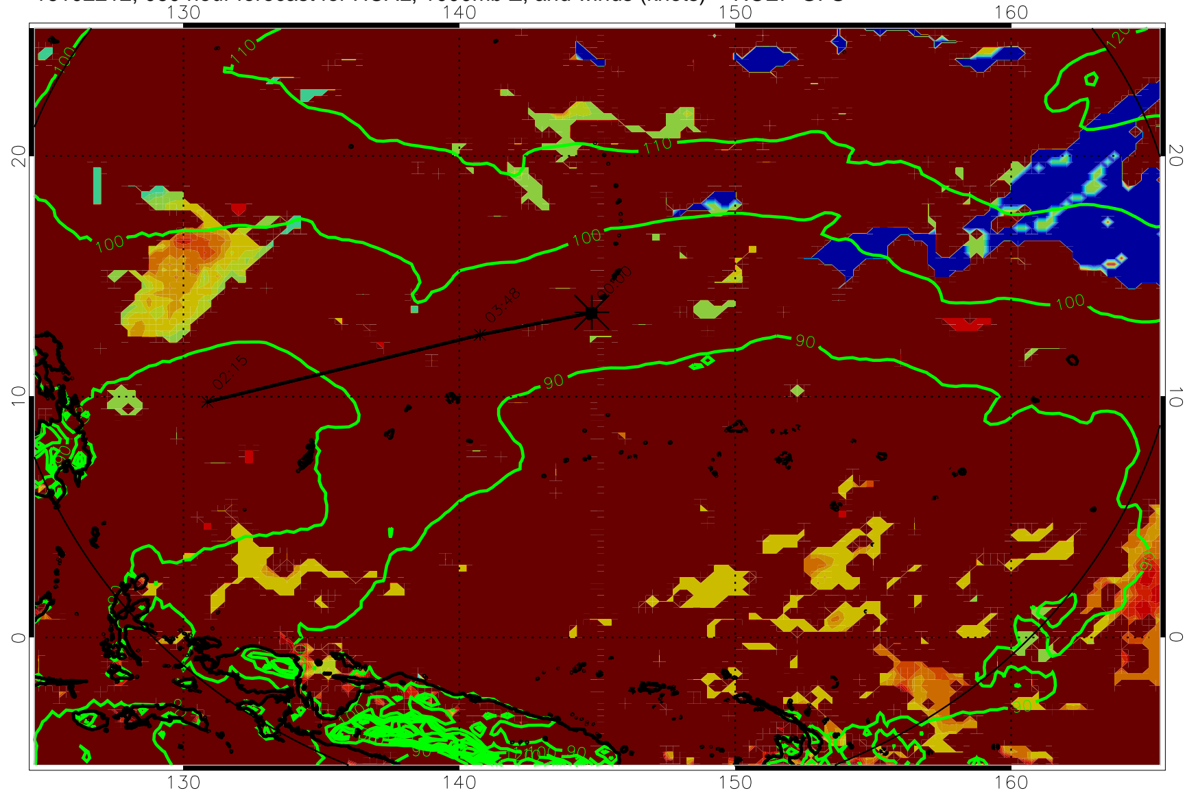
16102212, 060 hour forecast for HCAL, 1000mb Z, and winds (knots) -- NCEP GFS
