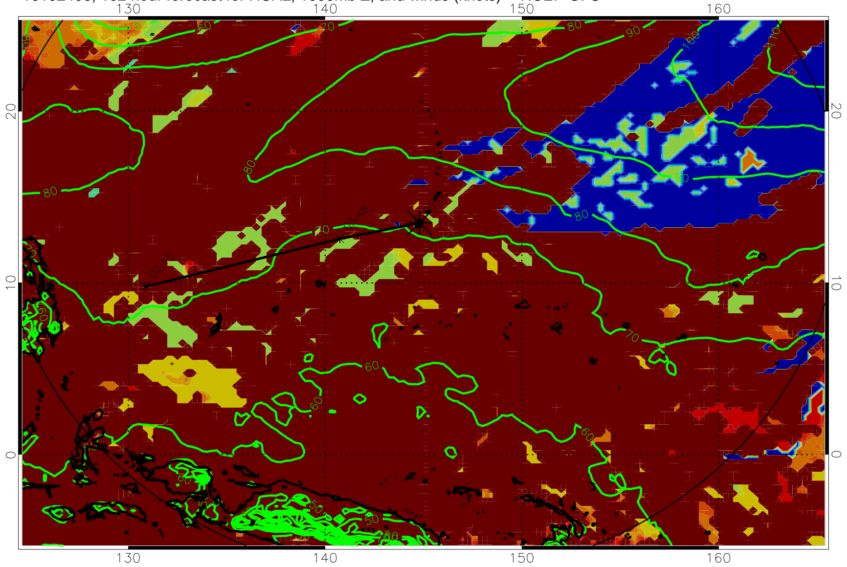
16102406, 102 hour forecast for HCAL, 1000mb Z, and winds (knots) -- NCEP GFS
