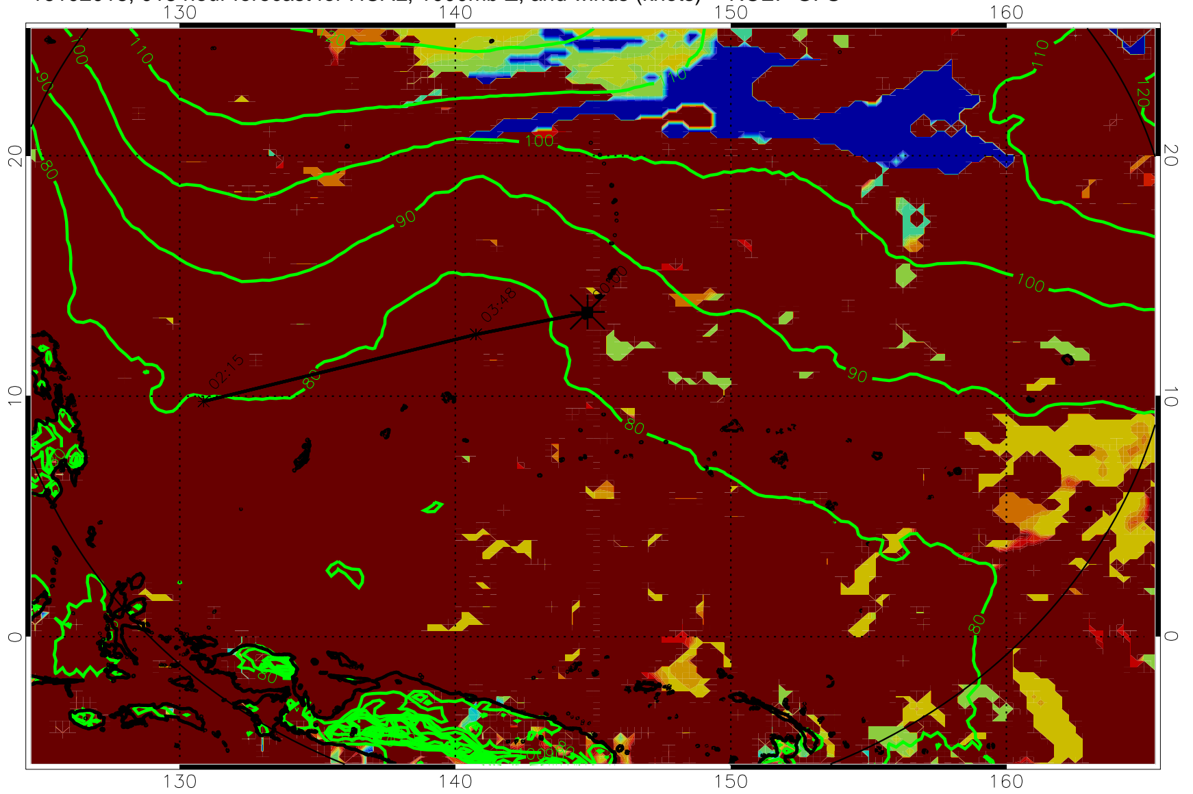
16102018, 018 hour forecast for HCAL, 1000mb Z, and winds (knots) -- NCEP GFS
