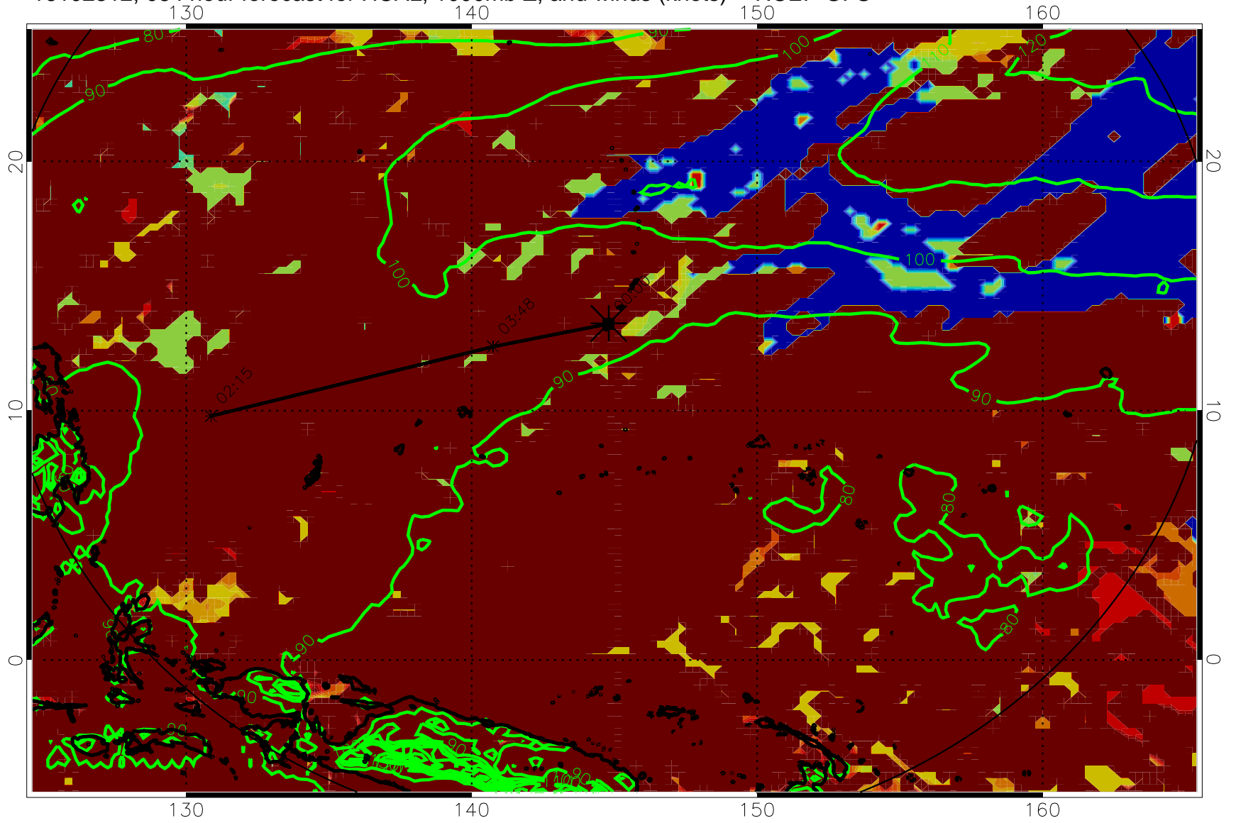
16102312, 084 hour forecast for HCAL, 1000mb Z, and winds (knots) -- NCEP GFS
