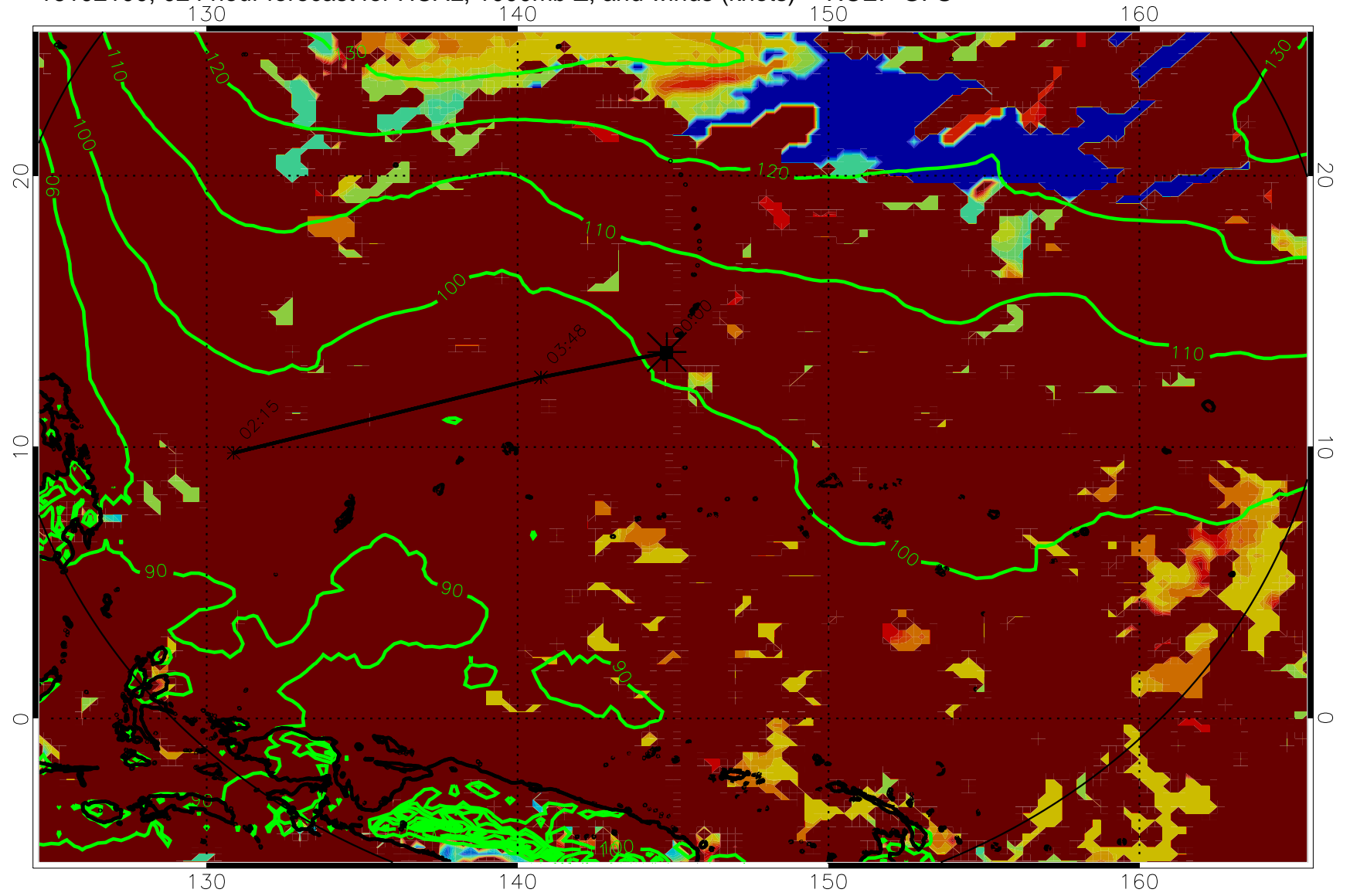
16102100, 024 hour forecast for HCAL, 1000mb Z, and winds (knots) -- NCEP GFS
