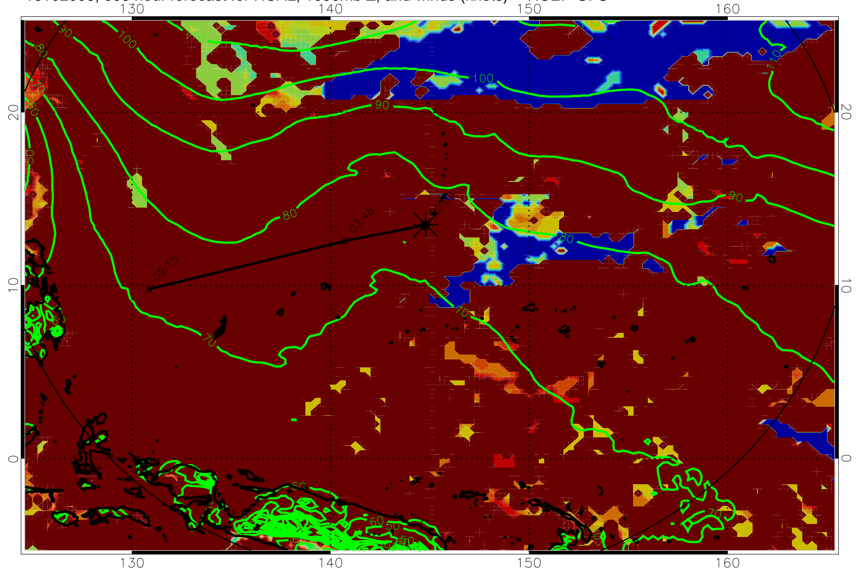
16102006, 006 hour forecast for HCAL, 1000mb Z, and winds (knots) -- NCEP GFS
