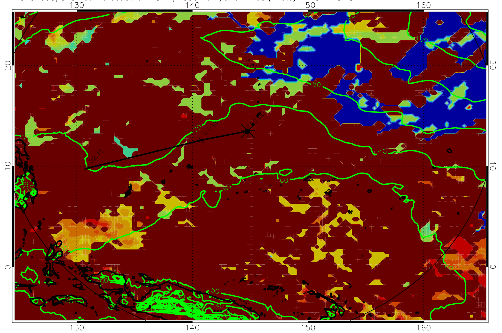
16102306, 078 hour forecast for HCAL, 1000mb Z, and winds (knots) -- NCEP GFS
