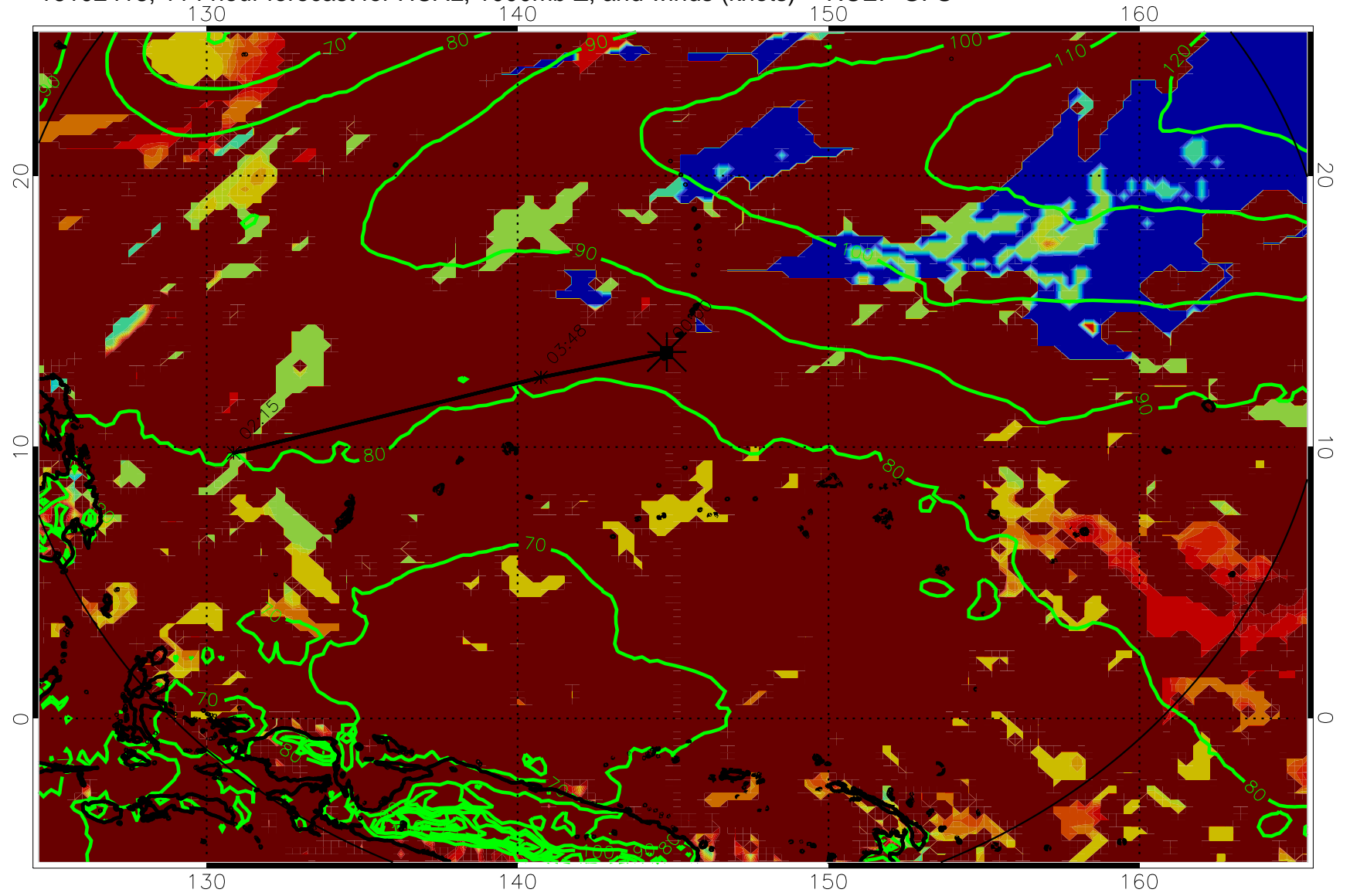
16102418, 114 hour forecast for HCAL, 1000mb Z, and winds (knots) -- NCEP GFS
