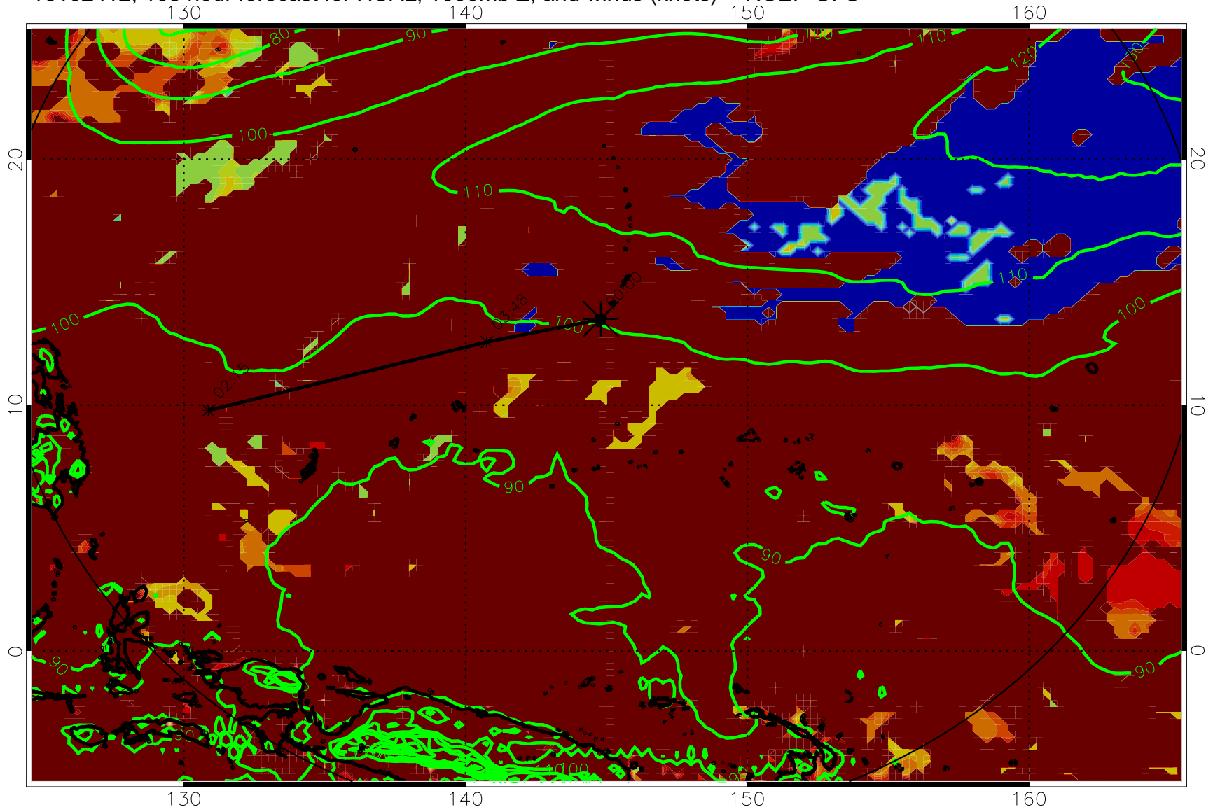
16102412, 108 hour forecast for HCAL, 1000mb Z, and winds (knots) -- NCEP GFS
