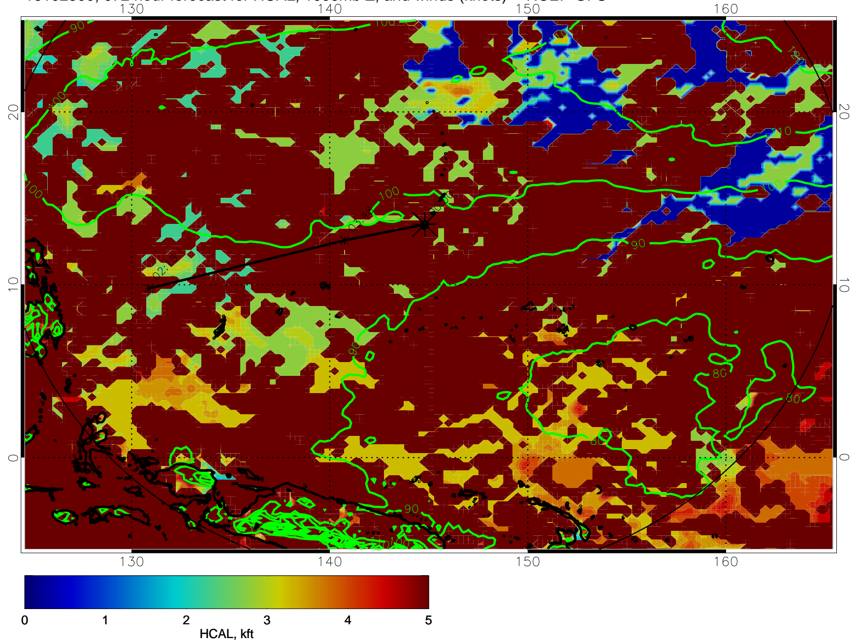
16102300, 072 hour forecast for HCAL, 1000mb Z, and winds (knots) -- NCEP GFS
