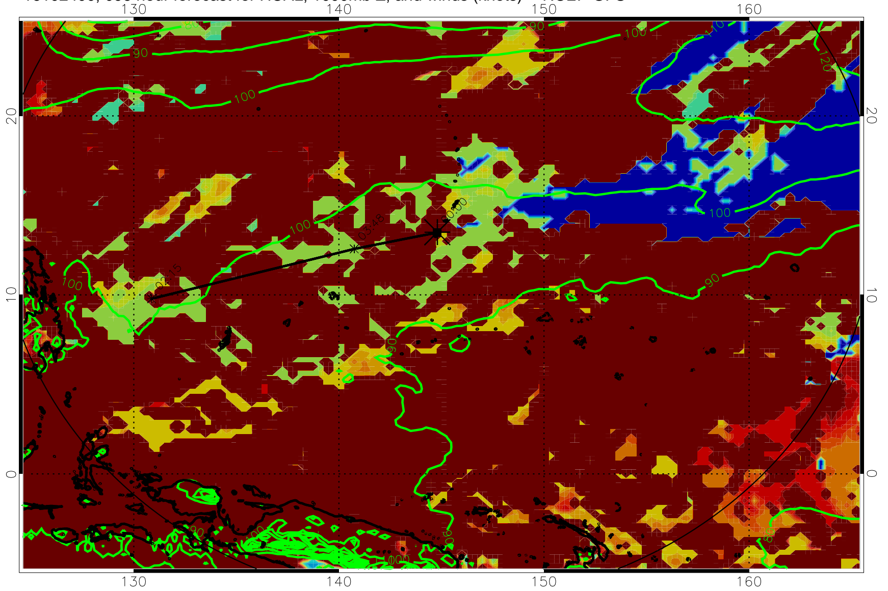
16102400, 096 hour forecast for HCAL, 1000mb Z, and winds (knots) -- NCEP GFS
