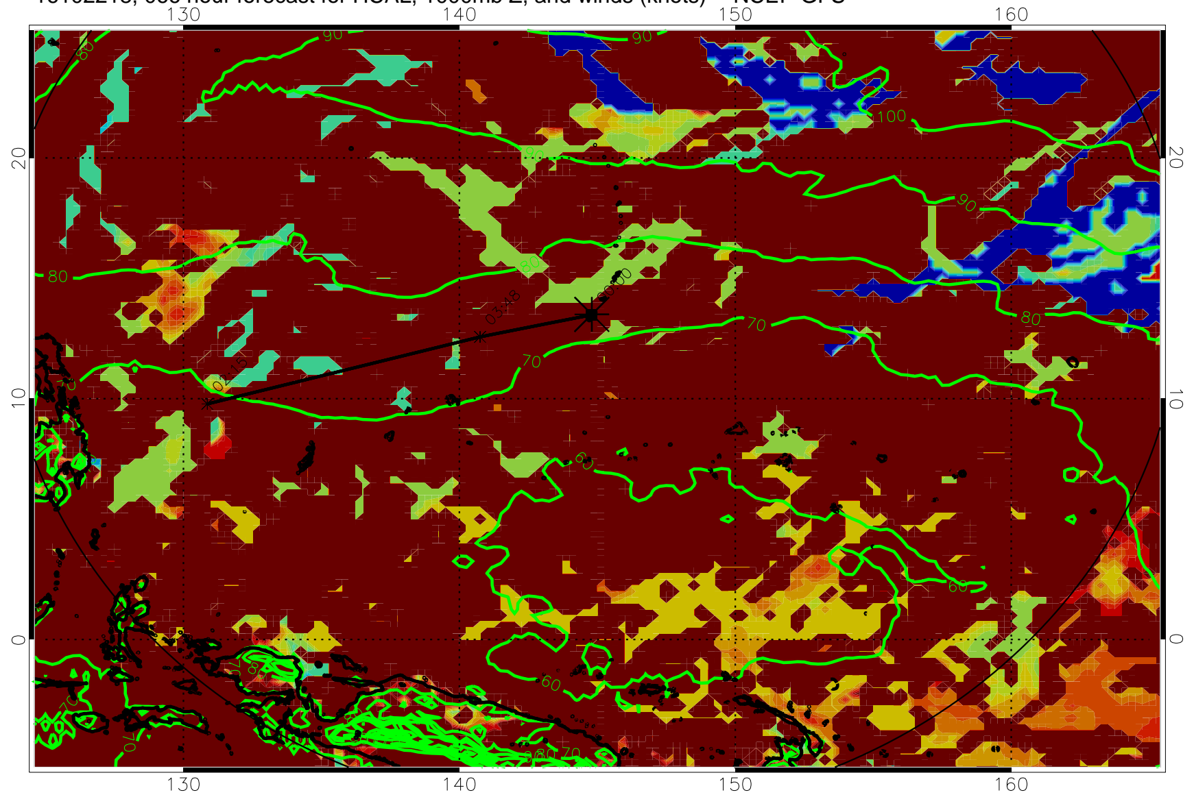
16102218, 066 hour forecast for HCAL, 1000mb Z, and winds (knots) -- NCEP GFS
