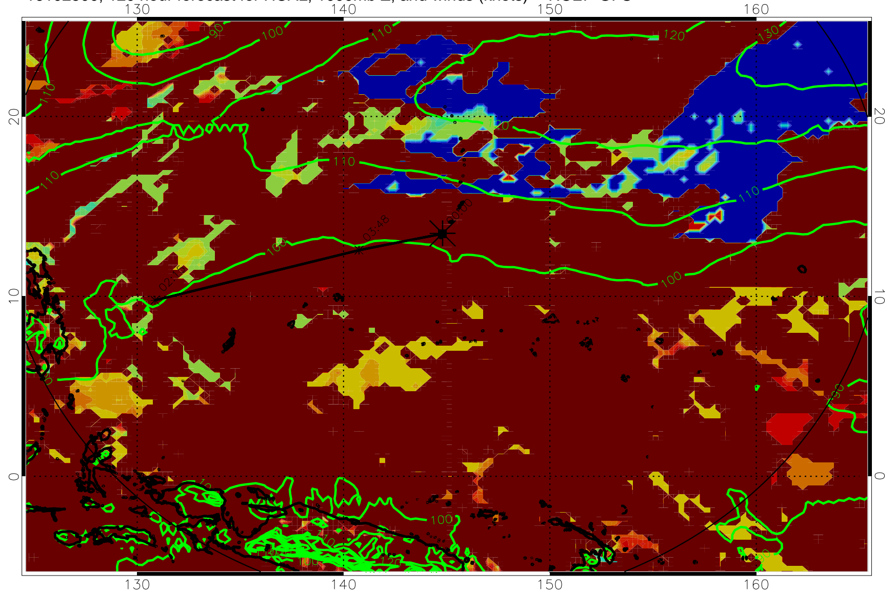
16102500, 120 hour forecast for HCAL, 1000mb Z, and winds (knots) -- NCEP GFS
