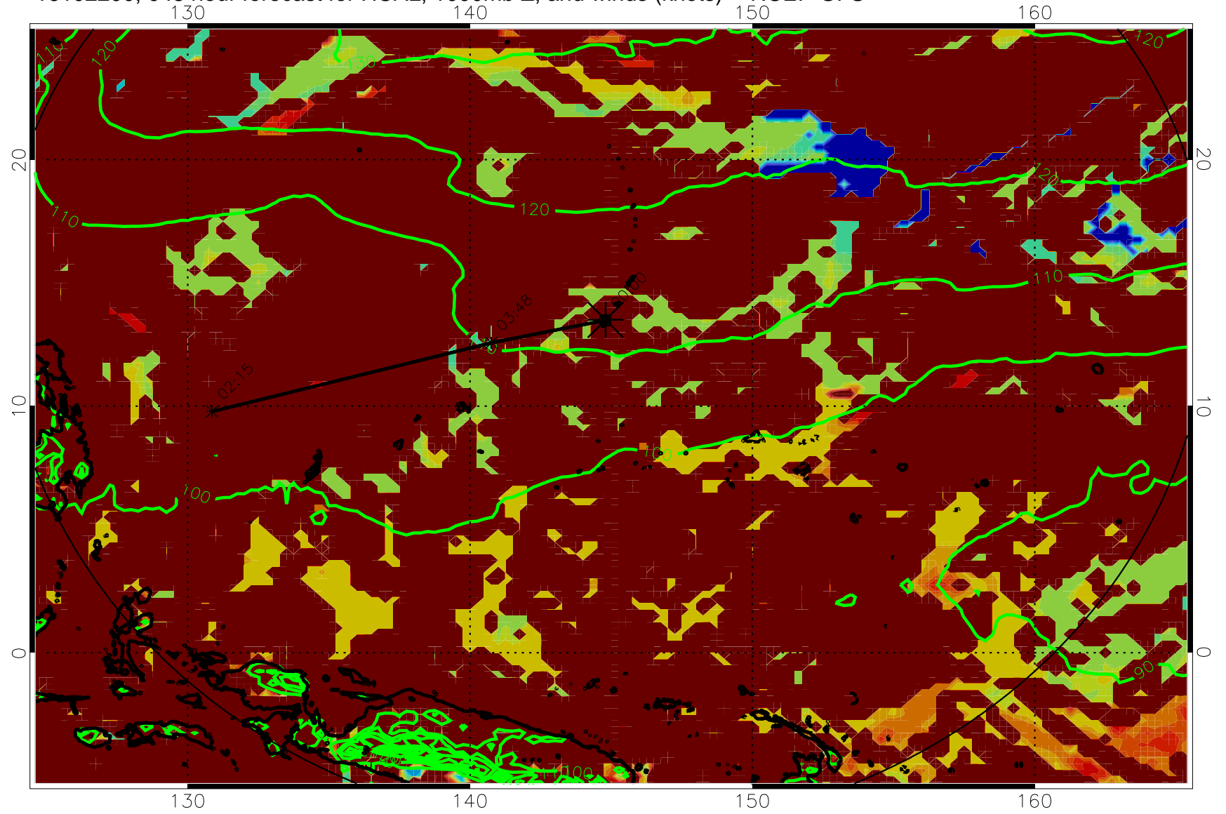
16102200, 048 hour forecast for HCAL, 1000mb Z, and winds (knots) -- NCEP GFS
