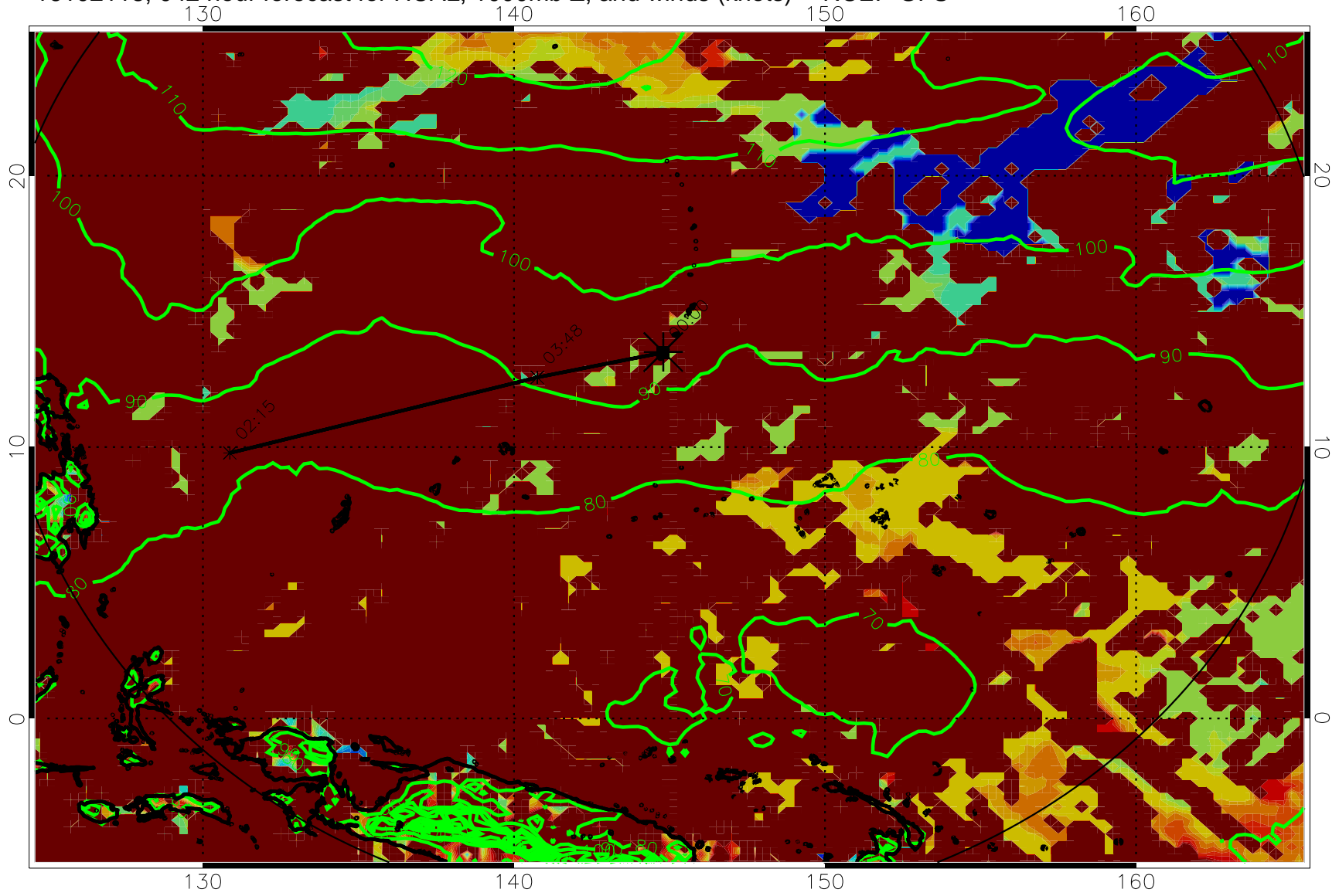
16102118, 04Z hour forecast for HCAL, 1000mb Z, and winds (knots) -- NCEP GFS
