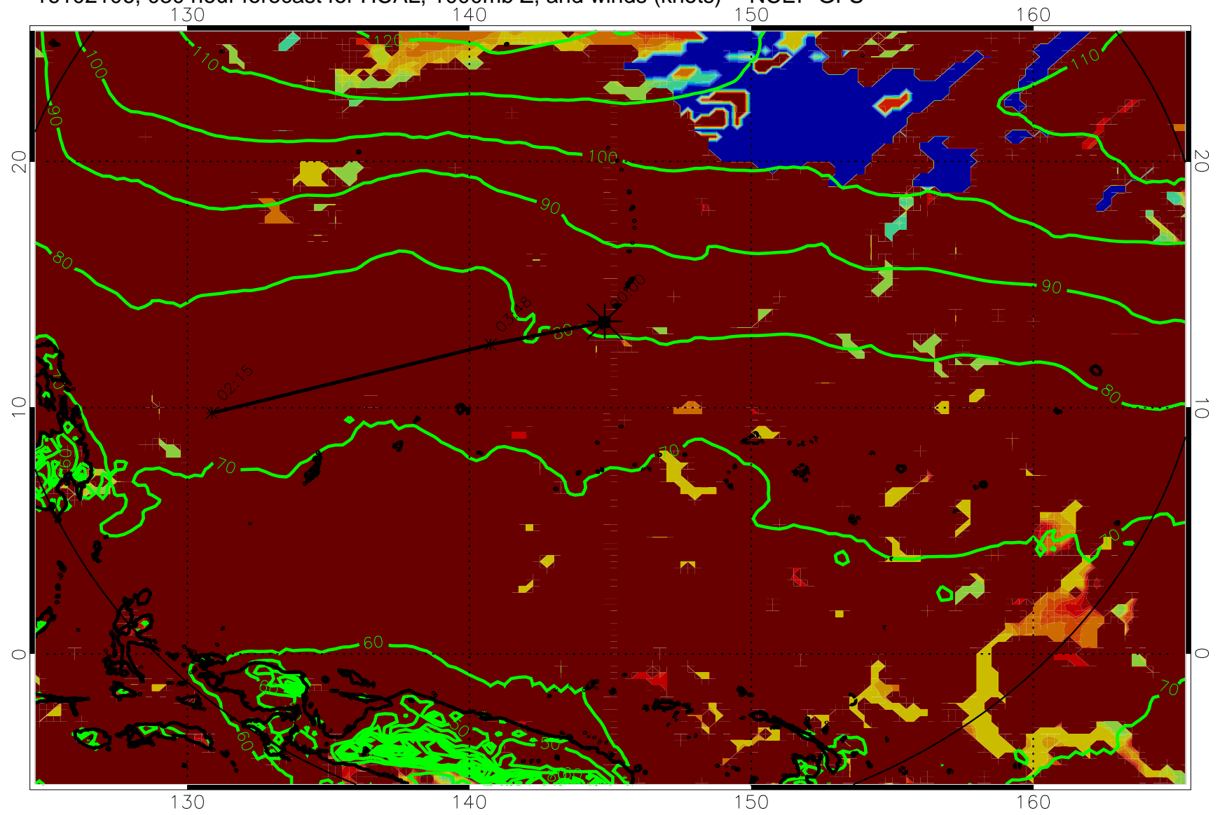
16102106, 030 hour forecast for HCAL, 1000mb Z, and winds (knots) -- NCEP GFS
