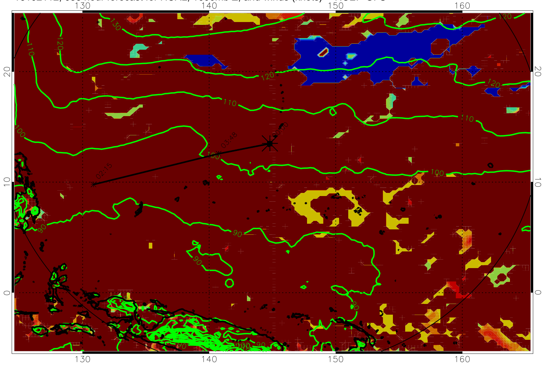
16102112, 036 hour forecast for HCAL, 1000mb Z, and winds (knots) -- NCEP GFS
