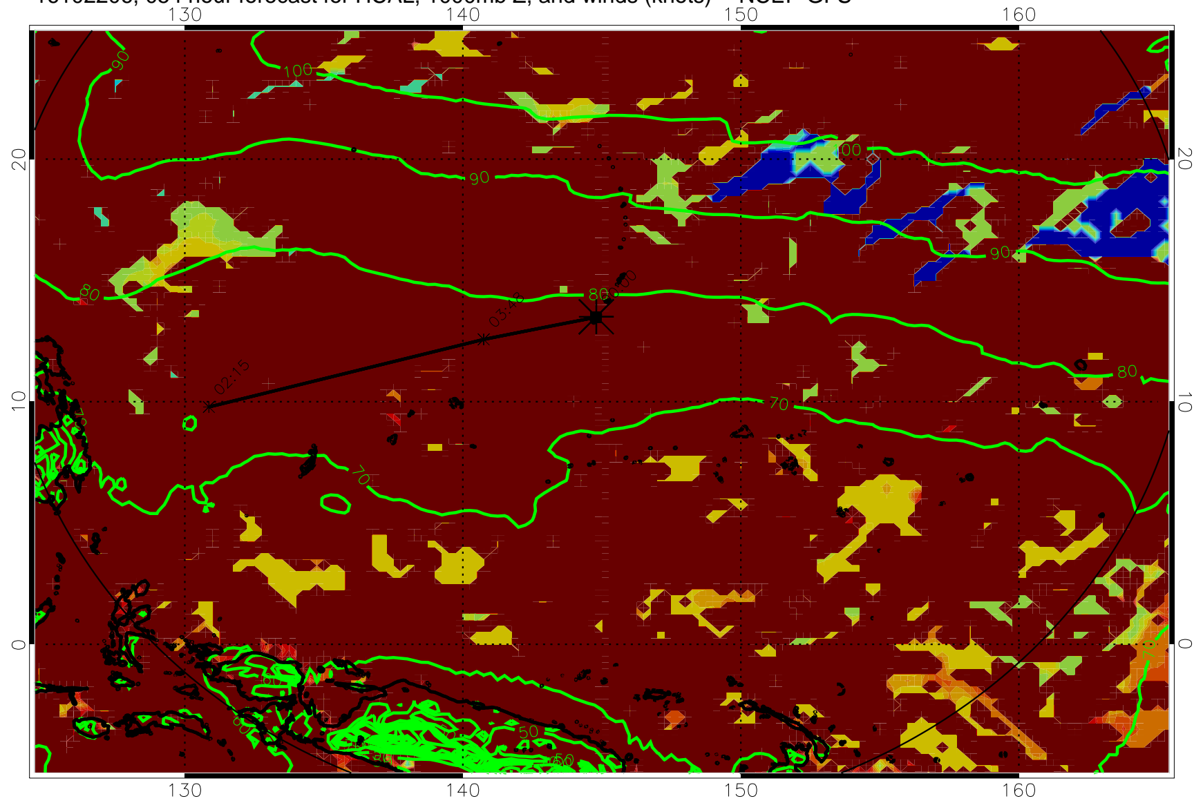
16102206, 054 hour forecast for HCAL, 1000mb Z, and winds (knots) -- NCEP GFS
