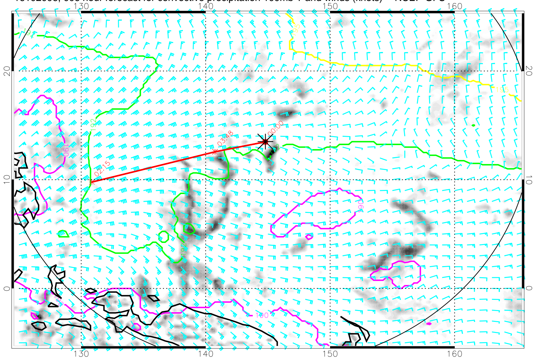
16102006, 006 hour forecast for convective precipitation 100mb T and winds (knots) -- NCEP GFS
