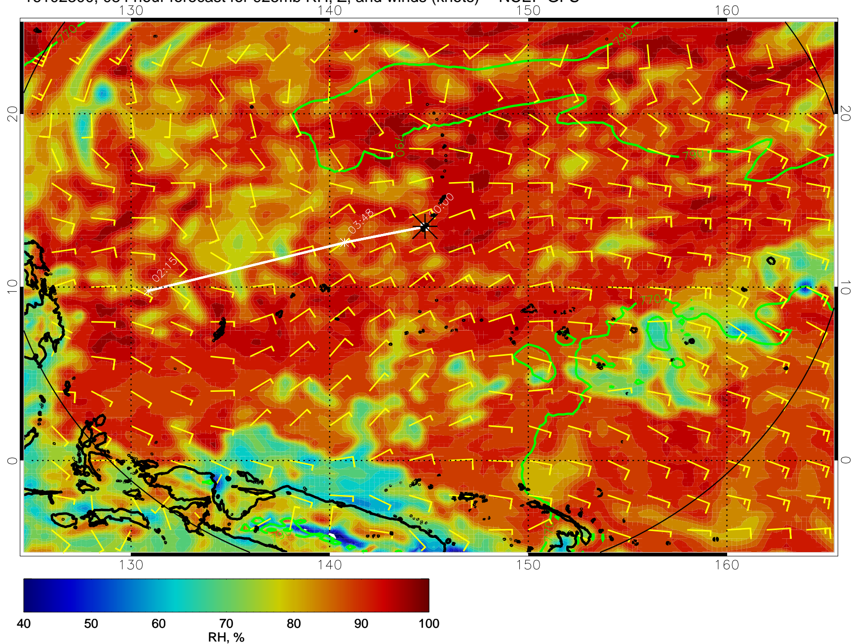
16102300, 084 hour forecast for 925mb RH, Z, and winds (knots) -- NCEP GFS
