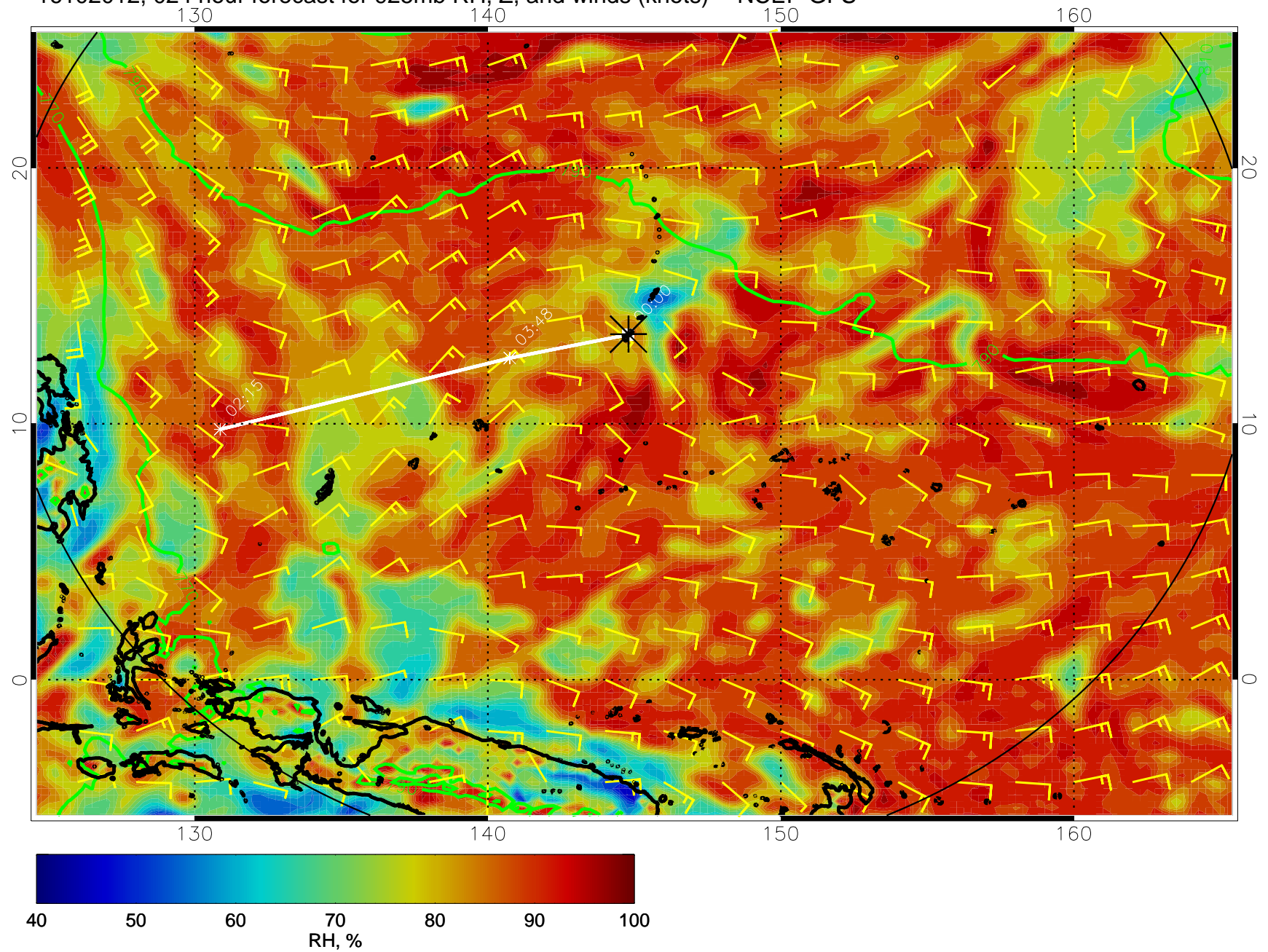
16102012, 024 hour forecast for 925mb RH, Z, and winds (knots) -- NCEP GFS
