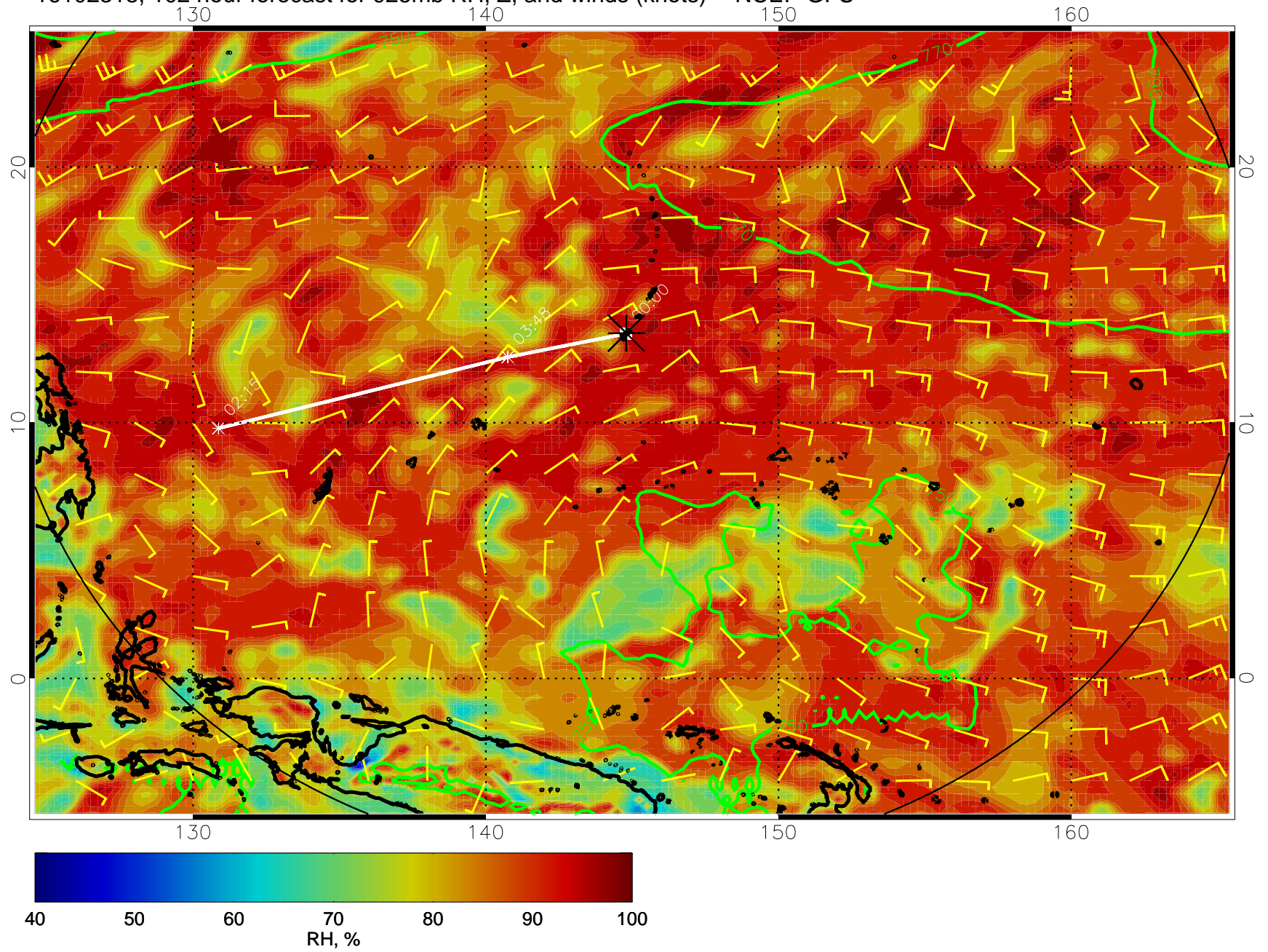
16102318, 102 hour forecast for 925mb RH, Z, and winds (knots) -- NCEP GFS
