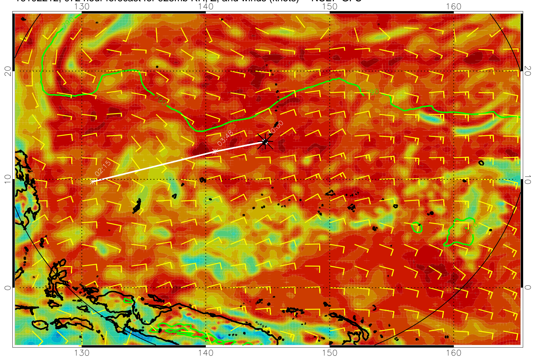
16102212, 072 hour forecast for 925mb RH, Z, and winds (knots) -- NCEP GFS
