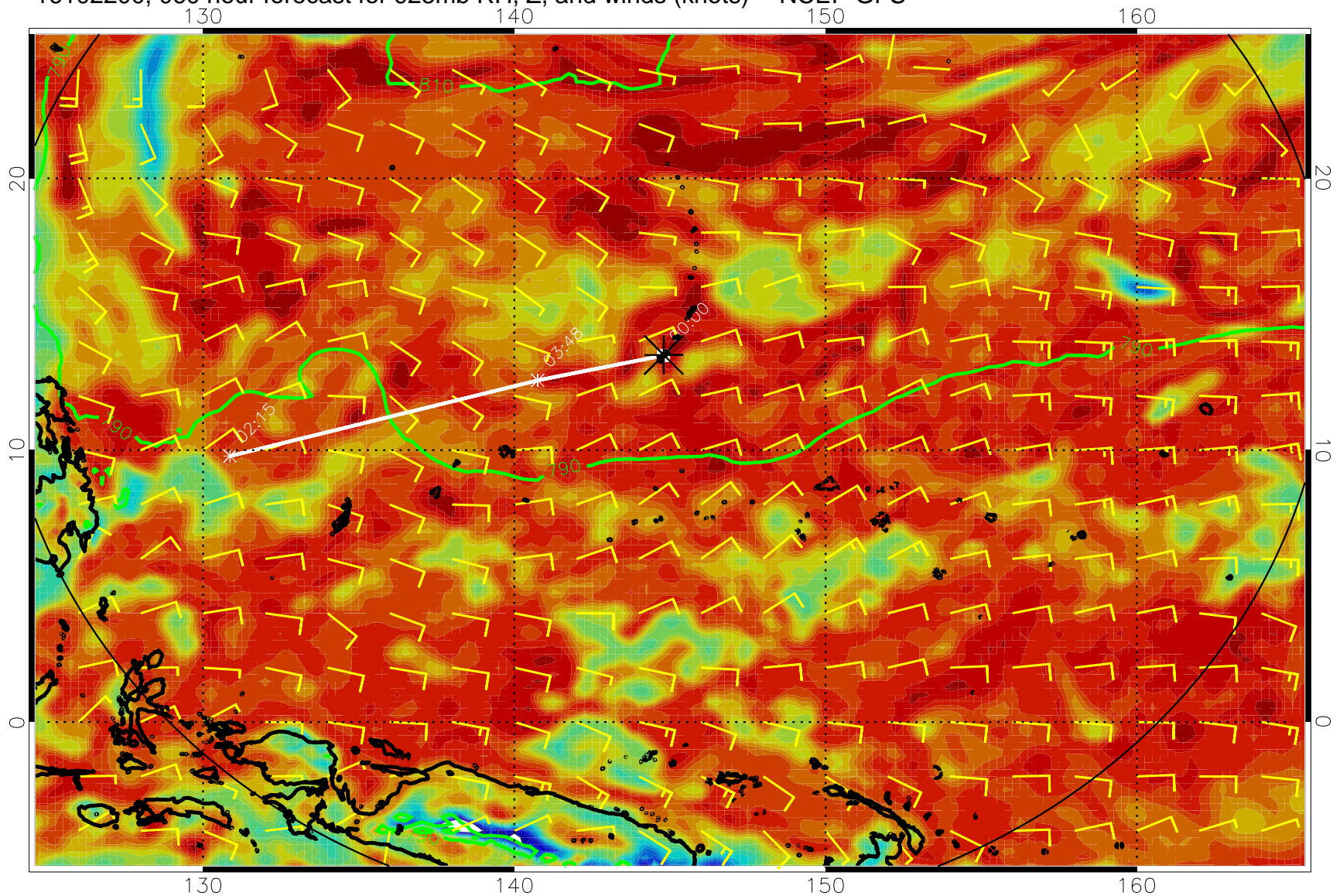
16102200, 060 hour forecast for 925mb RH, Z, and winds (knots) -- NCEP GFS
