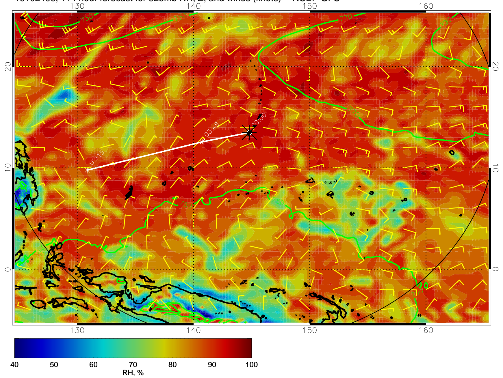
16102406, 114 hour forecast for 925mb RH, Z, and winds (knots) -- NCEP GFS
