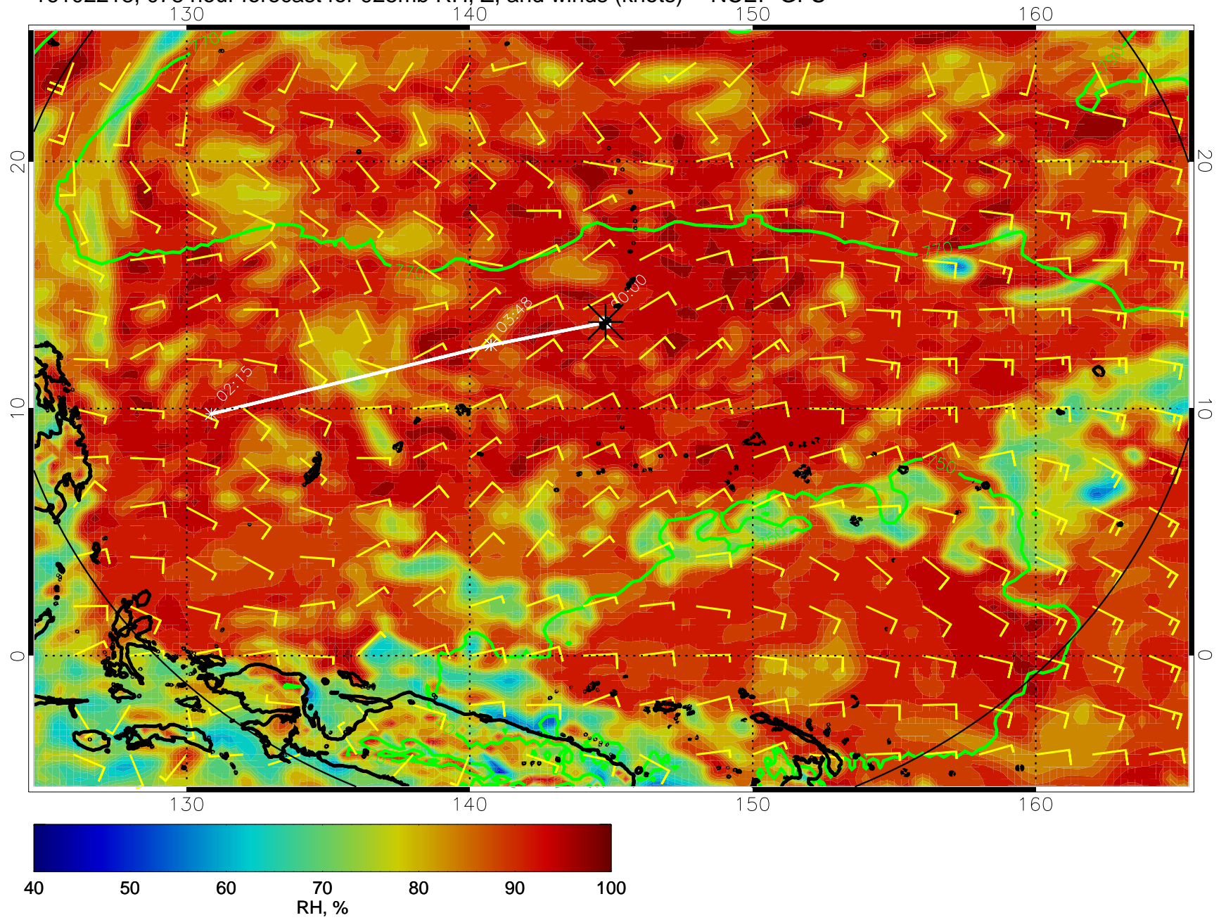
16102218, 078 hour forecast for 925mb RH, Z, and winds (knots) -- NCEP GFS
