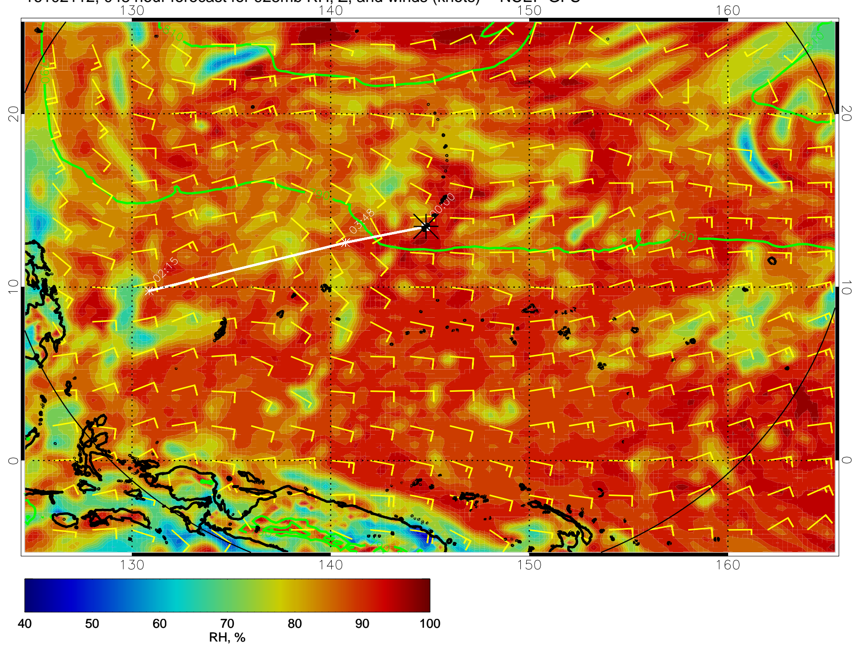
16102112, 048 hour forecast for 925mb RH, Z, and winds (knots) -- NCEP GFS
