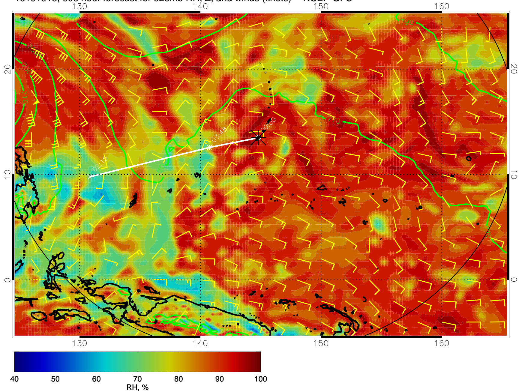
16101918, 006 hour forecast for 925mb RH, Z, and winds (knots) -- NCEP GFS
