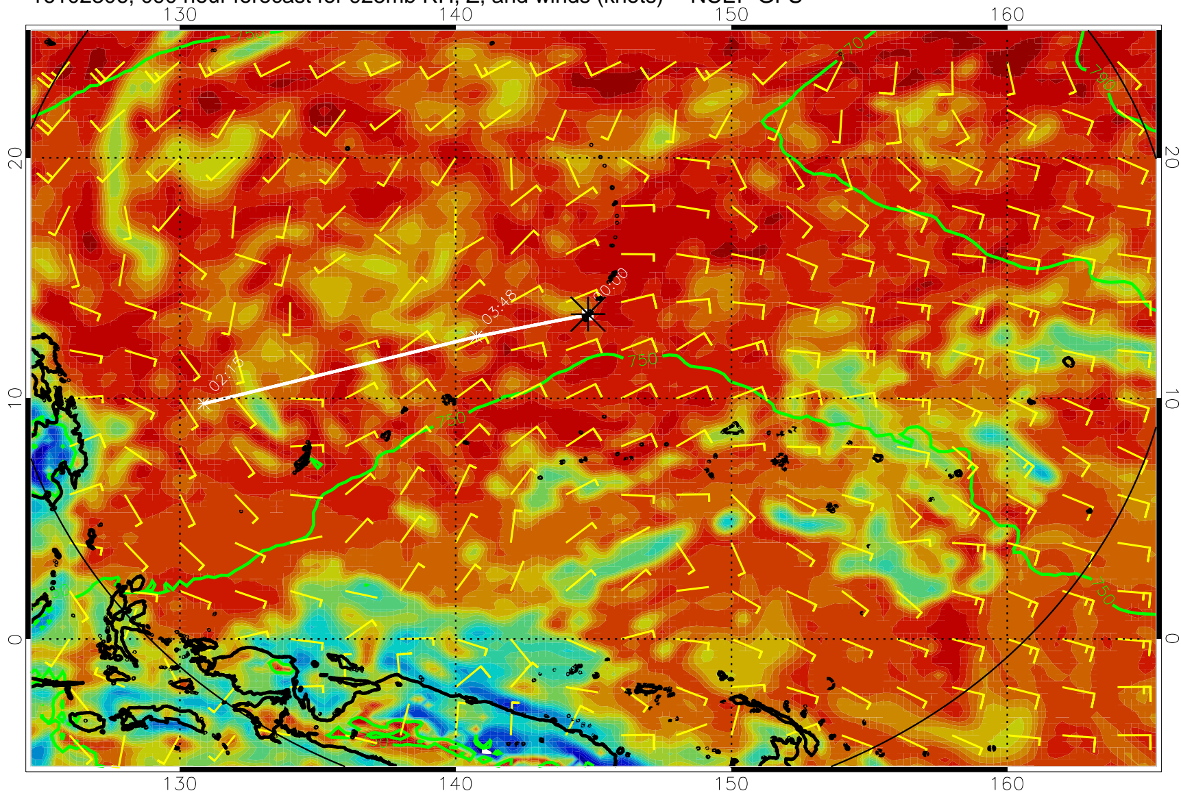
16102306, 090 hour forecast for 925mb RH, Z, and winds (knots) -- NCEP GFS
