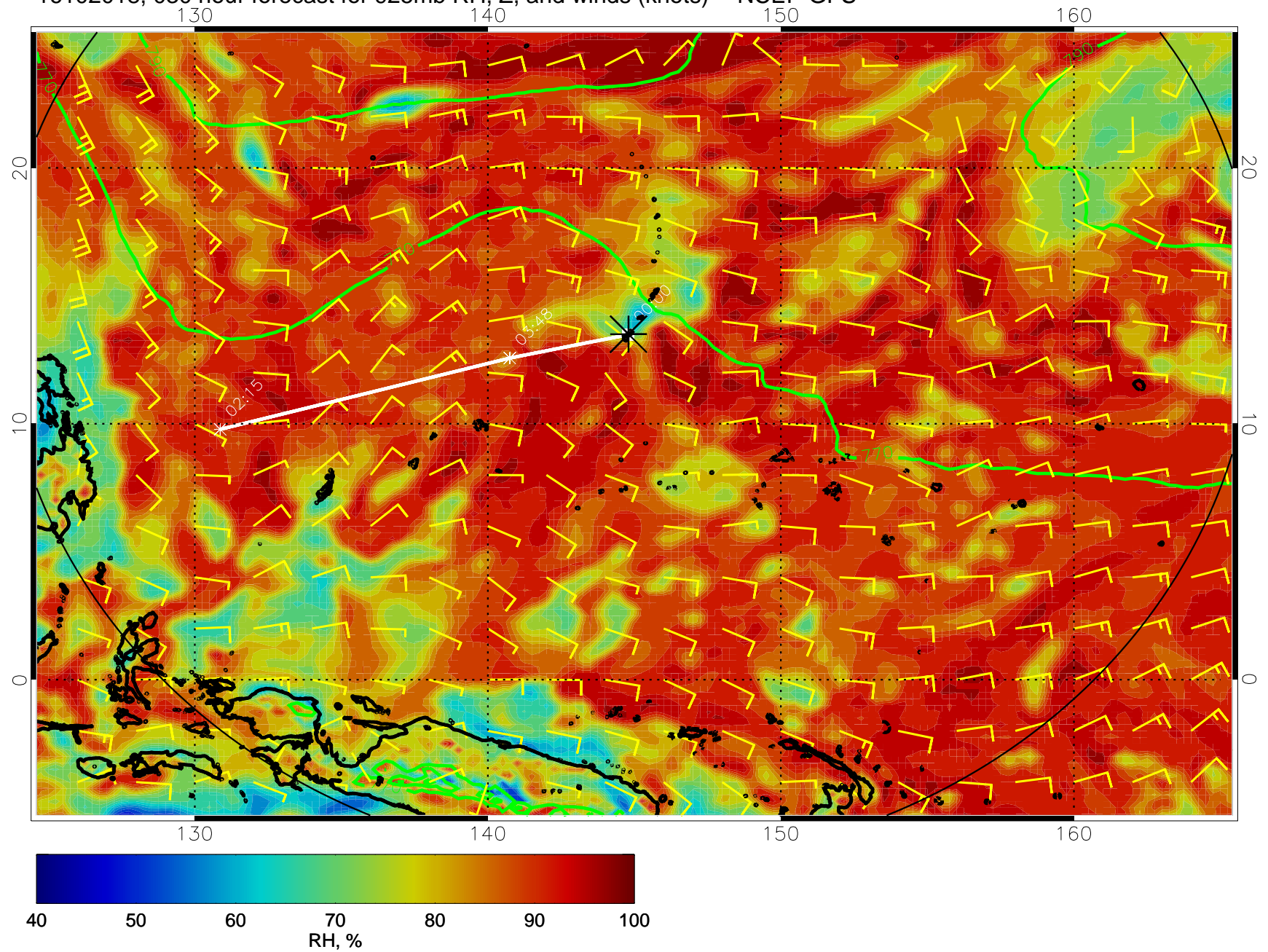
16102018, 030 hour forecast for 925mb RH, Z, and winds (knots) -- NCEP GFS
