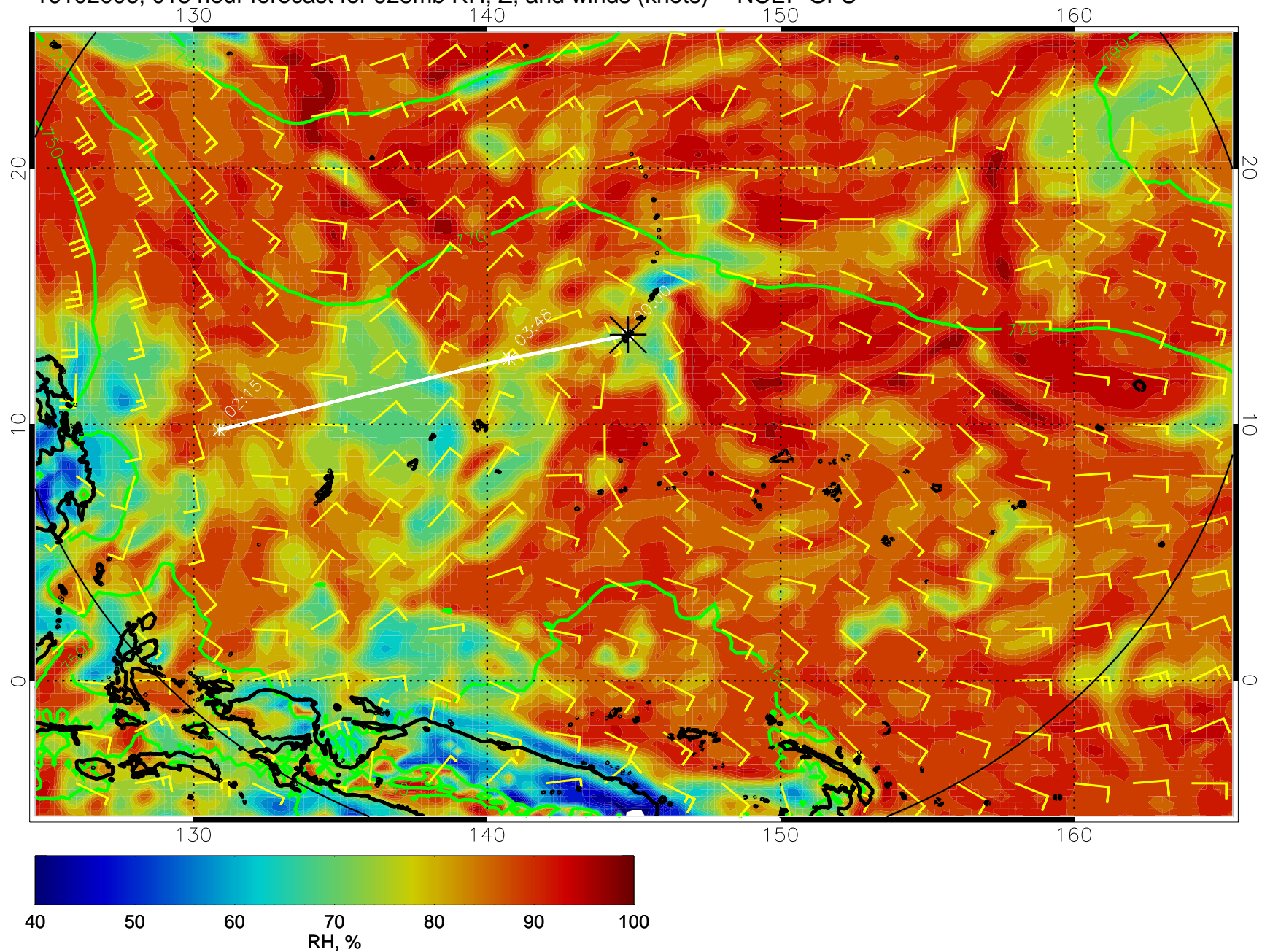
16102006, 018 hour forecast for 925mb RH, Z, and winds (knots) -- NCEP GFS
