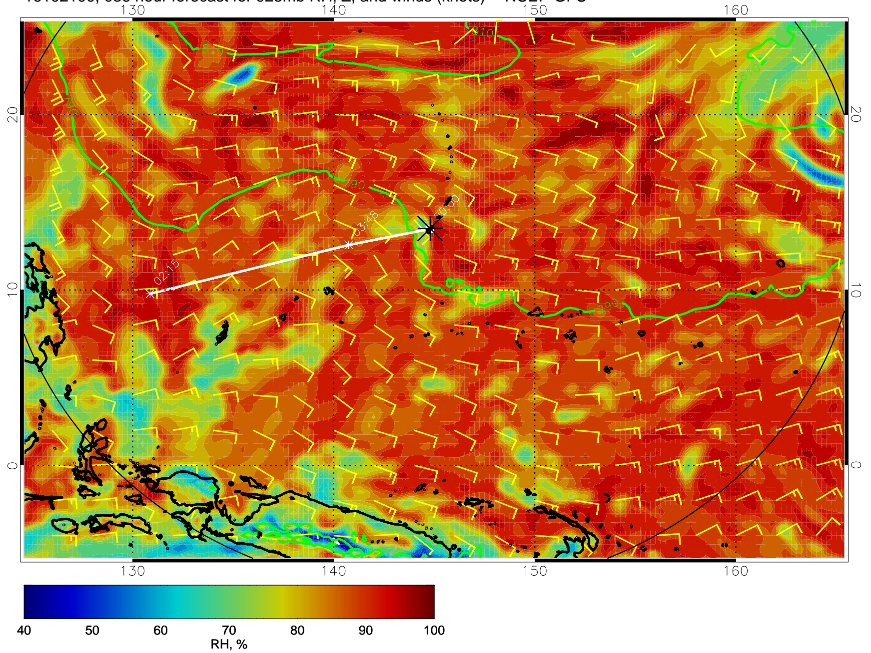
16102100, 036 hour forecast for 925mb RH, Z, and winds (knots) -- NCEP GFS
