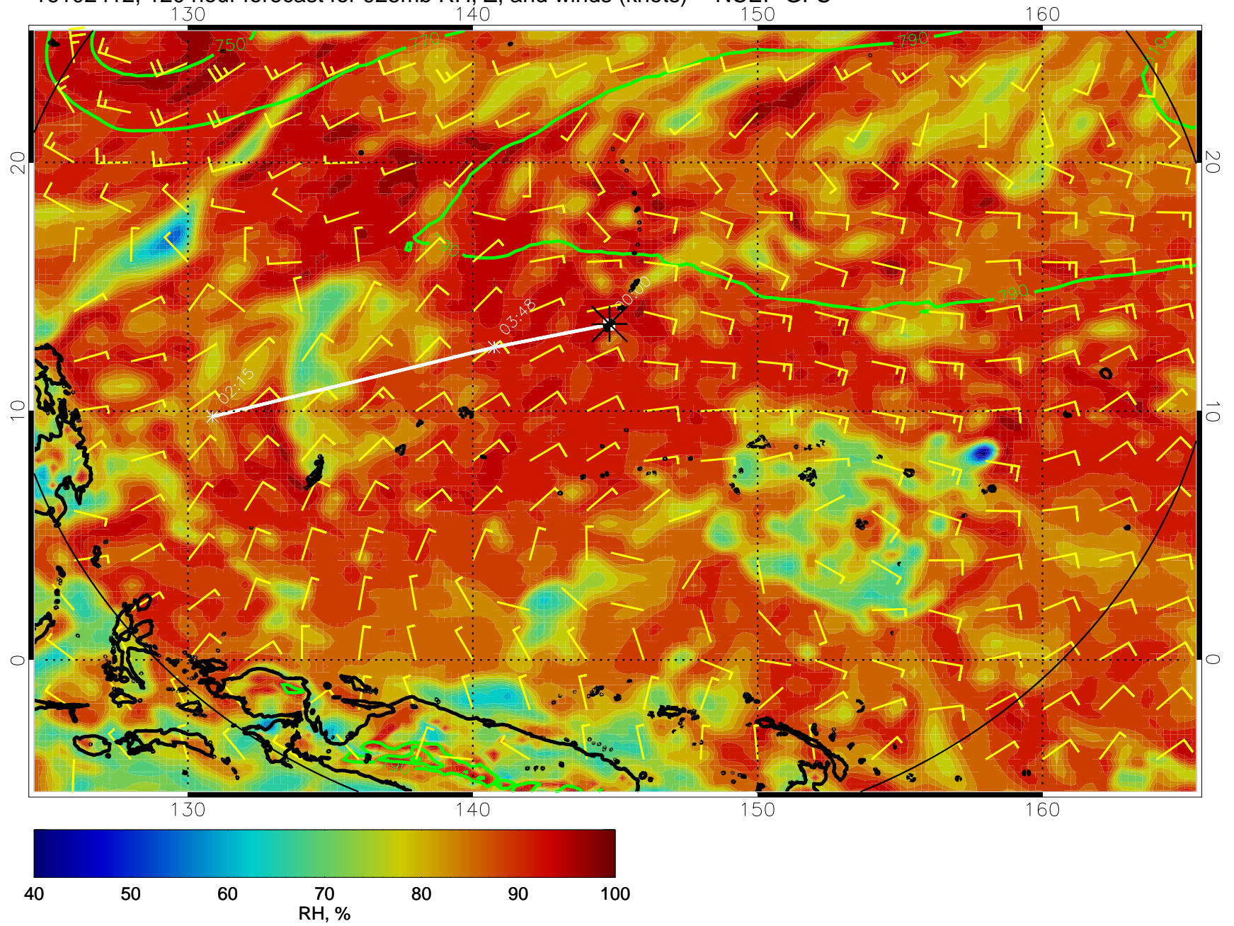
16102412, 120 hour forecast for 925mb RH, Z, and winds (knots) -- NCEP GFS
