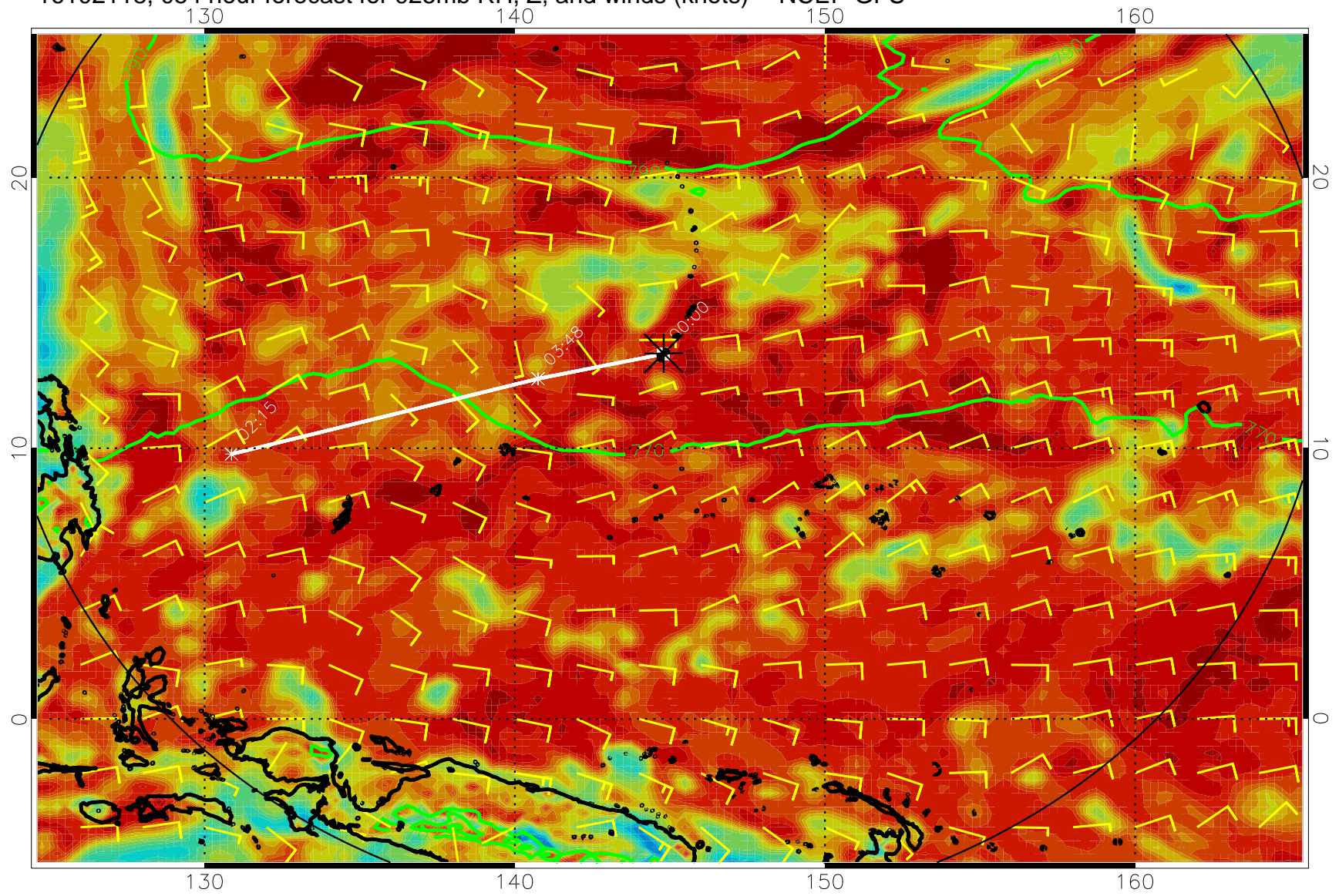
16102118, 054 hour forecast for 925mb RH, Z, and winds (knots) -- NCEP GFS
