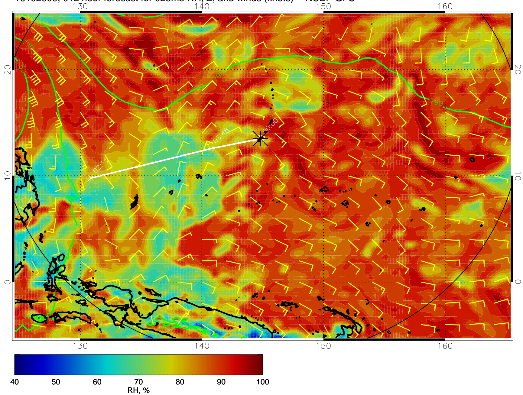
16102000, 012 hour forecast for 925mb RH, Z, and winds (knots) -- NCEP GFS
