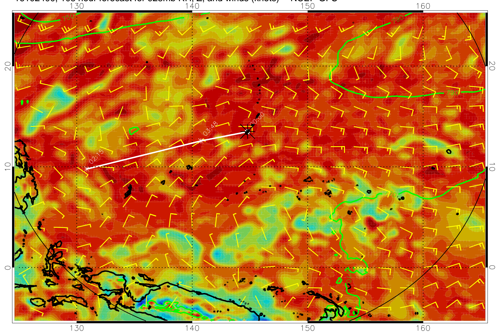
16102400, 108 hour forecast for 925mb RH, Z, and winds (knots) -- NCEP GFS
