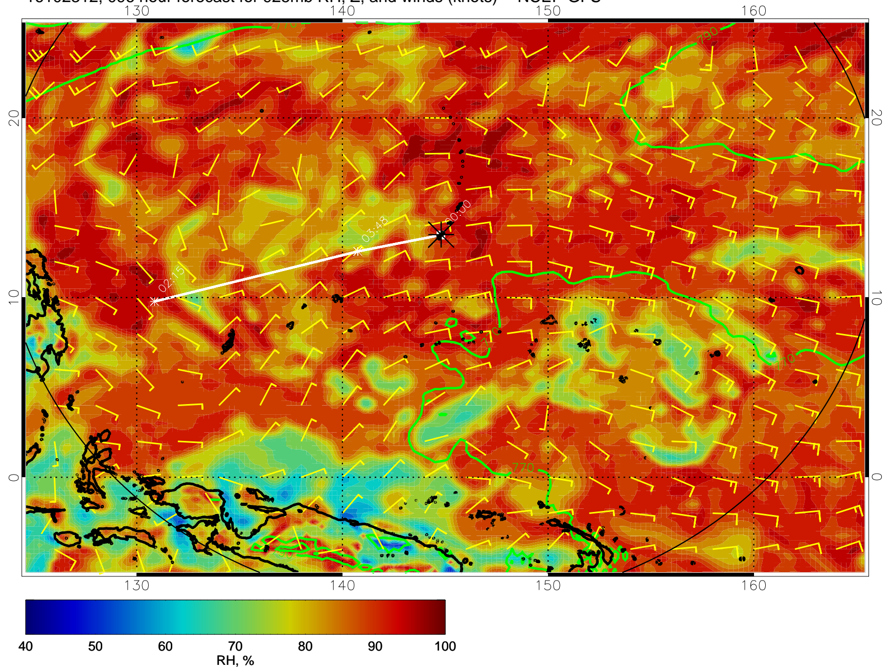
16102312, 096 hour forecast for 925mb RH, Z, and winds (knots) -- NCEP GFS
