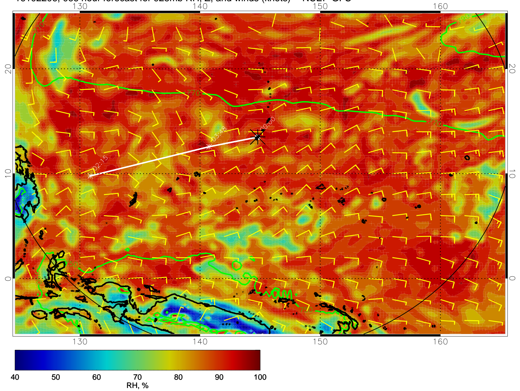
16102206, 066 hour forecast for 925mb RH, Z, and winds (knots) -- NCEP GFS
