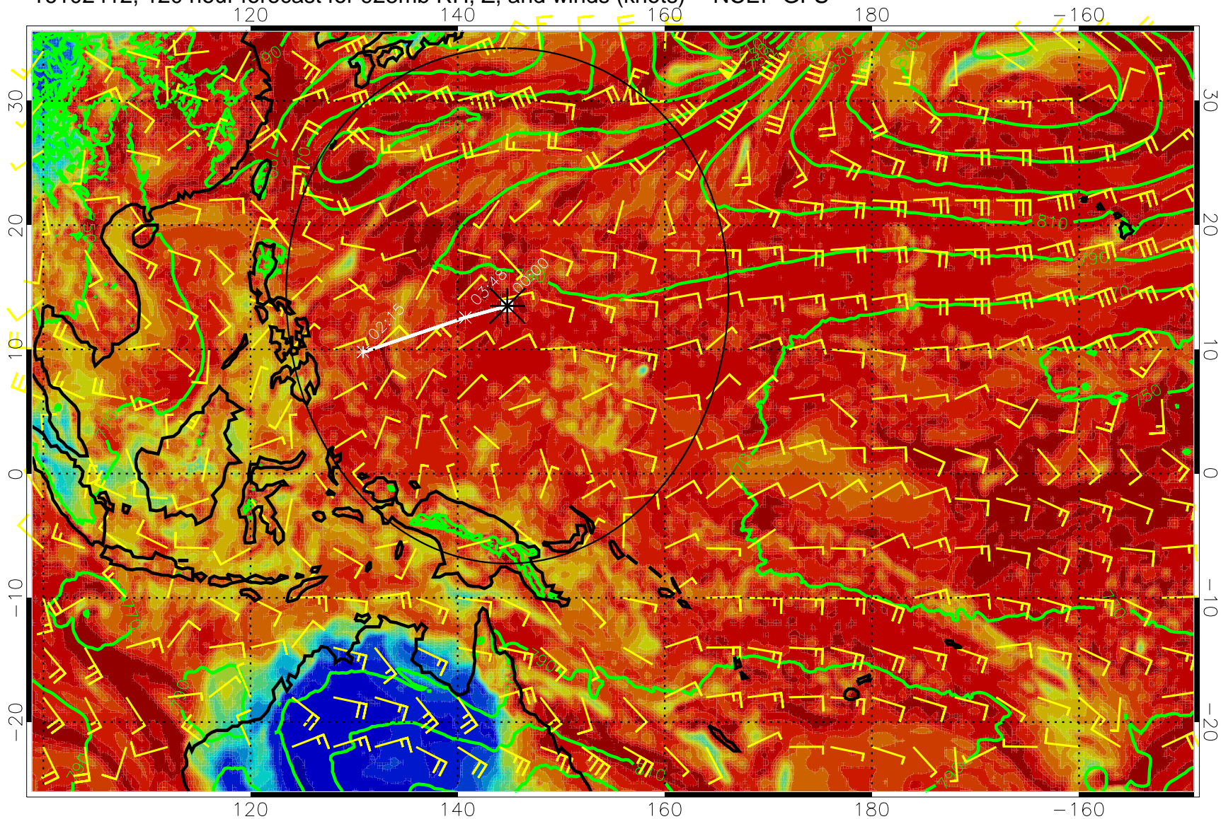
16102412, 120 hour forecast for 925mb RH, Z, and winds (knots) -- NCEP GFS
