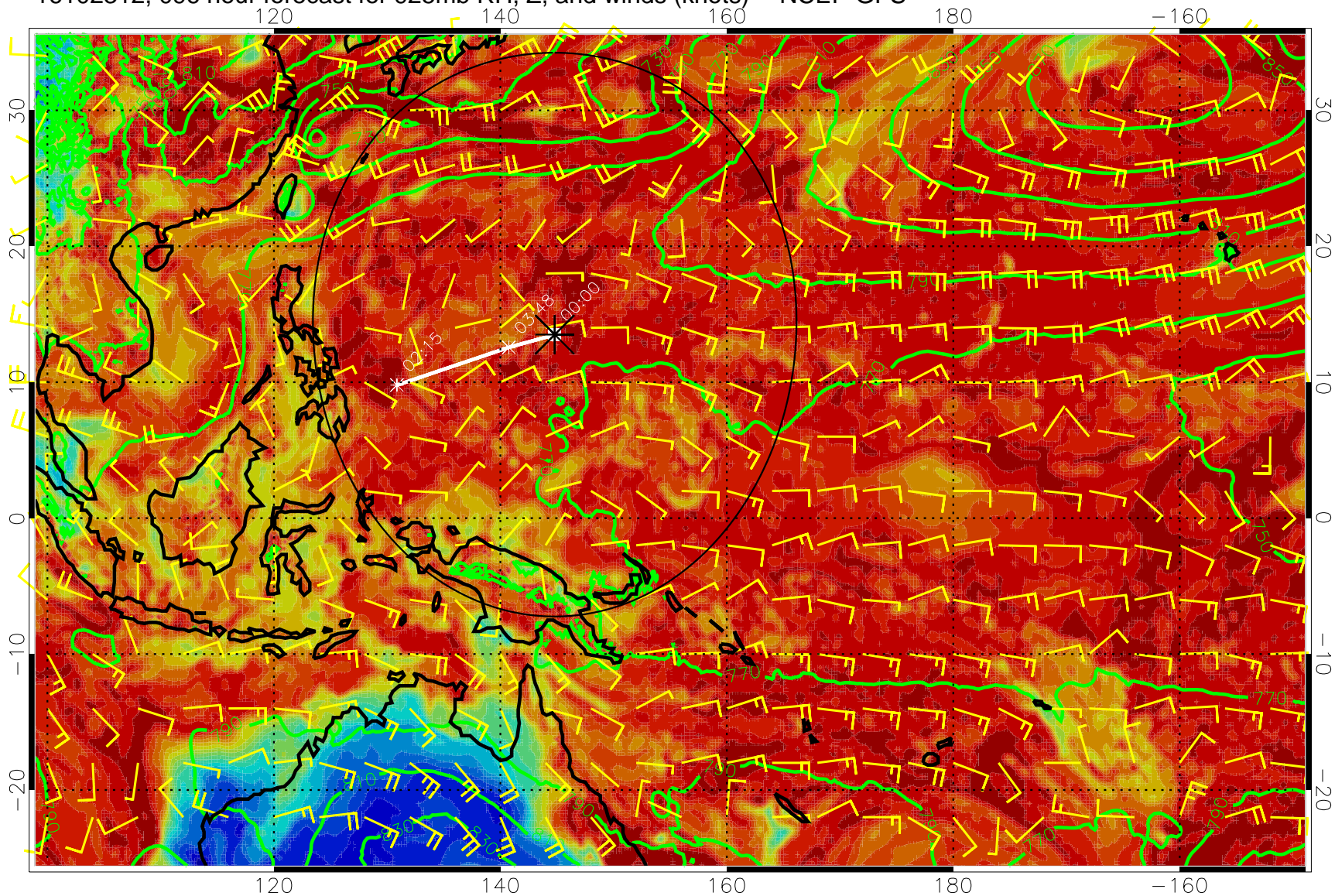
16102312, 096 hour forecast for 925mb RH, Z, and winds (knots) -- NCEP GFS
