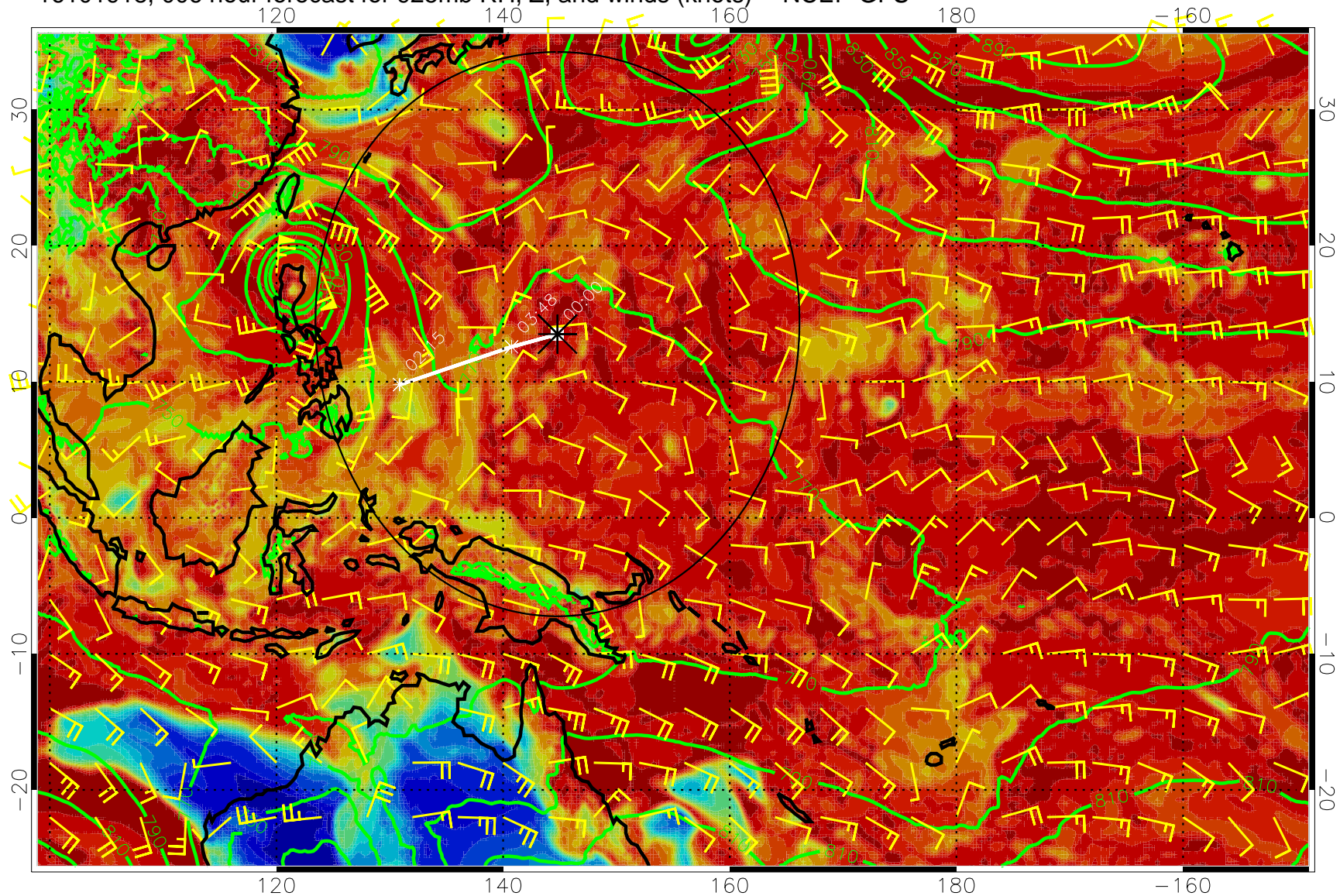
16101918, 006 hour forecast for 925mb RH, Z, and winds (knots) -- NCEP GFS
