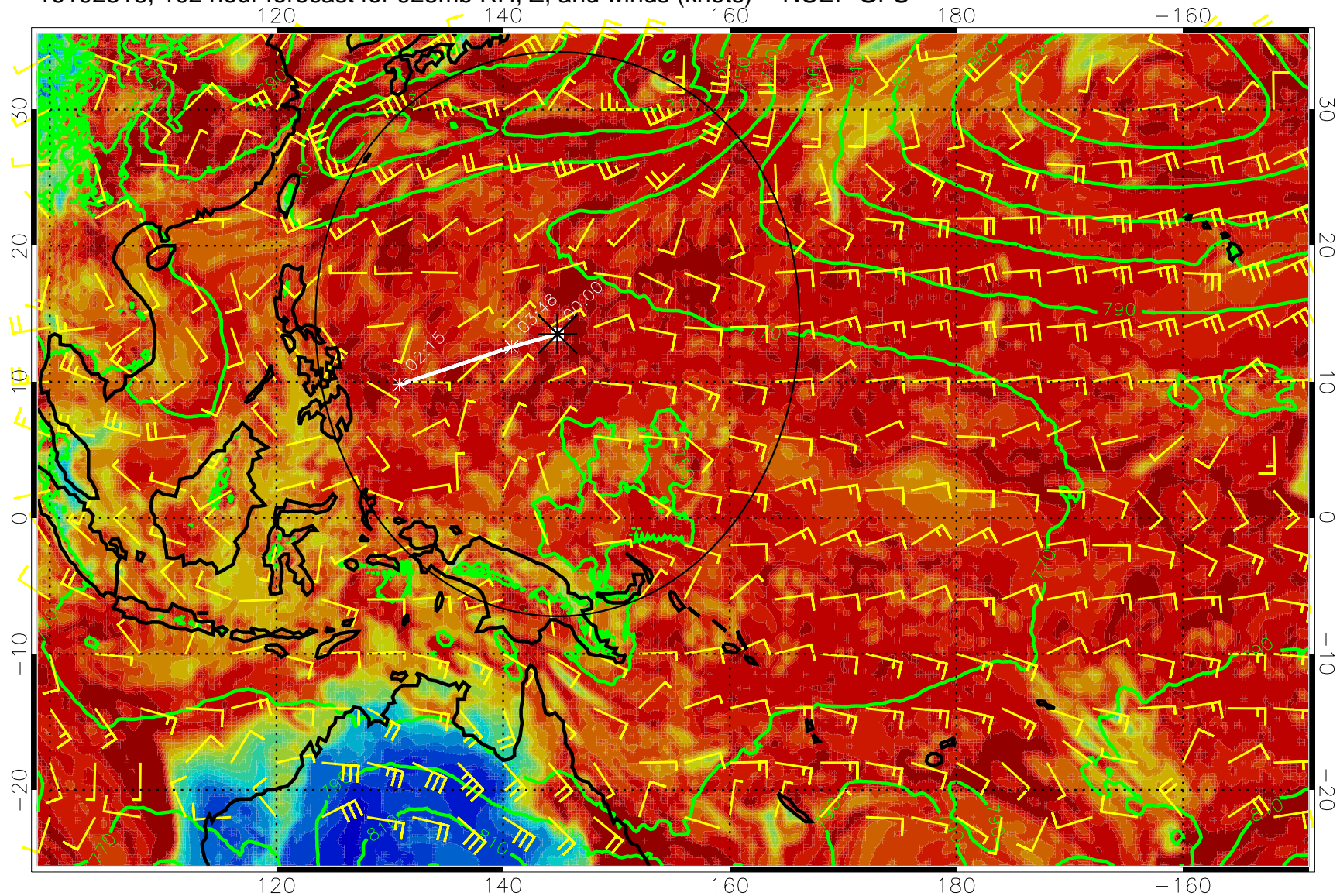
16102318, 102 hour forecast for 925mb RH, Z, and winds (knots) -- NCEP GFS
