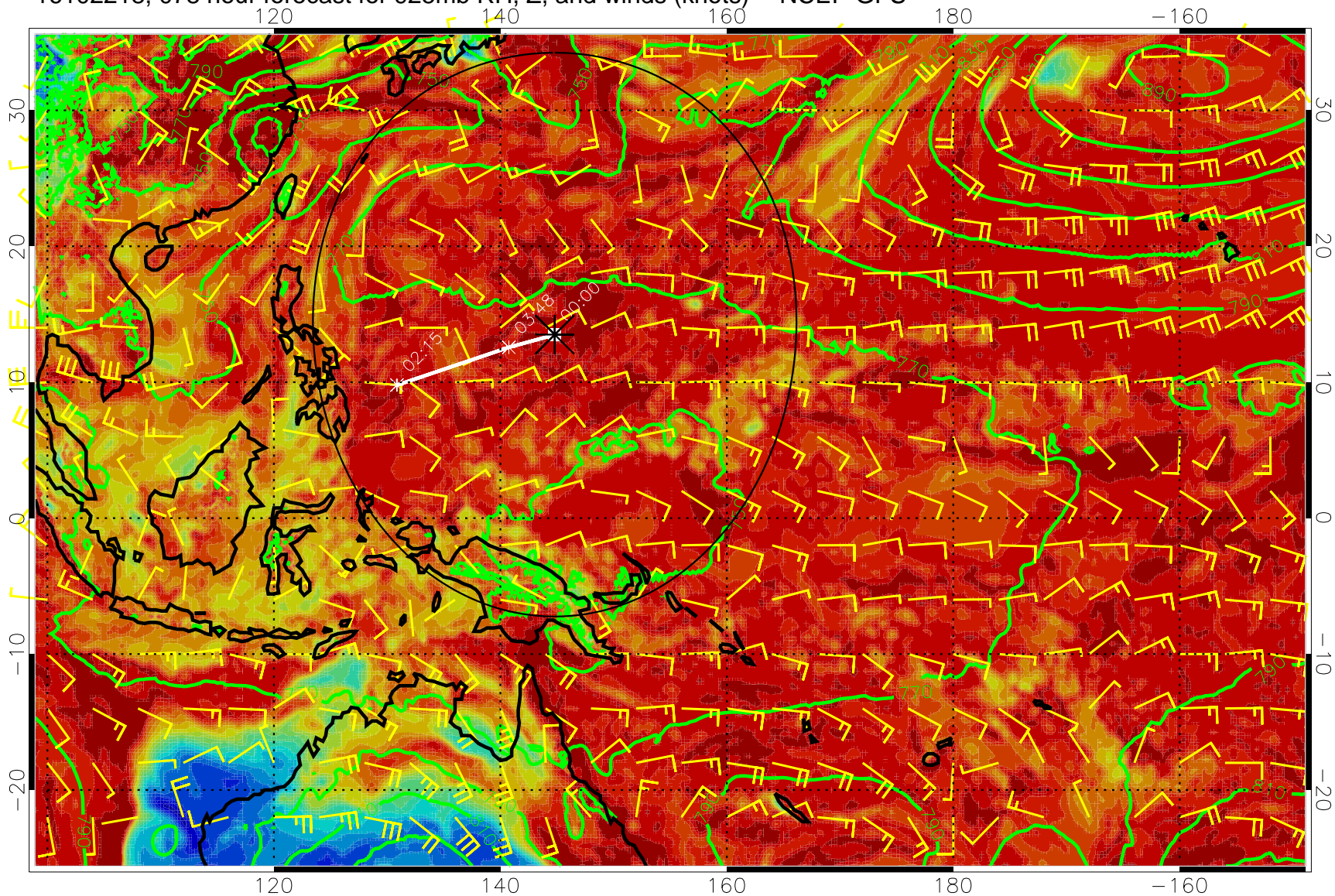
16102218, 078 hour forecast for 925mb RH, Z, and winds (knots) -- NCEP GFS
