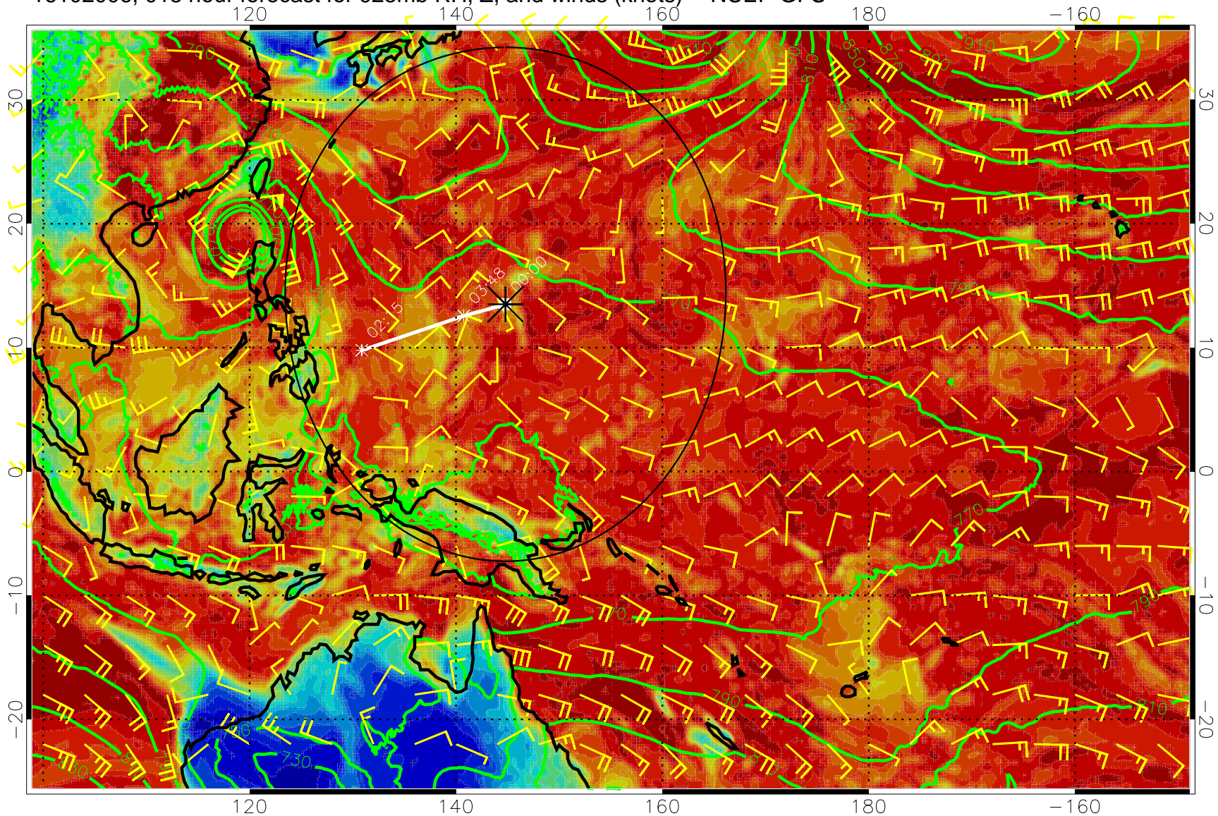
16102006, 018 hour forecast for 925mb RH, Z, and winds (knots) -- NCEP GFS
