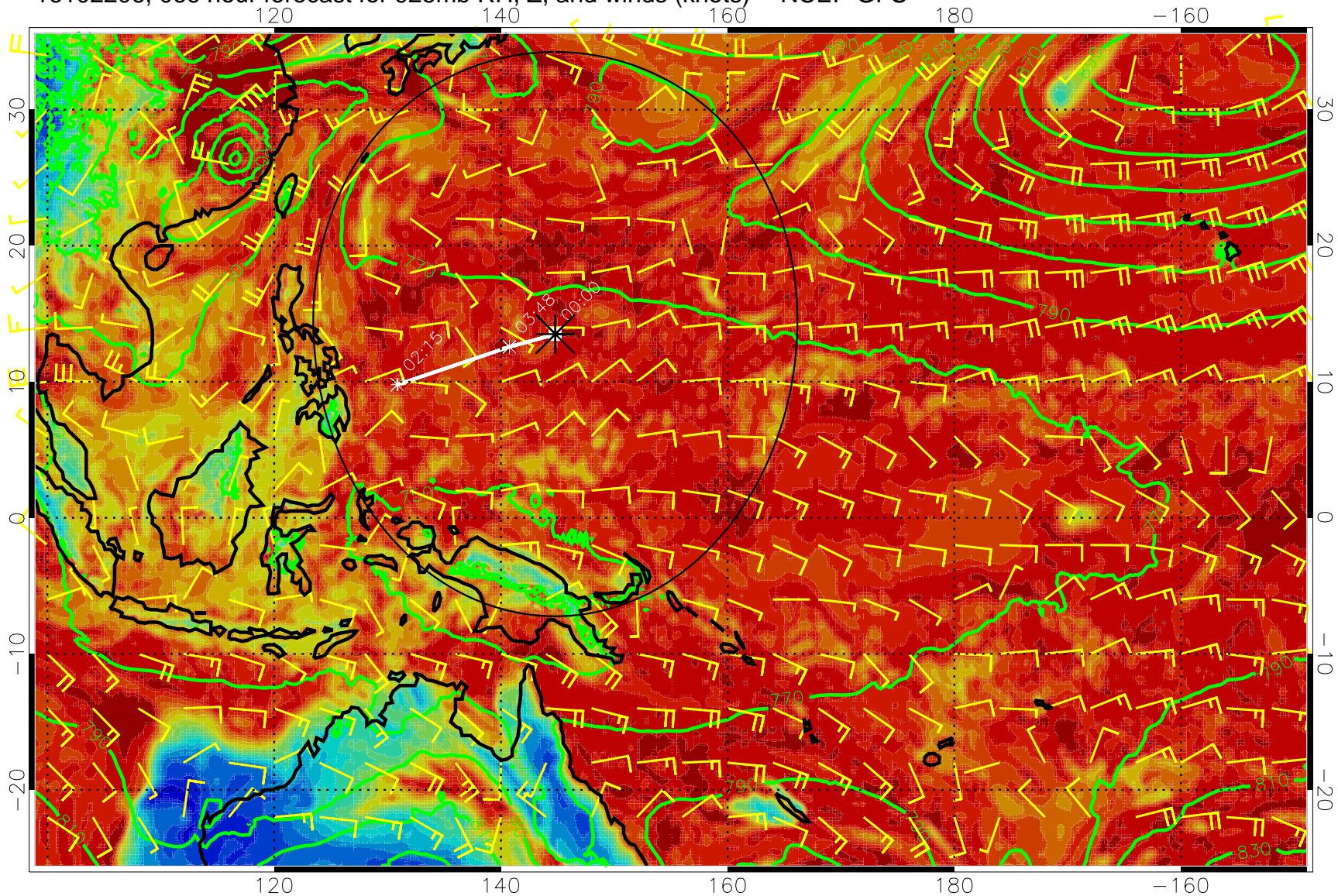
16102206, 066 hour forecast for 925mb RH, Z, and winds (knots) -- NCEP GFS
