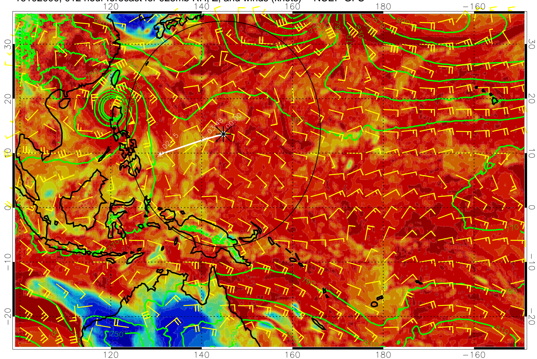
16102000, 012 hour forecast for 925mb RH, Z, and winds (knots) -- NCEP GFS
