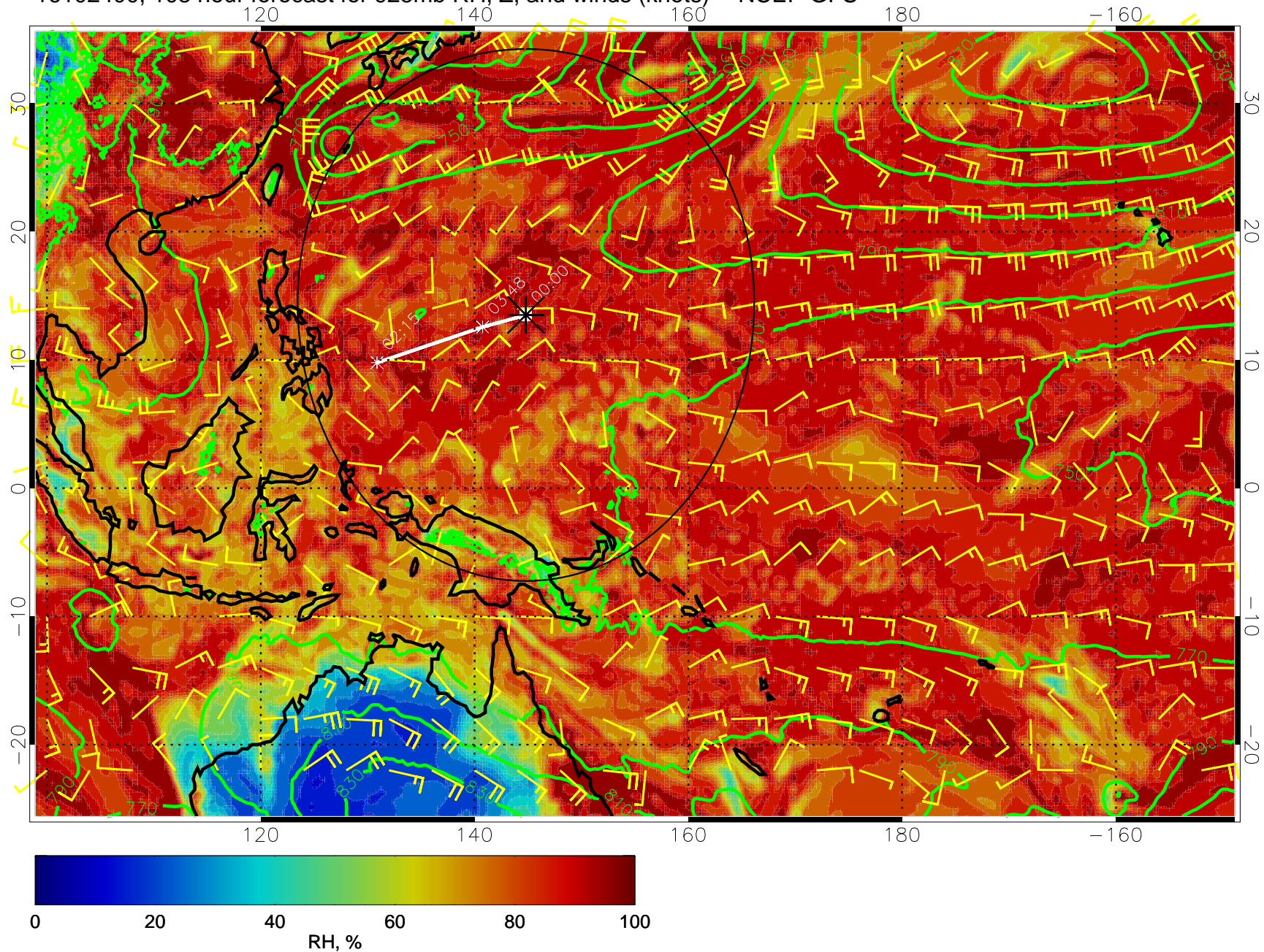
16102400, 108 hour forecast for 925mb RH, Z, and winds (knots) -- NCEP GFS
