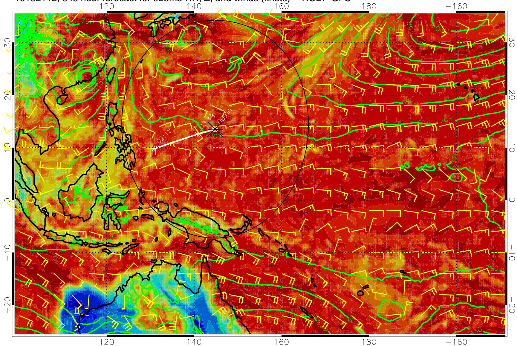
16102112, 048 hour forecast for 925mb RH, Z, and winds (knots) -- NCEP GFS
