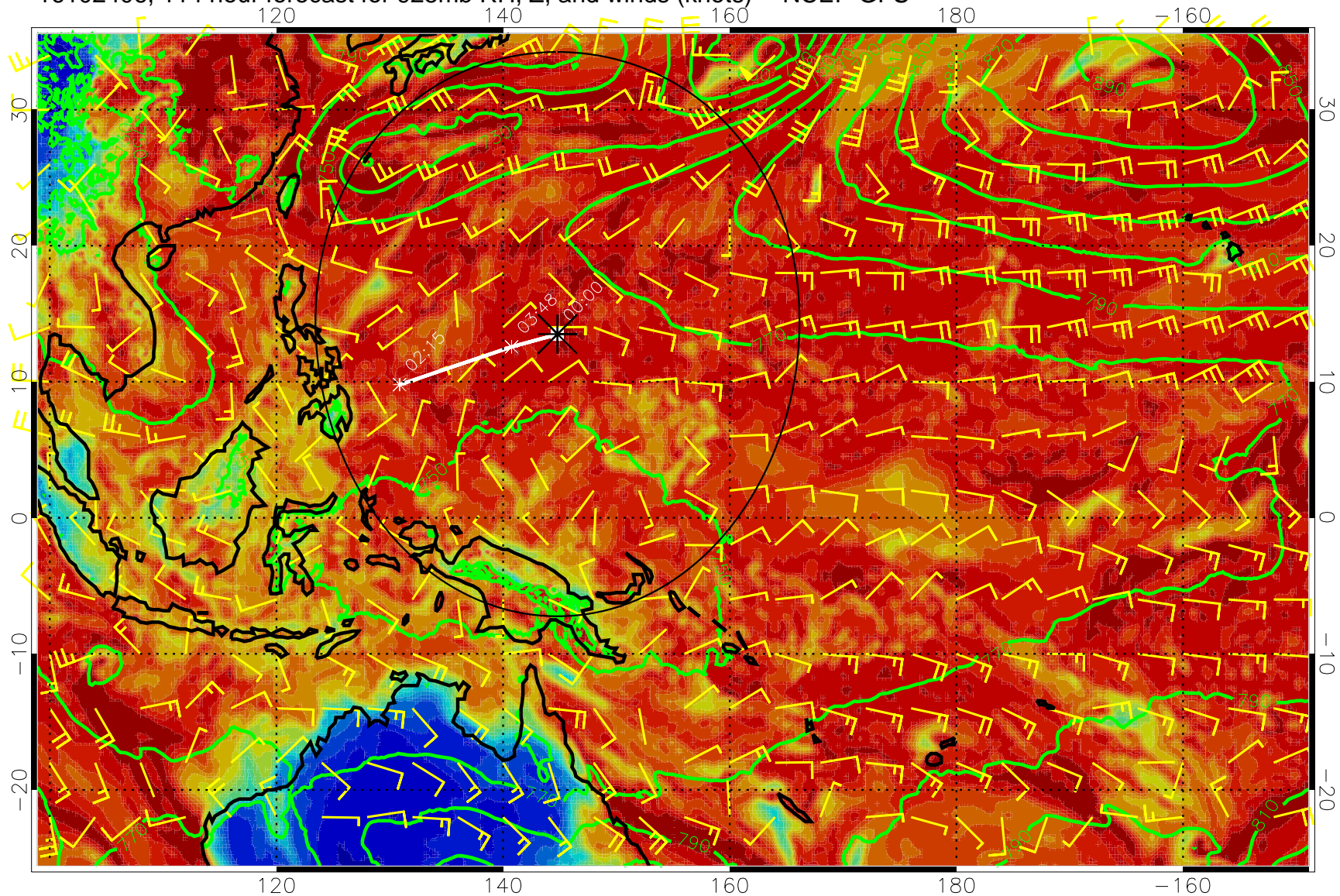
16102406, 114 hour forecast for 925mb RH, Z, and winds (knots) -- NCEP GFS
