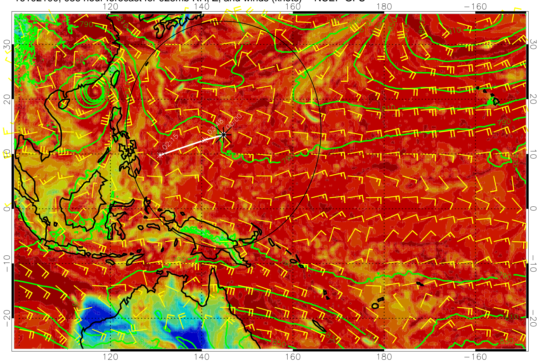
16102100, 036 hour forecast for 925mb RH, Z, and winds (knots) -- NCEP GFS
