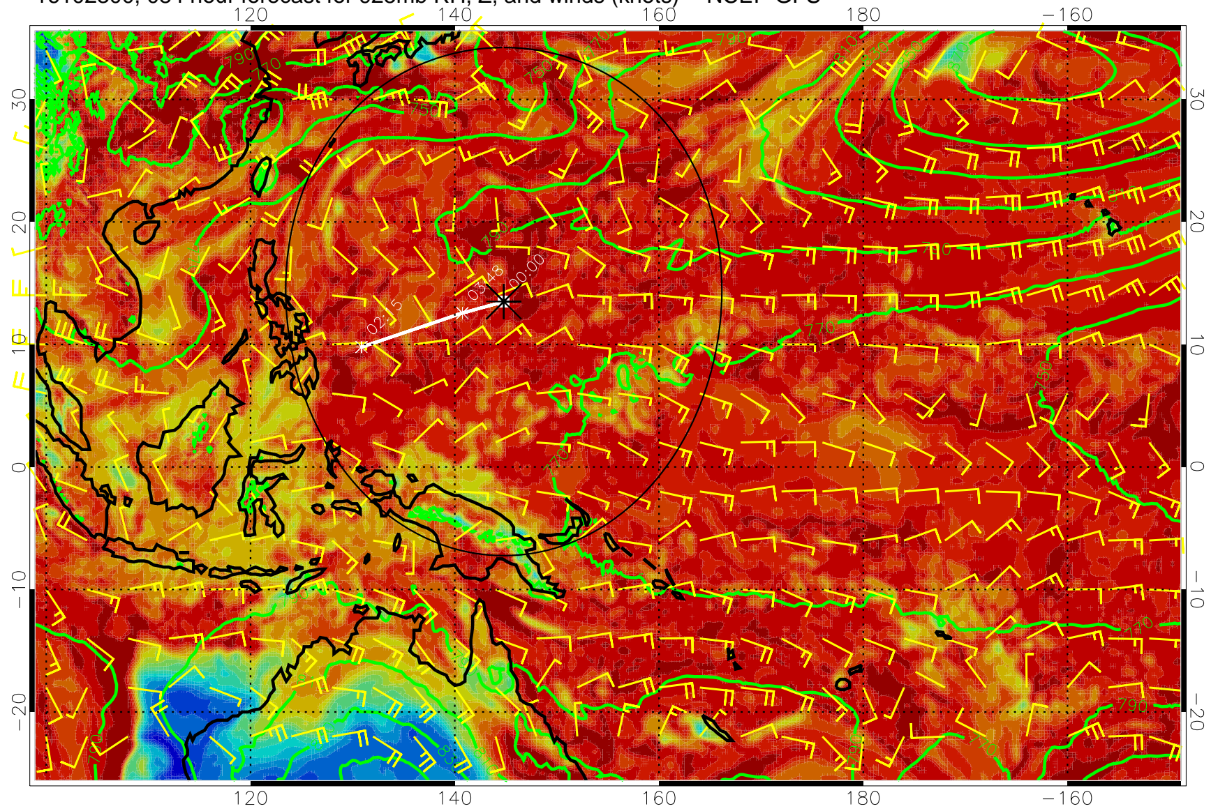
16102300, 084 hour forecast for 925mb RH, Z, and winds (knots) -- NCEP GFS
