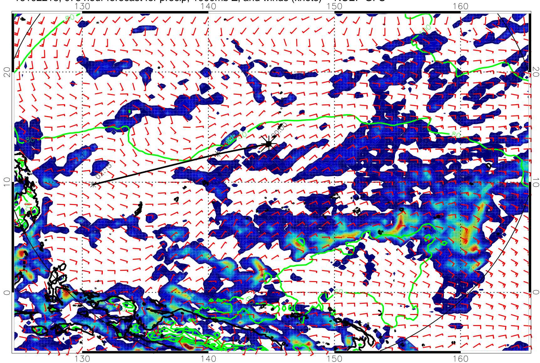
16102218, 078 hour forecast for precip, 1000mb Z, and winds (knots) -- NCEP GFS
