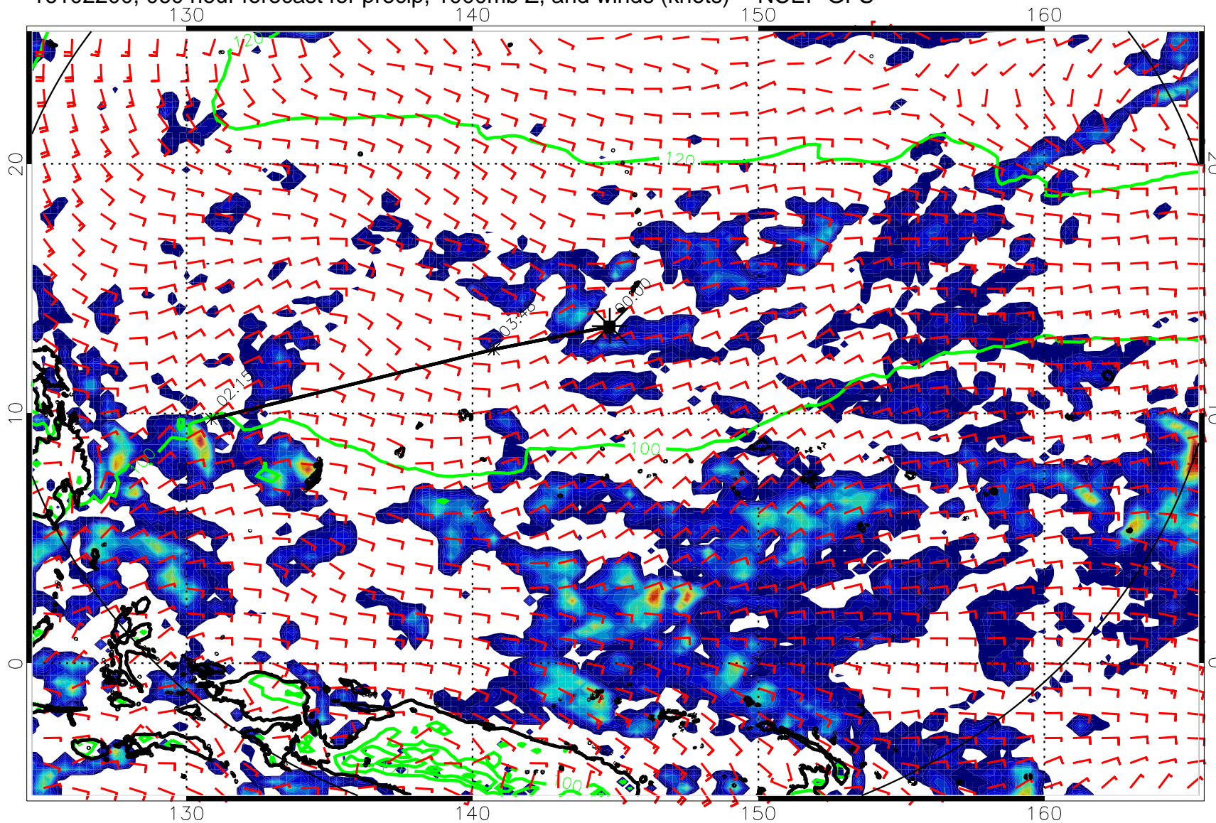
16102200, 060 hour forecast for precip, 1000mb Z, and winds (knots) -- NCEP GFS
