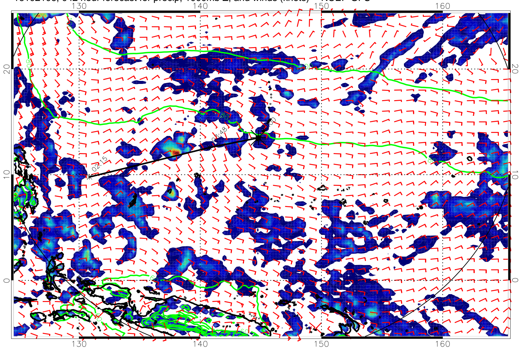
16102106, 042 hour forecast for precip, 1000mb Z, and winds (knots) -- NCEP GFS
