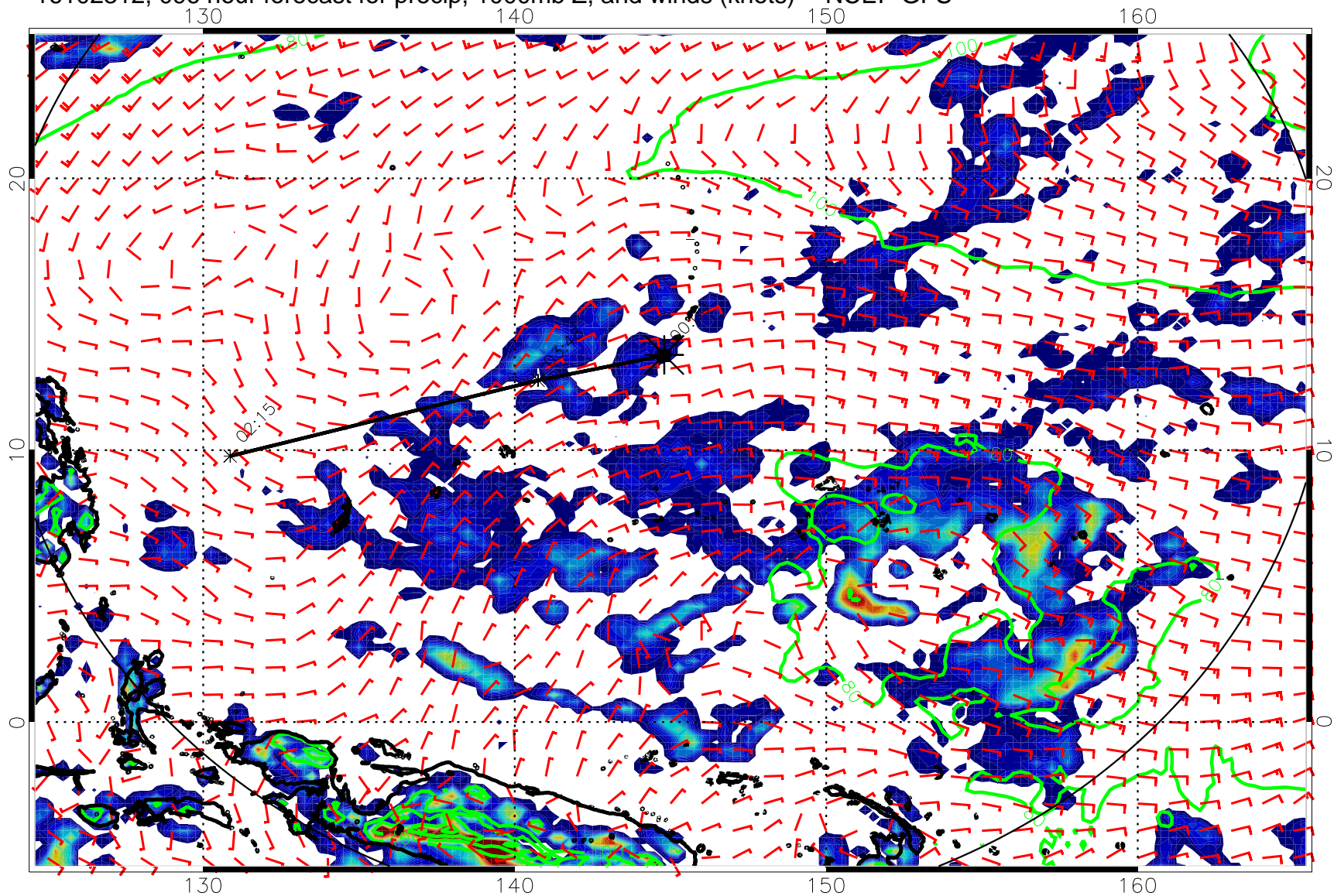
16102312, 096 hour forecast for precip, 1000mb Z, and winds (knots) -- NCEP GFS
