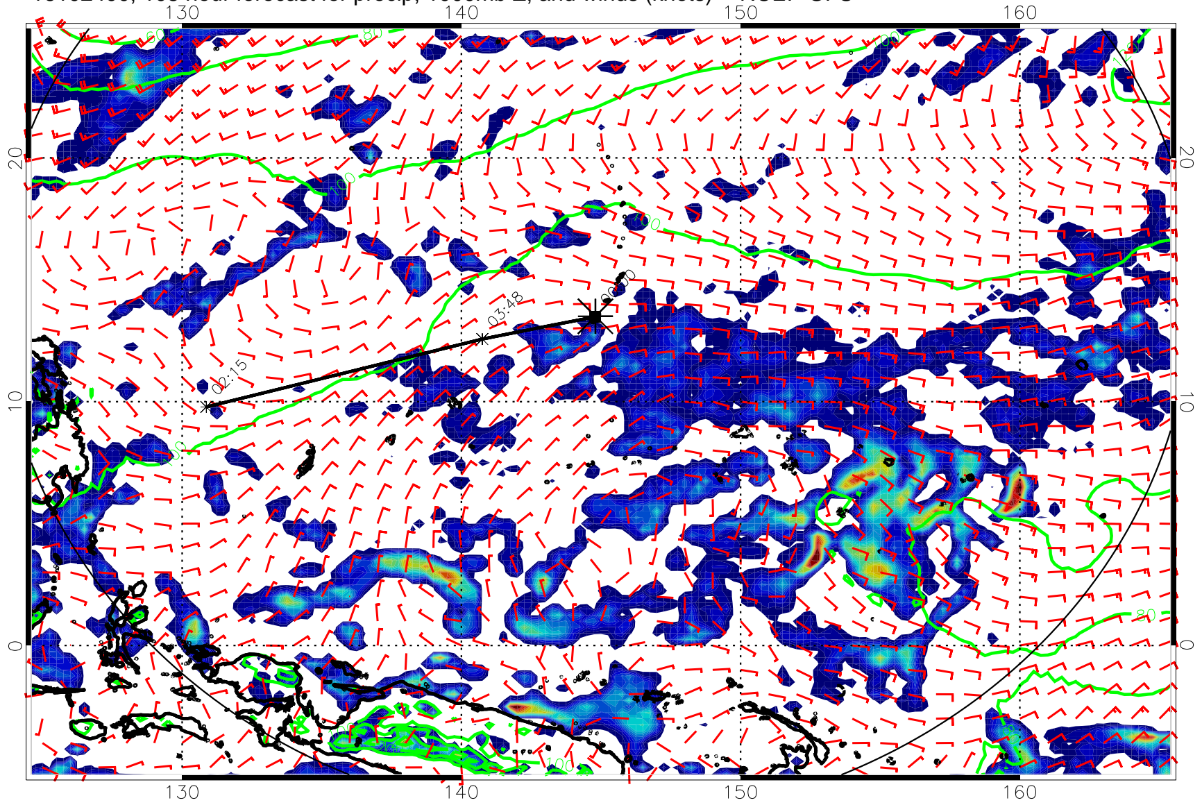
16102400, 108 hour forecast for precip, 1000mb Z, and winds (knots) -- NCEP GFS
