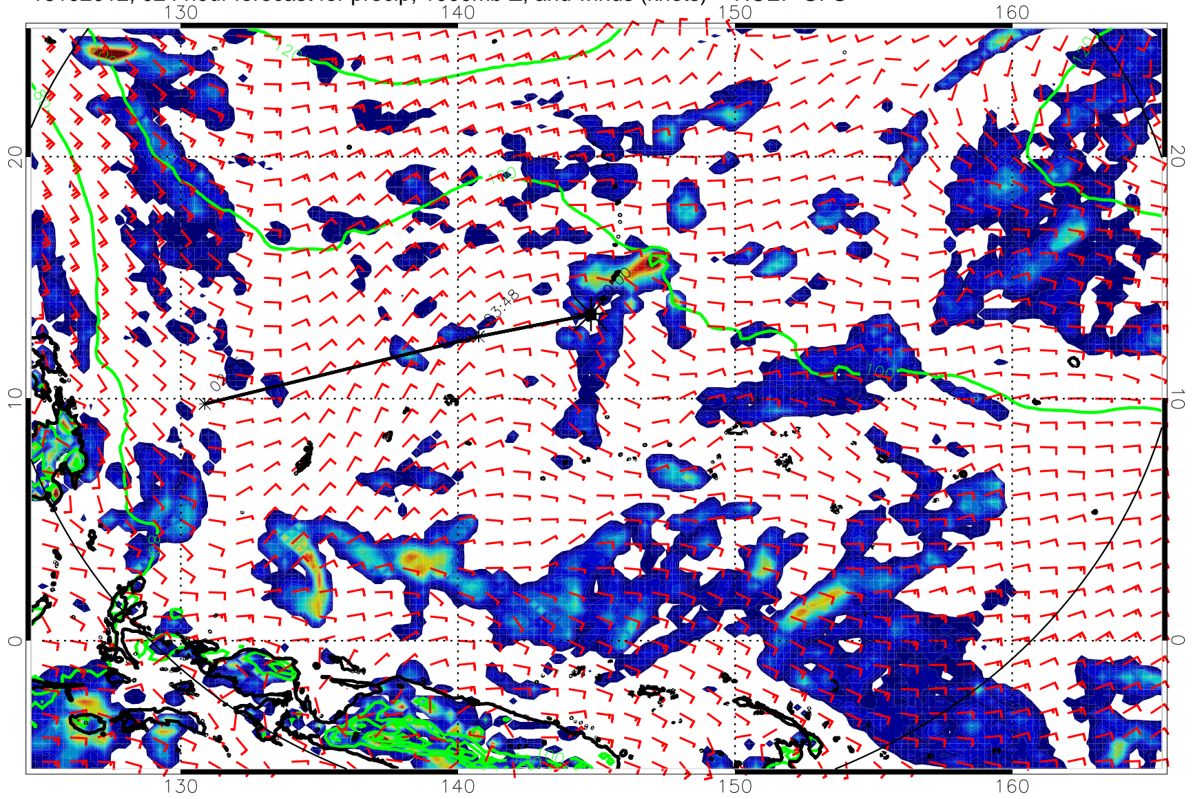
16102012, 024 hour forecast for precip, 1000mb Z, and winds (knots) -- NCEP GFS
