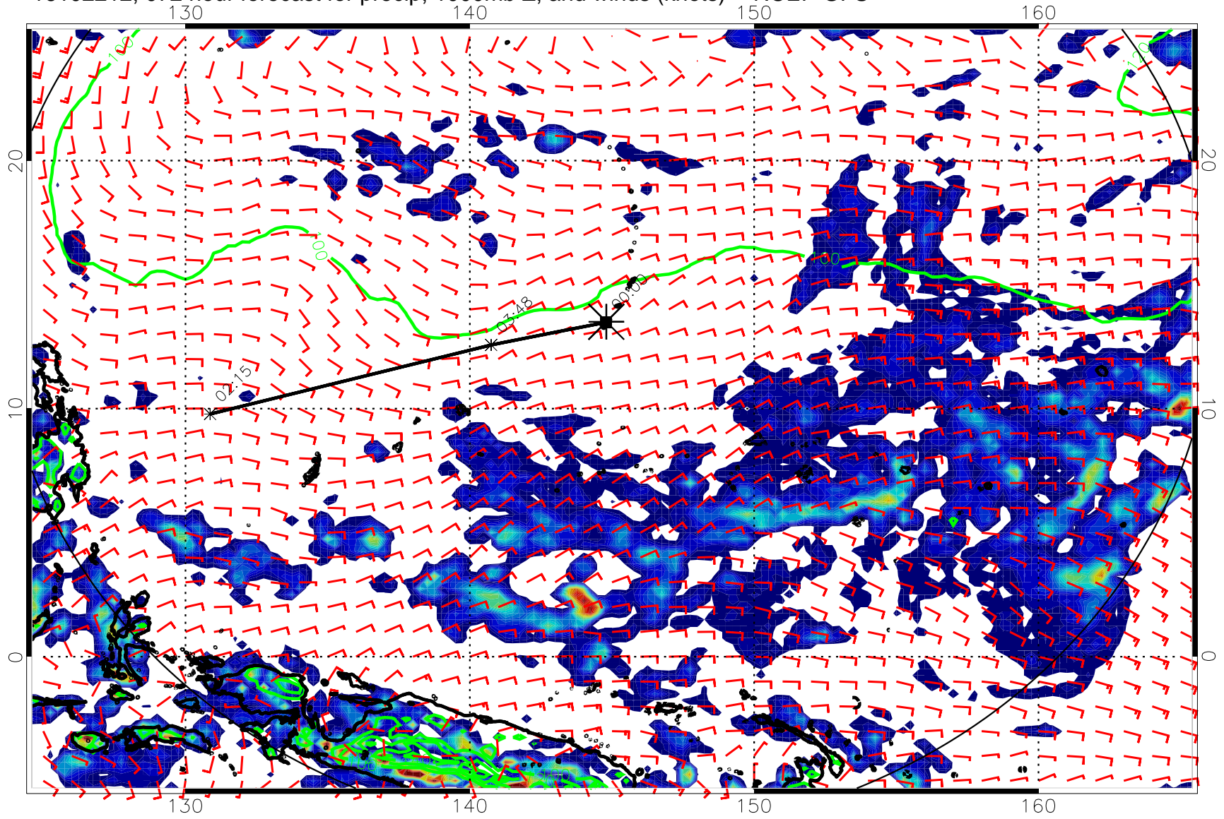
16102212, 072 hour forecast for precip, 1000mb Z, and winds (knots) -- NCEP GFS
