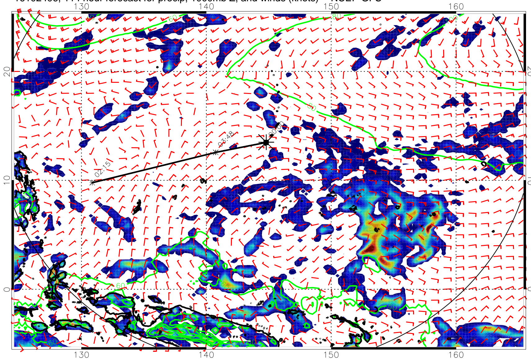
16102406, 114 hour forecast for precip, 1000mb Z, and winds (knots) -- NCEP GFS
