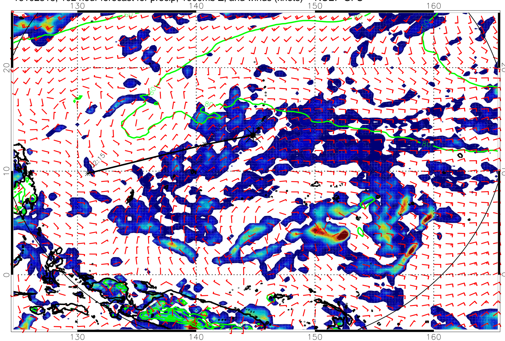
16102318, 102 hour forecast for precip, 1000mb Z, and winds (knots) -- NCEP GFS
