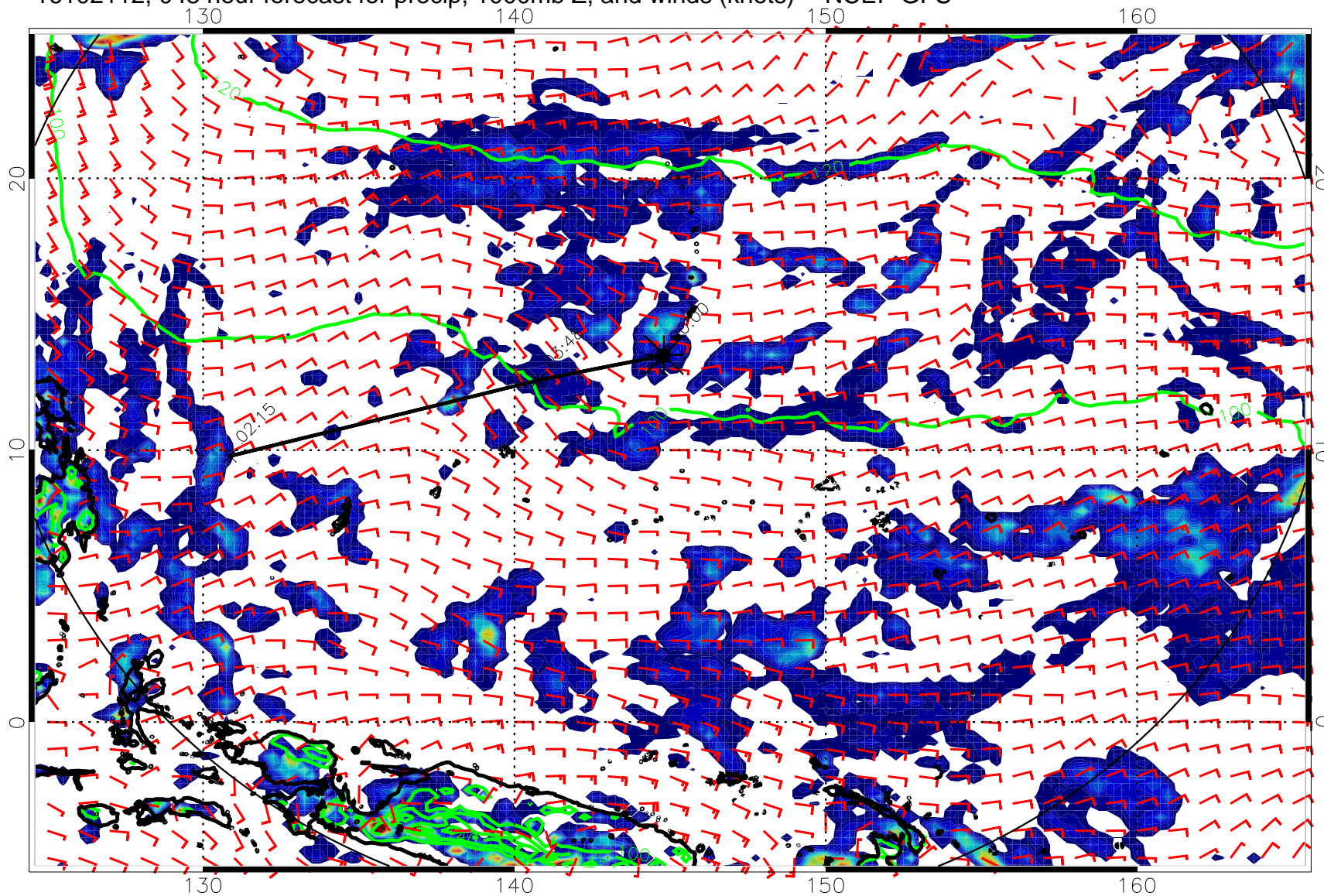
16102112, 048 hour forecast for precip, 1000mb Z, and winds (knots) -- NCEP GFS
