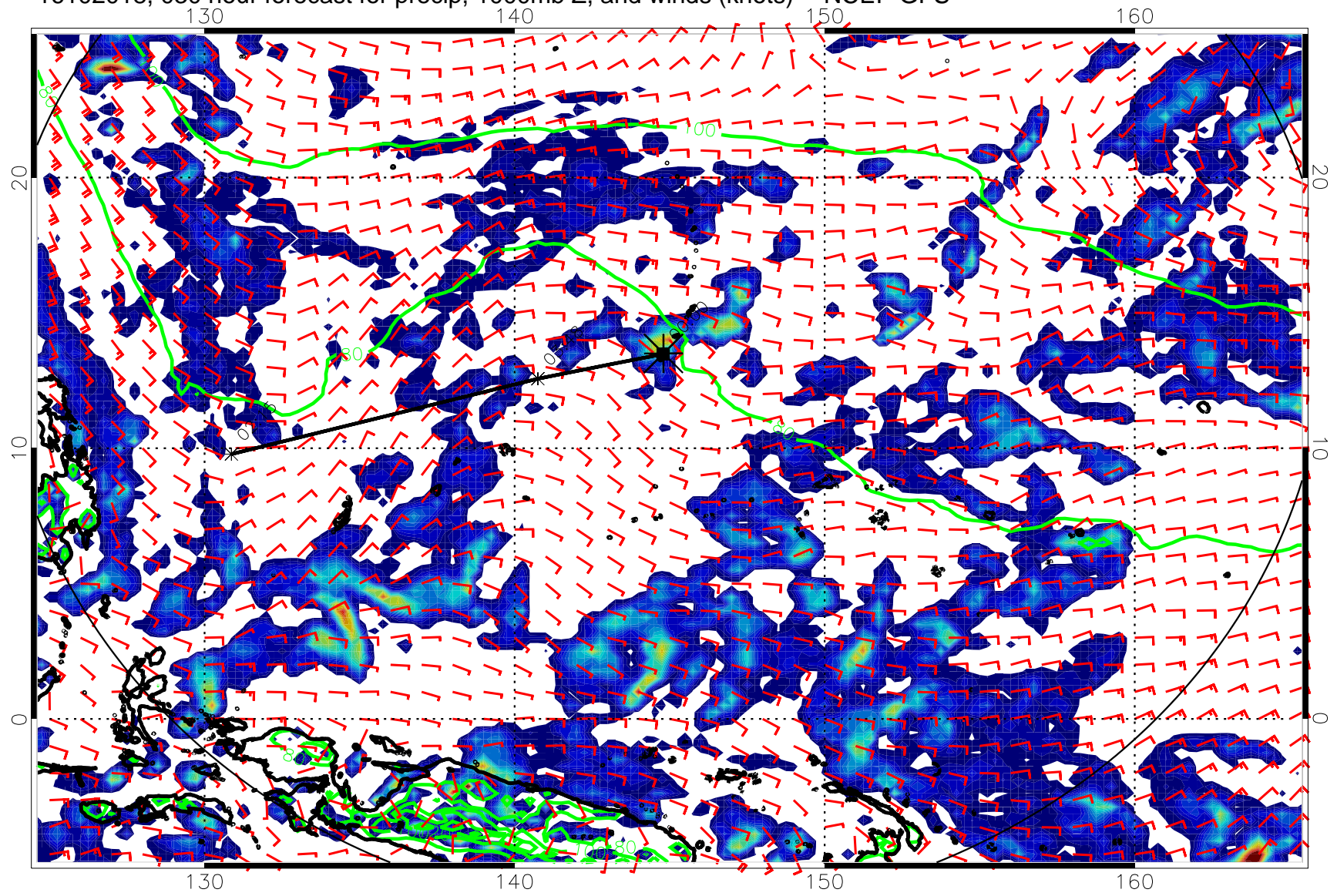
16102018, 030 hour forecast for precip, 1000mb Z, and winds (knots) -- NCEP GFS
