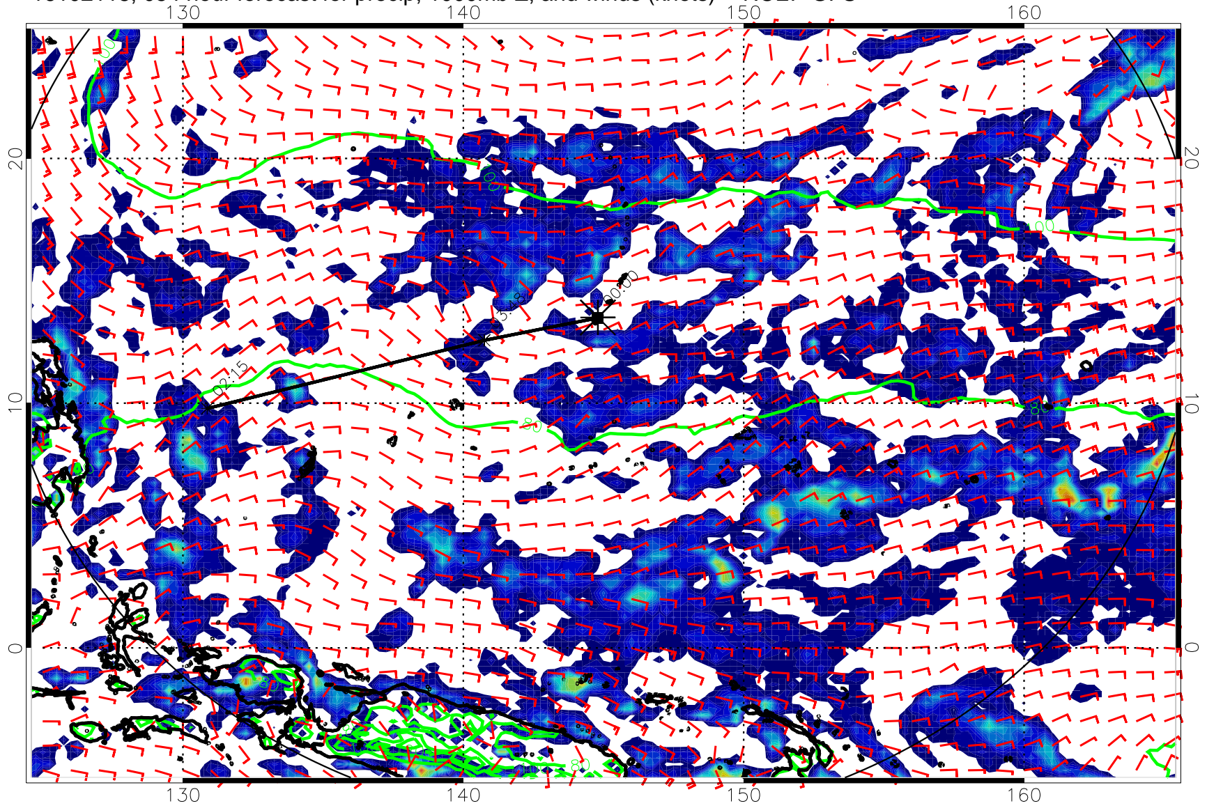
16102118, 054 hour forecast for precip, 1000mb Z, and winds (knots) -- NCEP GFS
