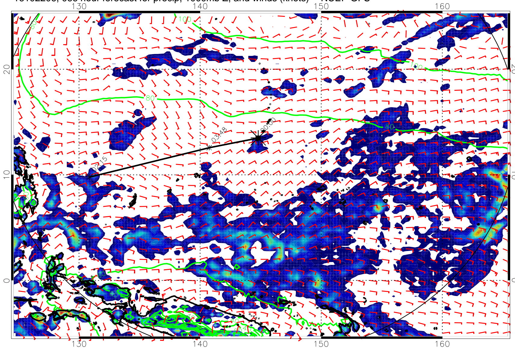
16102206, 066 hour forecast for precip, 1000mb Z, and winds (knots) -- NCEP GFS
