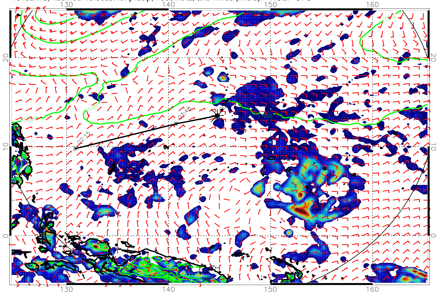
16102412, 120 hour forecast for precip, 1000mb Z, and winds (knots) -- NCEP GFS
