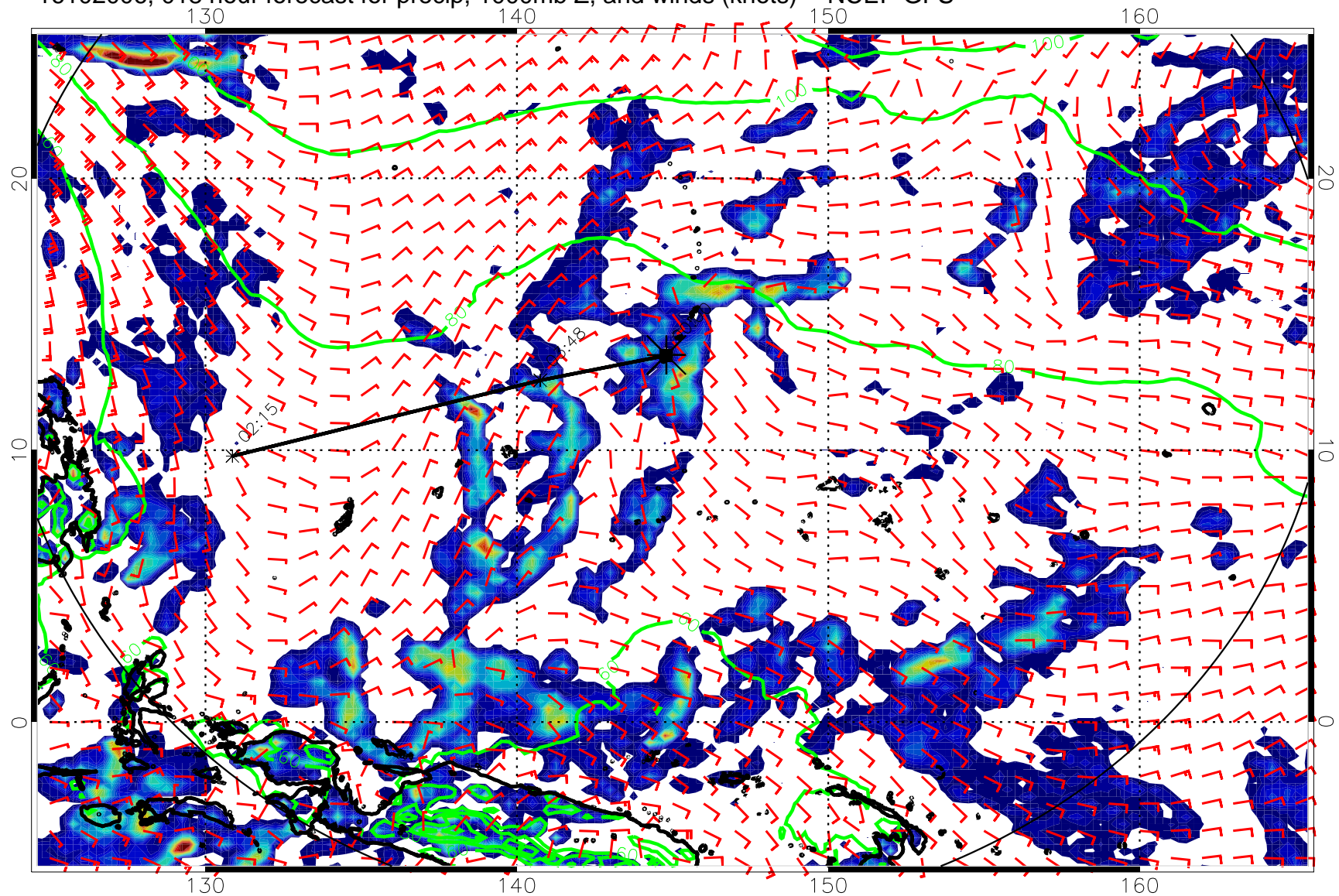
16102006, 018 hour forecast for precip, 1000mb Z, and winds (knots) -- NCEP GFS
