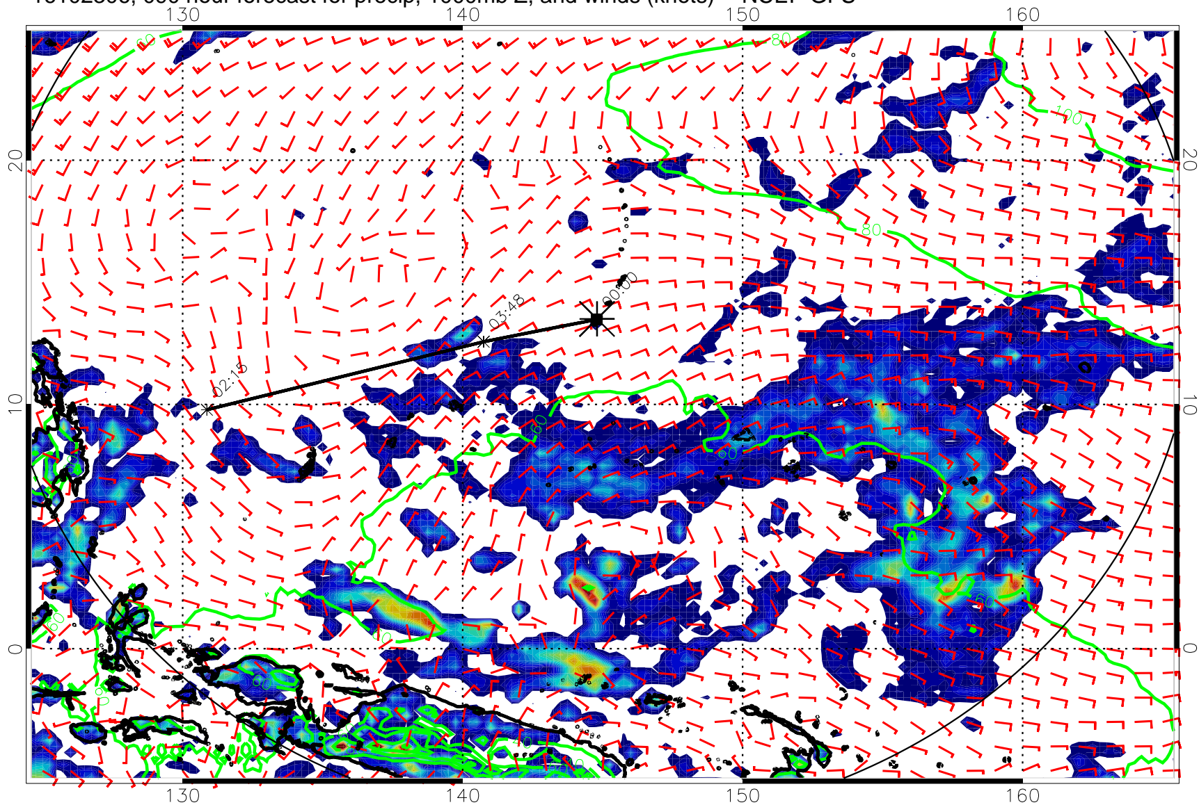
16102306, 090 hour forecast for precip, 1000mb Z, and winds (knots) -- NCEP GFS
