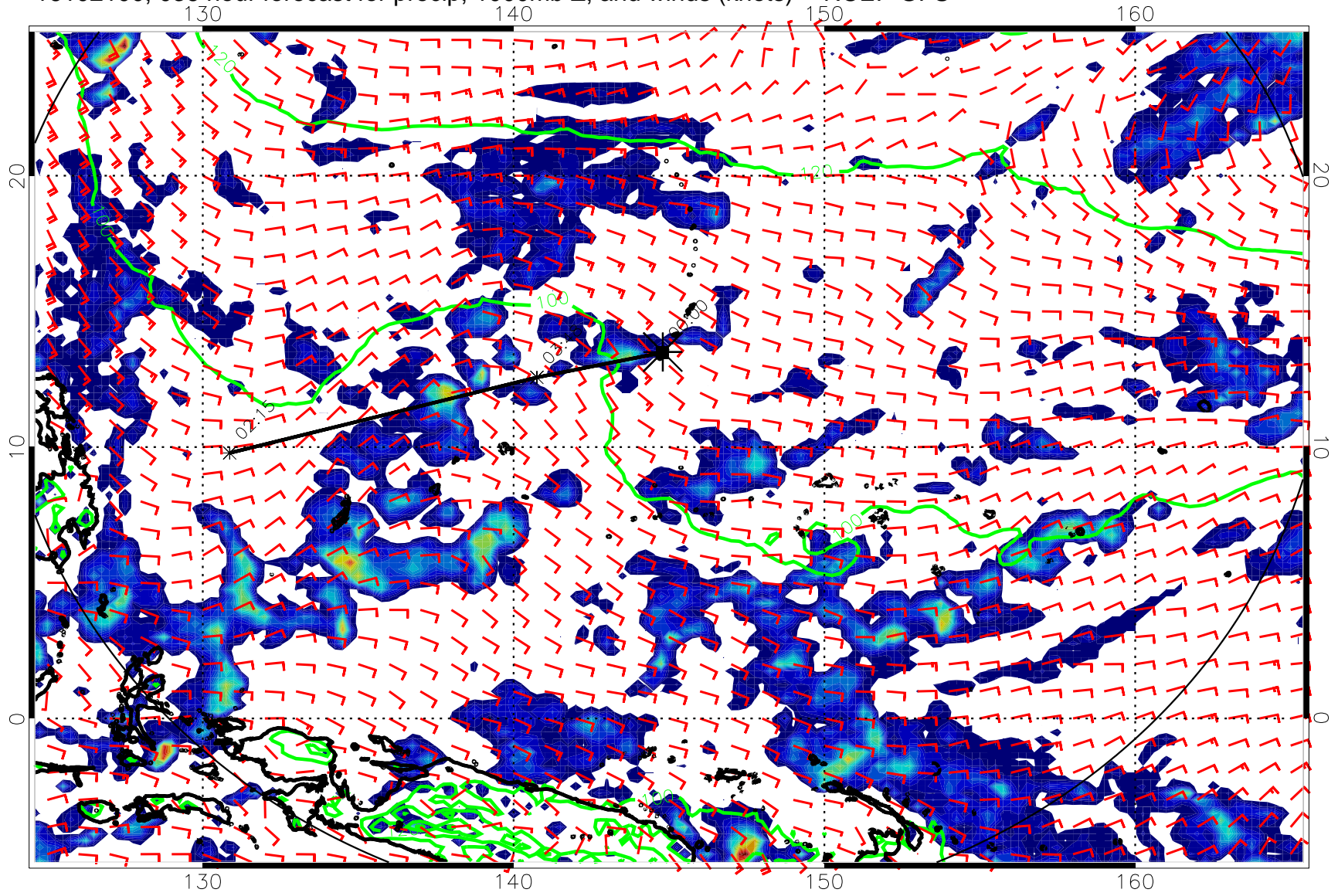
16102100, 036 hour forecast for precip, 1000mb Z, and winds (knots) -- NCEP GFS
