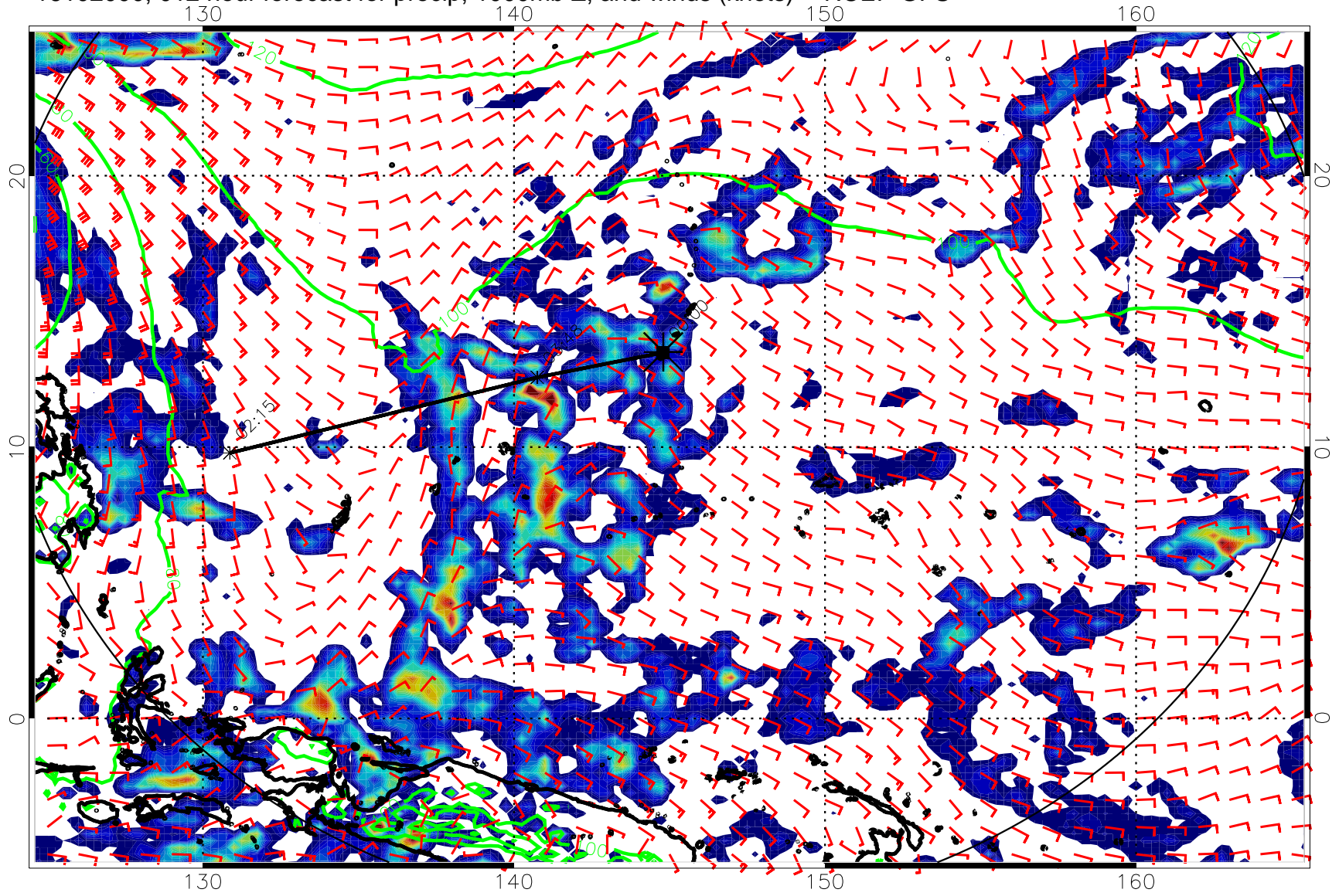
16102000, 012 hour forecast for precip, 1000mb Z, and winds (knots) -- NCEP GFS
