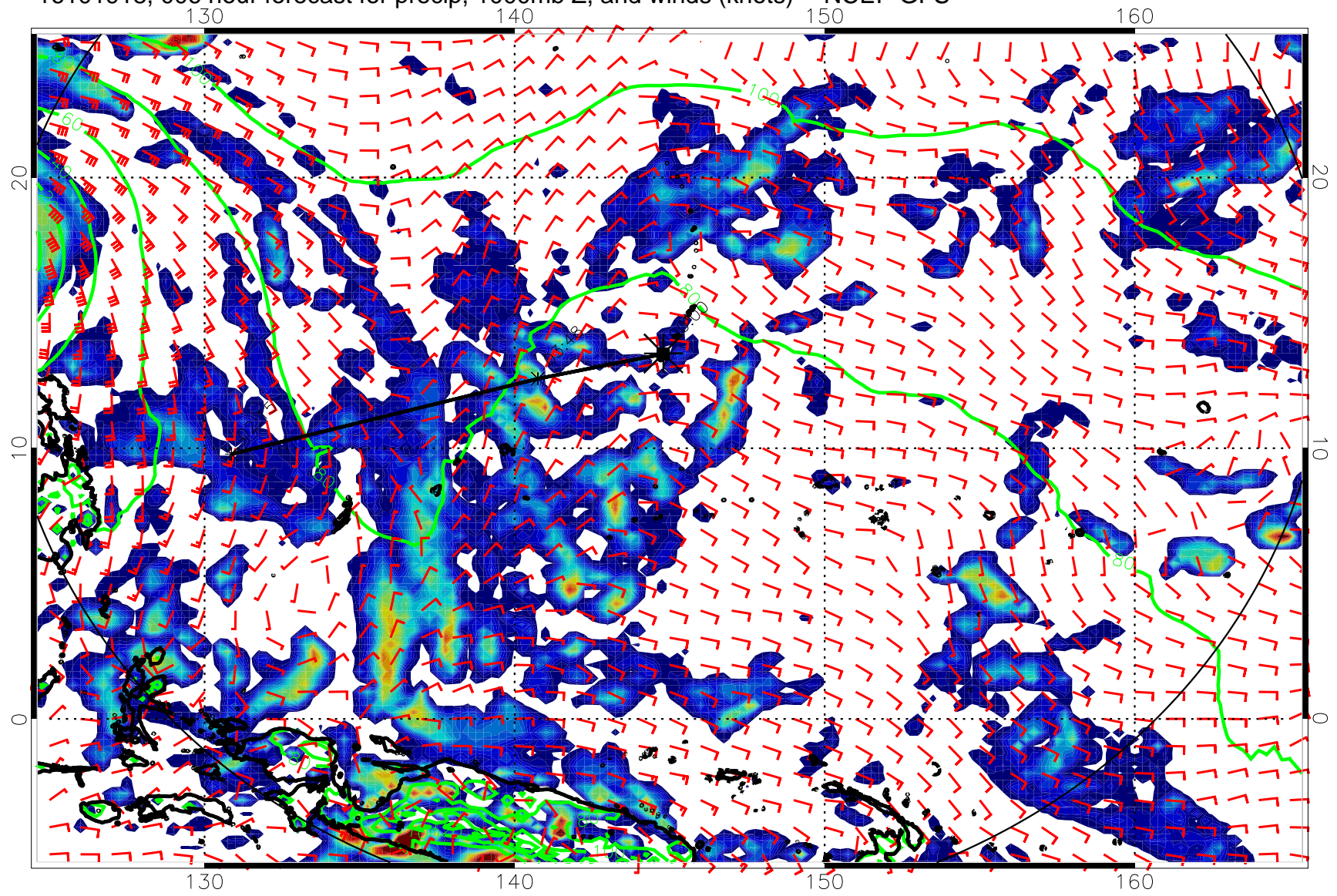
16101918, 006 hour forecast for precip, 1000mb Z, and winds (knots) -- NCEP GFS
