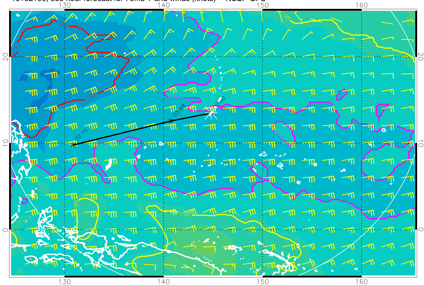
16102100, 036 hour forecast for 70mb T and winds (knots) -- NCEP GFS
