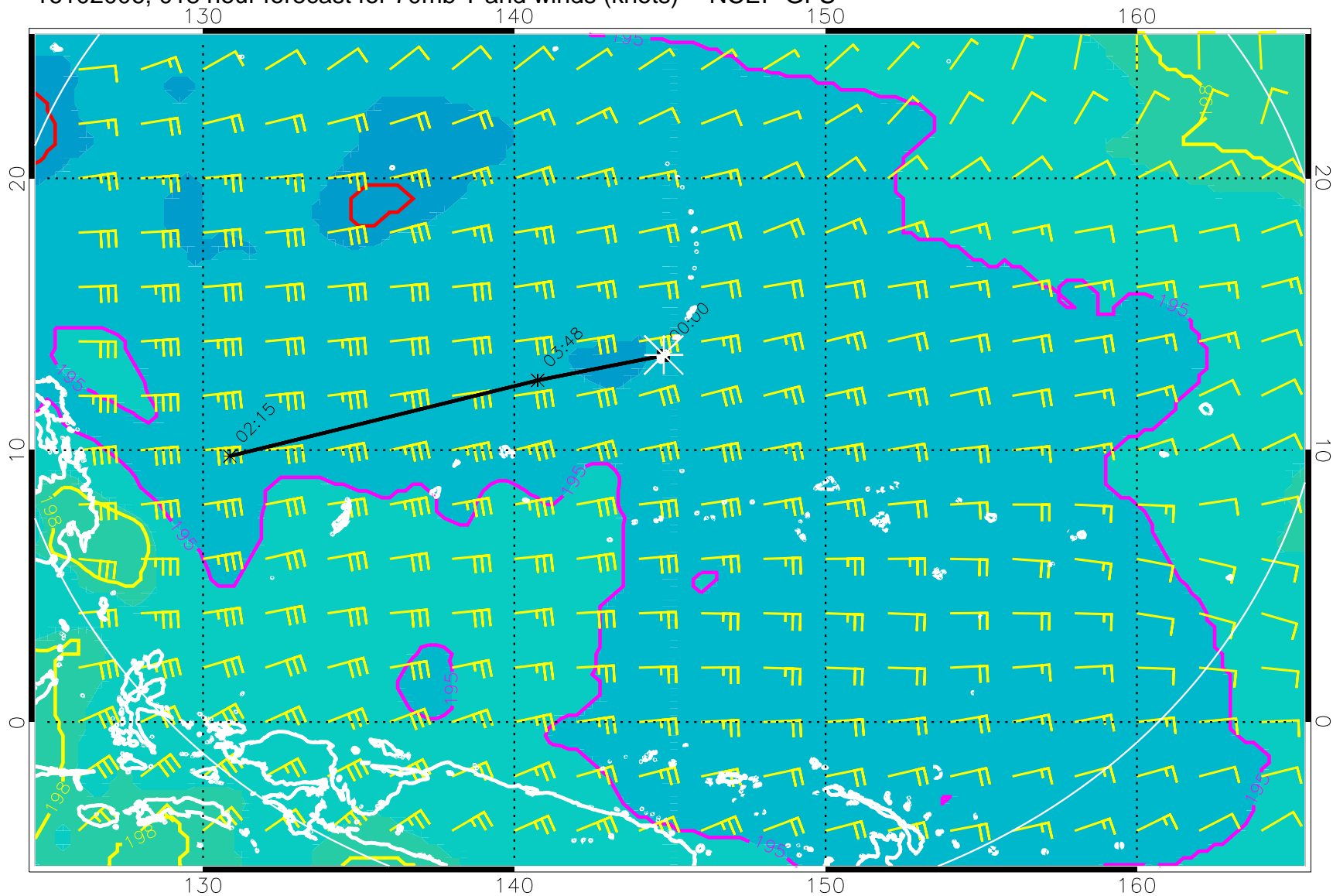
16102006, 018 hour forecast for 70mb T and winds (knots) -- NCEP GFS
