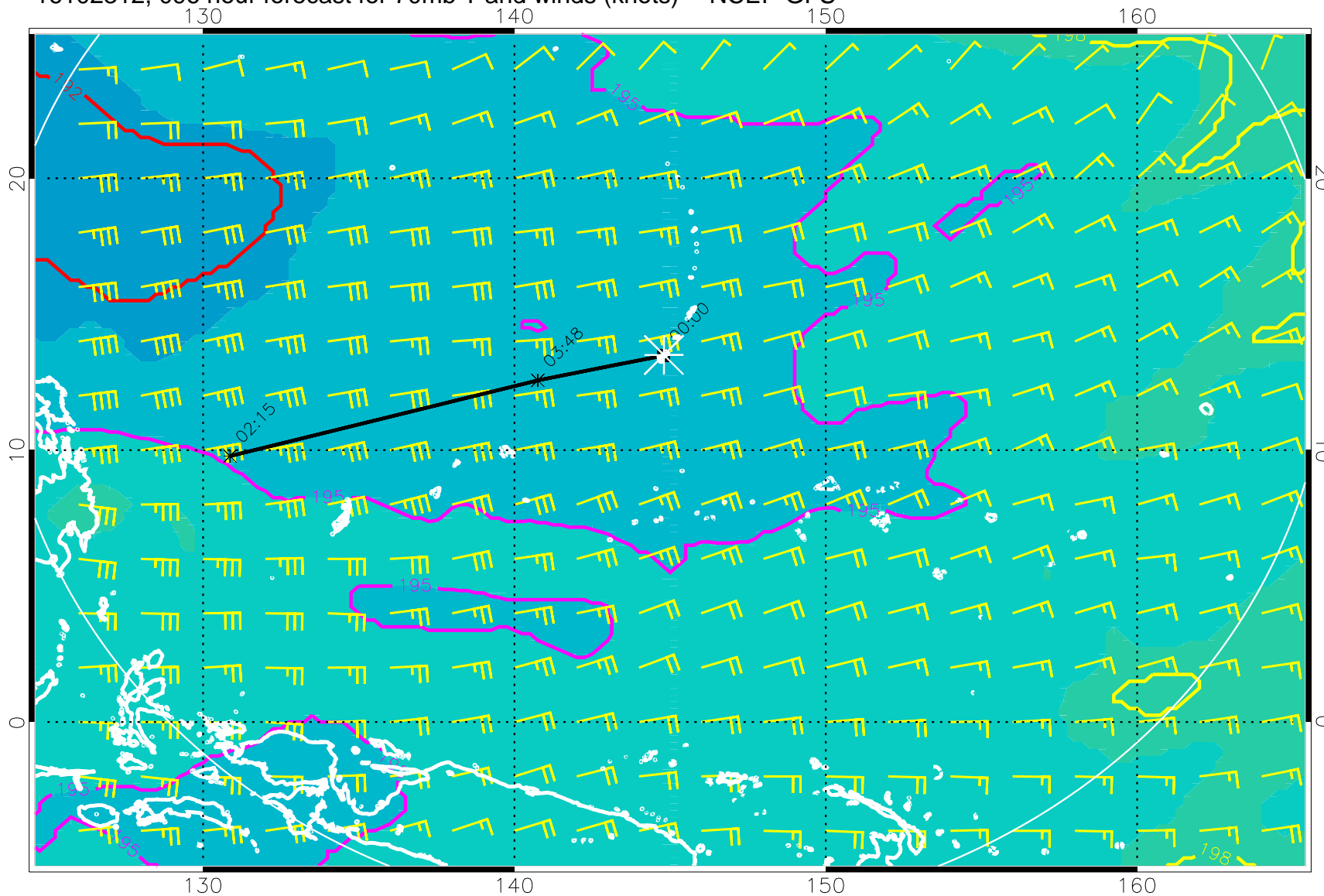
16102312, 096 hour forecast for 70mb T and winds (knots) -- NCEP GFS
