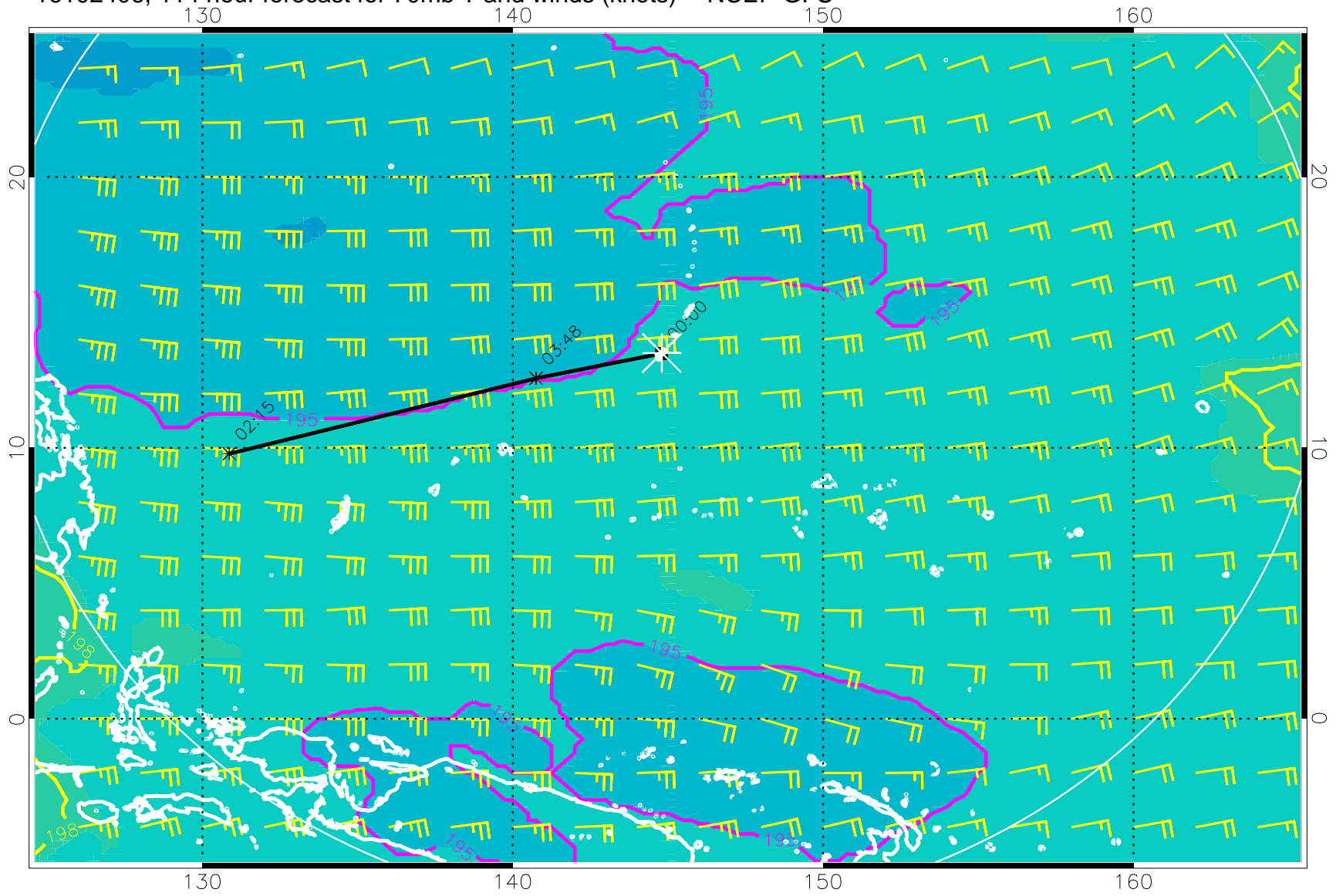
16102406, 114 hour forecast for 70mb T and winds (knots) -- NCEP GFS
