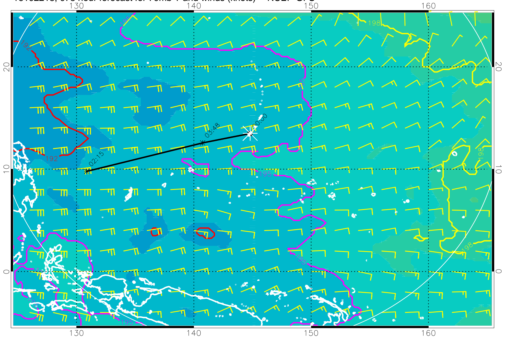
16102218, 078 hour forecast for 70mb T and winds (knots) -- NCEP GFS
