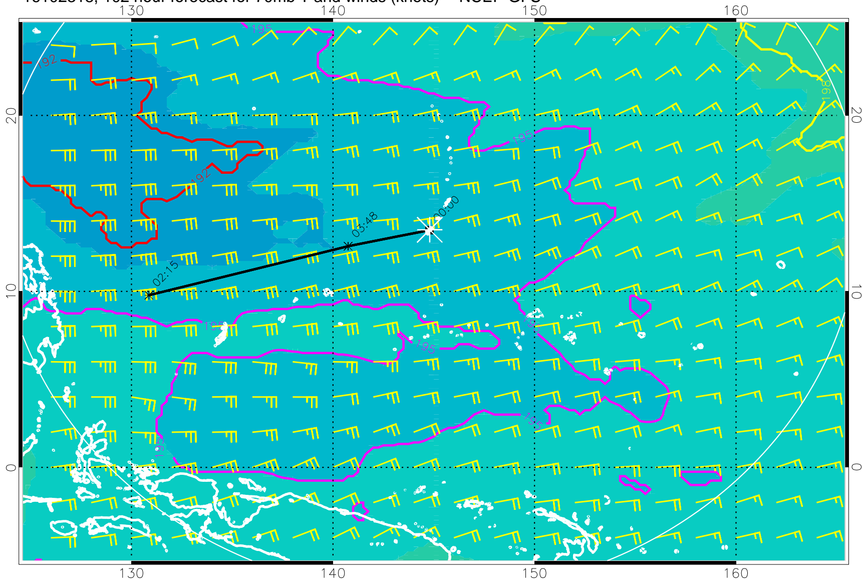
16102318, 102 hour forecast for 70mb T and winds (knots) -- NCEP GFS
