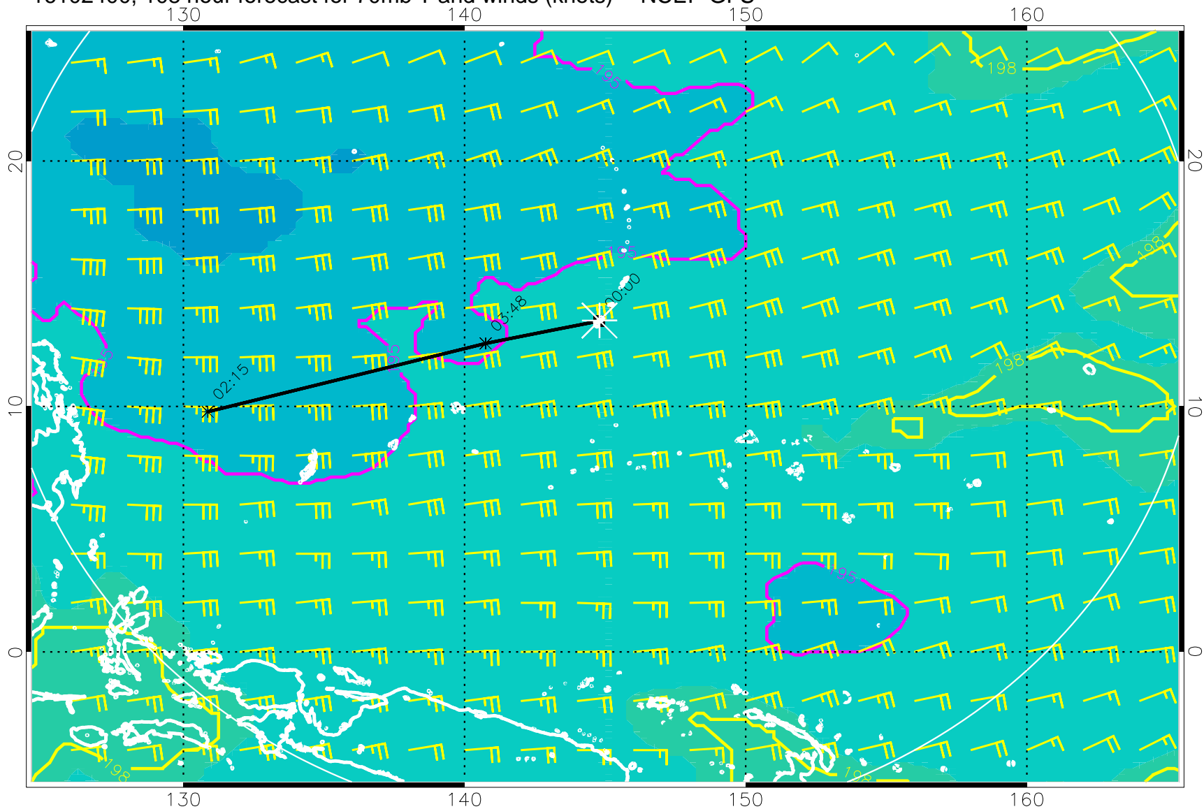
16102400, 108 hour forecast for 70mb T and winds (knots) -- NCEP GFS
