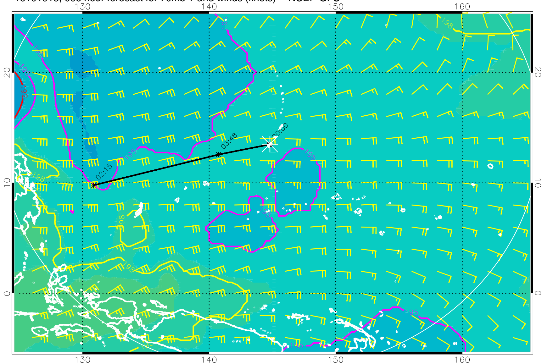
16101918, 006 hour forecast for 70mb T and winds (knots) -- NCEP GFS
