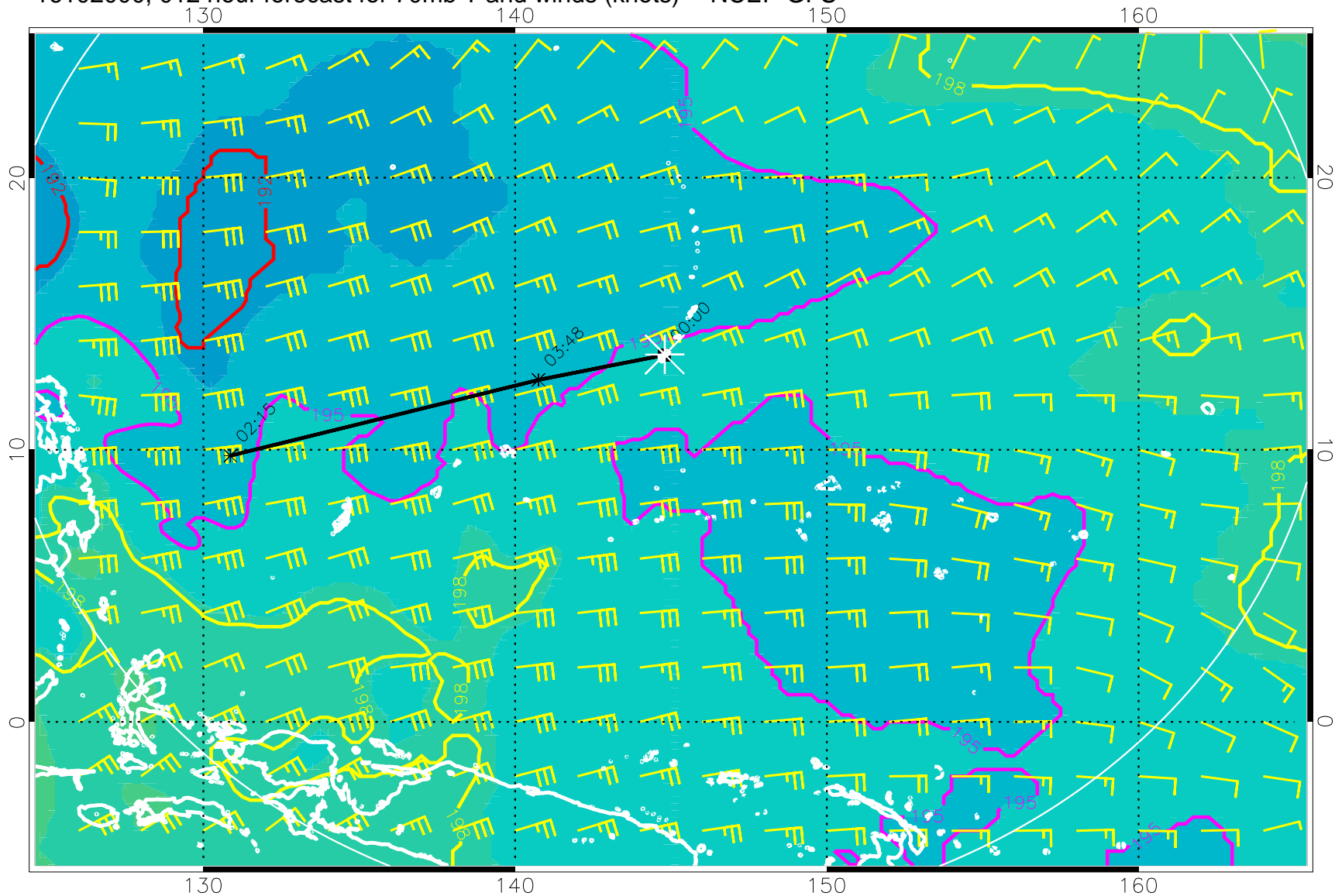
16102000, 012 hour forecast for 70mb T and winds (knots) -- NCEP GFS
