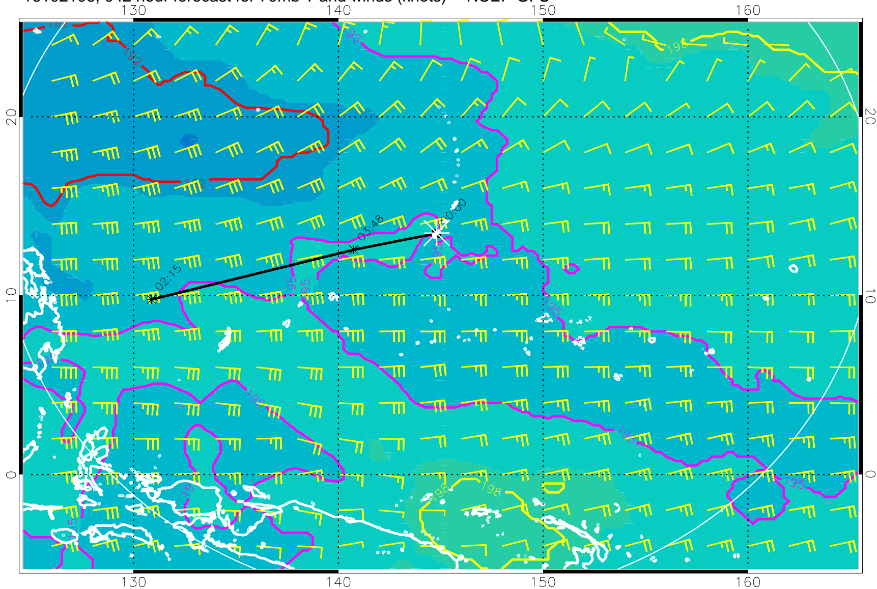
16102106, 042 hour forecast for 70mb T and winds (knots) -- NCEP GFS
