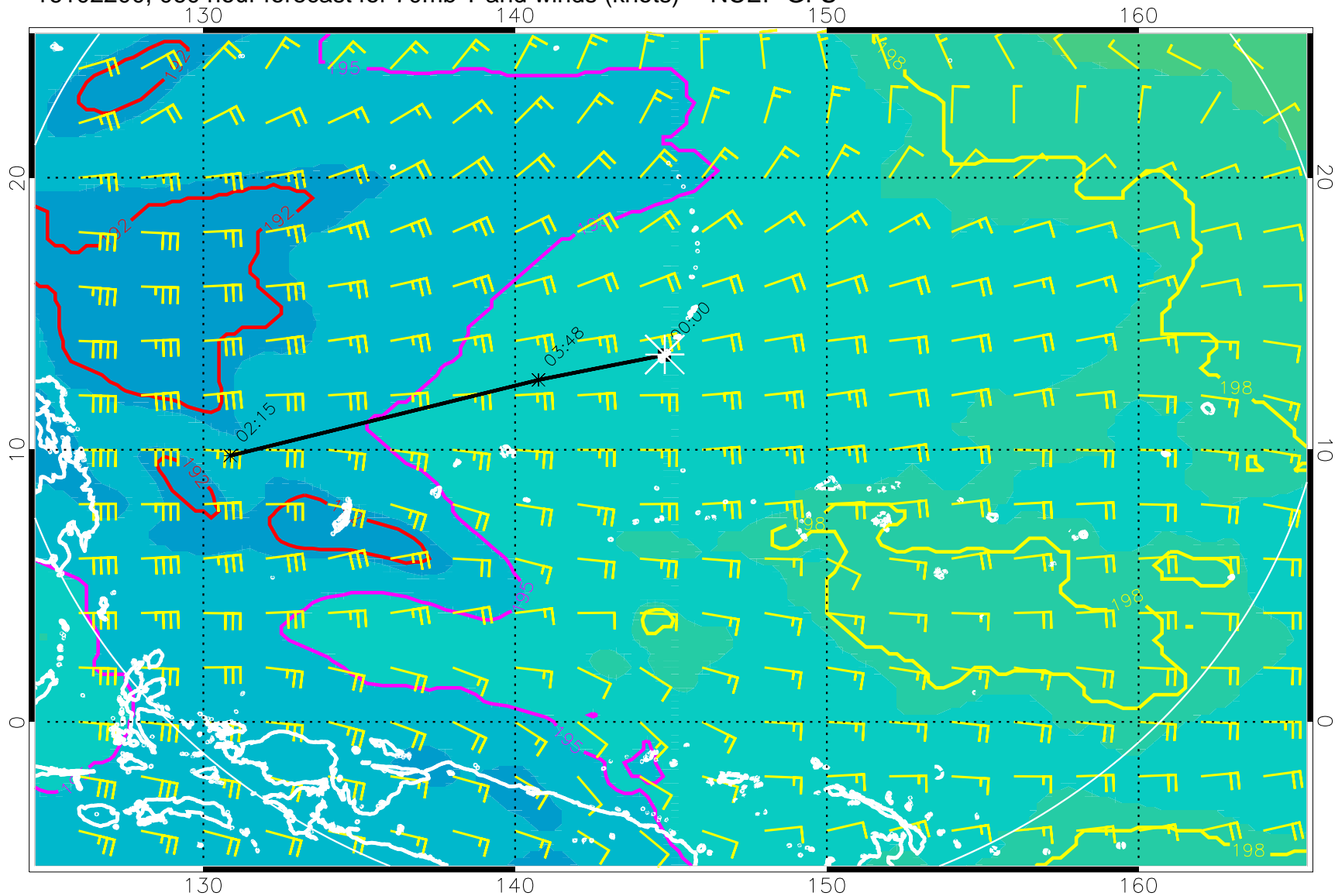
16102200, 060 hour forecast for 70mb T and winds (knots) -- NCEP GFS
