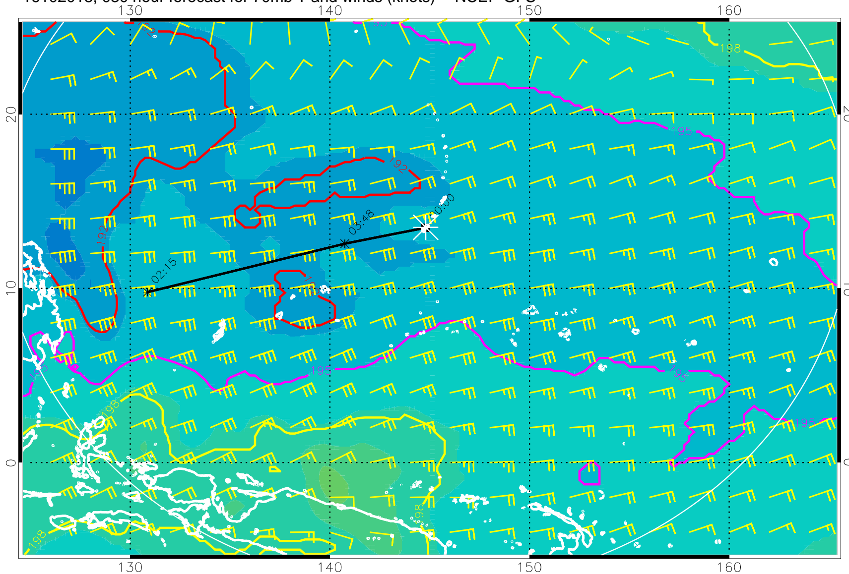
16102018, 030 hour forecast for 70mb T and winds (knots) -- NCEP GFS
