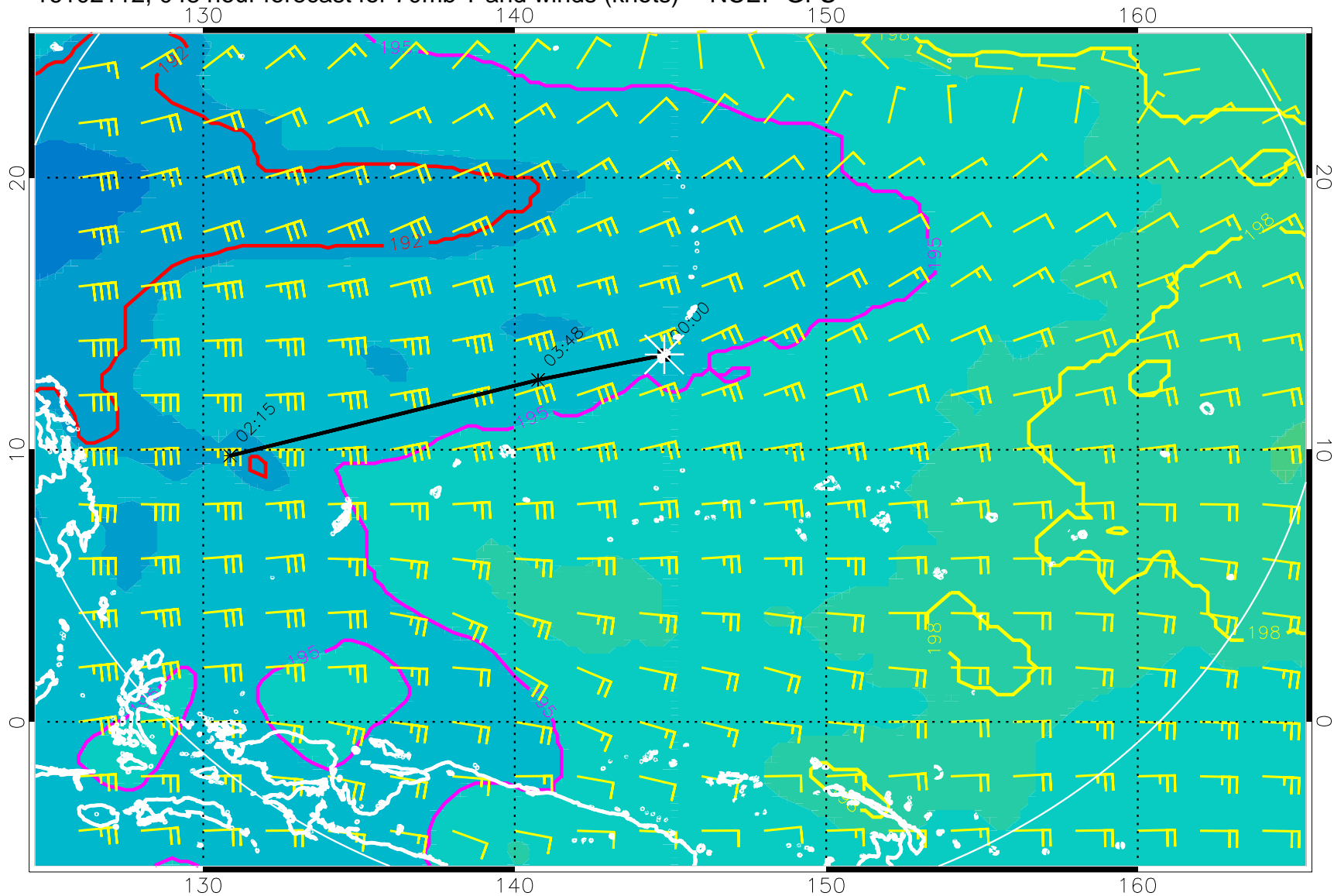
16102112, 048 hour forecast for 70mb T and winds (knots) -- NCEP GFS
