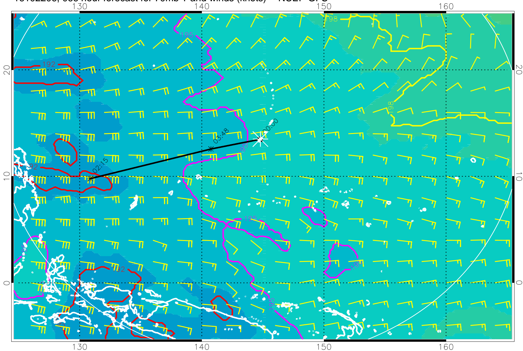
16102206, 066 hour forecast for 70mb T and winds (knots) -- NCEP GFS
