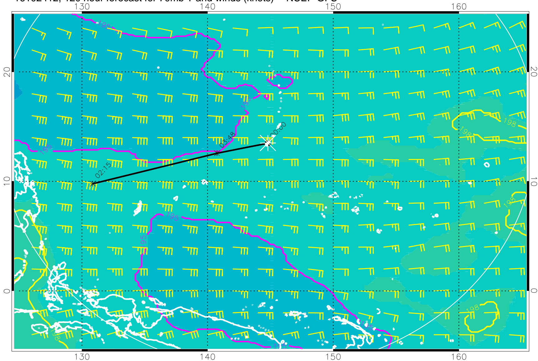
16102412, 120 hour forecast for 70mb T and winds (knots) -- NCEP GFS
