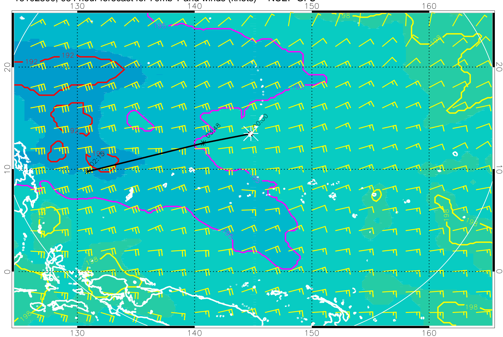
16102300, 084 hour forecast for 70mb T and winds (knots) -- NCEP GFS
