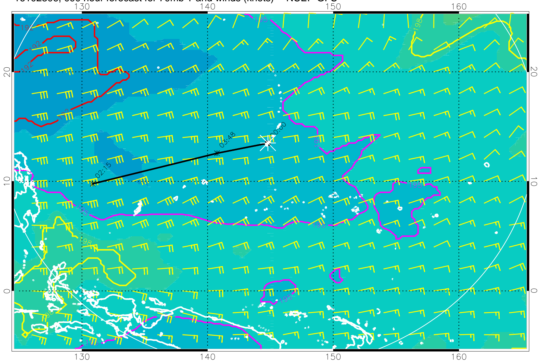
16102306, 090 hour forecast for 70mb T and winds (knots) -- NCEP GFS
