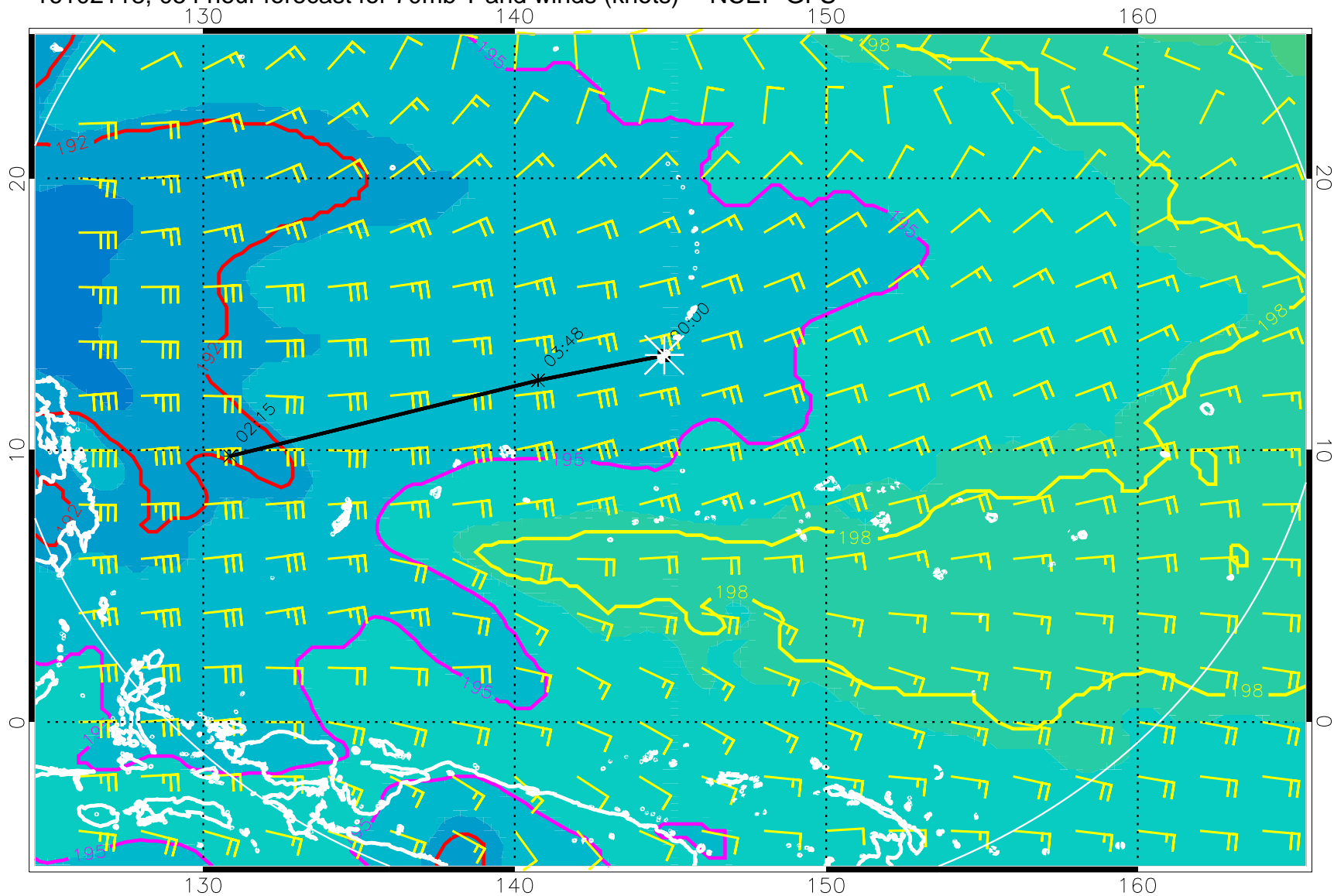
16102118, 054 hour forecast for 70mb T and winds (knots) -- NCEP GFS
