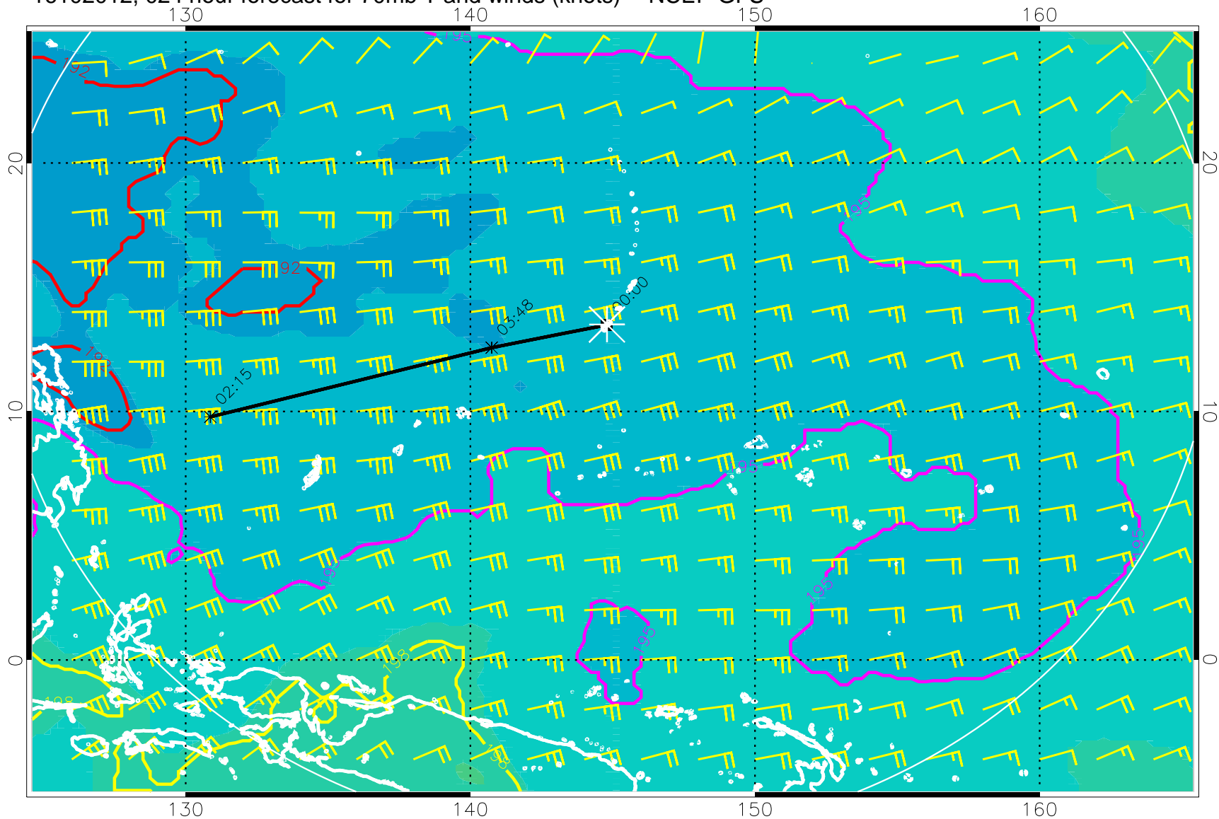
16102012, 024 hour forecast for 70mb T and winds (knots) -- NCEP GFS
