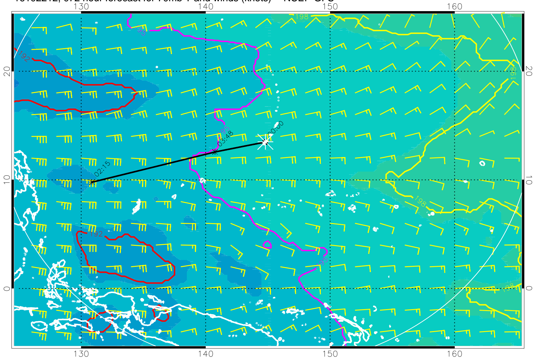
16102212, 072 hour forecast for 70mb T and winds (knots) -- NCEP GFS
