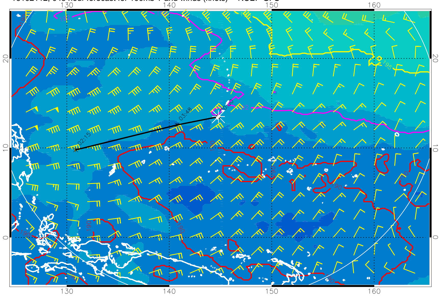
16102112, 048 hour forecast for 100mb T and winds (knots) -- NCEP GFS
