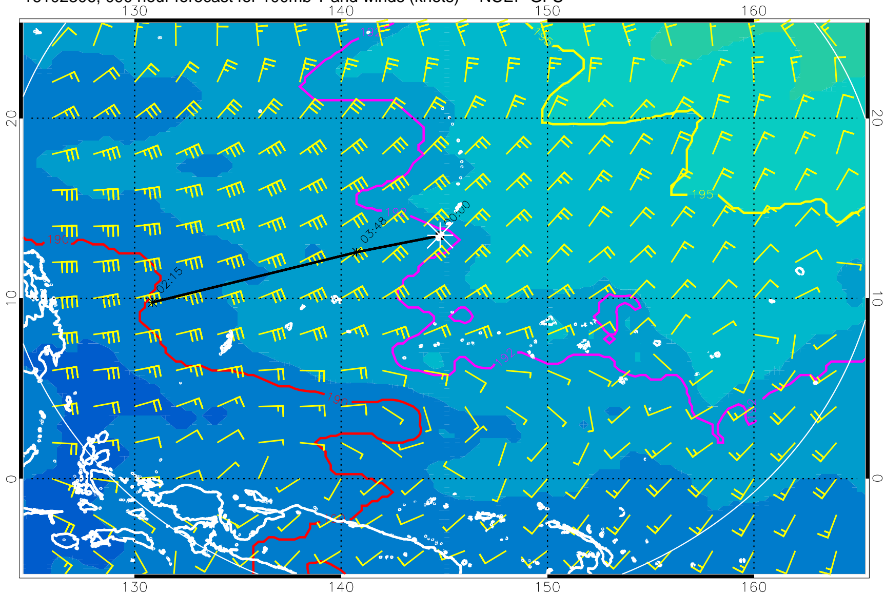
16102306, 090 hour forecast for 100mb T and winds (knots) -- NCEP GFS
