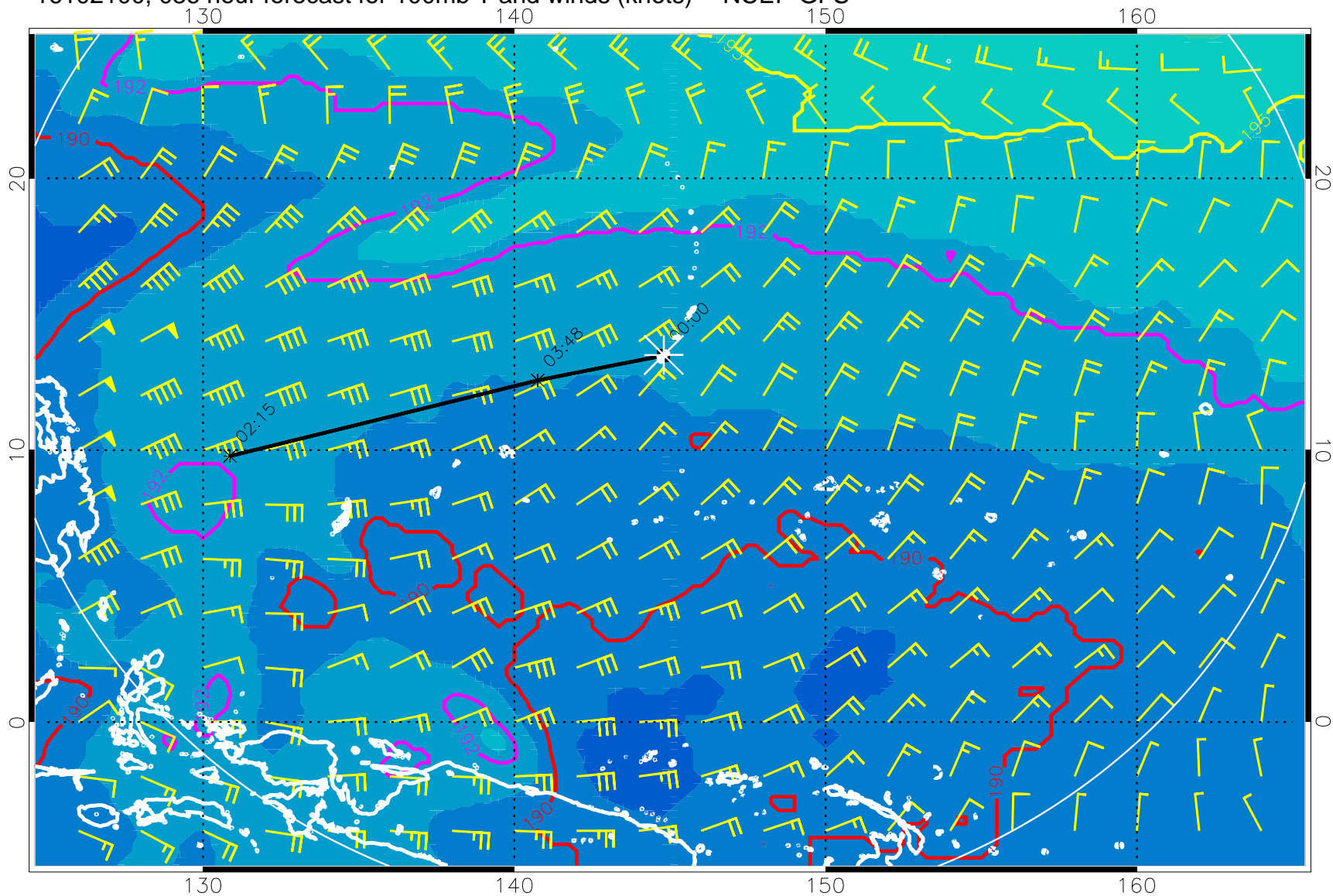
16102100, 036 hour forecast for 100mb T and winds (knots) -- NCEP GFS
