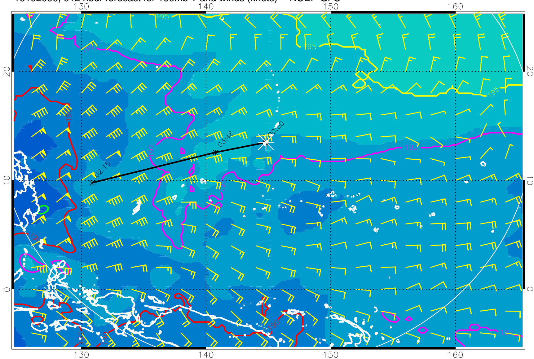
16102000, 012 hour forecast for 100mb T and winds (knots) -- NCEP GFS
