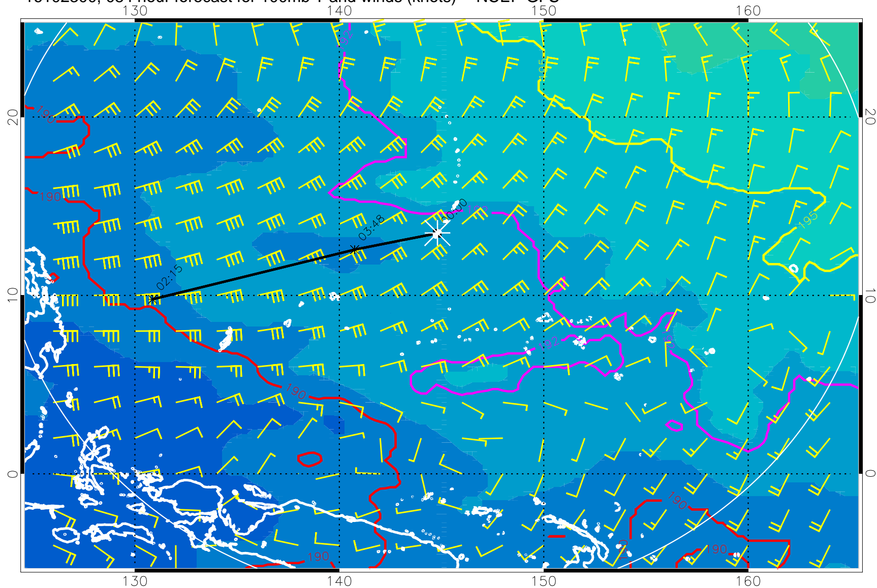
16102300, 084 hour forecast for 100mb T and winds (knots) -- NCEP GFS
