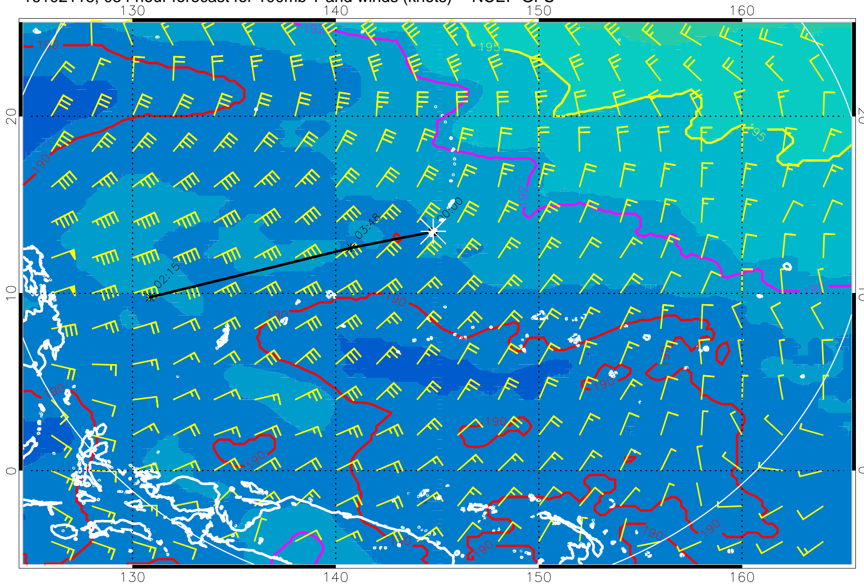
16102118, 054 hour forecast for 100mb T and winds (knots) -- NCEP GFS
