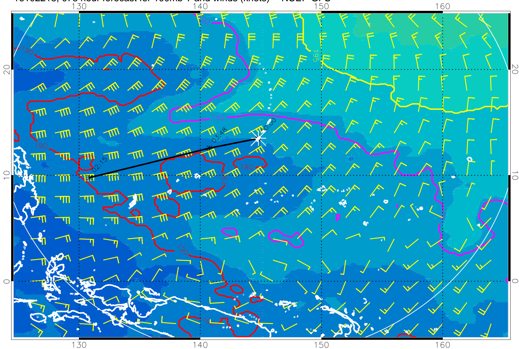
16102218, 078 hour forecast for 100mb T and winds (knots) -- NCEP GFS
