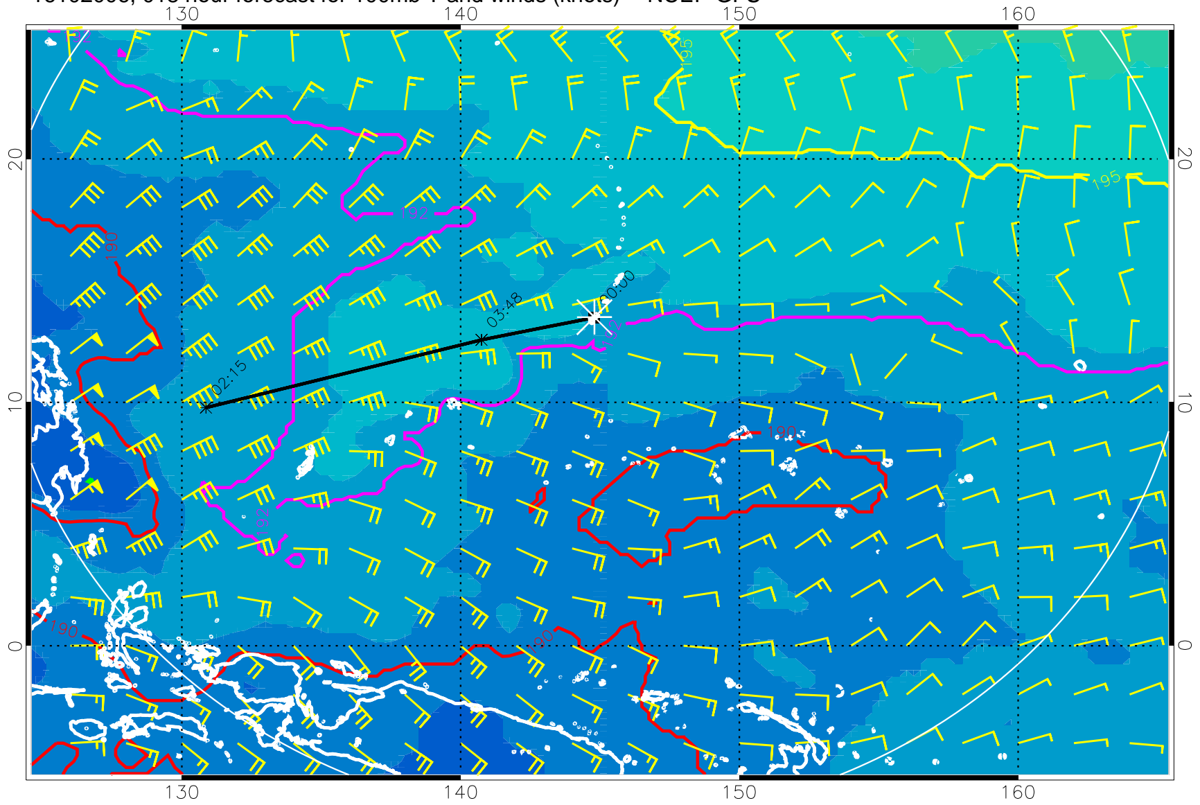
16102006, 018 hour forecast for 100mb T and winds (knots) -- NCEP GFS
