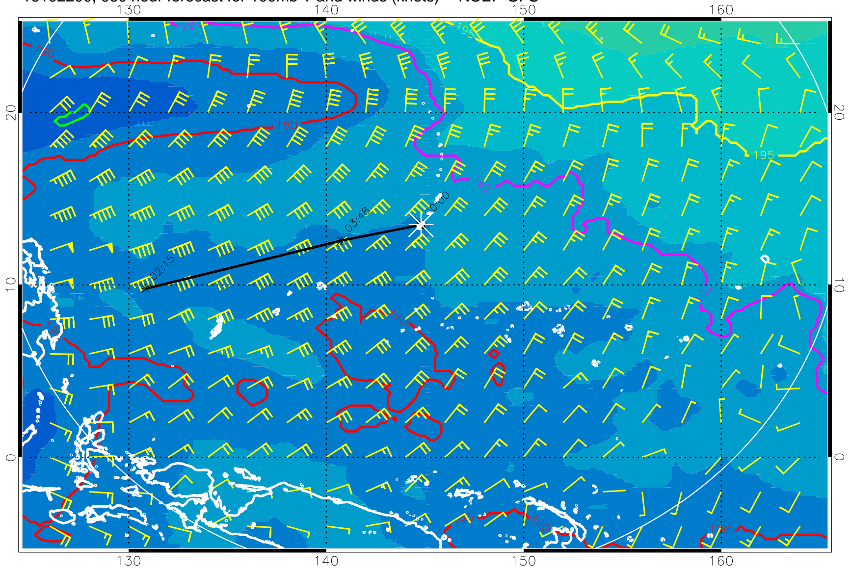
16102200, 060 hour forecast for 100mb T and winds (knots) -- NCEP GFS
