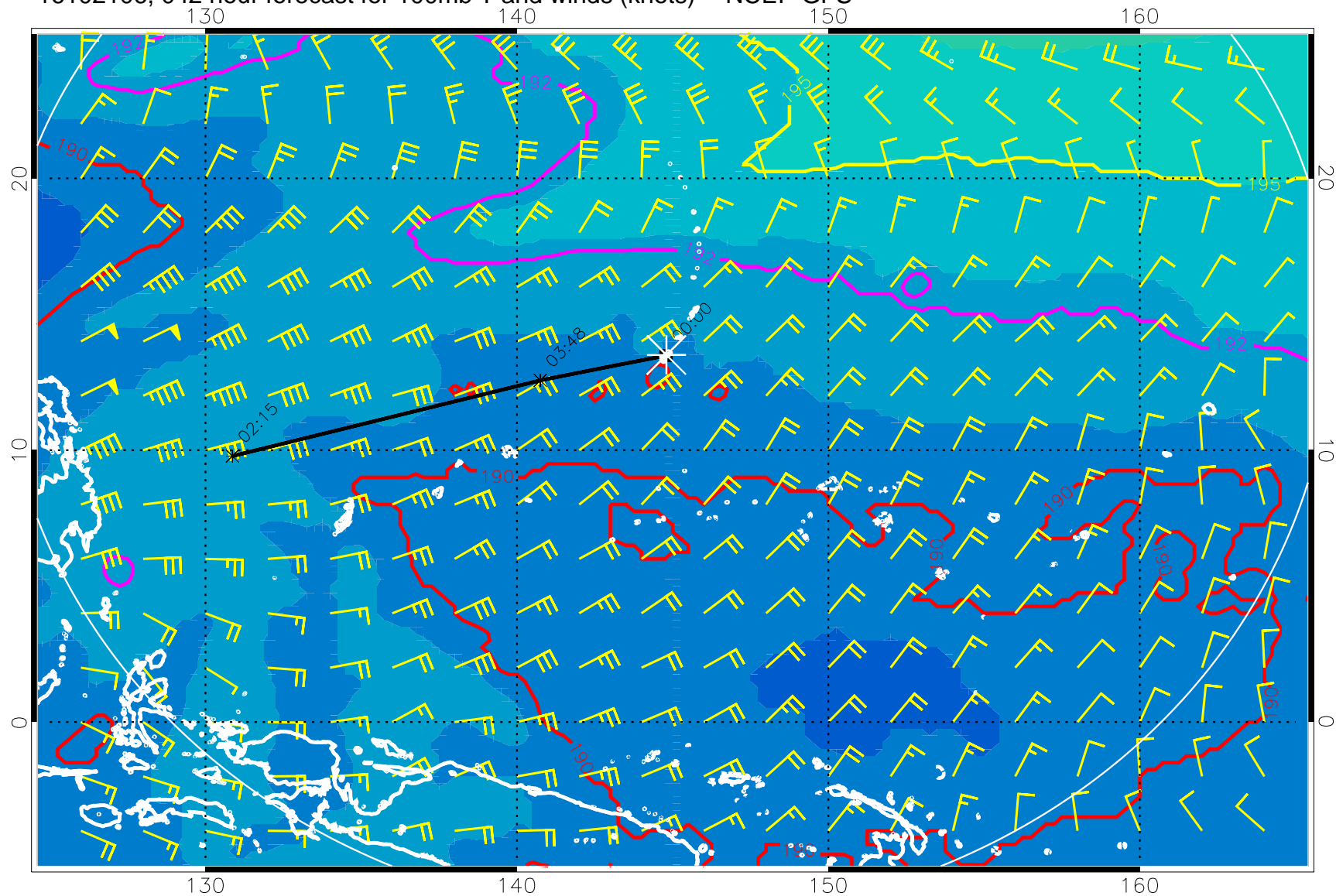
16102106, 042 hour forecast for 100mb T and winds (knots) -- NCEP GFS
