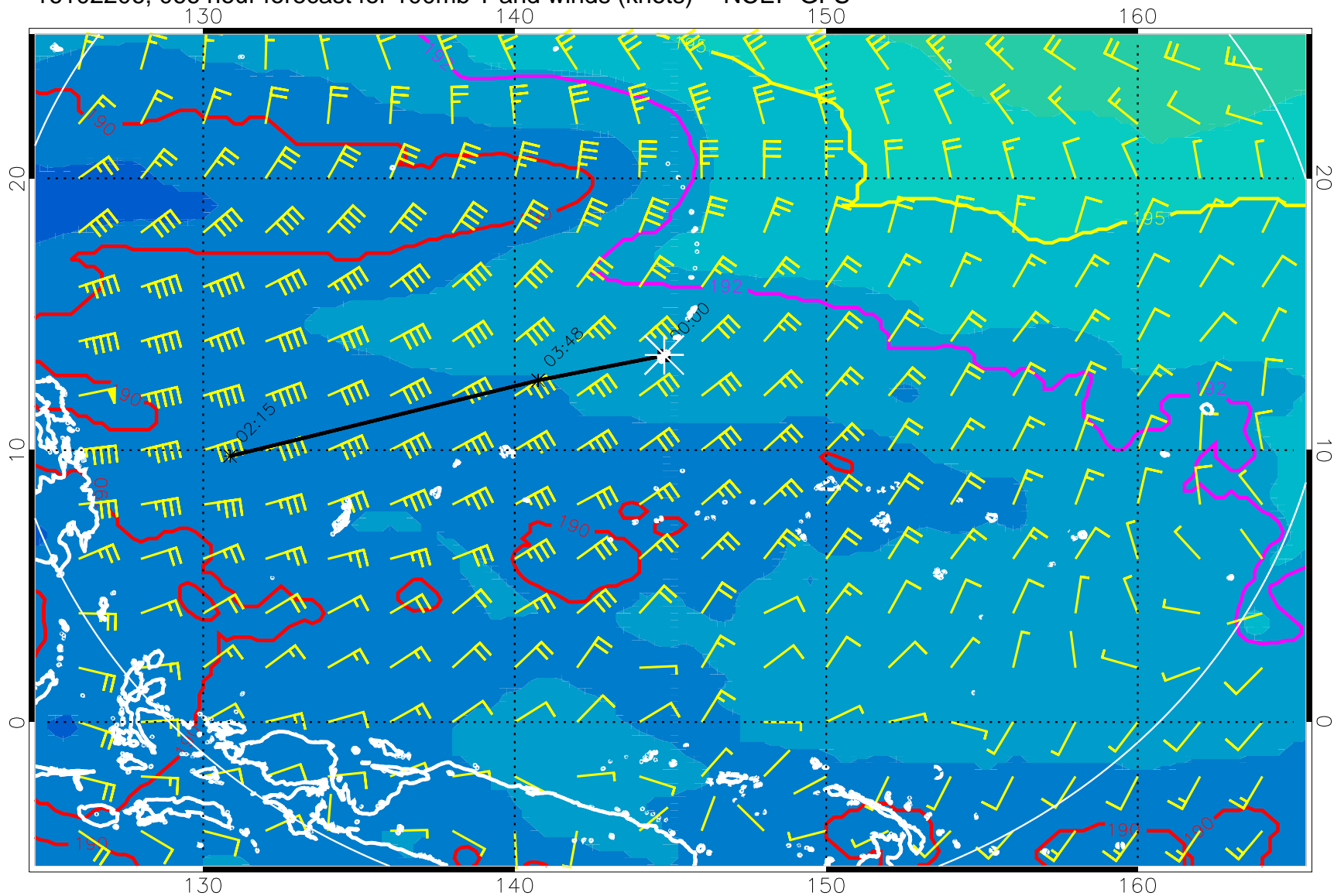
16102206, 066 hour forecast for 100mb T and winds (knots) -- NCEP GFS
