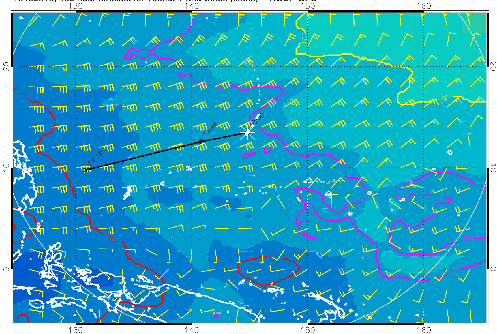
16102318, 102 hour forecast for 100mb T and winds (knots) -- NCEP GFS
