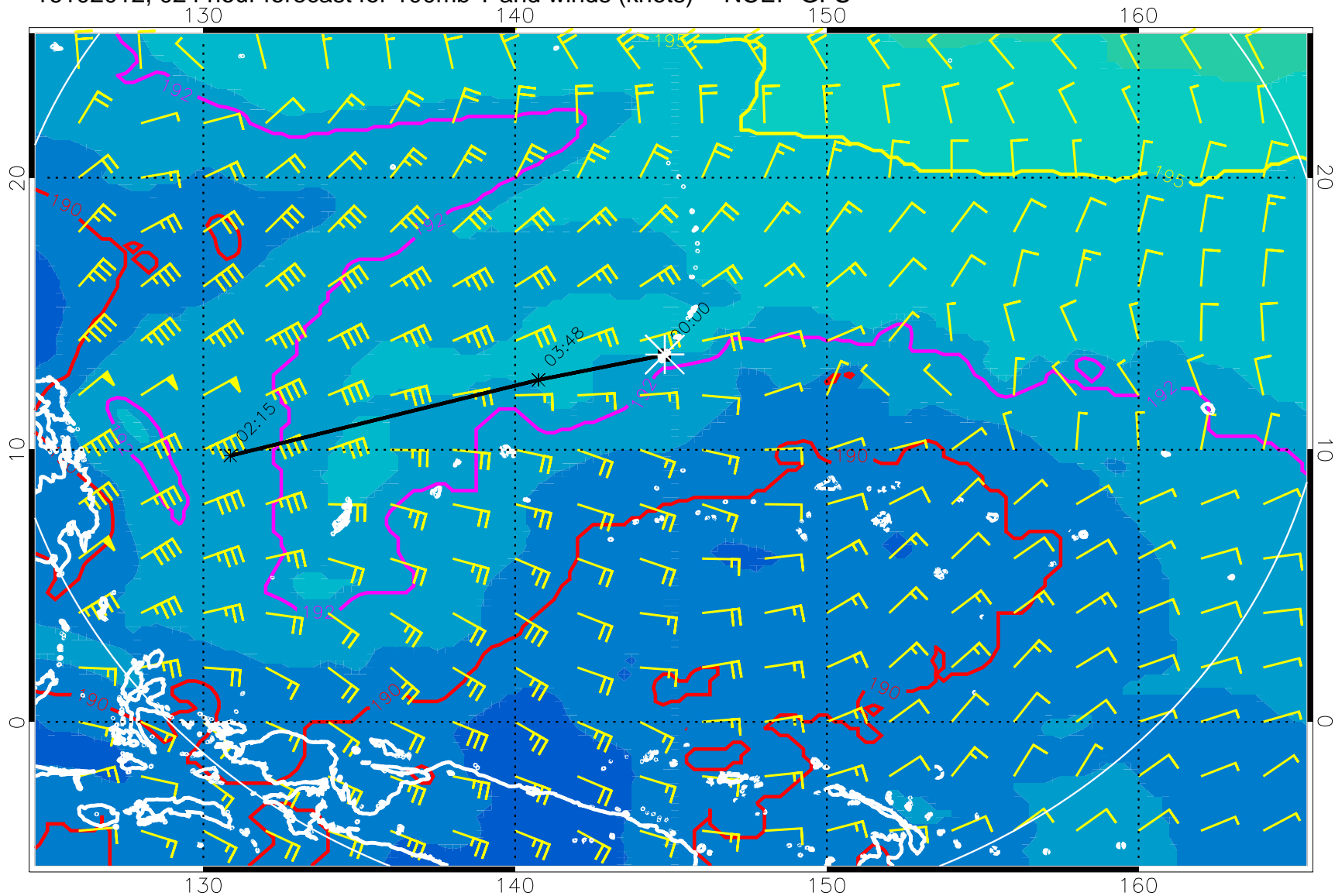
16102012, 024 hour forecast for 100mb T and winds (knots) -- NCEP GFS
