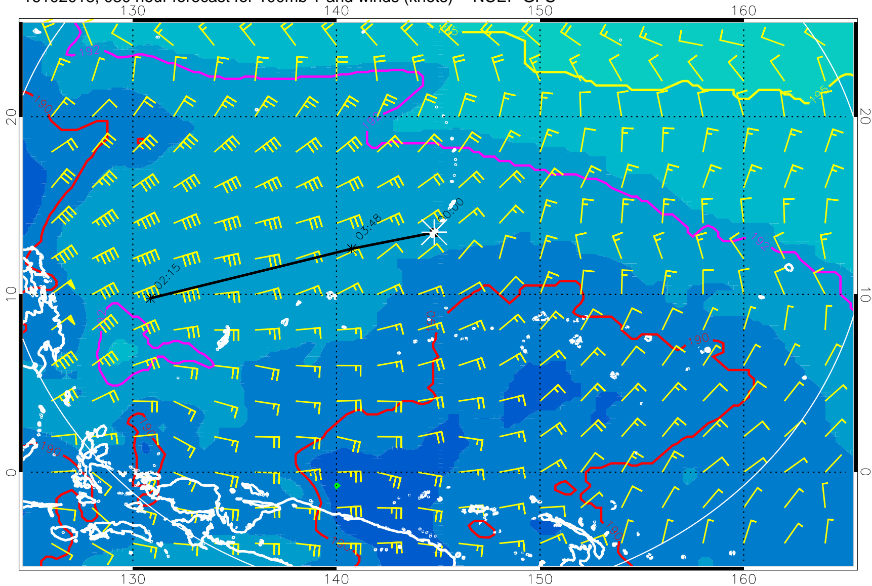
16102018, 030 hour forecast for 100mb T and winds (knots) -- NCEP GFS
