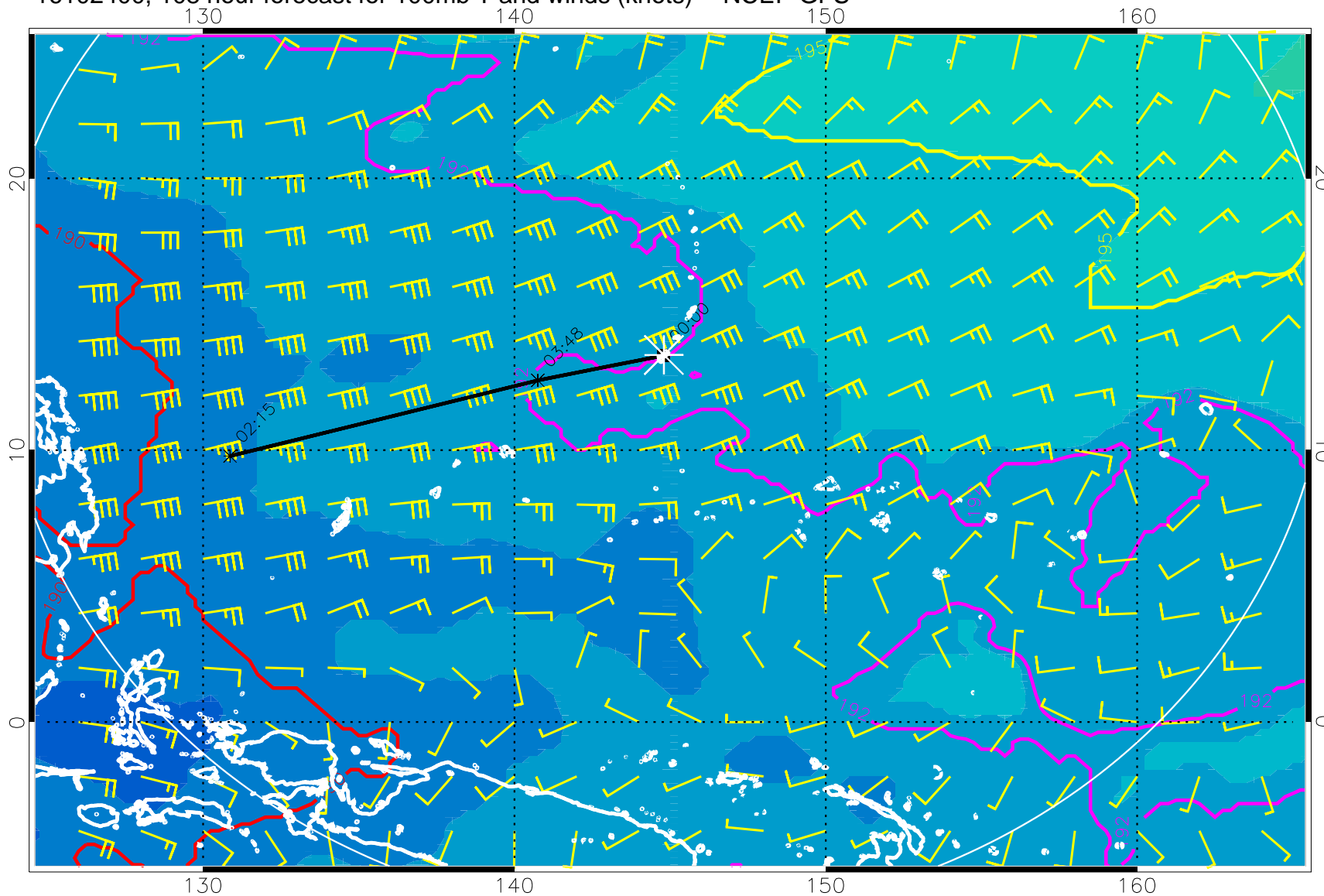
16102400, 108 hour forecast for 100mb T and winds (knots) -- NCEP GFS
