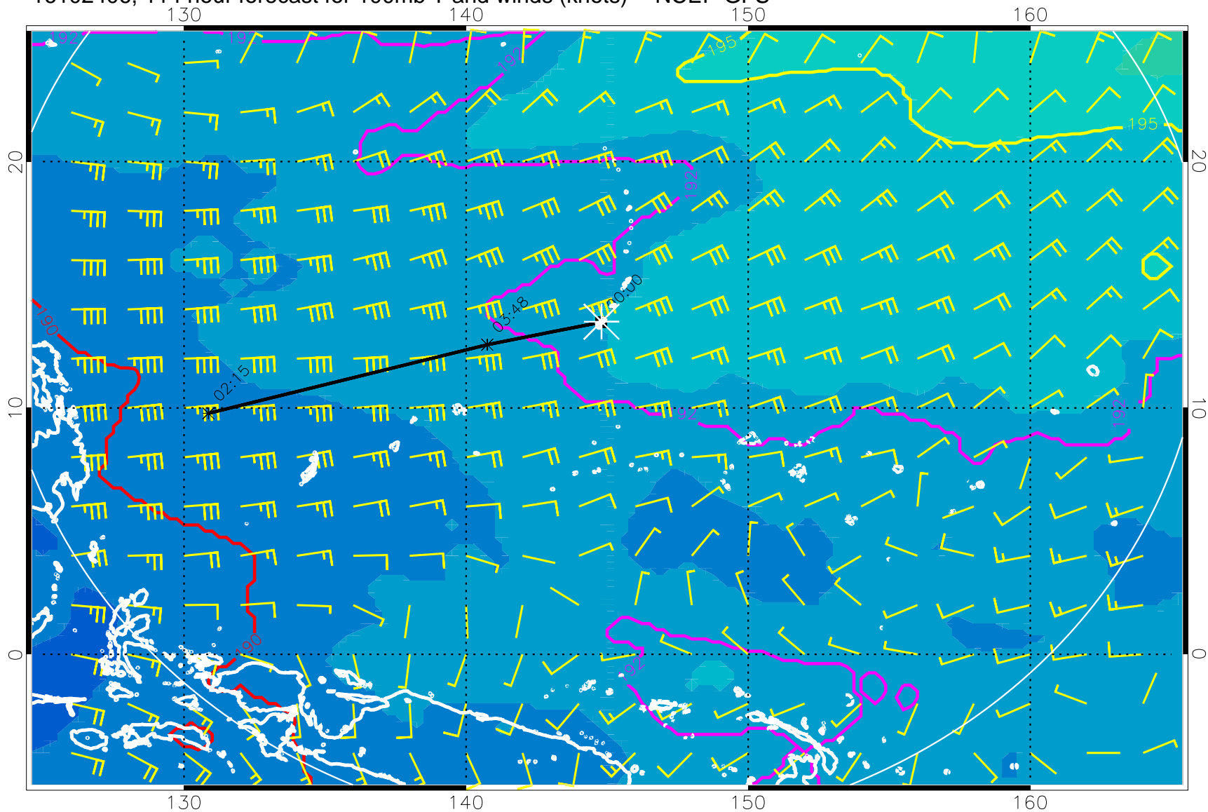
16102406, 114 hour forecast for 100mb T and winds (knots) -- NCEP GFS
