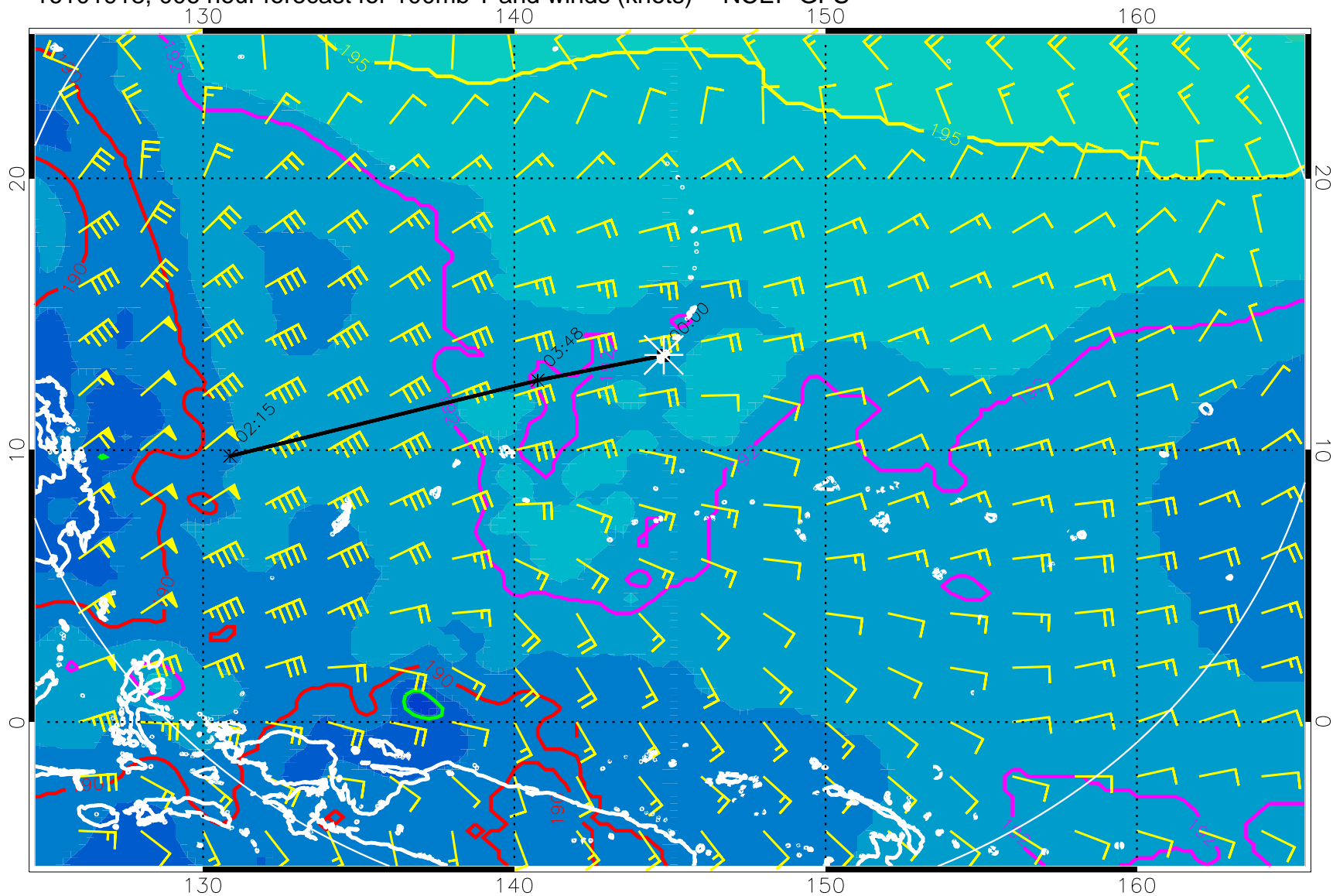
16101918, 006 hour forecast for 100mb T and winds (knots) -- NCEP GFS
