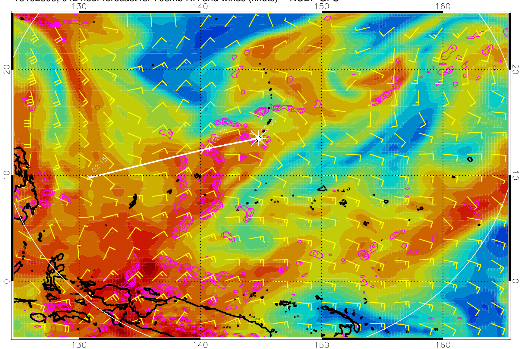
16102000, 012 hour forecast for 700mb RH and winds (knots) -- NCEP GFS
