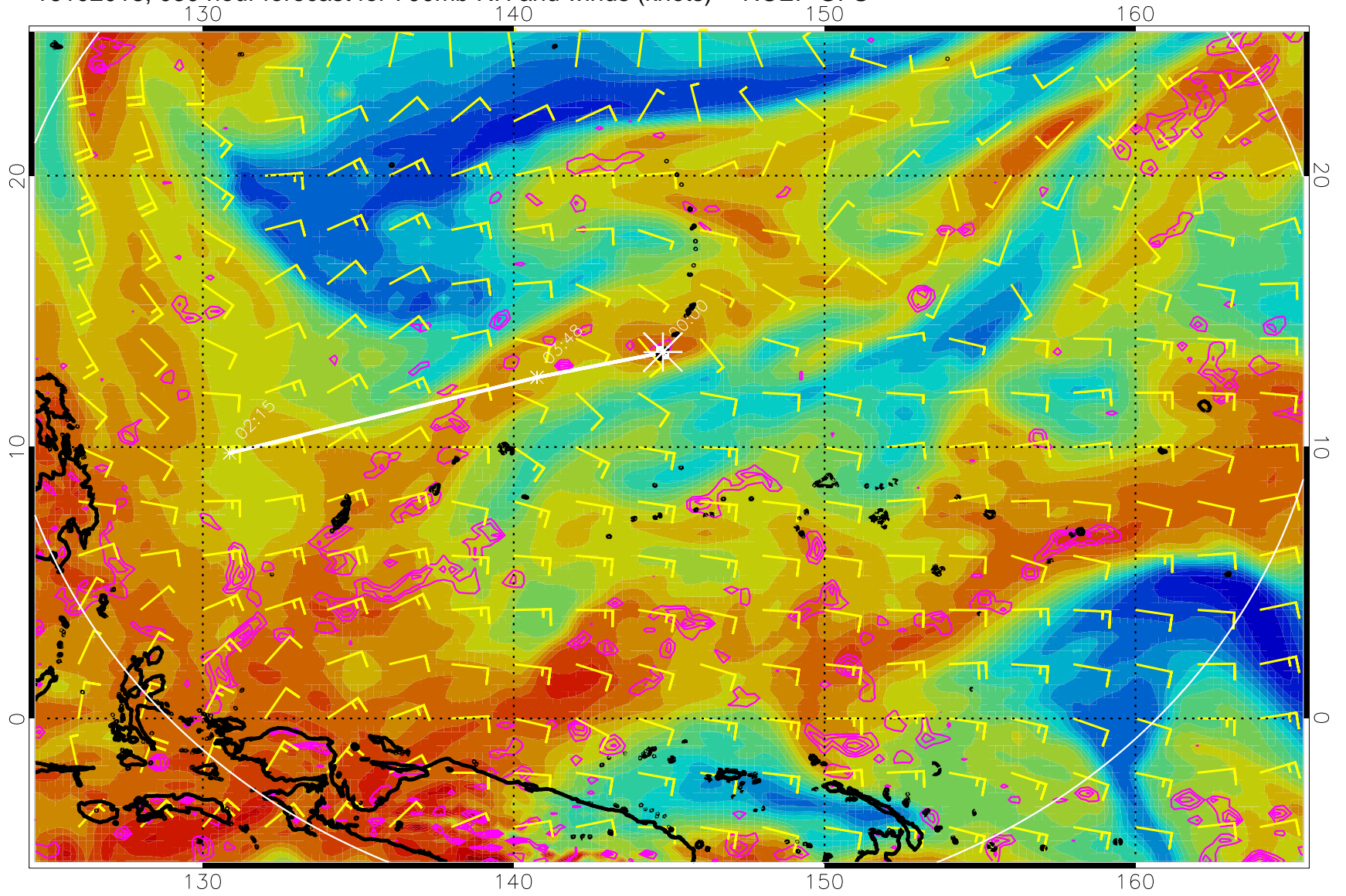
16102018, 030 hour forecast for 700mb RH and winds (knots) -- NCEP GFS
