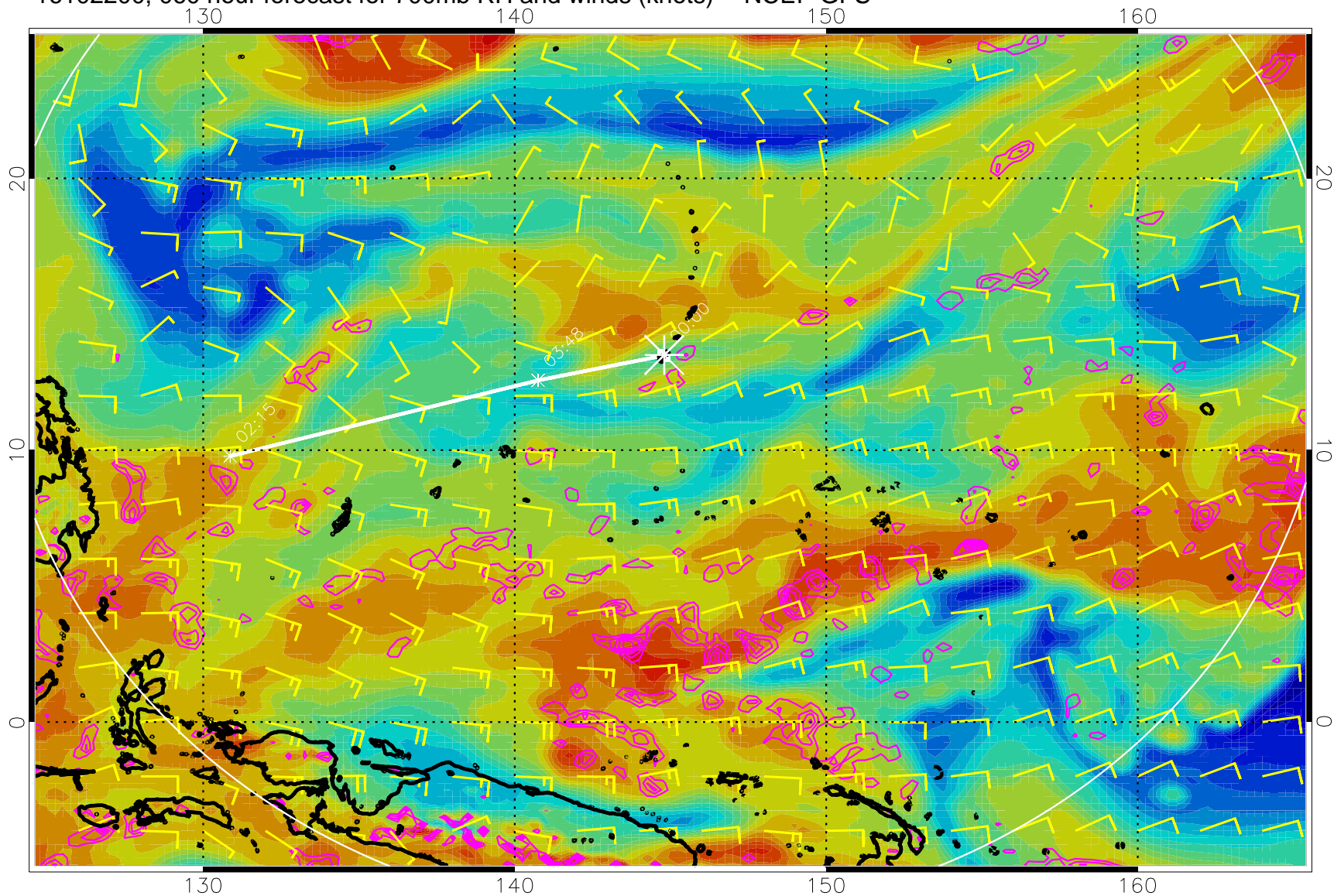
16102200, 060 hour forecast for 700mb RH and winds (knots) -- NCEP GFS
